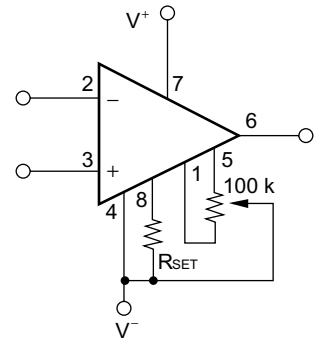
OFFSET VOLTAGE NULL CIRCUIT
