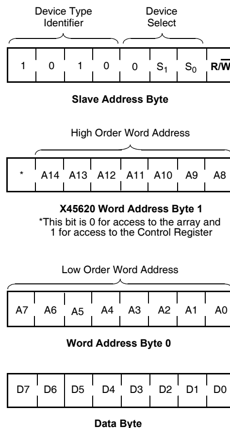
Figure 10. Device Addressing
