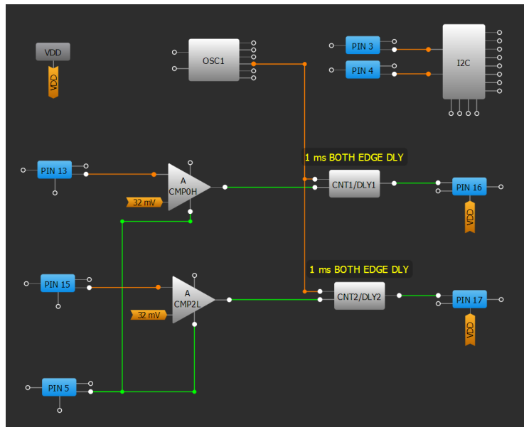
Figure 2: Testing Diagram
