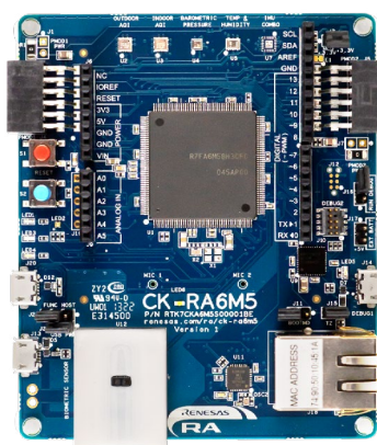
CK-RA6M5
