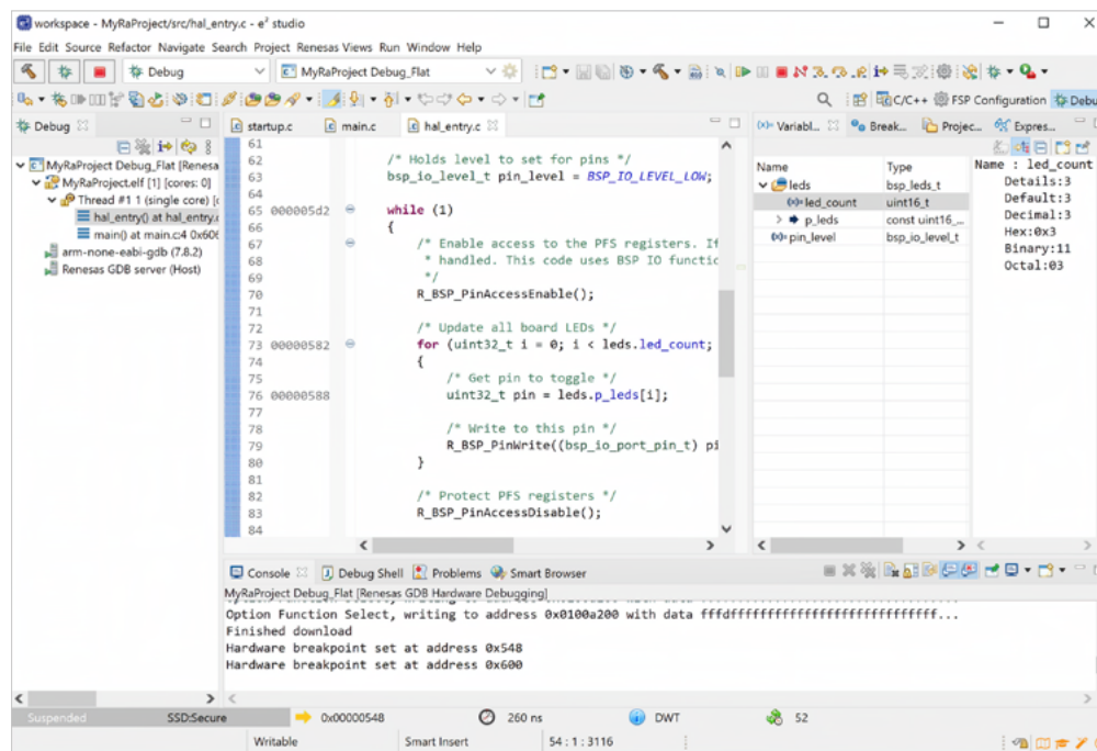
Figure 7-4: The Debug perspective of e 2 studio
