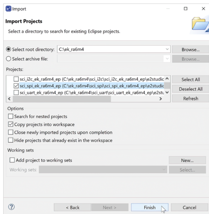
Figure 5-5: The projects found at a given location are listed for import
