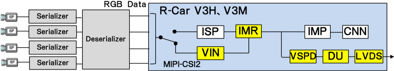
Fig.4 Connect four cameras with Serializer and Deserializer .
