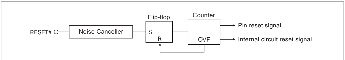
Figure 7.2.1 Reset Circuit
