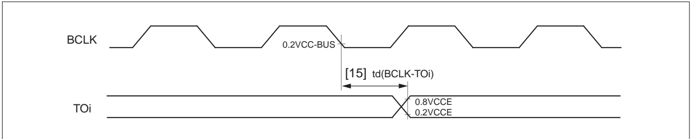
Figure 21.7.4 TOi Timing
