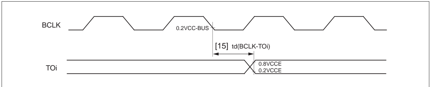
Figure 21.8.4 TOi Timing
