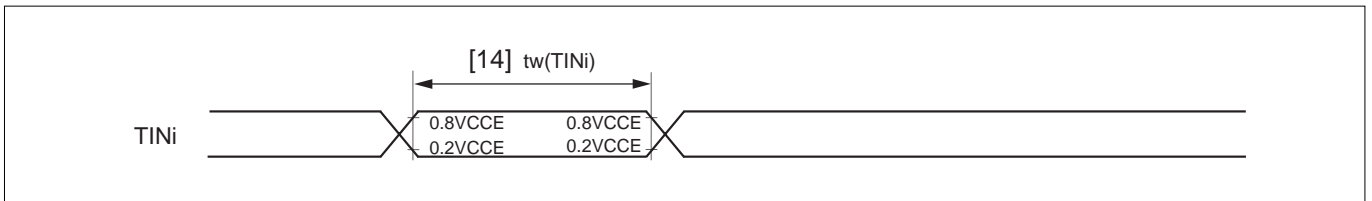
Figure 21.7.5 TINi Timing
