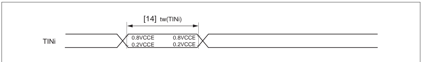
Figure 21.8.5 TINi Timing
