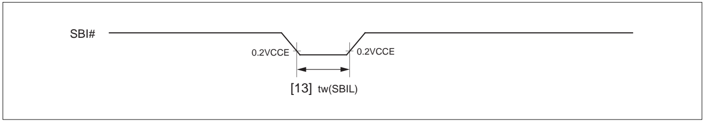
Figure 21.8.3 SBI Timing
