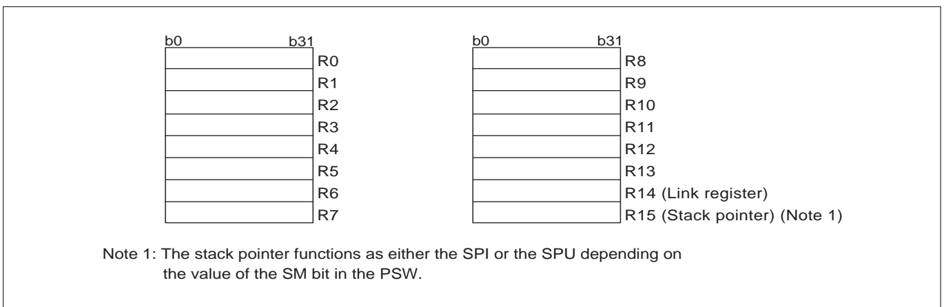
Figure 2.2.1 General-purpose Registers
