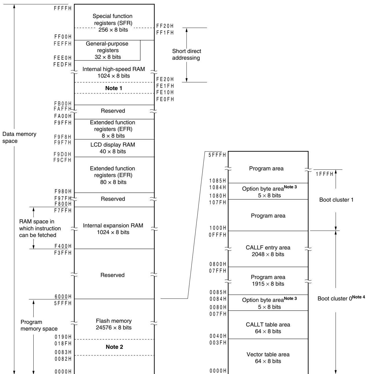
Figure 3-1. Memory Map ( \mu PD78F0836, 78F0838, 78F0840, 78F0842)
