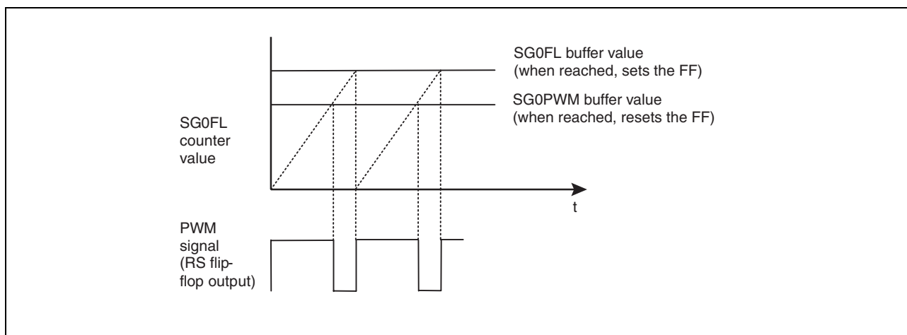
Figure 18-5. PWM Signal Generation
