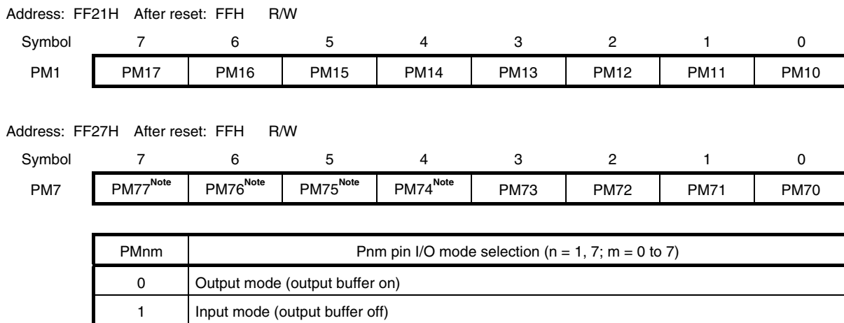
Figure 12-20. Format of Port Mode Registers 1 and 7 (PM1, PM7)
