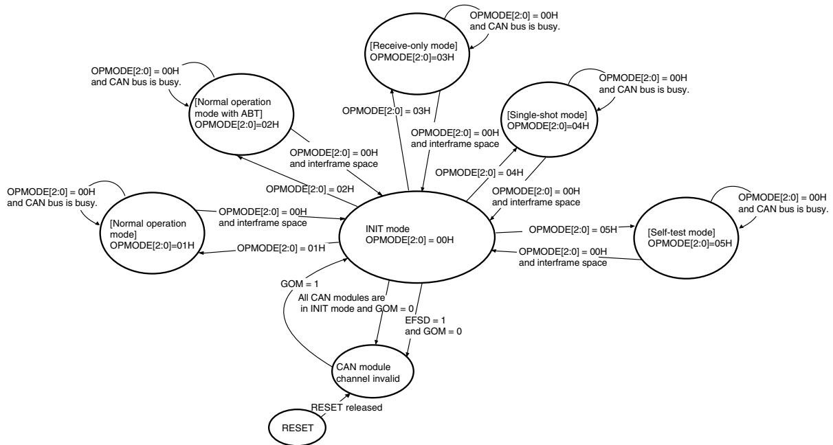
Figure 15-28. Transition to Operation Modes
