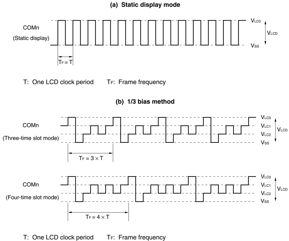
Figure 17-9. Common Signal Waveforms
