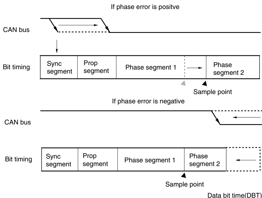
Figure 15-21. Resynchronization
