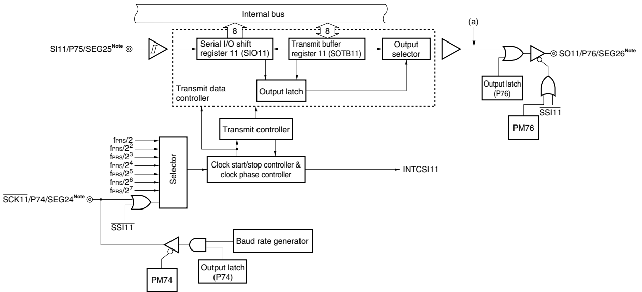
Figure 13-2. Block Diagram of Serial Interface CSI11
