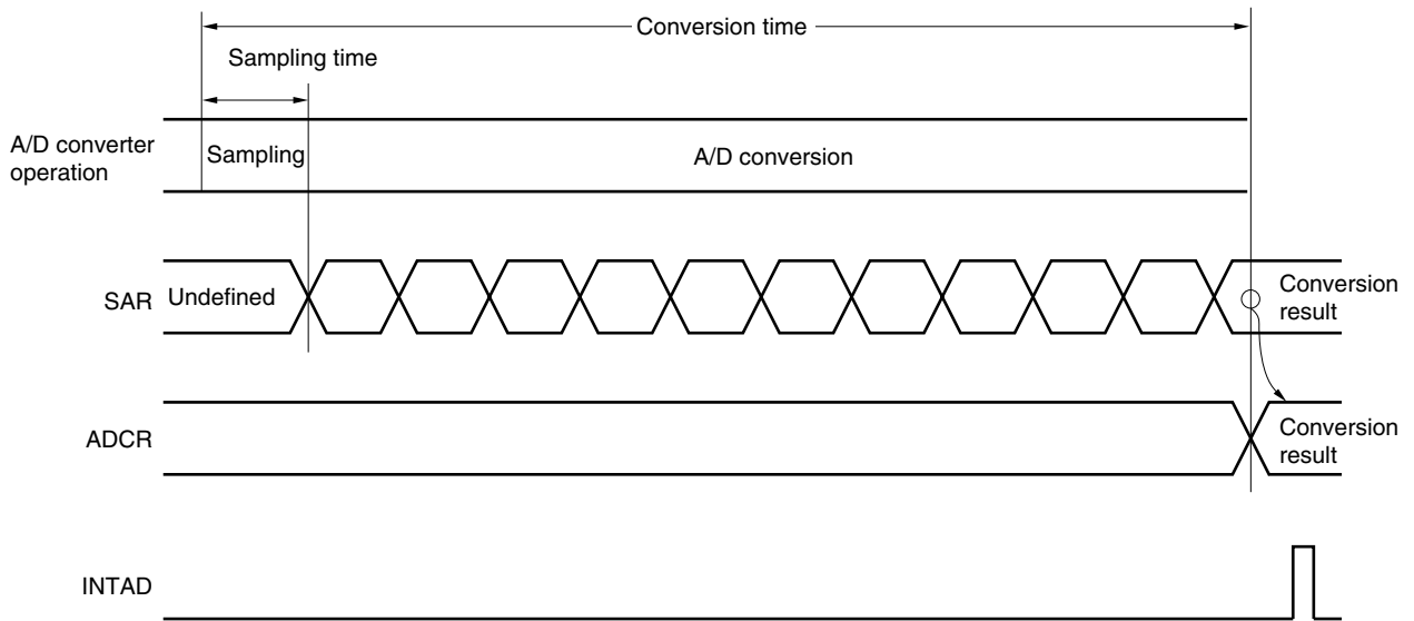
Figure 11-11. Basic Operation of A/D Converter
