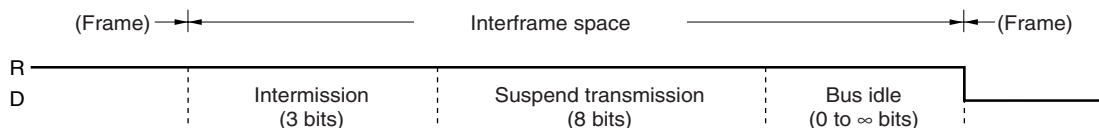
Figure 15-14. Interframe Space (Error Passive Node)
