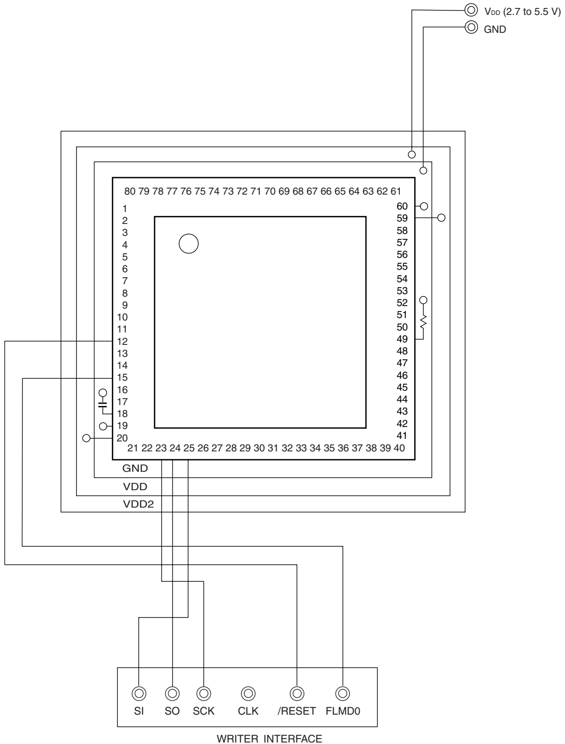
Figure 26-3. Example of Wiring Adapter for Flash Memory Writing in 3-Wire Serial I/O (CS110) Mode
