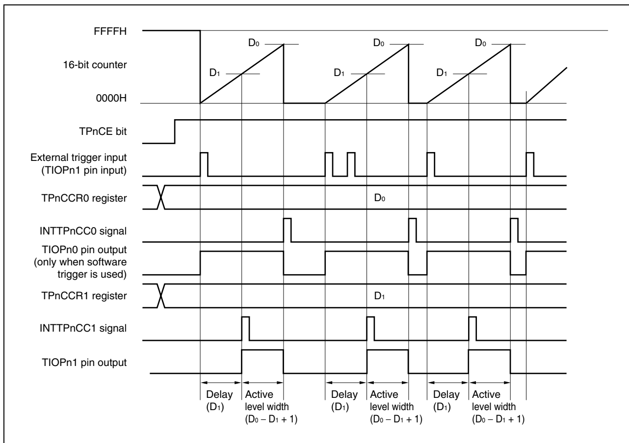
Figure 6-24. Basic Timing in One-shot Pulse Output Mode
