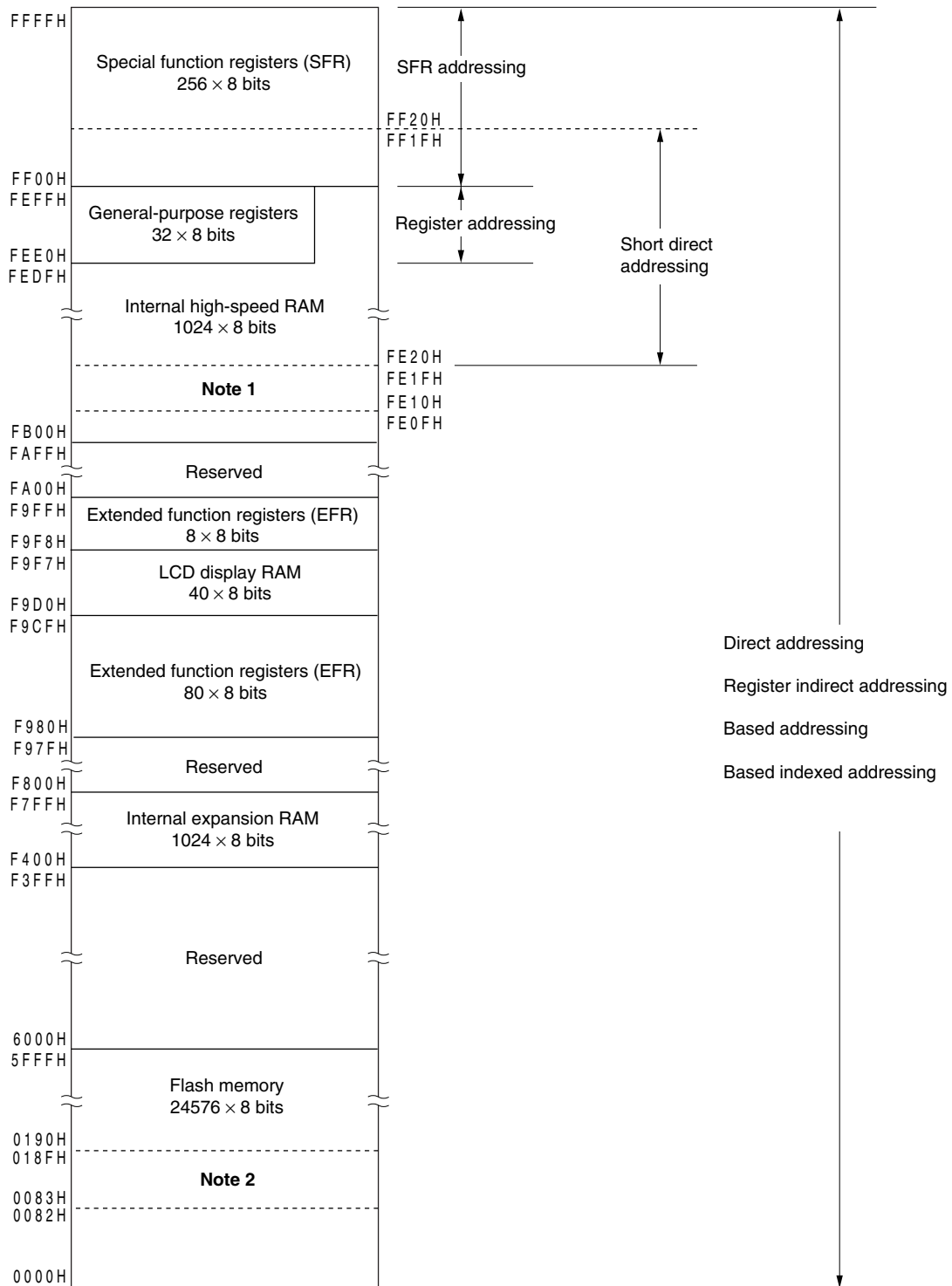
Figure 3-5. Correspondence between Data Memory and Addressing ( \mu PD78F0836, 78F0838, 78F0840, 78F0842)
