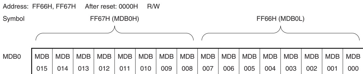
Figure 22-4. Format of Multiplication/Division Data Register B0 (MDB0)
