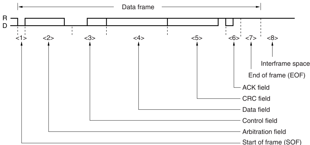
Figure 15-3. Data Frame
