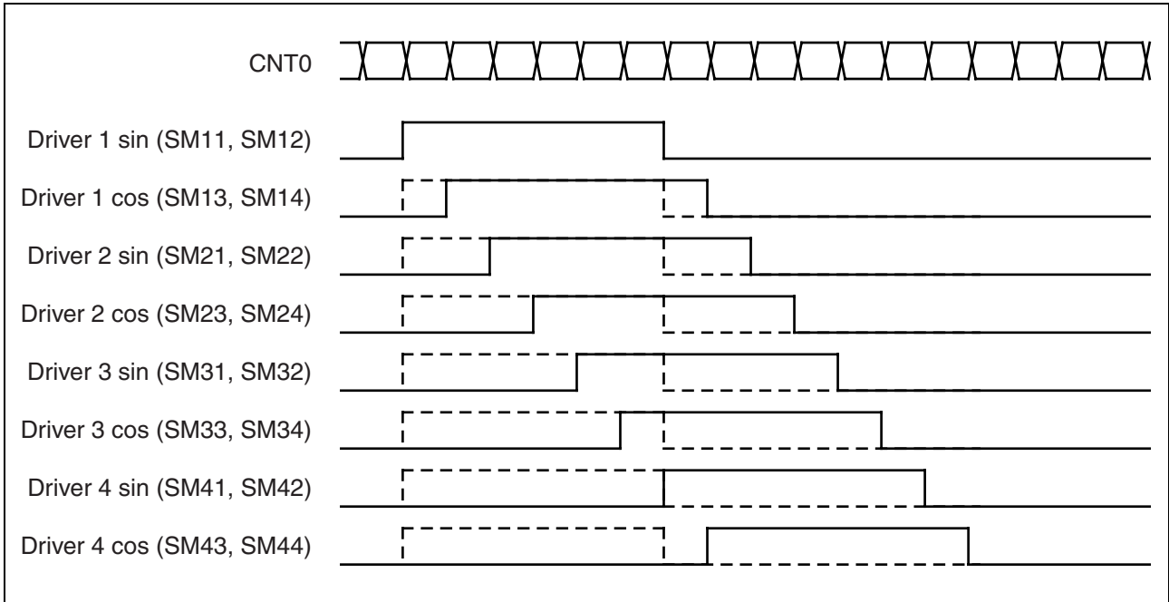
Figure 16-11. Output Timing of Signals SM11 to SM44
