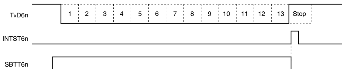
Figure 12-29. SBF Transmission
