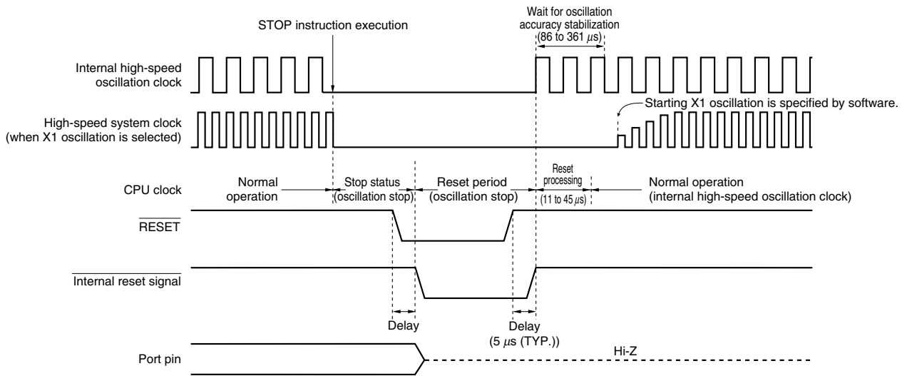
Figure 21-4. Timing of Reset in STOP Mode by \overline{\text{RESET}} Input
