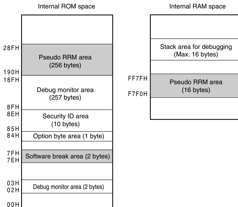
Figure 27-5. Reserved Area Used by QB-MINI2
