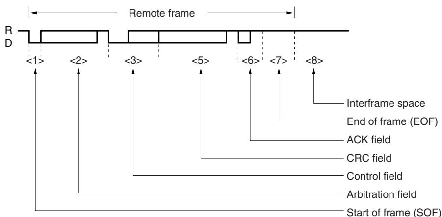
Figure 15-4. Remote Frame
