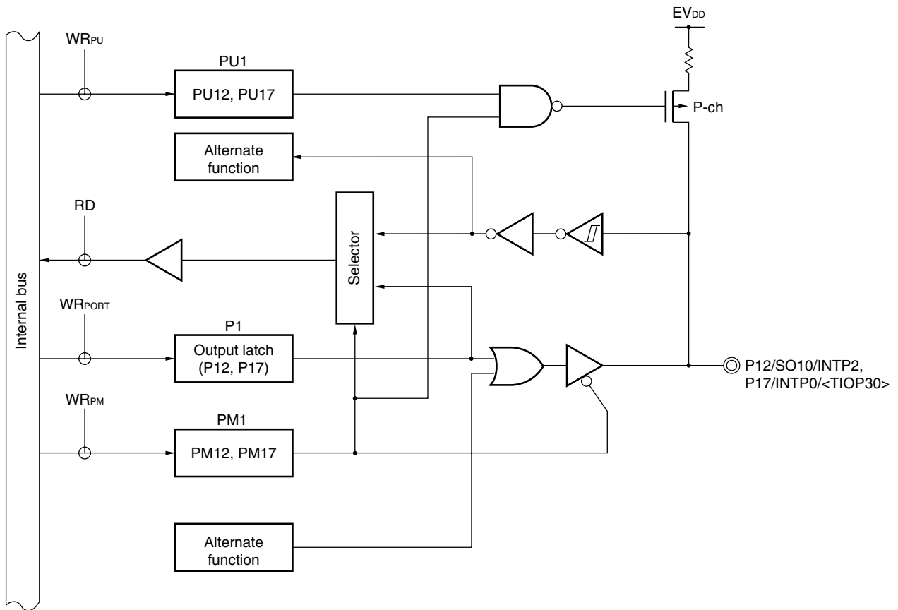
Figure 4-5. Block Diagram of P12 and P17
