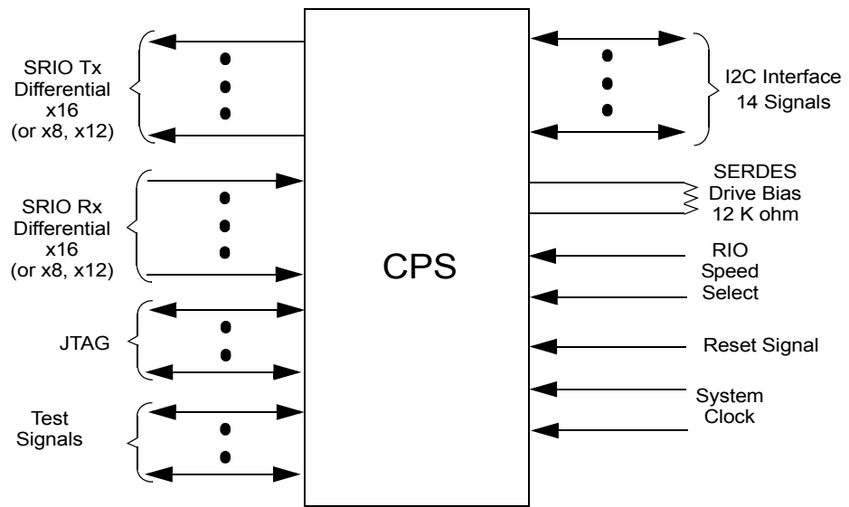
Figure 1.2 CPS Interconnect
