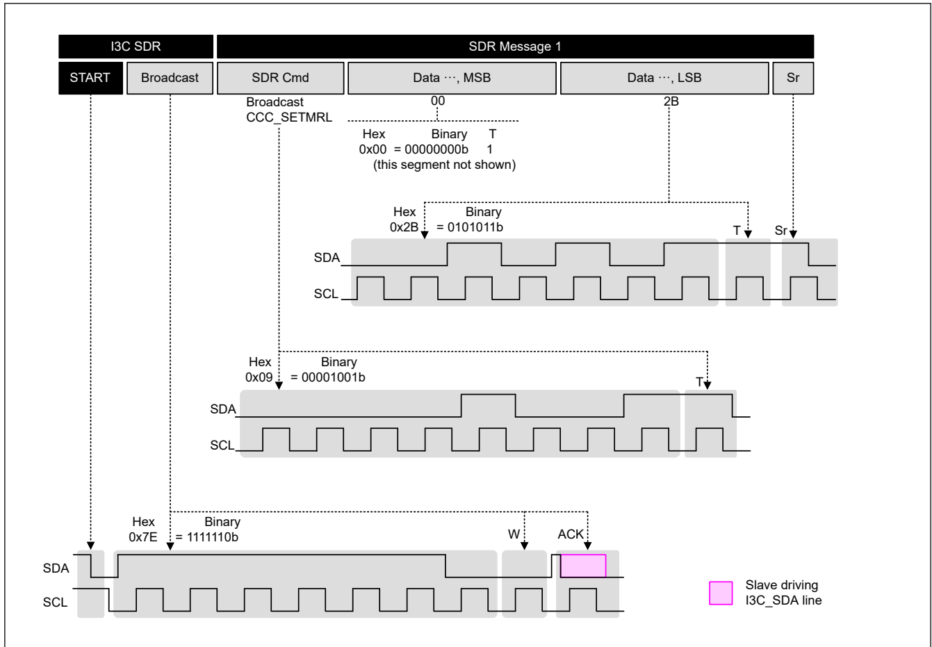
Figure 29.73 Example communication using I3C coding SDR with CCC broadcast
