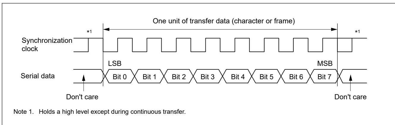
Figure 26.65 Data format in clock synchronous serial communications with LSB-first order
