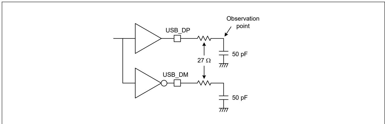
Figure 49.59 Test circuit in full-speed mode
