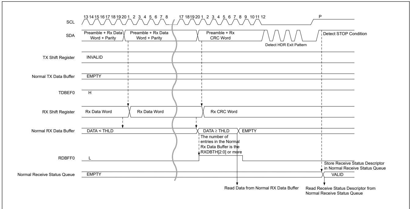
Figure 29.55 HDR data write transfer (HDR-DDR) timing (3/3)
