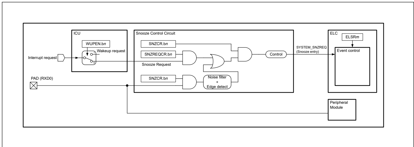
Figure 10.7 Snooze mode entry configuration
