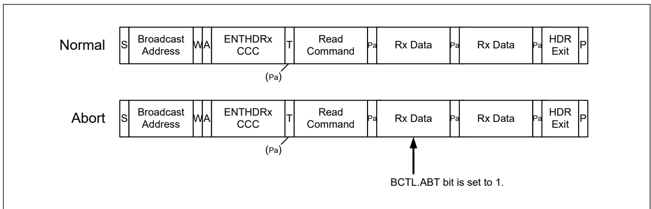
Figure 29.119 Abort operation of HDR-TSP/TSL read transfer
