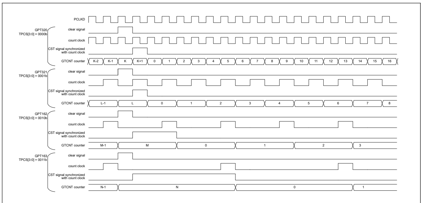
Figure 20.40 Example of Simultaneous Clearing Operation by Software (with Different Count Period)
