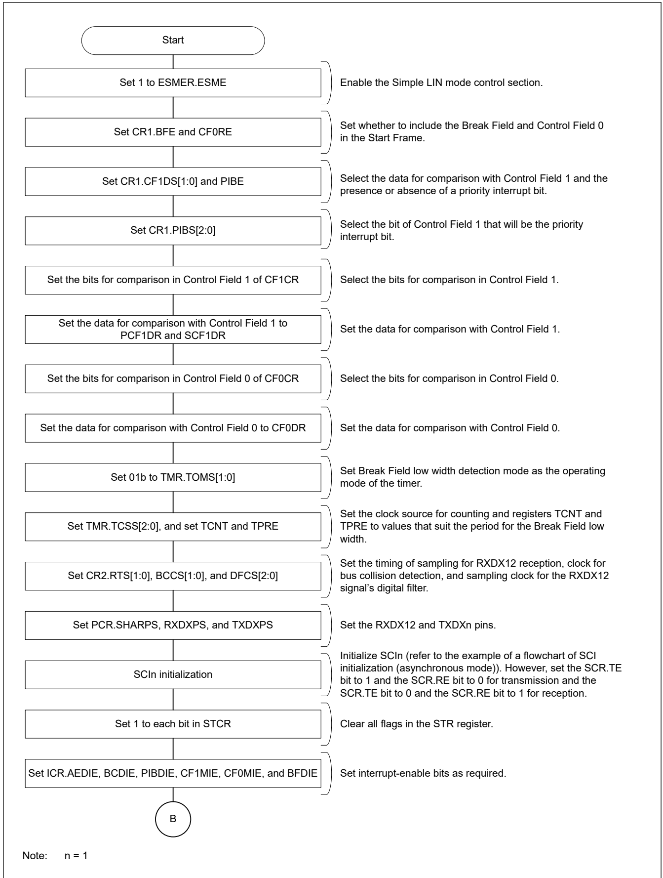
Figure 26.107 Sample flowchart for reception of a Start Frame (1)
