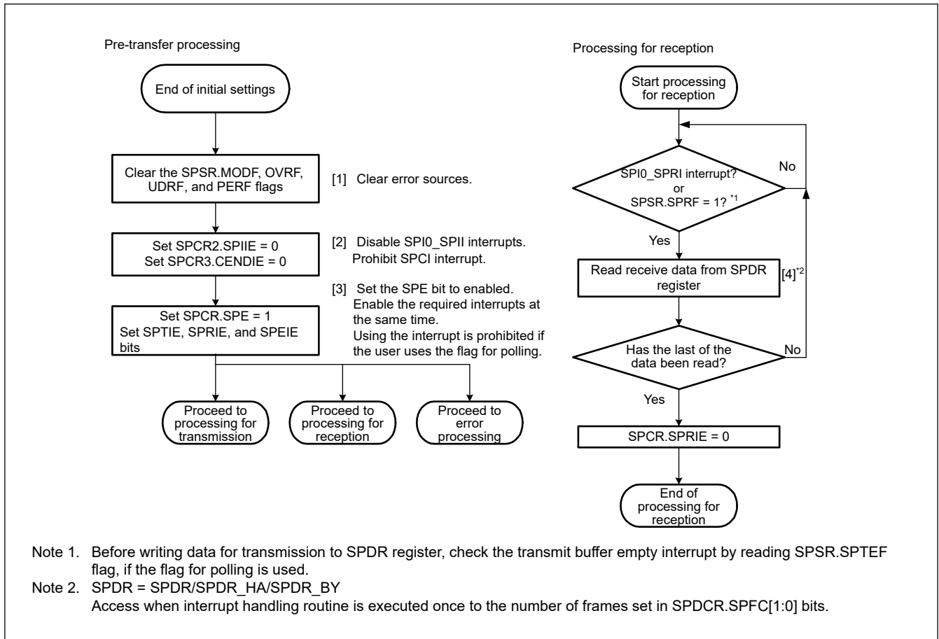
Figure 33.55 Transmission flow in slave mode
