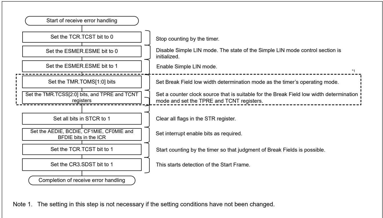
Figure 26.125 Example flowchart for receive error handling (during reception of the Start Frame)
