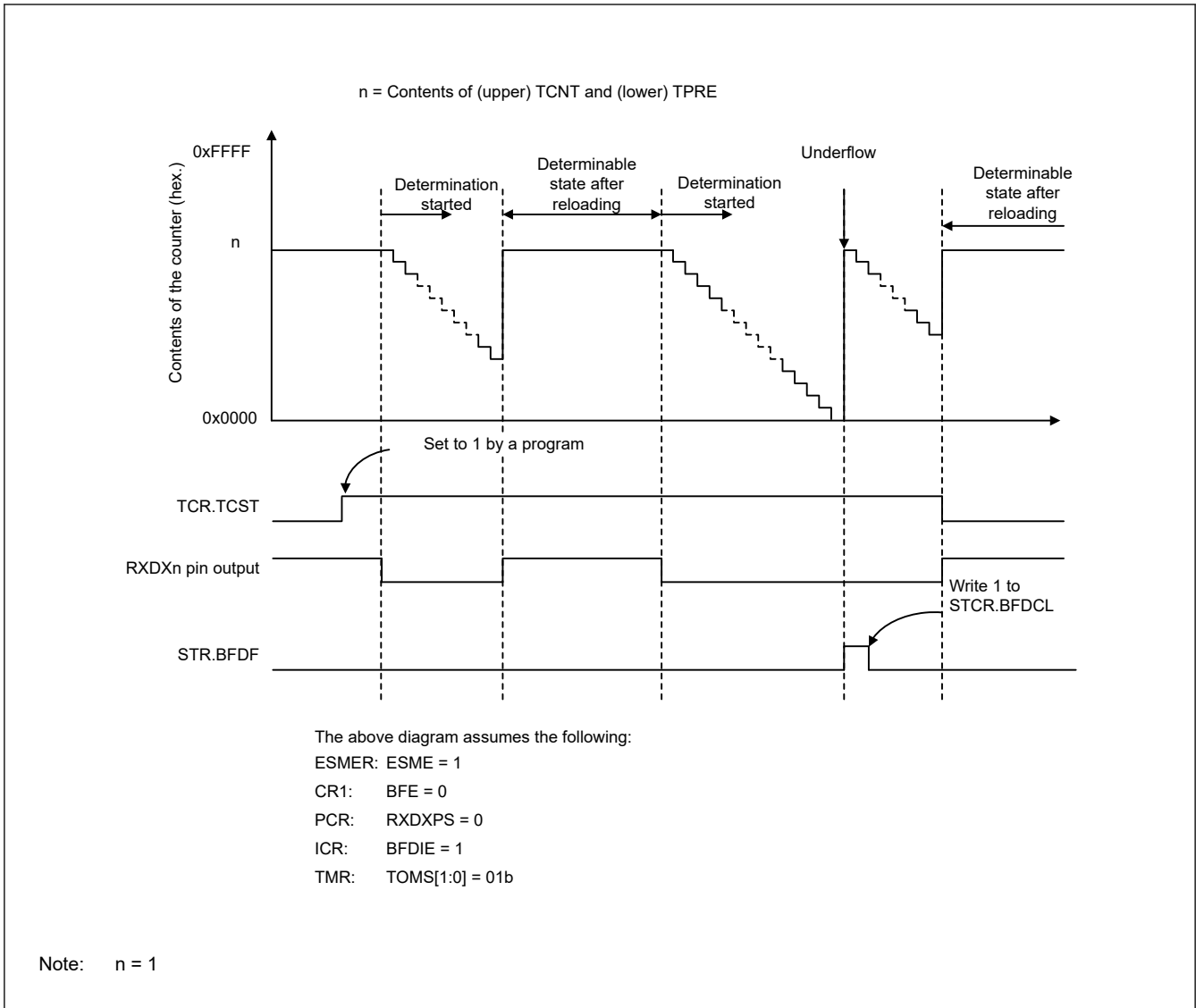
Figure 26.116 Example of operations in Break Field low width determination mode
