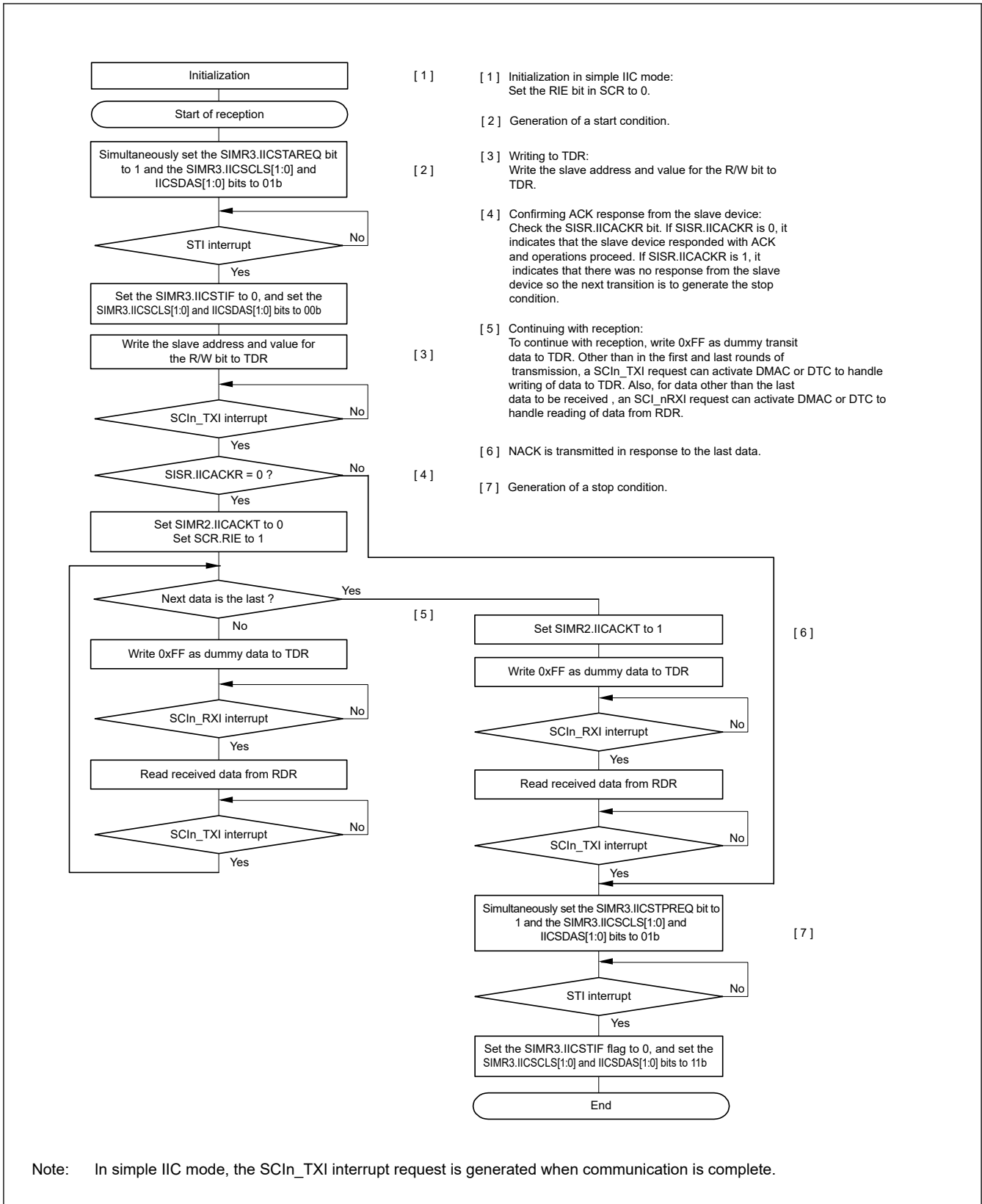
Figure 26.97 Example flow of master reception in simple IIC mode with transmission interrupts and reception interrupts
