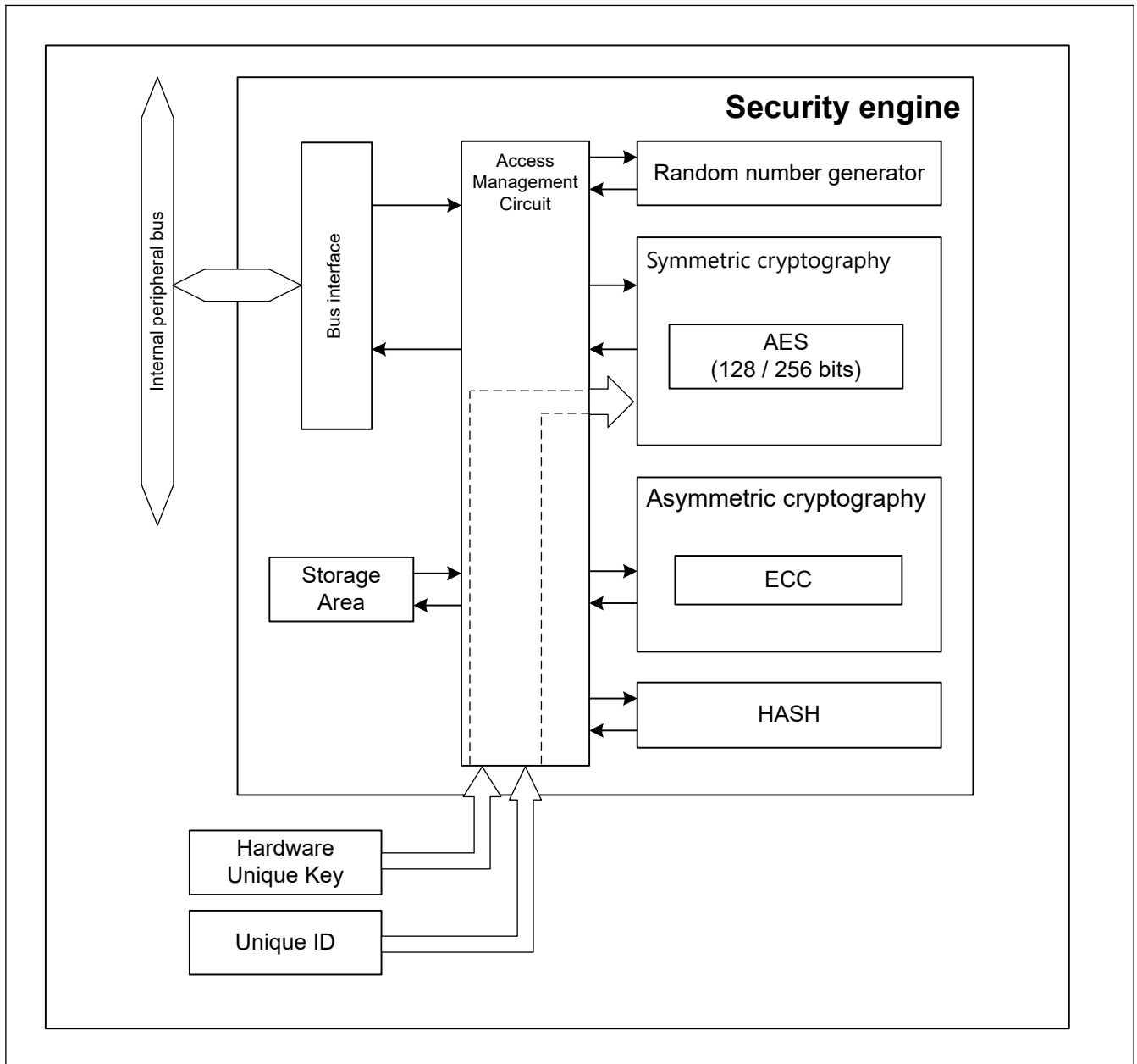
Figure 37.1 Security engine block diagram
