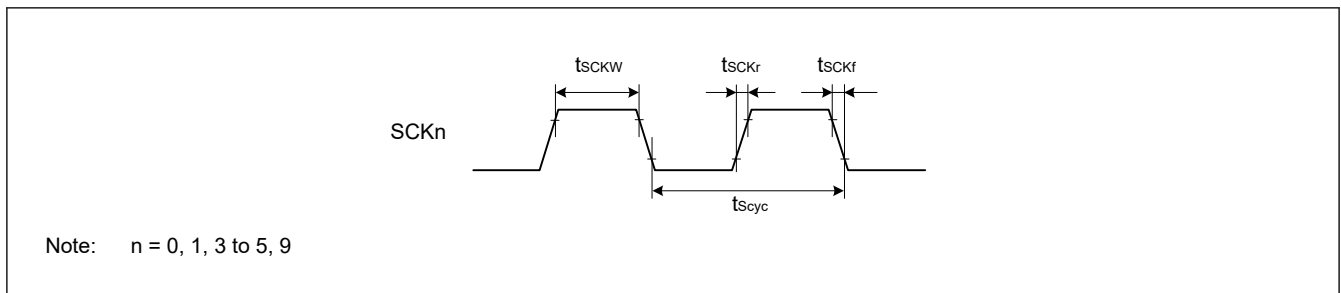
Figure 49.23 SCK clock input timing
