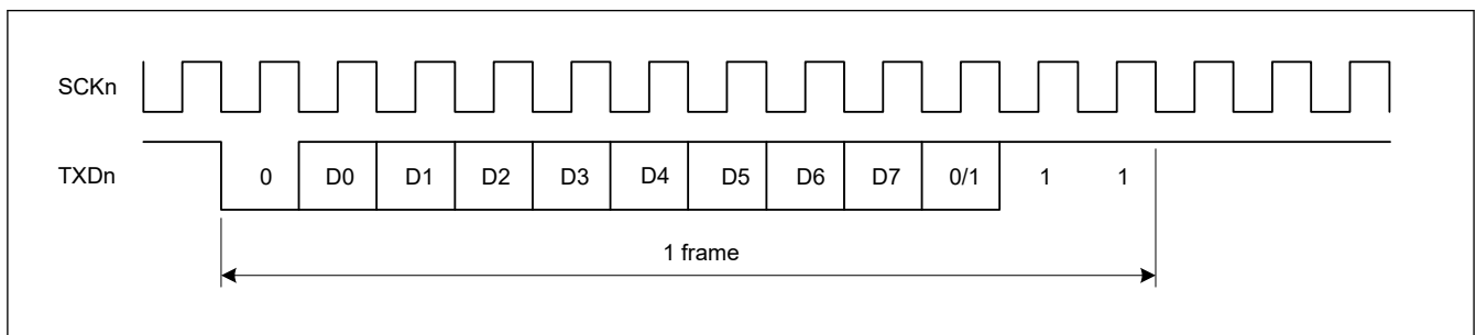
Figure 26.8 Phase relationship between output clock and transmit data in asynchronous mode when SMR.CHR = 0, PE = 1, MP = 0, and STOP = 1
