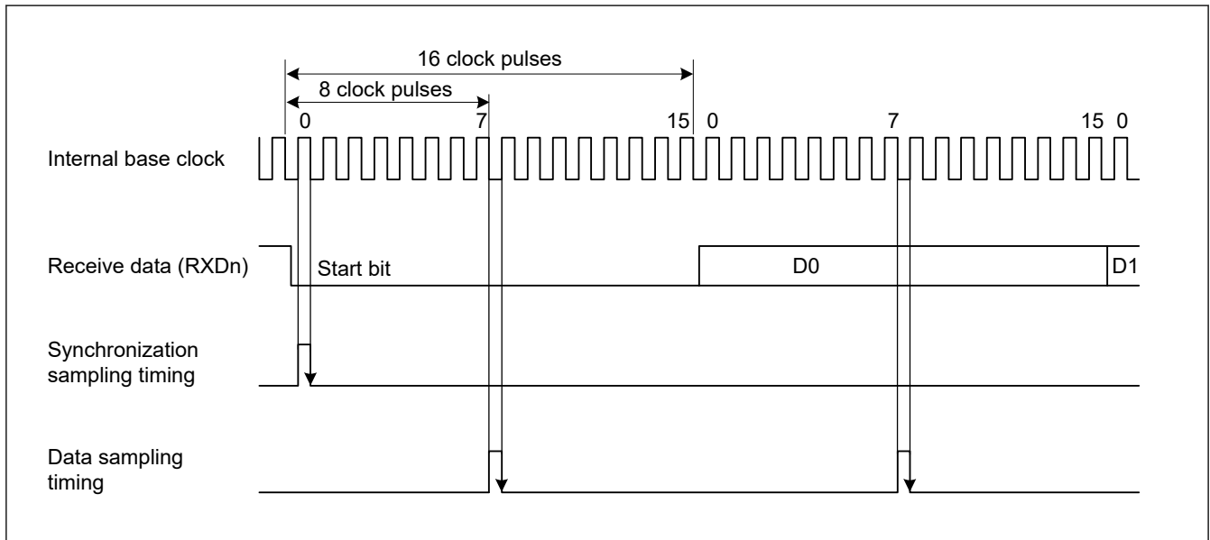
Figure 26.7 Receive data sampling timing in asynchronous mode
