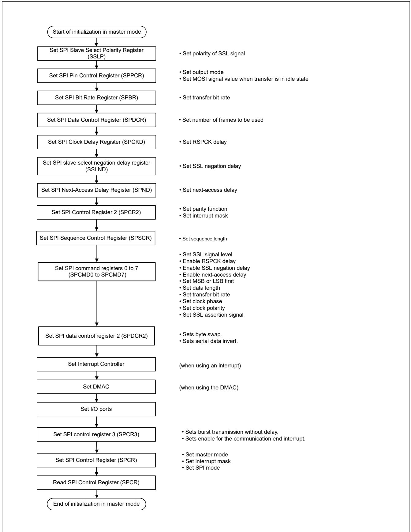
Figure 33.50 Example of initialization flow in master mode for SPI operation
