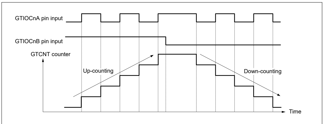
Figure 20.53 Example of phase counting mode 2 (C)
