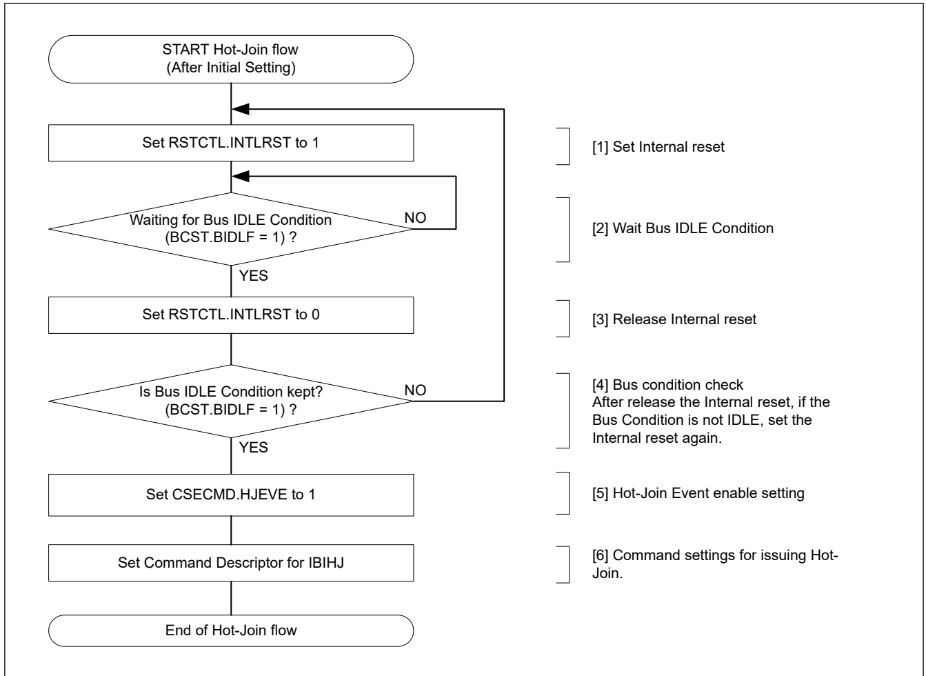
Figure 29.153 Hot-join flowchart after the I3C bus has already been configured
