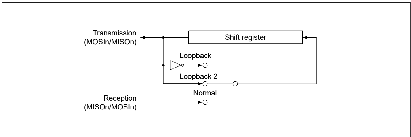
Figure 33.63 Configuration of shift register I/O paths in loopback mode for master mode
