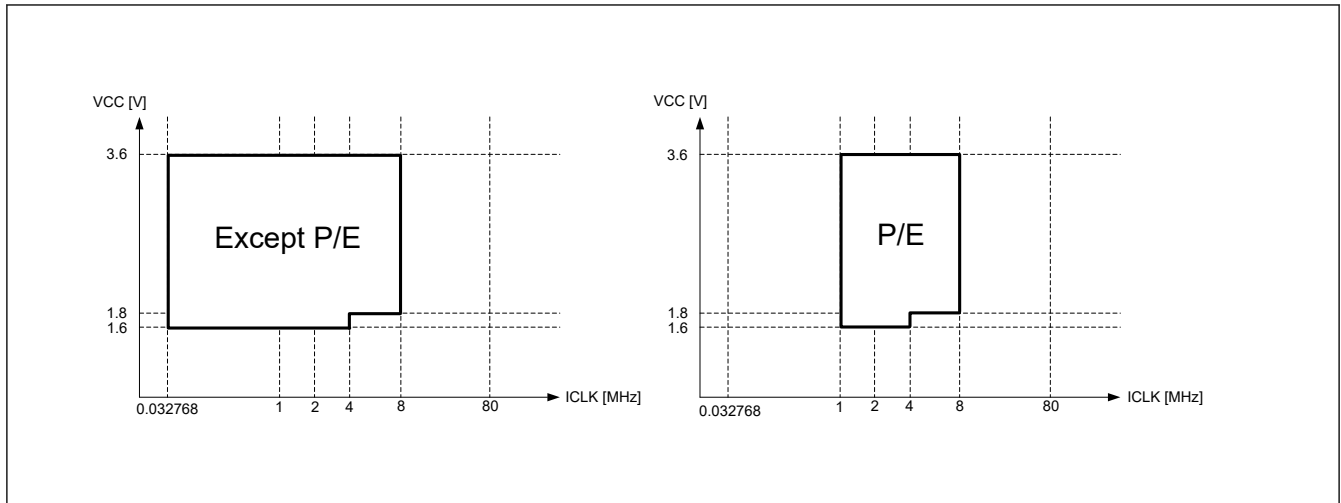
Figure 10.3 Operating voltages and frequencies in Middle-speed mode
