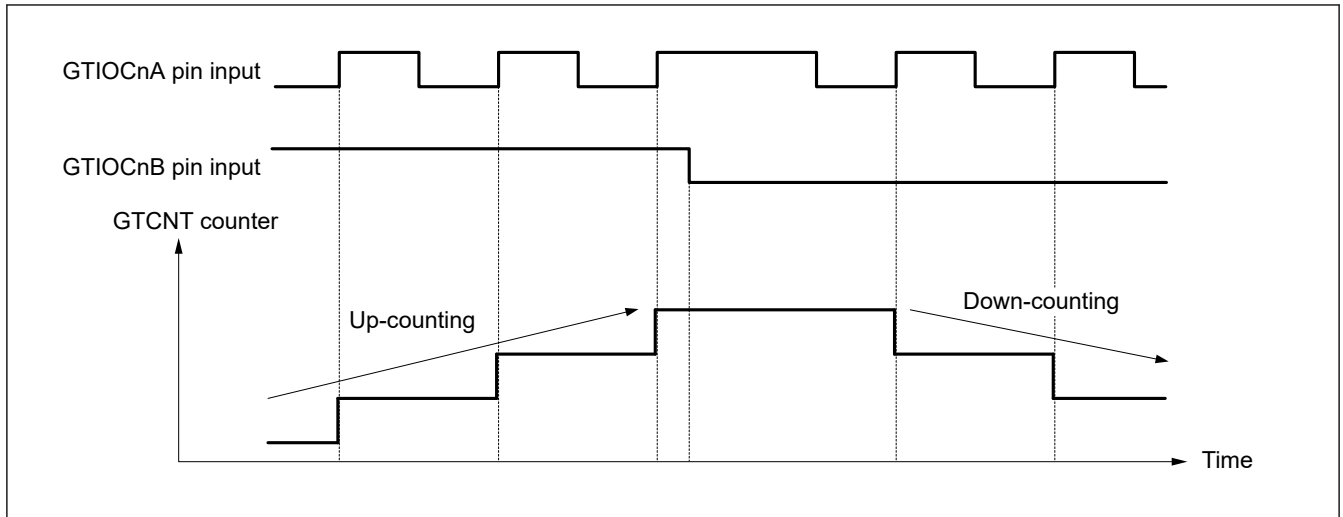
Figure 20.52 Example of phase counting mode 2 (B)
