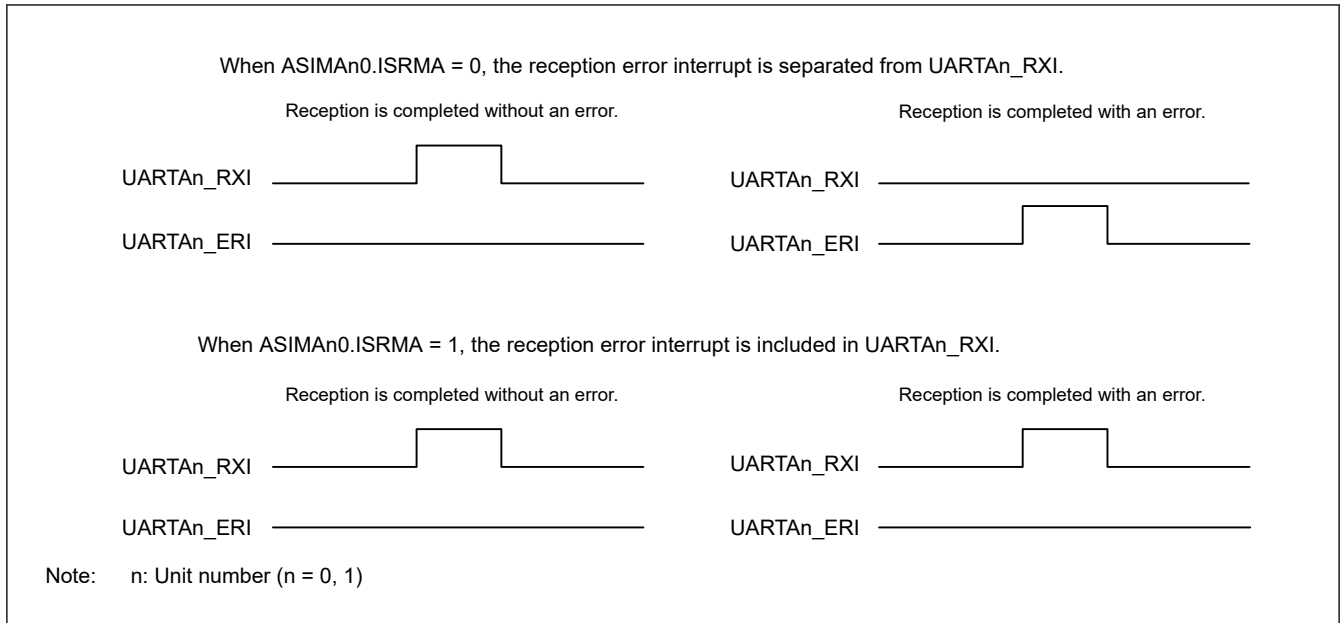
Figure 30.8 Various interrupt output waveforms depending on ASIMAn0.ISRMA setting
