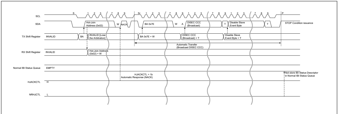
Figure 29.109 Hot-join event: NACK (HJACKCTL = 1) and NRHJCTL = 0
