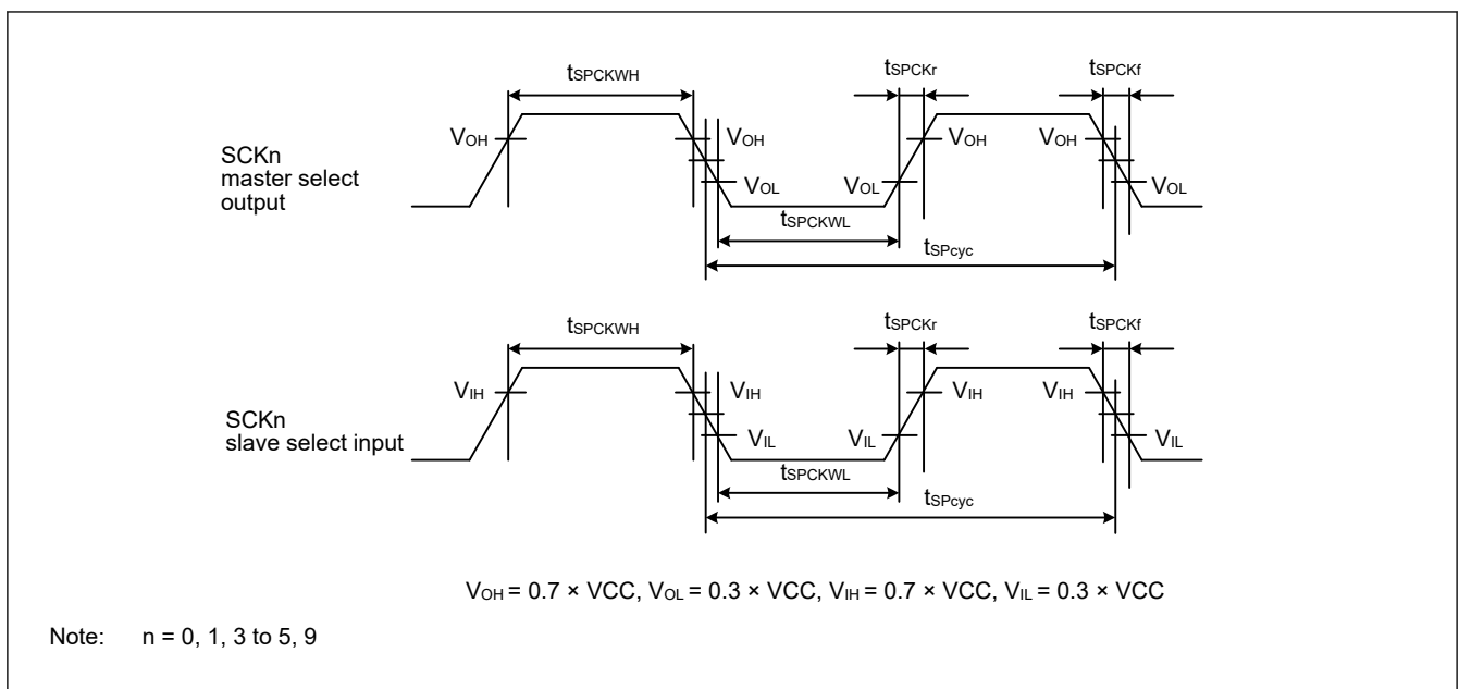
Figure 49.25 SCI simple SPI mode clock timing
