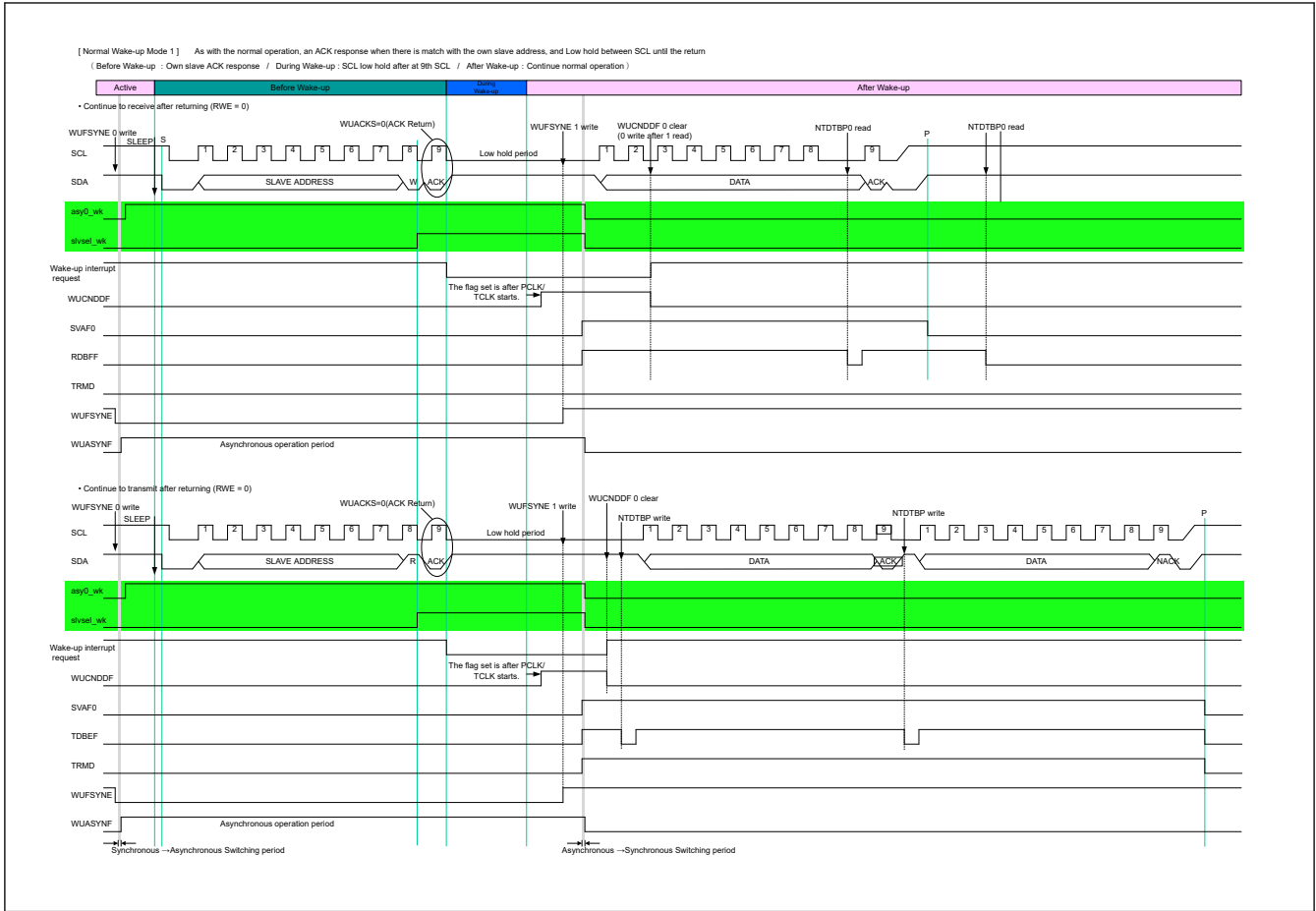
Figure 29.126 Timing of normal Wake-up mode 1
