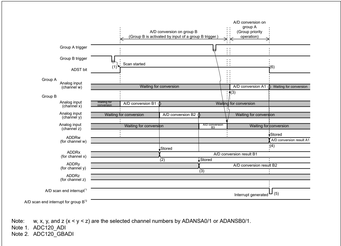
Figure 38.20 Group priority operation example 1-4: “Group A trigger is input during group B scan” when rescanning is disabled (when ADGSPCR.GBRSCN = 0, ADGSPCR.GBRP = 0)
