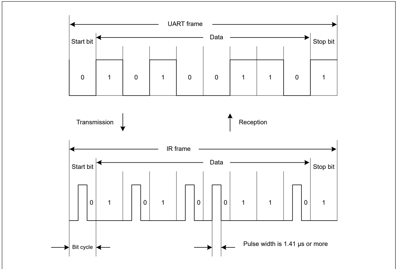
Figure 27.2 Transmission and reception through the IrDA interface
