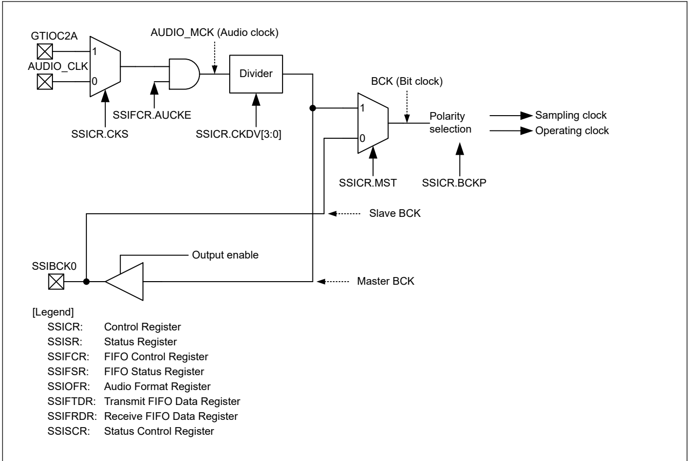
Figure 35.3 SSIE clock configuration
