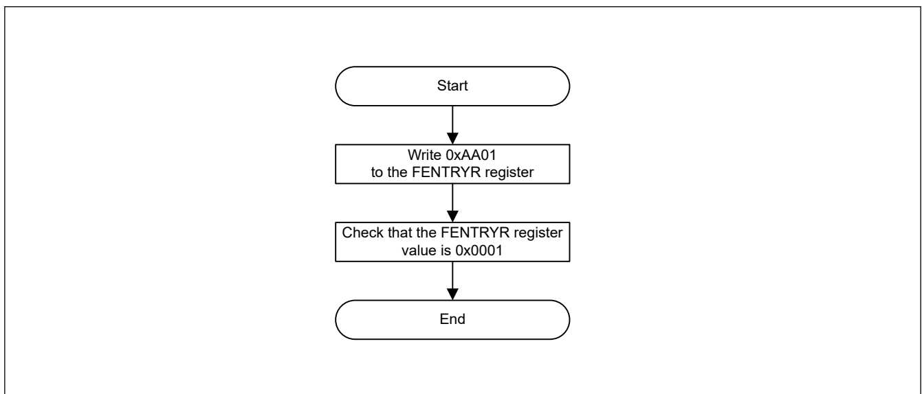
Figure 45.10 Procedure to transition to code flash P/E mode from read mode
