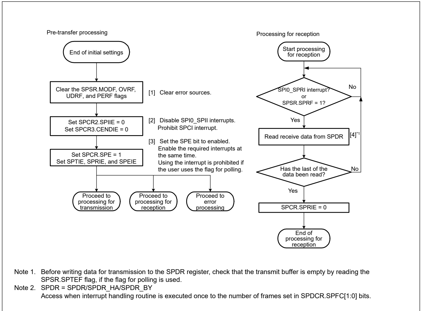
Figure 33.56 Reception flow in slave mode
