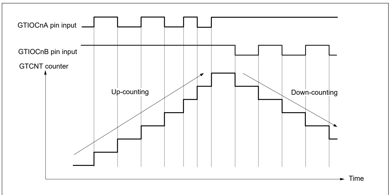
Figure 20.56 Example of phase counting mode 3 (C)
