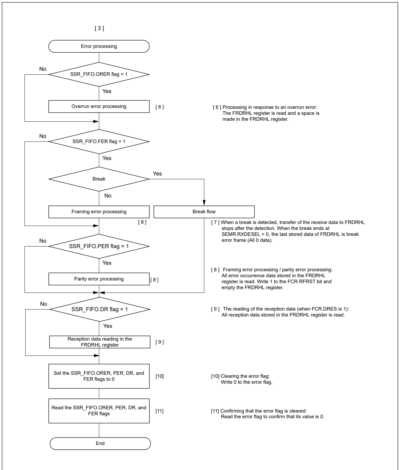
Figure 26.27 Example flow of serial reception in asynchronous mode with FIFO selected Address Matching Disabled (2)
