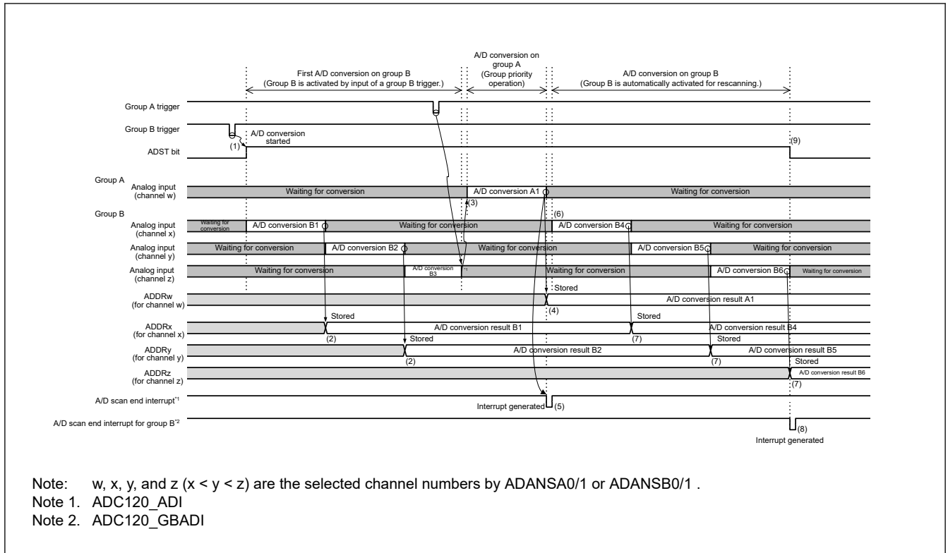
Figure 38.17 Example of group priority operation 1-1: Group A trigger input during group B scanning when rescanning is enabled (when ADGSPCR.GBRSCN = 1, ADGSPCR.GBRP = 0)
