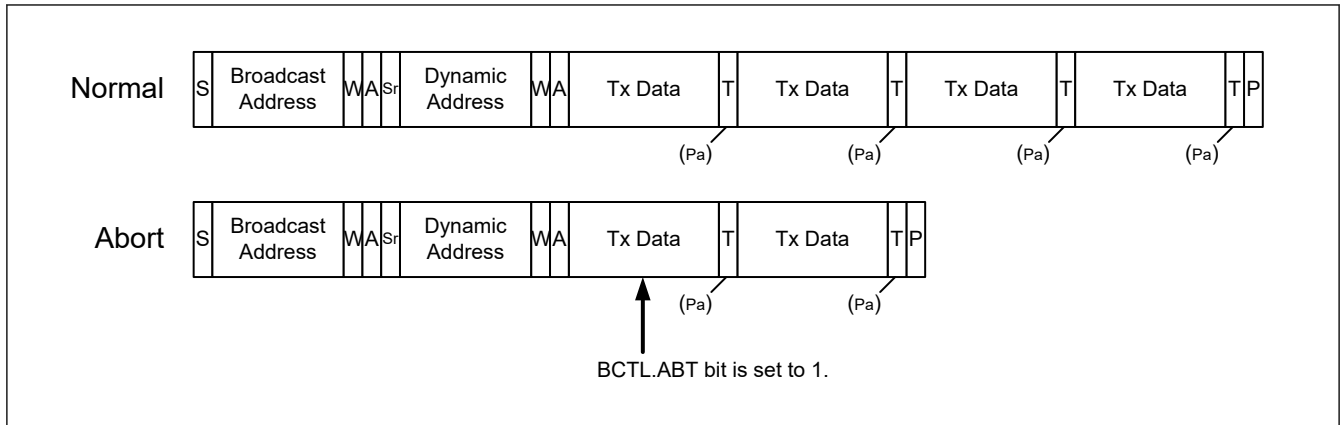
Figure 29.114 Abort operation of SDR write transfer
