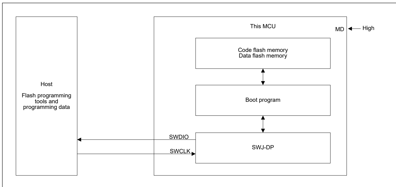
Figure 45.39 Block diagram of flash memory-related modules
