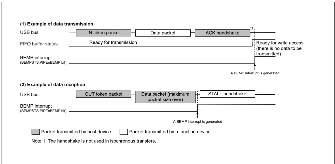
Figure 25.9 Timing of BEMP interrupt generation in device controller mode
