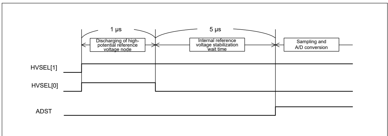
Figure 38.31 Procedure to select internal reference voltage as high-potential reference voltage
