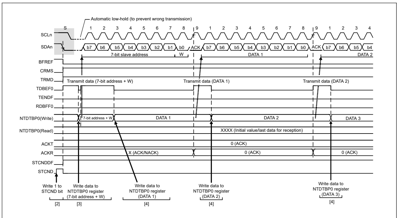
Figure 29.6 Master transmit operation timing (1) (7-bit address format)
