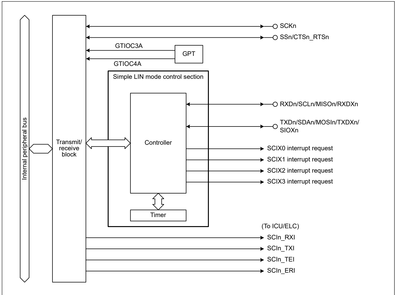
Figure 26.2 SCIn (n = 1) Simple LIN mode controller block diagram
