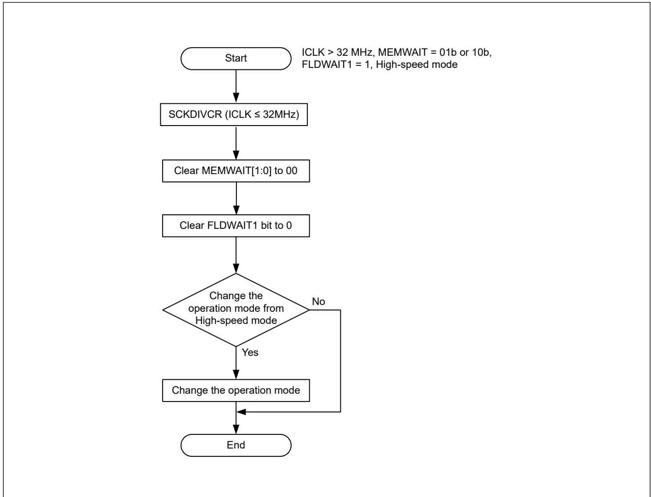
Figure 8.3 When setting ICLK ≤ 32 MHz from ICLK > 32 MHz
