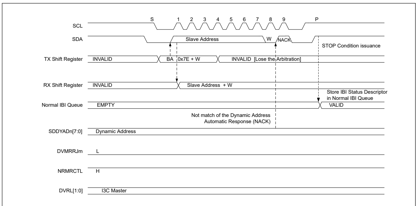
Figure 29.104 Mastership request : NACK (not match the DVDYAD[7:0] of DAT) and NRMRCTL = 1
