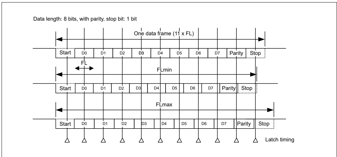
Figure 30.11 Permissible baud rate range during reception
