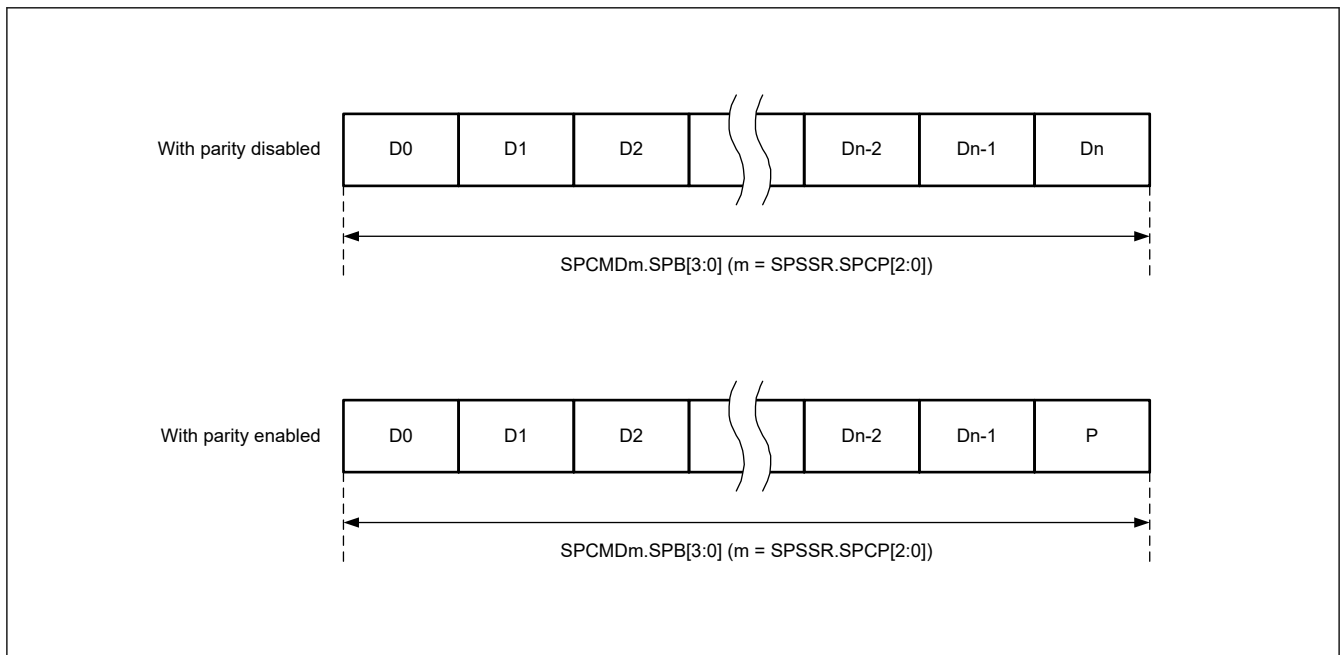
Figure 33.13 Data format with parity disabled and enabled
