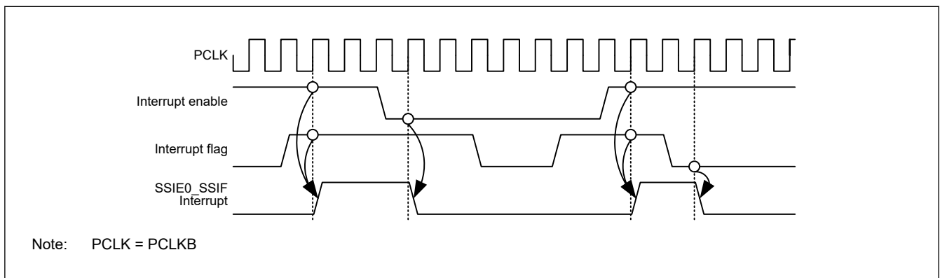
Figure 35.58 Timing diagram of the common interrupt source, SSIE0_SSIF
