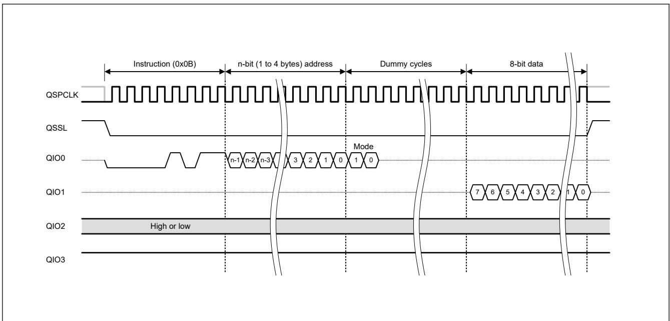
Figure 34.19 Fast Read bus cycle
