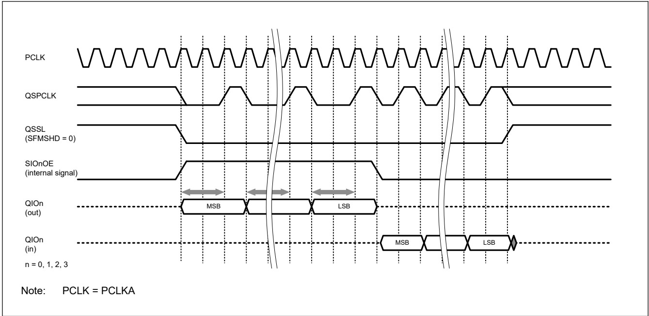
Figure 34.15 Setup time adjustment for serial data output using the SFMOSW bit
