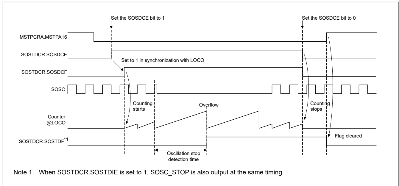
Figure 8.11 Timing of oscillation stop detection by sub clock oscillation stop detector
