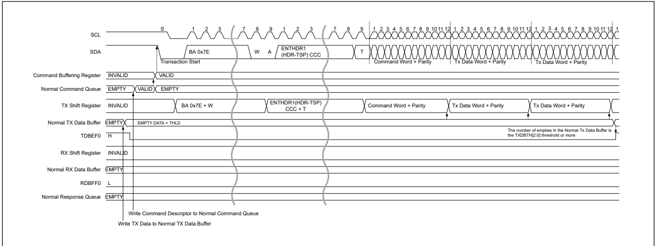
Figure 29.28 HDR data write transfer (HDR-TSP, TSL) timing (1/2)
