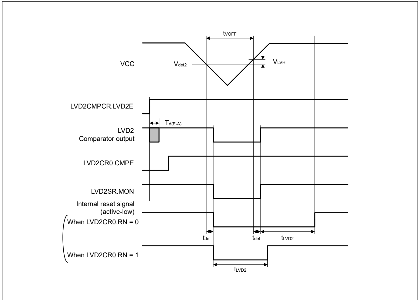
Figure 49.69 Voltage detection circuit timing (V det2 )
