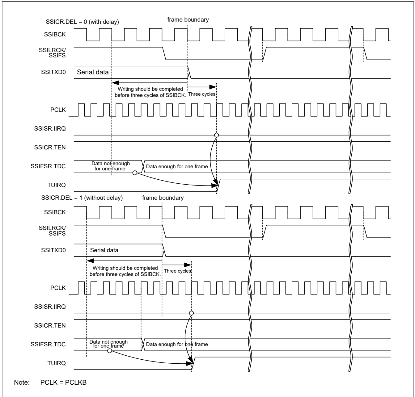
Figure 35.19 TUIRQ setting timing (when communication continues)
