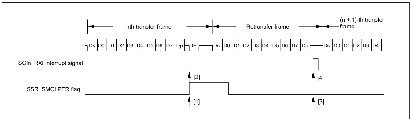
Figure 26.85 Data re-transfer operation in smart card interface reception mode
