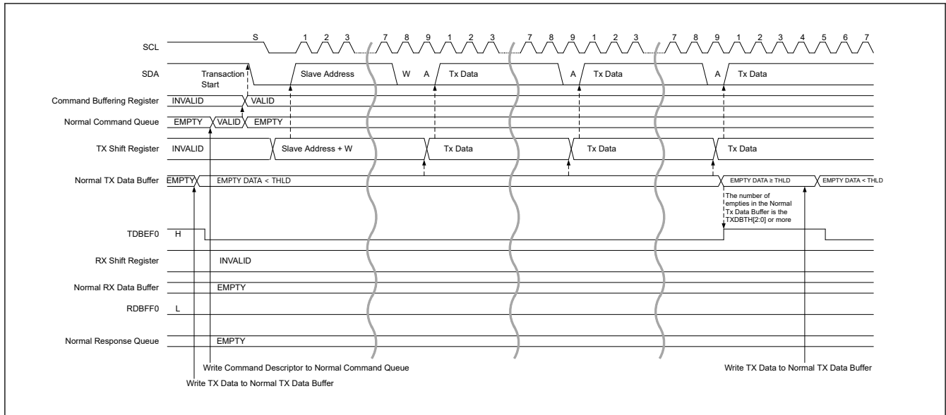
Figure 29.18 Legacy I 2 C message data write timing (1/2)
