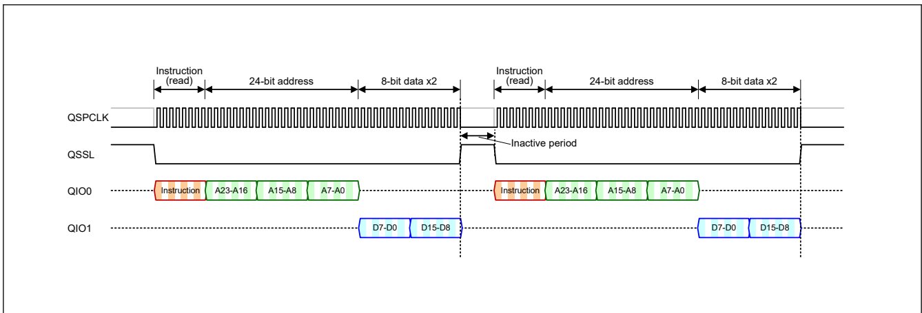
Figure 34.32 Successive data read operations based on individual conversion
