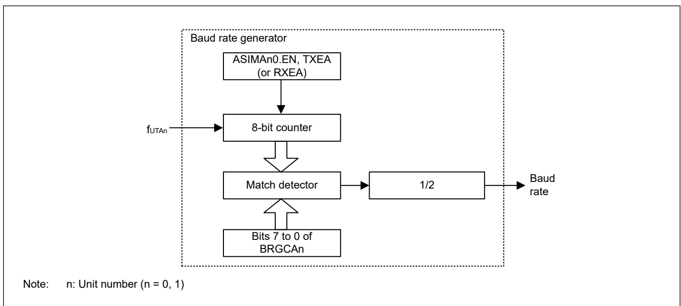
Figure 30.10 Configuration of baud rate generator
