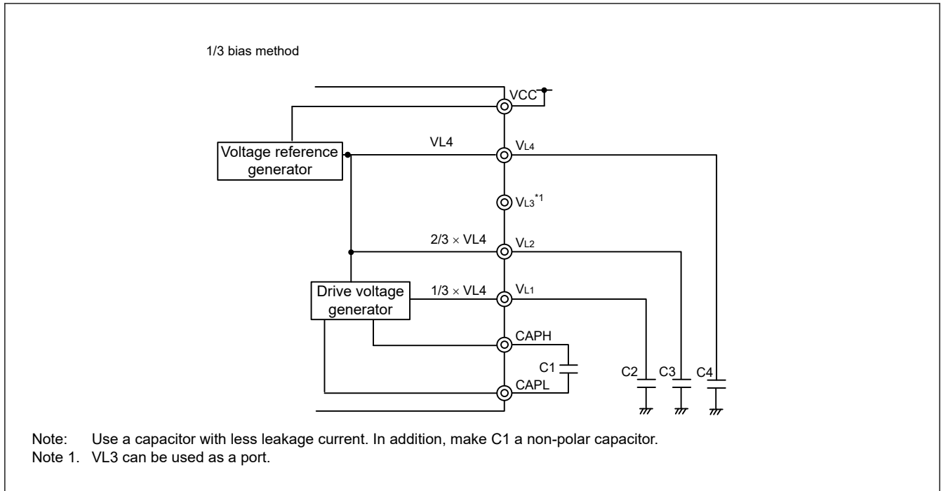
Figure 46.15 Examples of LCD drive power connections using VL4 reference mode of capacitor split method
