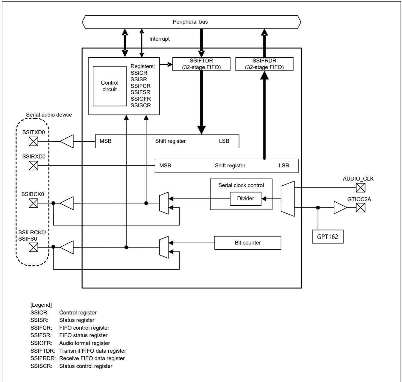
Figure 35.2 SSIE block diagram
