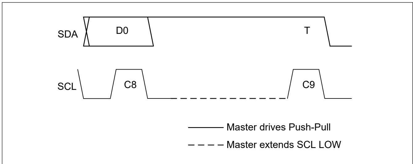
Figure 29.95 Master clock stalling in write parity bit
