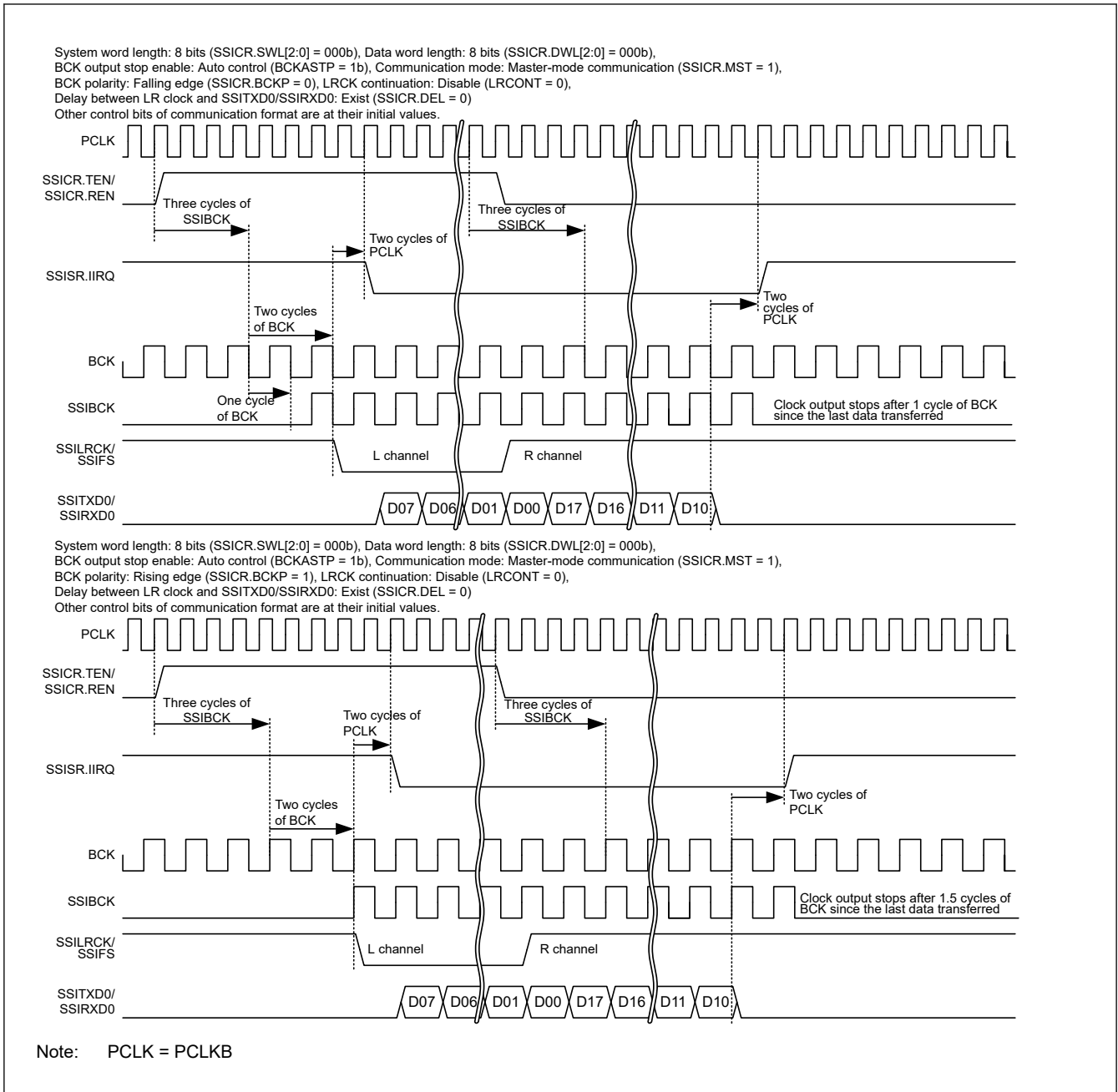
Figure 35.34 Example operation of the BCKASTP bit (communication operation with BCKASTP = 1)
