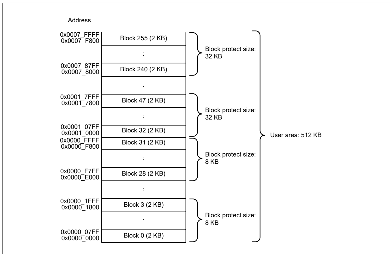
Figure 45.2 Map of the code flash memory in linear mode
