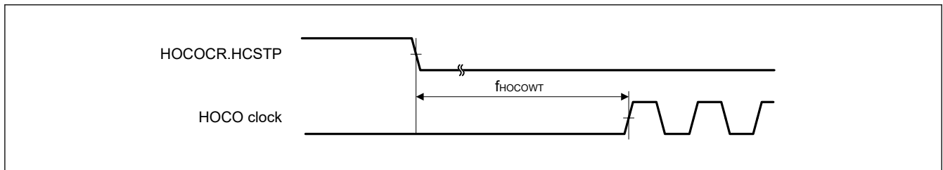
Figure 49.8 HOCO clock oscillation start timing (started by setting the HOCOCR.HCSTP bit)
