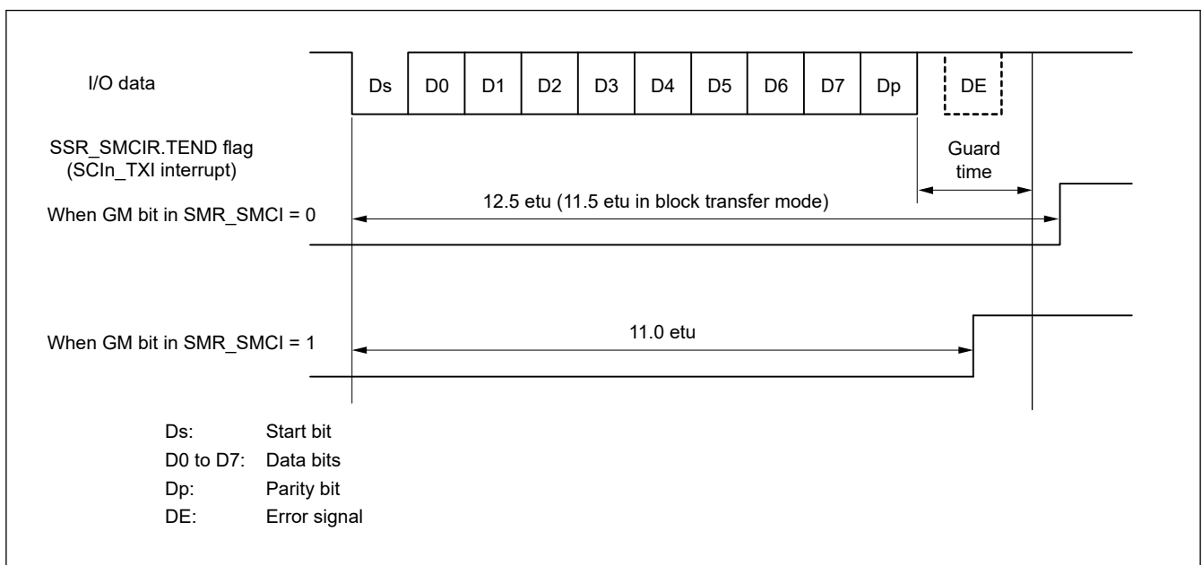
Figure 26.83 SSR.TEND flag generation timing during transmission
