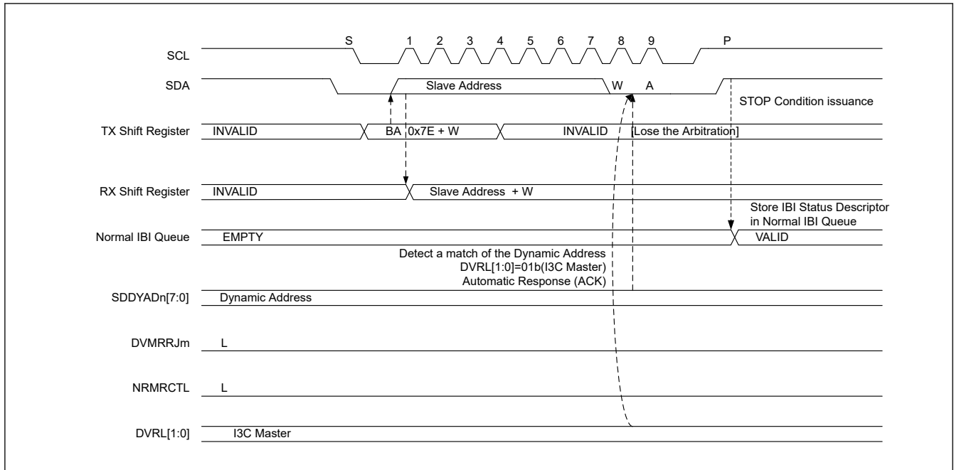
Figure 29.103 Mastership request : ACK
