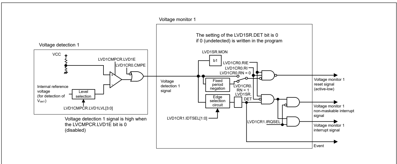
Figure 7.2 Block diagram of voltage monitor 1 interrupt and reset circuit
