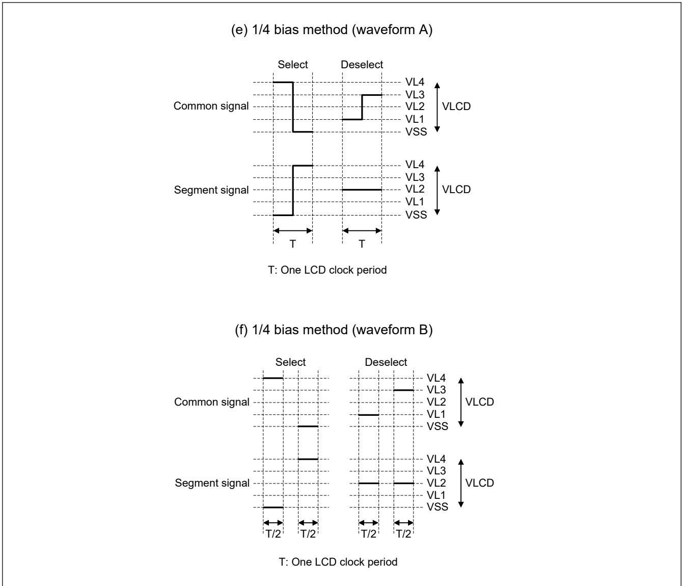
Figure 46.21 Voltages and phases of common and segment signals (3 of 3)
