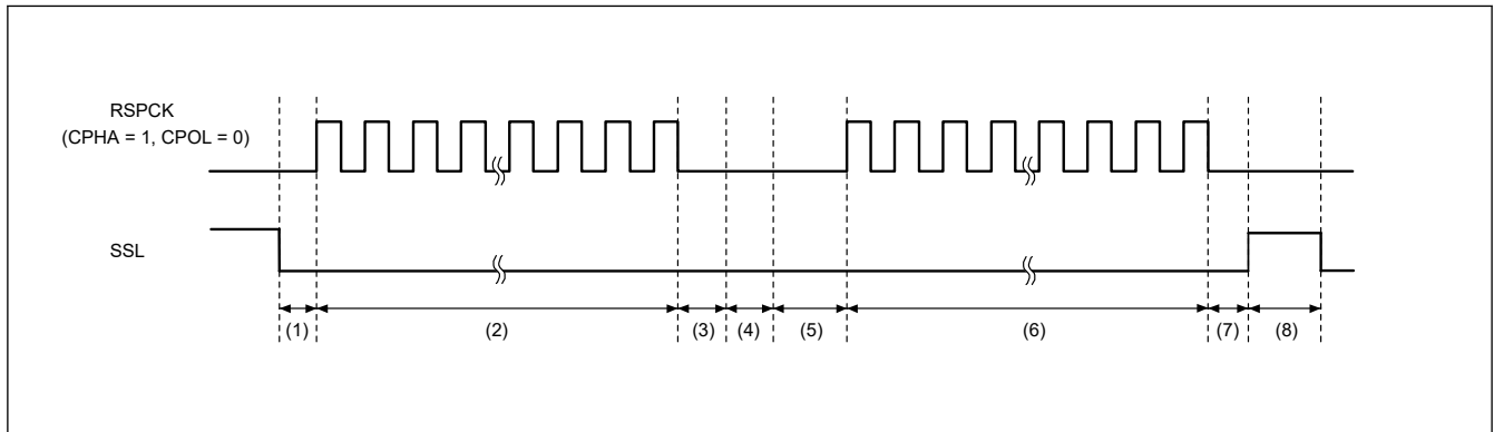
Figure 33.48 Example of burst transfer operation using the SSLKP bit (BFDS = 0)
