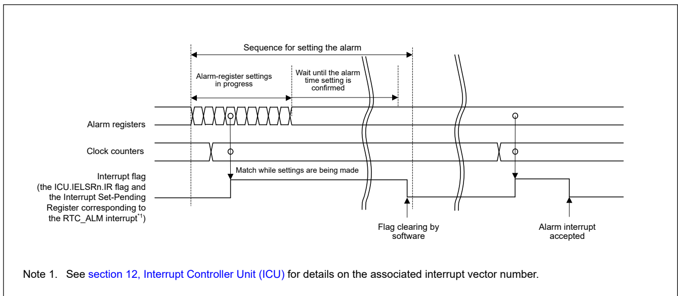
Figure 22.10 Timing for the alarm interrupt (RTC_ALM)
