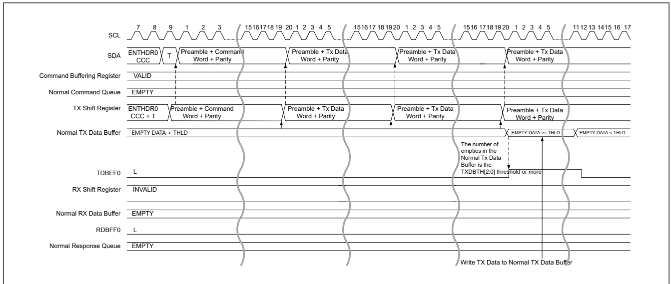
Figure 29.25 HDR data write transfer (HDR-DDR) timing (2/4)
