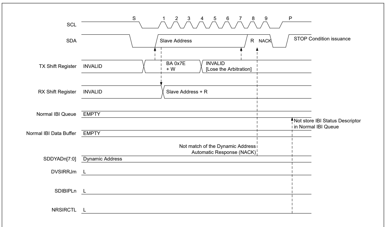
Figure 29.100 Slave interrupt request : NACK (not match the SDDYAD[7:0] of DAT) and NRSIRCTL = 0
