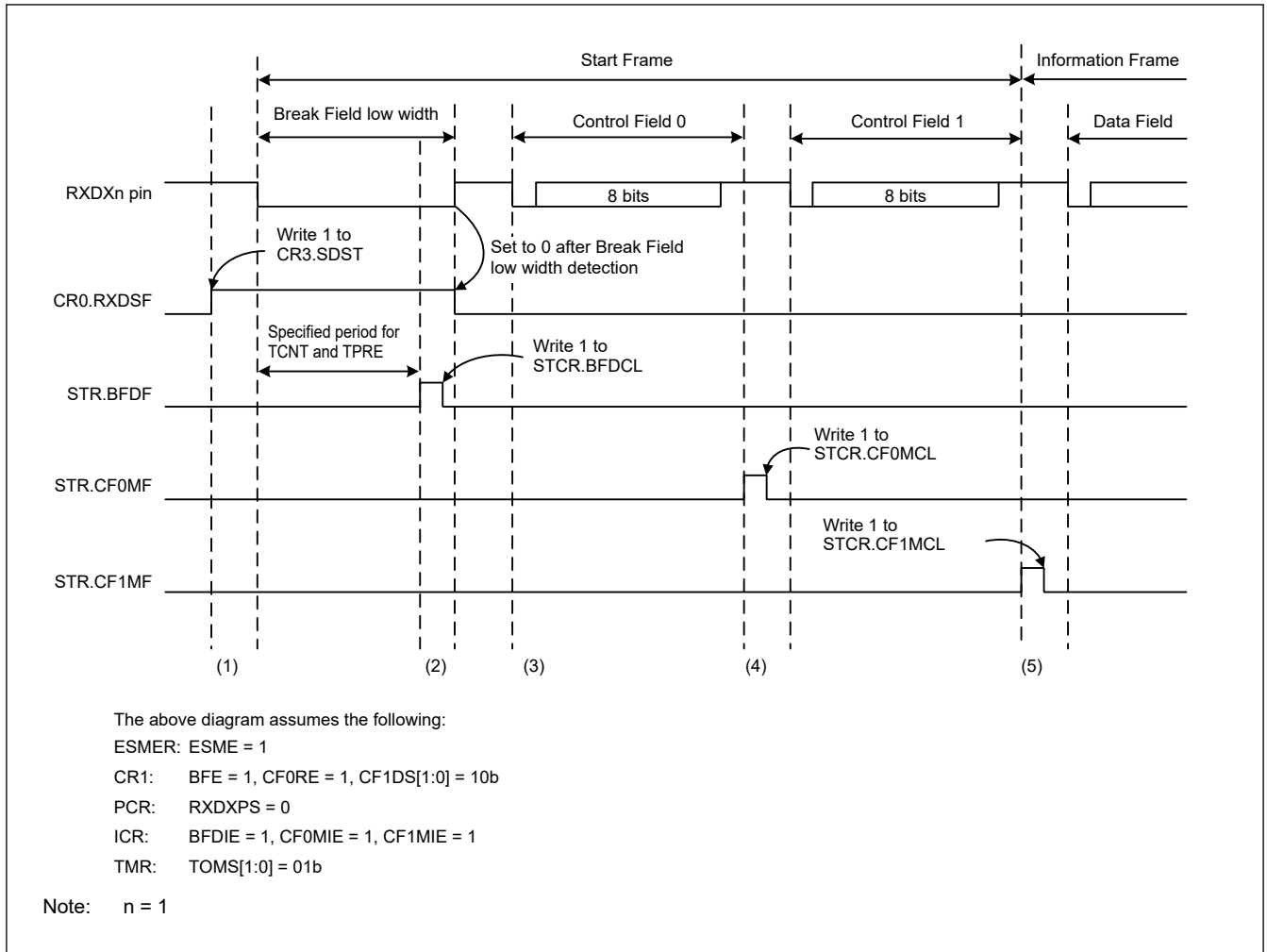
Figure 26.106 Example of operations at the time of Start Frame reception
