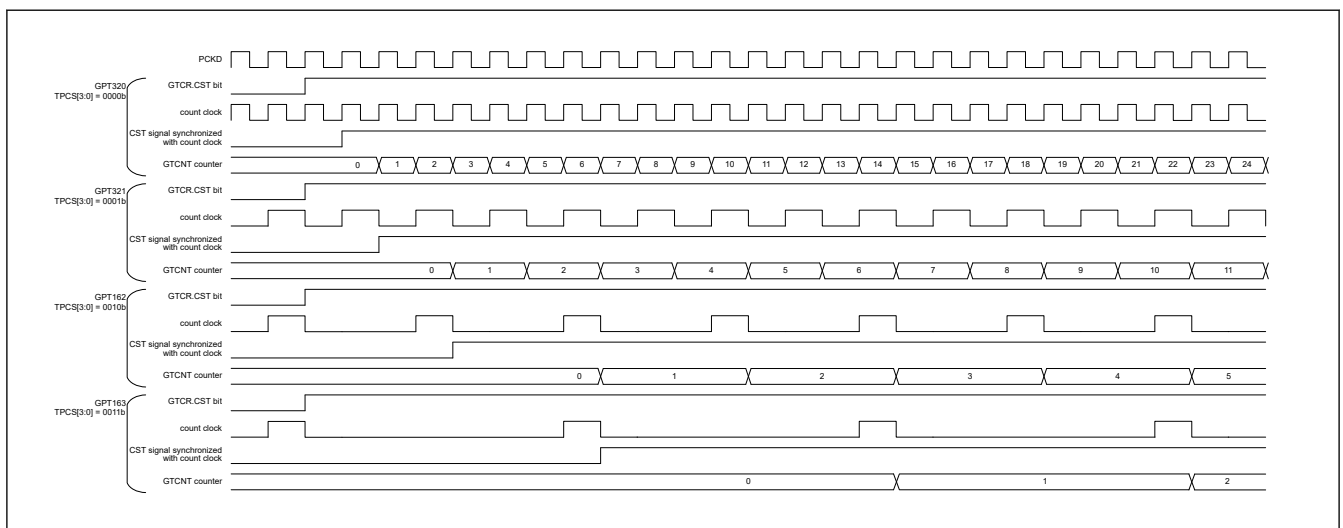
Figure 20.38 Example of Simultaneous Start Operation by Software (with Different Count Period)
