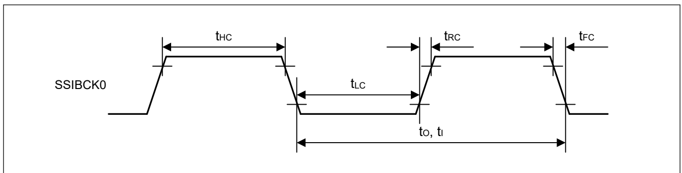
Figure 49.52 SSIE clock input/output timing
