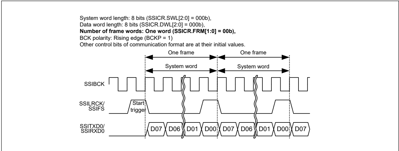
Figure 35.37 Short frame in monaural format (without padding: system word length = data word length)
