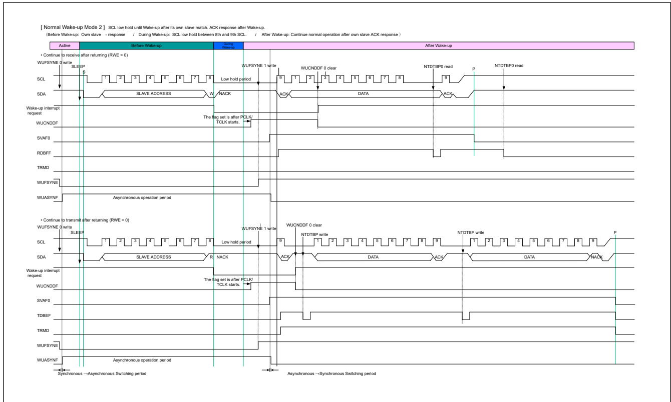
Figure 29.128 Timing of normal Wake-up mode 2
