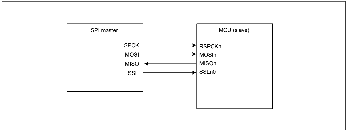
Figure 33.6 Single-master/single-slave configuration example with the MCU as a slave and CPHA = 0
