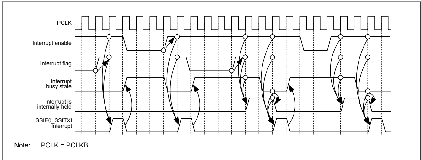
Figure 35.59 SSIE0_SSITXI interrupt timing diagram
