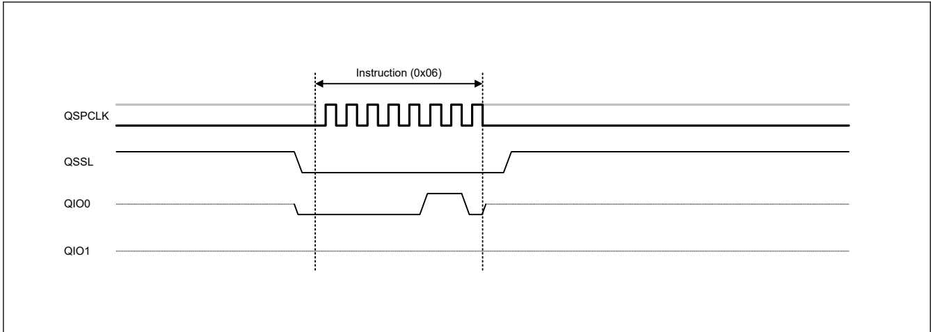
Figure 34.31 Write Enable bus cycle
