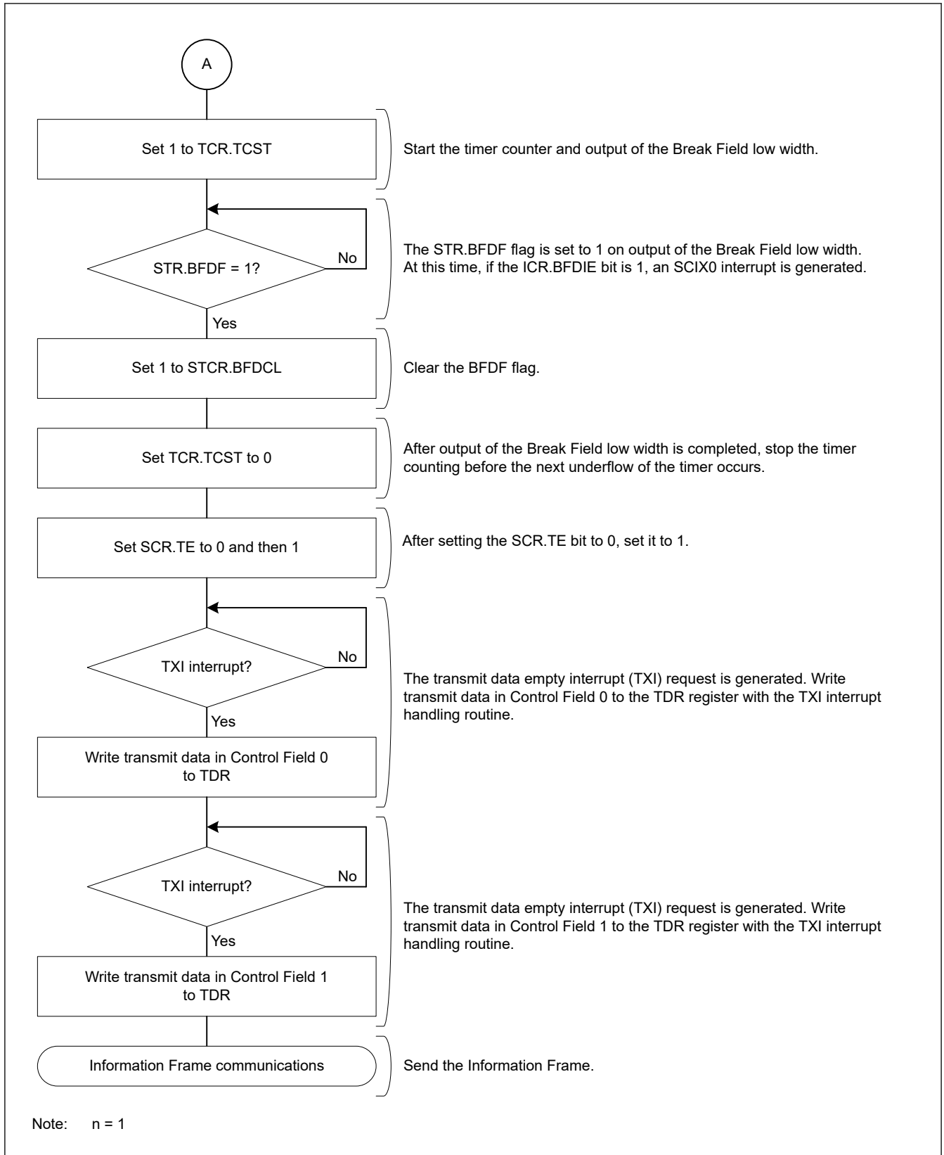
Figure 26.104 Example of Start Frame transmission (2/2)
