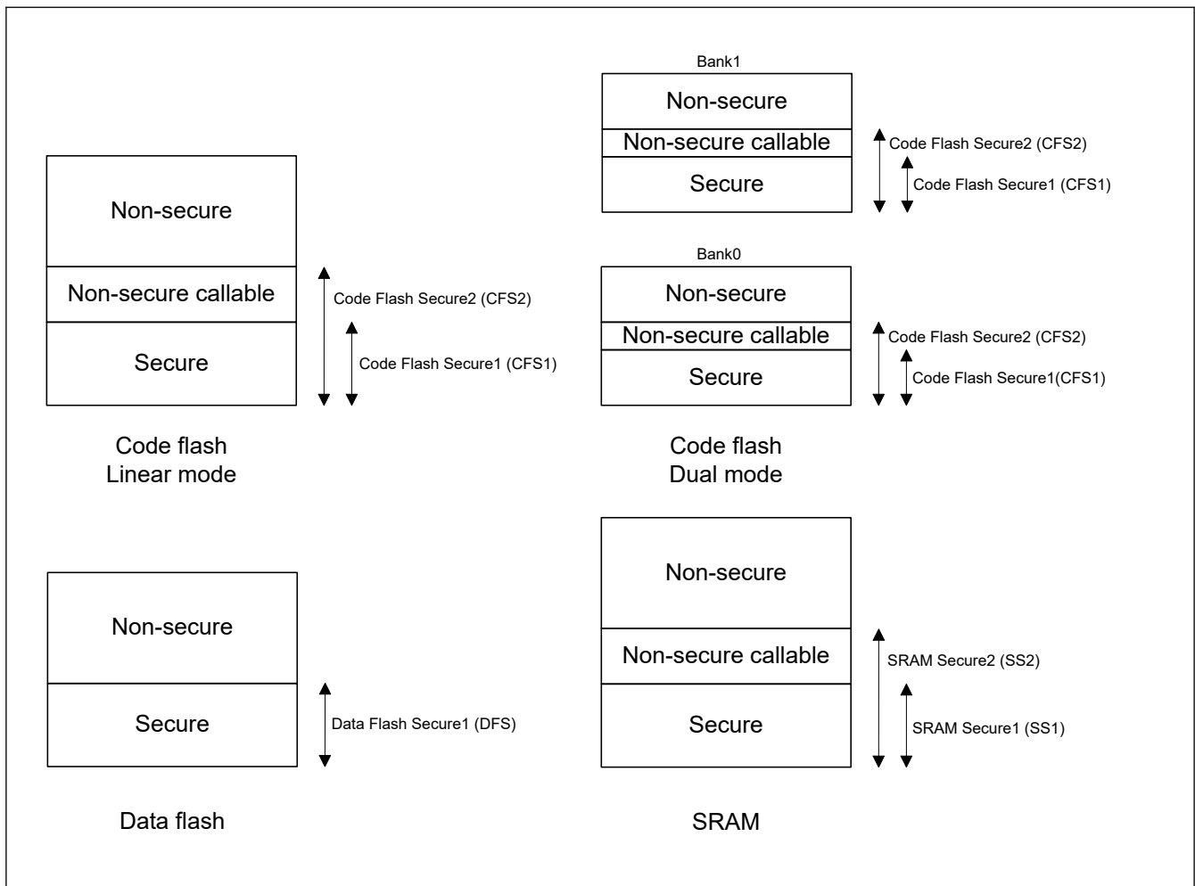
Figure 48.1 Memory mapping
