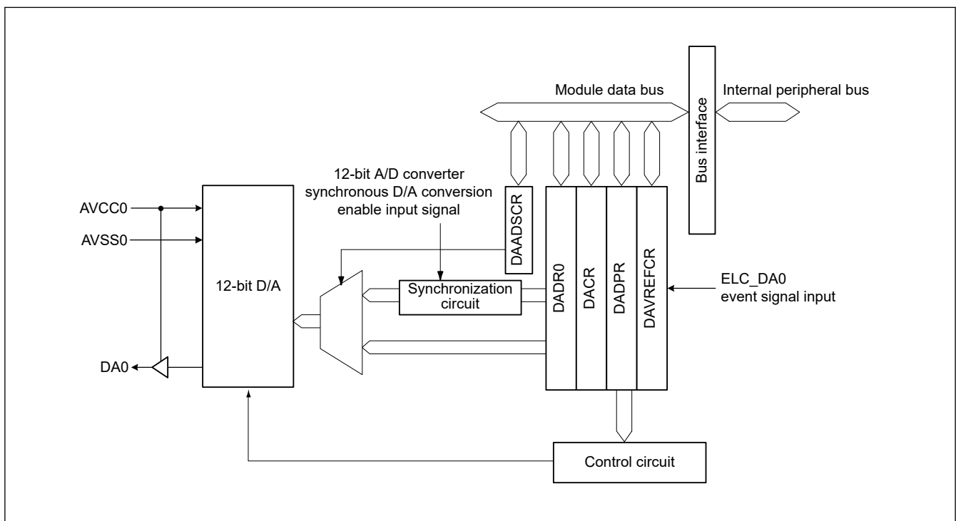
Figure 39.1 DAC12 block diagram
