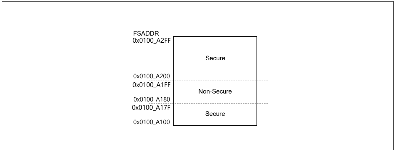
Figure 45.33 Secure/non-secure region in option-setting memory
