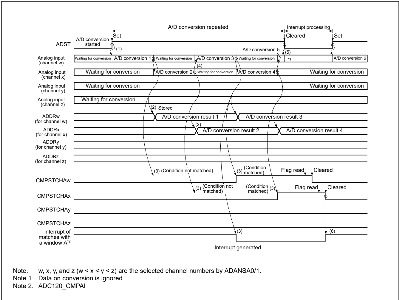
Figure 38.22 Example of compare function operation, when the analog inputs (channel w to z) are compared
