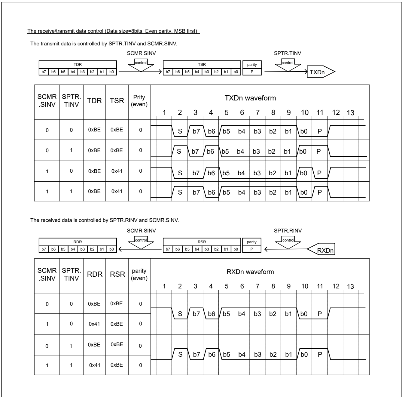
Figure 26.5 Example of the receive/transmit data control
