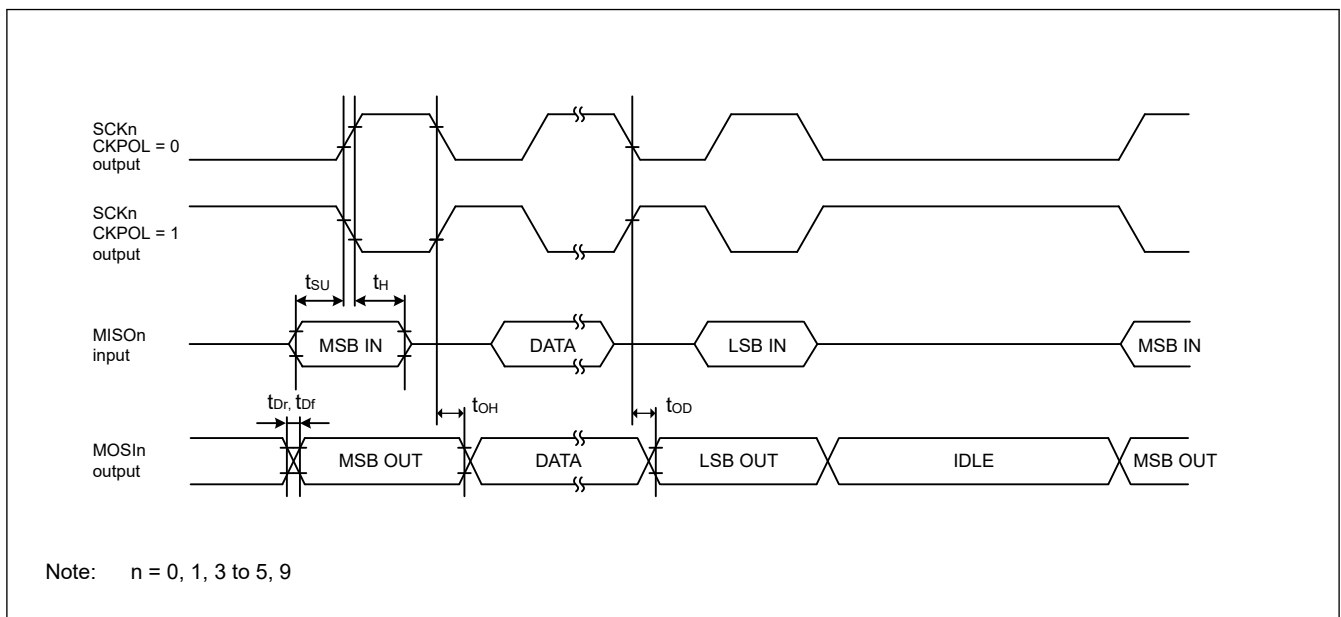
Figure 49.26 SCI simple SPI mode timing (master, CKPH = 1)
