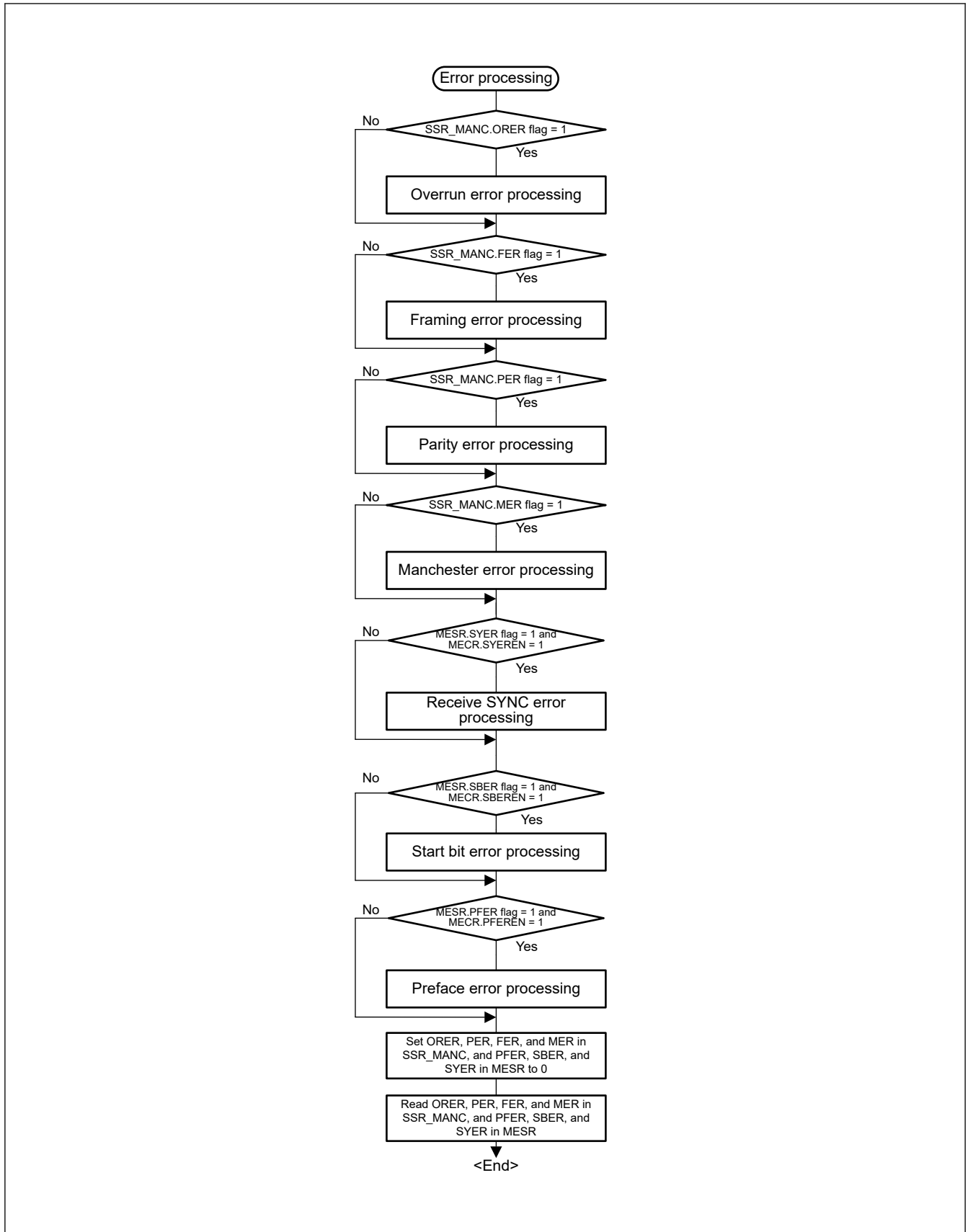
Figure 26.62 Example of Serial Reception Flowchart in Manchester Mode (Error Processing)
