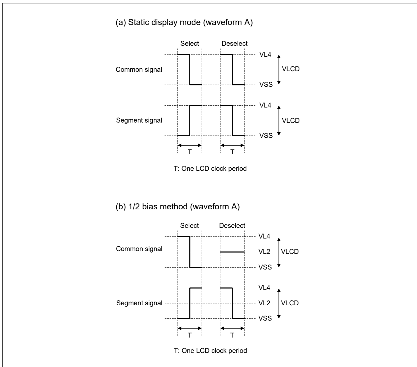
Figure 46.19 Voltages and phases of common and segment signals (1 of 3)
