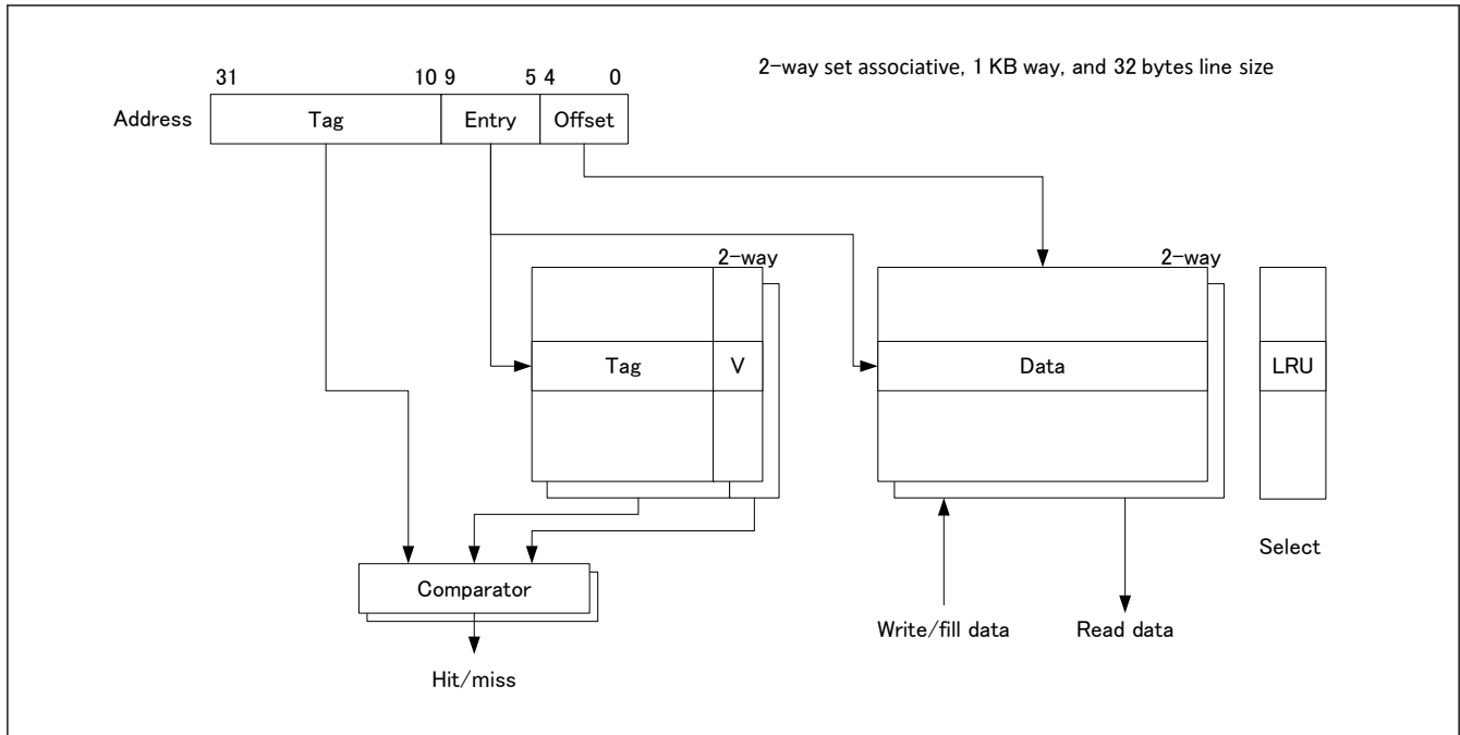
Figure 13.5 Cache structure for 2-way set associative of 2 KB capacity and 32 bytes line size
