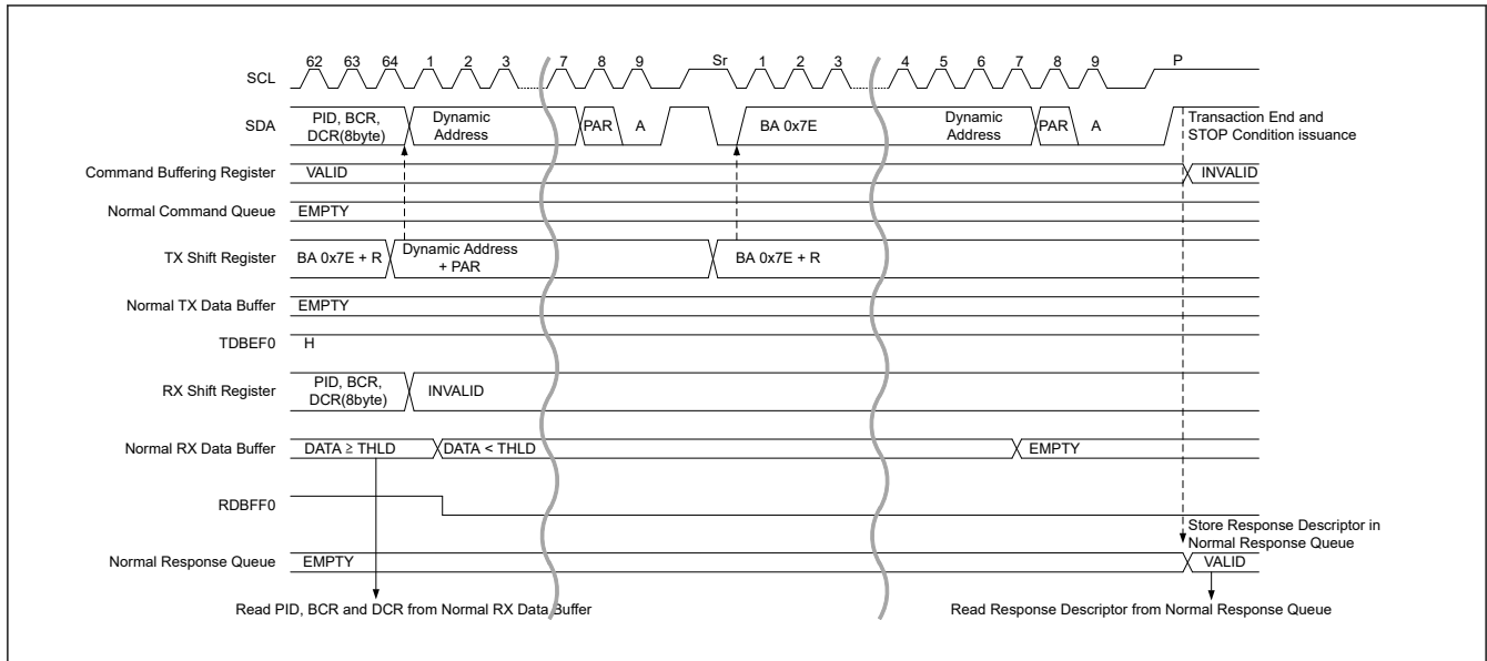
Figure 29.14 Dynamic address assign procedure (ENTDAA CCC) timing (3/3)
