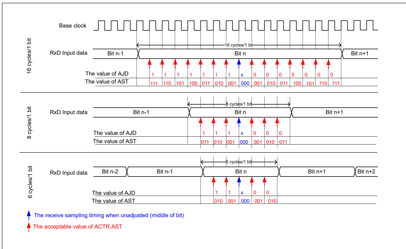
Figure 26.34 Overview of the adjustment operation for the reception sampling timing (asynchronous mode using internal clock)
