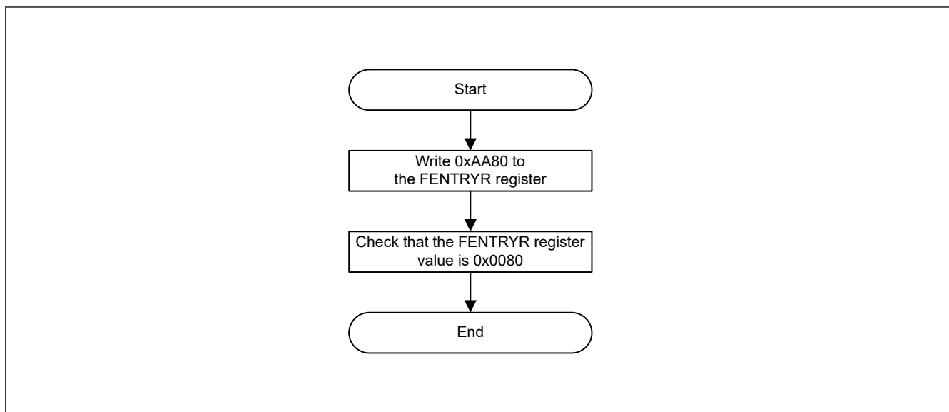
Figure 45.11 Procedure to transition to data flash P/E mode from read mode
