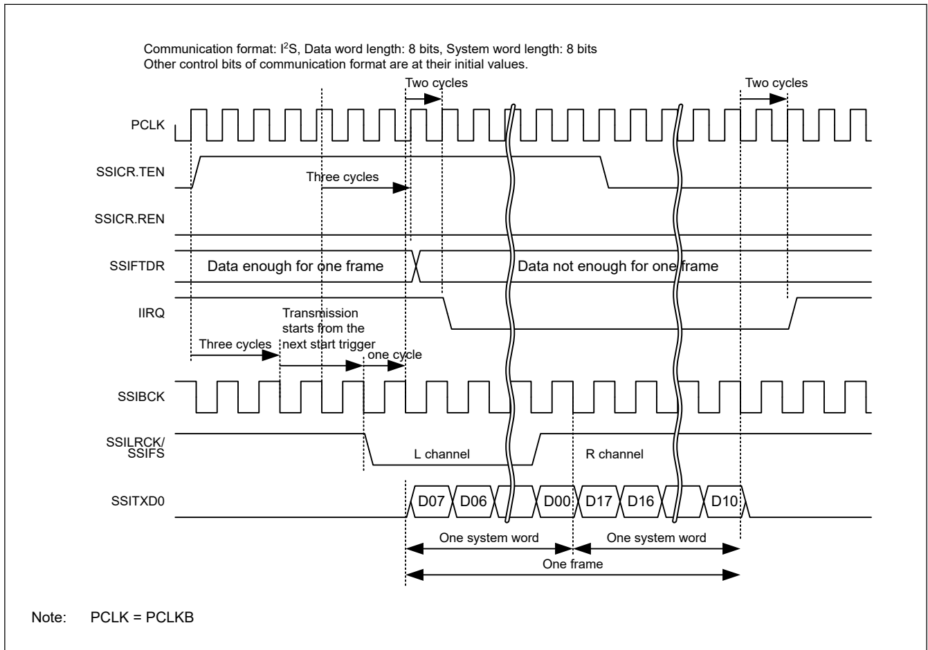
Figure 35.13 IIRQ setting timing (transmission)
