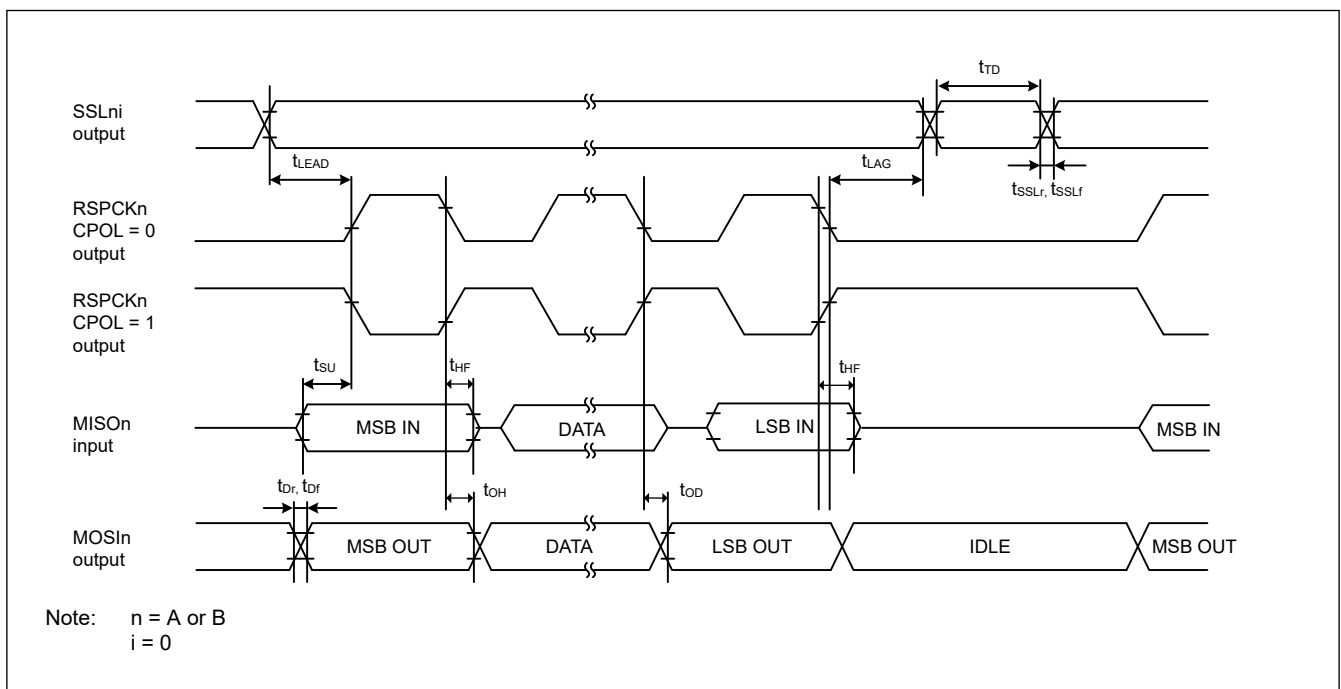
Figure 49.33 SPI timing (master, CPHA = 0) (bit rate: PCLKB division ratio is set to 1/2)
