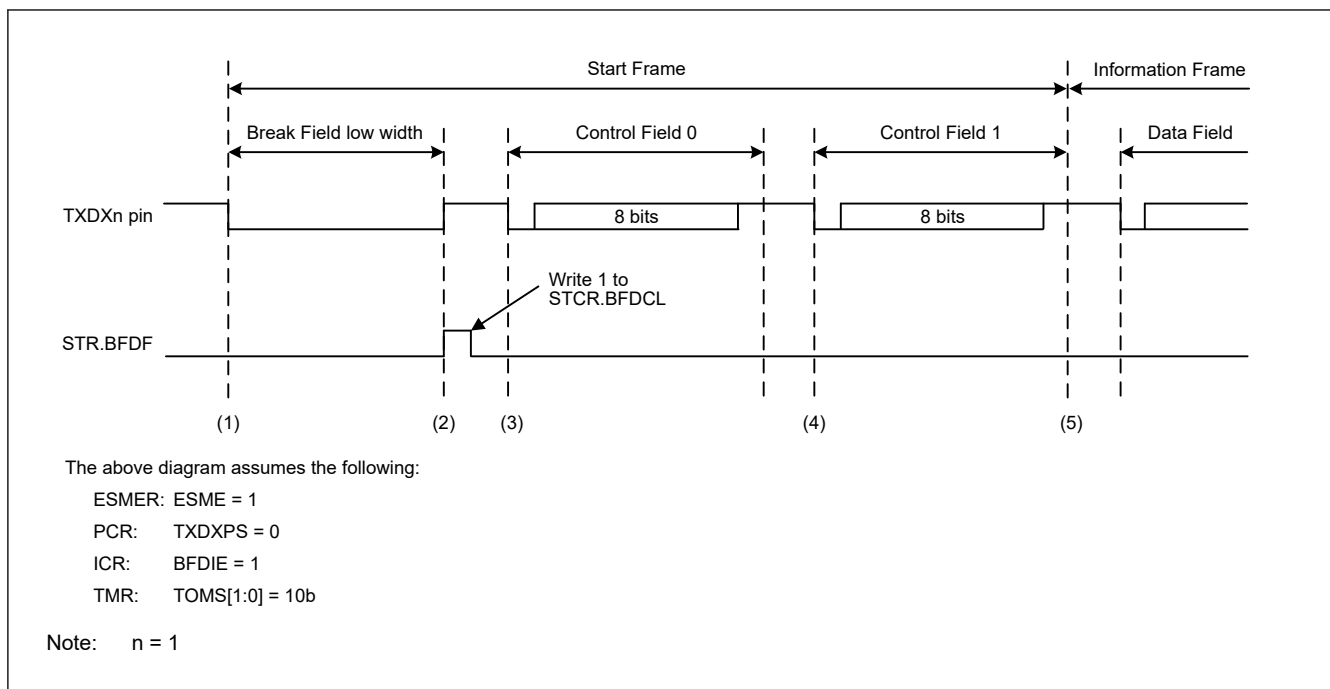
Figure 26.102 Example of operations when transmitting a Start Frame
