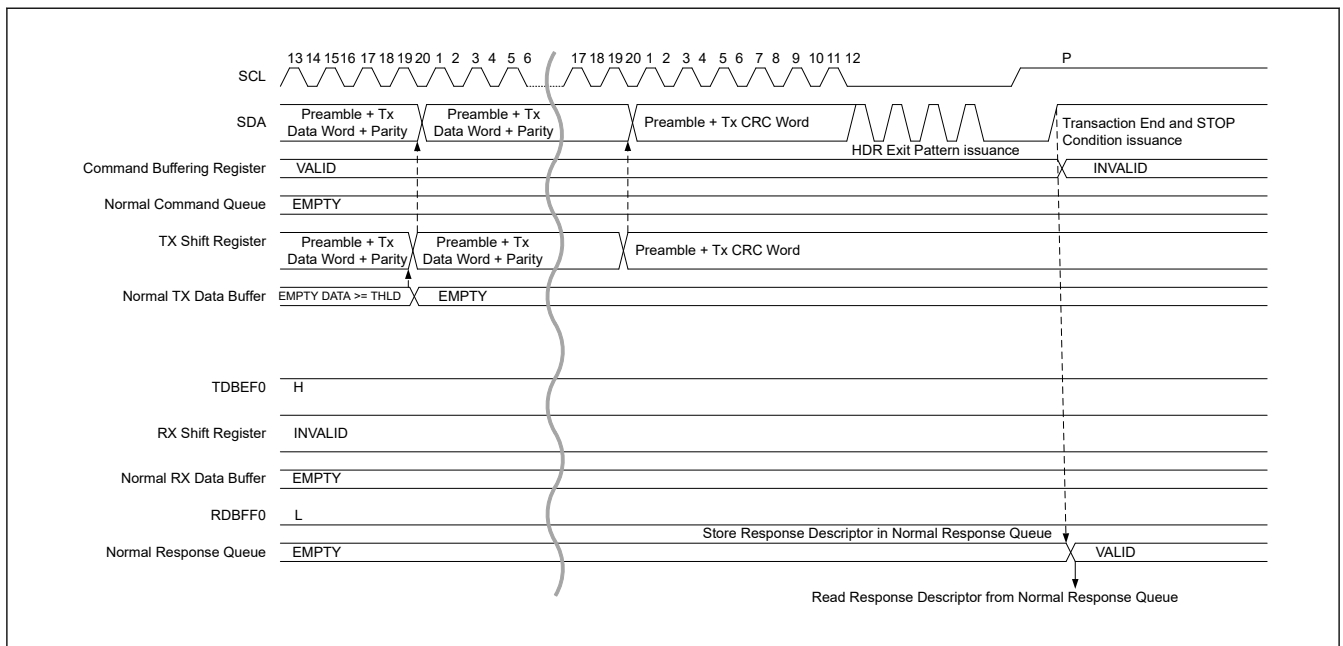
Figure 29.27 HDR data write transfer (HDR-DDR) timing (4/4)
