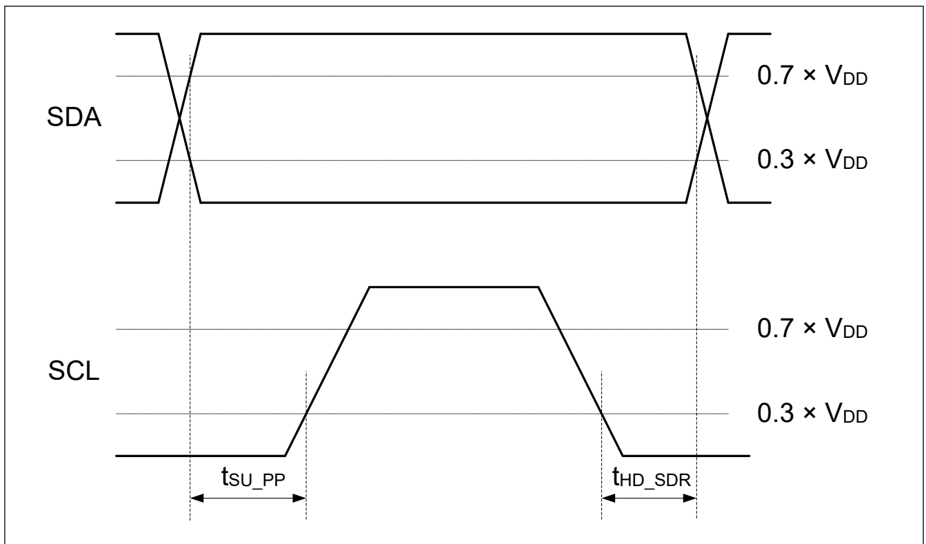
Figure 49.49 Master SDR timing
