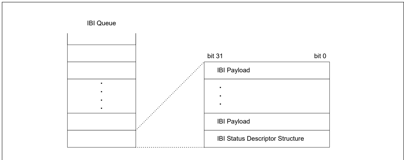
Figure 29.4 IBI status descriptor data structure
