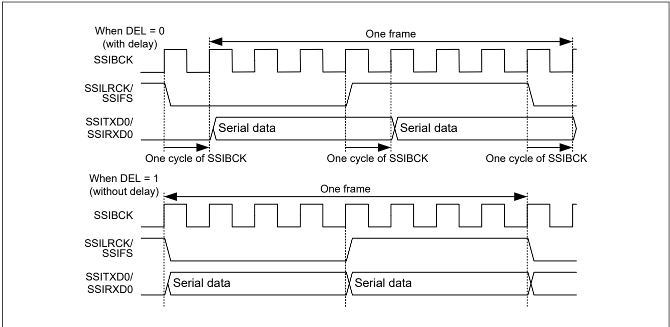
Figure 35.6 Setting of delay in serial data
