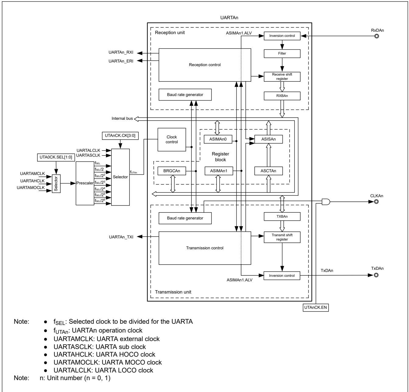
Figure 30.1 Block diagram of UARTn
