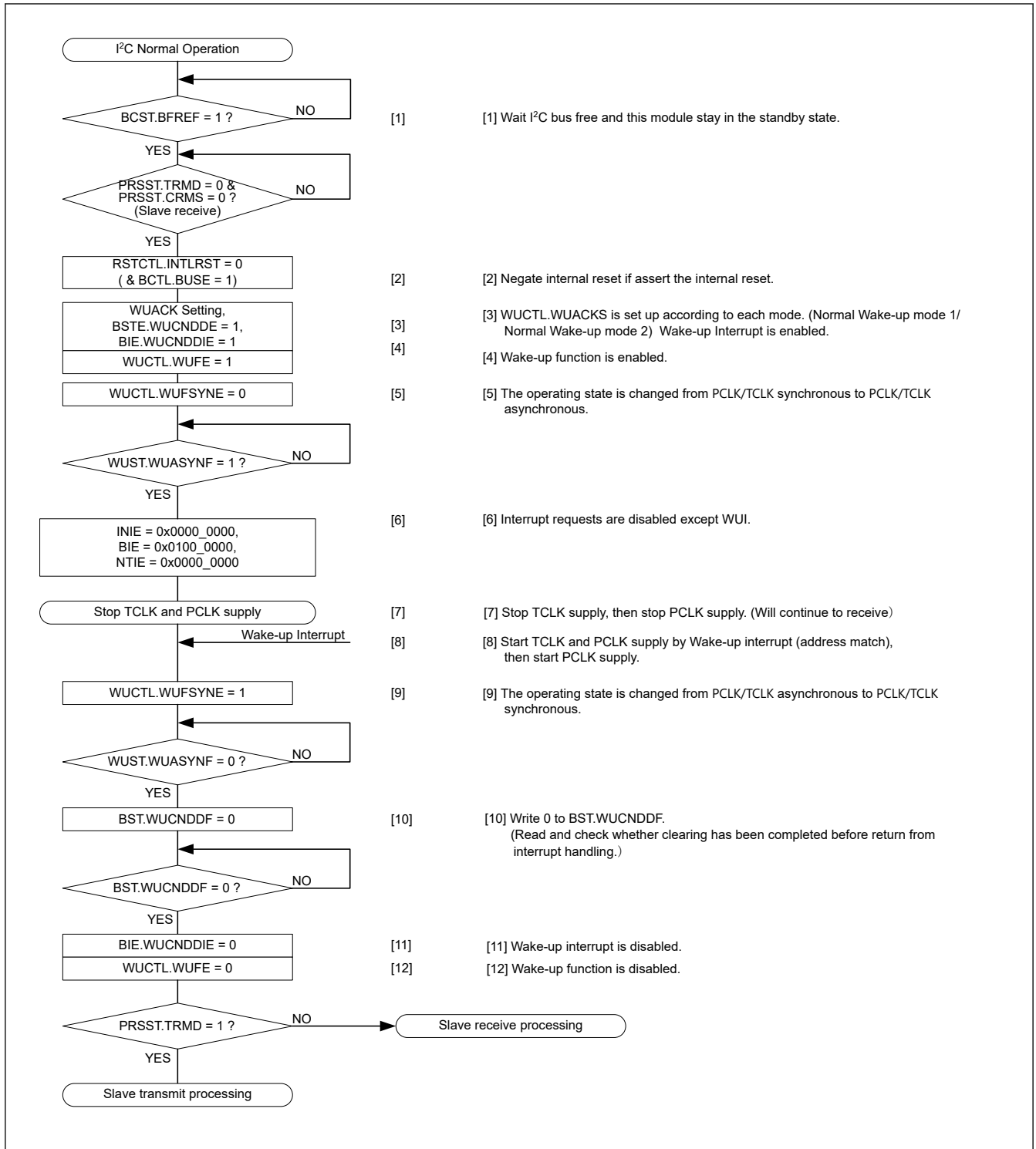
Figure 29.127 Use case of normal WU mode 2 (Wake-up recovery by a Wake-up interrupt triggered by the match of the slave address)
