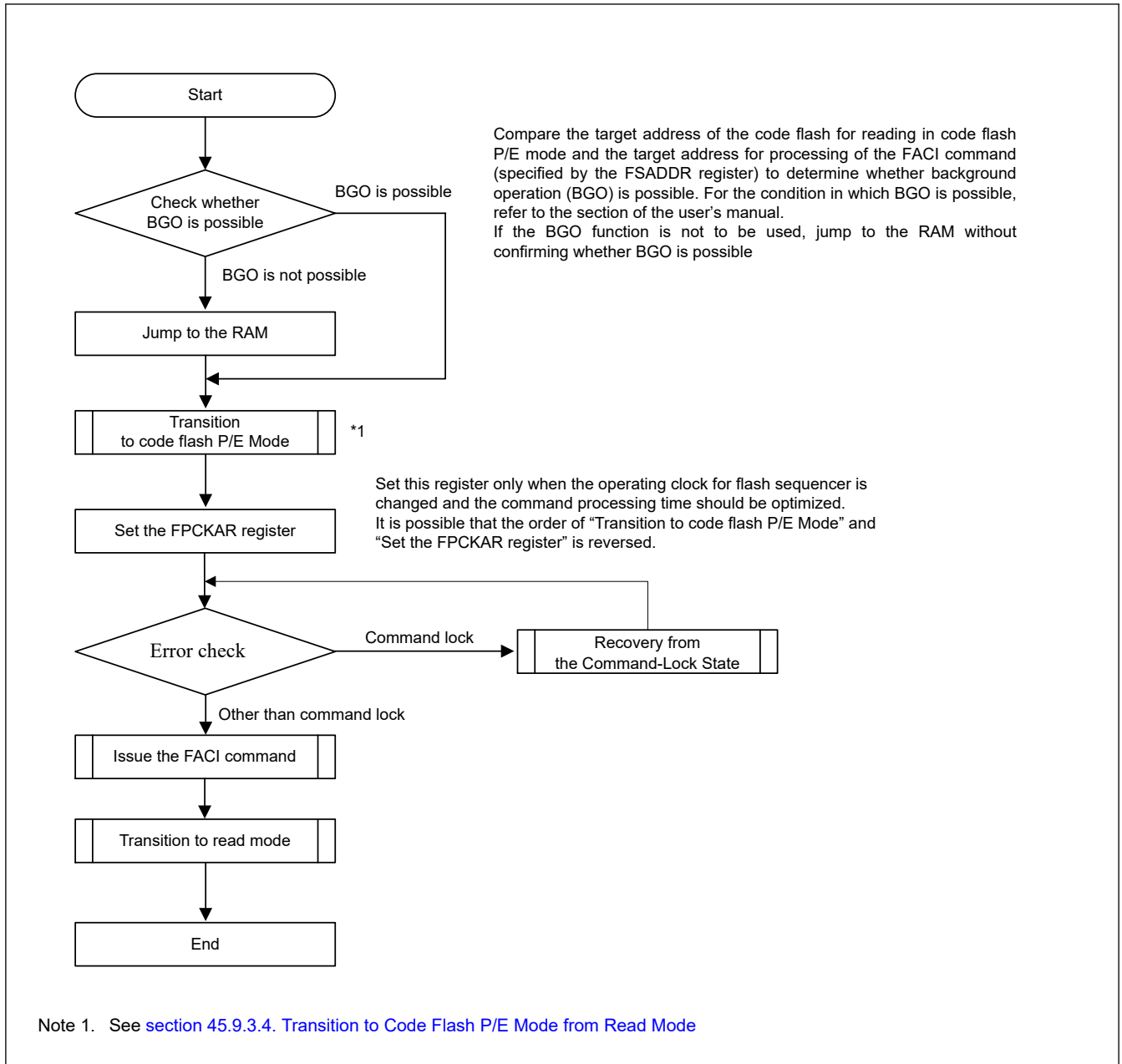
Figure 45.7 Overview of command usage in code flash P/E mode
