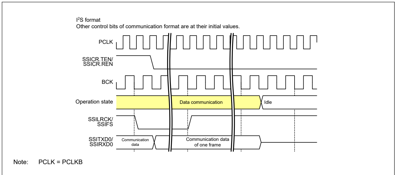
Figure 35.47 Halt from the data communication (without padding bits)
