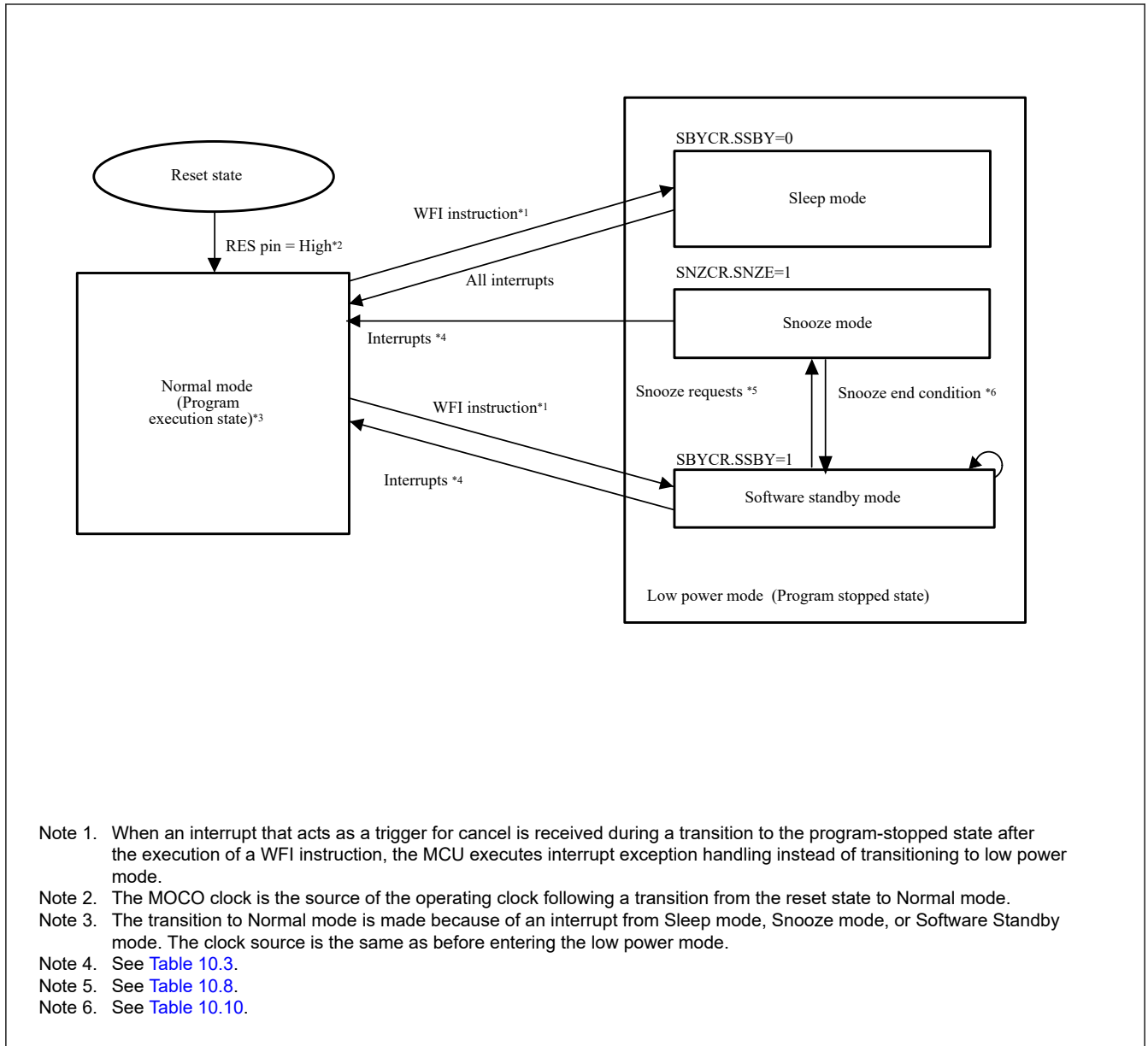
Figure 10.1 Mode transitions
