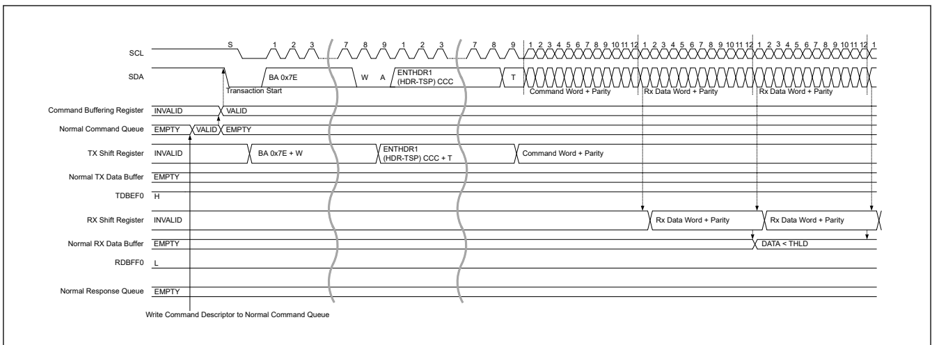
Figure 29.32 HDR data read transfer (HDR-TSP, TSL) timing (1/2)
