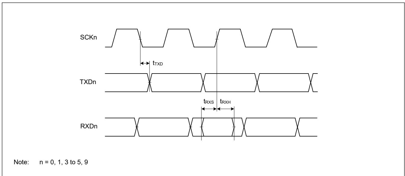
Figure 49.24 SCI input/output timing in clock synchronous mode
