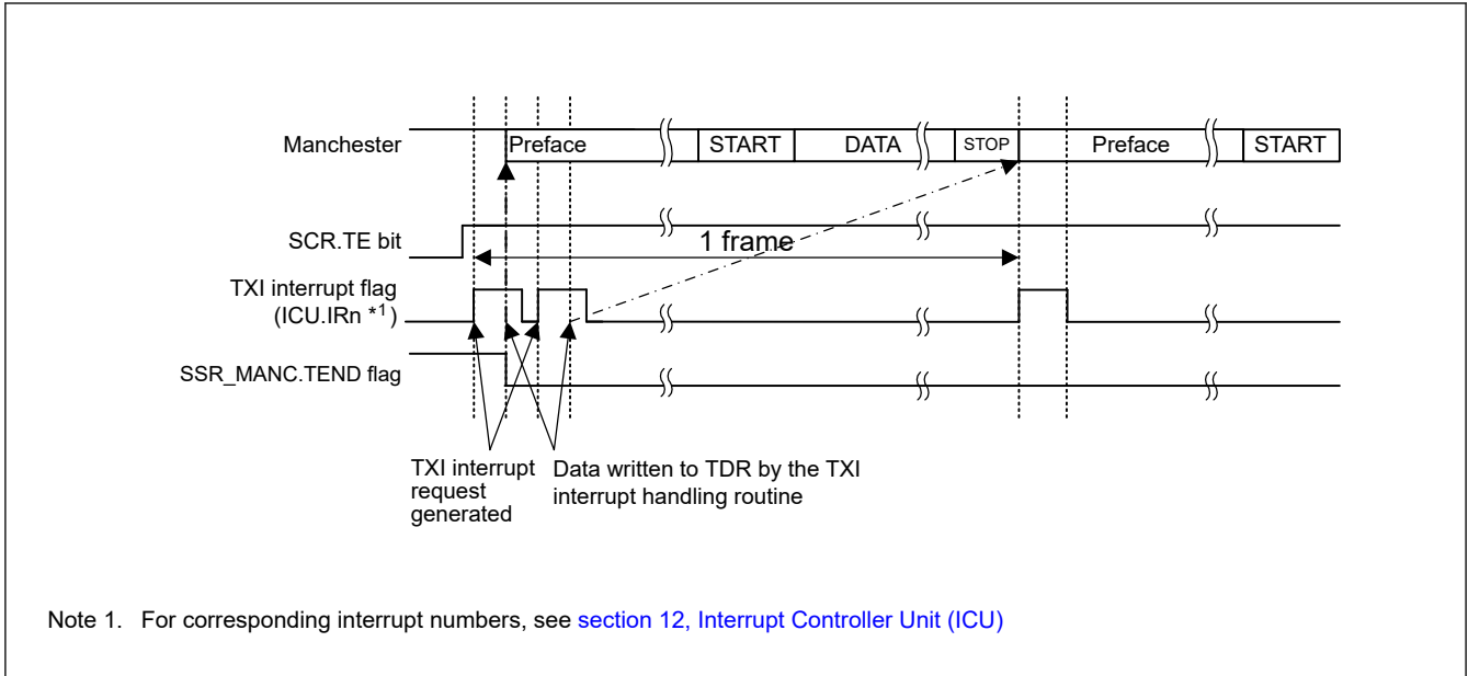
Figure 26.56 Example of Start-of-Transmission Operation for Serial Transmission in Manchester mode (with Preface but Without the CTS Function)
