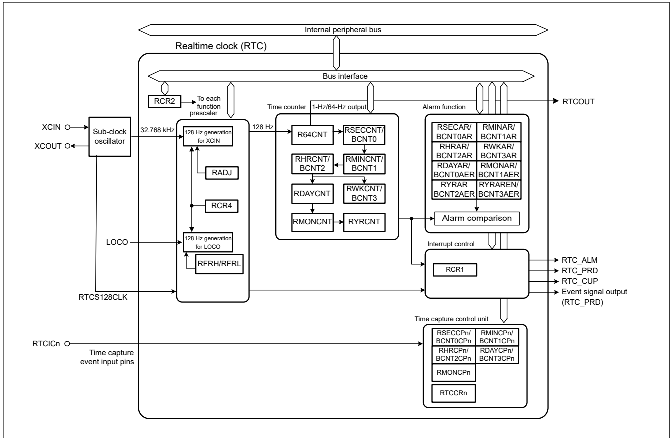
Figure 22.1 RTC block diagram
