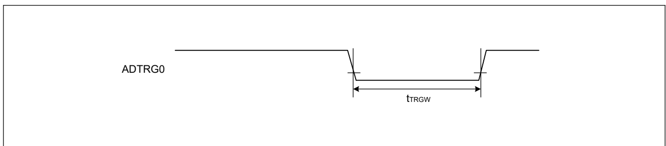
Figure 49.22 ADC12 trigger input timing
