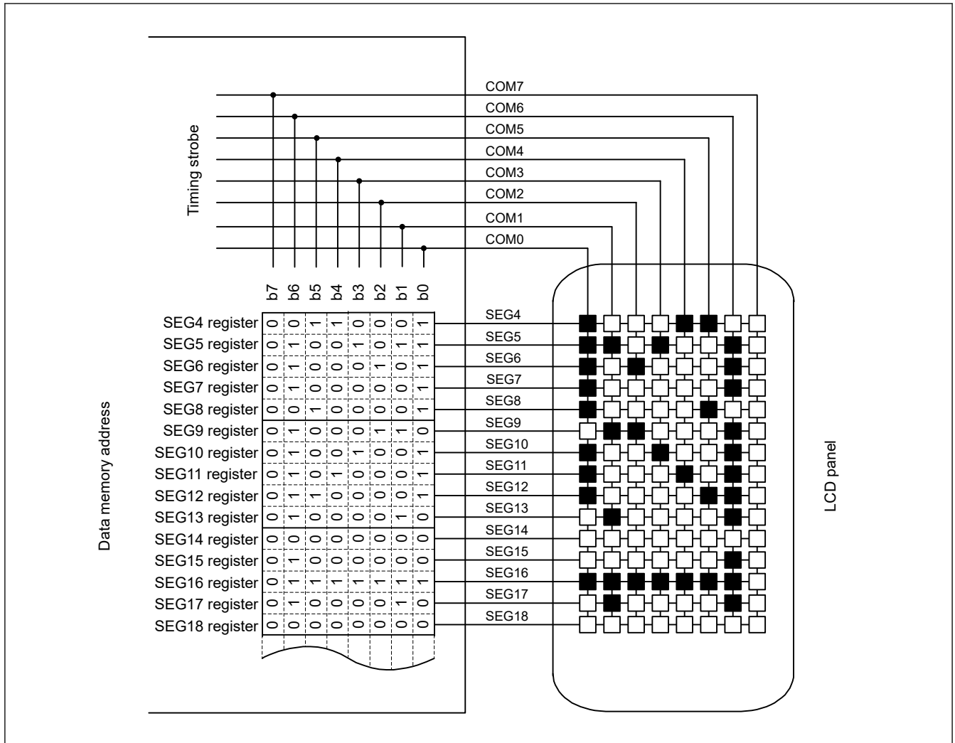
Figure 46.41 Example of connecting eight-time slice LCD panel
