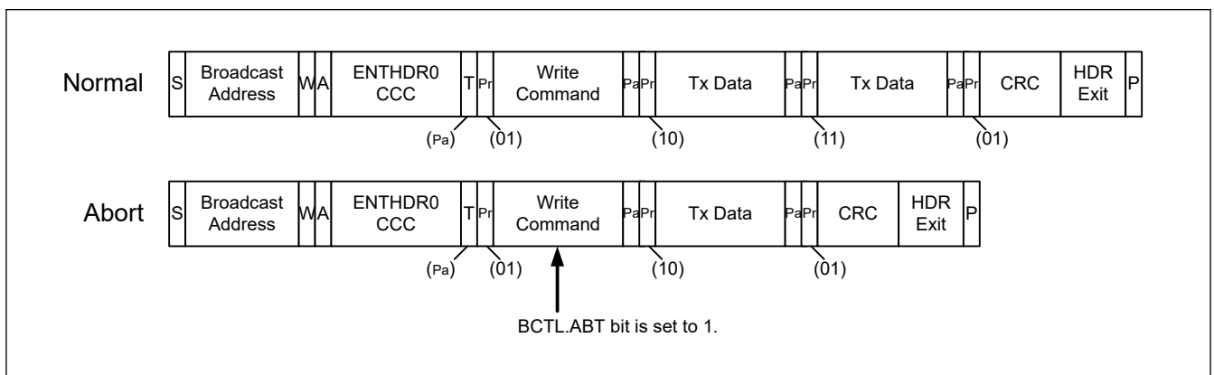
Figure 29.116 Abort operation of HDR-DDR write transfer
