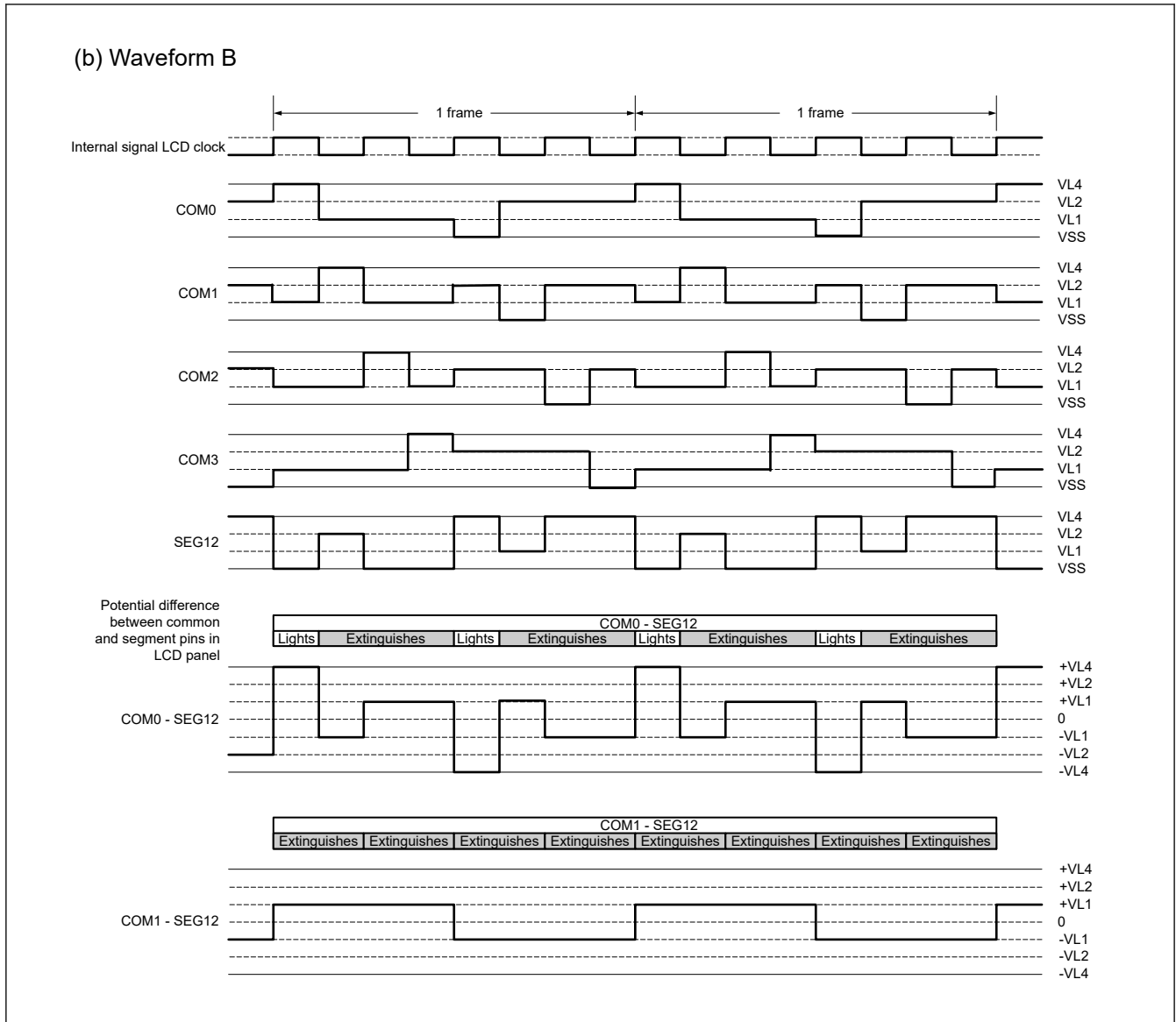
Figure 46.35 Four-time slice LCD drive waveform examples between SEG12 and each common signal using 1/3 bias method (2 of 2)
