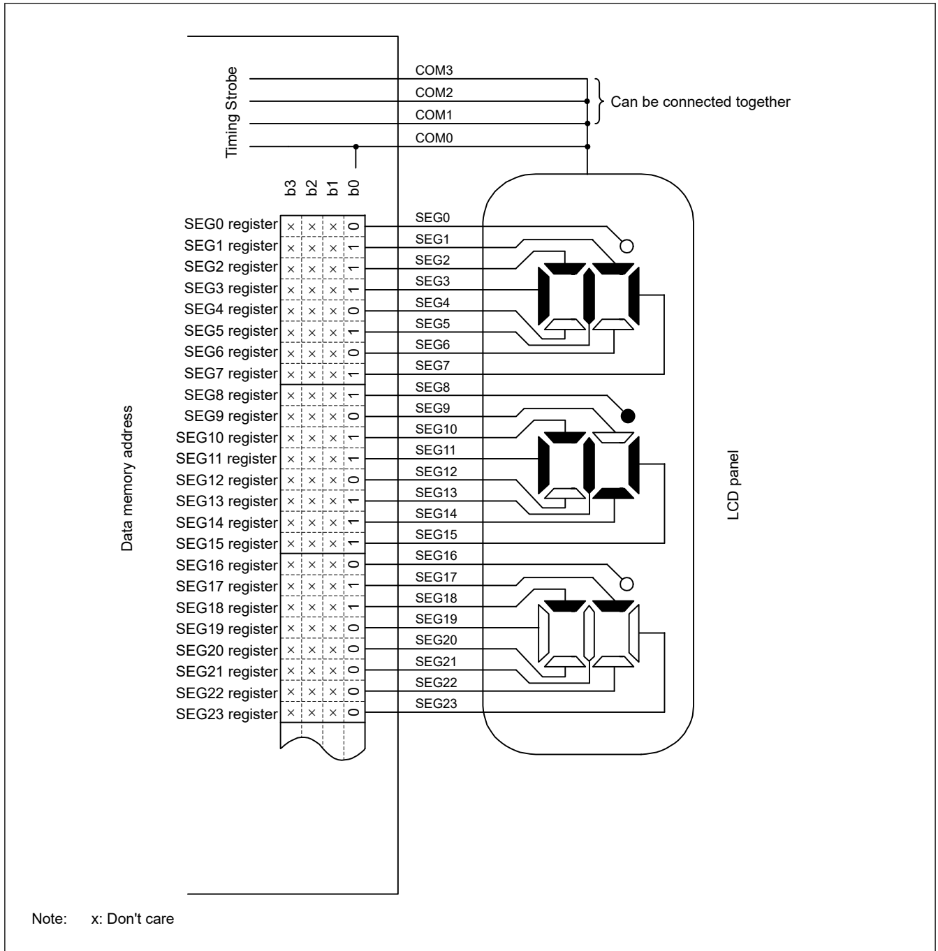
Figure 46.23 Example of connecting static LCD panel
