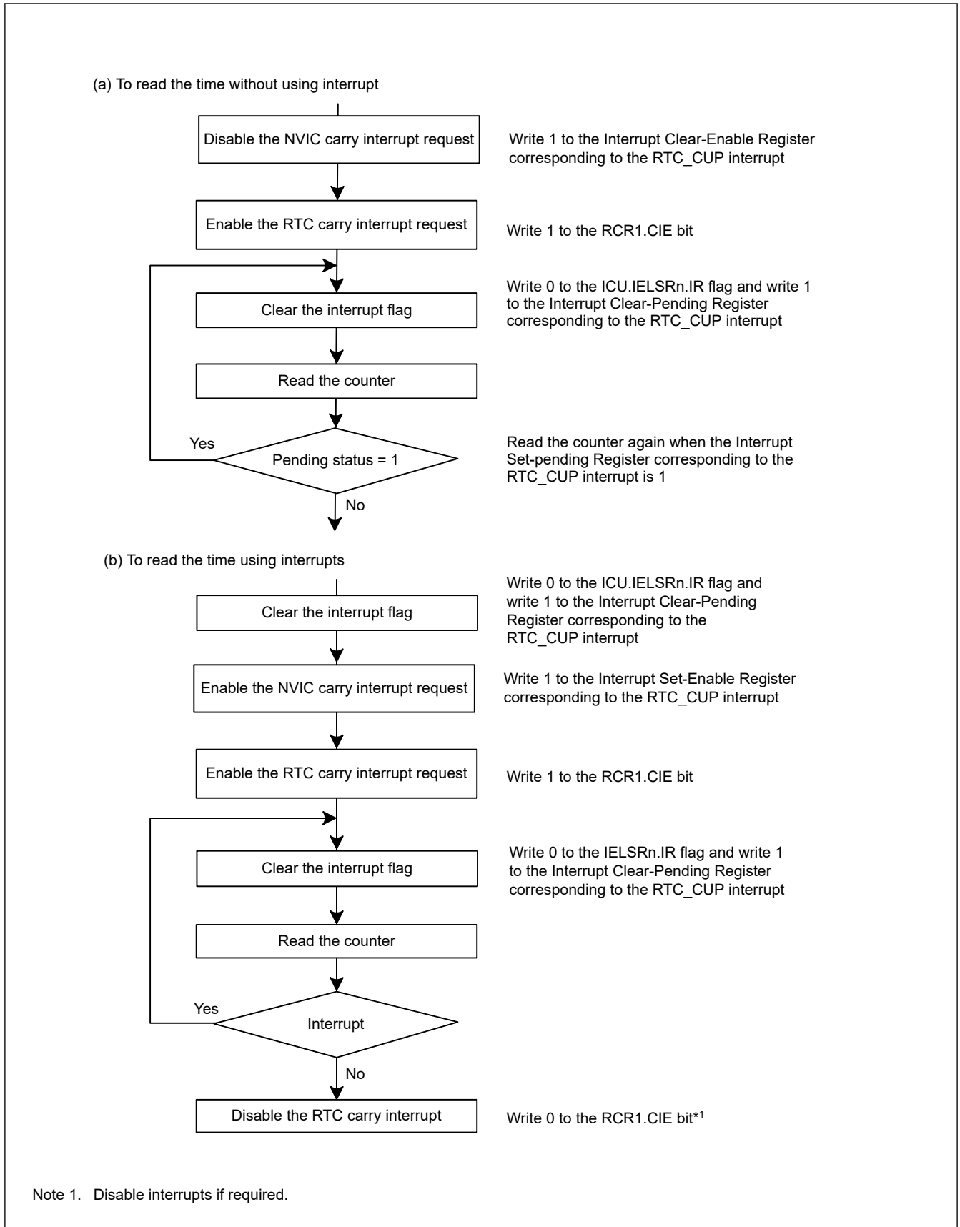
Figure 22.5 Reading time
