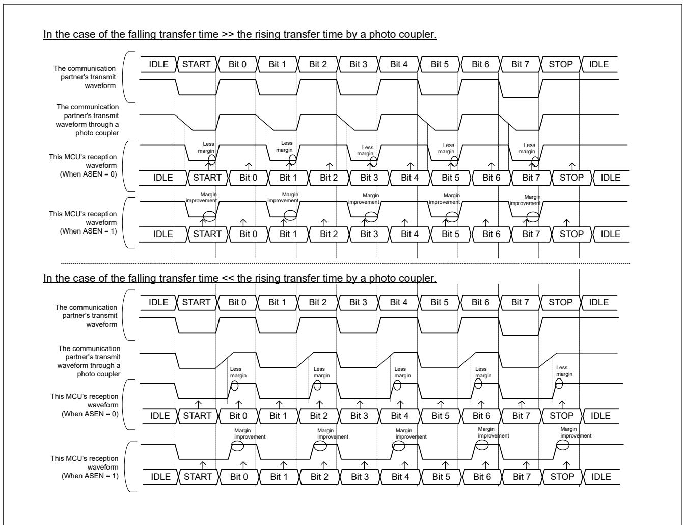
Figure 26.33 Example of improvement in reception margin by the reception sampling timing adjustment function
