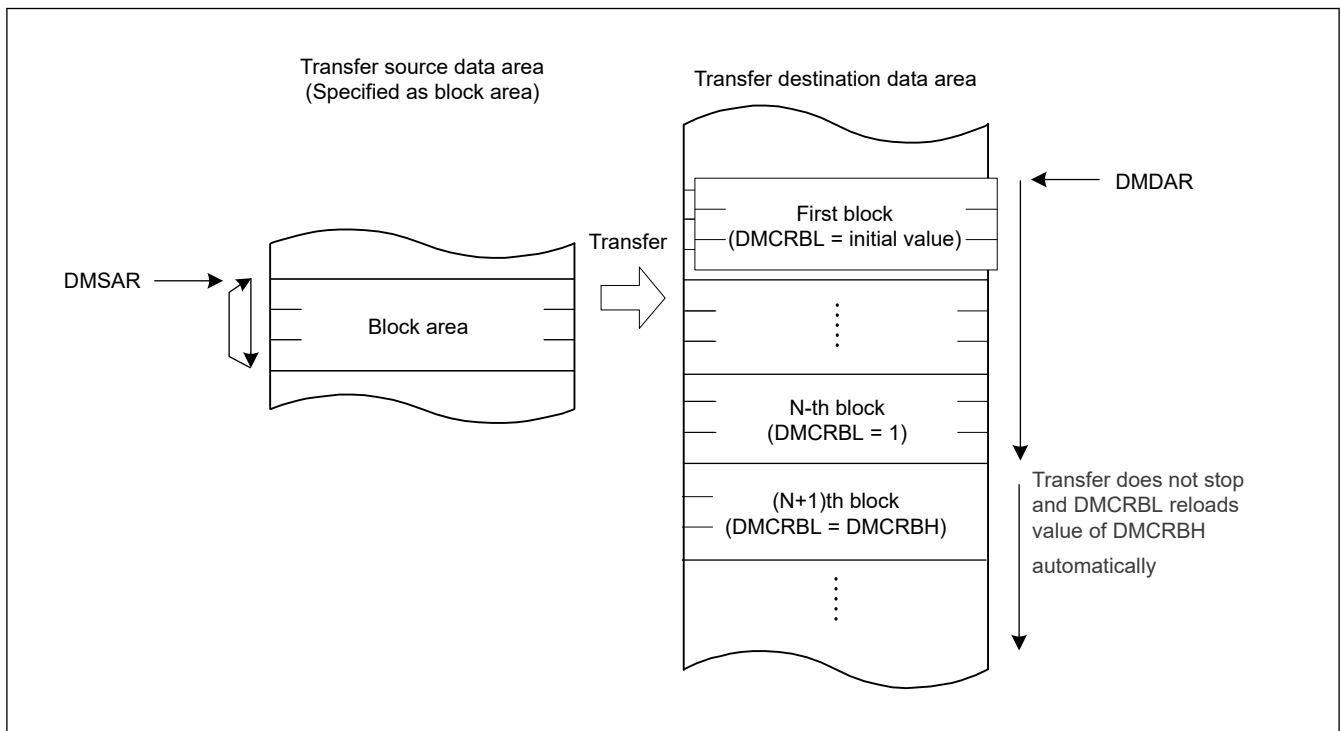
Figure 15.10 Operation in block transfer mode when DMTMD.TKP bit is set to 1
