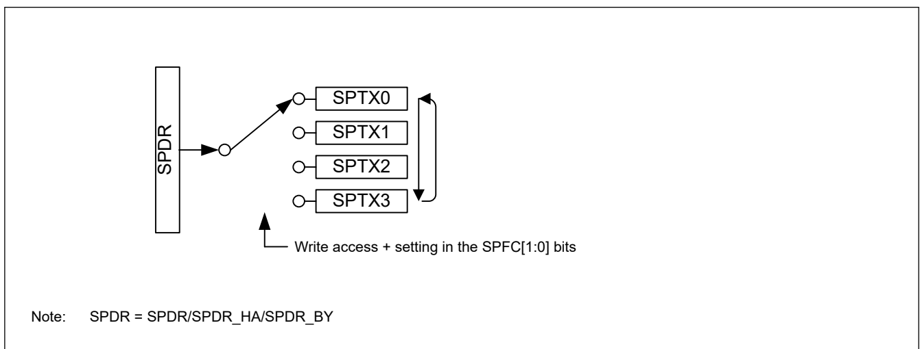
Figure 33.3 Configuration of SPDR/SPDR_HA/SPDR_BY for write access
