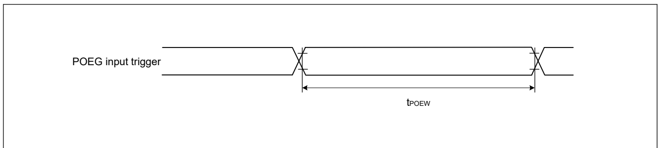
Figure 49.19 POEG input trigger timing
