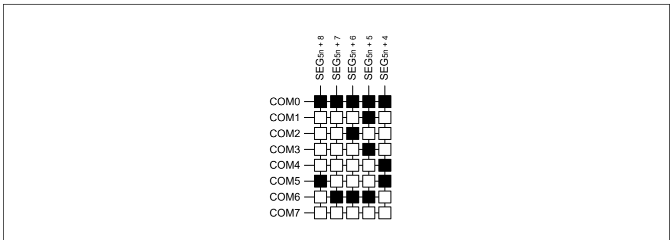
Figure 46.40 Eight-time slice LCD display pattern and electrode connections
