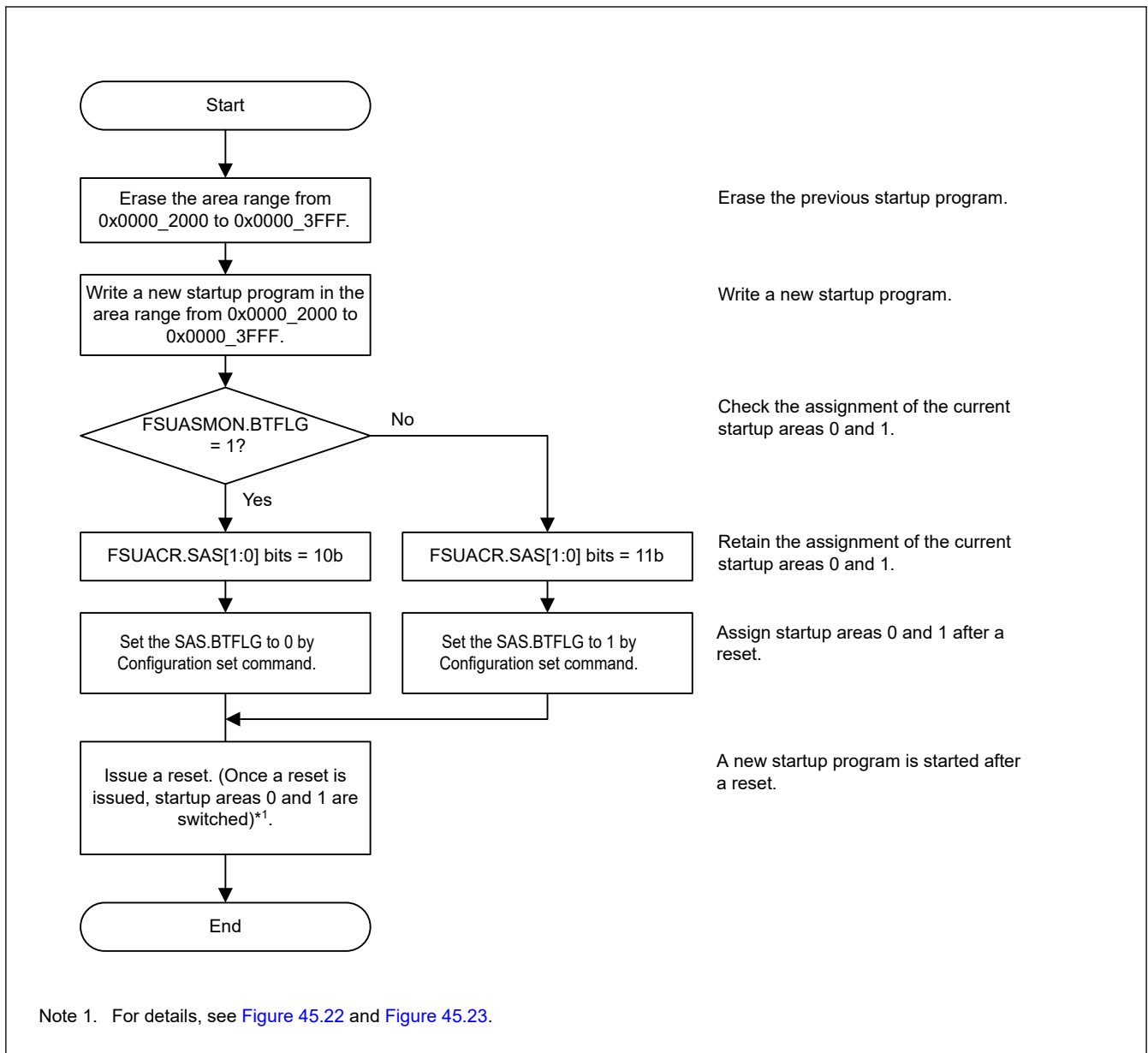
Figure 45.24 Concept of protection of the startup program
