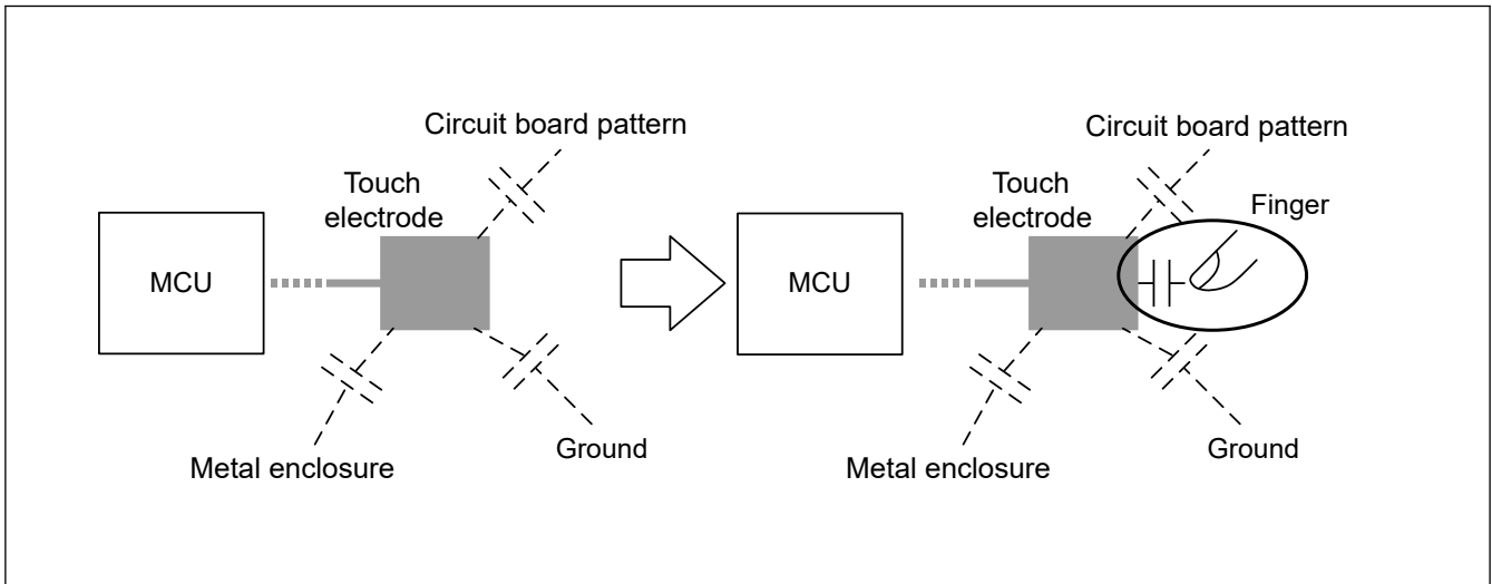
Figure 42.1 Increased electrostatic capacitance because of the presence of a finger
