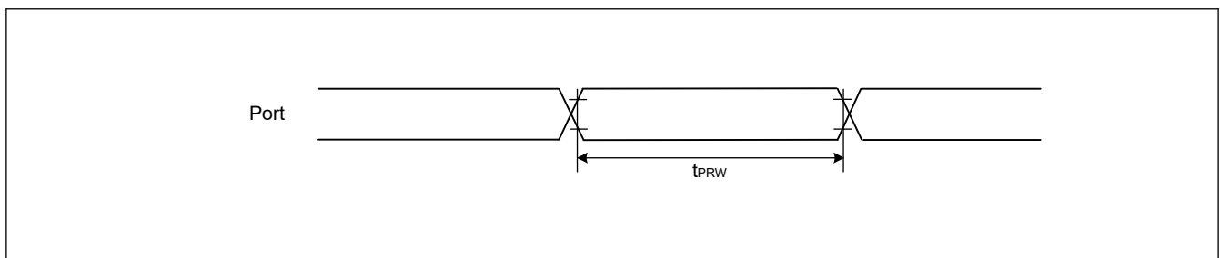
Figure 49.18 I/O ports input timing
