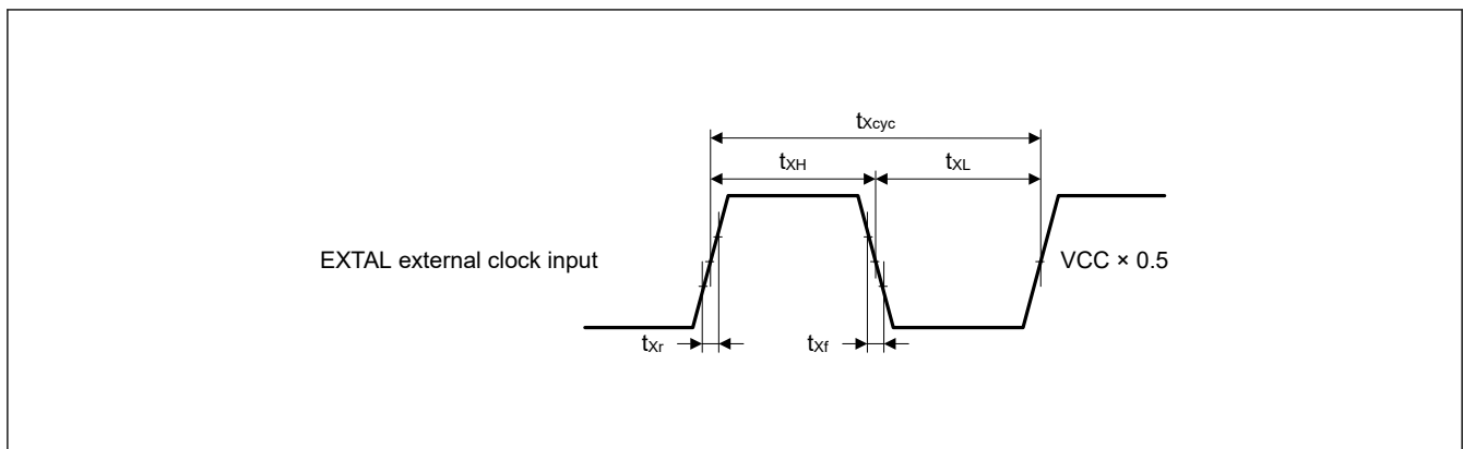
Figure 49.6 EXTAL external clock input timing
