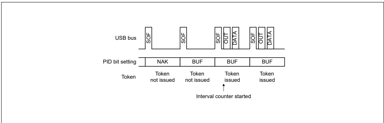
Figure 25.12 Token issuance when IITV = 0
