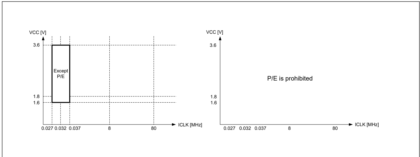
Figure 10.5 Operating voltages and frequencies in Subosc-speed mode
