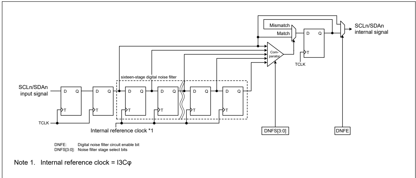
Figure 29.137 Block diagram of digital noise filter circuit
