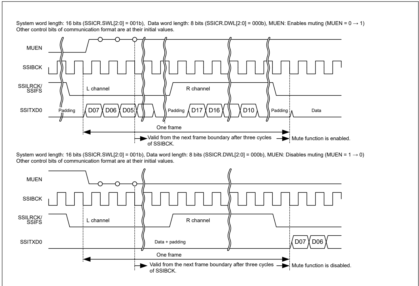
Figure 35.4 Transmit data with the mute function set
