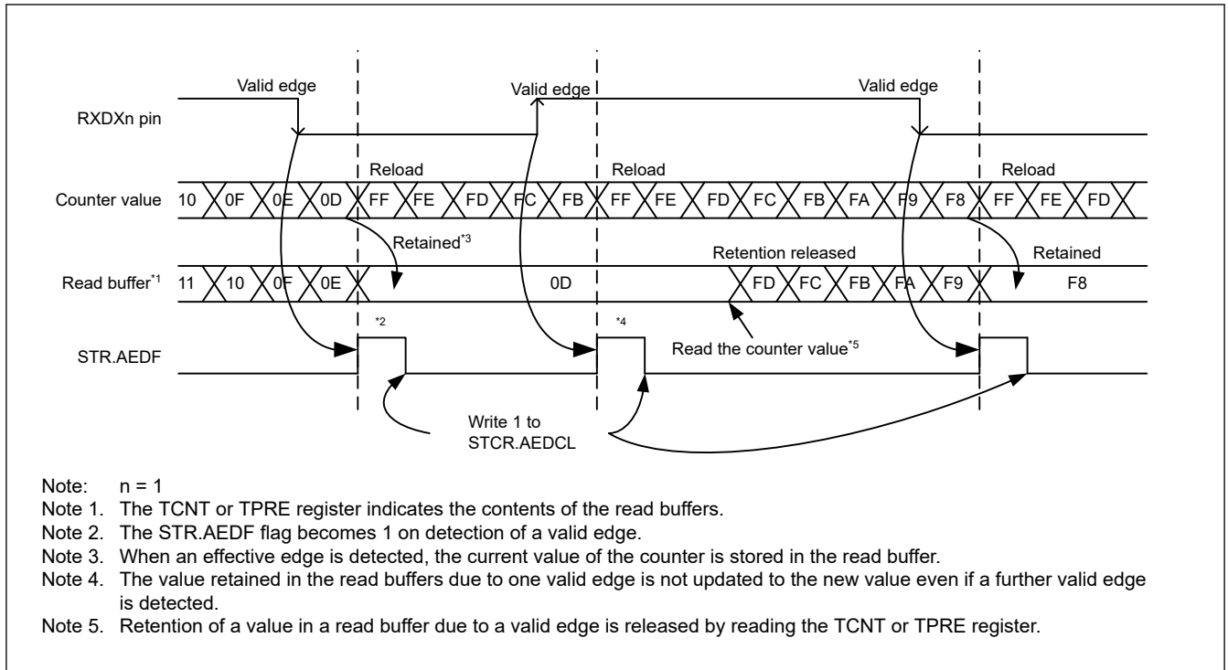
Figure 26.113 Example of operations for bit rate measurement
