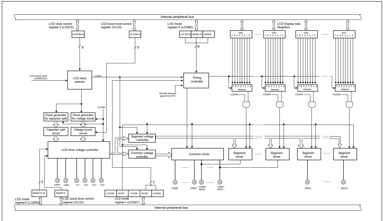
Figure 46.1 SLCDC block diagram
