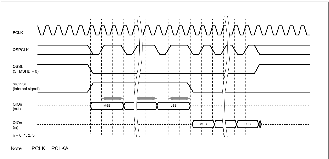
Figure 34.16 Hold time adjustment for serial data output using the SFMOHW bit
