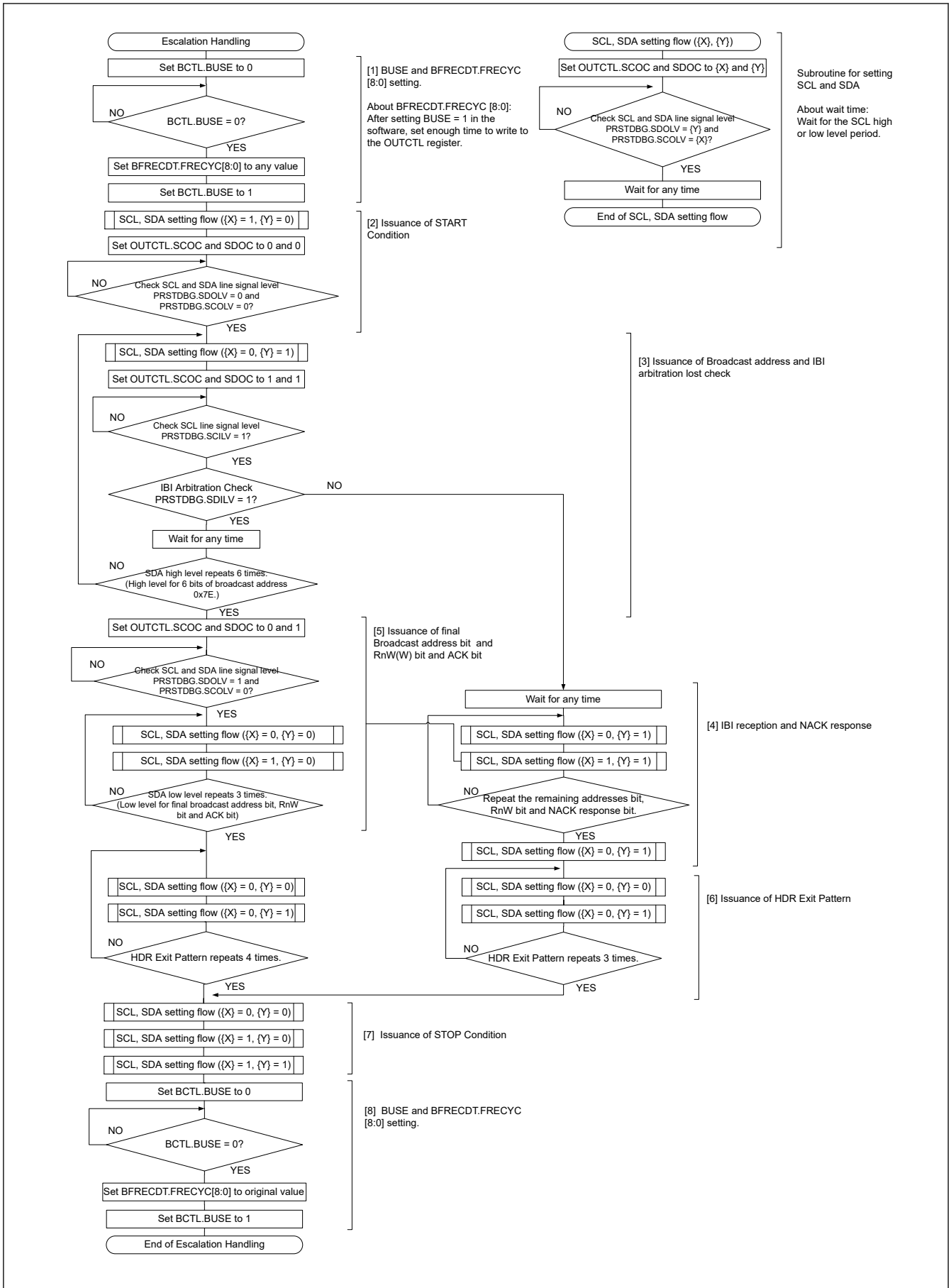
Figure 29.122 Escalation handling flowchart for I3C master
