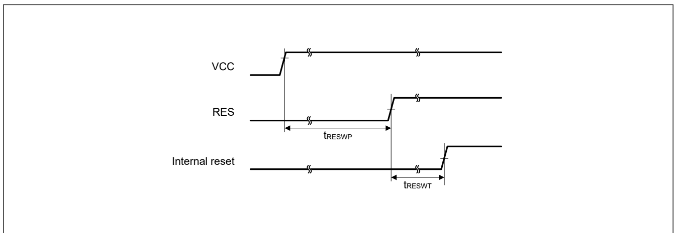
Figure 49.11 Reset input timing at power-on
