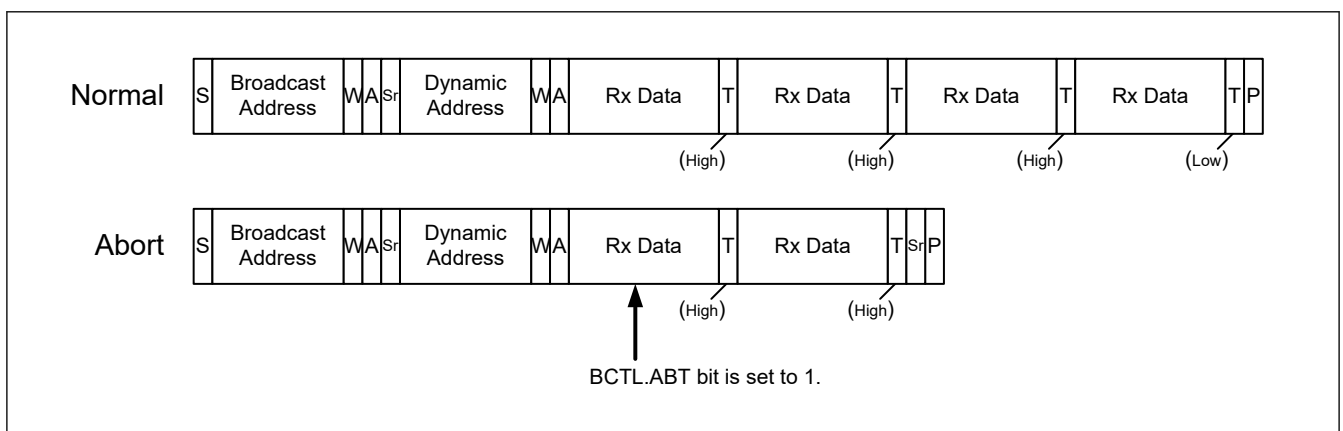
Figure 29.115 Abort operation of SDR read transfer
