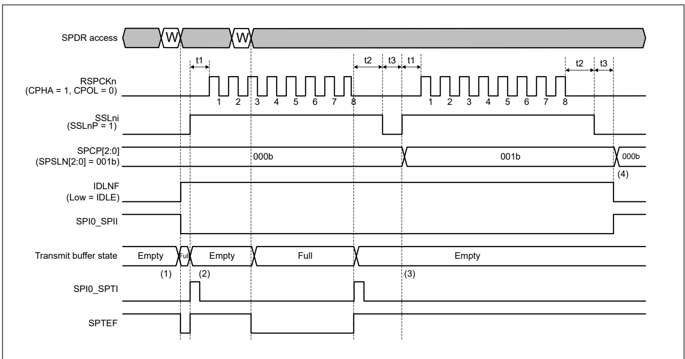
Figure 33.31 Example of idle interrupt operation (master mode)
