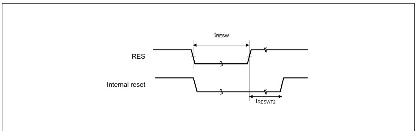
Figure 49.12 Reset input timing (1)
