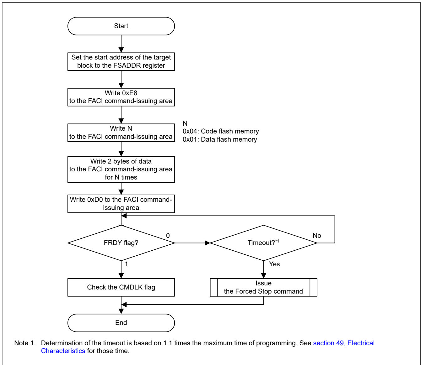
Figure 45.14 Usage flow of the program command
