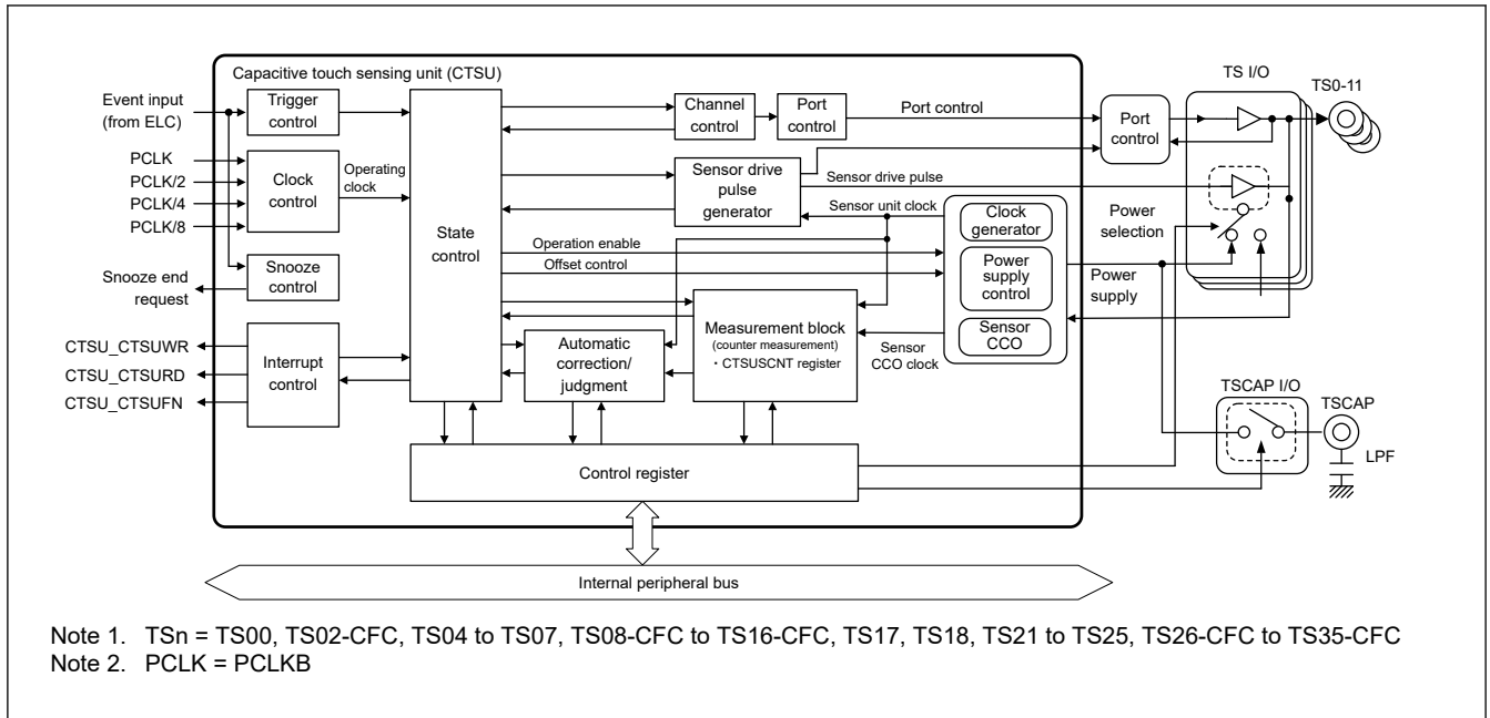
Figure 42.3 CTSU block diagram
