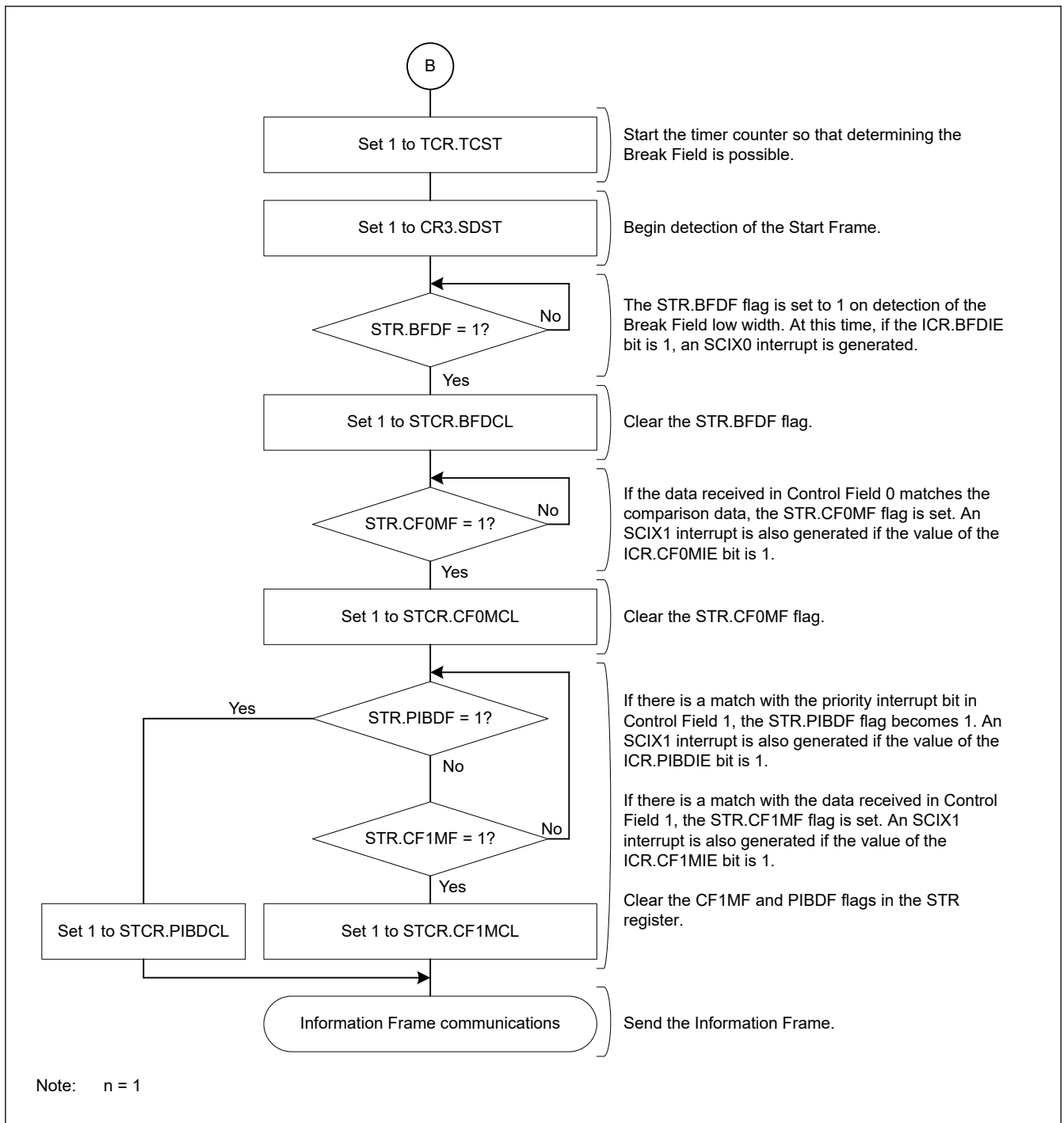
Figure 26.108 Sample flowchart for reception of a Start Frame (2)
