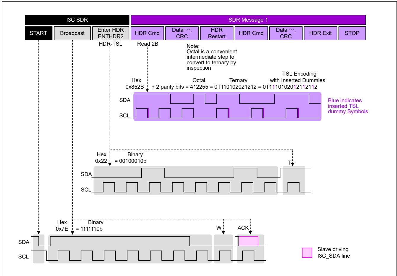
Figure 29.75 Example communication using HDR-TSL protocol
