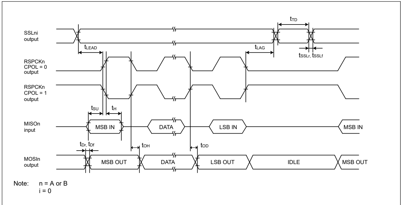
Figure 49.32 SPI timing (master, CPHA = 0) (bit rate: PCLKB division ratio is set to any value other than 1/2)
