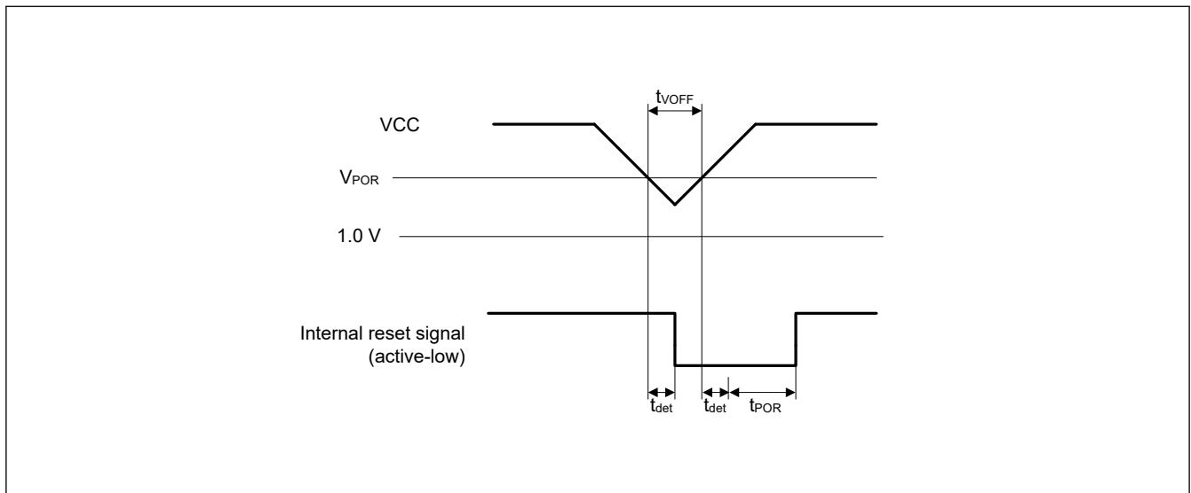
Figure 49.65 Voltage detection reset timing
