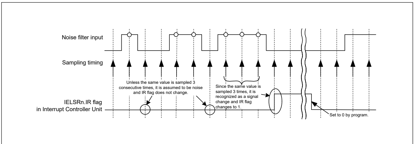
Figure 41.6 Noise filter and interrupt operation example
