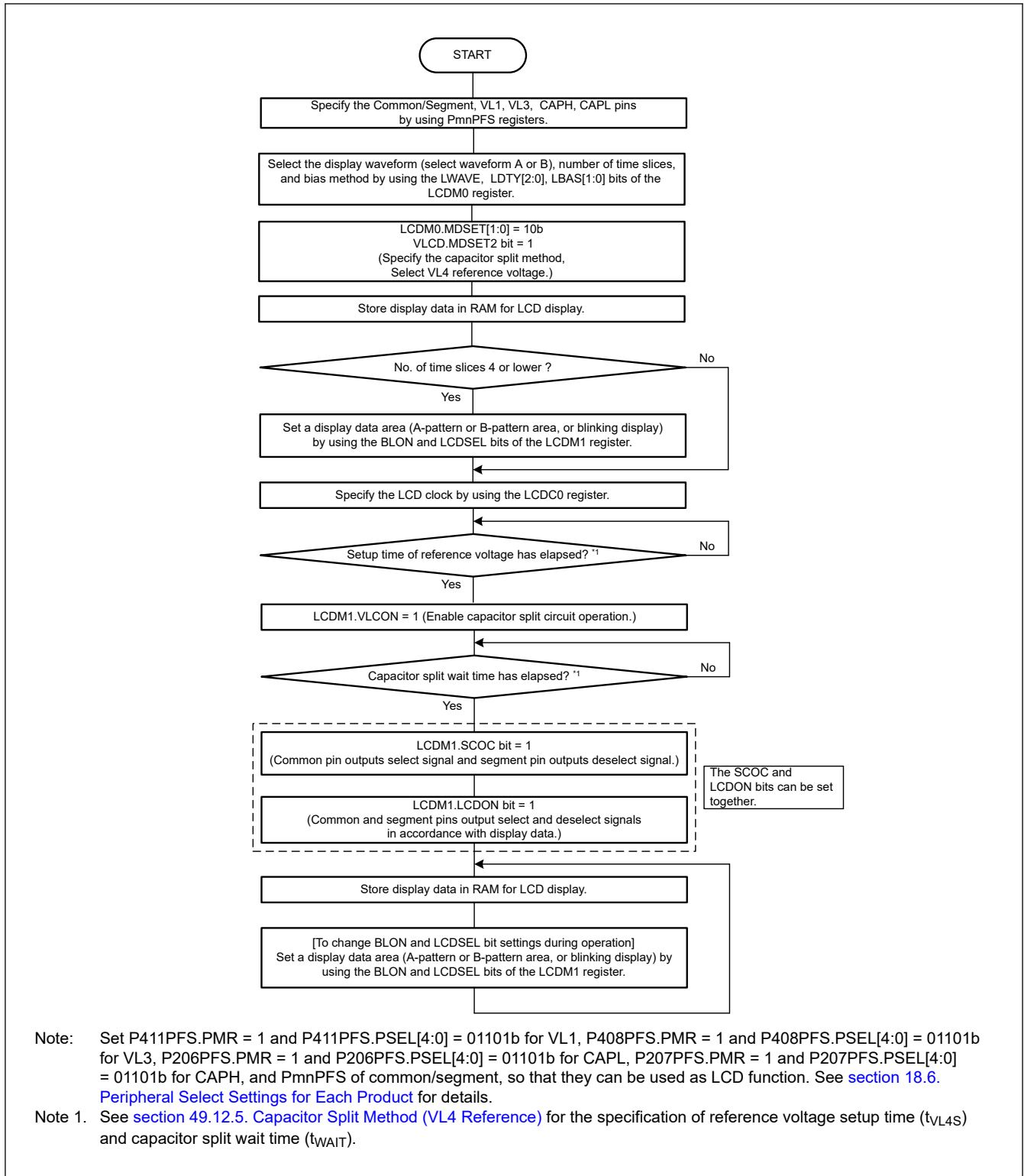
Figure 46.8 Setting procedure for VL4 reference mode of capacitor split method during normal liquid crystal waveform display
