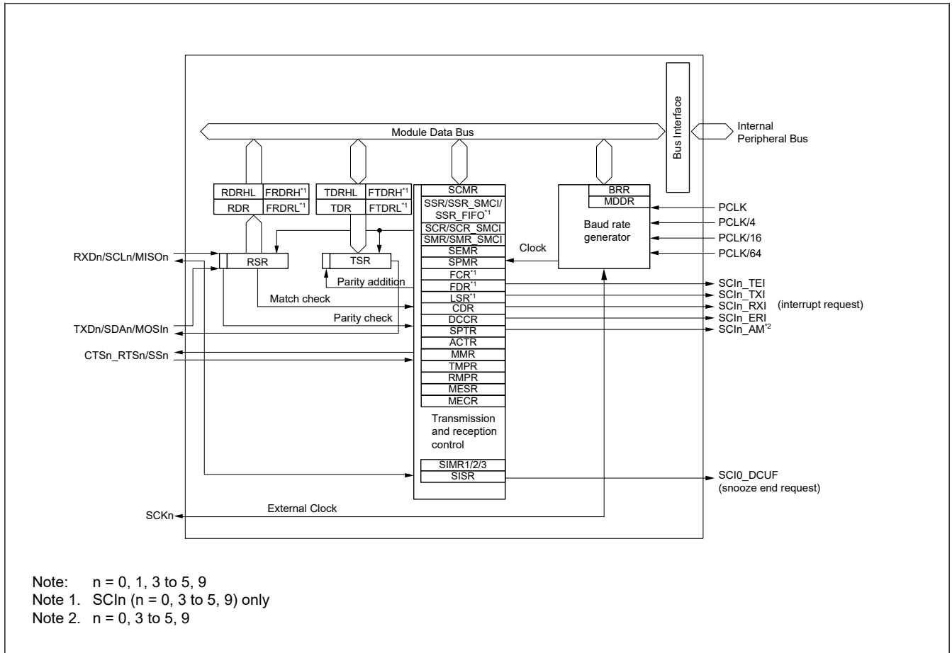
Figure 26.1 SCI block diagram
