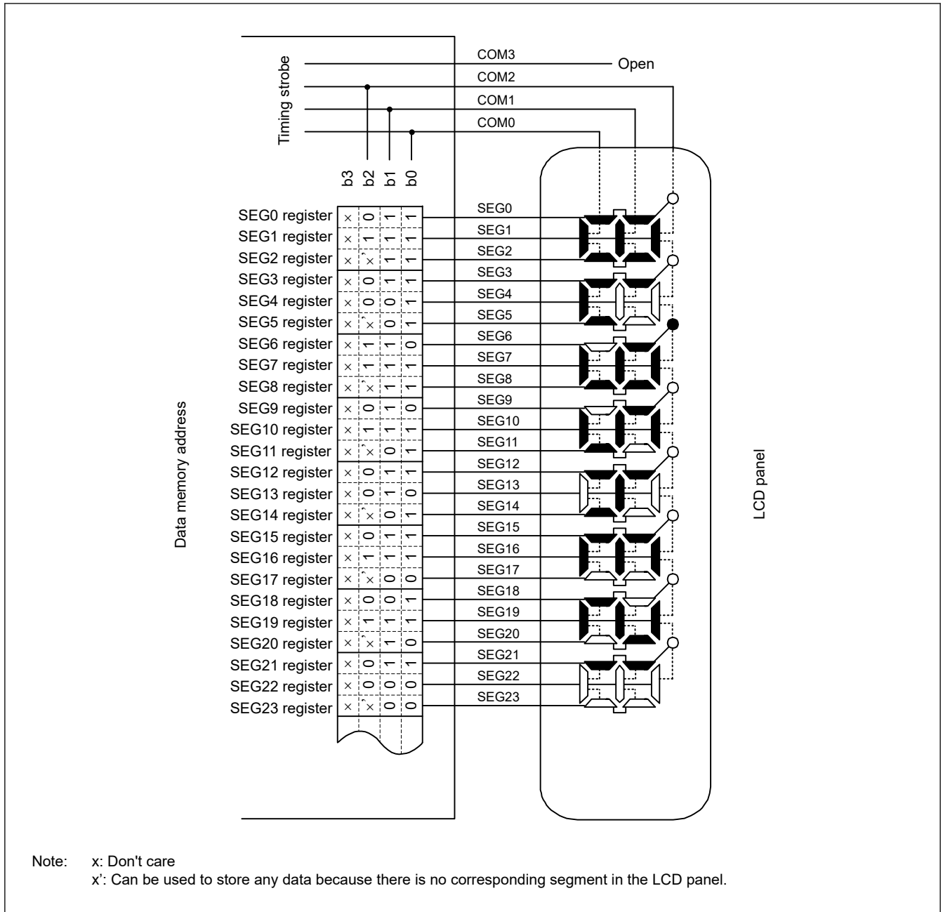
Figure 46.29 Example of connecting three-time slice LCD panel
