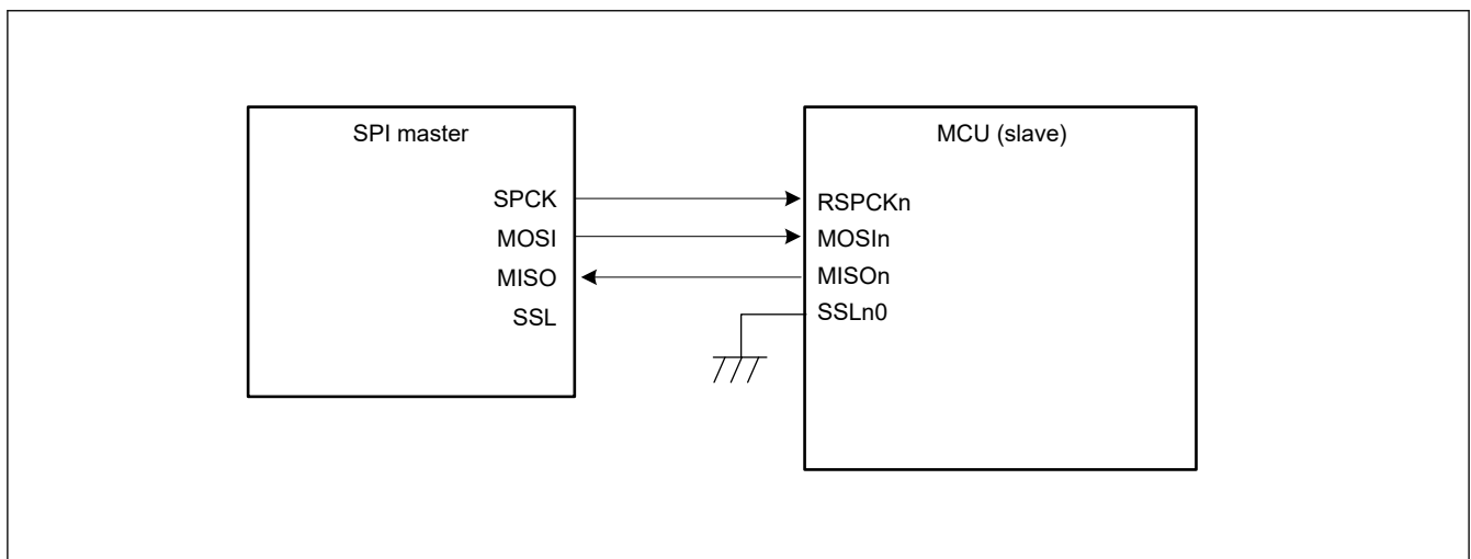
Figure 33.7 Single-master/single-slave configuration example with the MCU as a slave and CPHA = 1
