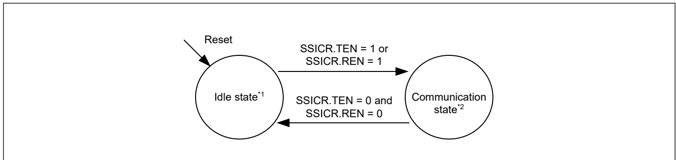
Figure 35.42 SSIE state transition
