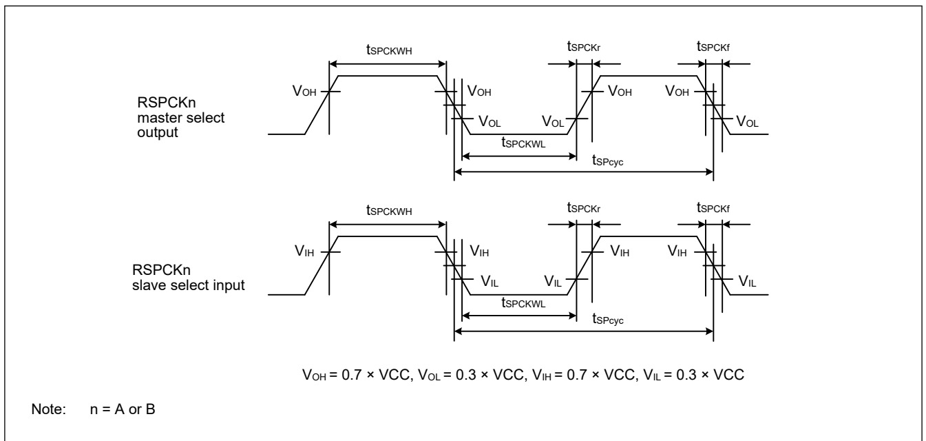
Figure 49.31 SPI clock timing
