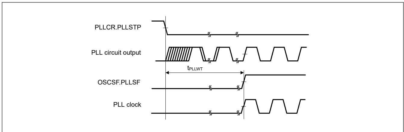
Figure 49.9 PLL clock oscillation start timing (PLL is Operated after Main Clock Oscillation Has Settled)
