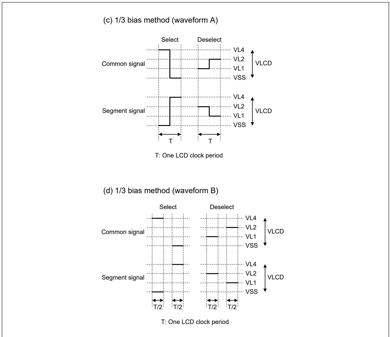
Figure 46.20 Voltages and phases of common and segment signals (2 of 3)
