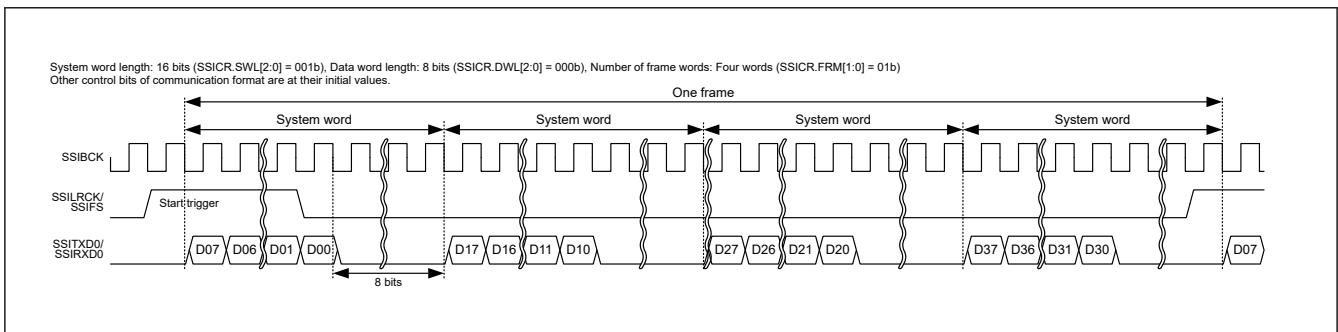
Figure 35.41 TDM format (with padding: system word length > data word length)
