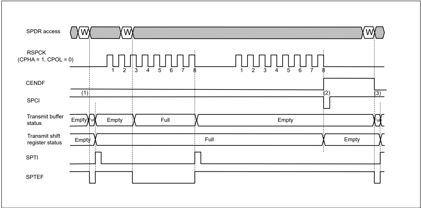
Figure 33.36 Example of Communication End Interrupt Operation (Transmit-Receive/Transmit Slave mode on Clock Synchronous Operation)
