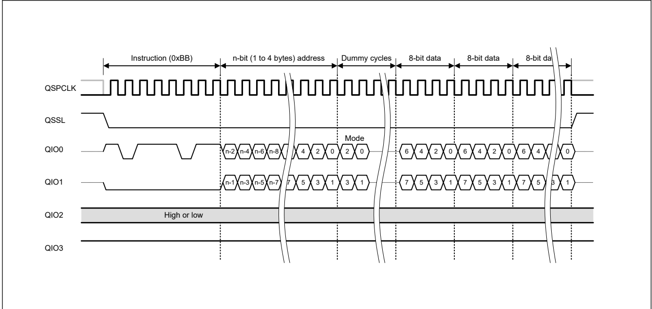
Figure 34.23 Fast Read Dual I/O bus cycle (with extended SPI protocol)
