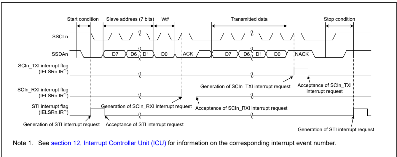
Figure 26.94 Example 2 of operations for master transmission in simple IIC mode with 7-bit slave addresses, ACK interrupts, and NACK interrupts
