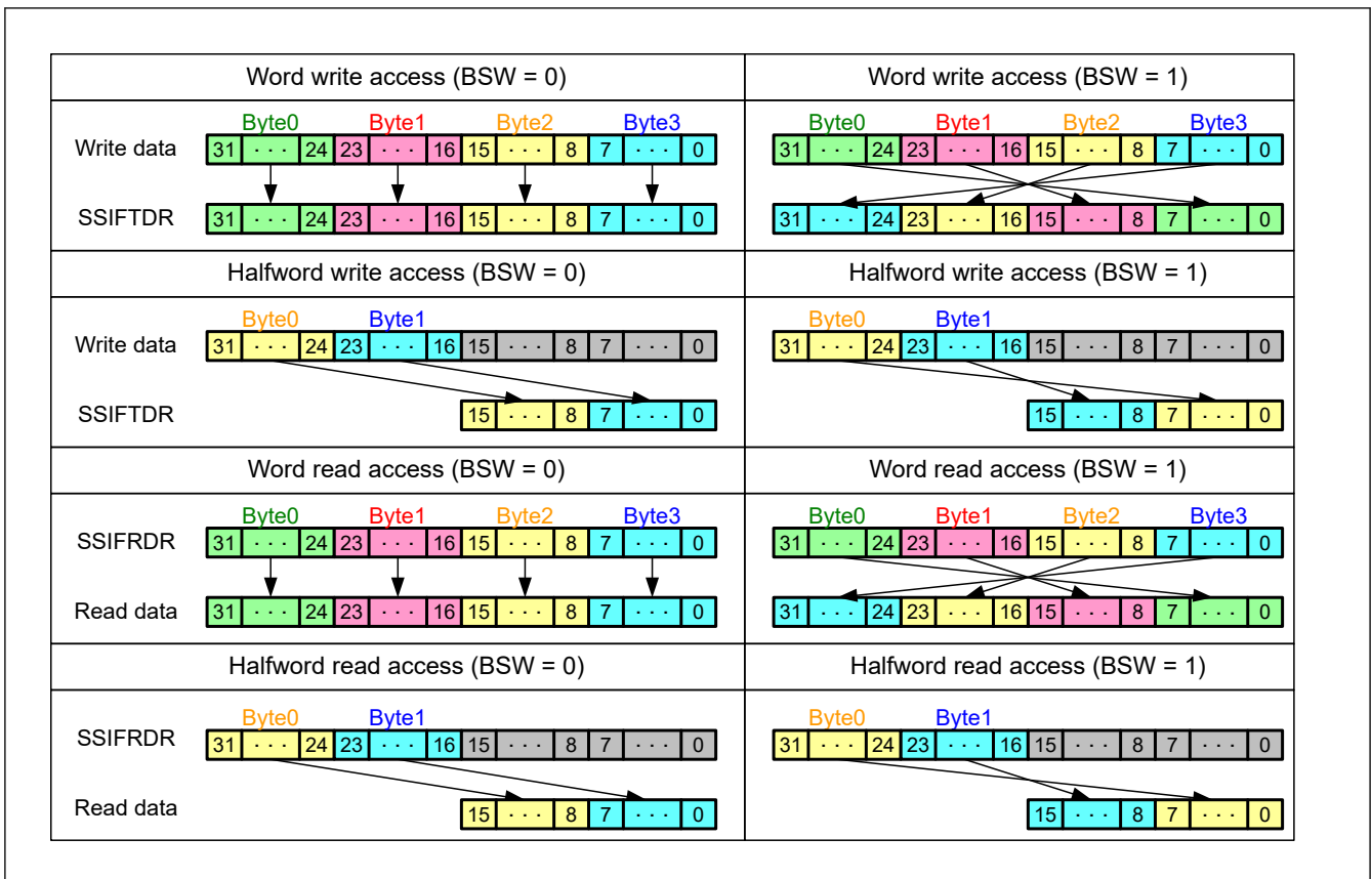
Figure 35.23 Operation example of byte swap
