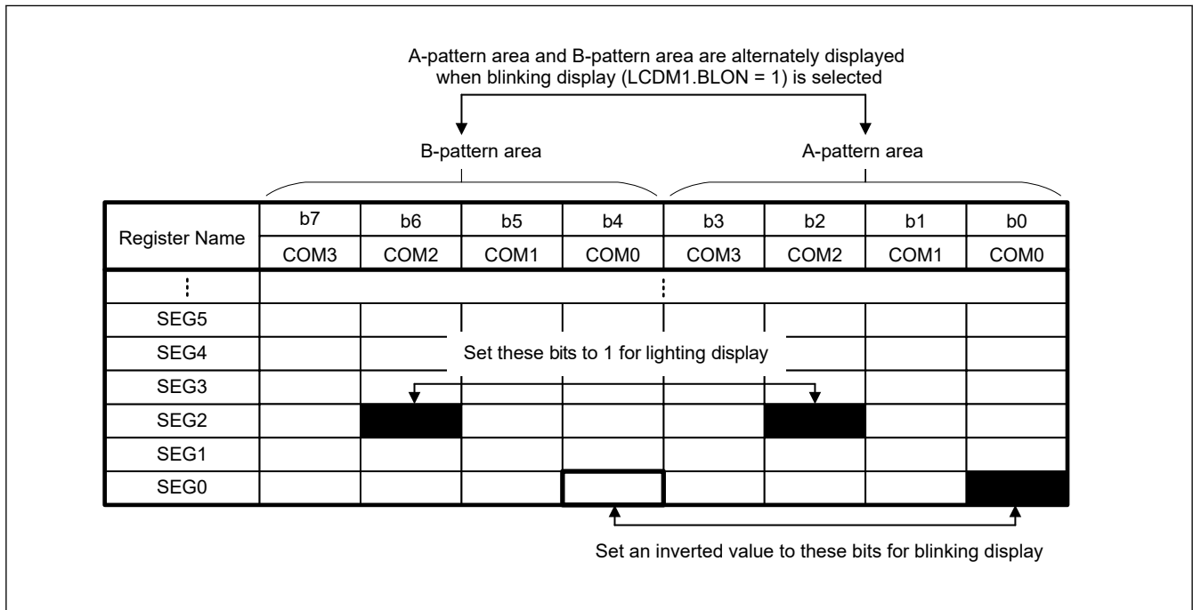
Figure 46.2 Example for setting LCD Display Data registers when the pattern is changed
