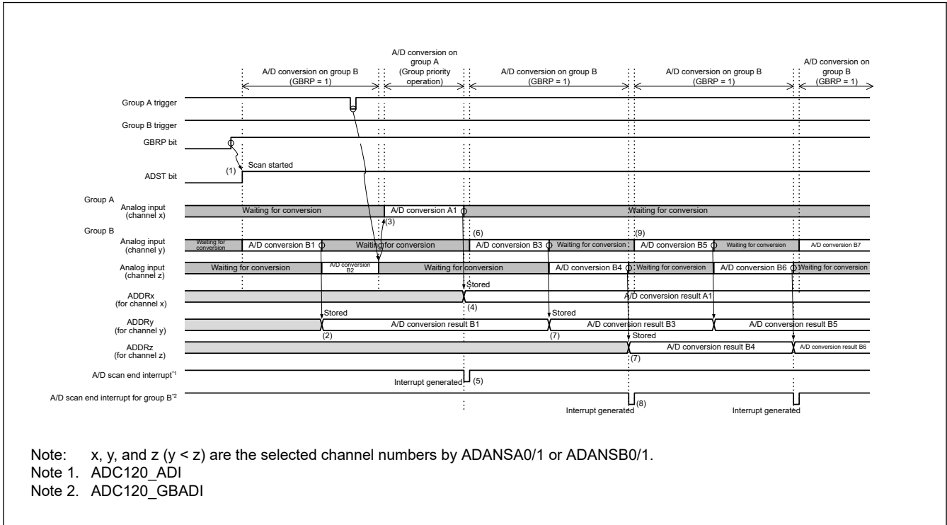
Figure 38.21 Group priority operation example 1-5: Continuously activating single scan for group B (when ADGSPCR.GBRP = 1 )
