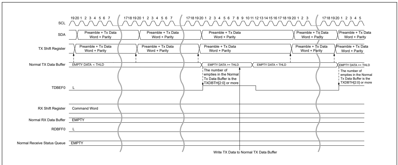
Figure 29.59 HDR data read transfer (HDR-DDR) timing (2/3)
