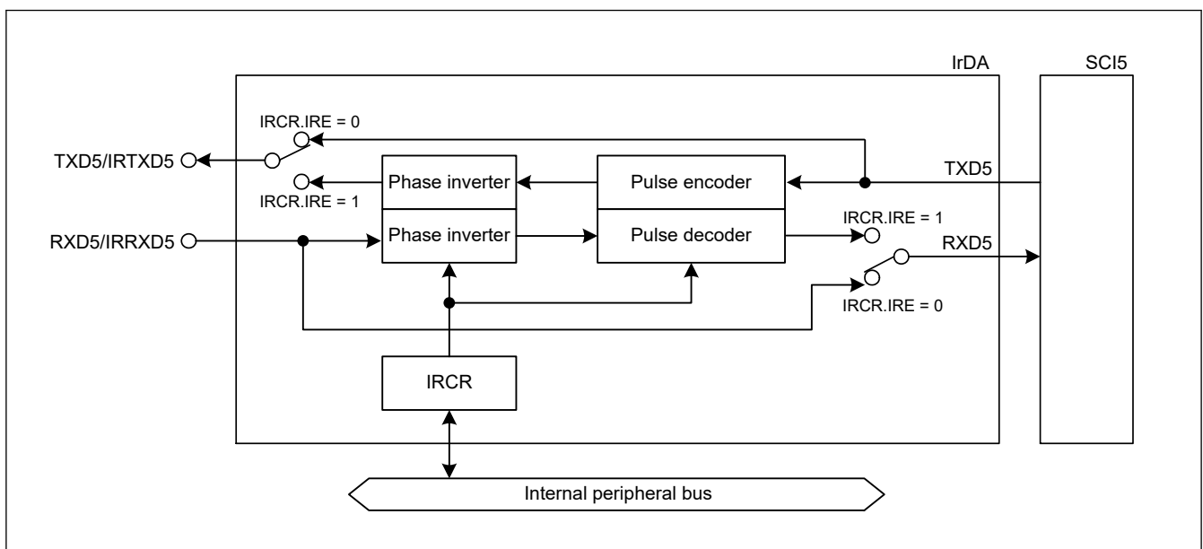
Figure 27.1 Association between the IrDA interface and SCI5
