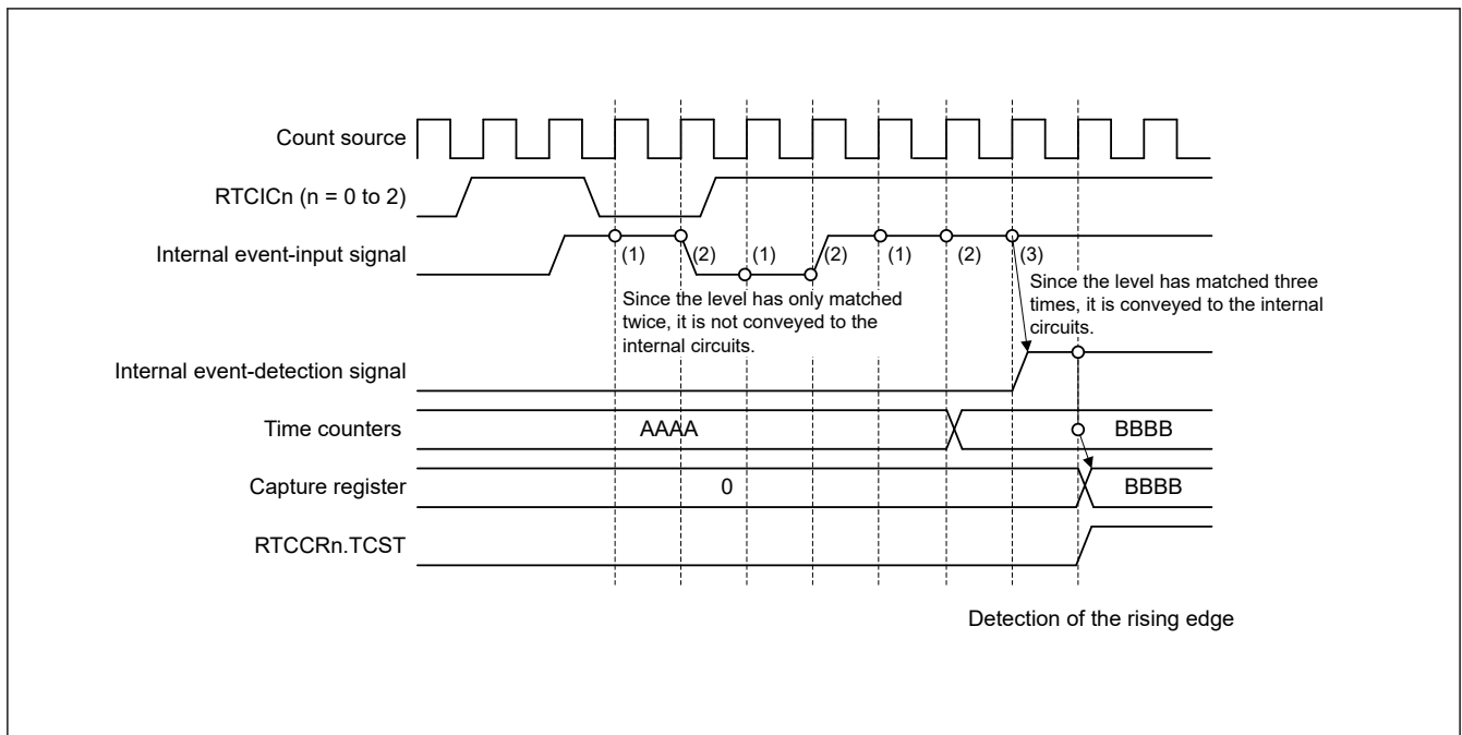
Figure 22.9 Timing of a time capture operation with the noise filter on
