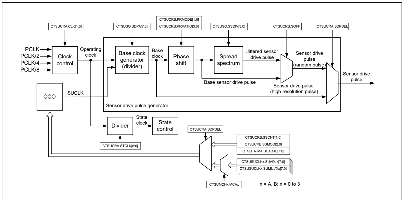
Figure 42.4 Generation of sensor drive pulse
