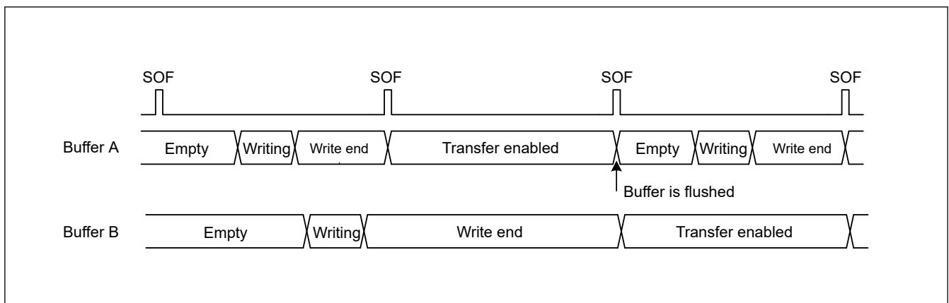
Figure 25.17 Example buffer flush operation
