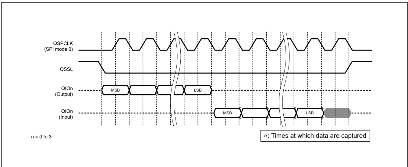
Figure 34.8 Basic serial interface timing (SPI mode 0)
