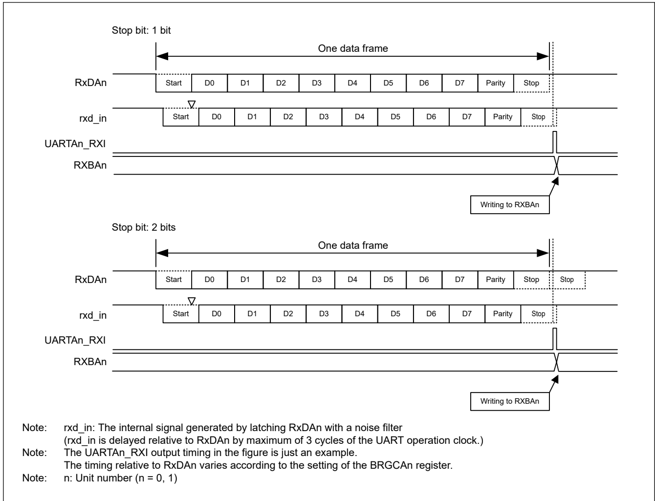
Figure 30.7 Timing of UART receive operation
