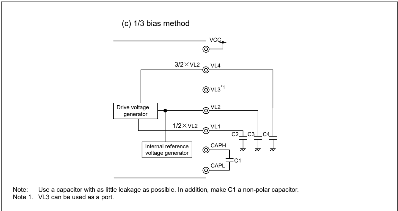
Figure 46.13 Examples of LCD drive power connections using VL2 reference mode of internal voltage boosting method
