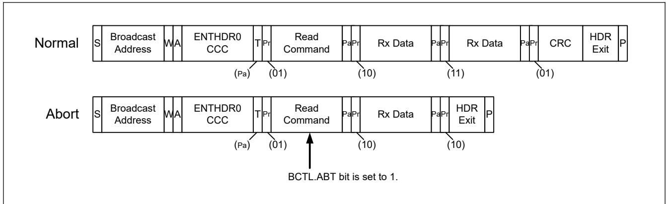
Figure 29.117 Abort operation of HDR-DDR read transfer
