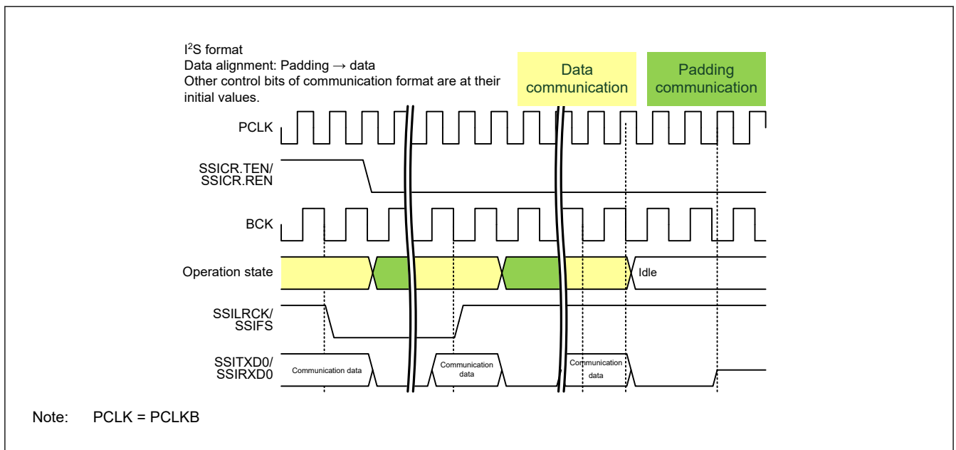
Figure 35.49 Halt from data communication (with padding bits)
