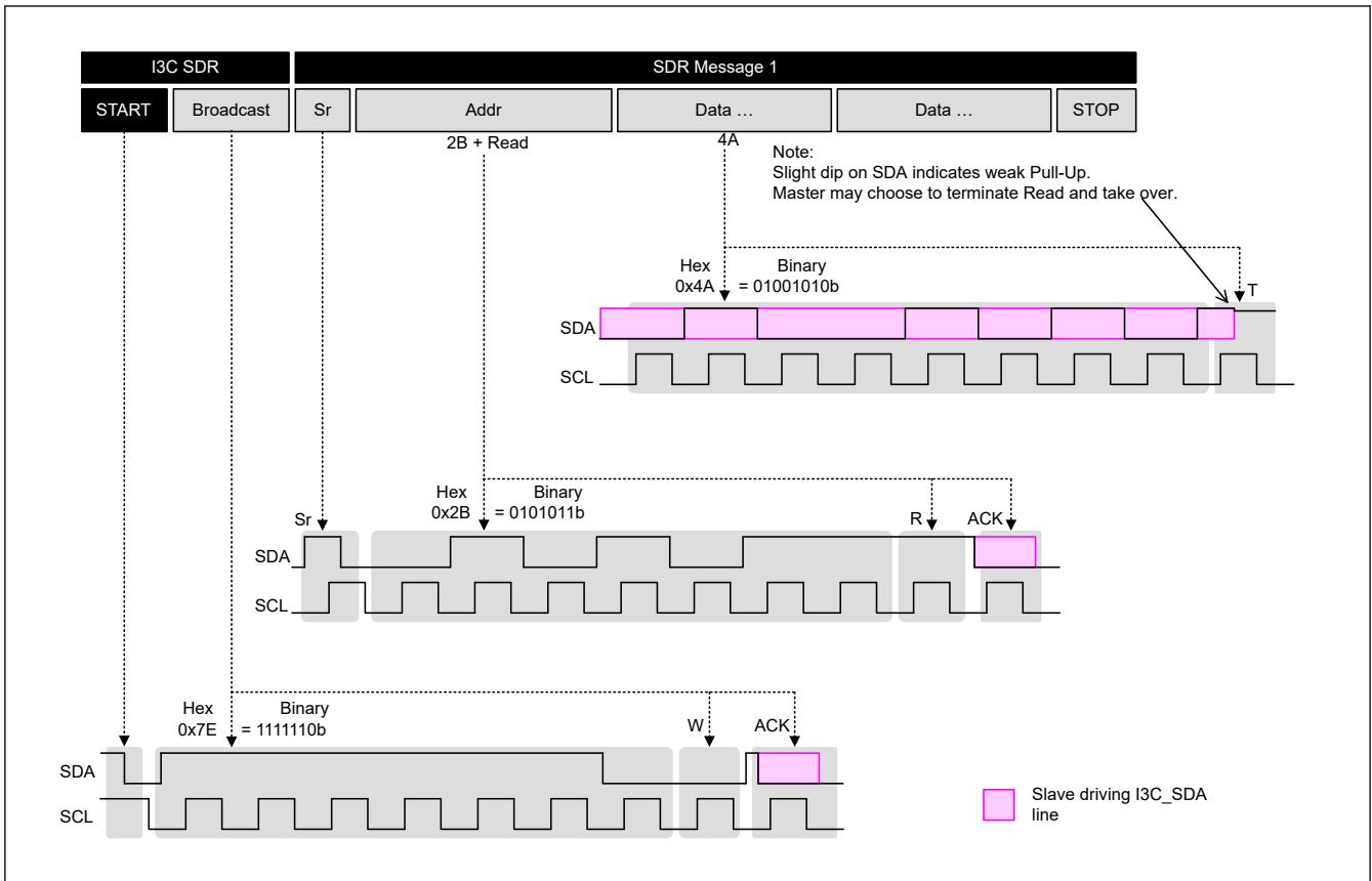
Figure 29.70 Example communication using I3C coding SDR with broadcast (0x7E)
