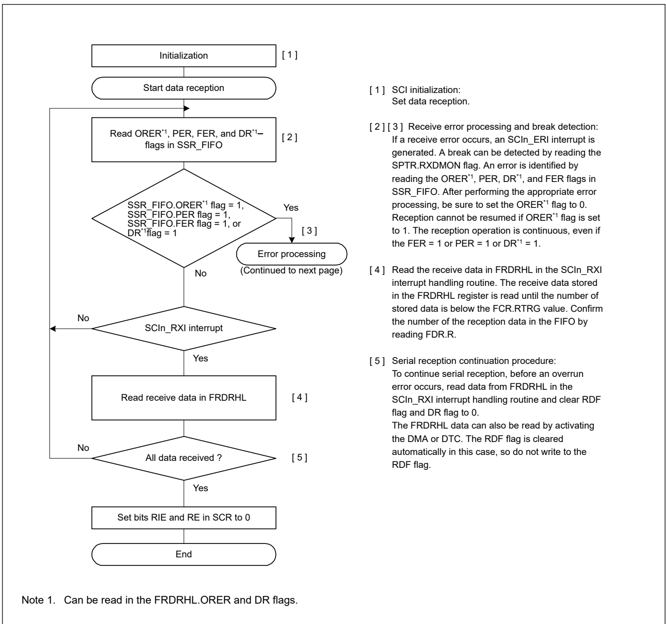
Figure 26.26 Example flow of serial reception in asynchronous mode with FIFO selected and Address Matching Enabled (1)
