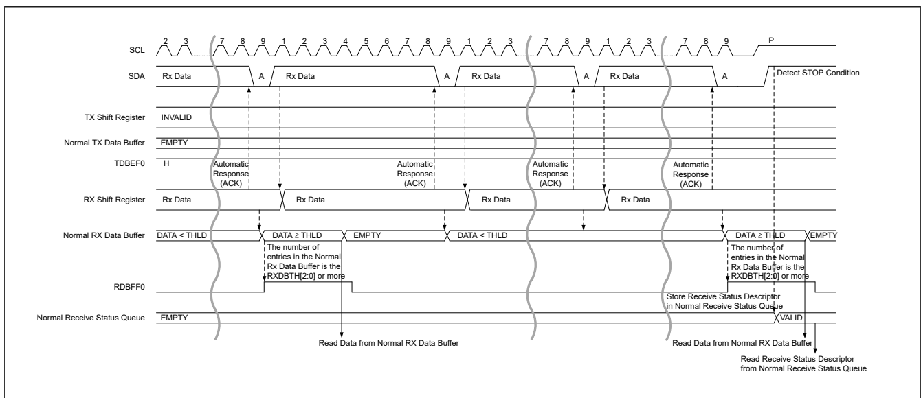
Figure 29.48 Legacy I 2 C message data write transfer timing (2/2)
