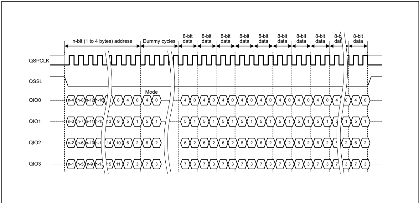
Figure 34.28 Fast Read Quad I/O bus cycle in XIP mode
