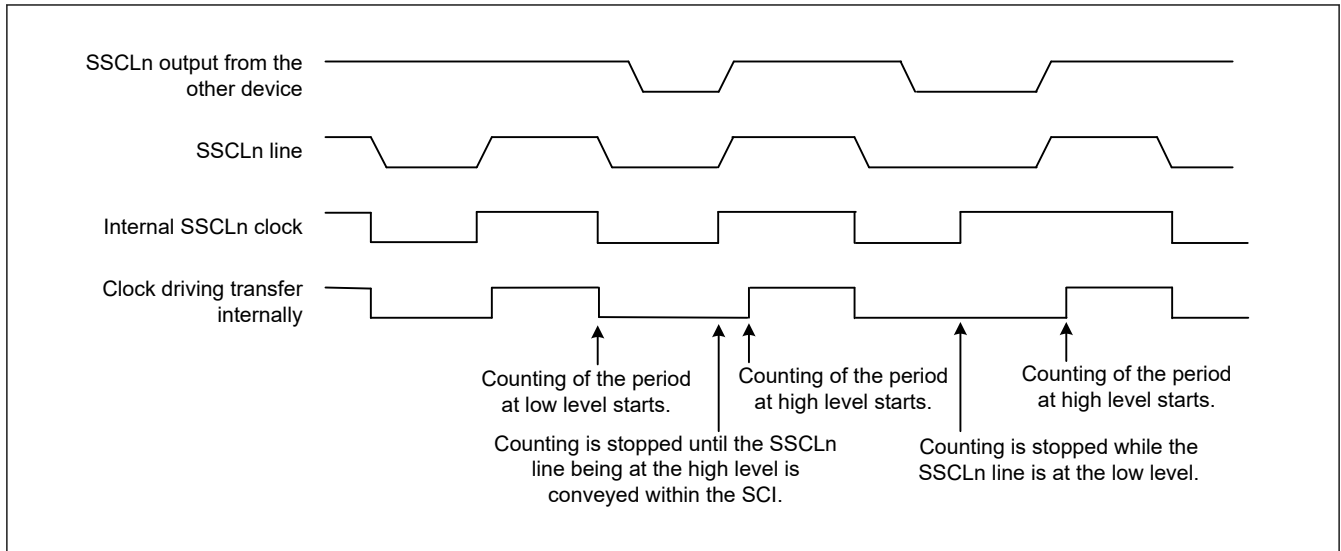
Figure 26.91 Example operations for clock synchronization
