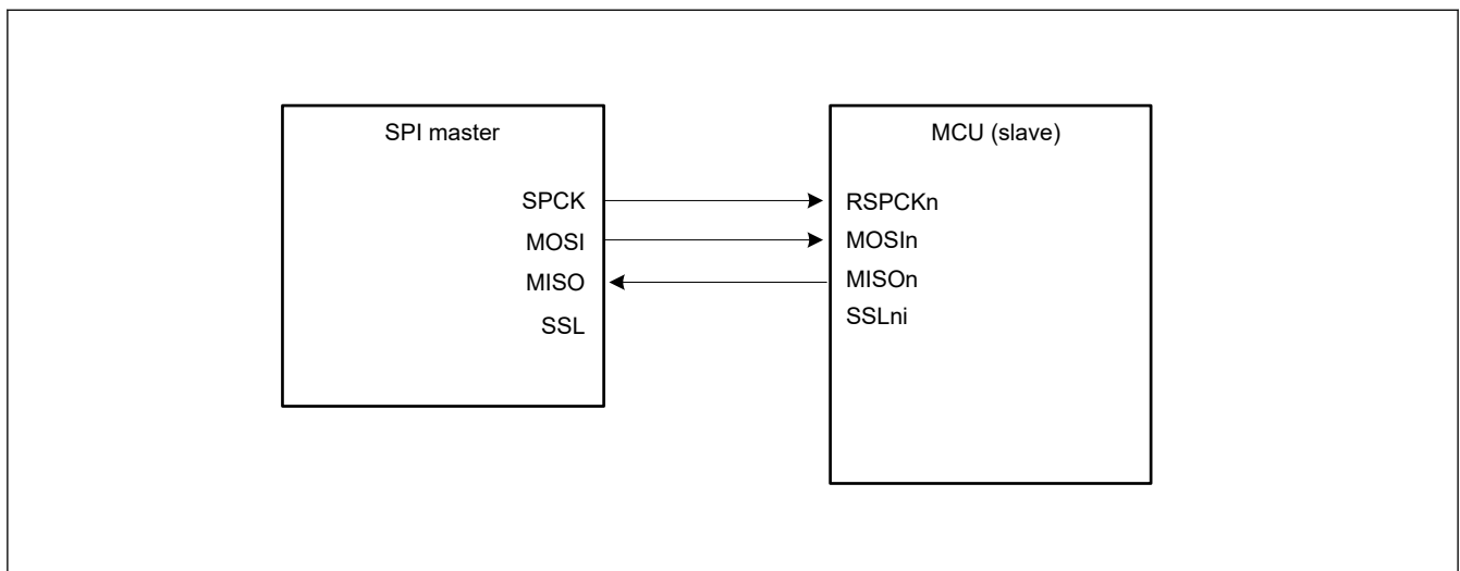
Figure 33.12 Clock synchronous master/slave configuration example with the MCU as a slave and CPHA = 1
