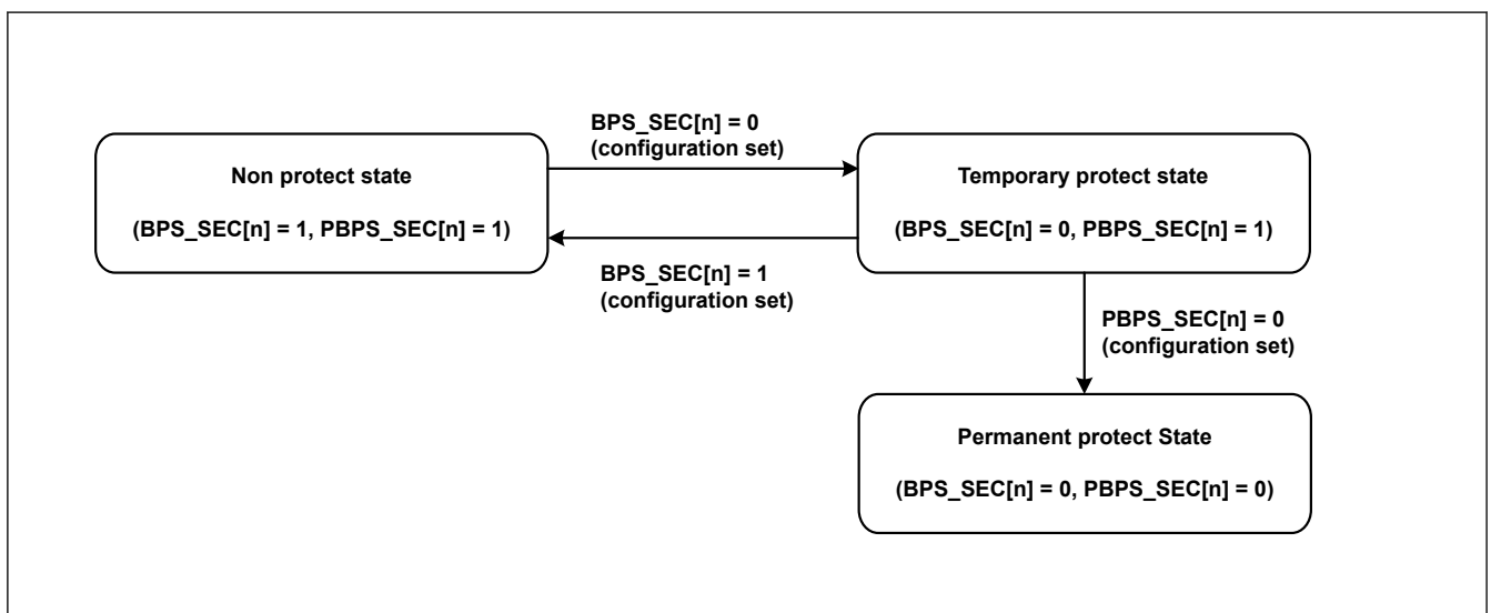
Figure 45.30 Status transition of flash sequencer by BPS_SEC[n] and PBPS_SEC[n]
