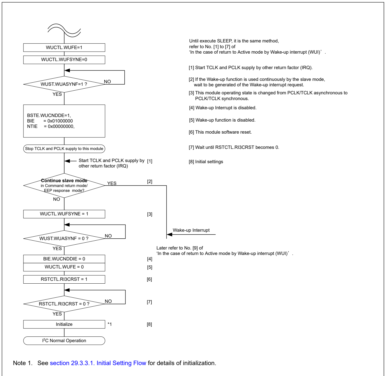
Figure 29.130 Use case of command recover mode and EEP response mode (Wake-up recovery by other recovery causes (IRQ))
