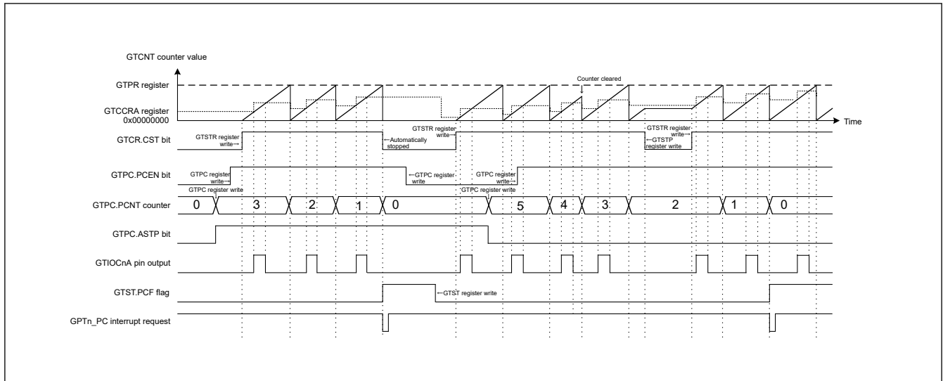
Figure 20.48 Example of PWM cycle count function (saw-wave one-shot pulse mode)
