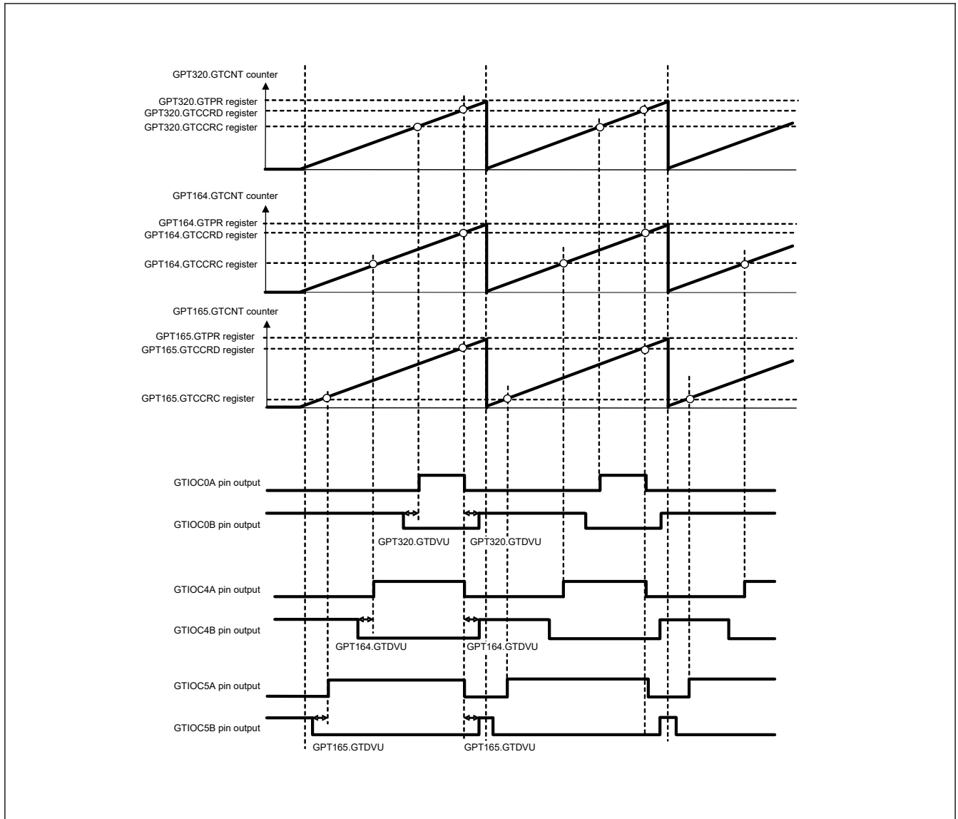
Figure 20.44 Example of 3-phase saw-wave complementary PWM output with automatic dead time setting
