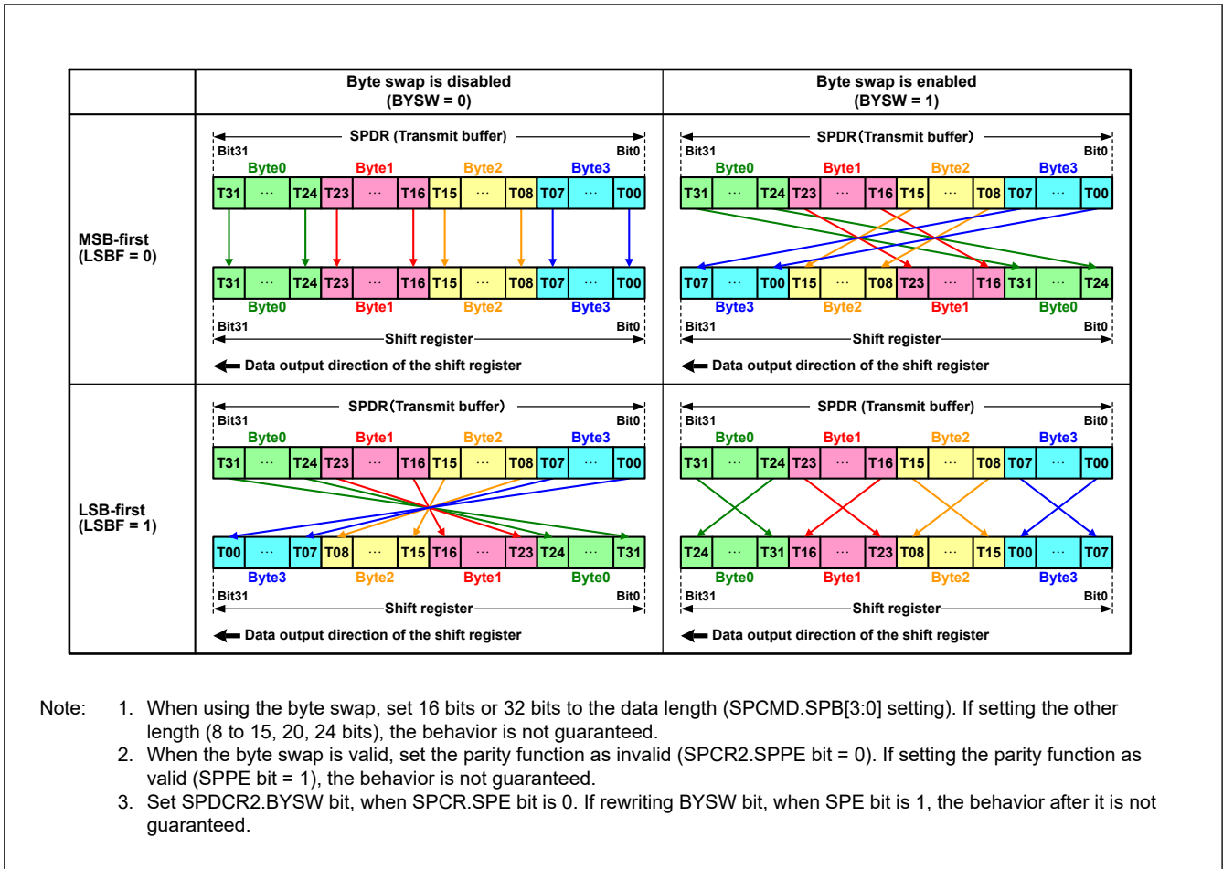
Figure 33.22 Byte swap with MSB/LSB transfer
