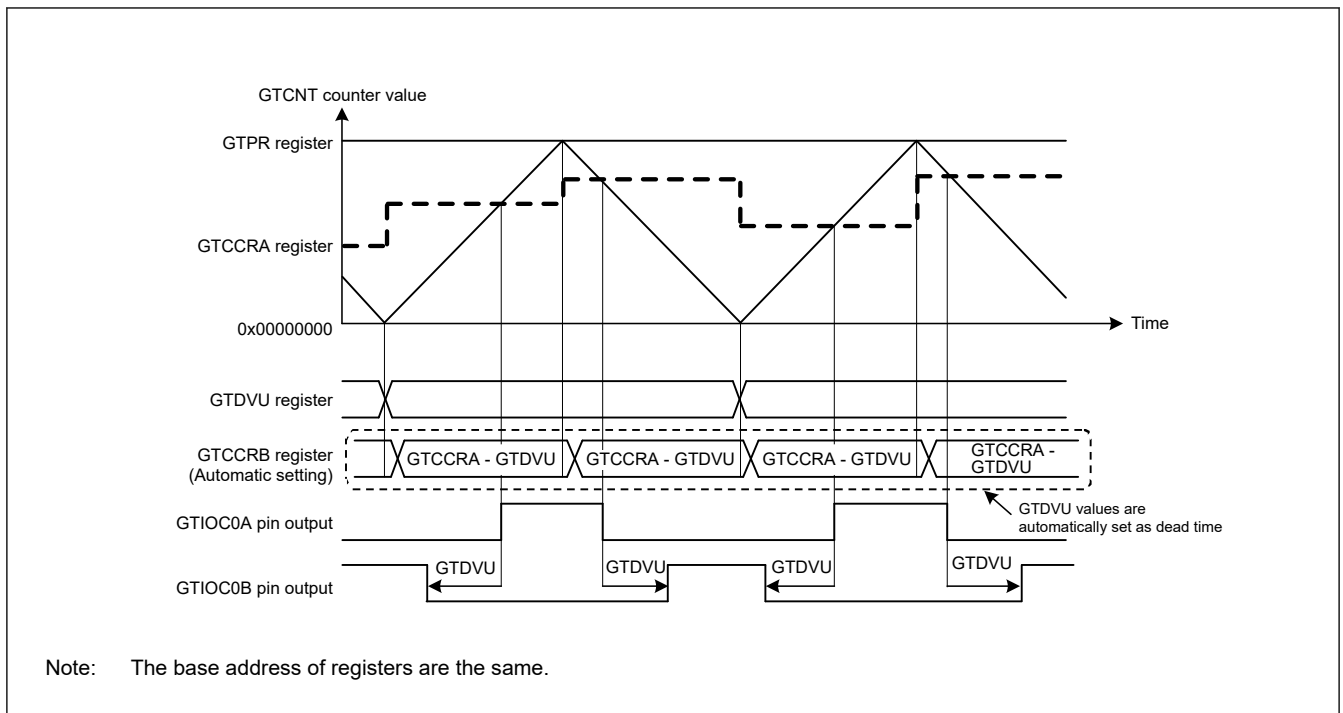
Figure 20.27 Example of automatic compare-match value setting function with dead time in triangle-wave PWM mode 2 or 3, and active-high
