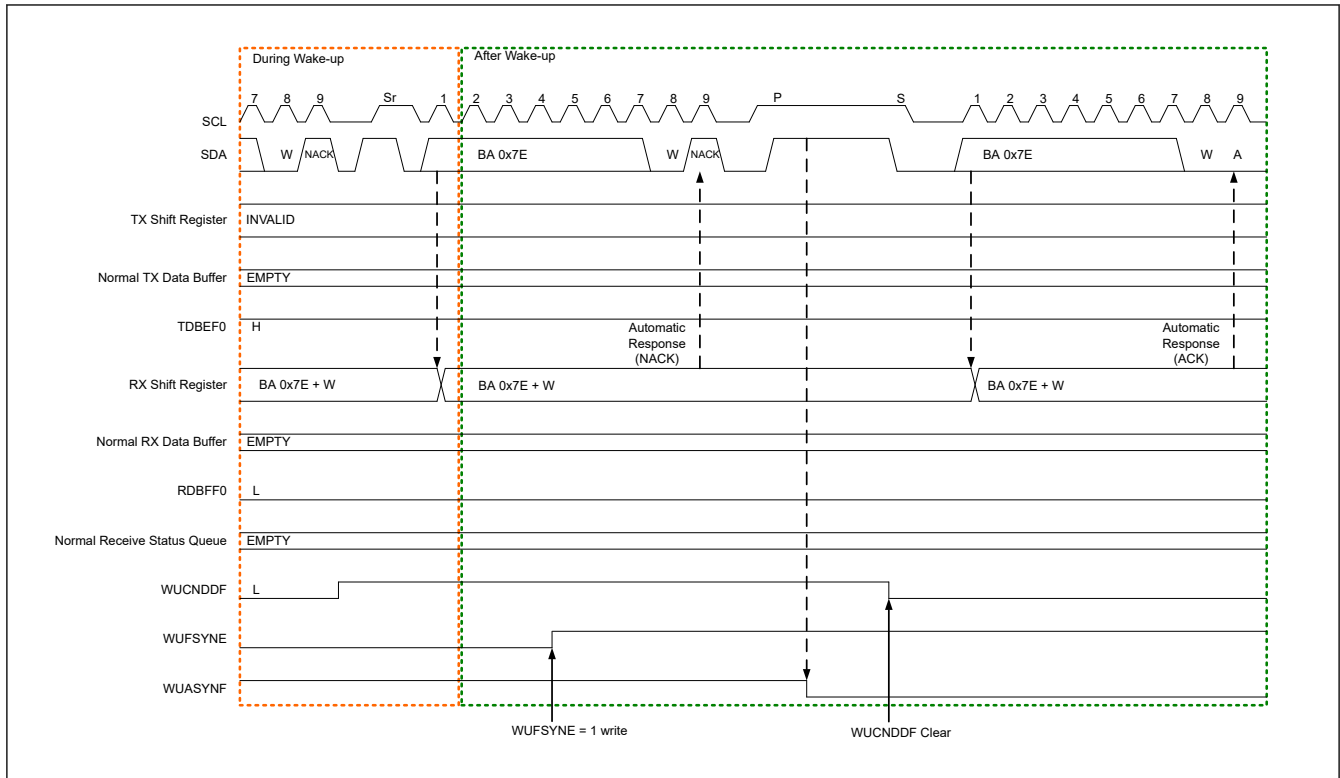
Figure 29.134 I3C slave Wake-up operation (2/2)
