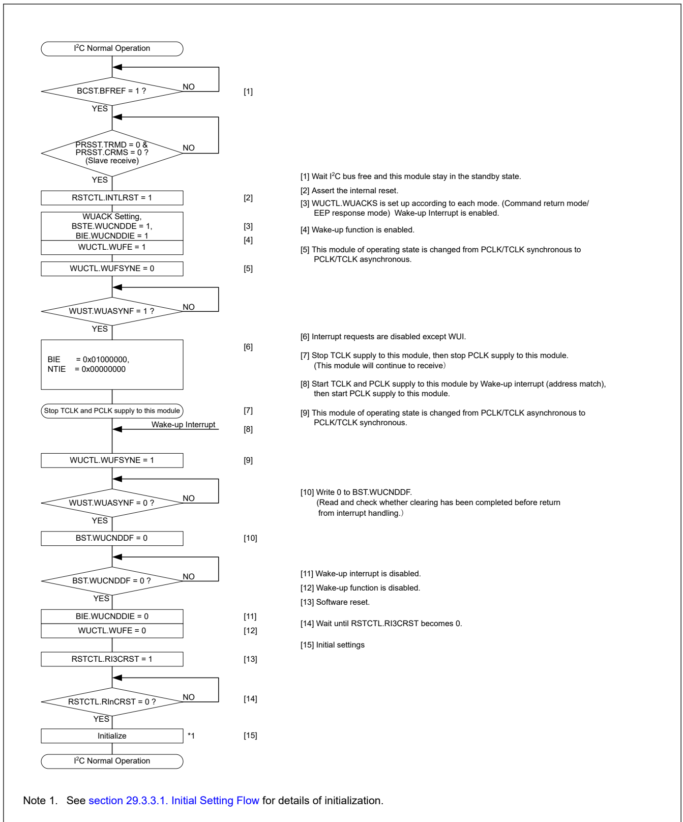
Figure 29.129 Use case of command recover mode and EEP response mode (Wake-up recovery by a Wake-up interrupt triggered by the match of the slave address)
