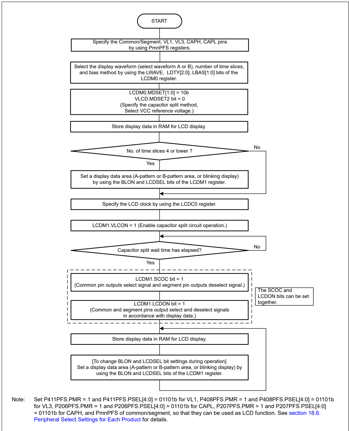
Figure 46.7 Setting procedure for VCC reference mode of capacitor split method during normal liquid crystal waveform display
