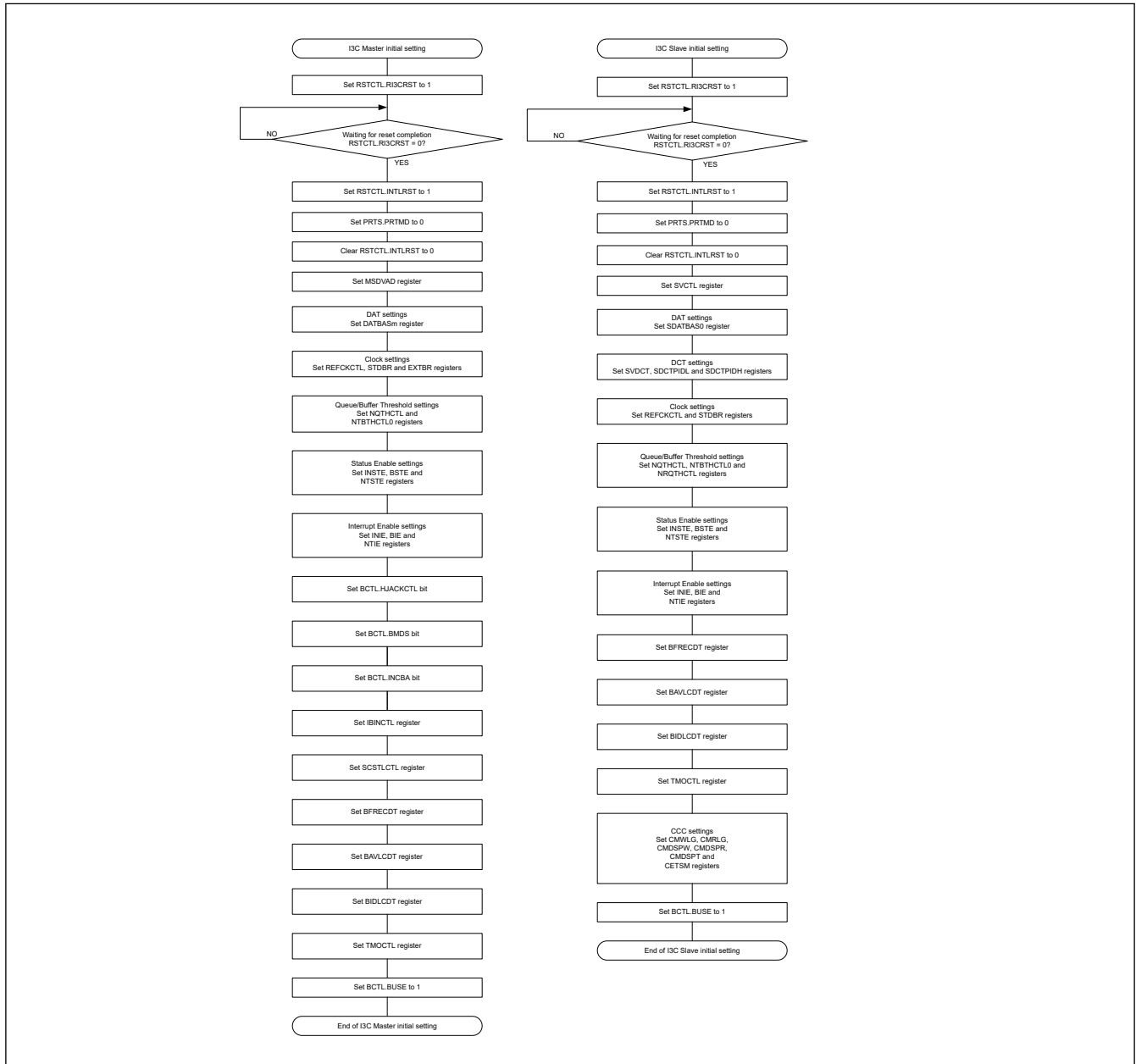
Figure 29.139 Example of each initialization flowchart for I3C master mode and slave mode
