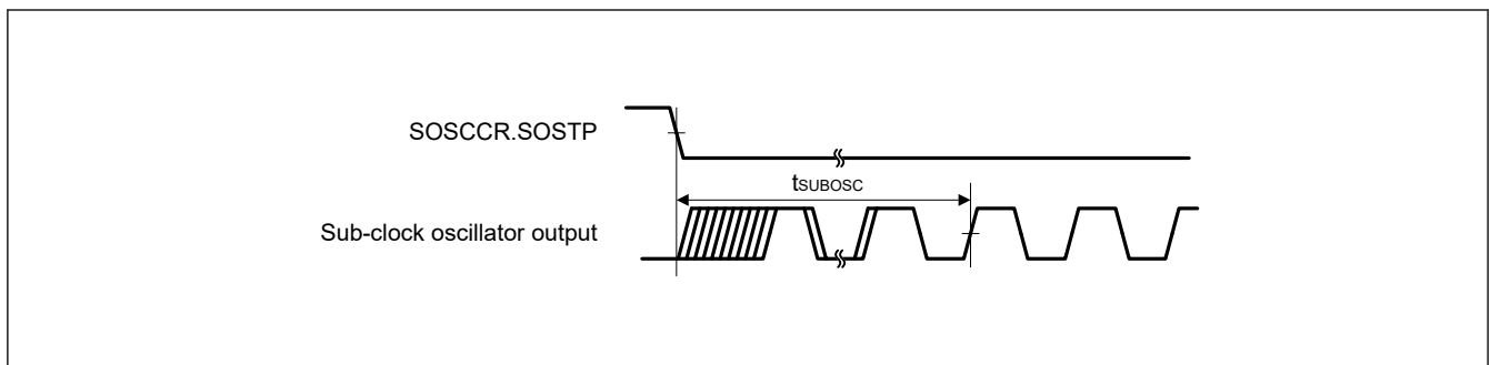
Figure 49.10 Sub-clock oscillation start timing
