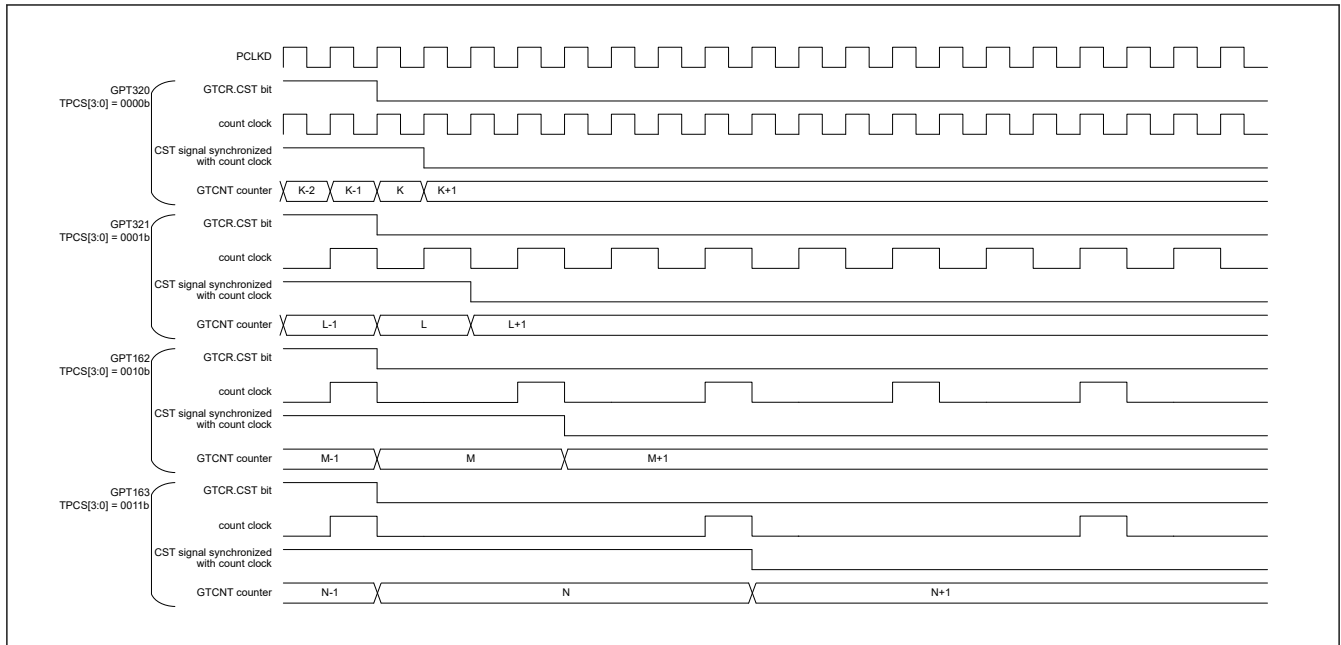
Figure 20.39 Example of Simultaneous Stop Operation by Software (with Different Count Period)
