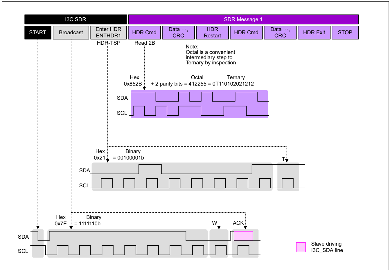
Figure 29.76 Example communication using HDR-TSP protocol
