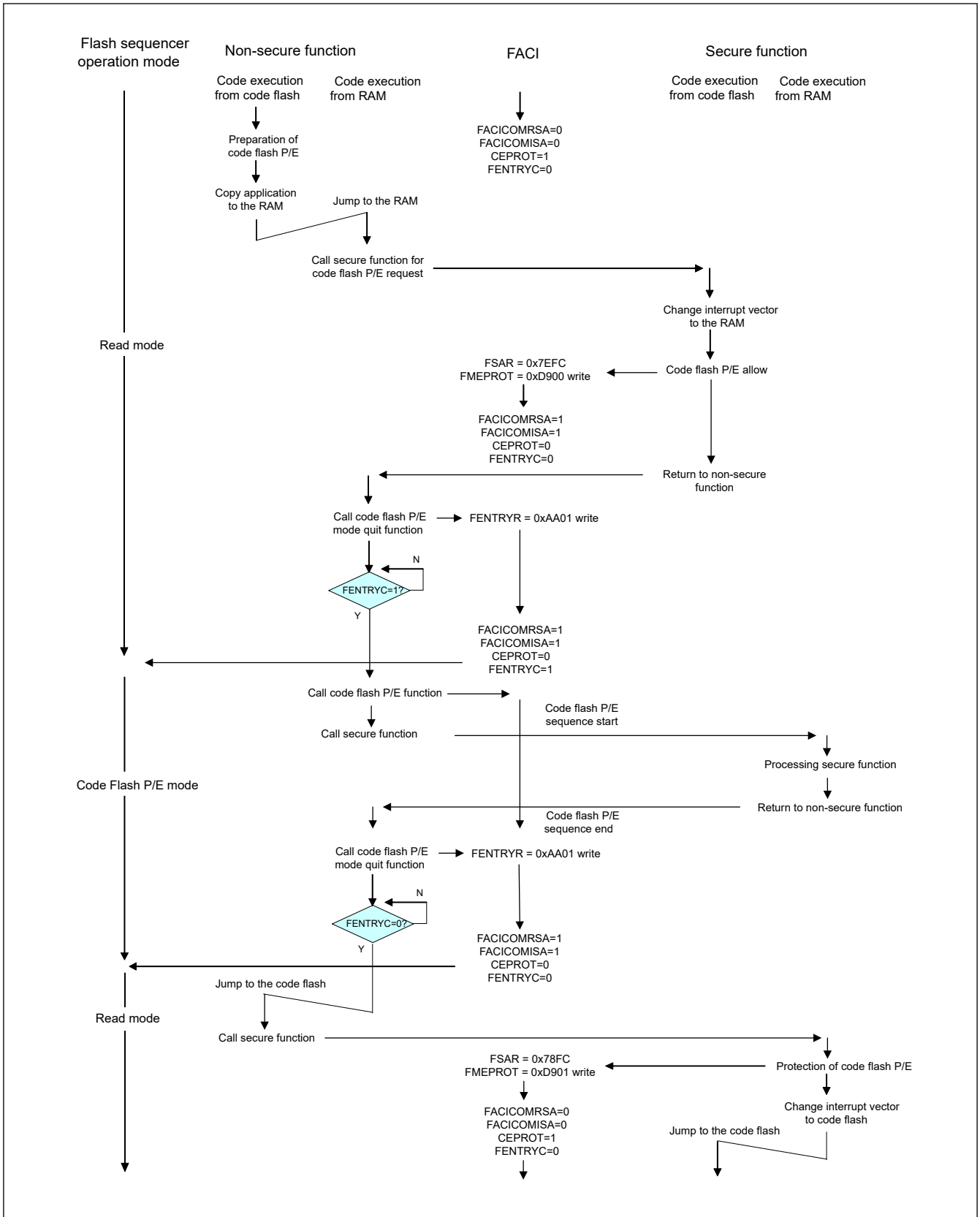
Figure 45.35 Code flash P/E sequence example by non-secure function (1) (using non-secure function for code flash P/E)
