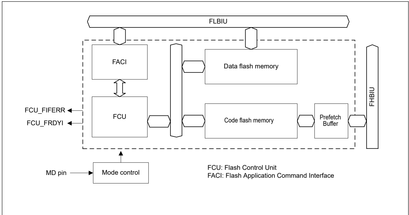
Figure 45.1 Block diagram of flash memory-related modules
