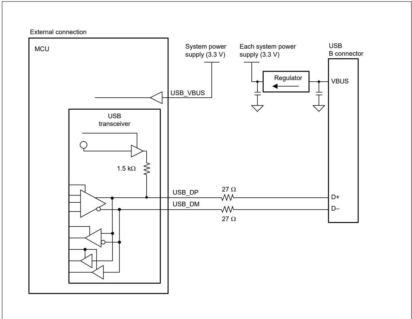
Figure 25.5 Example device connection in a bus-powered state
