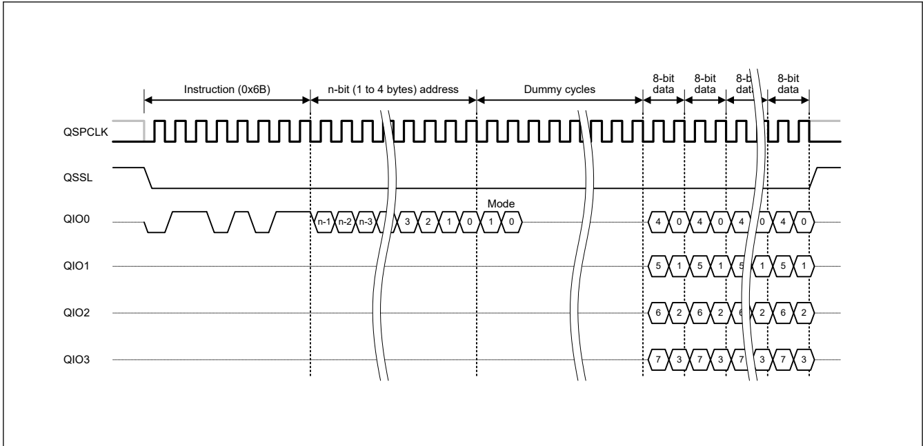
Figure 34.25 Fast Read Quad Output bus cycle (with extended SPI protocol)
