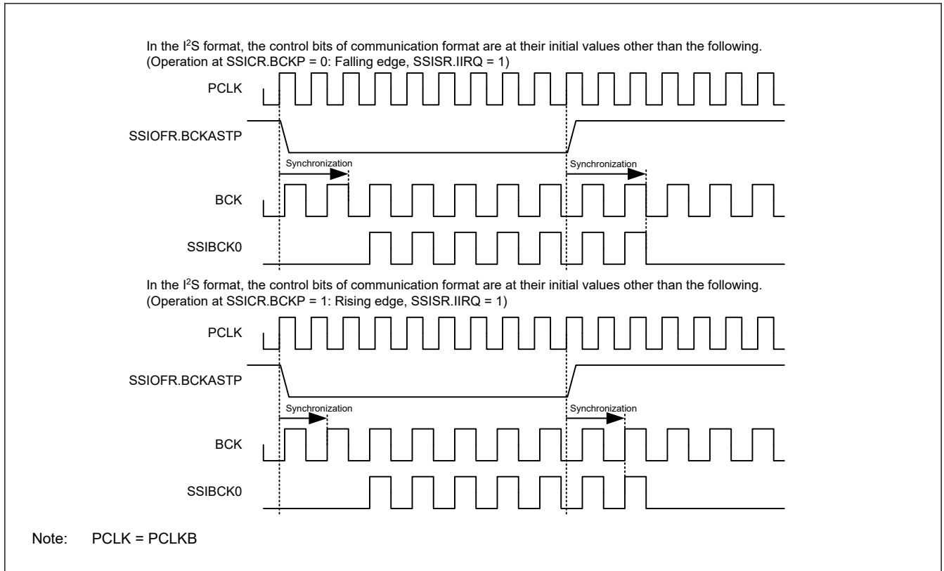
Figure 35.44 Example of stopping SSIBCK0 with SSIOFR.BCKASTP
