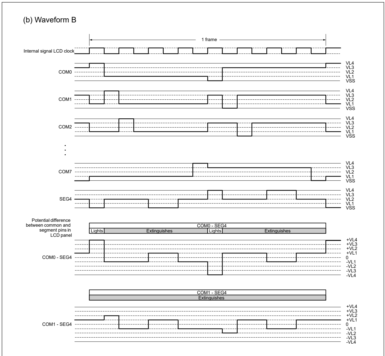
Figure 46.43 Eight-time slice LCD drive waveform examples between SEG4 and each common signal using 1/4 bias method (2 of 2)
