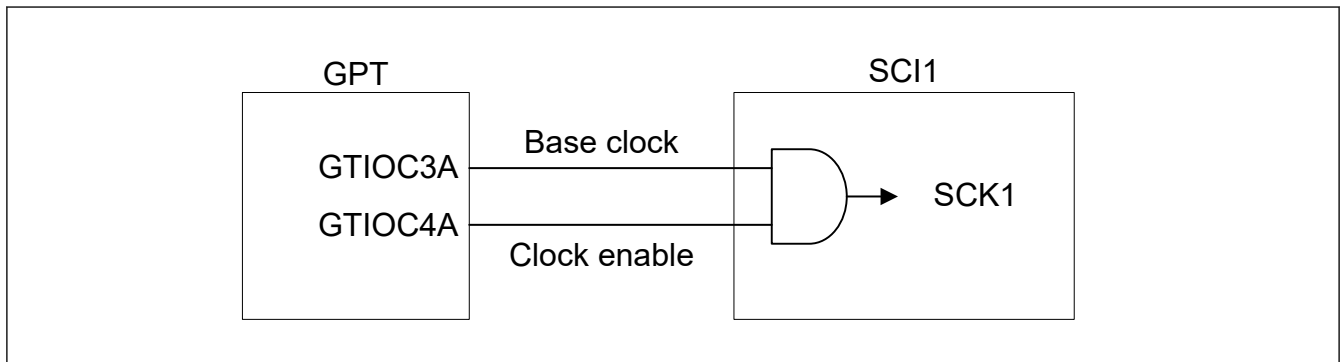
Figure 26.3 Example of GPT and SCI connection
