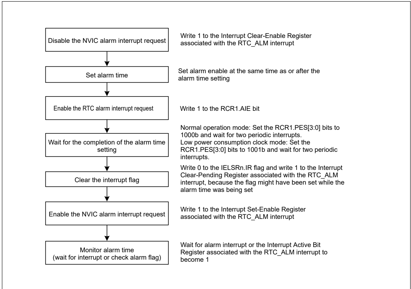
Figure 22.6 Using the alarm function
