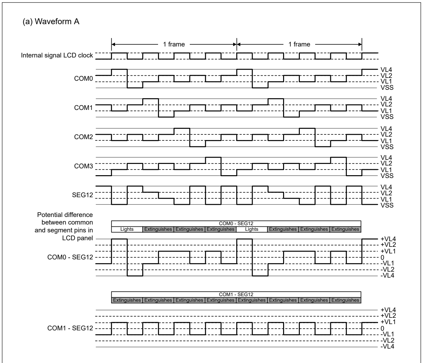
Figure 46.34 Four-time slice LCD drive waveform examples between SEG12 and each common signal using 1/3 bias method (1 of 2)
