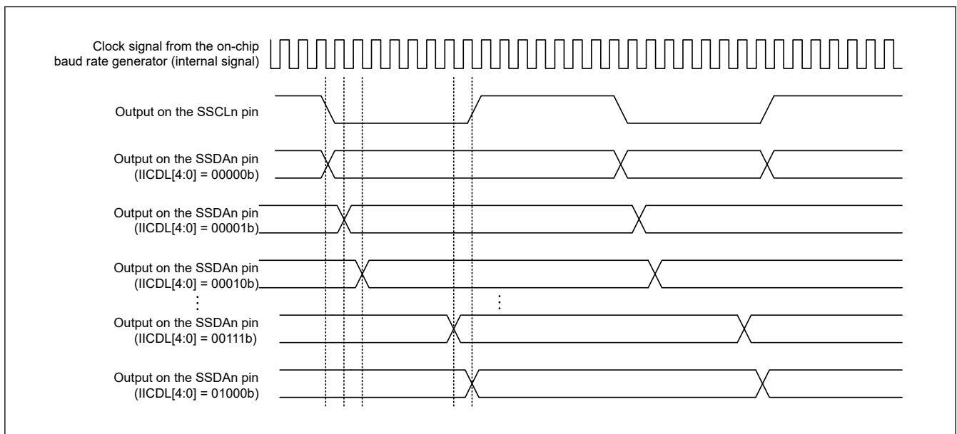
Figure 26.92 Timing of delays in SDAn output
