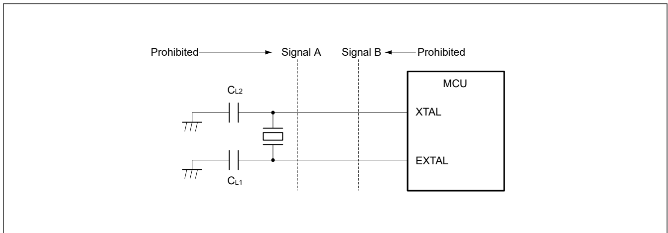
Figure 8.15 Signal routing in board design for oscillation circuit
