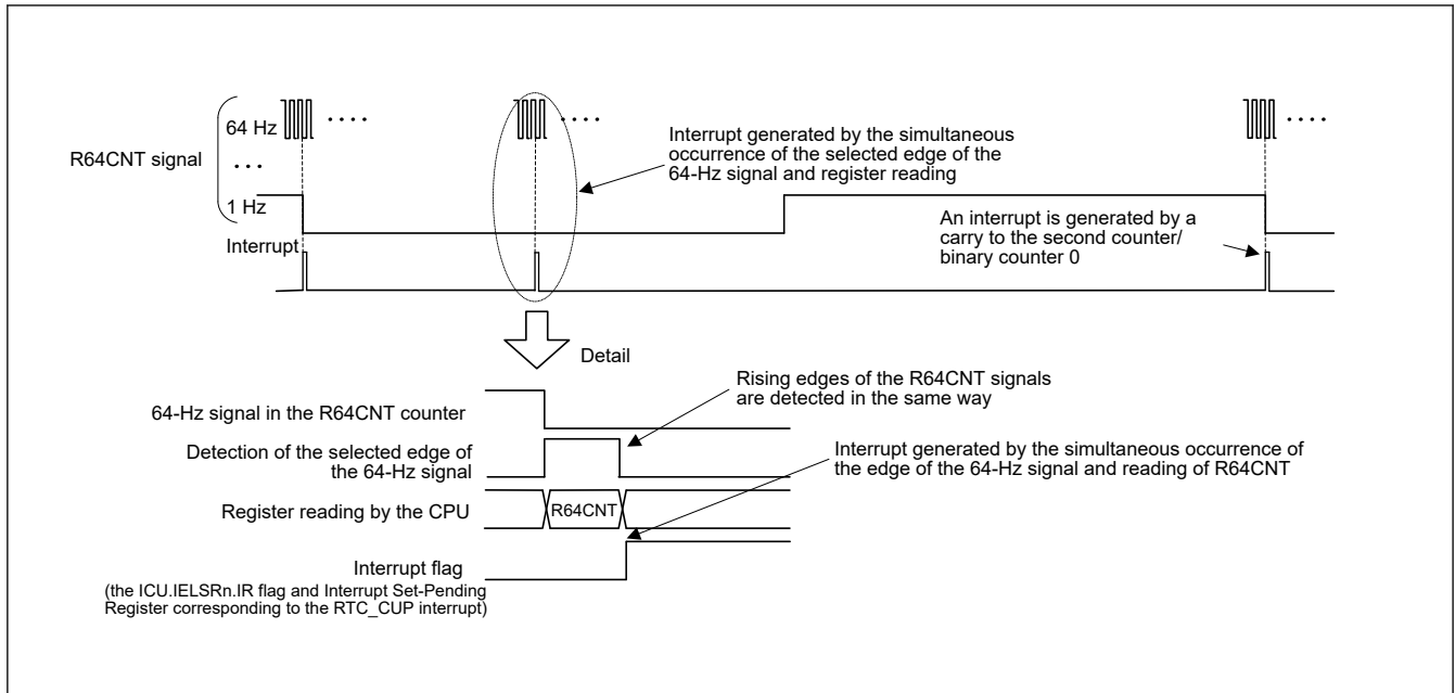
Figure 22.11 Timing for the carry interrupt (RTC_CUP)
