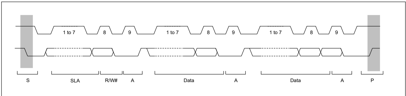
Figure 29.69 I 2 C bus timing (SLA = 7 bits)
