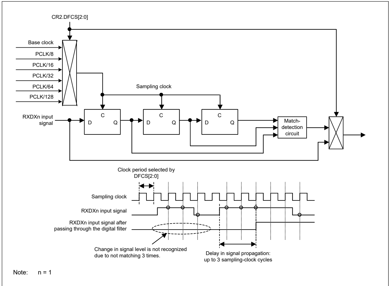
Figure 26.112 Example of operations with the digital filter
