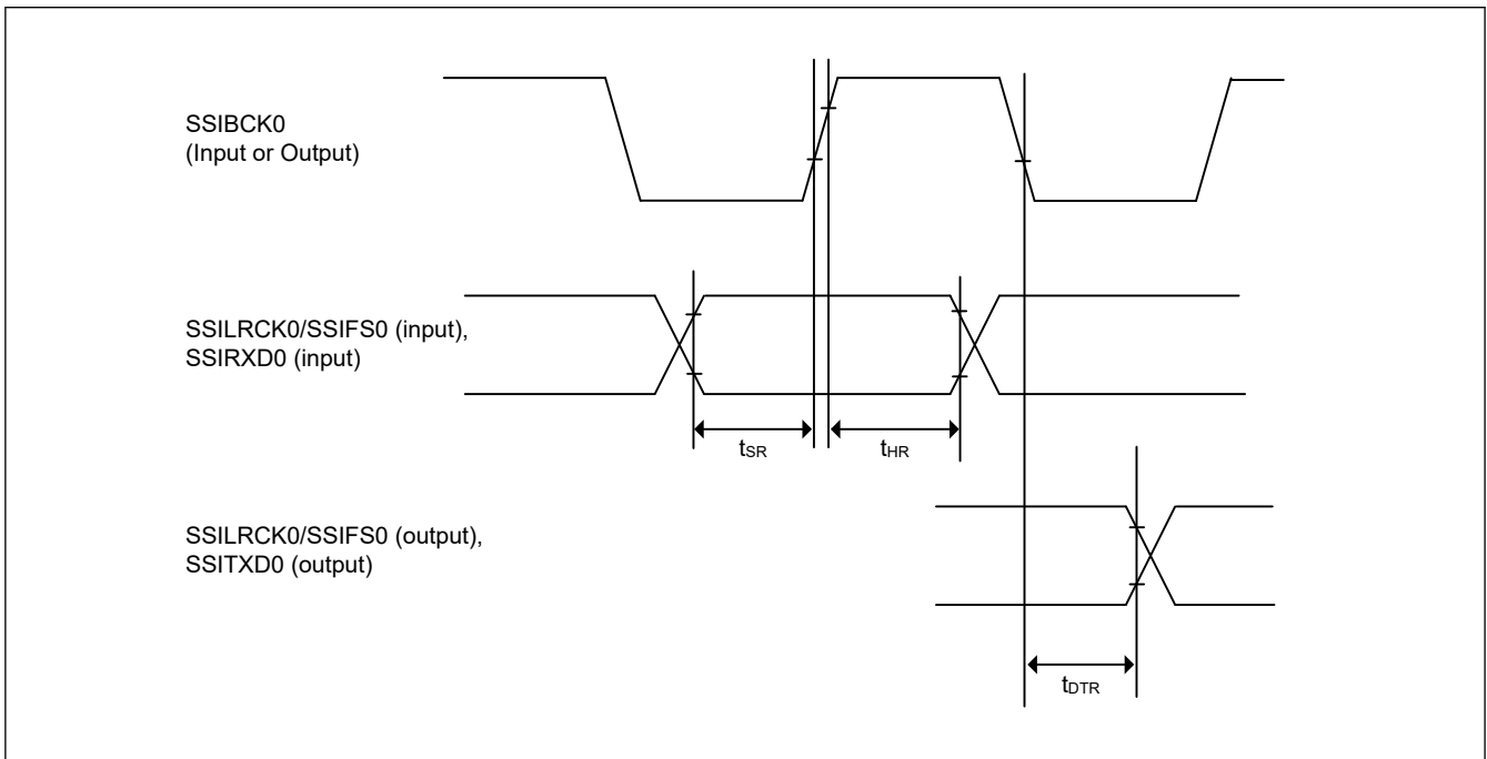
Figure 49.54 SSIE data transmit and receive timing when SSICR.BCKP = 0
