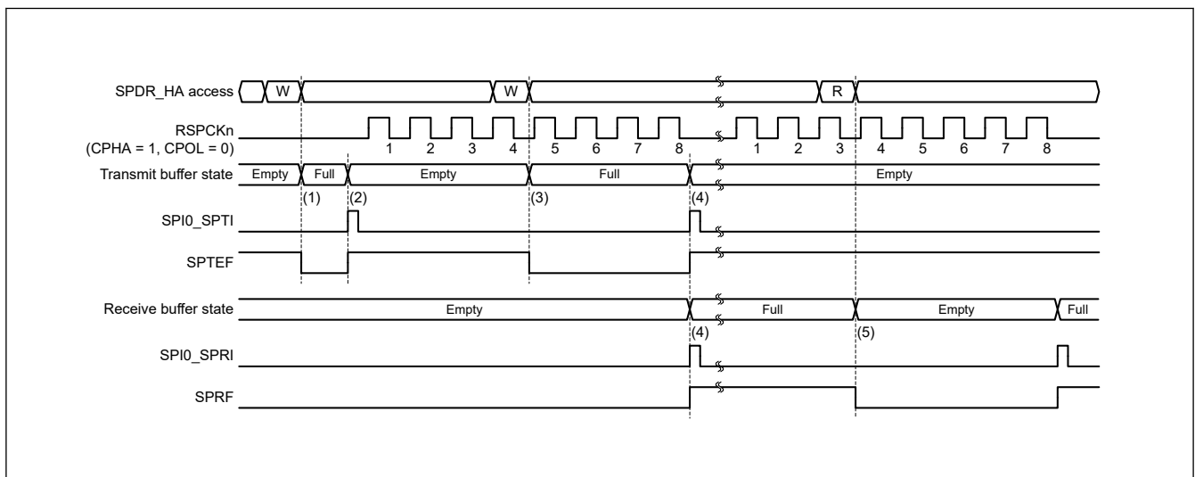
Figure 33.30 Operation example of the SPI0_SPTI and SPI0_SPRI interrupts when CPHA = 1 and CPOL = 0 in master mode
