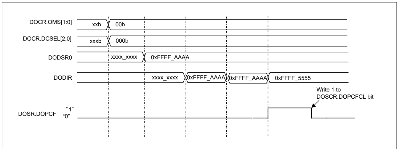
Figure 43.2 Example of Operation in Data Comparison Mode (Detection condition: Mismatch)
