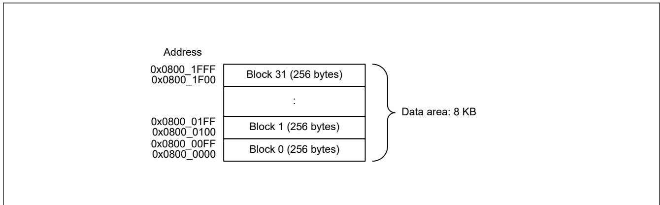
Figure 45.4 Map of the data flash memory
