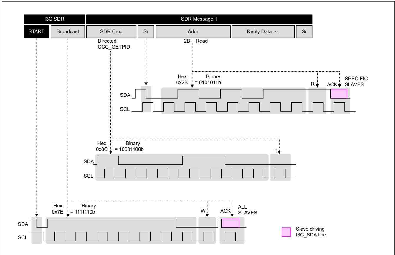
Figure 29.72 Example communication using I3C coding SDR with CCC direct addressing
