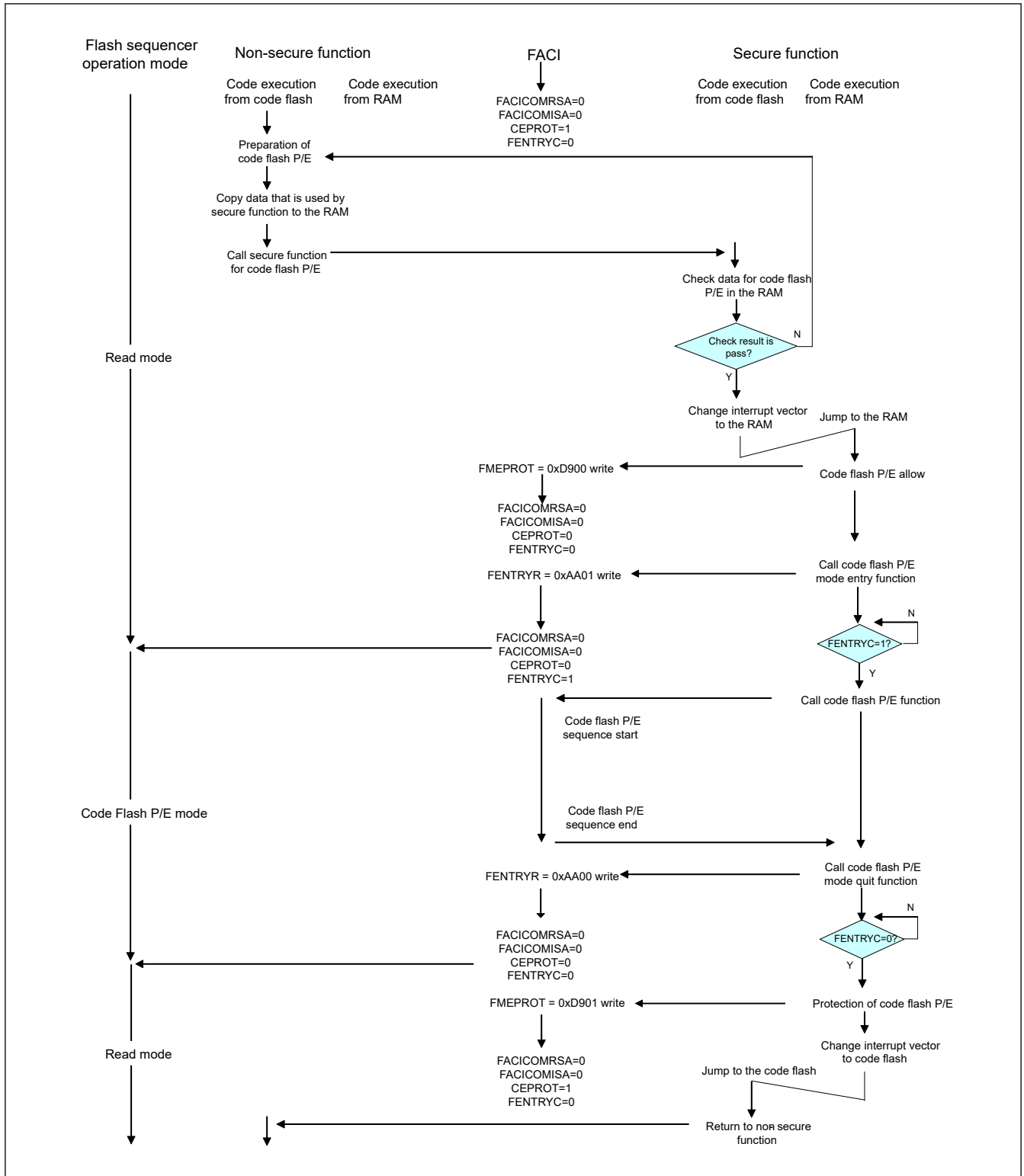
Figure 45.34 Code flash P/E sequence example by non-secure function (using secure function for code flash P/E)
