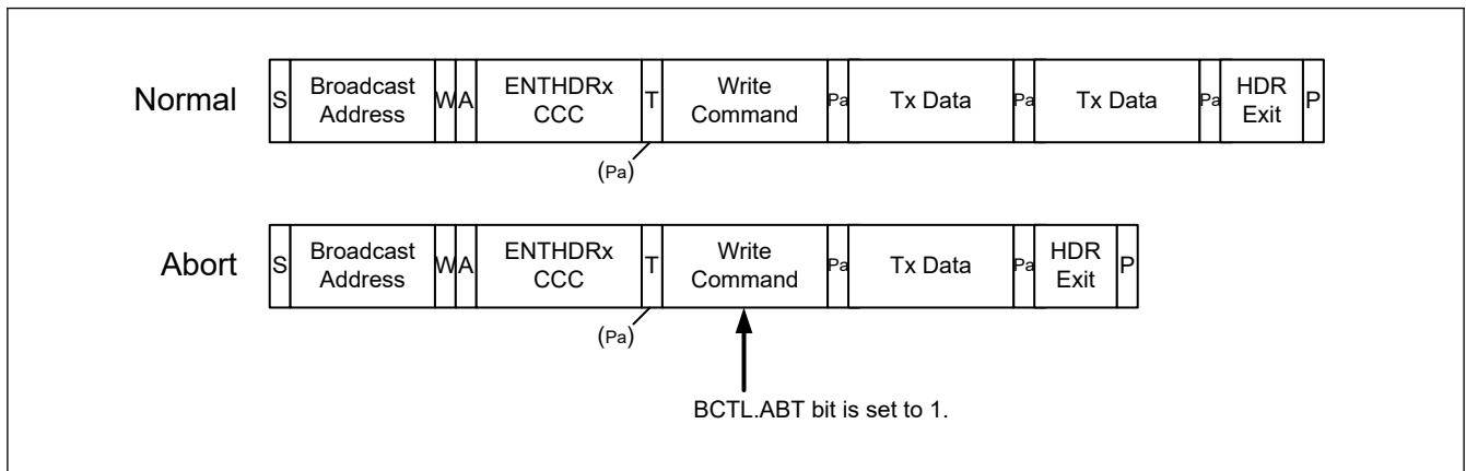
Figure 29.118 Abort operation of HDR-TSP/TSL write transfer
