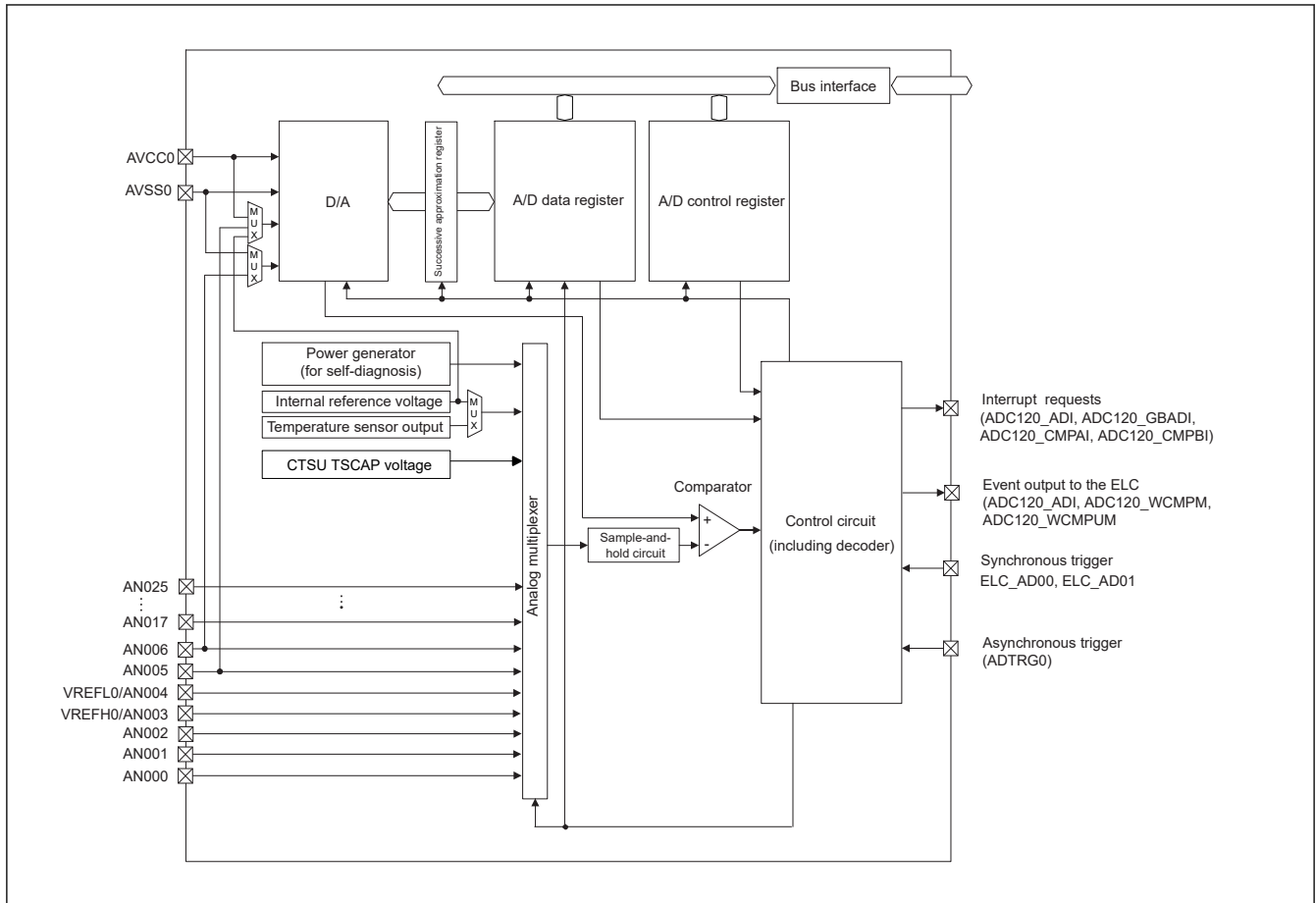
Figure 38.1 ADC12 block diagram
