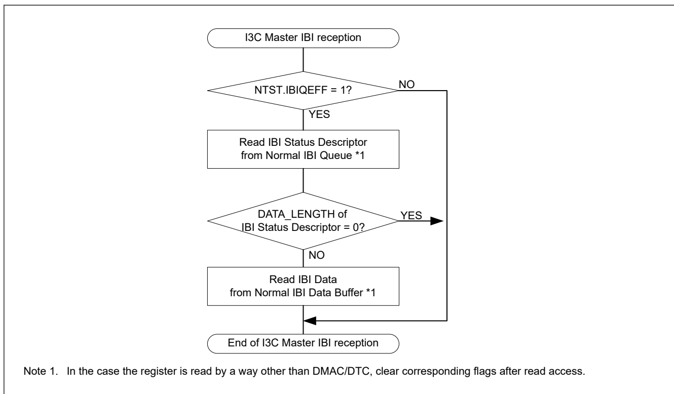
Figure 29.146 Example of I3C master IBI reception flowchart
