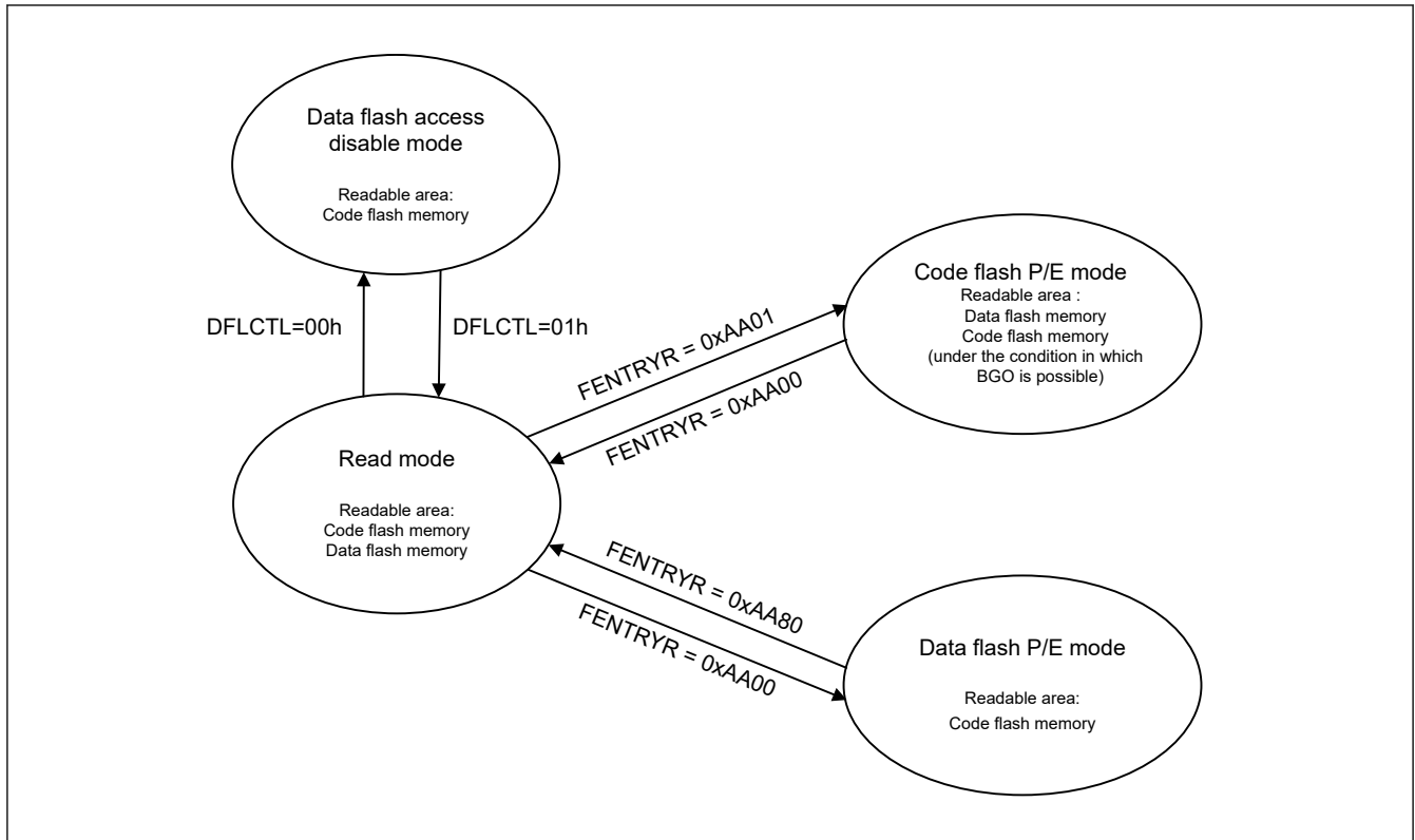
Figure 45.6 Modes of the flash sequencer
