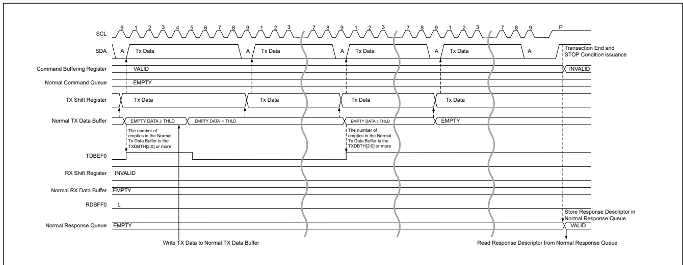
Figure 29.19 Legacy I 2 C message data write timing (2/2)
