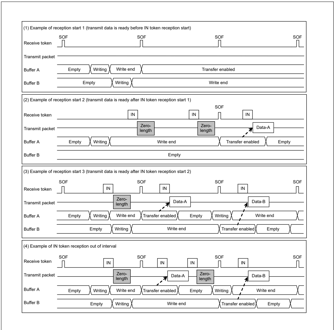
Figure 25.16 Example data setup operation
