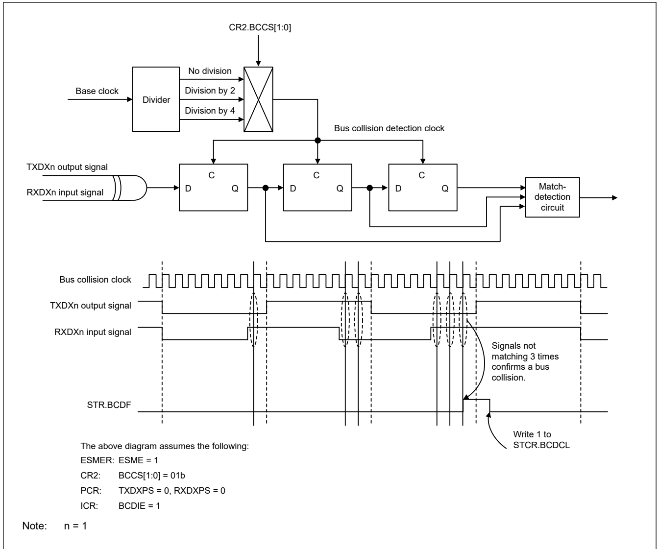
Figure 26.111 Example of operations with bus collision detection
