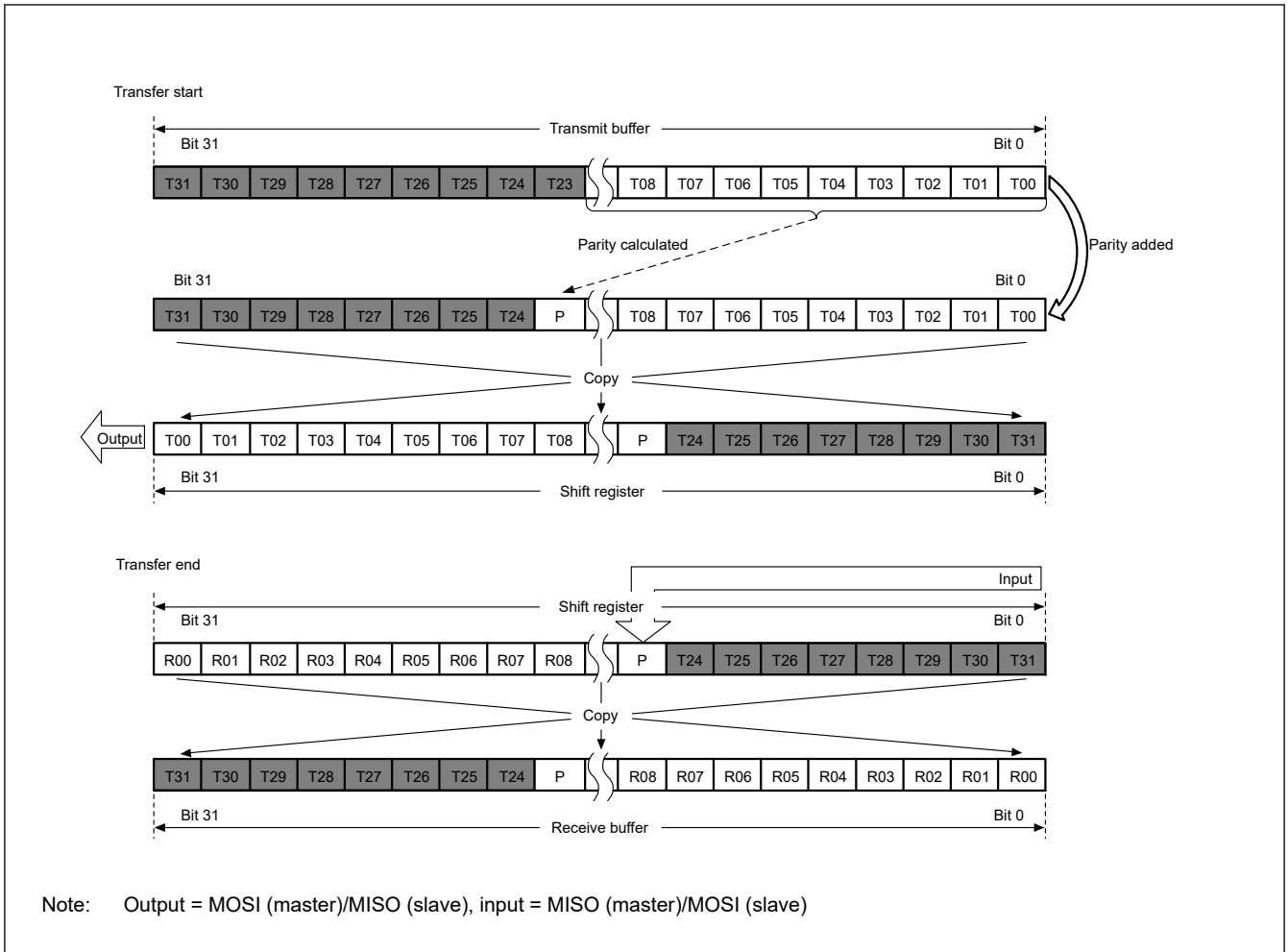
Figure 33.21 LSB-first transfer with 24-bit data and parity enabled
