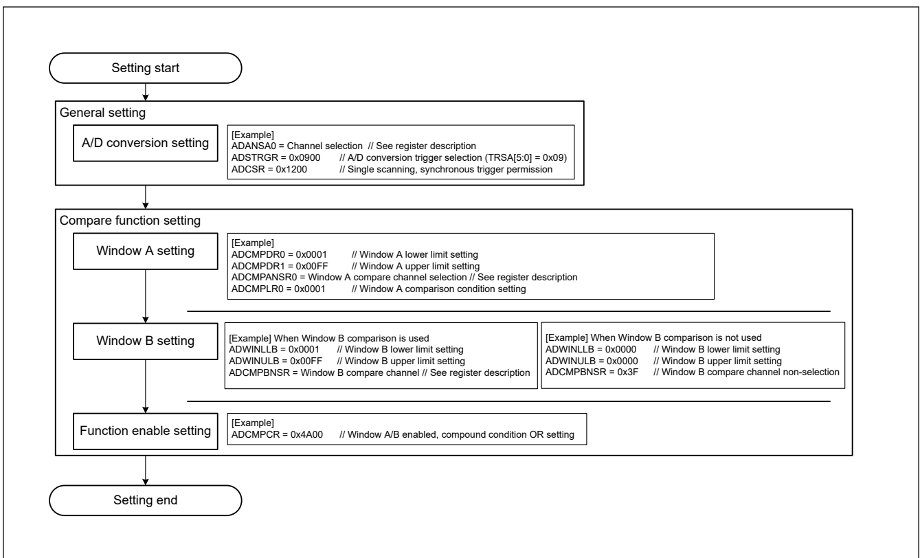
Figure 38.23 Setting example when using the event output of the compare function
