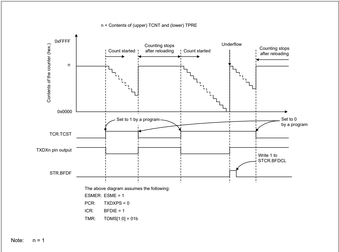
Figure 26.115 Example of operations in Break Field low width output mode
