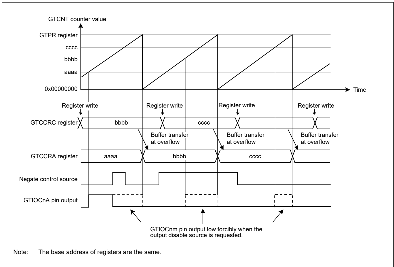
Figure 20.69 Example of GTIOcnm pin output disable control operation in saw-wave up-counting, buffer operation, active level 1, high output at GTCCRA compare match, low output at cycle end, and low output at output disable (n = 0 to 5, m = A, B)
