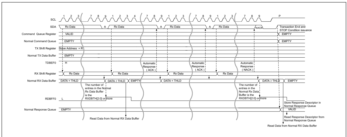
Figure 29.21 SDR data read transfer timing (2/2)
