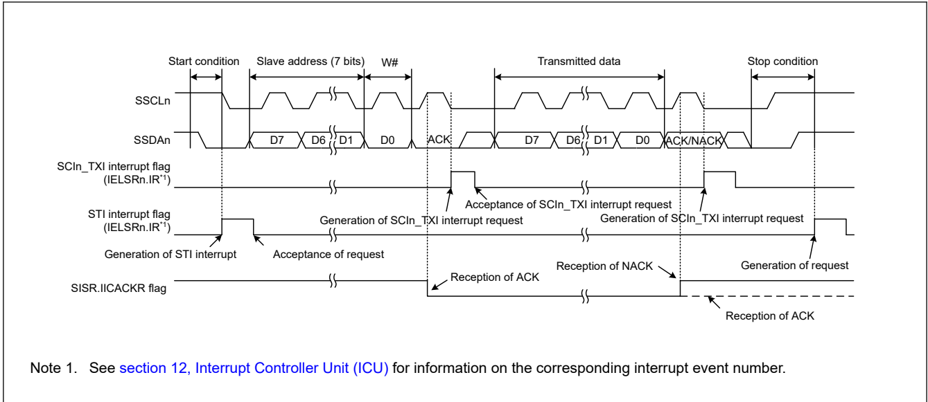
Figure 26.93 Example 1 of operations for master transmission in simple IIC mode with 7-bit slave addresses, transmission interrupts, and reception interrupts
