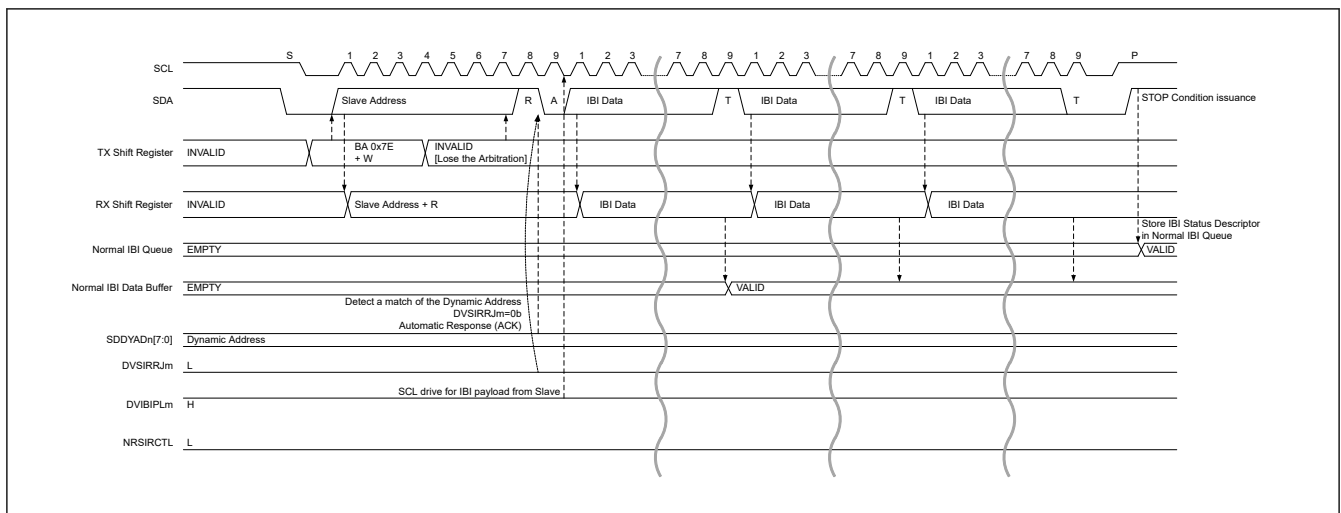
Figure 29.98 Slave interrupt request : ACK and DVIBIPL = 1
