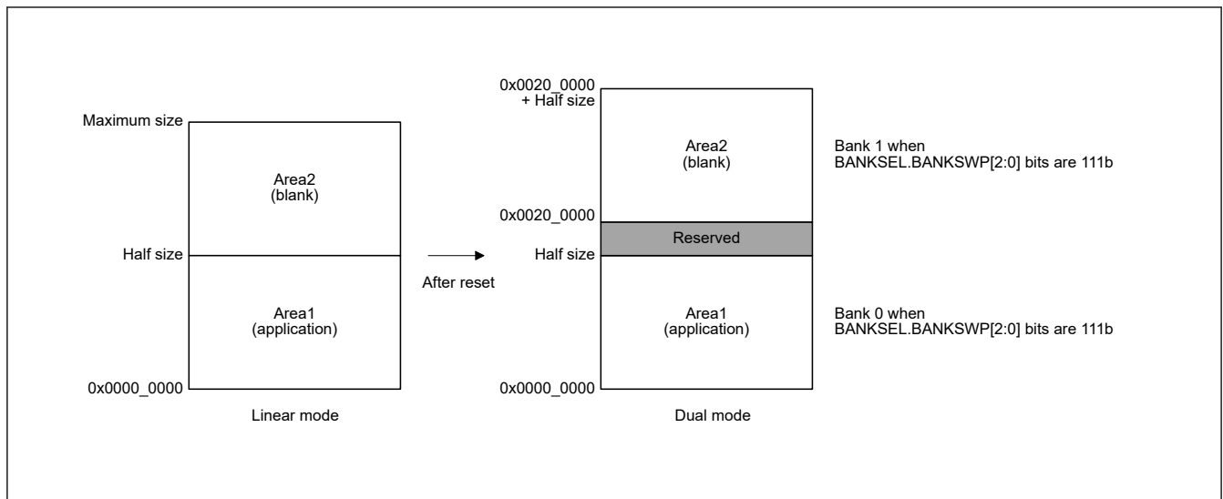
Figure 45.42 Programming the application for the dual mode in the linear mode
