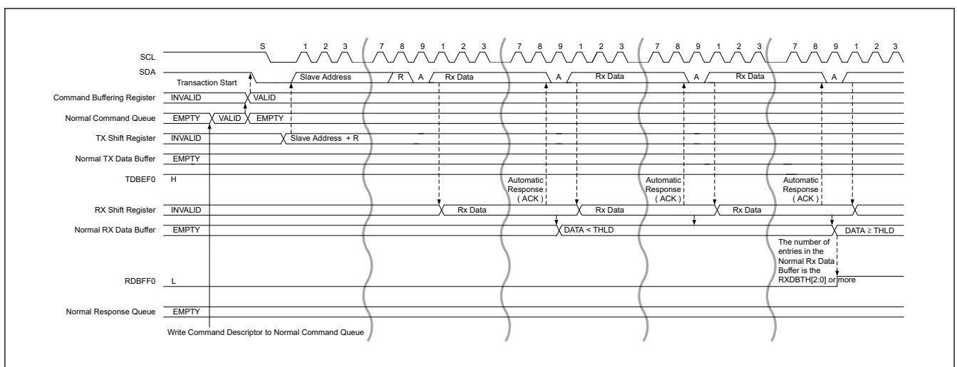
Figure 29.22 Legacy I2C message data read transfer timing (1/2)
