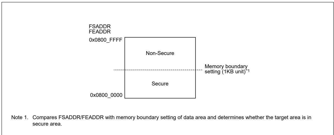
Figure 45.32 Secure/non-secure region in data area
