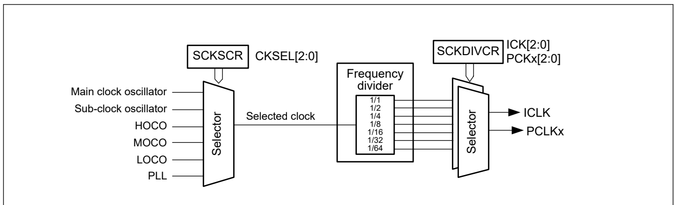
Figure 8.13 Block diagram of clock source selector
