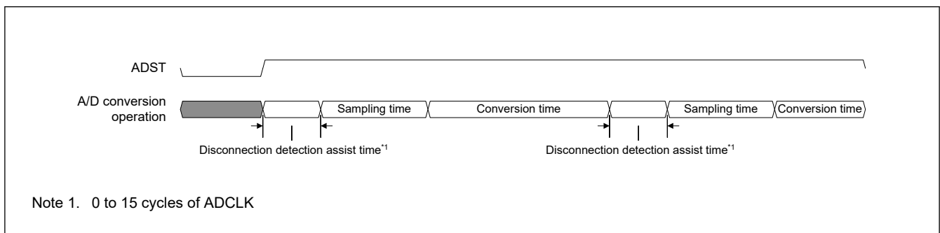
Figure 38.27 Operation of A/D conversion when disconnection detection assist function is used
