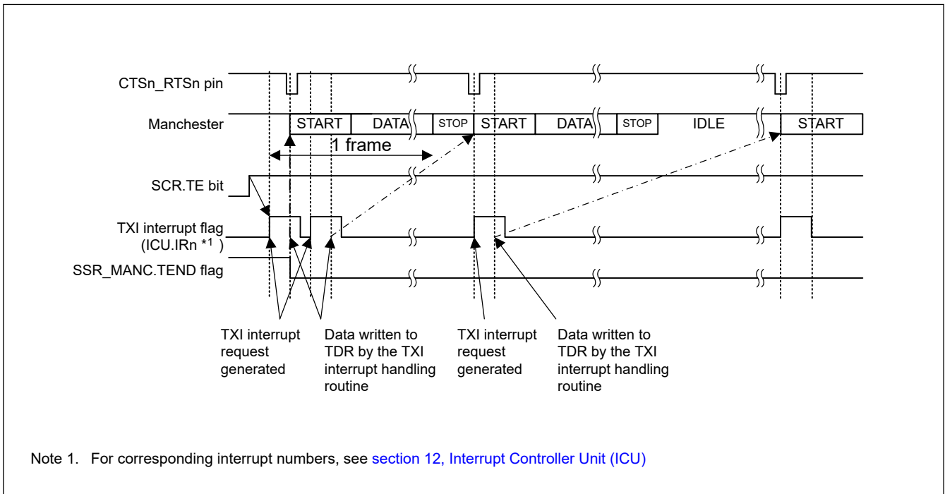
Figure 26.57 Example of Start-of-Transmission Operation for Serial Transmission in Manchester Mode (Without Preface but with the CTS Function)
