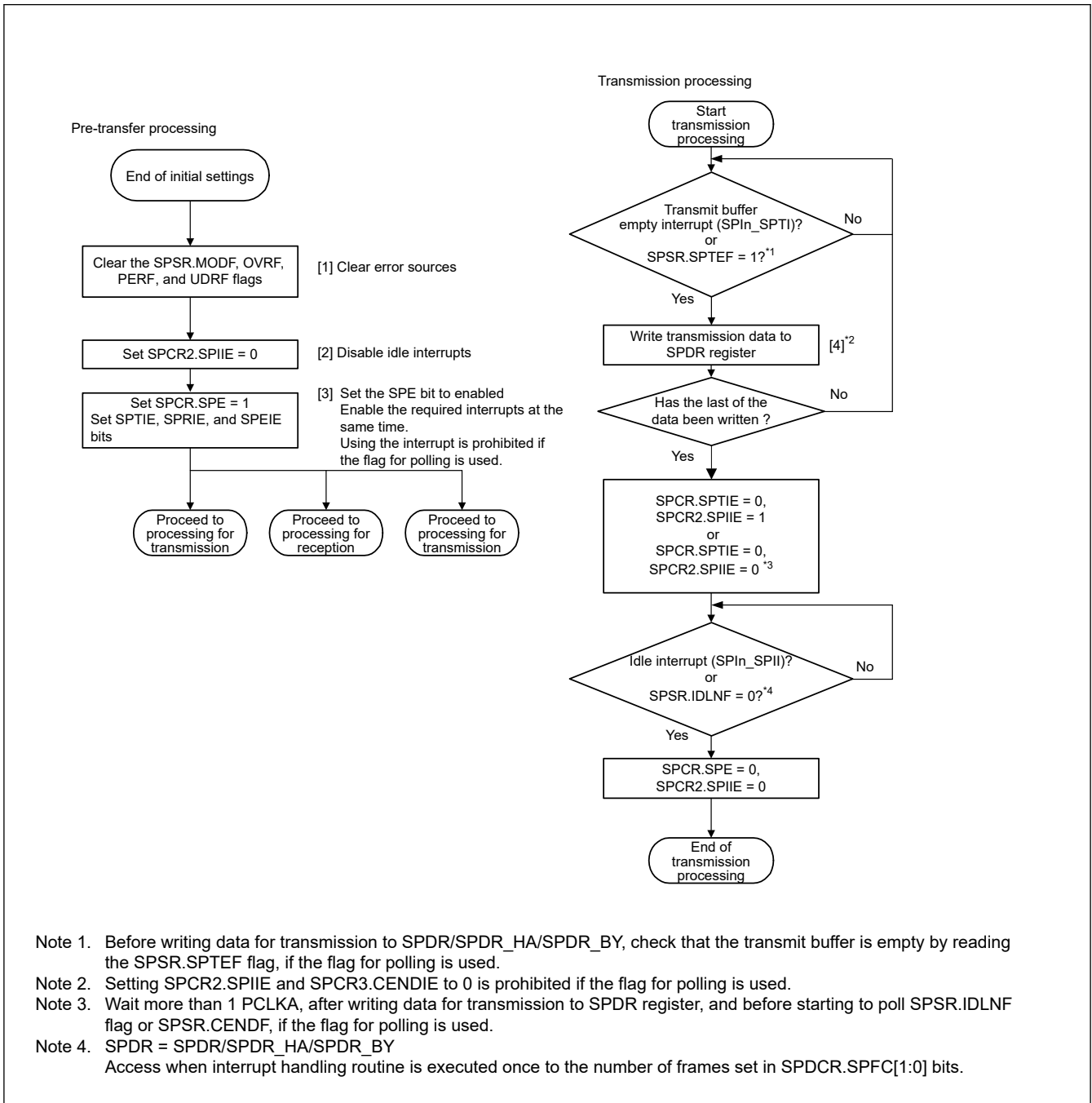
Figure 33.51 Transmission flow in master mode
