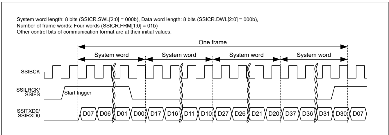
Figure 35.40 TDM format (without padding: system word length = data word length)
