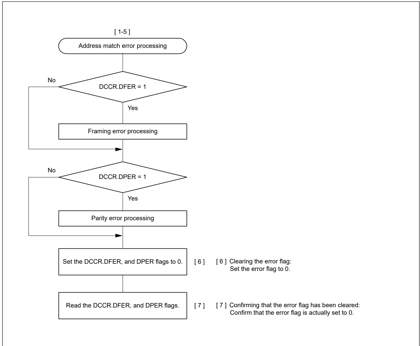
Figure 26.23 Example Flowchart of Serial Reception in Asynchronous Mode (FIFO not Selected and Address Matching Enabled) (2)
