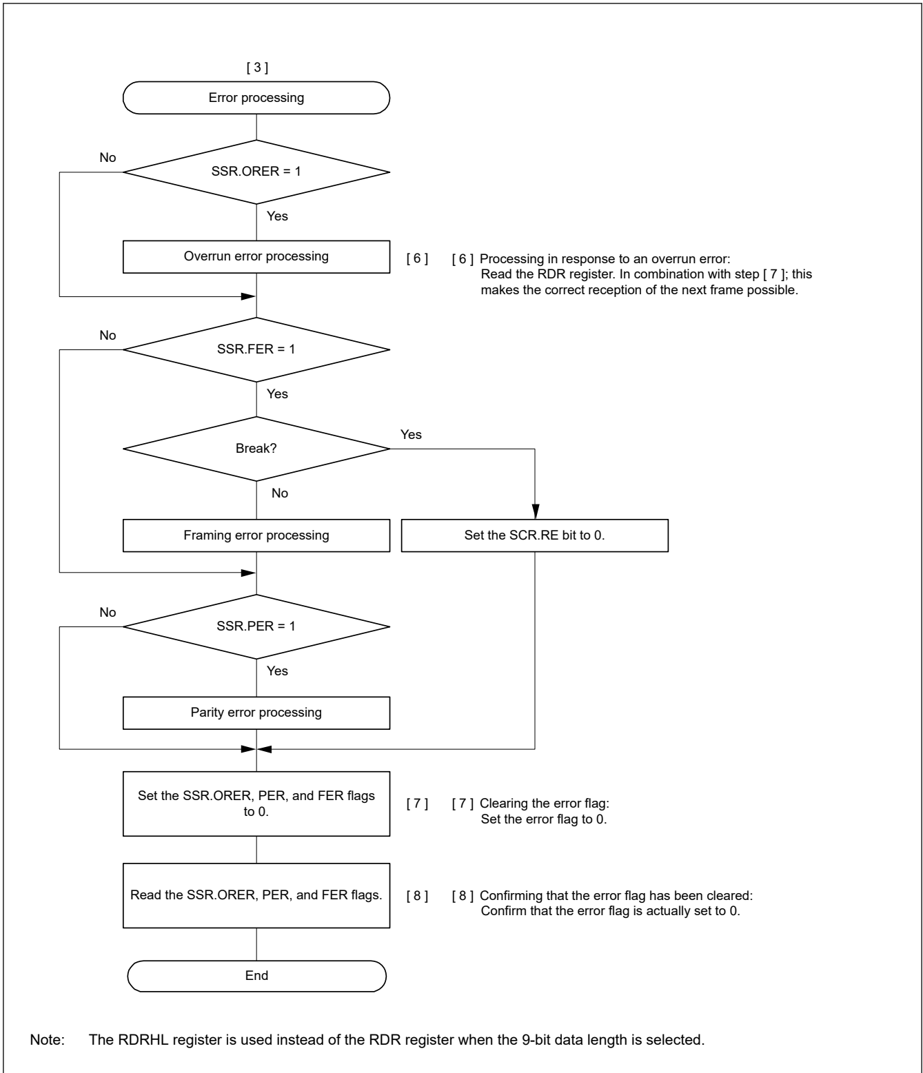
Figure 26.24 Example Flowchart of Serial Reception in Asynchronous Mode (FIFO not Selected and Address Matching Enabled) (3)
