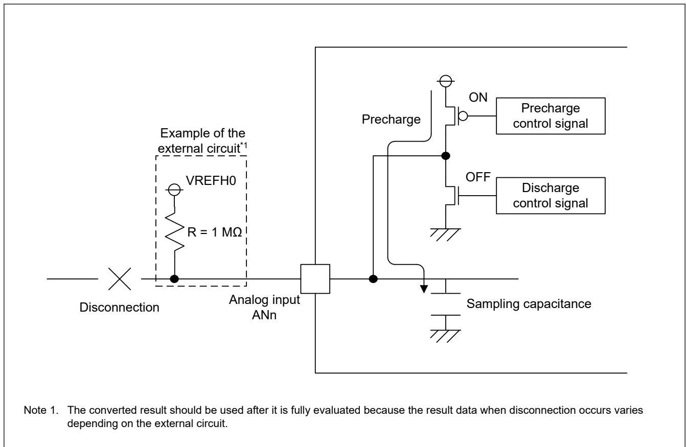
Figure 38.28 Example of disconnection detection when precharge is selected
