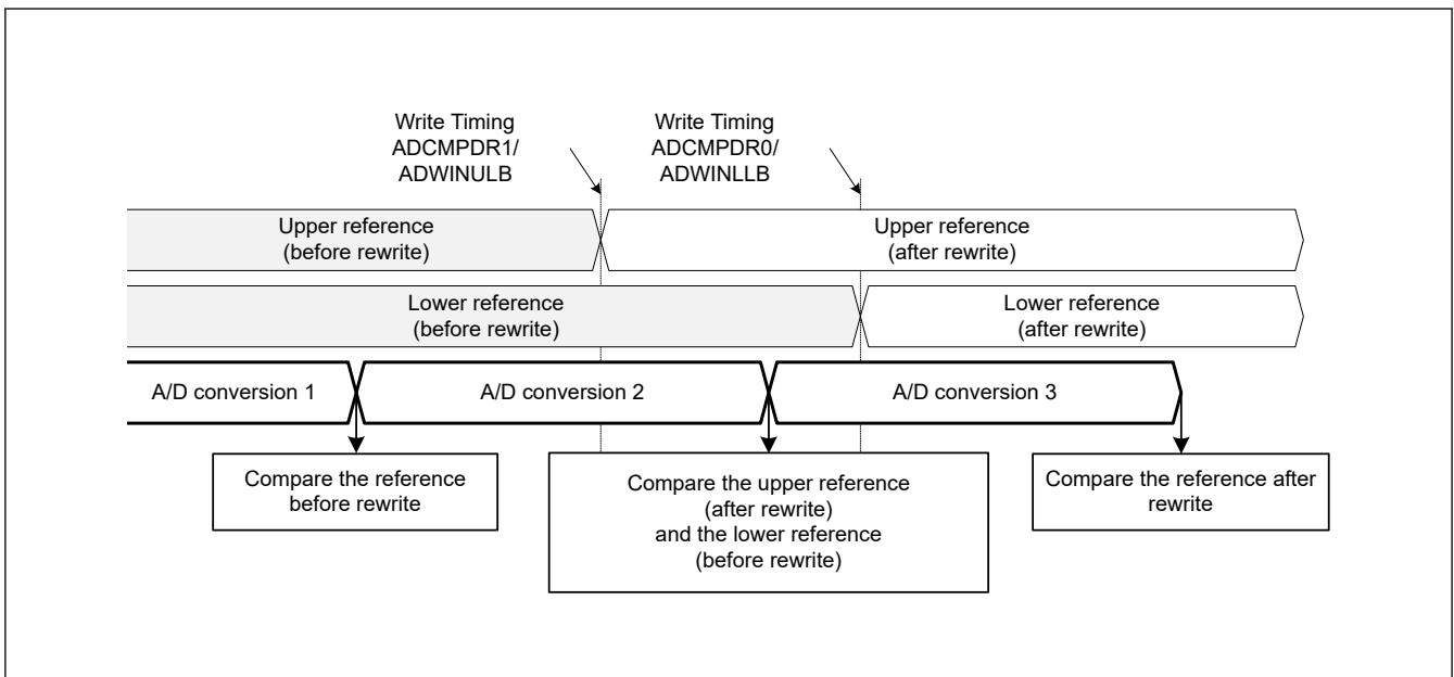
Figure 38.4 Comparison between upper and lower references before and after a rewrite
