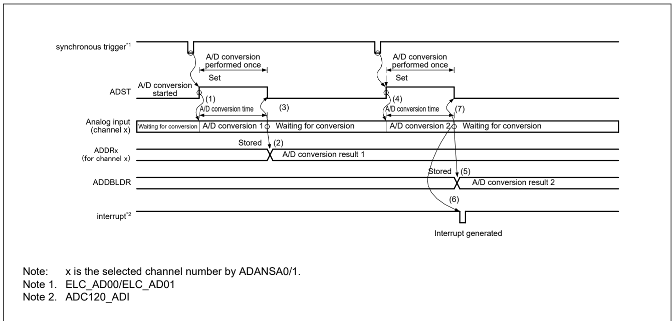
Figure 38.10 Example operation in single scan mode when double-trigger mode is selected and the analog input (channel x) is duplicated
