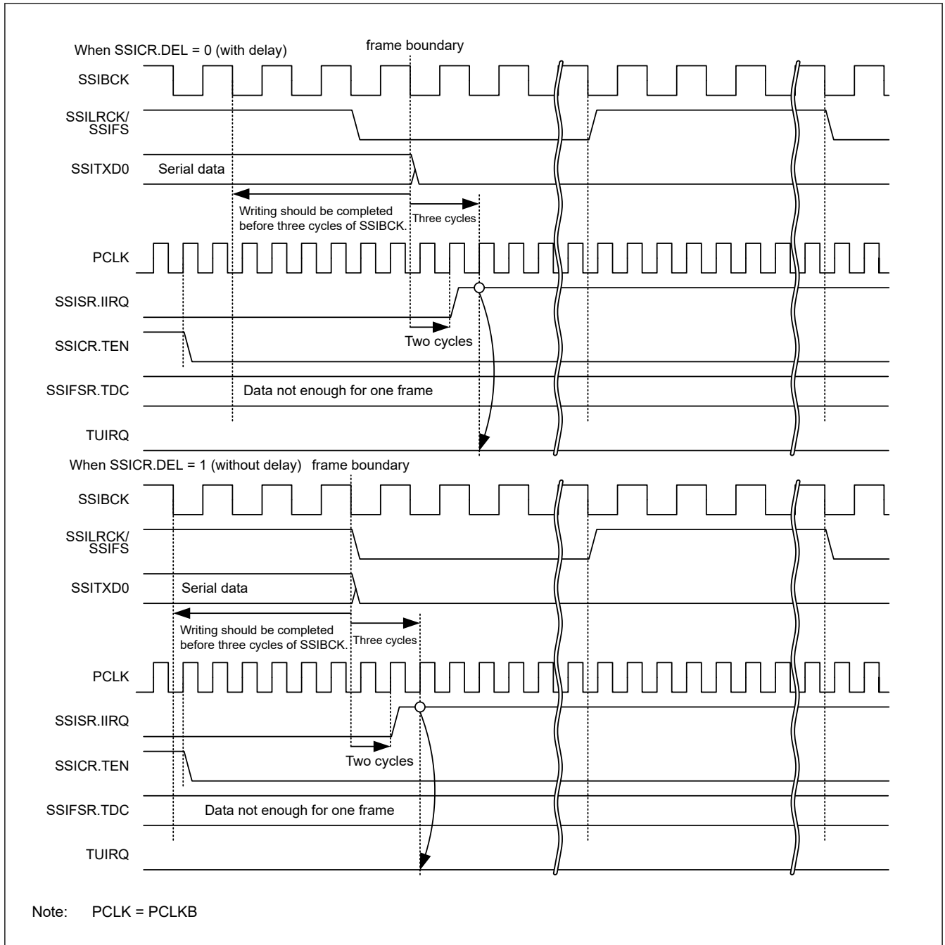
Figure 35.20 TUIRQ setting timing (when communication stops)
