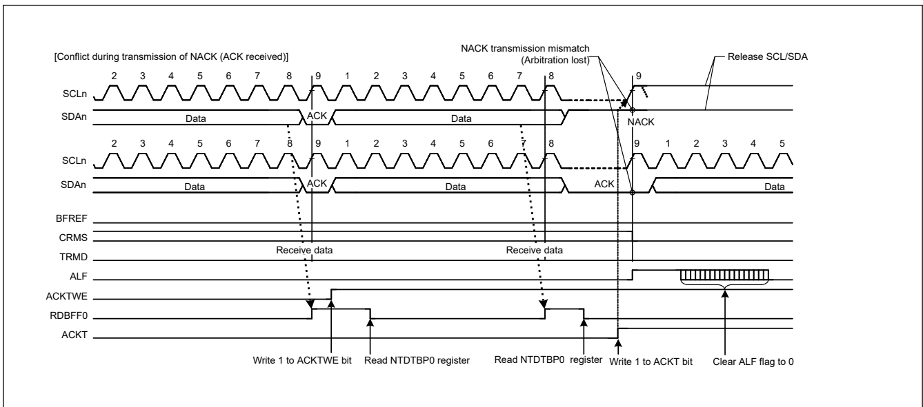
Figure 29.89 Example of arbitration-lost detection during transmission of NACK (NALE = 1)
