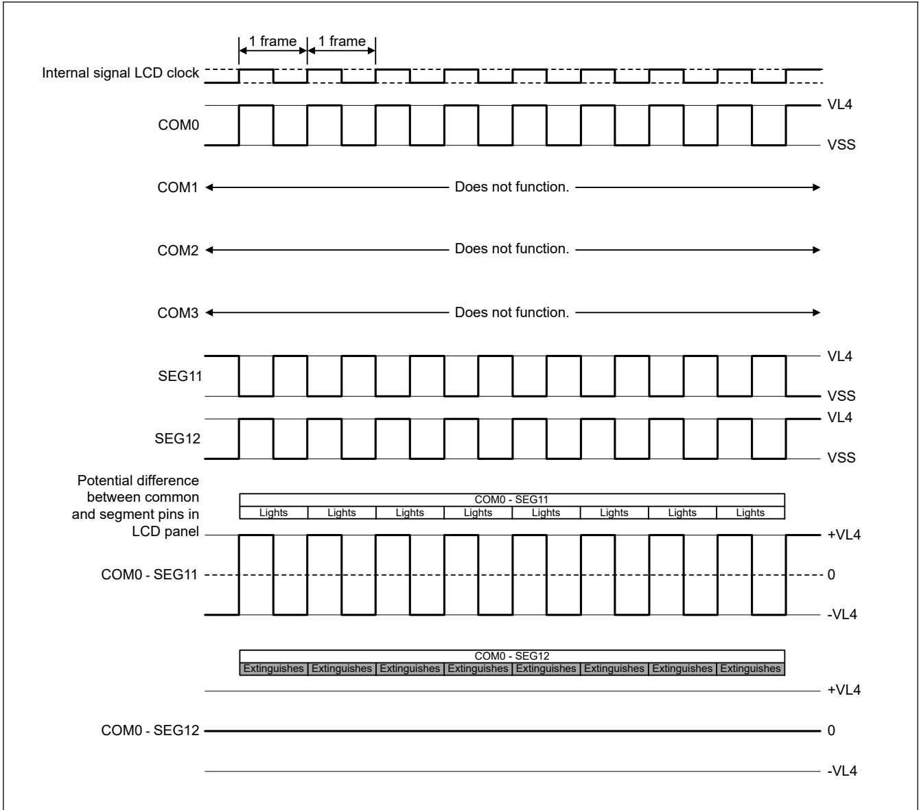
Figure 46.24 Static LCD drive waveform examples for SEG11, SEG12, and COM0
