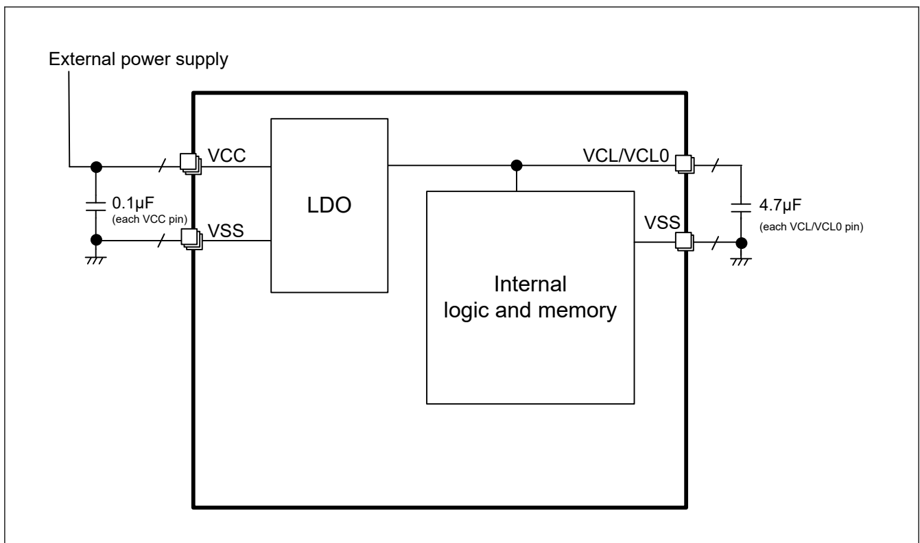
Figure 47.1 LDO settings
