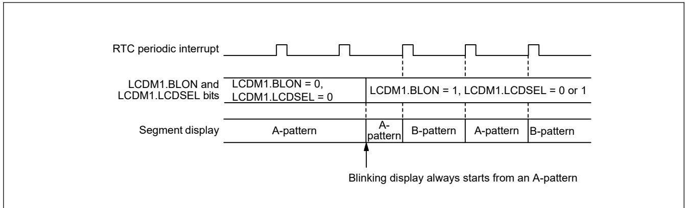
Figure 46.3 Switching operation from A-pattern display to blinking display
