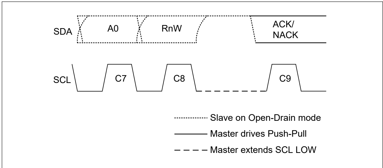
Figure 29.94 Master clock stalling in ACK phase
