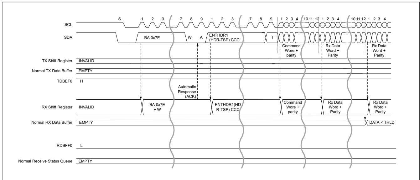
Figure 29.56 HDR data write transfer (HDR-TSP, TSL) timing (1/2)
