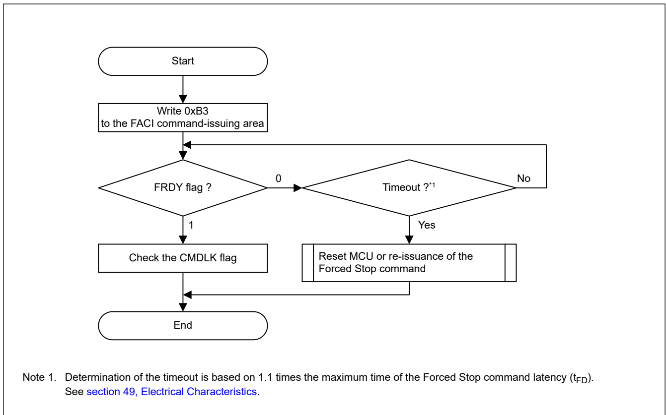
Figure 45.18 Usage flow of the Forced Stop command
