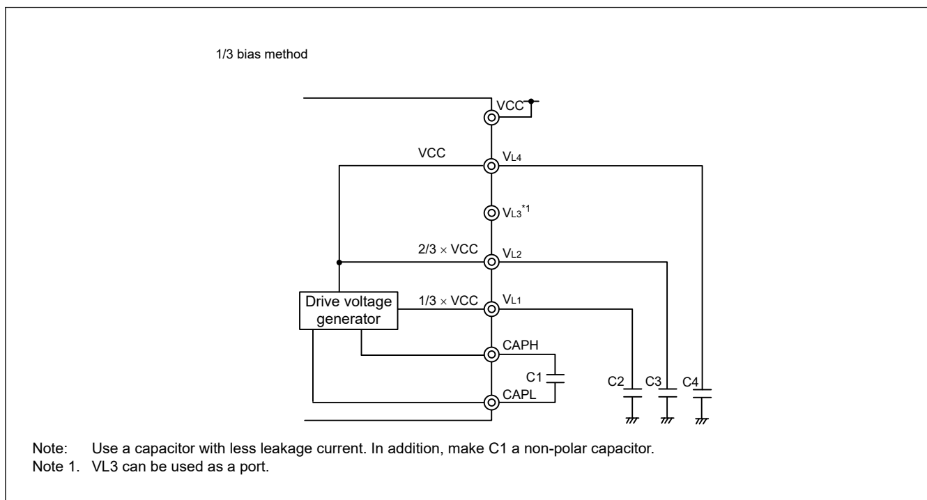
Figure 46.14 Examples of LCD drive power connections using VCC reference mode of capacitor split method
