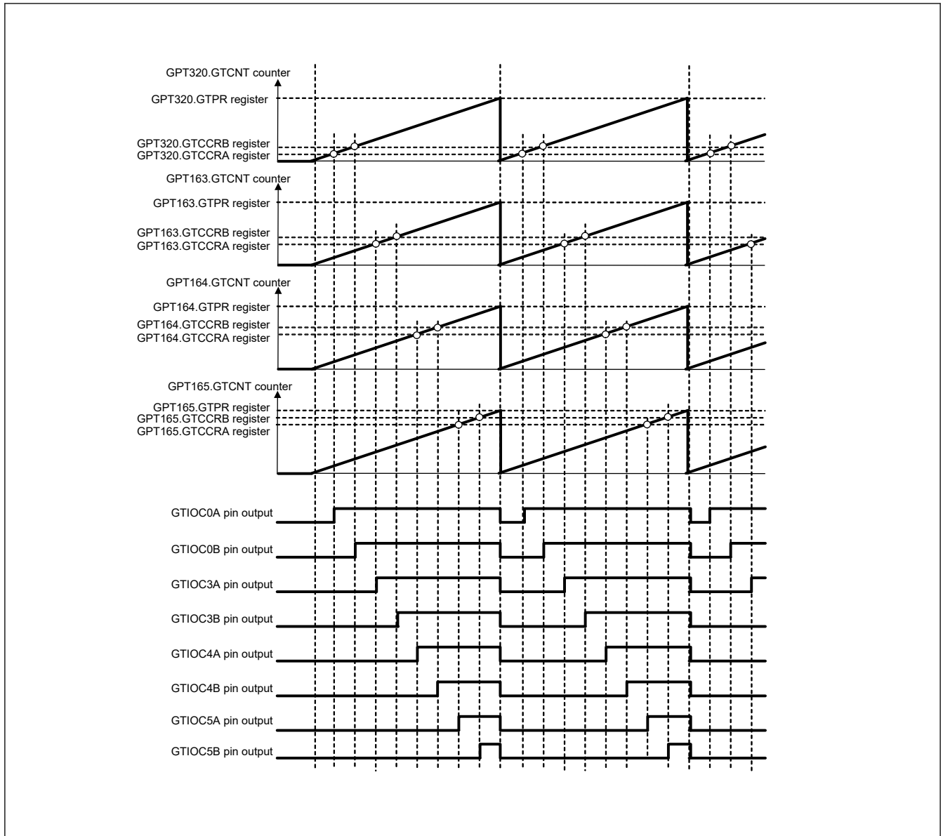
Figure 20.42 Example of synchronized PWM output
