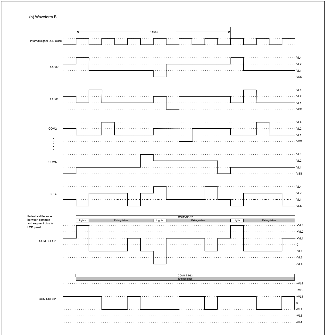
Figure 46.39 Six-time slice LCD drive waveform examples between SEG2 and each common signal using 1/3 bias method
