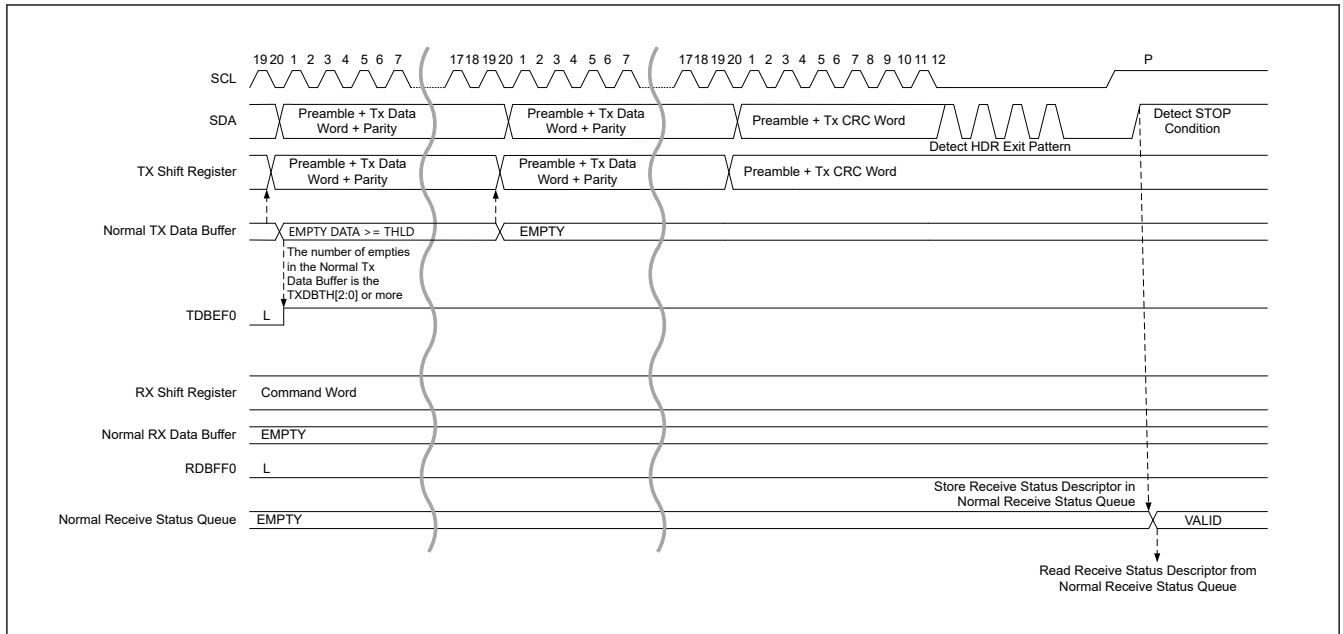
Figure 29.60 HDR data read transfer (HDR-DDR) timing (3/3)
