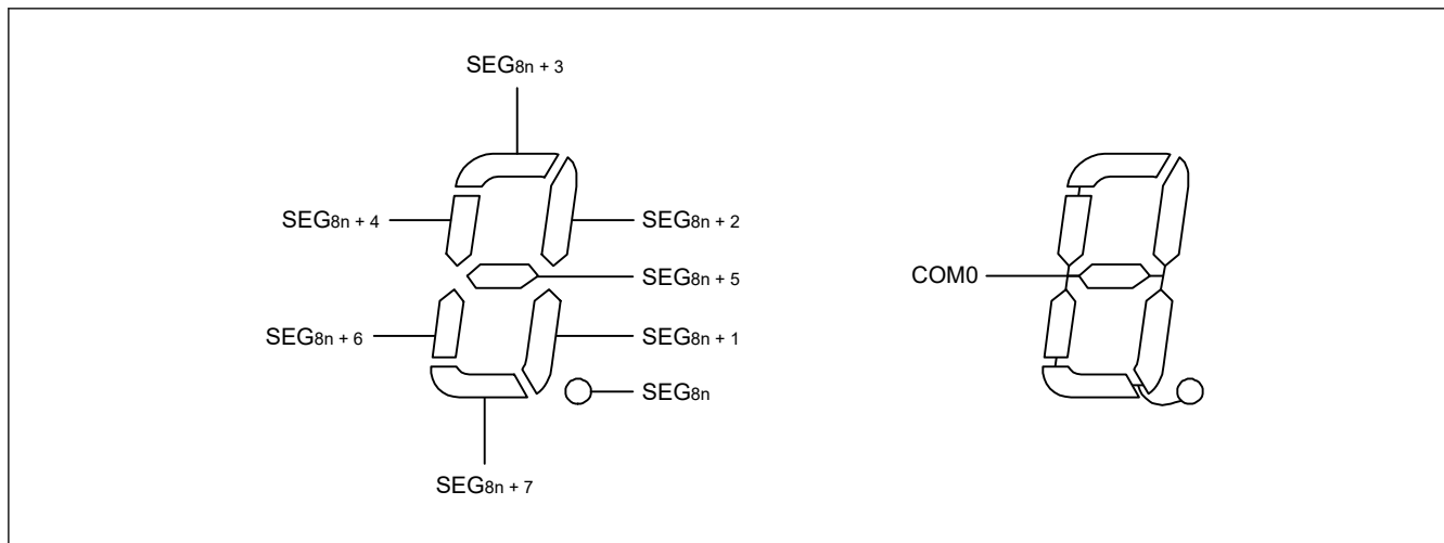
Figure 46.22 Static LCD display pattern and electrode connections
