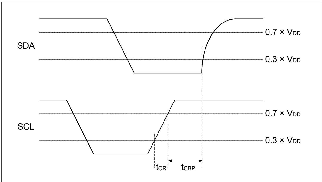
Figure 49.46 I3C STOP condition timing
