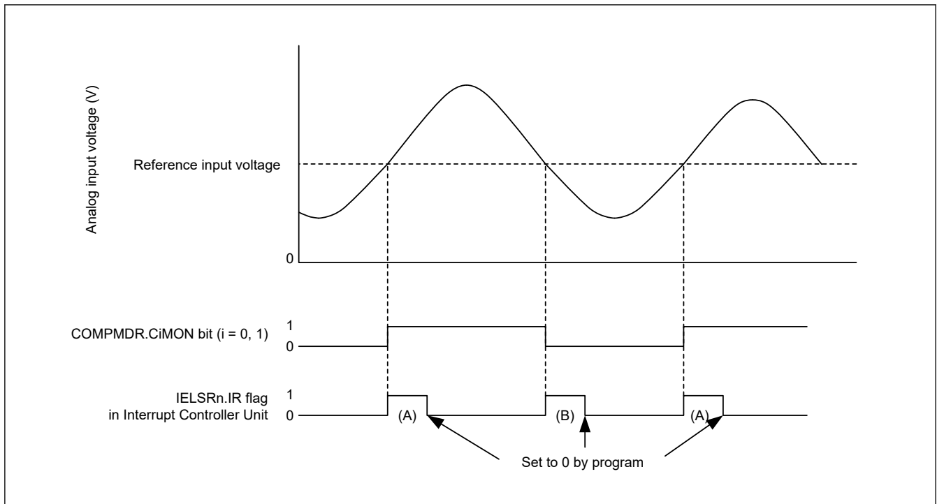
Figure 41.3 Operating example of ACMPLPi ( i = 0, 1 ) when window function is disabled
