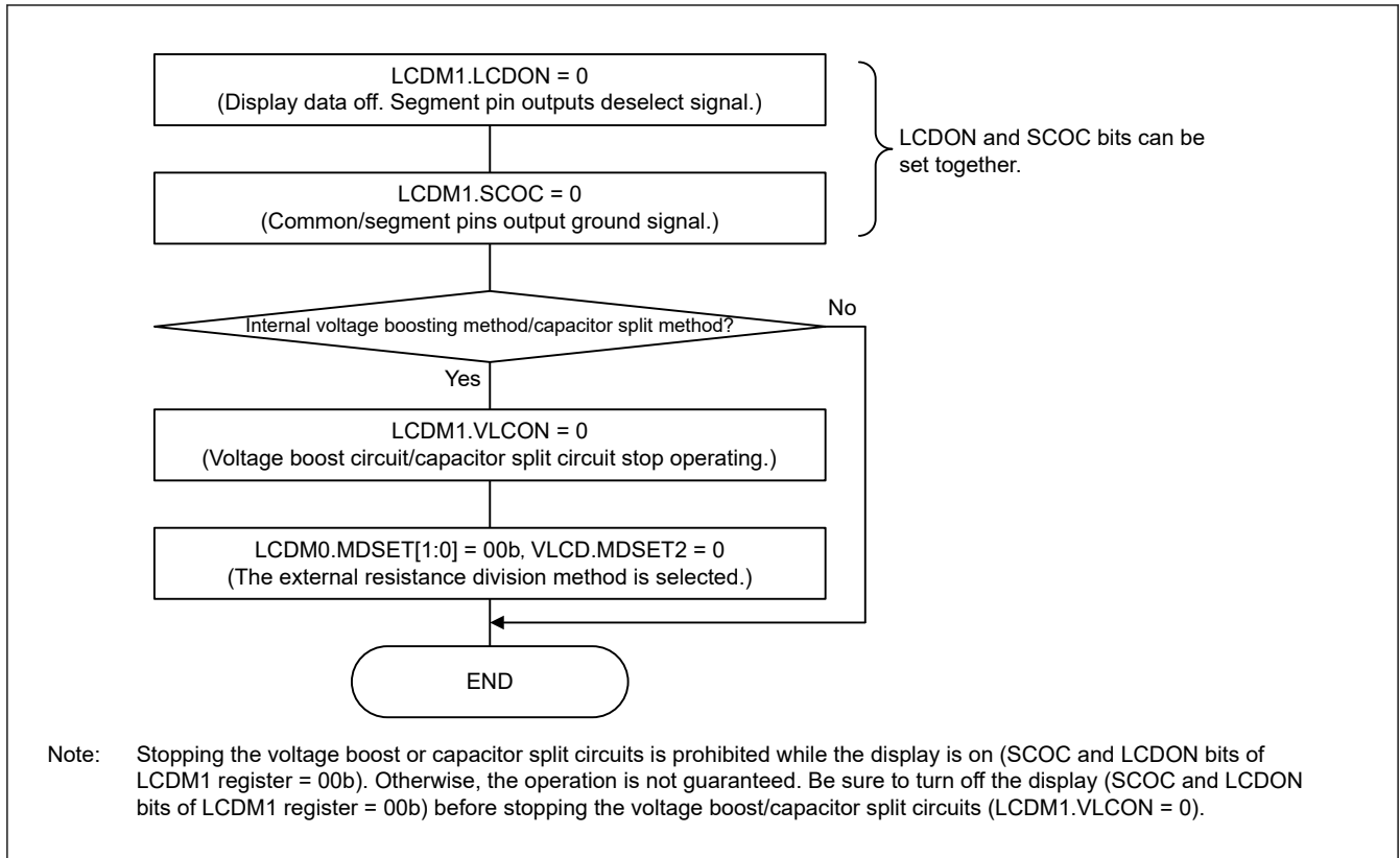
Figure 46.9 Operation stop procedure during normal liquid crystal waveform (A or B) display
