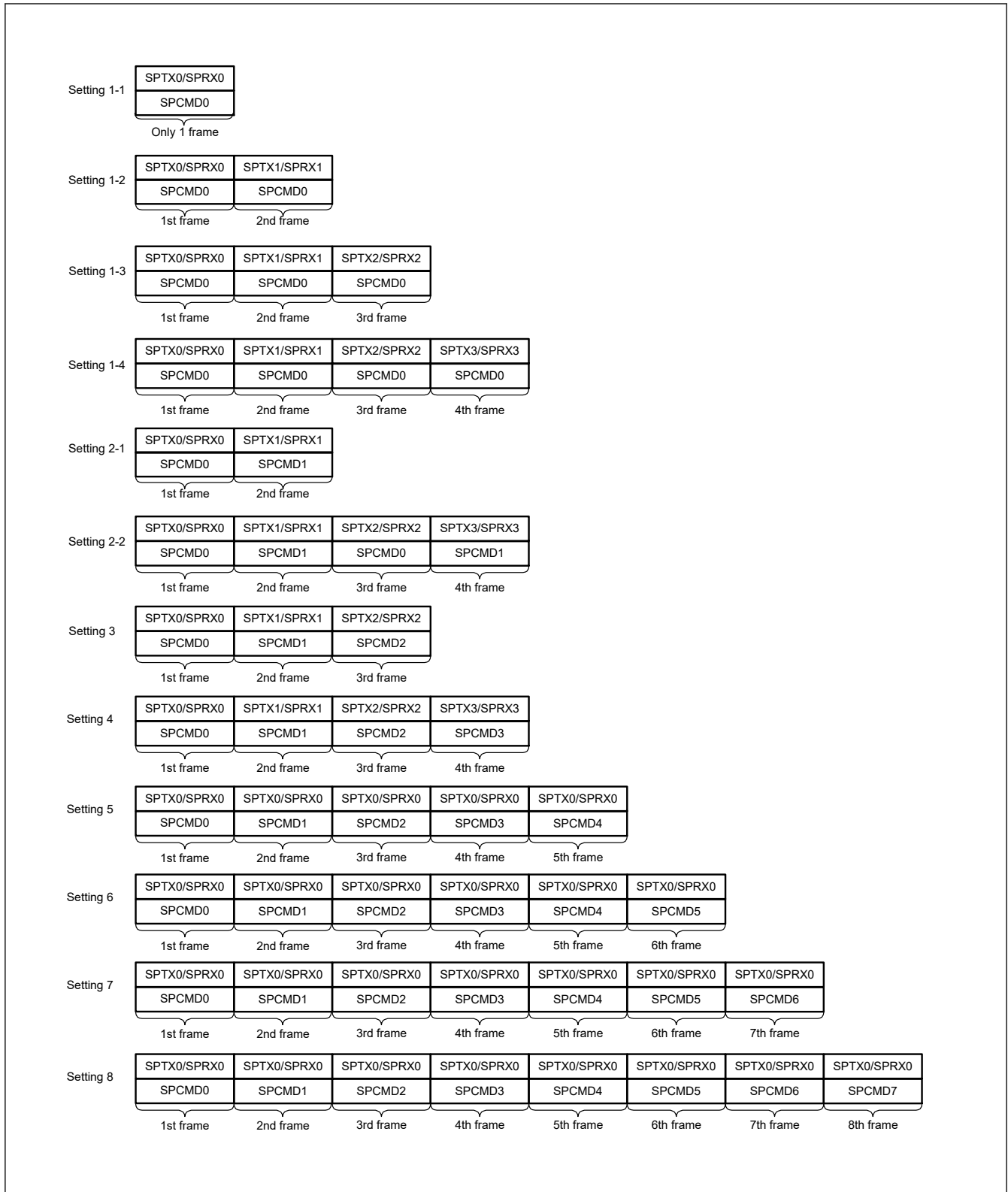
Figure 33.47 Correspondence between SPI Command Register and transmit and receive buffers in sequence operations
