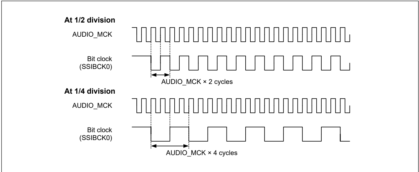
Figure 35.5 Sampling frequencies in master-mode communication
