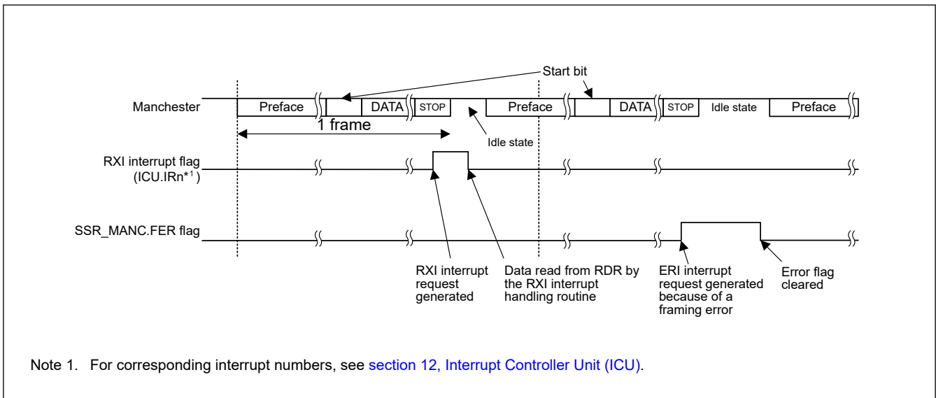
Figure 26.60 Example of Operation for Serial Data Reception in Manchester mode (with a Preface)
