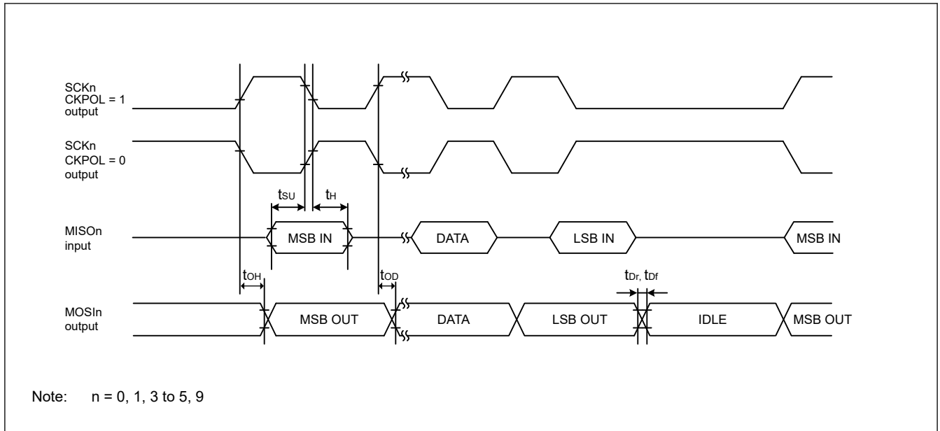
Figure 49.27 SCI simple SPI mode timing (master, CKPH = 0)
