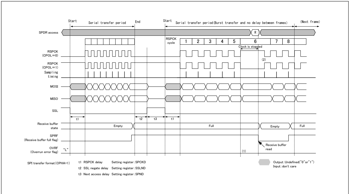
Figure 33.42 Clock stop waveform when serial transfer continues in the receive buffer full in master mode (at burst transfer and no delay between frames CPHA = 1)
