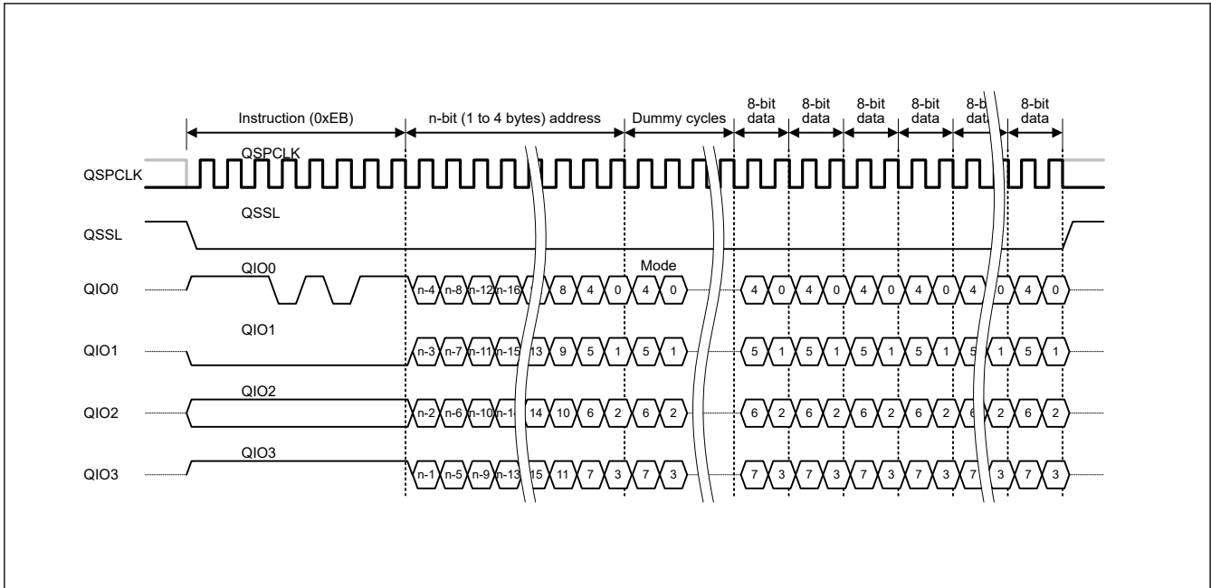
Figure 34.27 Fast Read Quad I/O bus cycle
