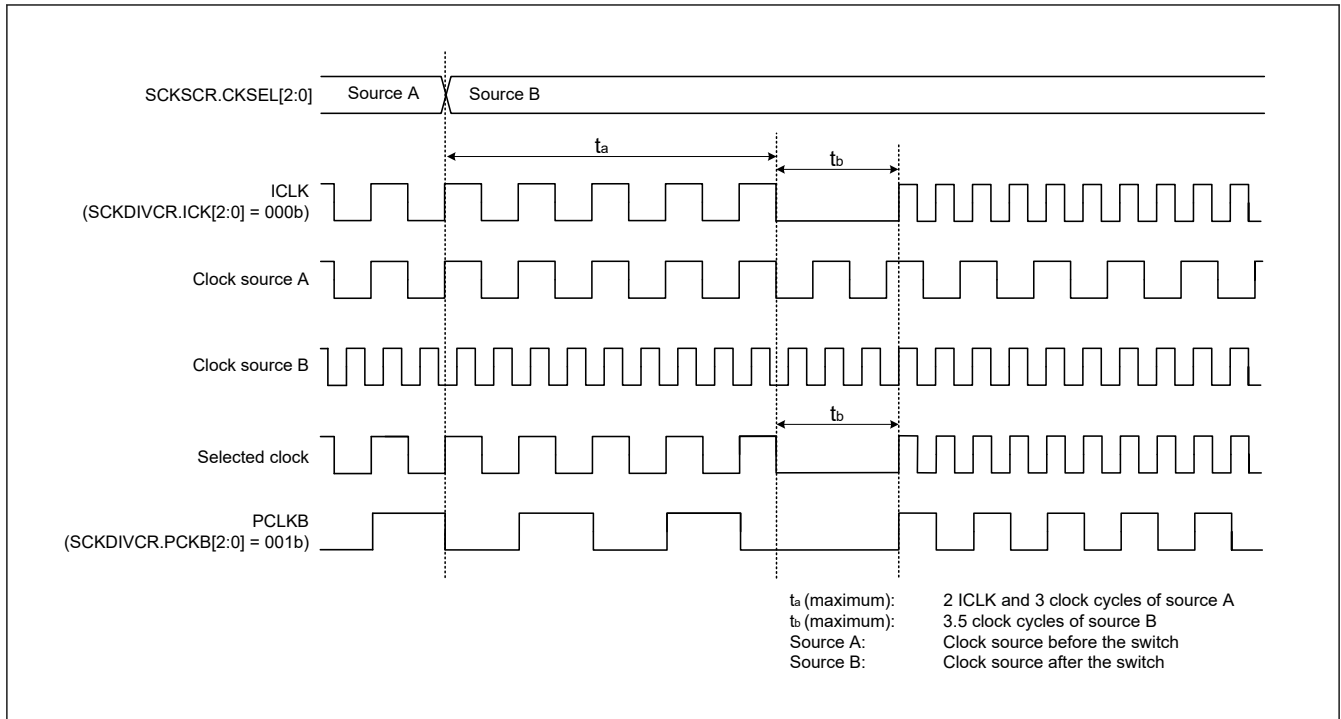
Figure 8.14 Timing of clock source switching
