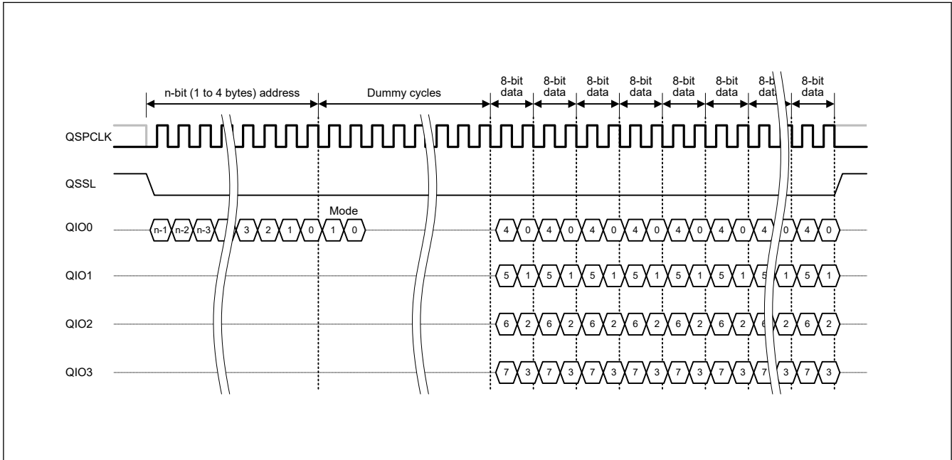
Figure 34.26 Fast Read Quad Output bus cycle in XIP mode (with extended SPI protocol)
