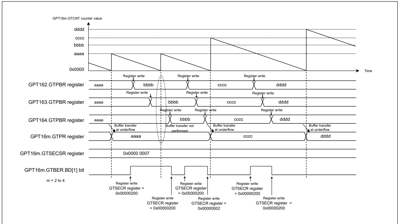
Figure 20.68 Example of multiple channel operation for disabling buffer operation (saw waves, single buffer operation)
