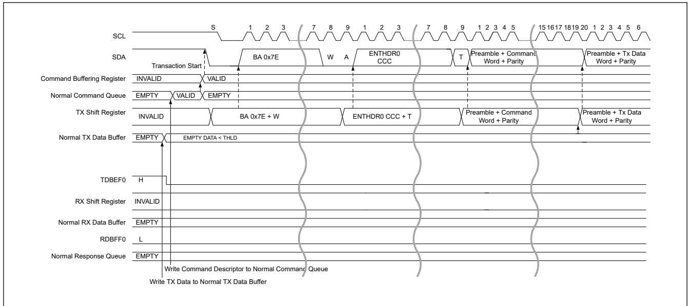
Figure 29.24 HDR data write transfer (HDR-DDR) timing (1/4)
