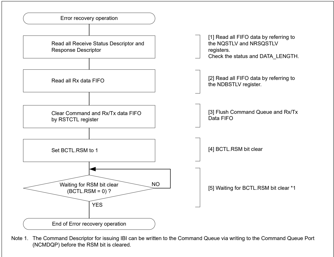
Figure 29.121 Example of error recovery operation flowchart for I3C slave
