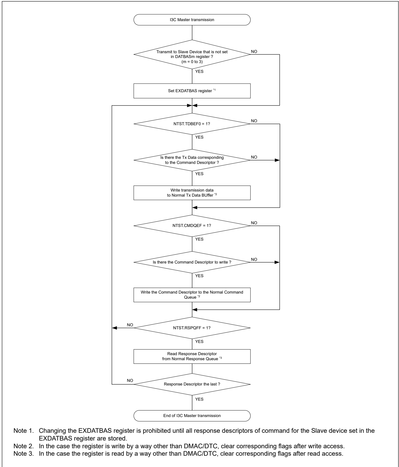
Figure 29.144 Example of I3C master transmission flowchart (normal FIFO buffer transfer)
