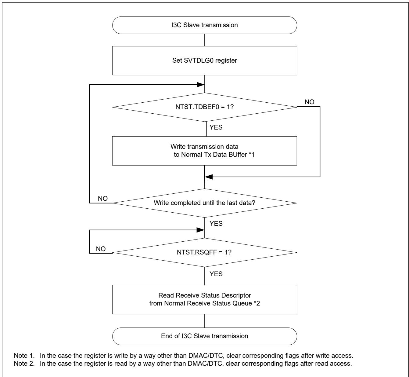
Figure 29.150 Example of I3C slave transmission flowchart (normal FIFO buffer transfer)
