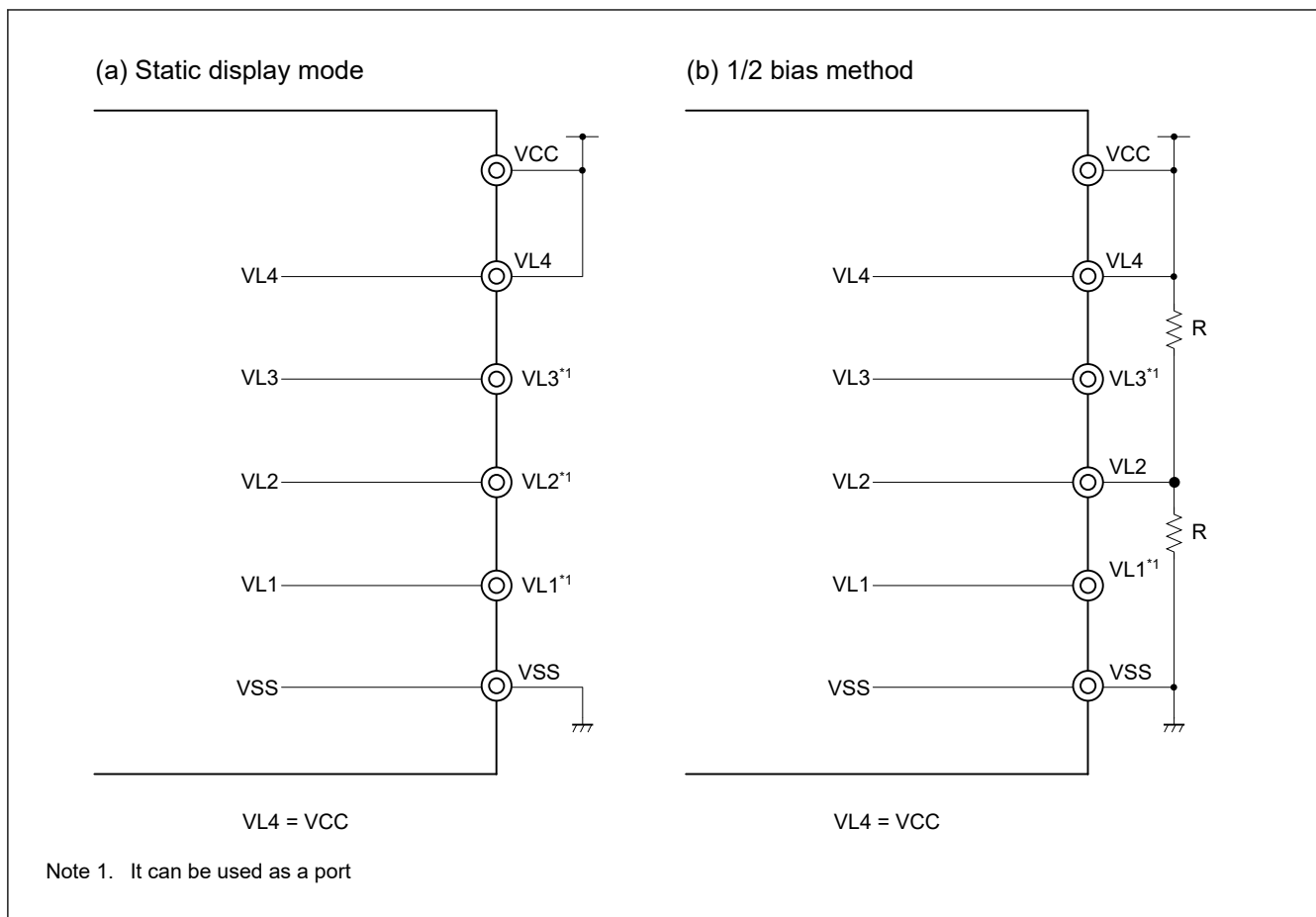
Figure 46.10 Examples of LCD drive power connections using the external resistance division method (1 of 2)
