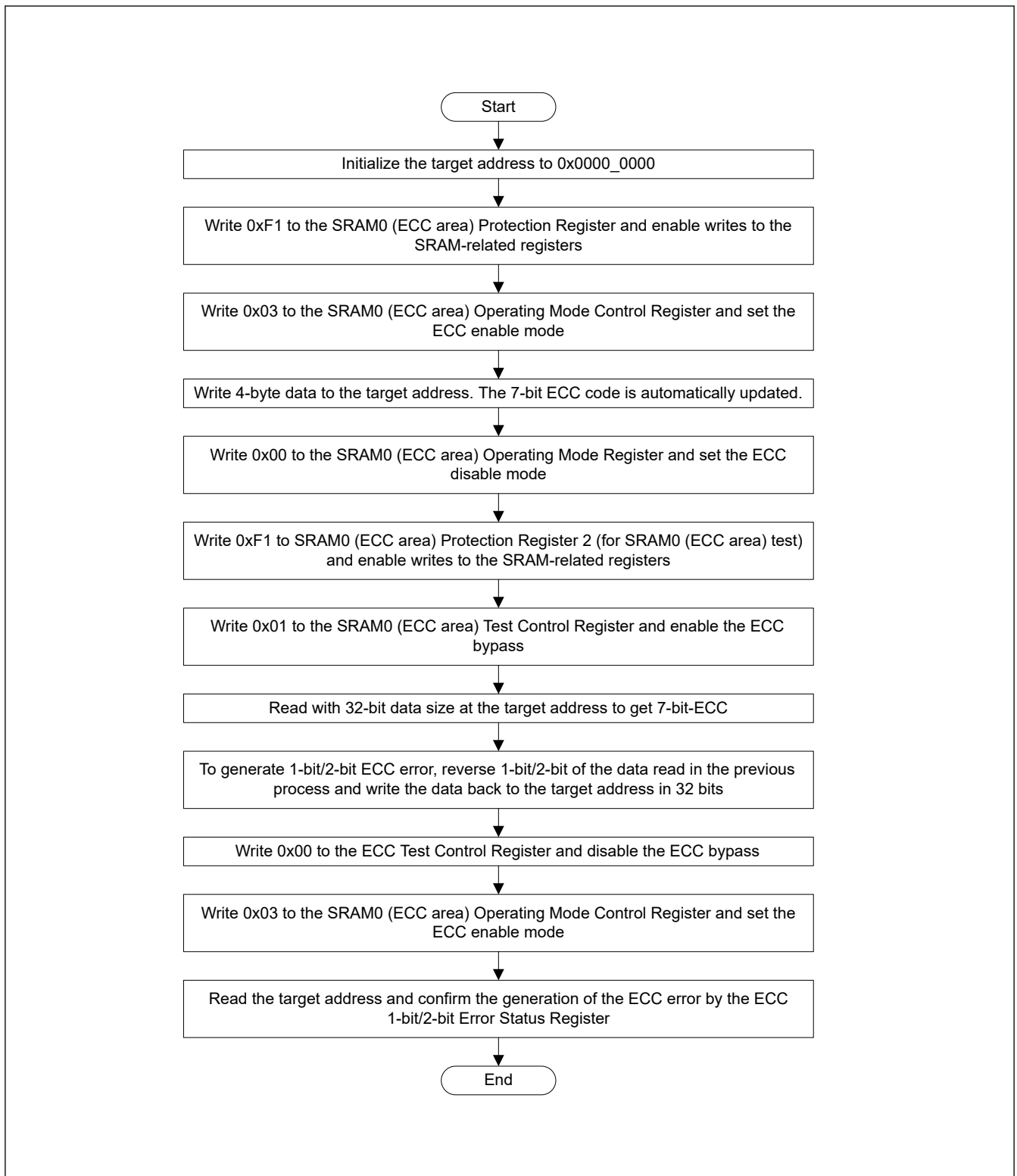
Figure 44.1 ECC decoder testing
