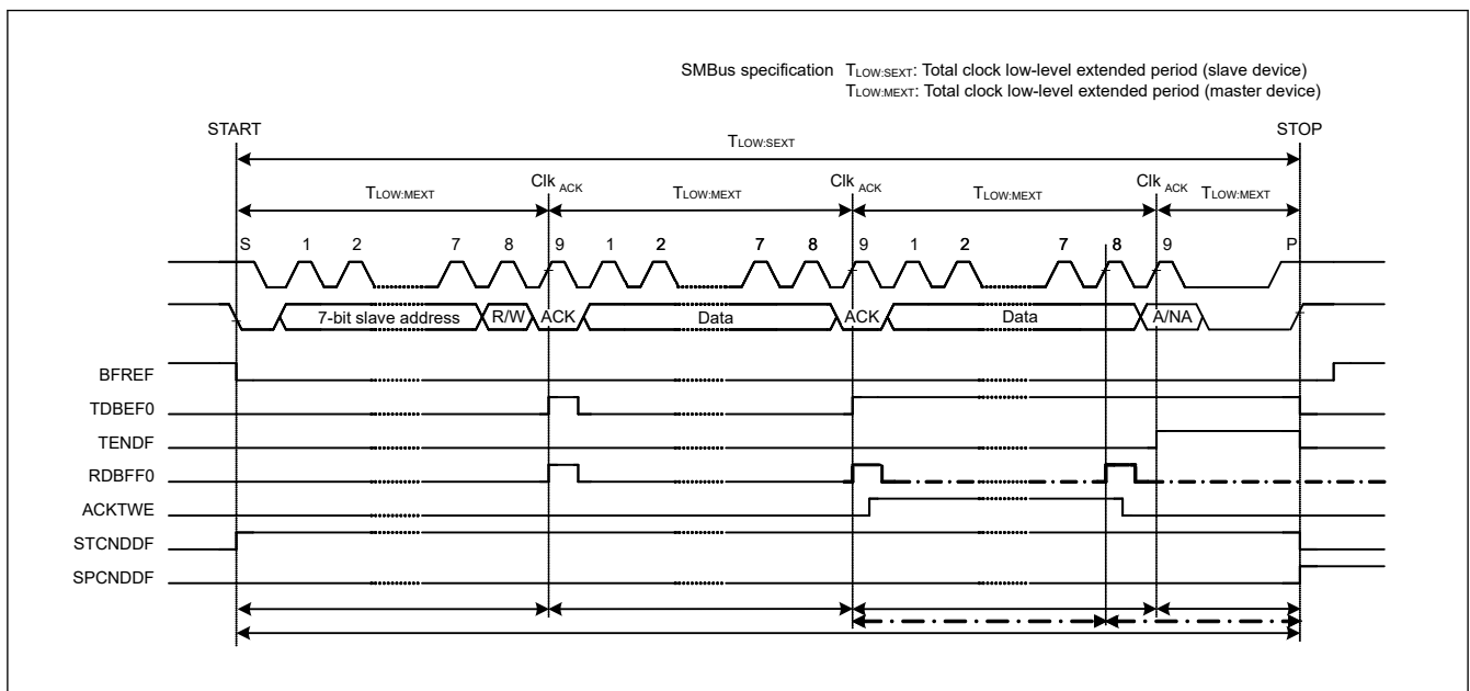
Figure 29.112 SMBus timeout measurement
