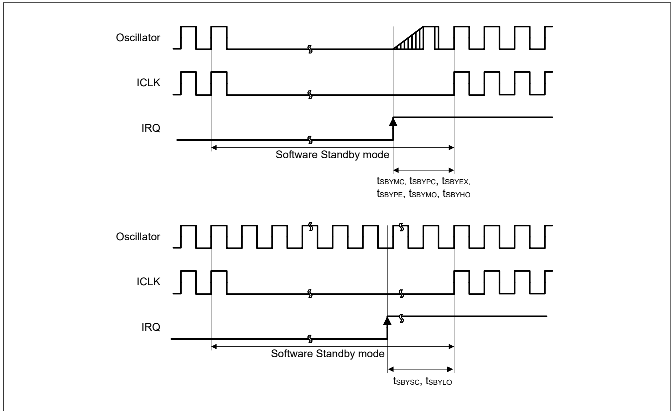
Figure 49.14 Software Standby mode cancellation timing
