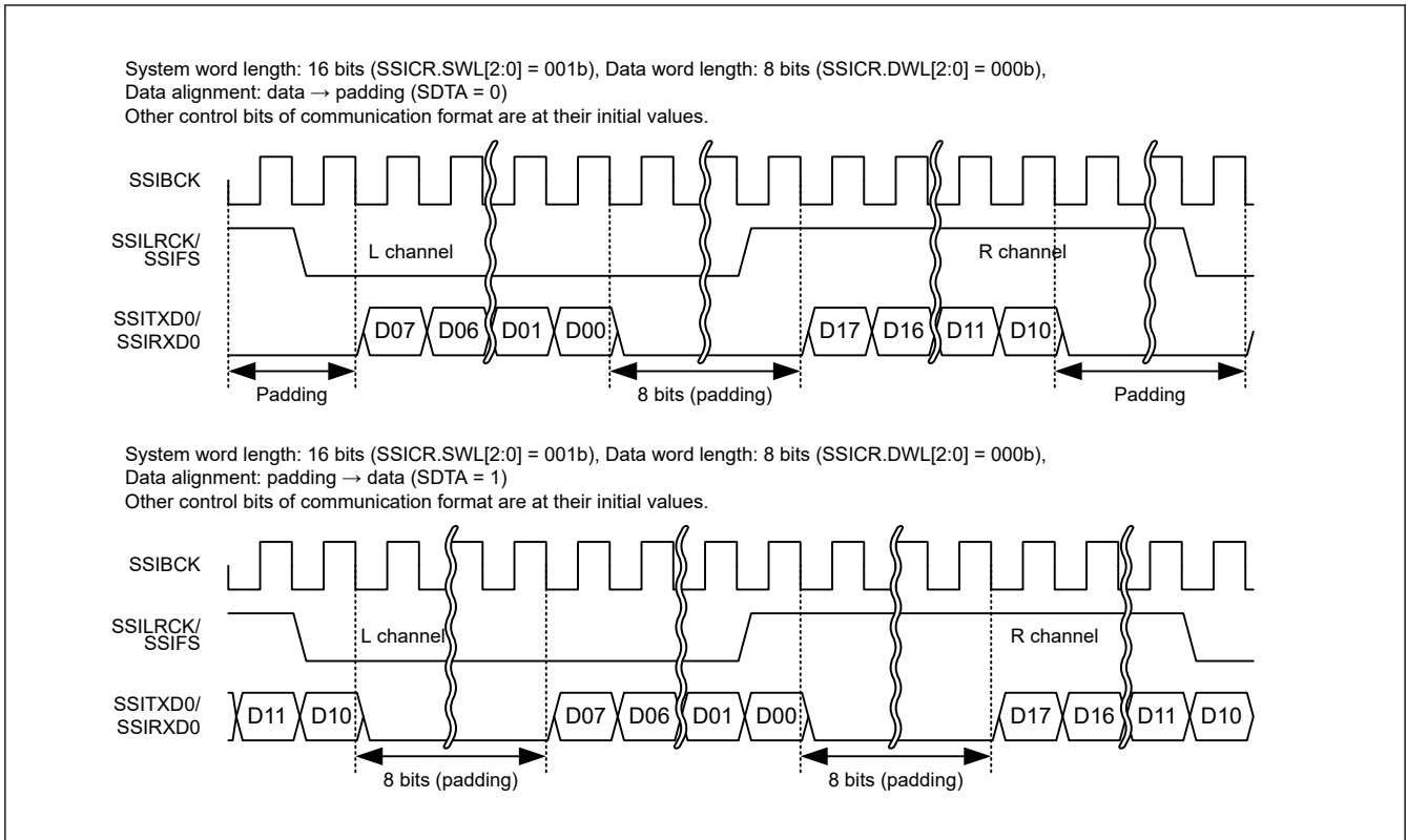
Figure 35.9 Alignment setting of serial data with padding bits
