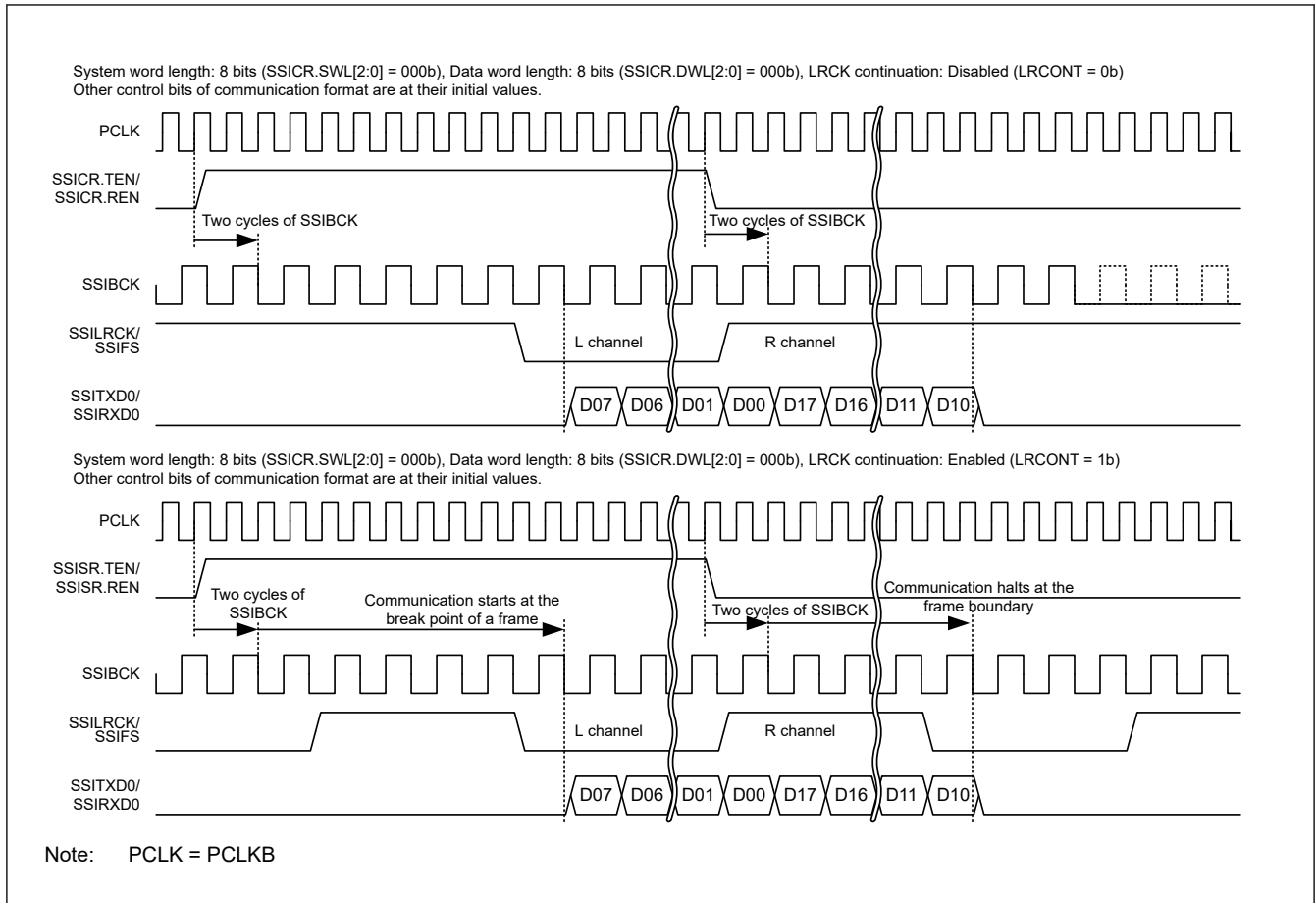
Figure 35.32 Example of LR clock/frame synchronization continuation operation
