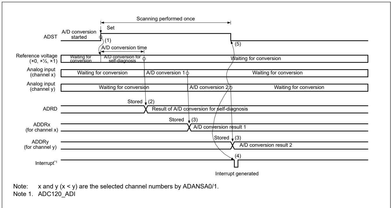
Figure 38.8 Example basic operation in single scan mode when the analog inputs (channel x and y) are selected with self-diagnosis
