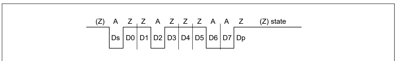
Figure 26.79 Direct convention with SDIR in SCMR = 0, SINV in SCMR = 0, and PM in SMR_SMCI = 0
