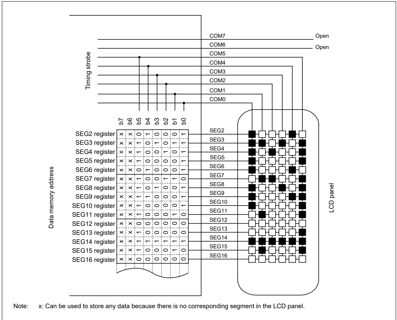
Figure 46.37 Example of connecting six-time slice LCD panel
