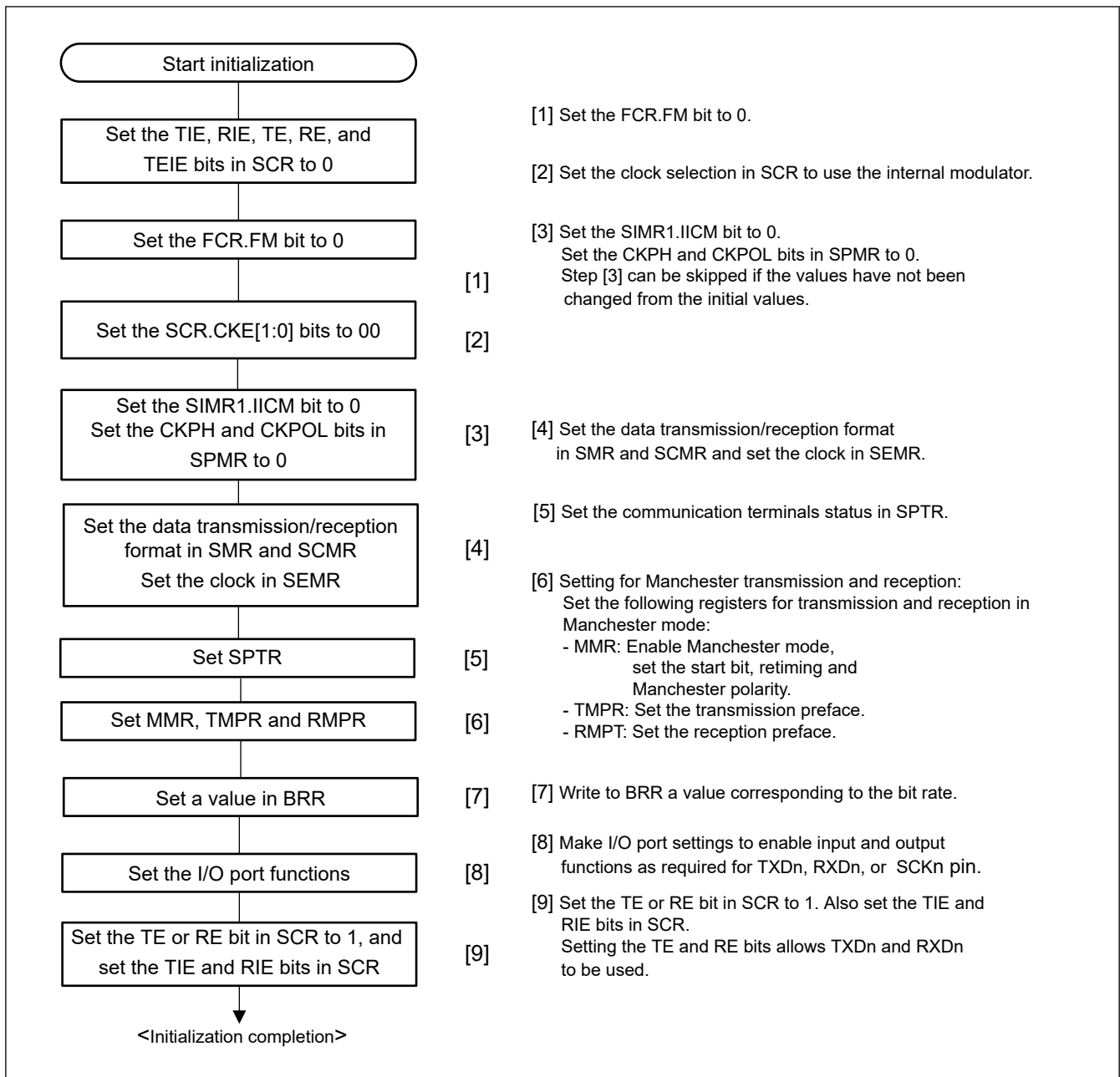
Figure 26.54 SCI Initialization Flow in Manchester Mode
