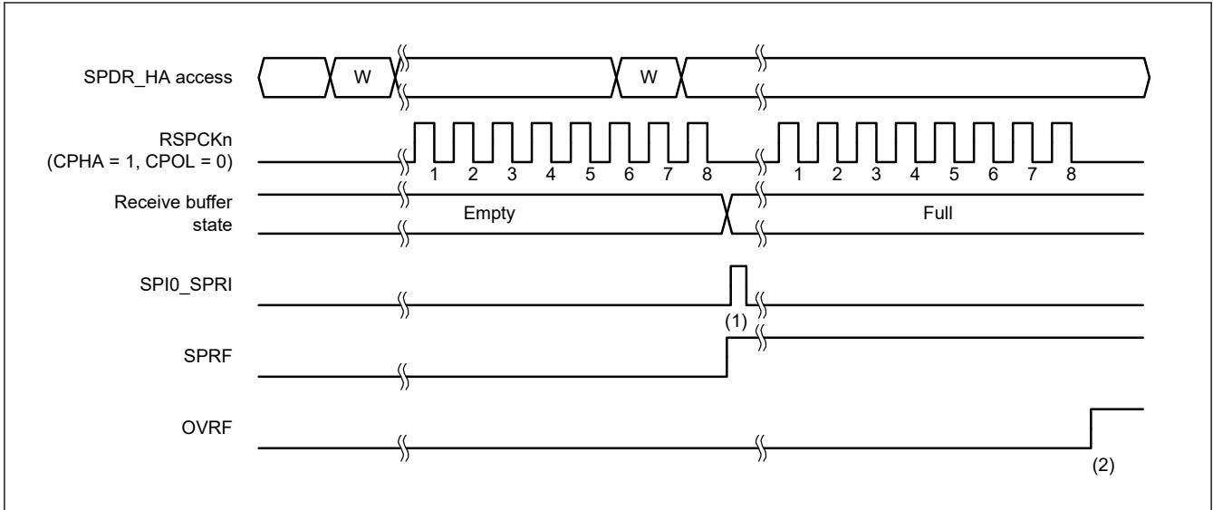
Figure 33.26 Operation example when SPCR3.ETXMD = 0 and SPCR.TXMD = 0
