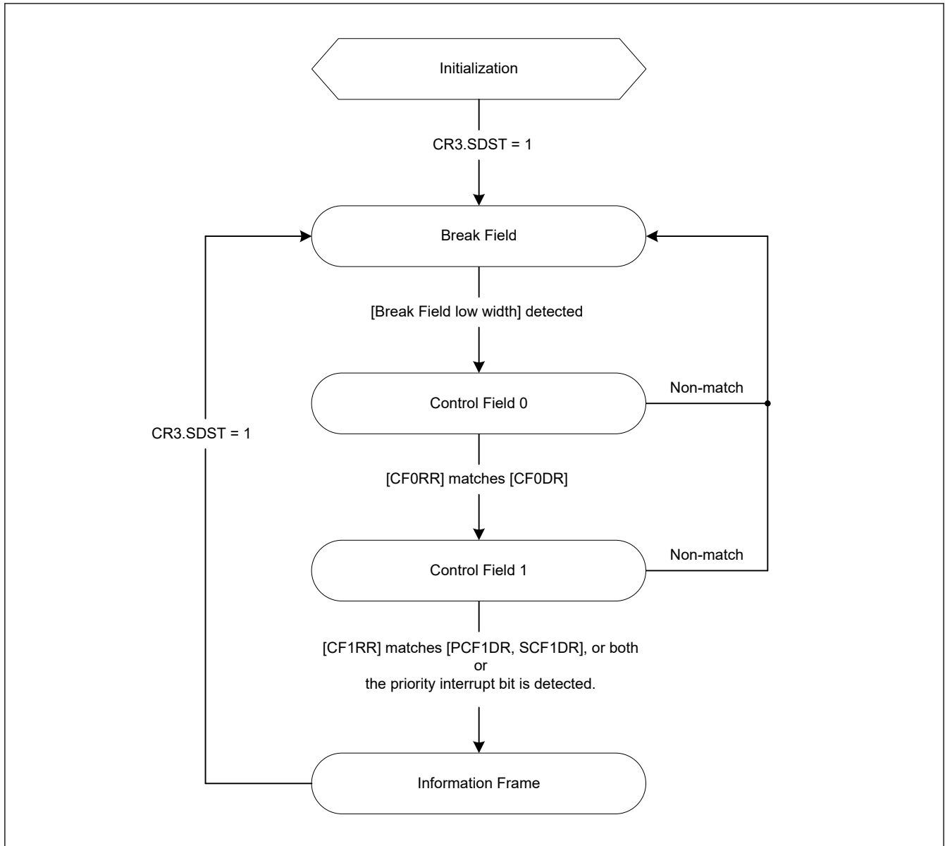
Figure 26.109 State transitions when receiving a Start Frame
