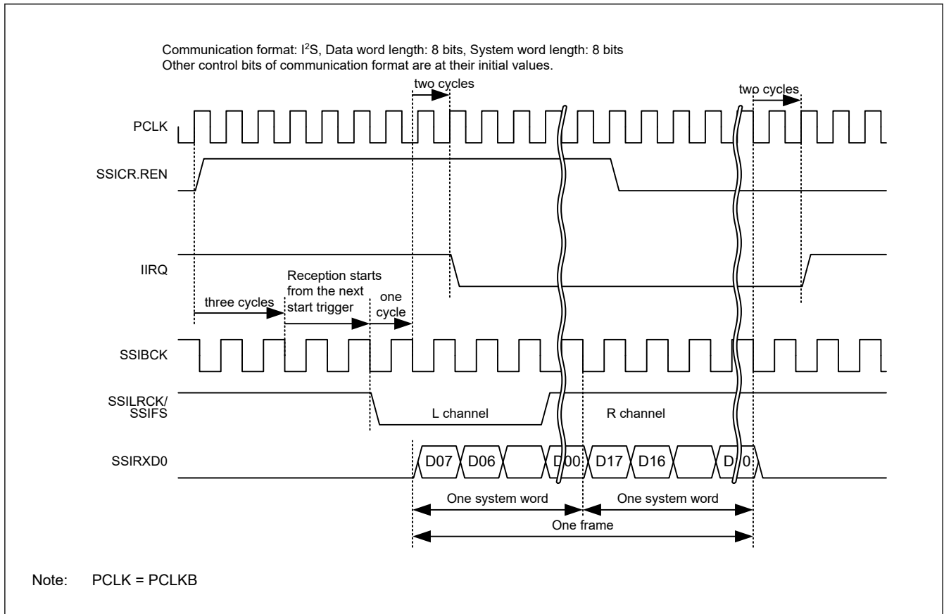
Figure 35.14 IIRQ setting timing (reception)
