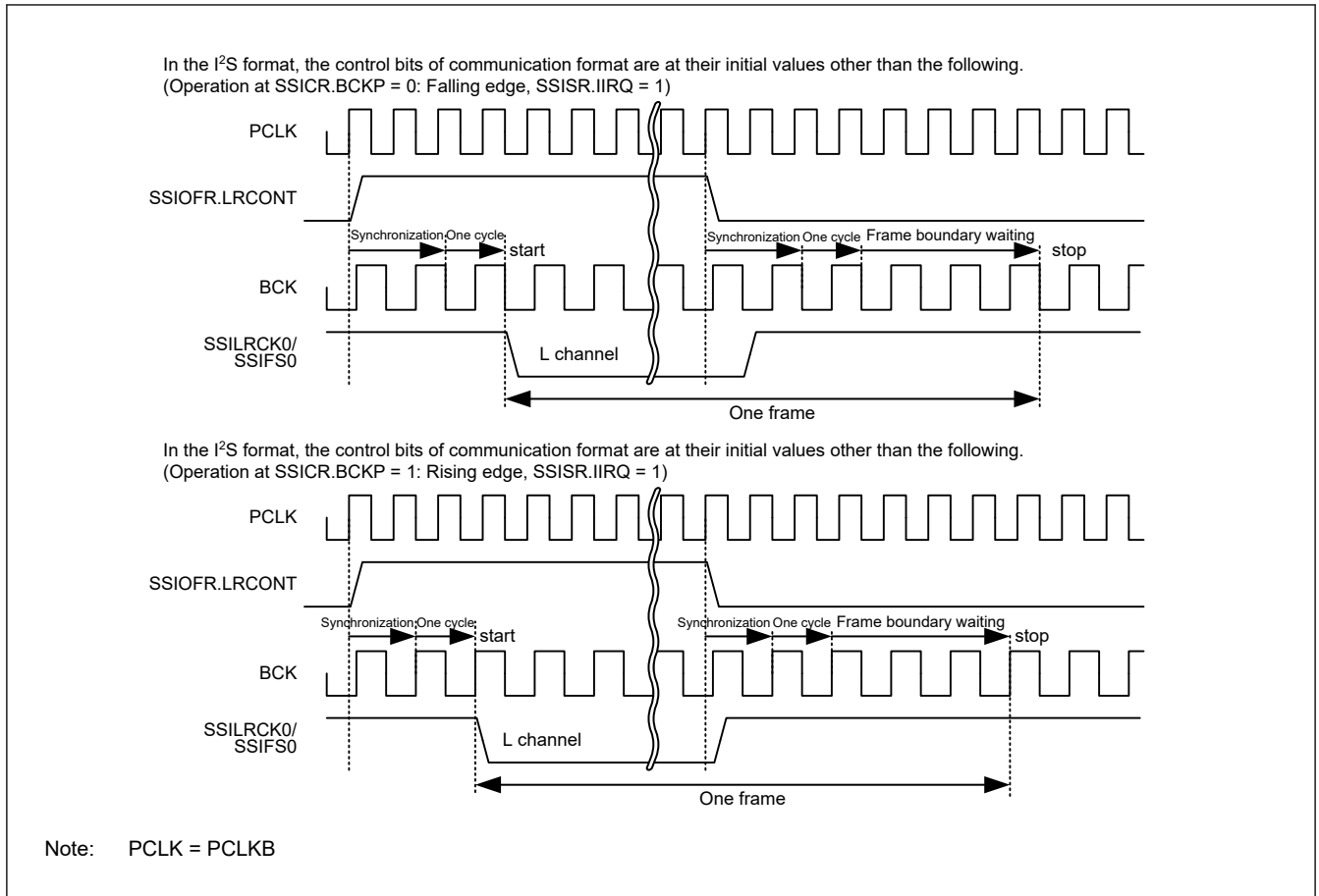
Figure 35.43 Example of disabling LR clock/frame synchronization continuation by SSIOFR.LRCONT
