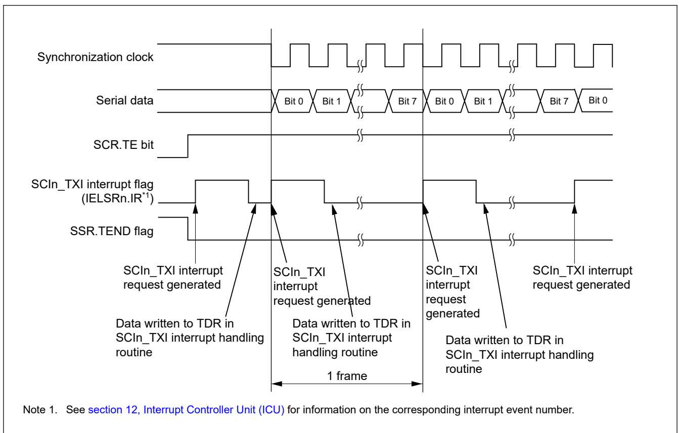
Figure 26.66 Example of serial data transmission in clock synchronous mode when the CTS function is not used at the beginning of transmission
