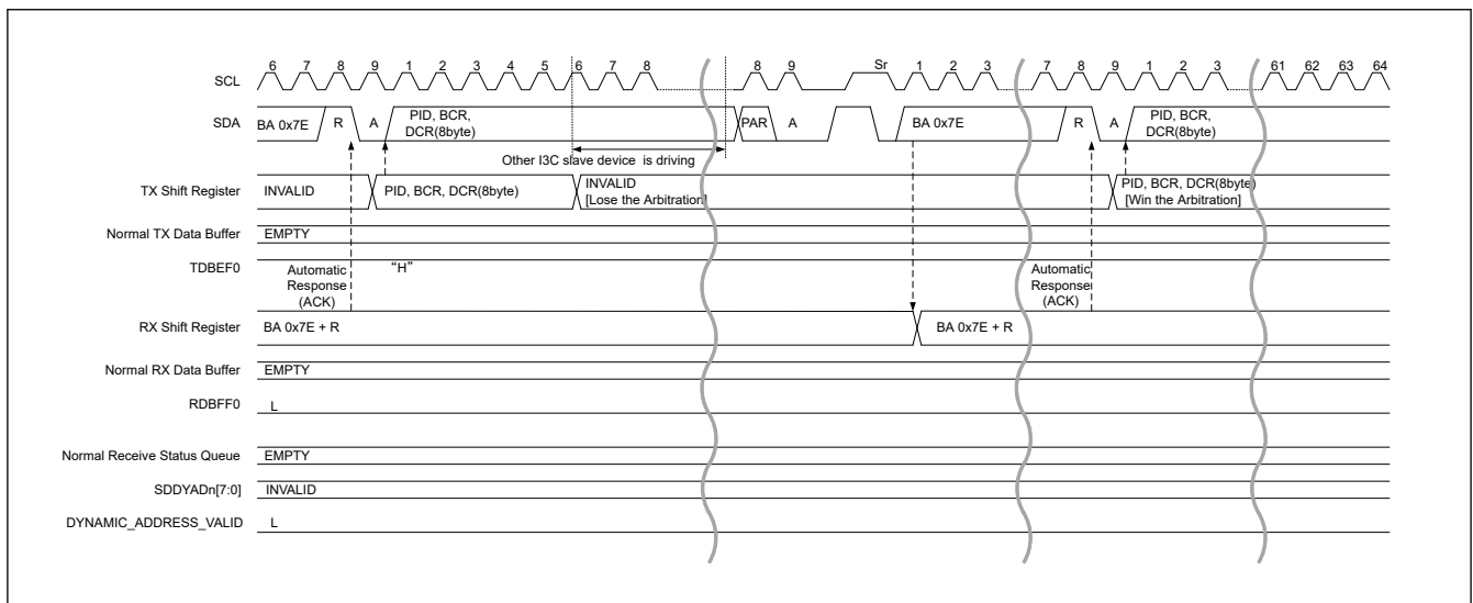
Figure 29.42 Dynamic address assign procedure (ENTDAACCC) timing (2/3)
