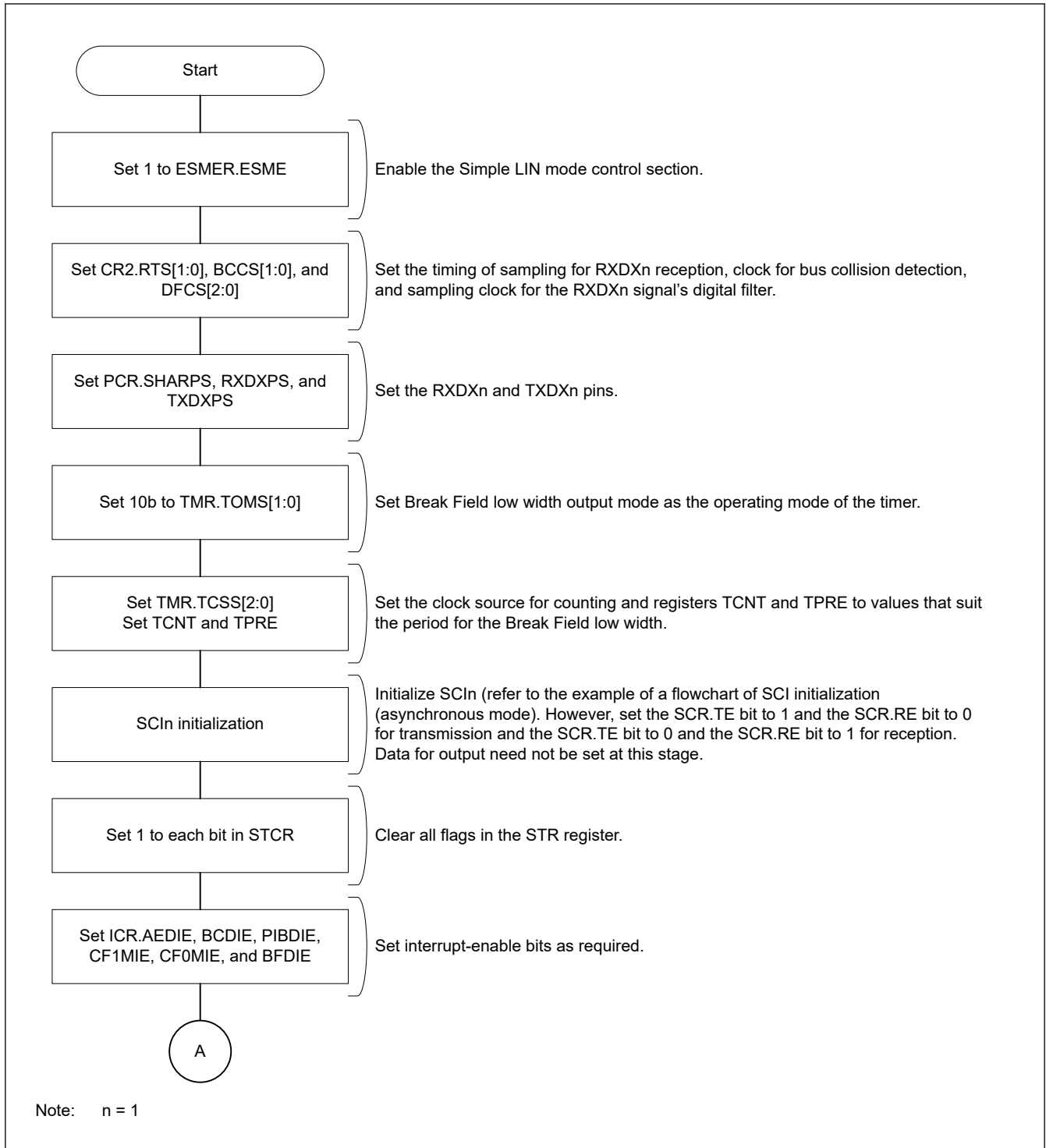
Figure 26.103 Example of Start Frame transmission (1/2)
