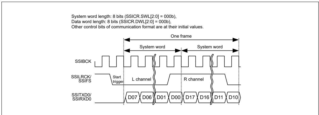
Figure 35.36 I 2 S format (without padding: system word length = data word length)
