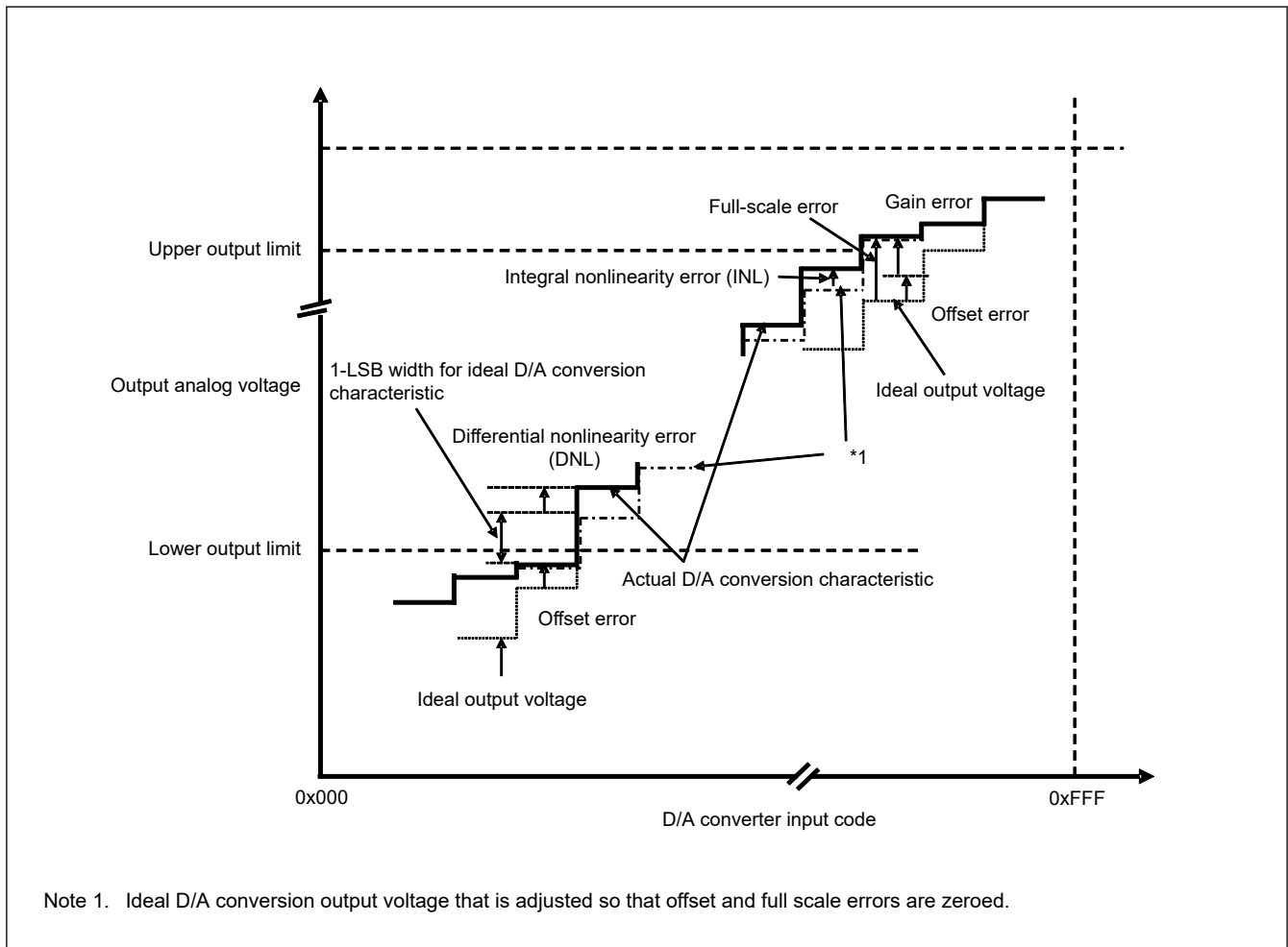
Figure 49.63 Illustration of D/A converter characteristic terms
