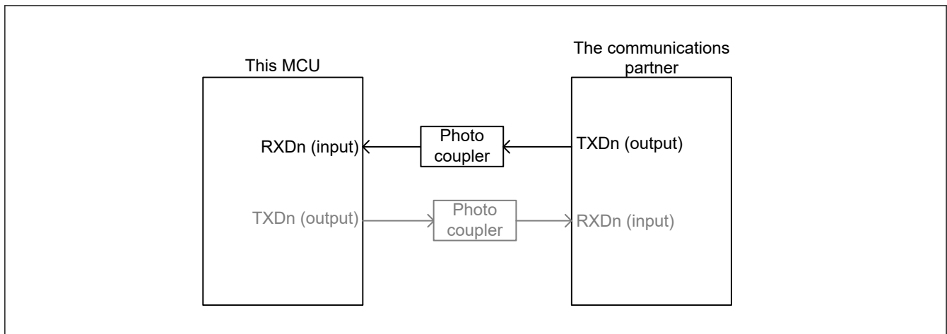
Figure 26.31 Block diagram image of the reception through a photo coupler
