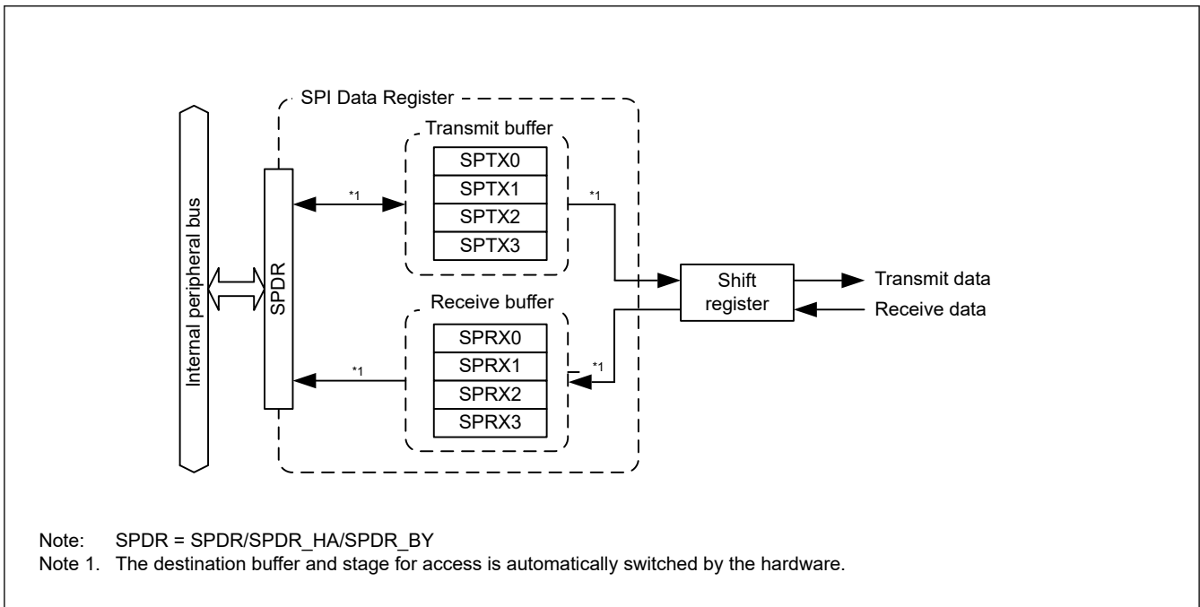
Figure 33.2 Configuration of SPDR/SPDR_HA/SPDR_BY
