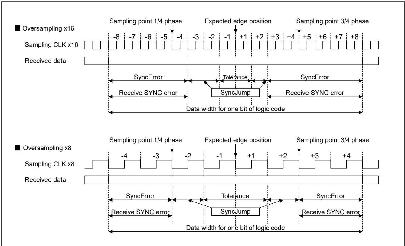
Figure 26.63 Conceptual Image of Reception Retiming Range
