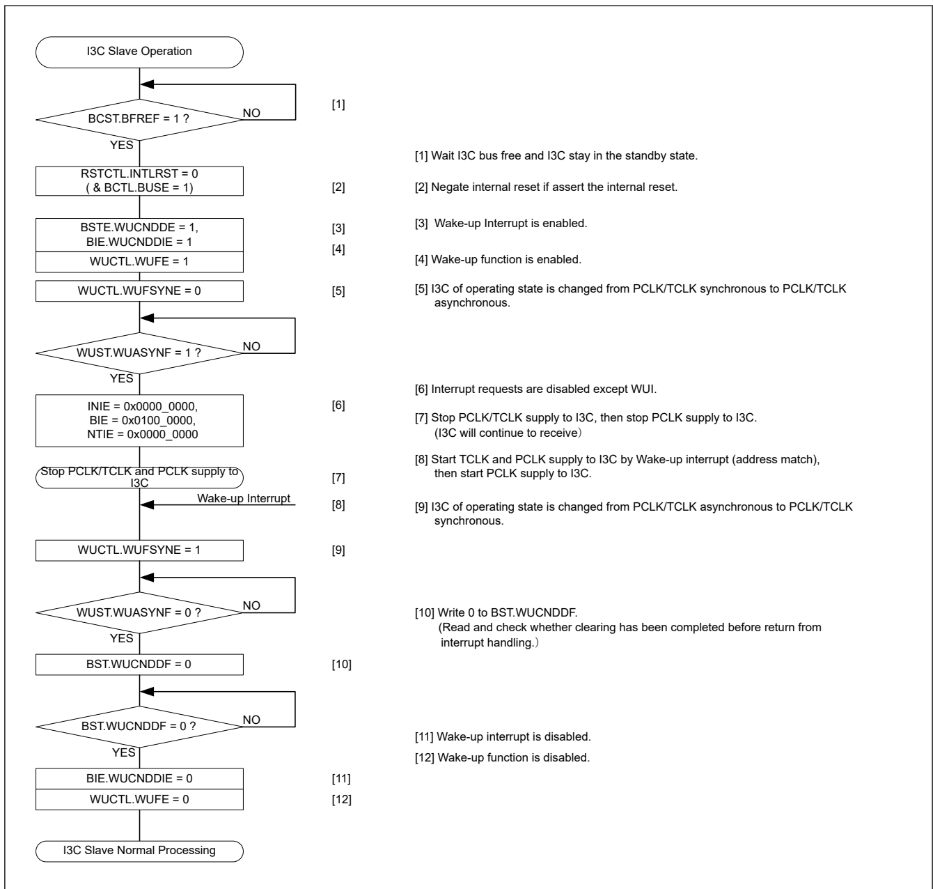
Figure 29.154 Use case of I3C slave Wake-up (Wake-up recovery by a Wake-up interrupt triggered by the match of the slave address)
