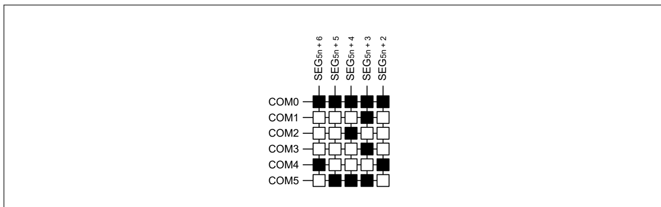
Figure 46.36 Six-time slice LCD display pattern and electrode connections
