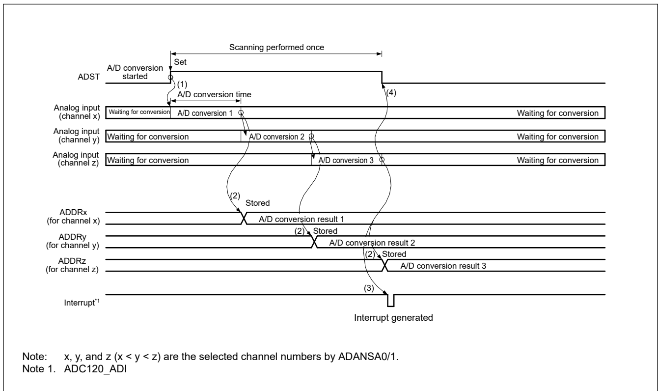
Figure 38.7 Example basic operation in single scan mode when the analog inputs (channel x to z) are selected
