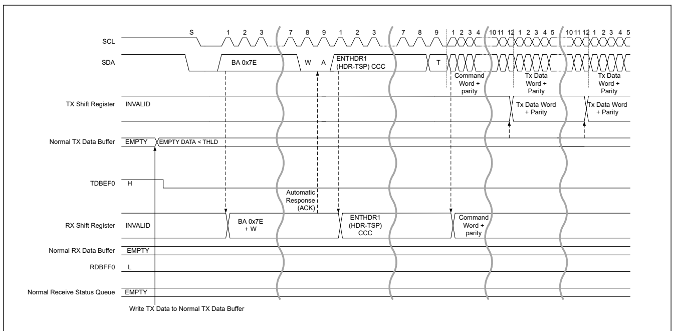
Figure 29.61 HDR data read transfer (HDR-TSP, TSL) timing (1/2)
