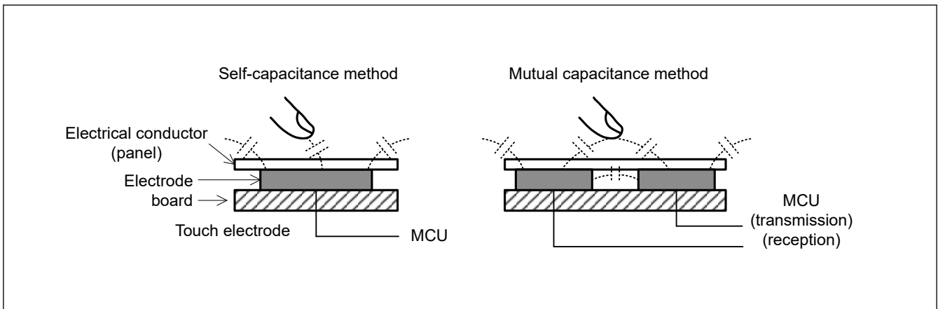
Figure 42.2 Self-capacitance and mutual capacitance methods
