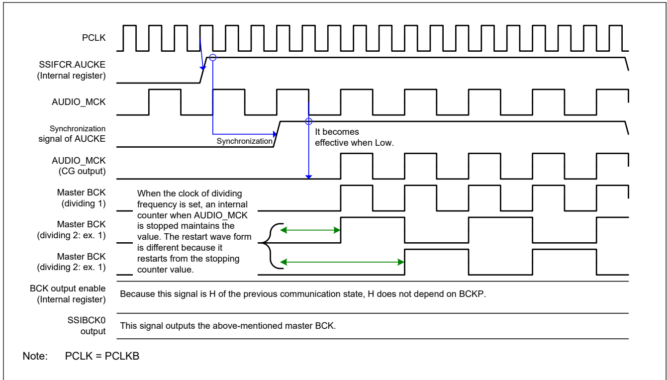
Figure 35.26 Timing diagram for the operation from stop of communication to start of master-mode communication
