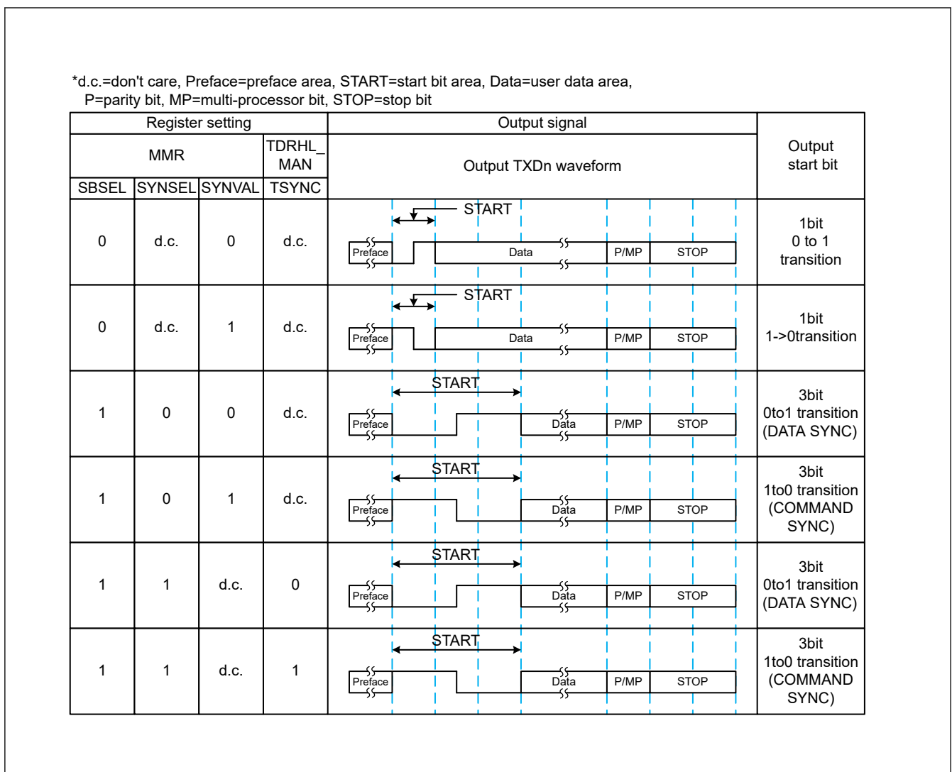
Figure 26.52 Settings Related to and Format of the Start Bit Area at Transmission
