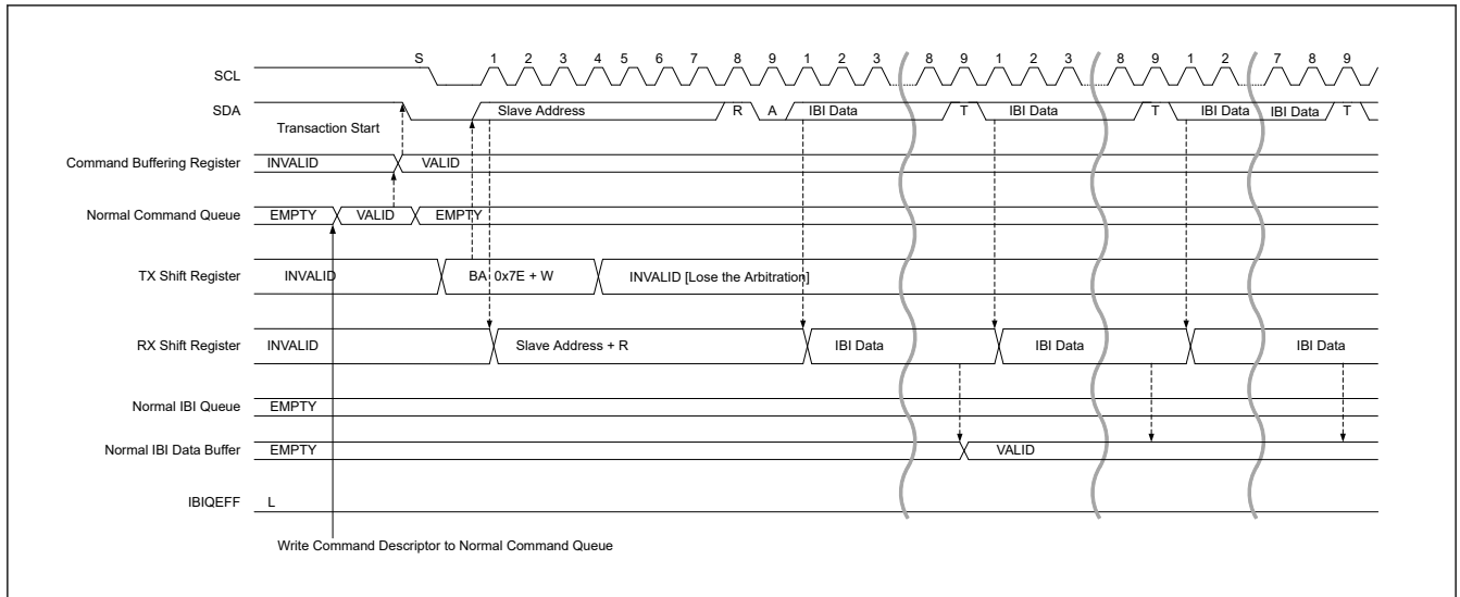
Figure 29.34 I3C master IBI transfer timing (1/2)
