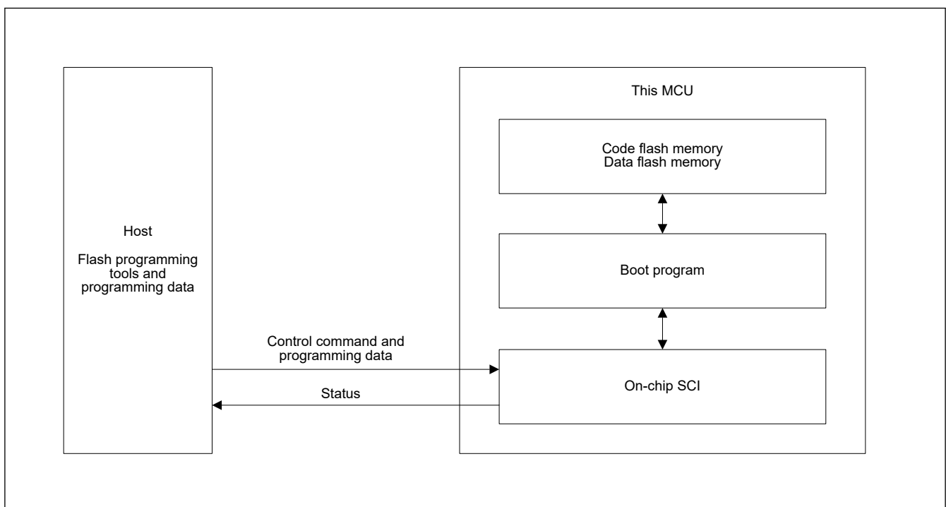
Figure 45.37 System configuration for operations in boot mode (for the SCI interface)
