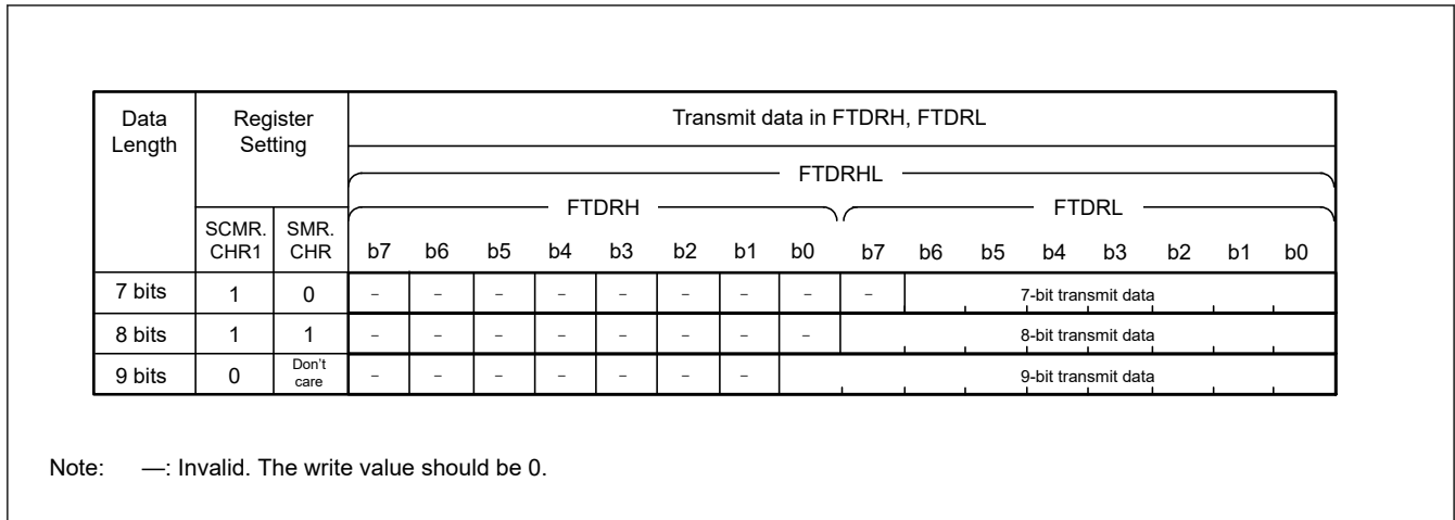
Figure 26.16 Data format written to FTDRH and FTDRL with FIFO selected
