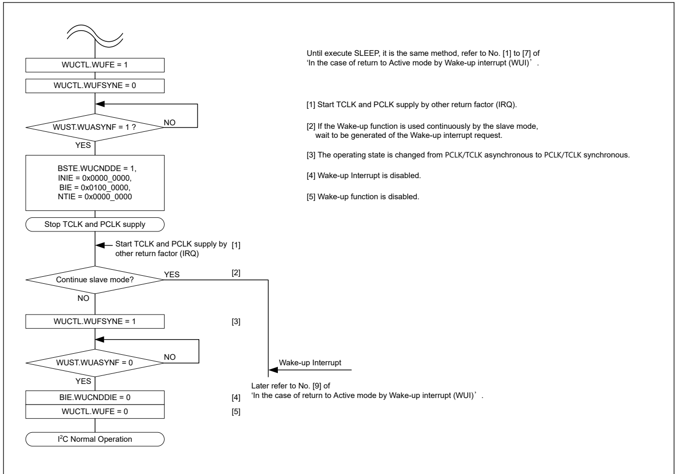
Figure 29.125 Use case of normal WU modes 1 and 2 (Wake-up recovery by other recovery causes (IRQ))
