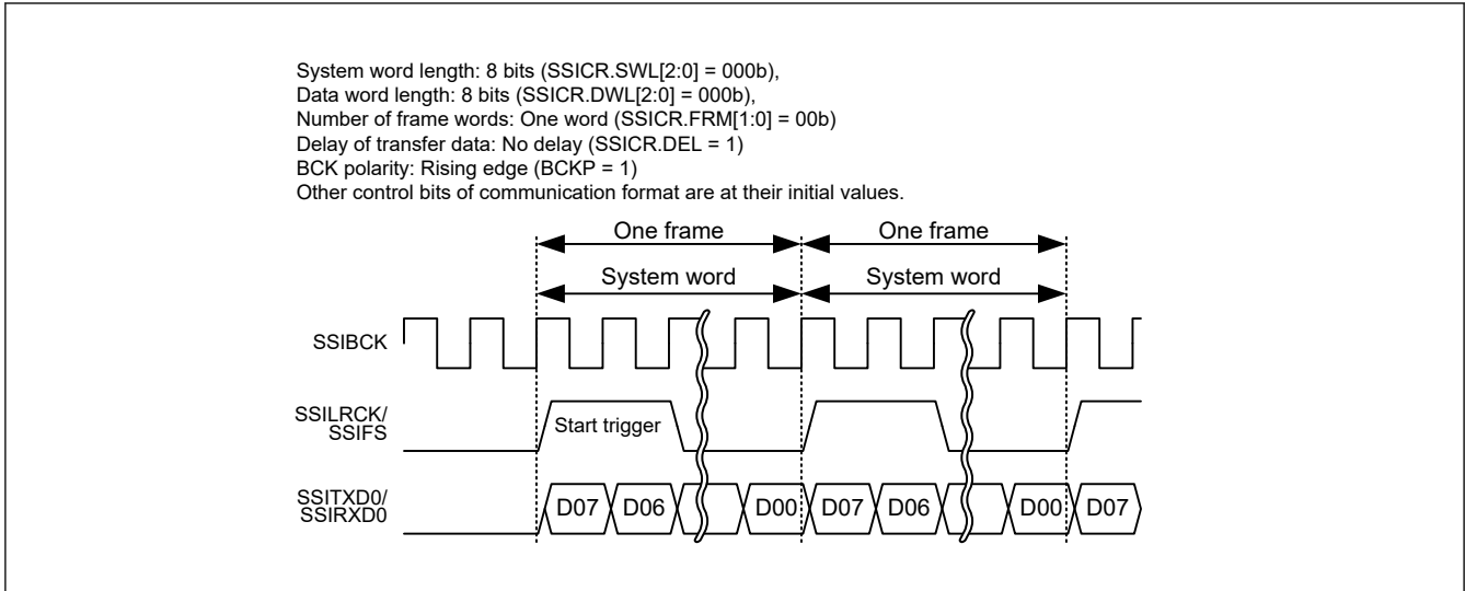
Figure 35.39 Long frame in monaural format (without padding)
