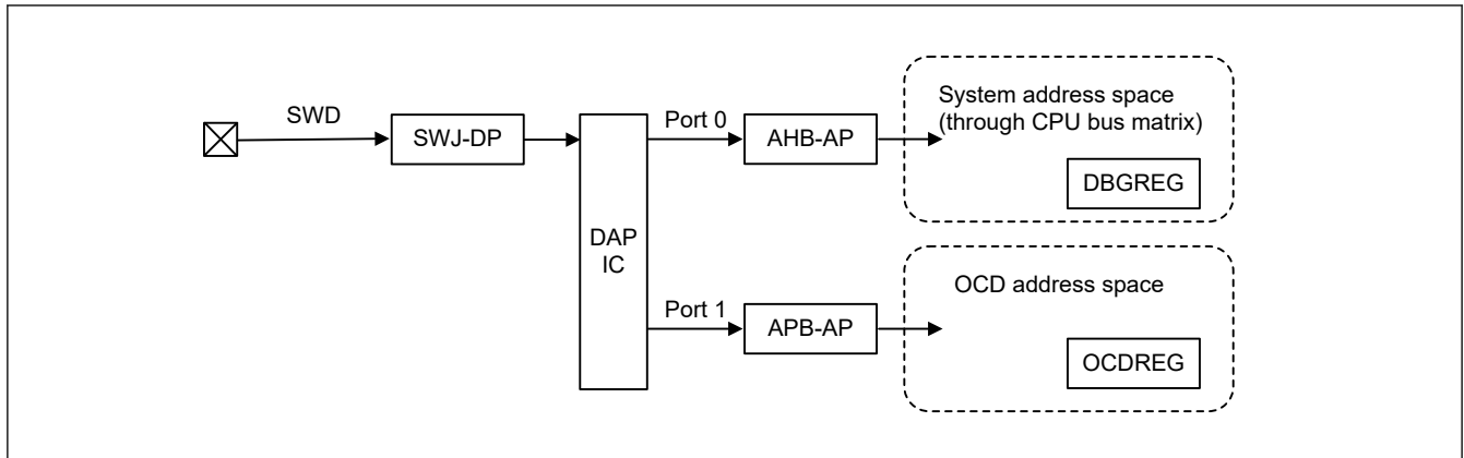
Figure 2.3 SWD authentication block diagram
