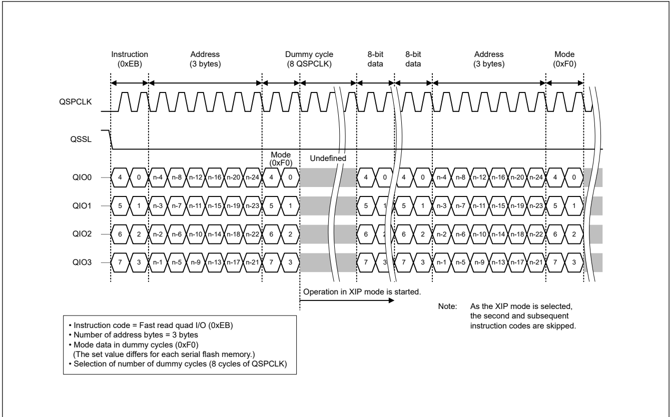
Figure 34.35 XIP mode control data
