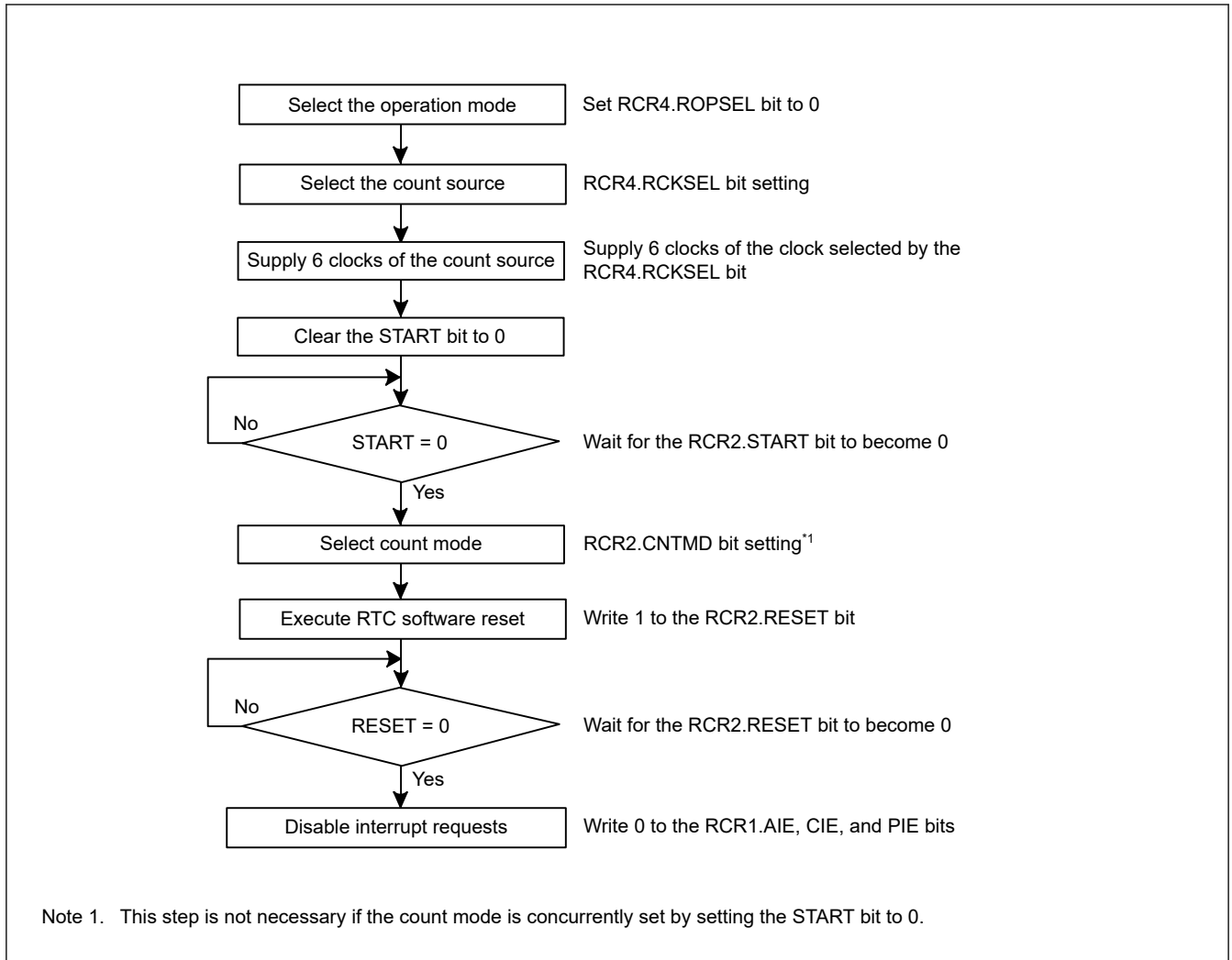
Figure 22.13 Initialization procedure
