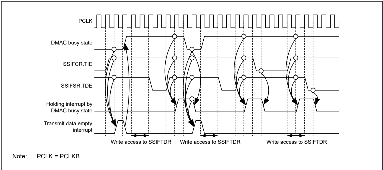
Figure 35.22 Timing of transmit data empty interrupt
