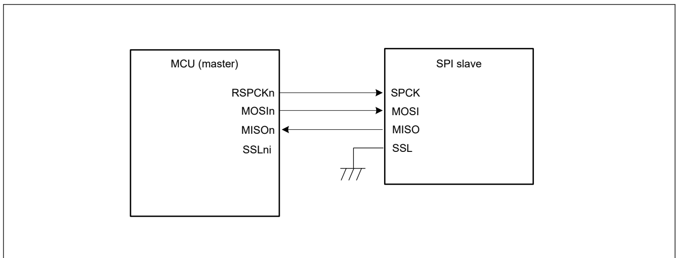
Figure 33.5 Single-master/single-slave configuration example with the MCU as a master
