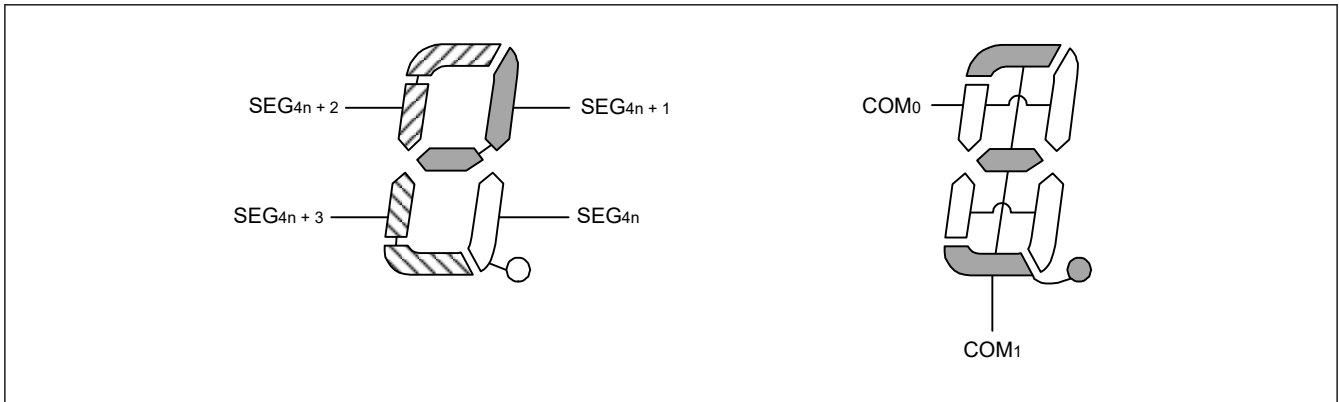
Figure 46.25 Two-time slice LCD display pattern and electrode connections
