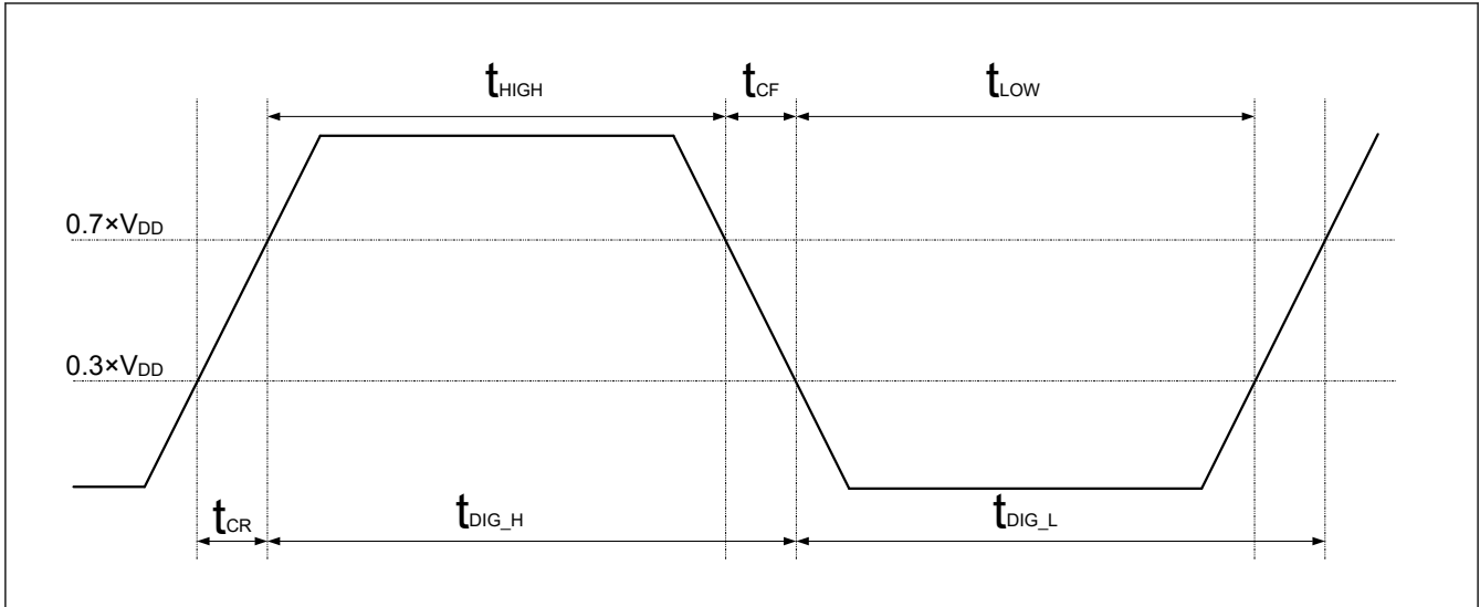
Figure 49.43 tDIG_H and tDIG_L
