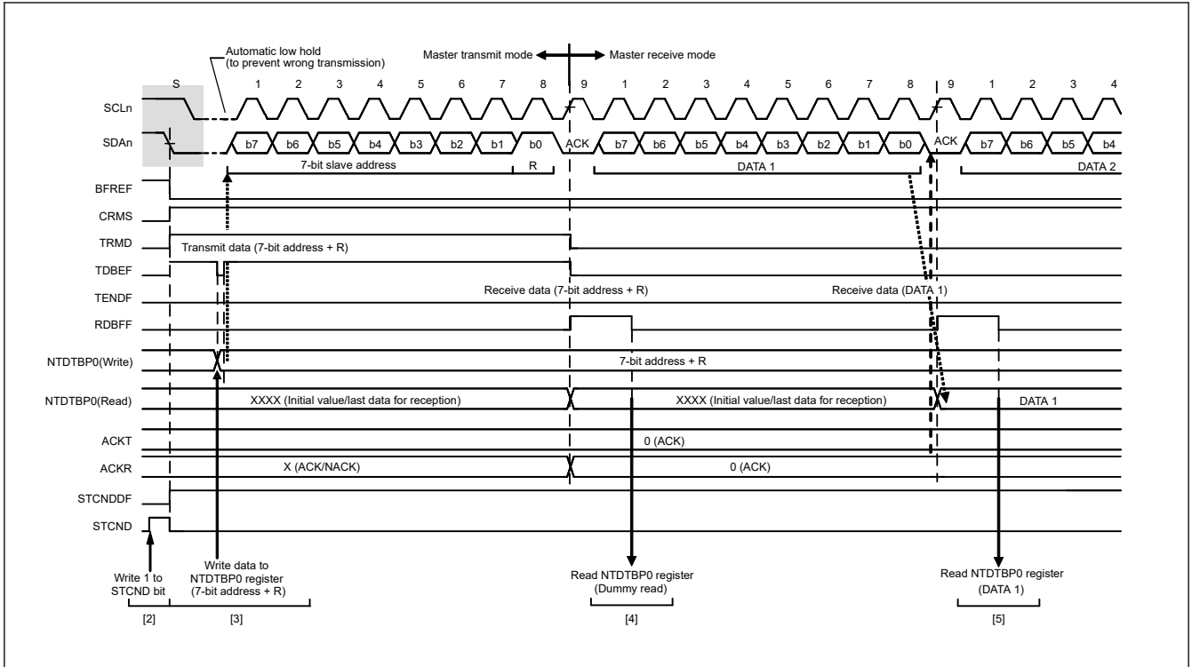
Figure 29.9 Master receive operation timing (1) (7-bit address format, when ACKTWE = 0)
