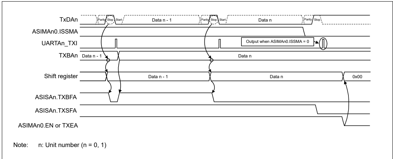
Figure 30.6 Timing when continuous transmission is completed
