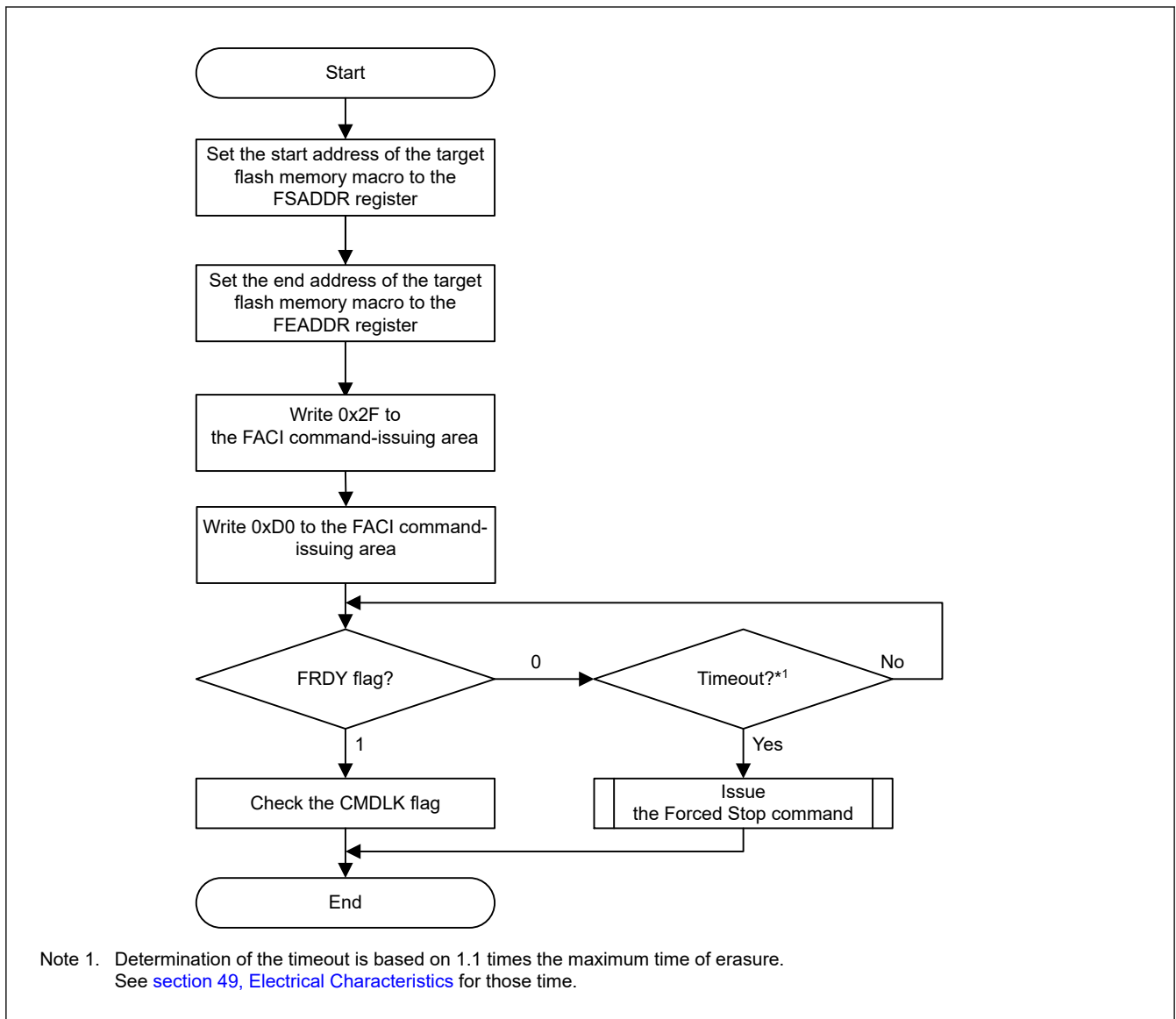
Figure 45.16 Usage flow of the Chip Erase command
