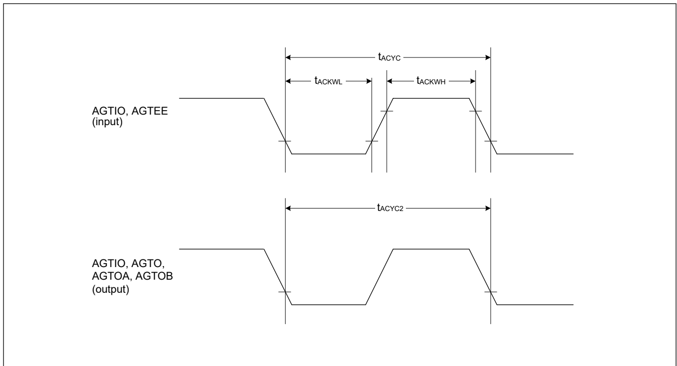
Figure 49.21 AGT I/O timing
