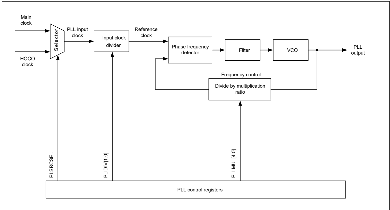
Figure 8.12 PLL block diagram
