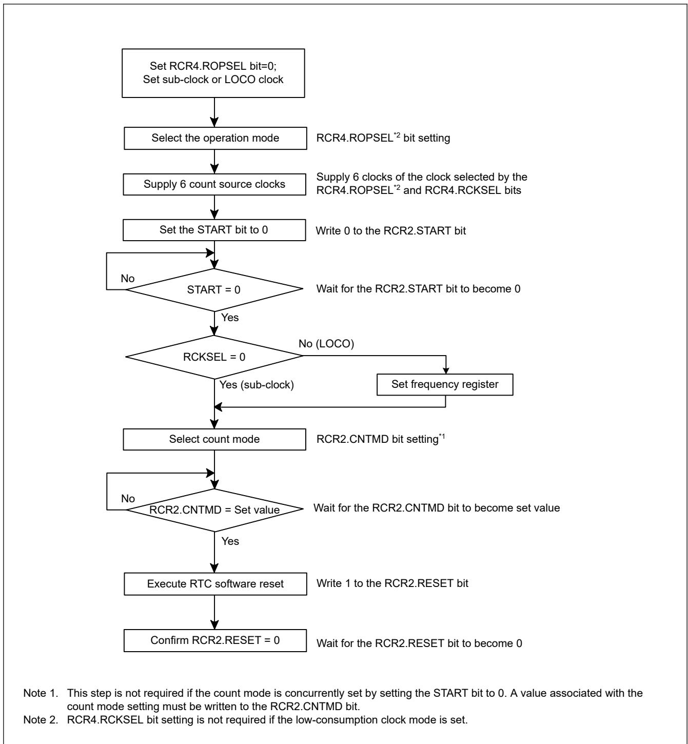
Figure 22.2 Clock and count mode setting procedure
