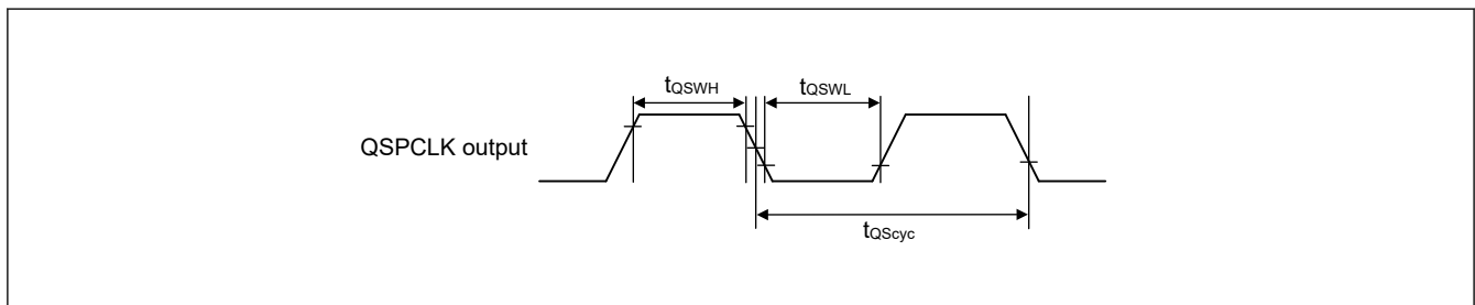
Figure 49.38 QSPI clock timing
