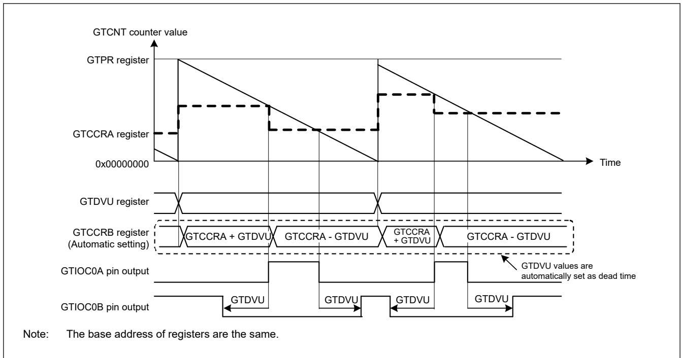
Figure 20.25 Example of automatic dead time setting function operation in saw-wave one-shot pulse mode, down-counting, and active-high
