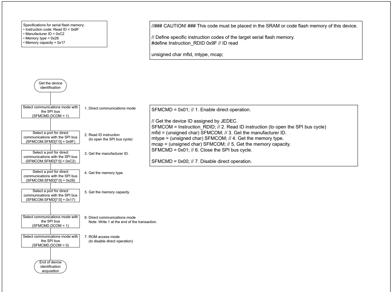
Figure 34.38 Flowchart of Device ID Acquisition
