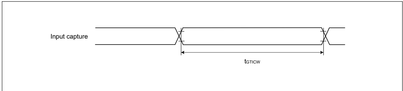
Figure 49.20 GPT input capture timing
