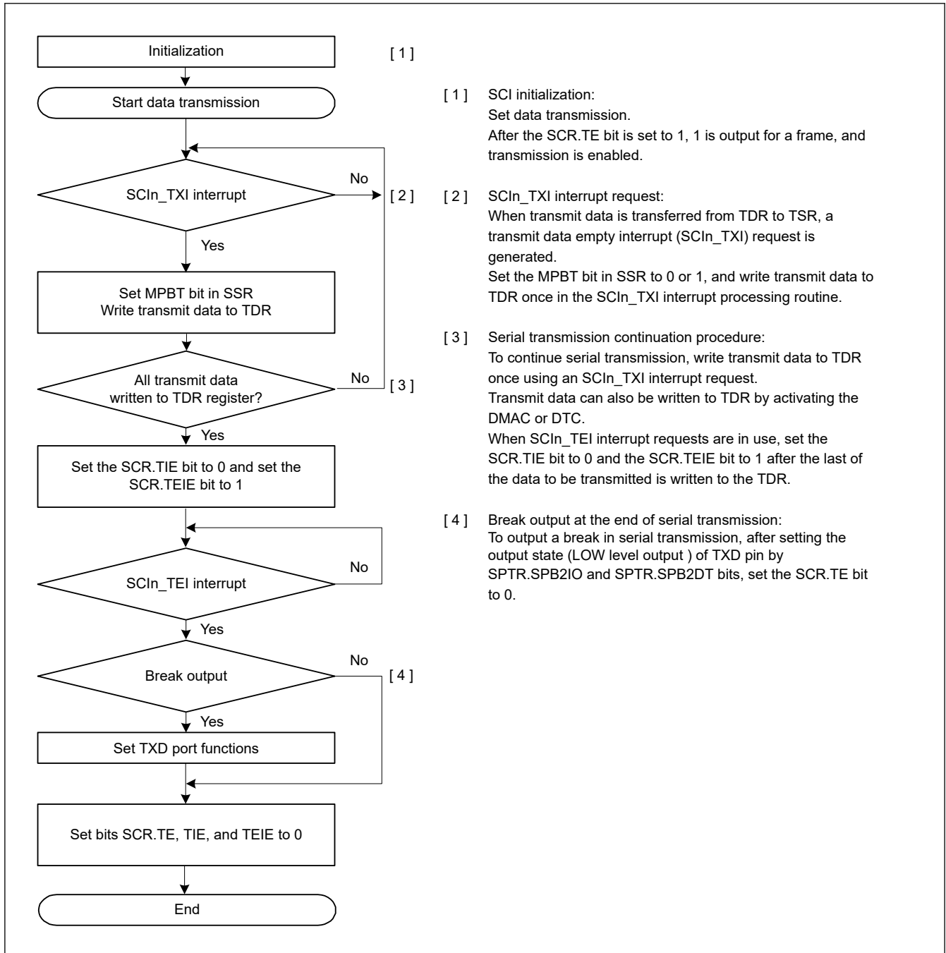
Figure 26.41 Example flow of multi-processor serial transmission with non-FIFO selected
