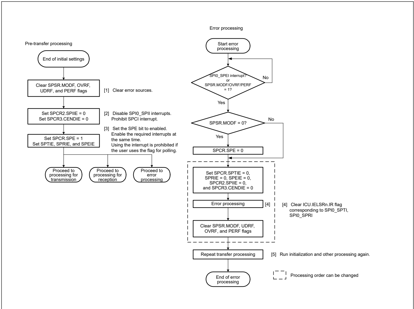
Figure 33.57 Error processing flow for slave mode
