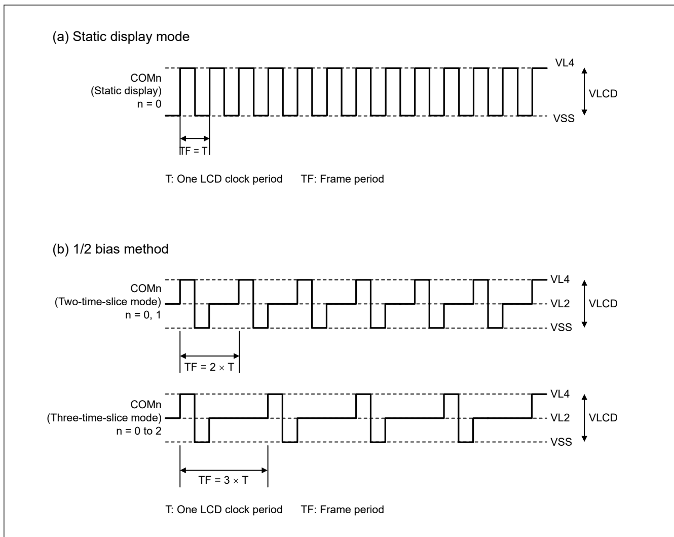
Figure 46.17 Common signal waveforms (1 of 2)
