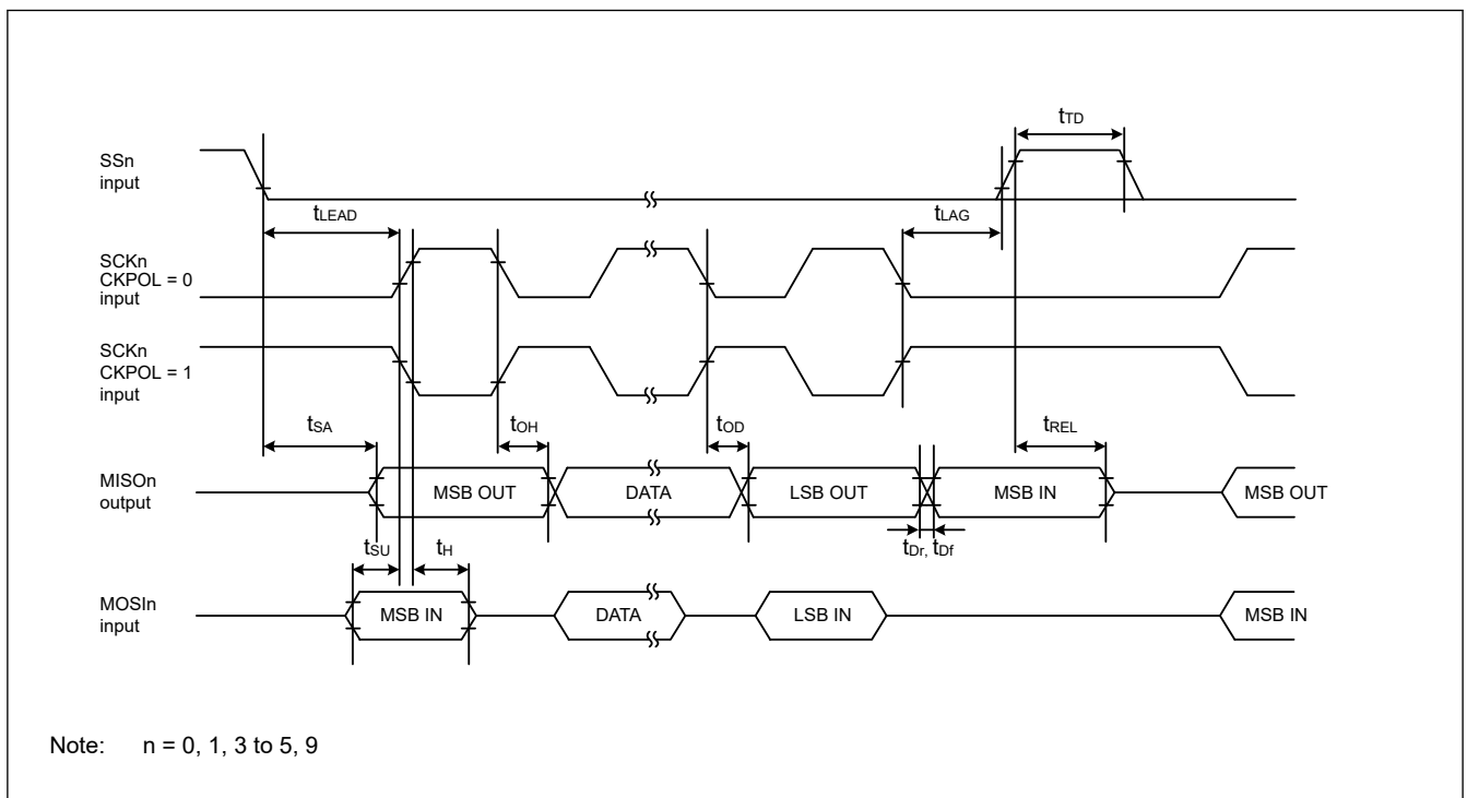
Figure 49.28 SCI simple SPI mode timing (slave, CKPH = 1)
