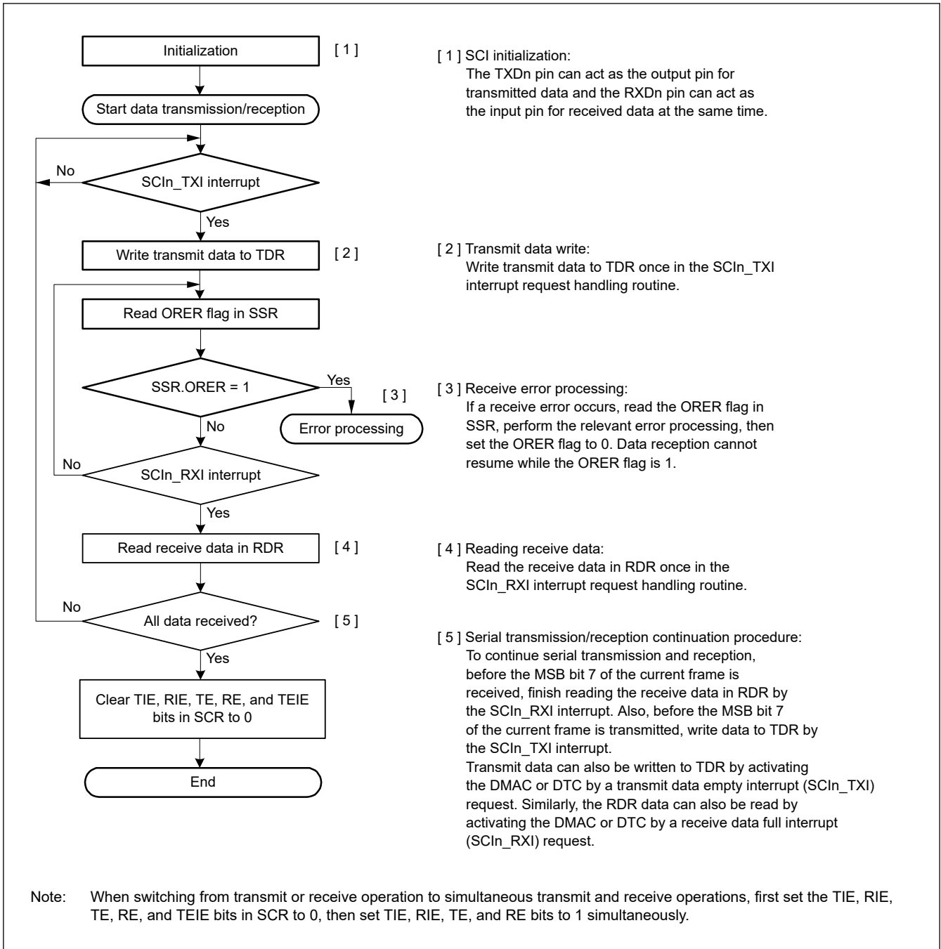
Figure 26.75 Example flow of simultaneous serial transmission and reception in clock synchronous mode with non-FIFO selected
