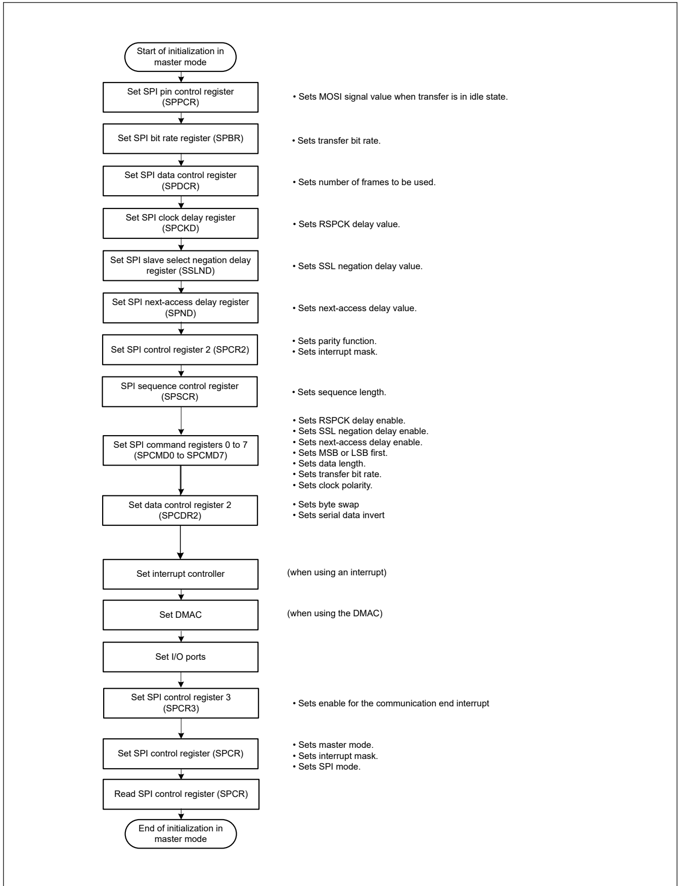
Figure 33.61 Example of initialization flow in master mode for clock synchronous operation
