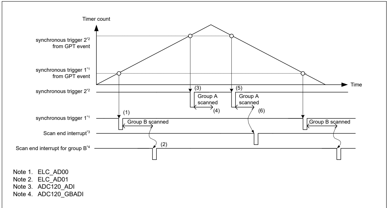
Figure 38.15 Example basic operation in group scan mode with double-trigger mode when synchronous triggers from the ELC are used
