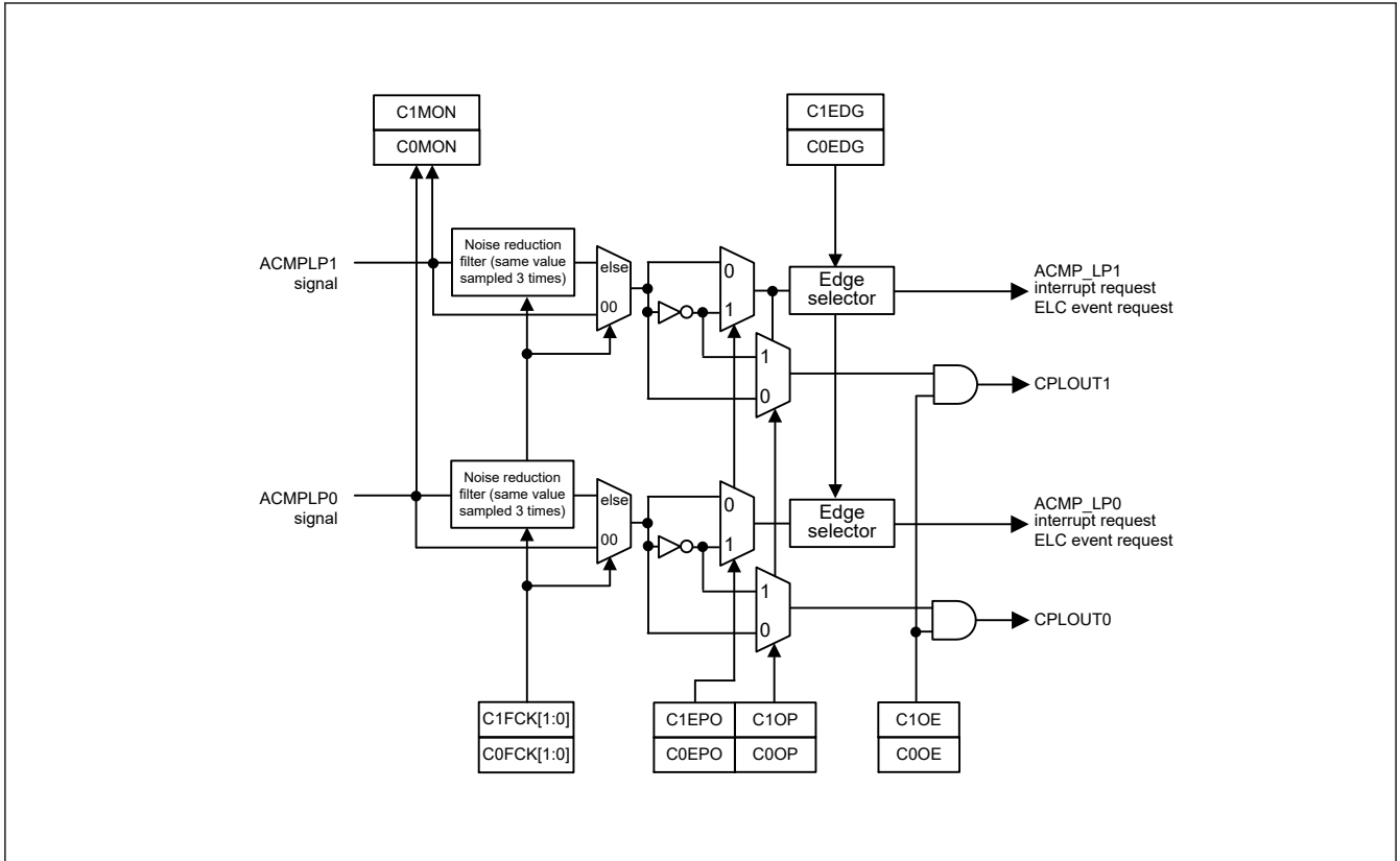
Figure 41.5 Noise filter and edge detection configuration
