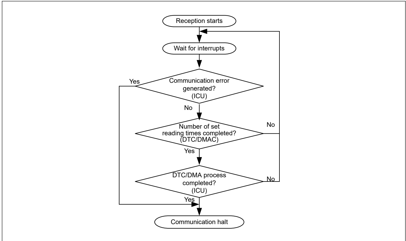
Figure 35.54 Reception procedure
