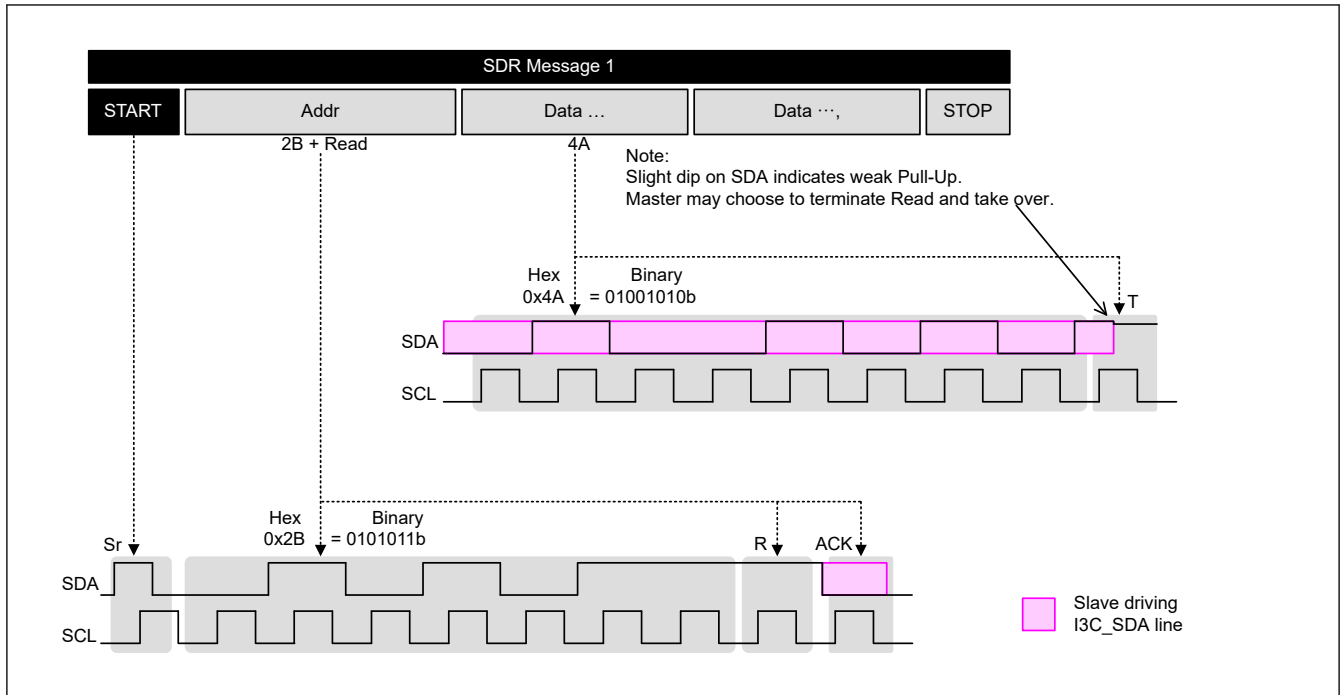
Figure 29.71 Example communication using I3C coding SDR without broadcast (0x7E)
