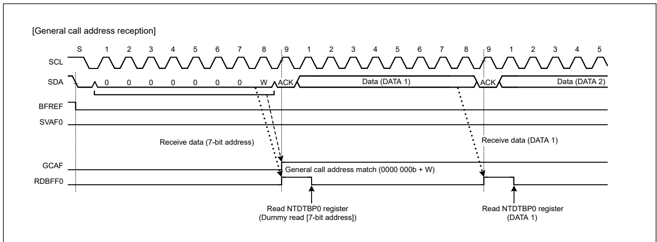
Figure 29.83 Timing of GCAF flag setting during reception of general call address
