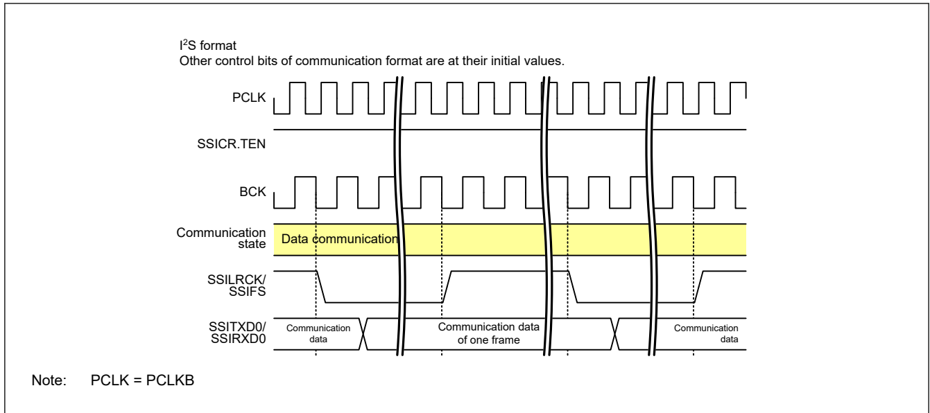
Figure 35.46 Continuation of the data communication
