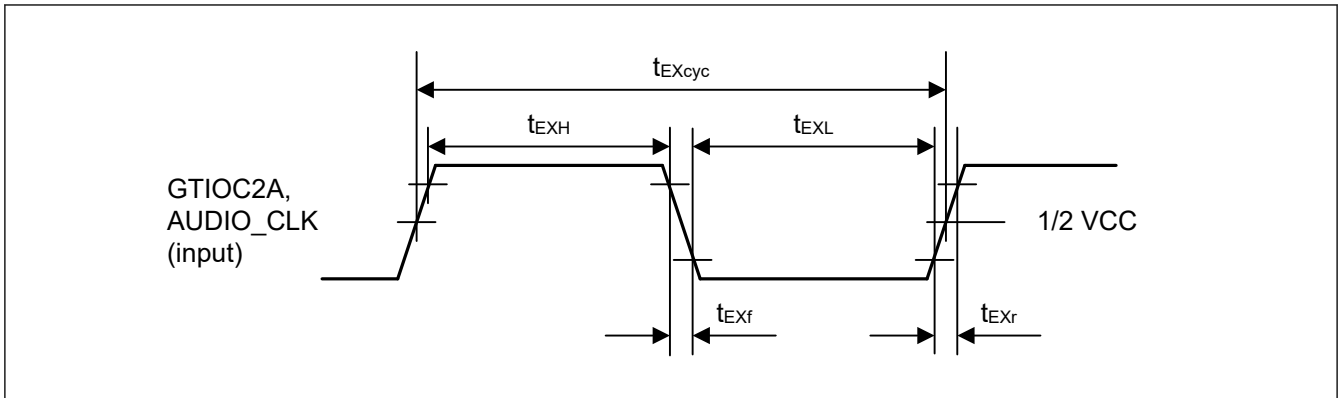
Figure 49.53 Clock input timing
