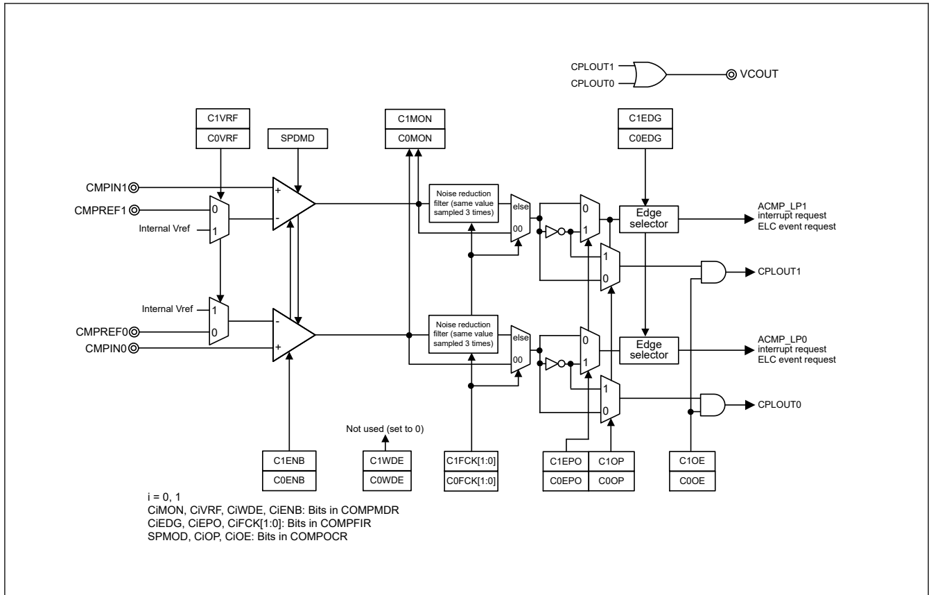
Figure 41.1 ACMPLP block diagram when window function is disabled
