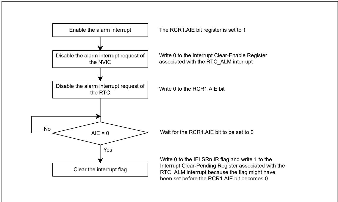
Figure 22.7 Procedure for disabling alarm interrupt request
