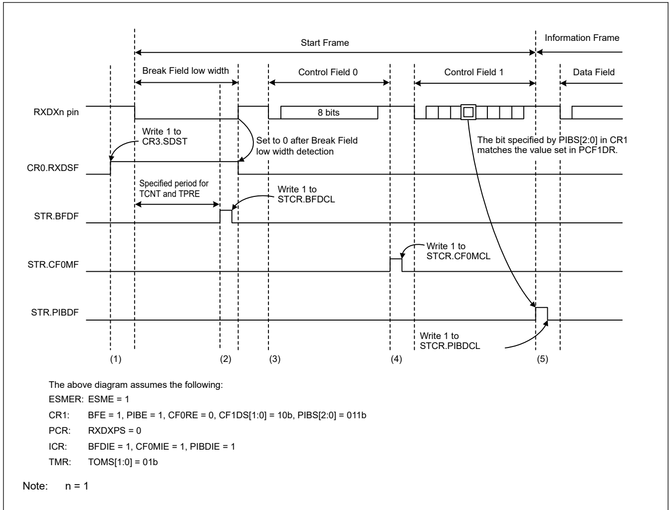
Figure 26.110 Example of operations when receiving a Start Frame while the CR1.PIBE bit is 1
