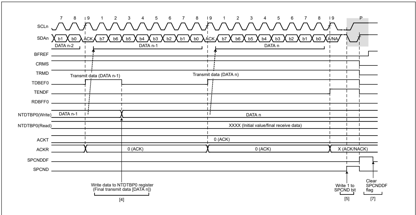
Figure 29.8 Master transmit operation timing (3)
