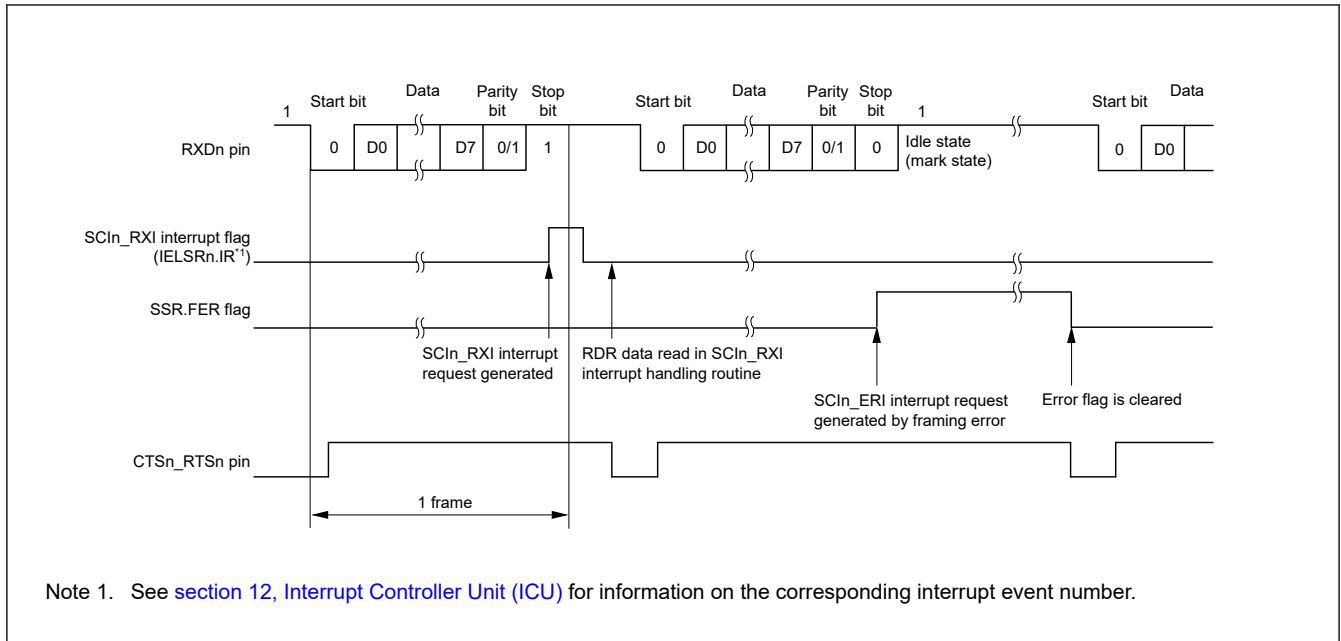
Figure 26.19 Example of SCI operation for serial reception in asynchronous mode (2) when RTS function is used, and with 8-bit data, parity bit, and 1 stop bit
