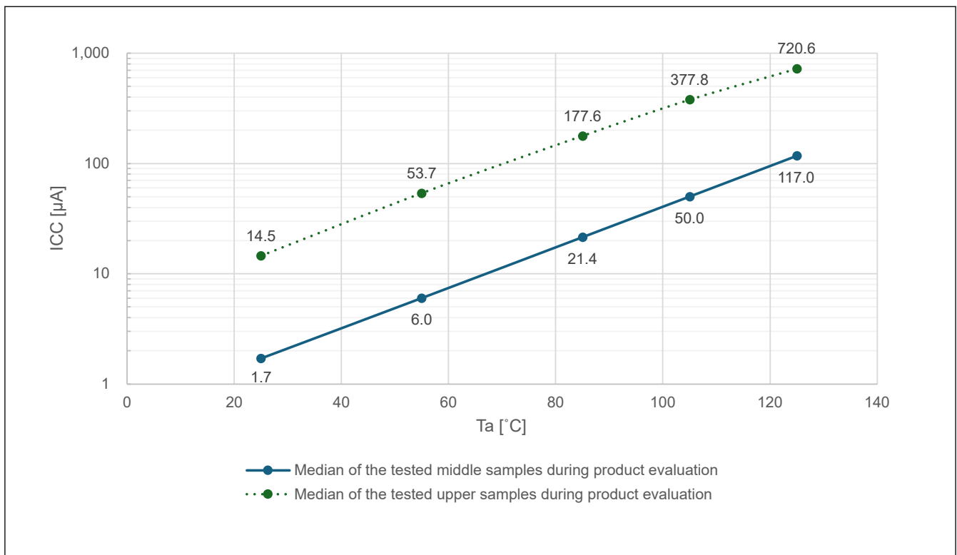
Figure 49.2 Temperature dependency in Software Standby mode (reference data)
