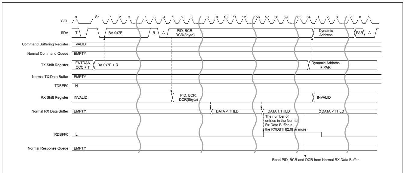
Figure 29.13 Dynamic address assign procedure (ENTDAA CCC) timing (2/3)
