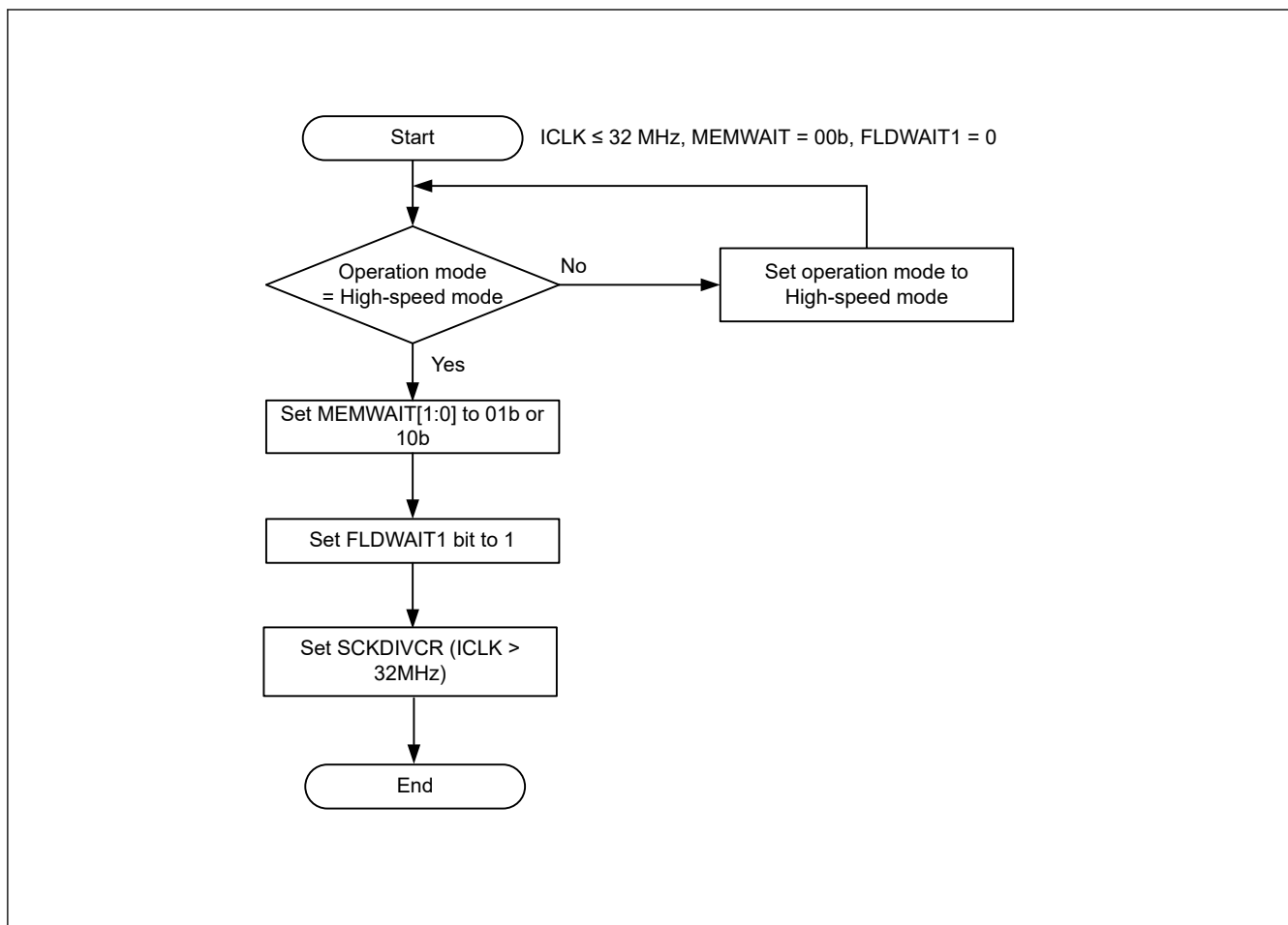
Figure 8.2 When setting ICLK > 32 MHz
