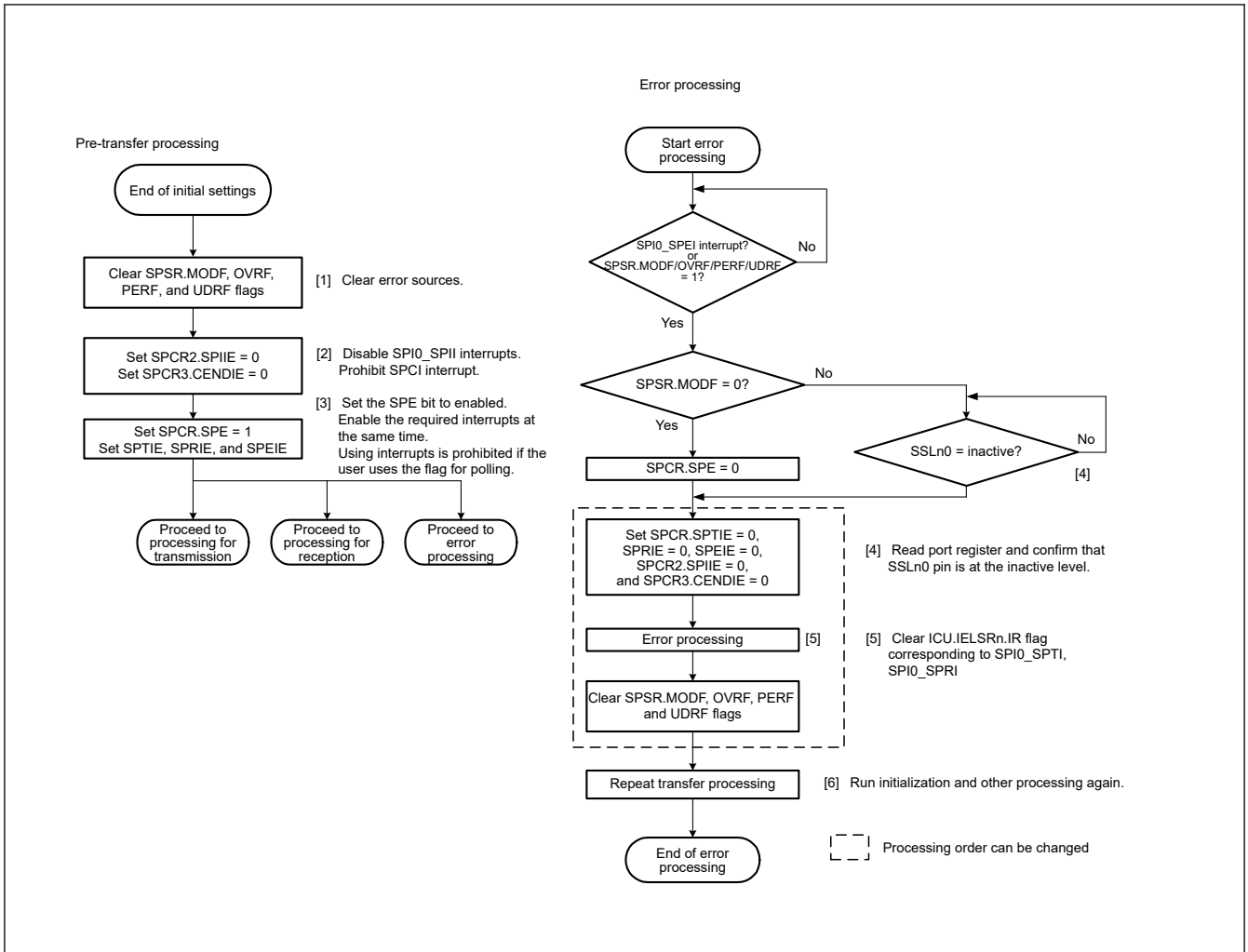
Figure 33.53 Error processing flow in master mode
