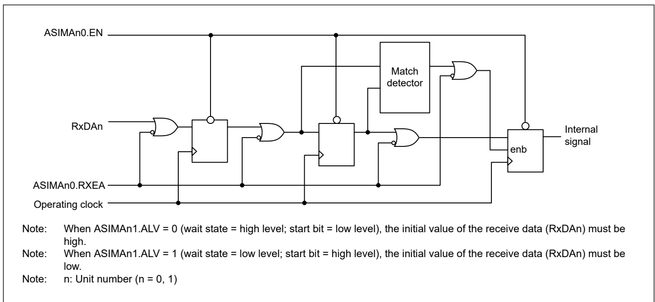
Figure 30.9 Noise filter
