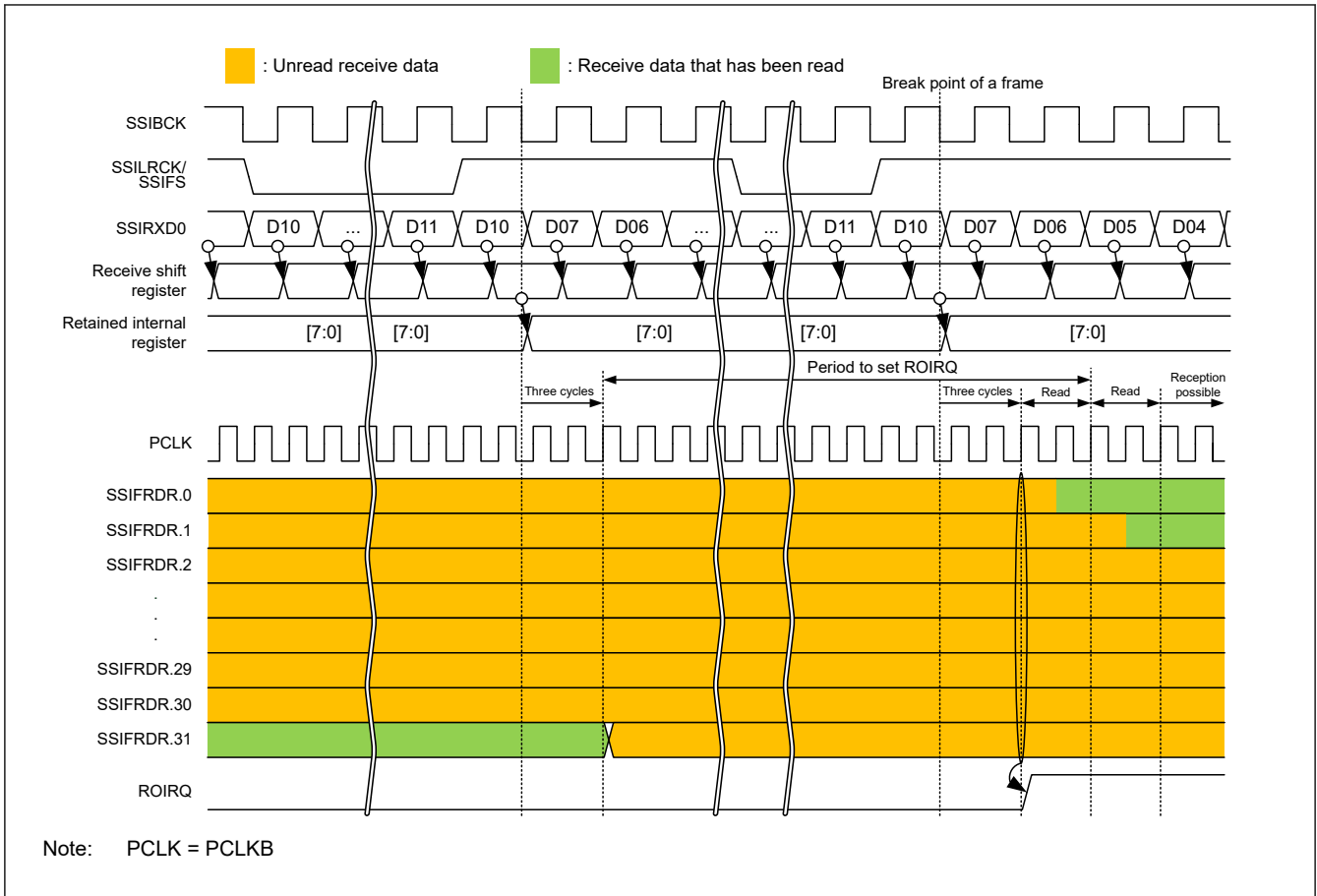
Figure 35.15 ROIRQ setting timing
