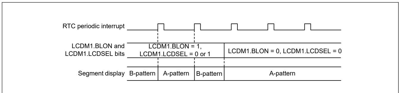
Figure 46.4 Switching operation from blinking display to A-pattern display
