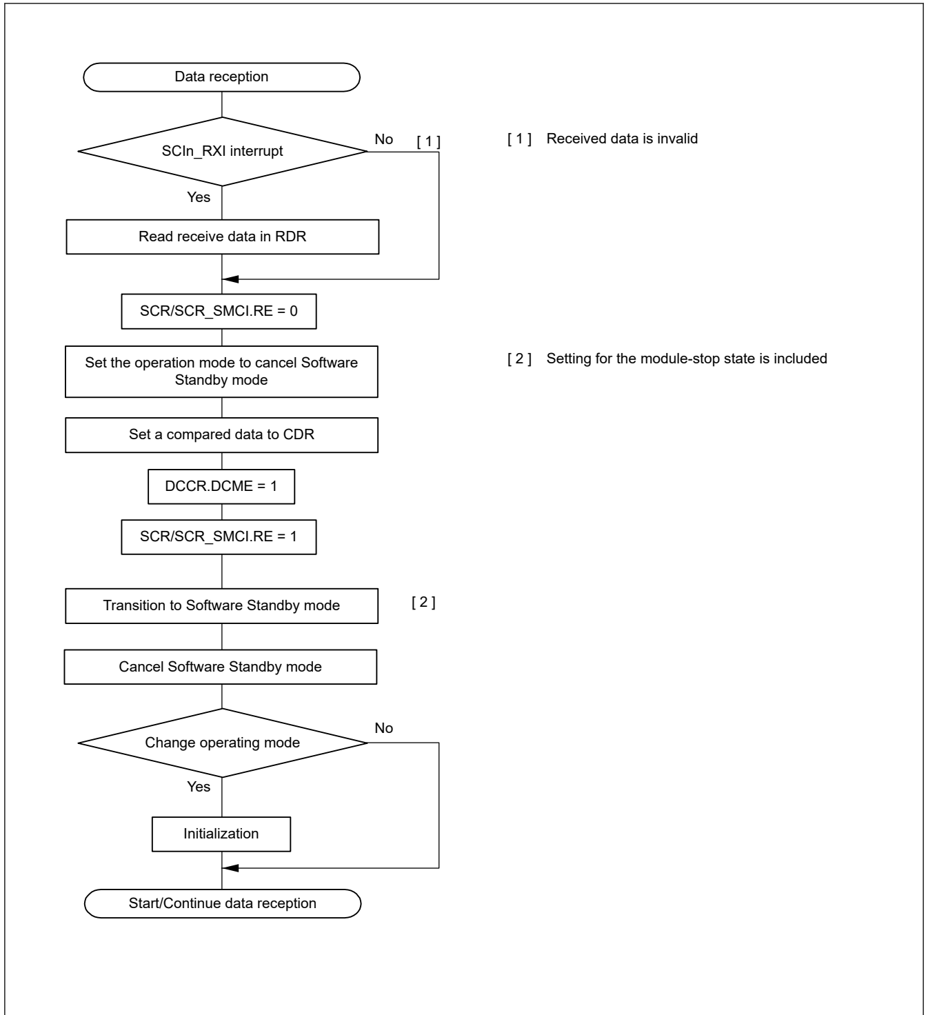
Figure 26.122 Example flow of transition to Software Standby mode during reception with address match
