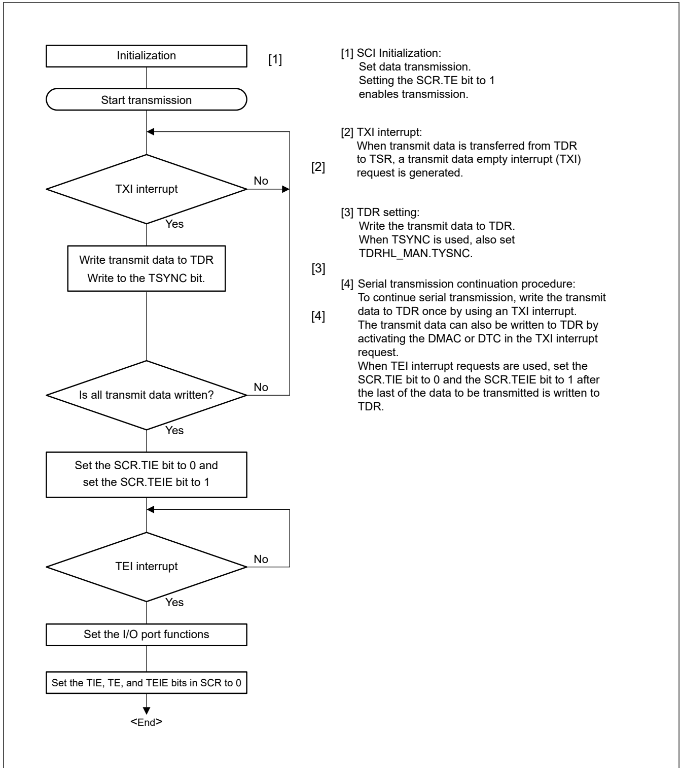
Figure 26.55 Example of Serial Transmission Flowchart in Manchester Mode
