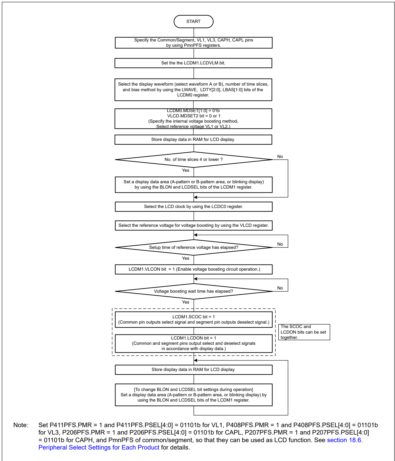
Figure 46.6 Setting procedure for internal voltage boosting method during normal liquid crystal waveform display
