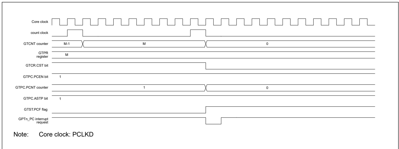
Figure 20.49 Example of the timing of operations for PWM cycle count function (saw-wave one-shot pulse mode, up-counting)
