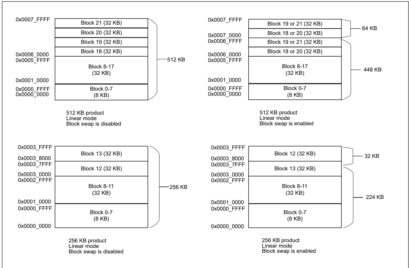
Figure 6.2 Mapping of the flash memory in linear mode
