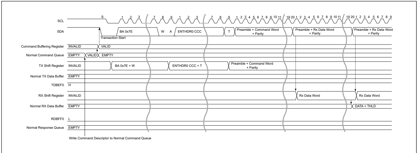
Figure 29.30 HDR data read transfer (HDR-DDR) timing (1/2)
