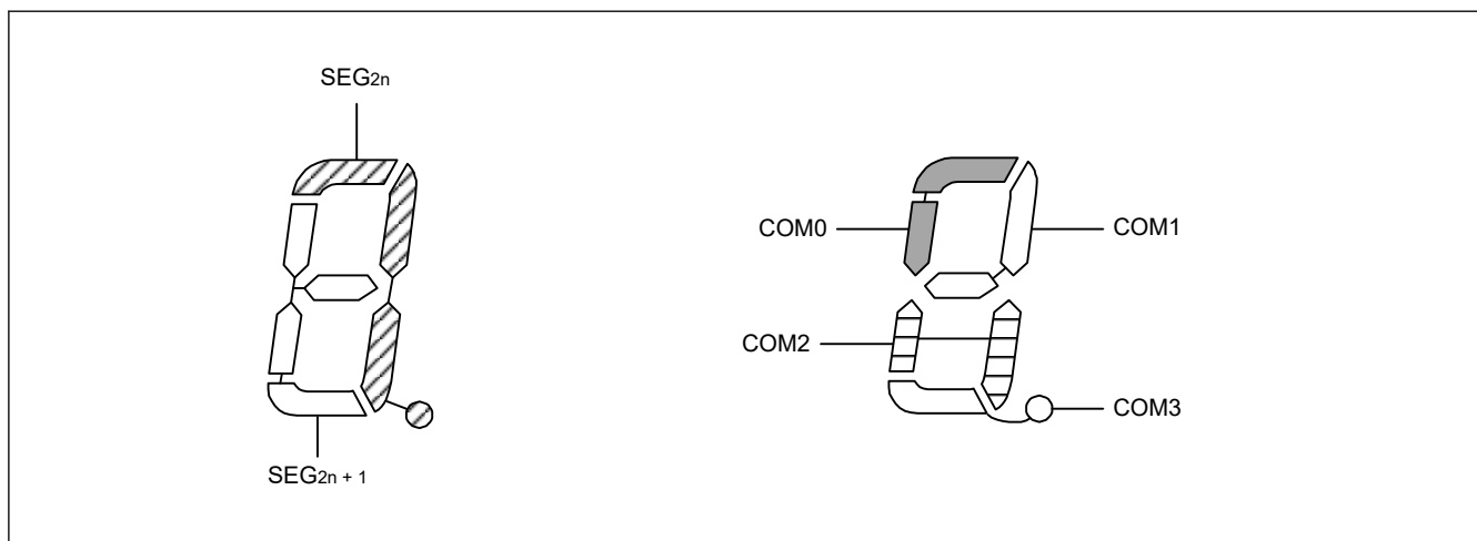
Figure 46.32 Four-time slice LCD display pattern and electrode connections
