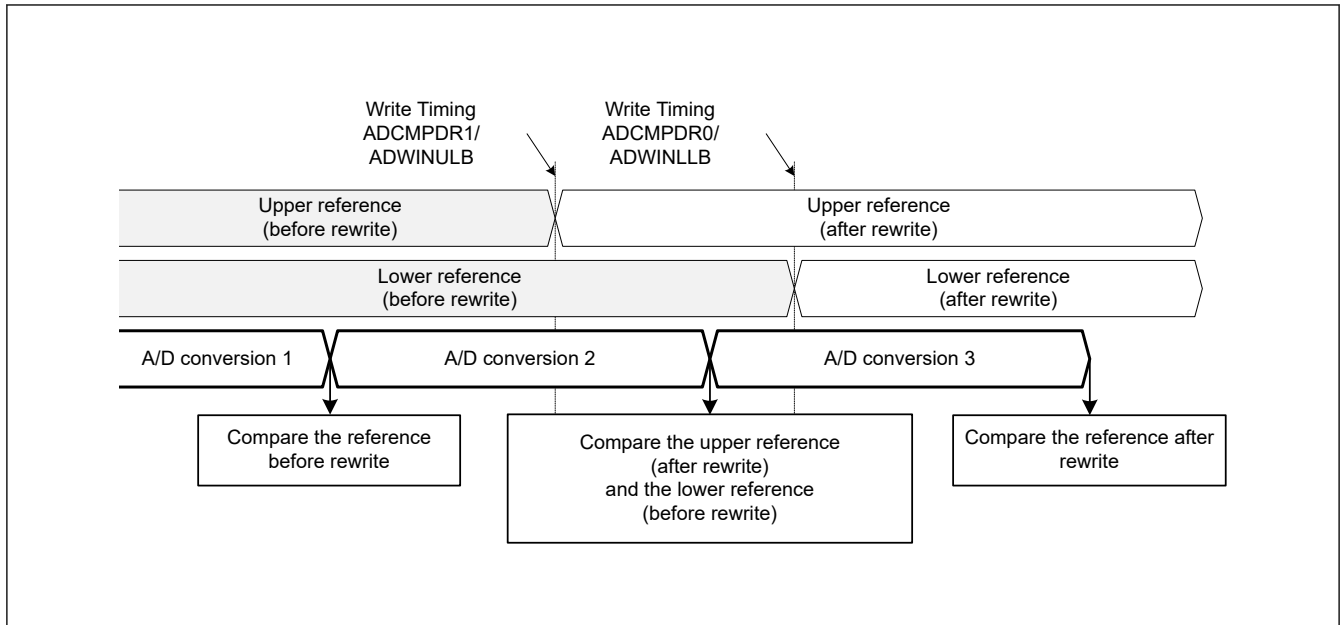
Figure 38.5 Comparison between upper and lower references before and after a rewrite
