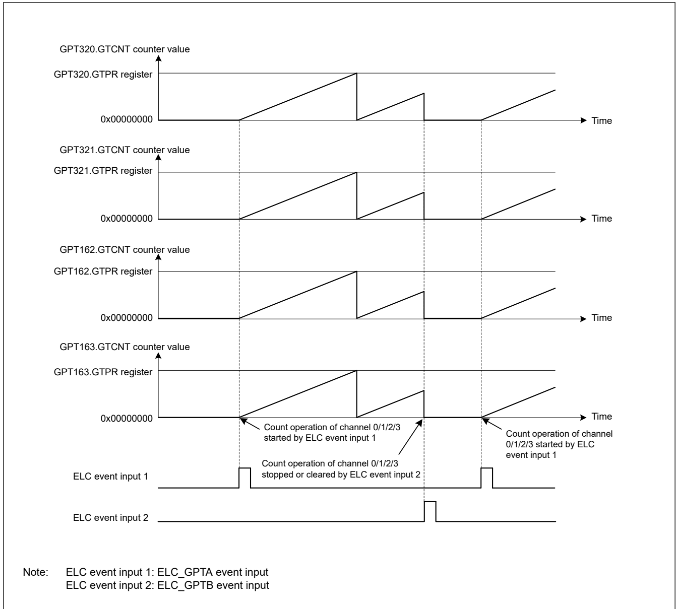
Figure 20.41 Example of a simultaneous start, stop, and clear by a hardware source with the same count cycle (GTPR register value)
