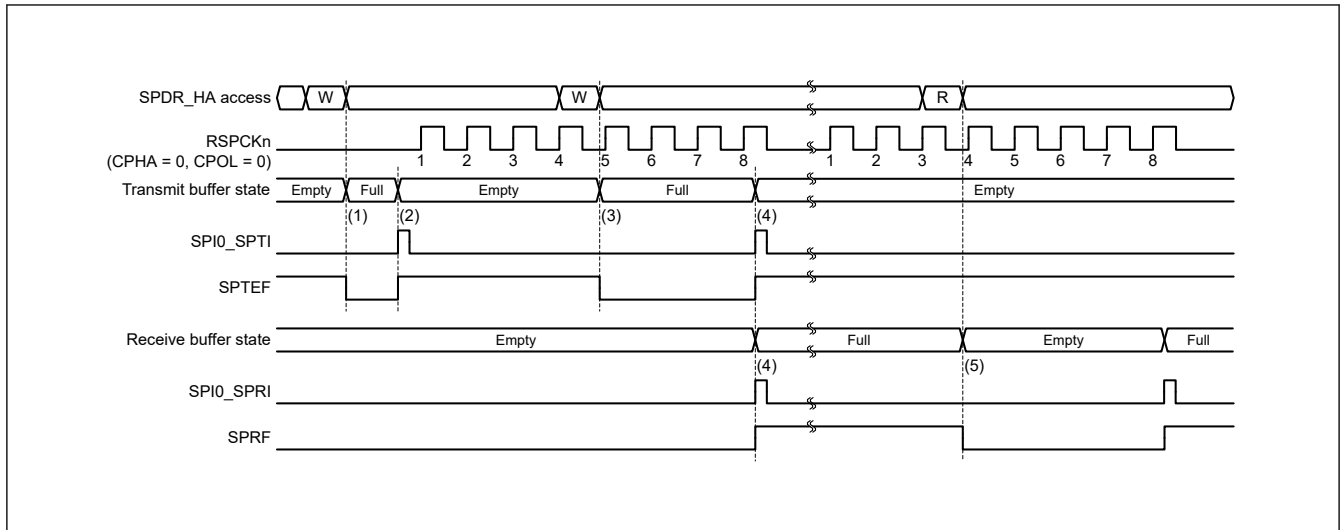
Figure 33.29 Operation example of the SPI0_SPTI and SPI0_SPRI interrupts when CPHA = 0 and CPOL = 0 in master mode
