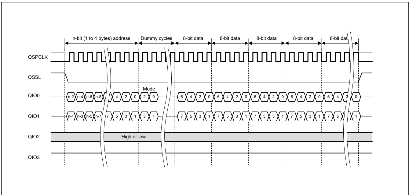
Figure 34.24 Fast Read Dual I/O bus cycle in XIP mode
