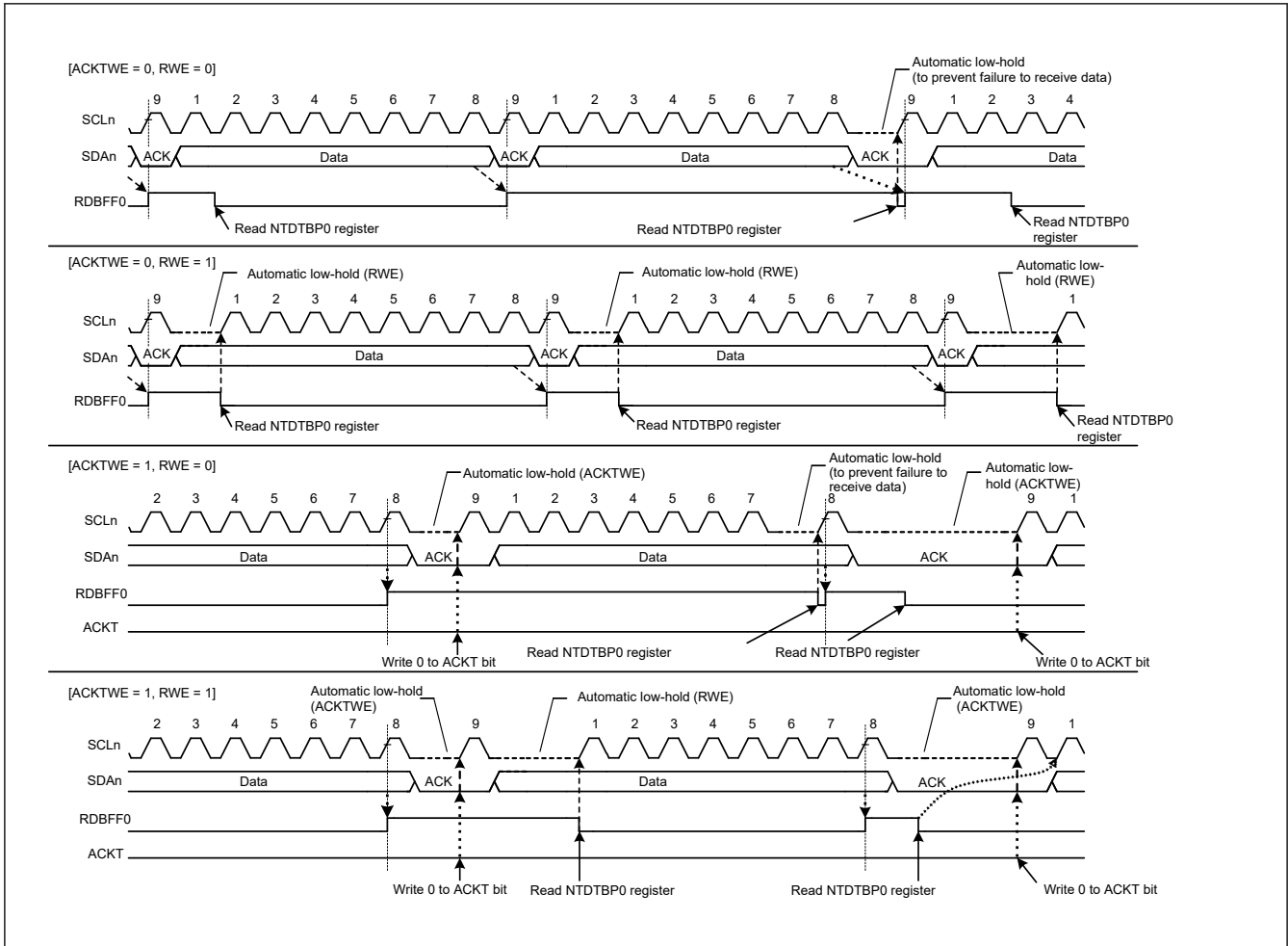
Figure 29.93 Automatic low-hold operation in receive mode (using ACKTWE and RWE bits)
