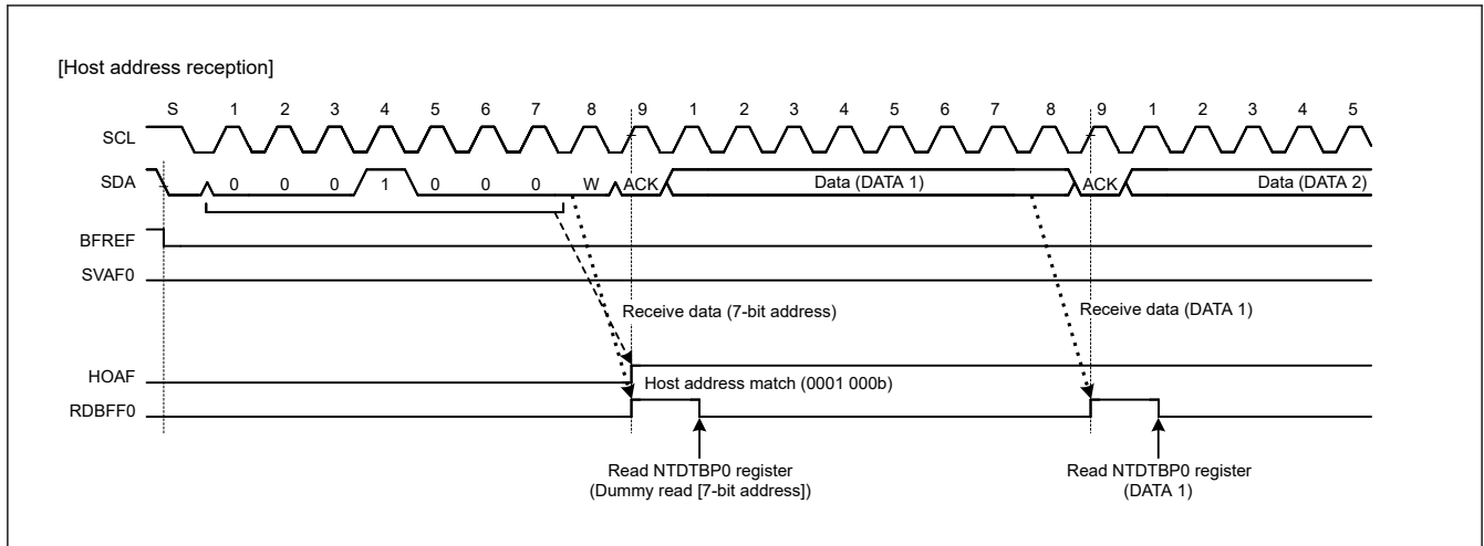
Figure 29.85 HOAF flag set timing during reception of host address
