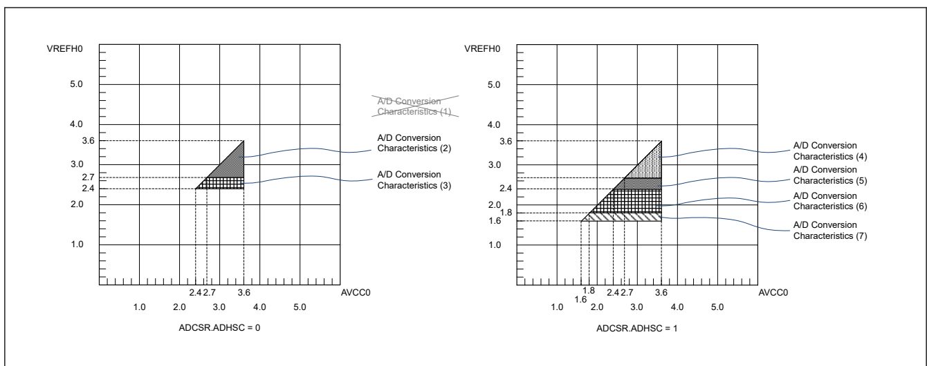
Figure 49.60 AVCC0 to VREFH0 voltage range
