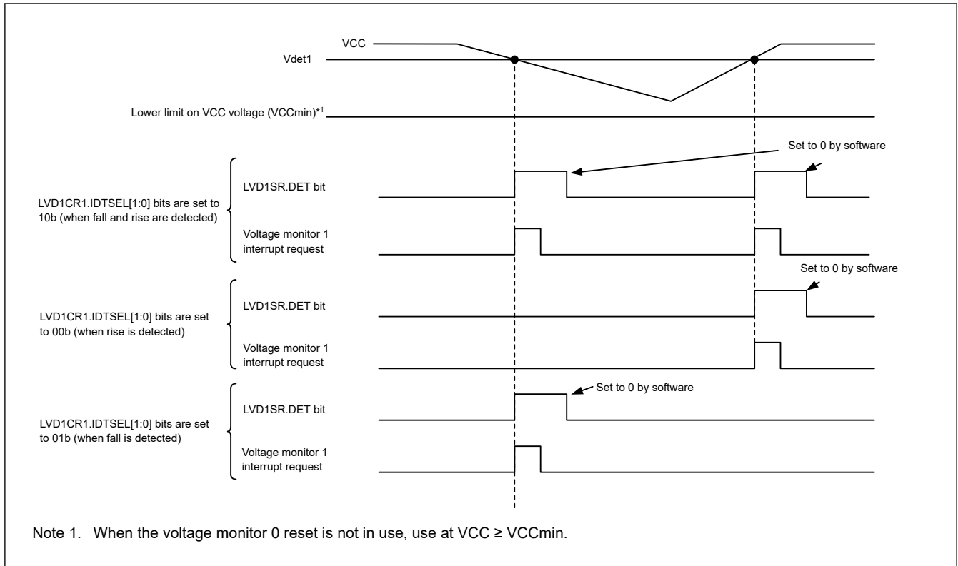
Figure 7.5 Example of voltage monitor 1 interrupt operation
