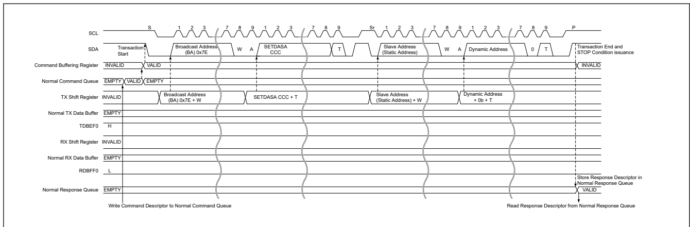
Figure 29.15 Dynamic address assign procedure (SETDASA CCC) timing
