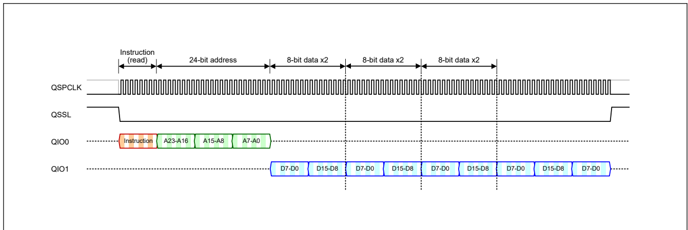
Figure 34.33 Successive data read operations using the prefetch function
