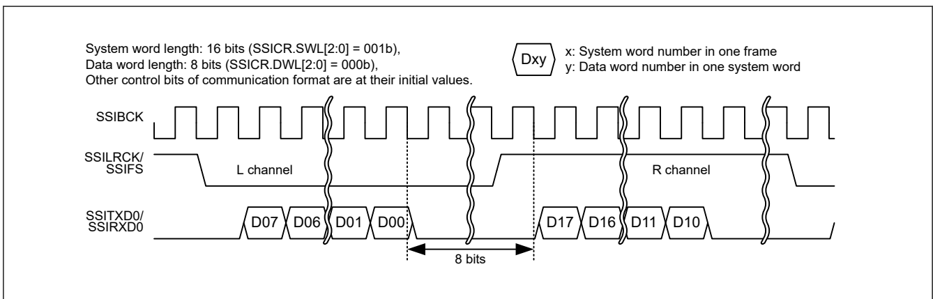
Figure 35.35 Example of padding bit transfer (I 2 S format: system word length > data word length)
