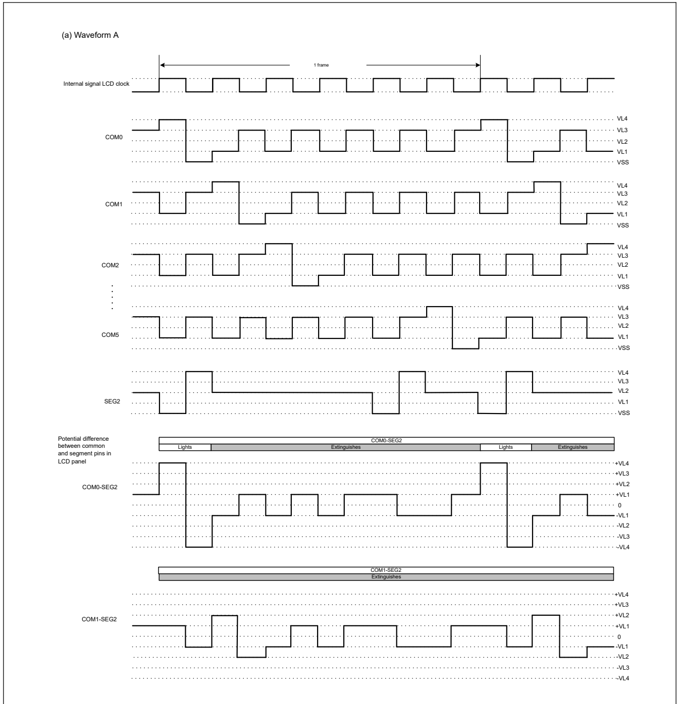
Figure 46.38 Six-time slice LCD drive waveform examples between SEG2 and each common signal using 1/4 bias method
