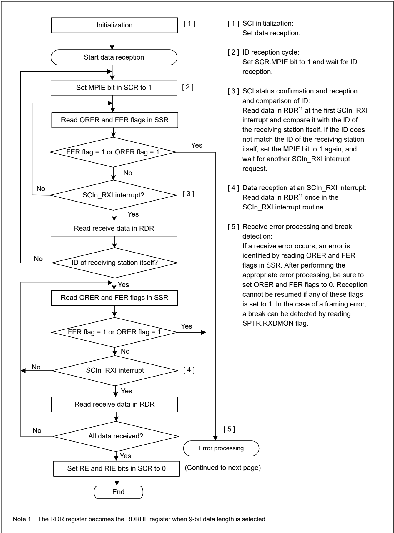
Figure 26.45 Example flow of multi-processor serial reception with non-FIFO selected (1)
