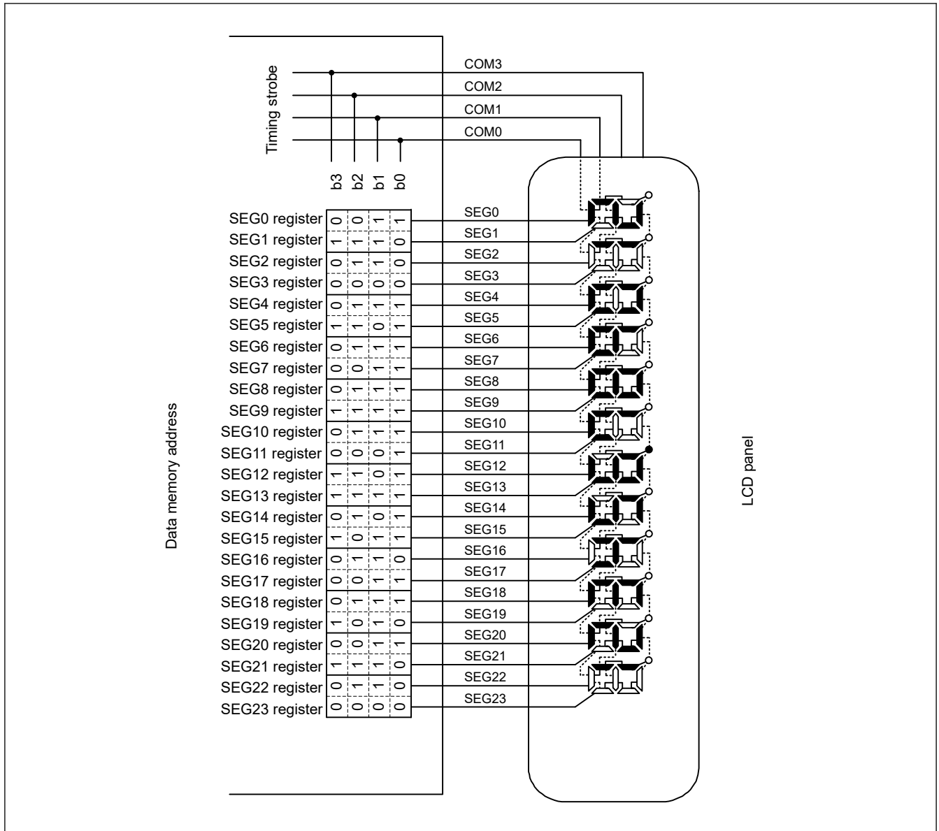
Figure 46.33 Example of connecting four-time slice LCD panel
