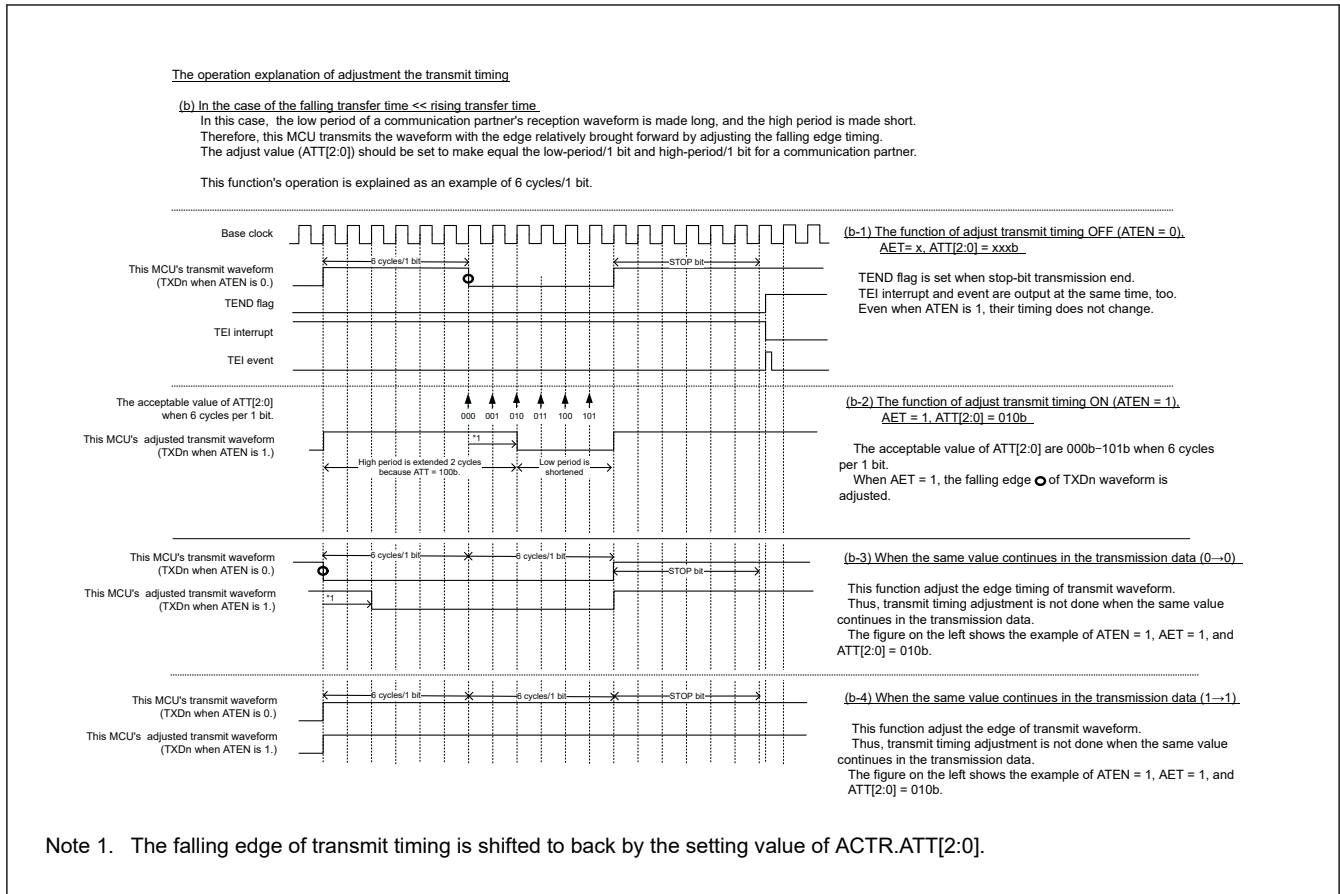
Figure 26.39 The adjustment operation explanation for the transmit timing when AET is 1
