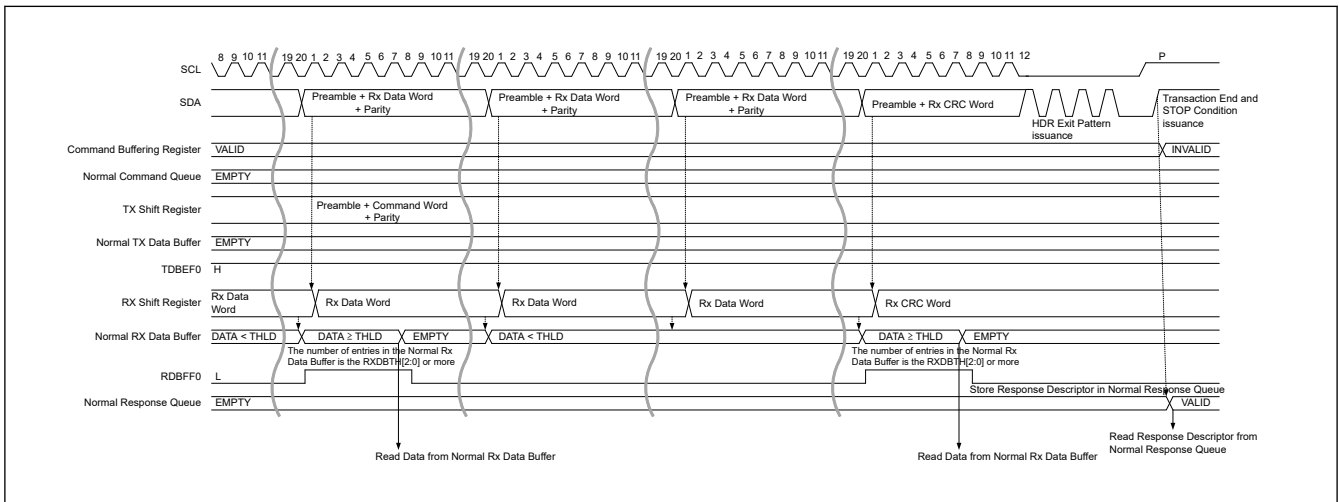
Figure 29.31 HDR data read transfer (HDR-DDR) timing (2/2)
