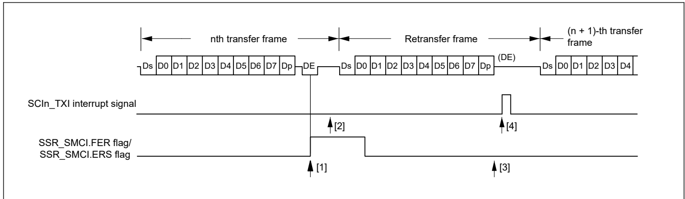
Figure 26.82 Data re-transfer operation in smart card interface transmission mode
