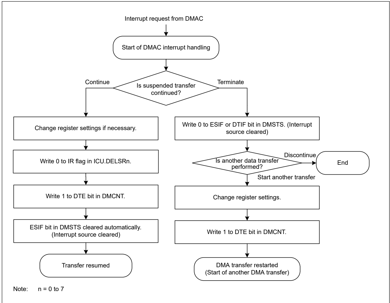
Figure 15.34 DMAC interrupt handling routine to resume/terminate DMA transfer
