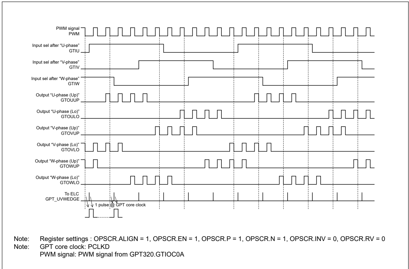
Figure 20.62 Example of 6-phase PWM output operation with chopper control
