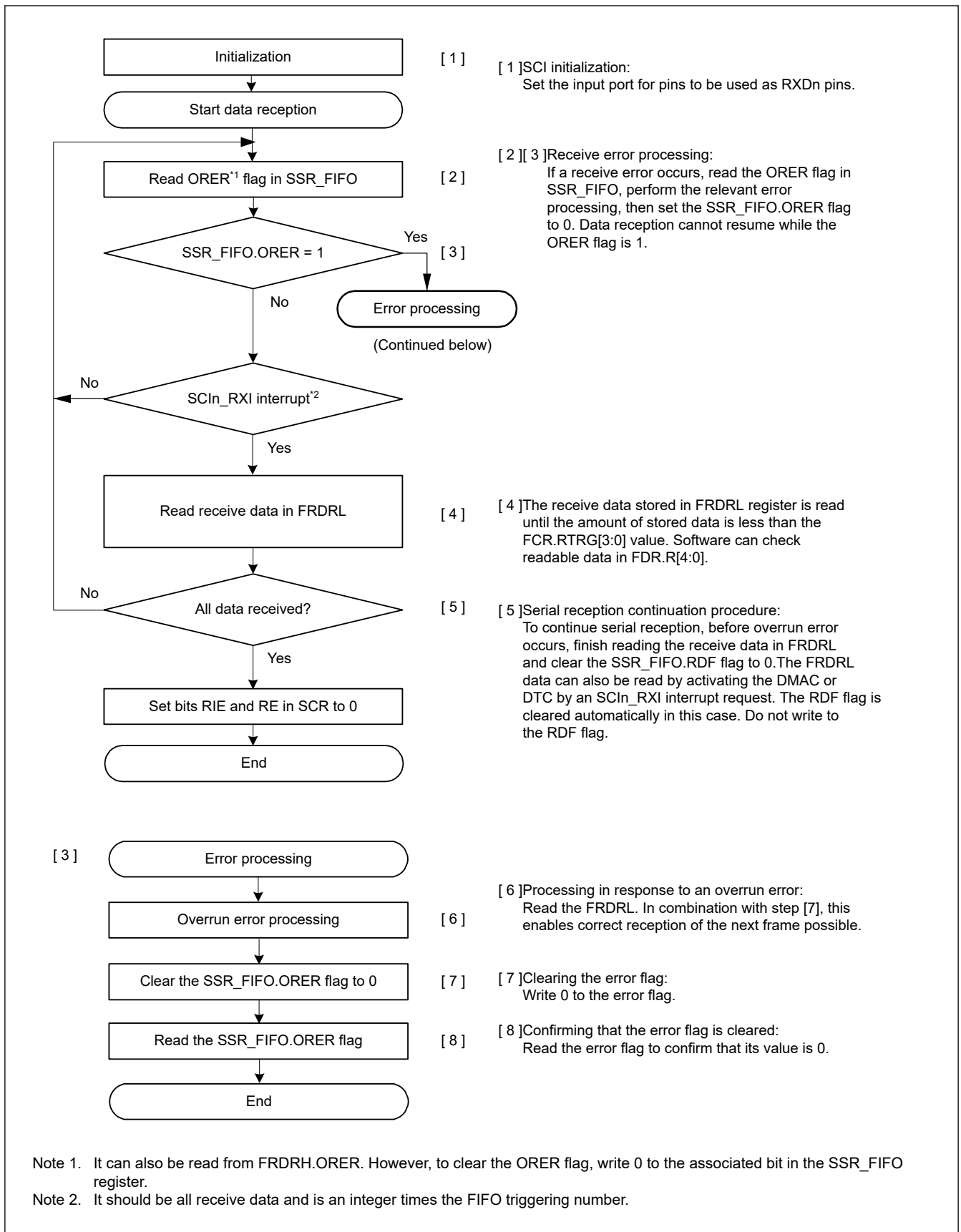
Figure 26.74 Example flow of serial reception in clock synchronous mode with FIFO selected
