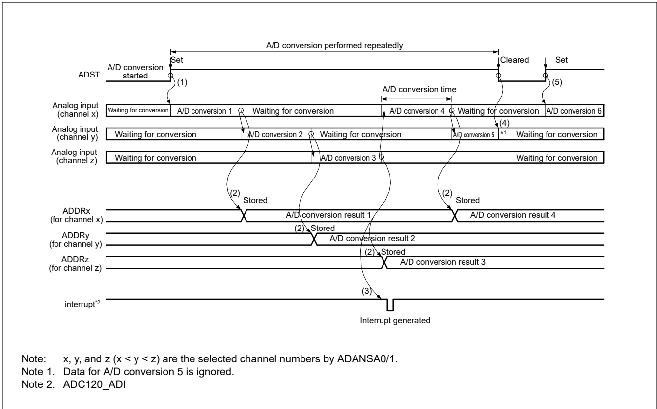
Figure 38.12 Example basic operation in continuous scan mode when the analog inputs (channel x to z) are selected
