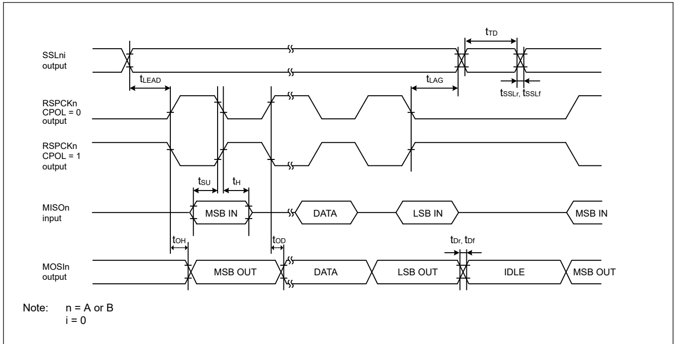
Figure 49.34 SPI timing (master, CPHA = 1) (bit rate: PCLKB division ratio is set to any value other than 1/2)
