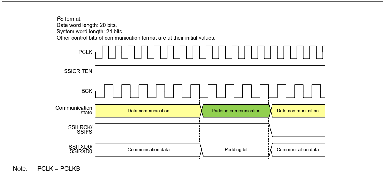
Figure 35.48 Transition from data communication to padding communication
