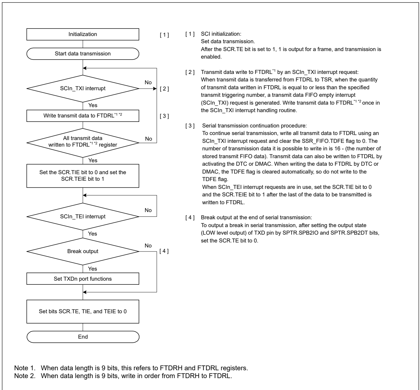
Figure 26.17 Example flow of serial transmission in asynchronous mode with FIFO selected
