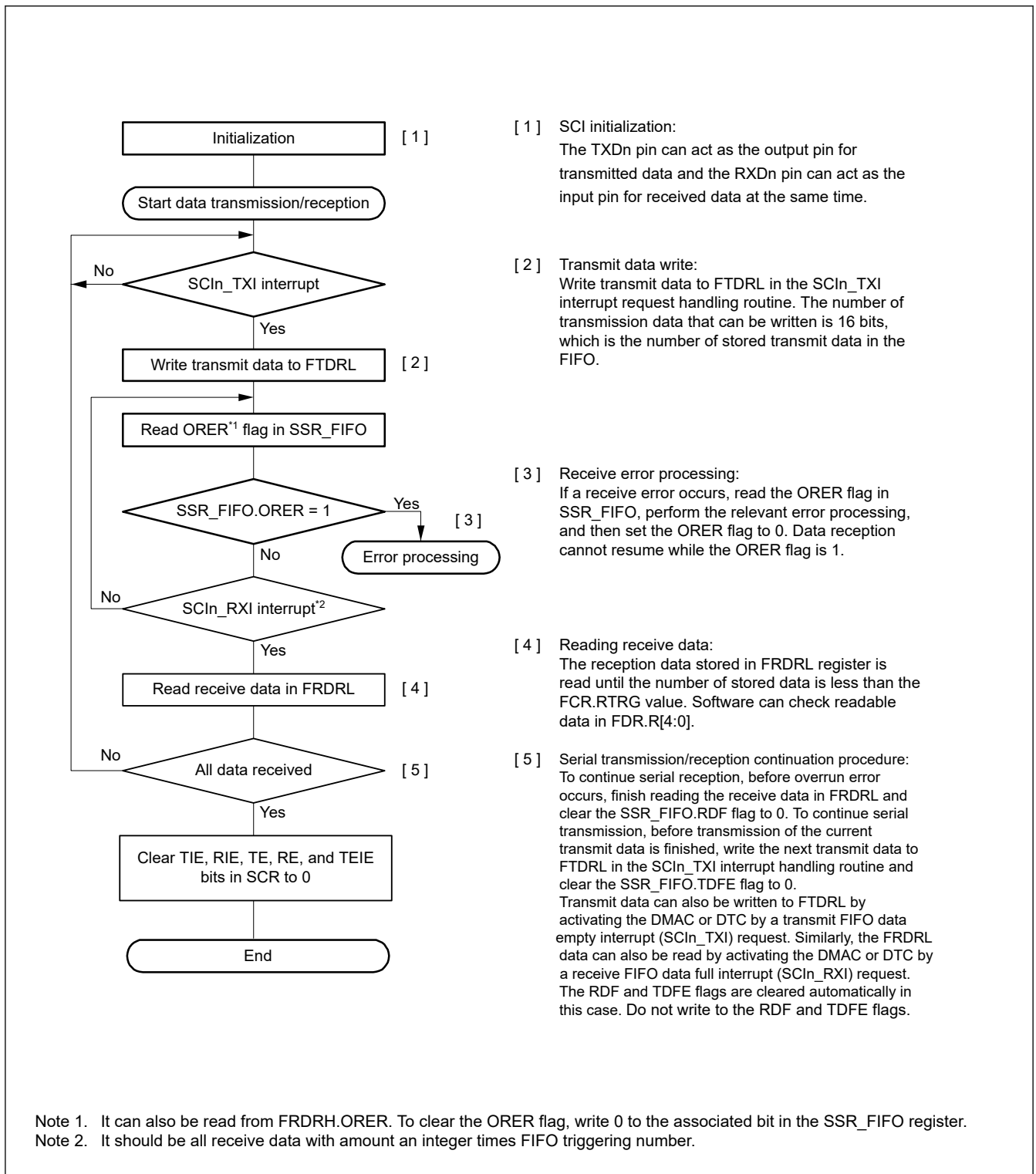
Figure 26.76 Example flow of simultaneous serial transmission and reception in clock synchronous mode with FIFO selected
