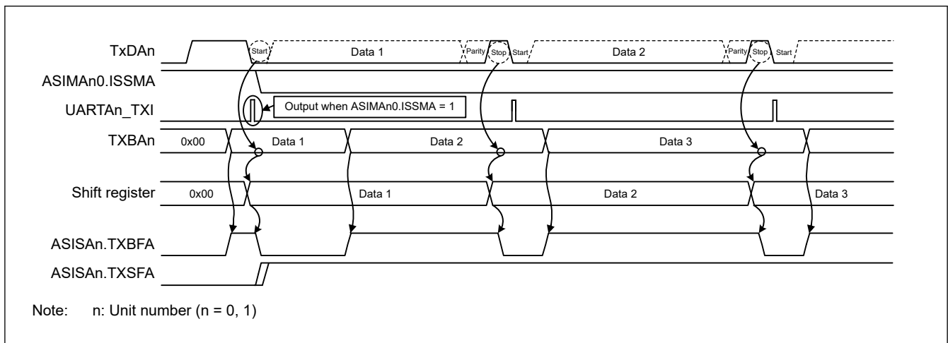
Figure 30.5 Timing when continuous transmission is started
