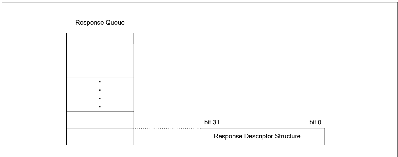
Figure 29.3 Response descriptor data structure
