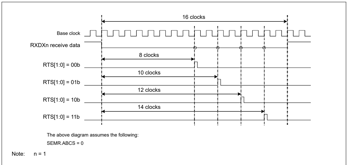
Figure 26.114 Timing for sampling of data received through RXDXn
