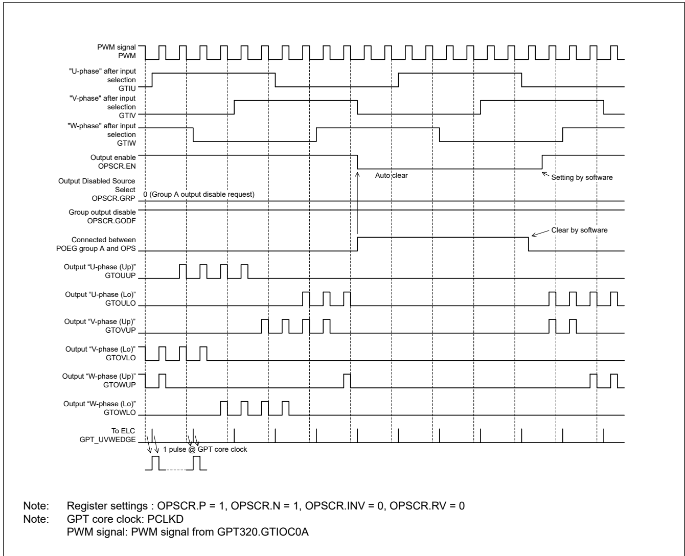
Figure 20.63 Example of group output disable control operation
