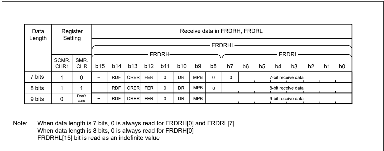
Figure 26.47 Data format stored in FRDRH and FRDRL in multi-processor mode with FIFO selected
