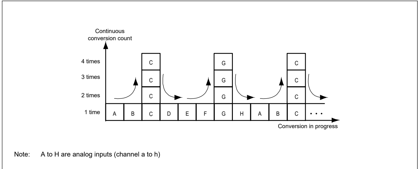
Figure 38.2 Scan conversion sequence with ADADC.ADC[2:0] = 011b, set 1 for analog inputs C and G by ADADS0/1
