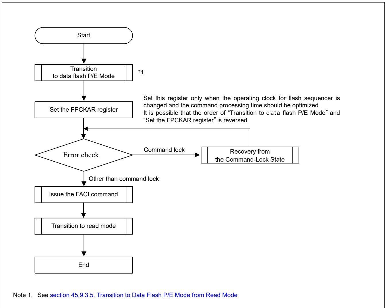
Figure 45.8 Overview of command usage in data flash P/E mode
