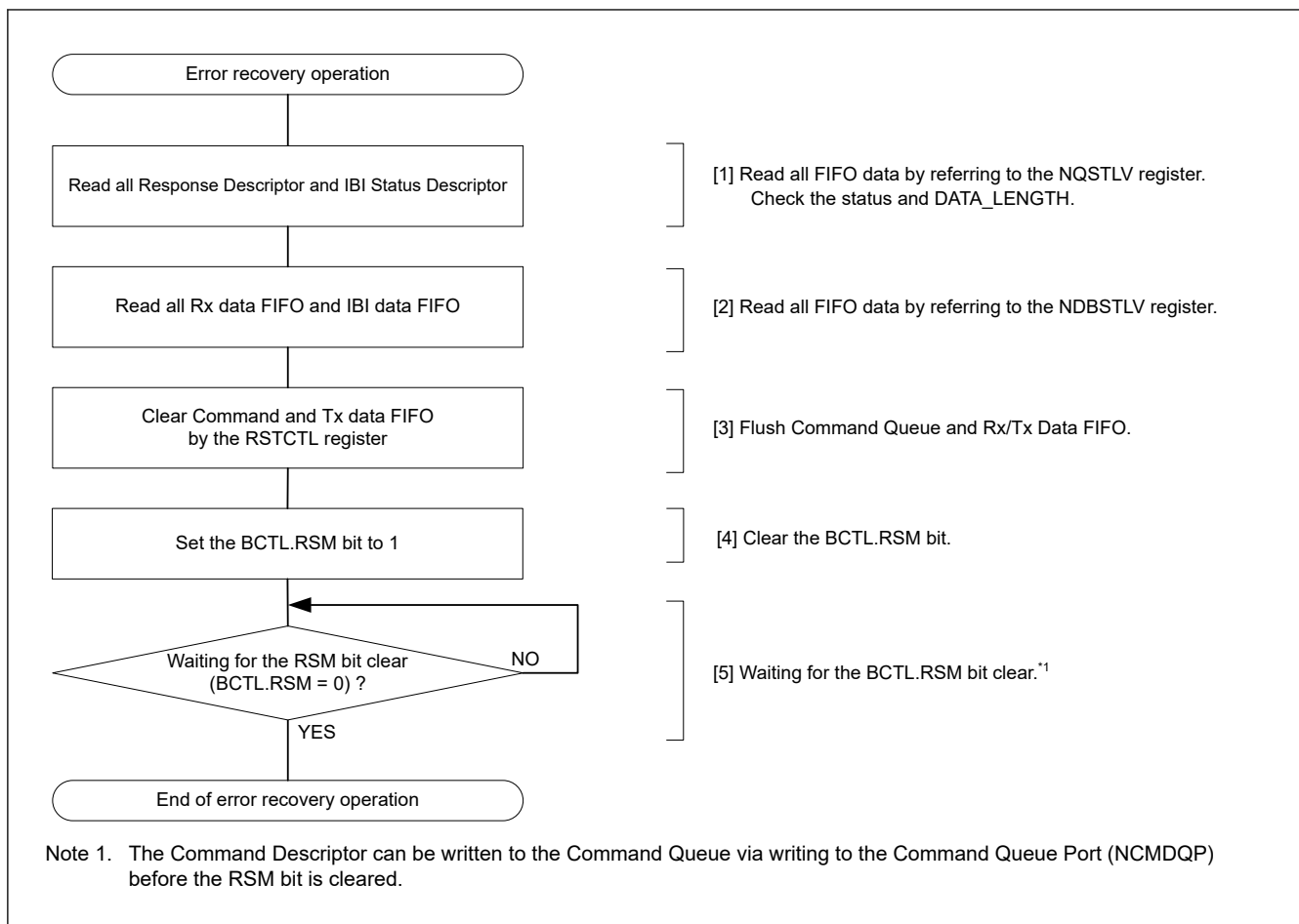
Figure 29.120 Example of error recovery operation flowchart for I3C master
