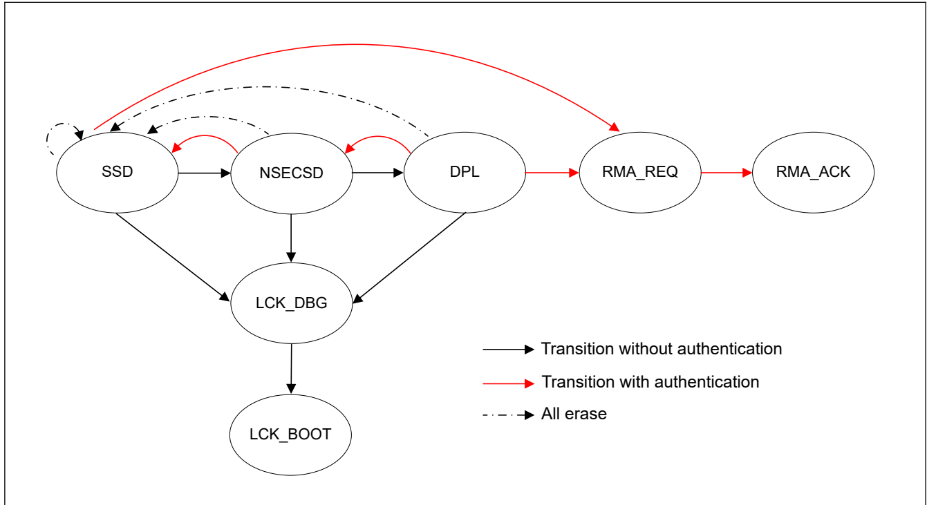
Figure 48.2 Illustration of the device lifecycle
