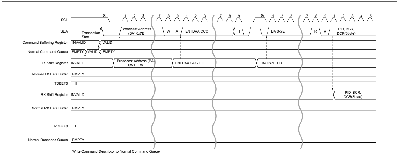
Figure 29.12 Dynamic address assign procedure (ENTDAA CCC) timing (1/3)
