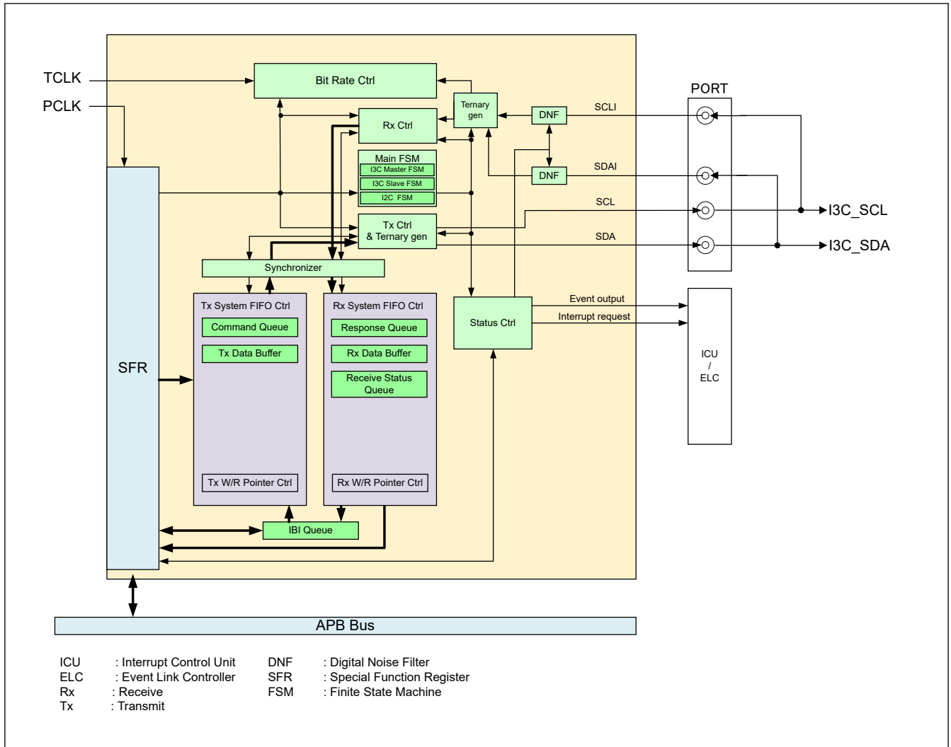
Figure 29.1 I3C block diagram
