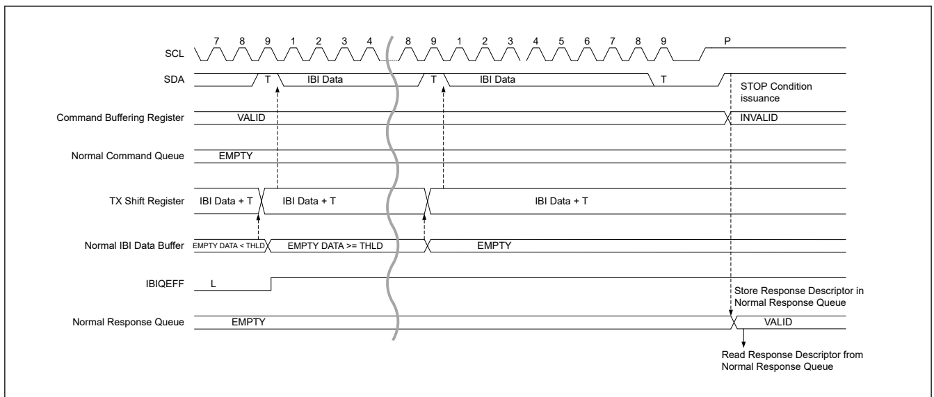
Figure 29.64 I3C slave IBI transfer timing (2/2)
