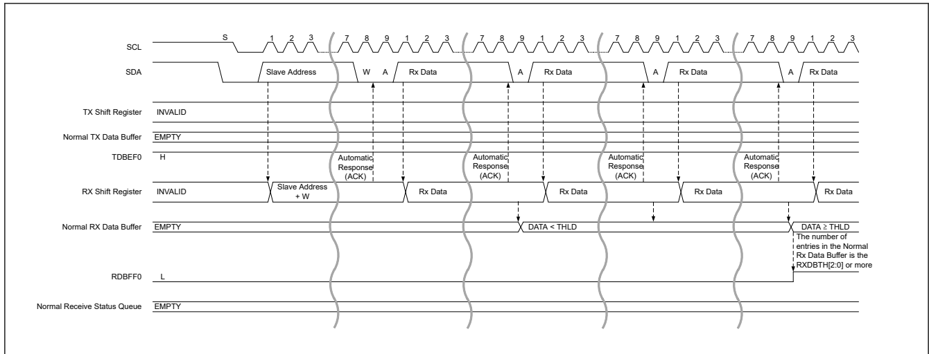
Figure 29.47 Legacy I 2 C message data write transfer timing (1/2)
