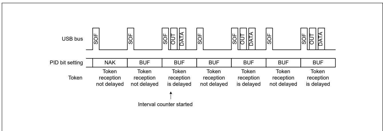
Figure 25.15 Relationship between frames and expected token reception when IITV[2:0] ≠ 0
