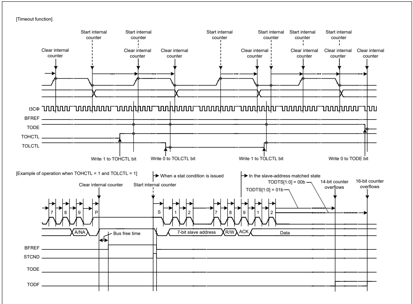
Figure 29.113 Timeout error detection (TODE, TODTS[1:0], TOHCTL, and TOLCTL bits)
