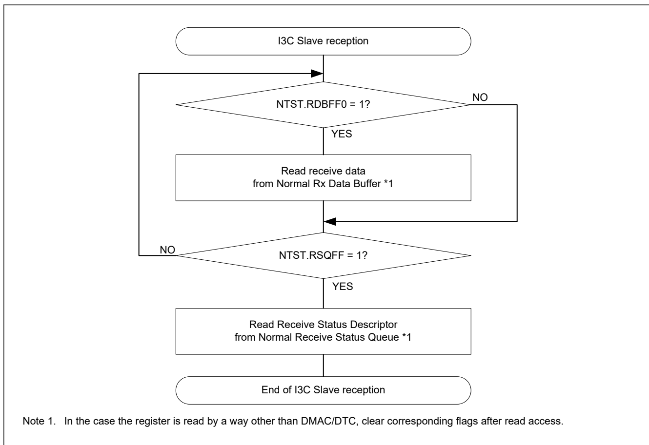
Figure 29.151 Example of I3C slave reception flowchart (normal FIFO buffer transfer)
