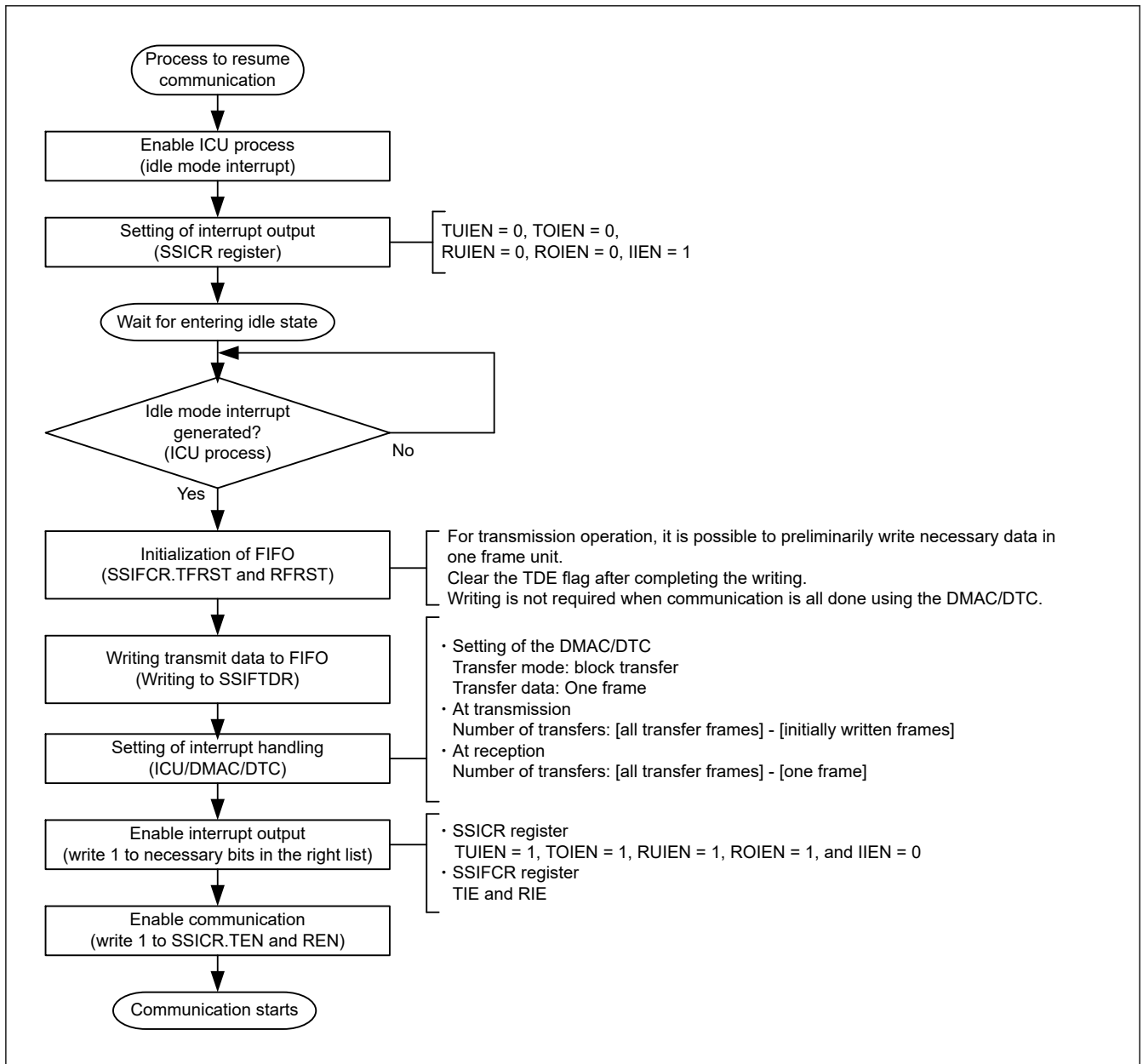
Figure 35.57 Procedure to resume communication (CPU operation procedure)
