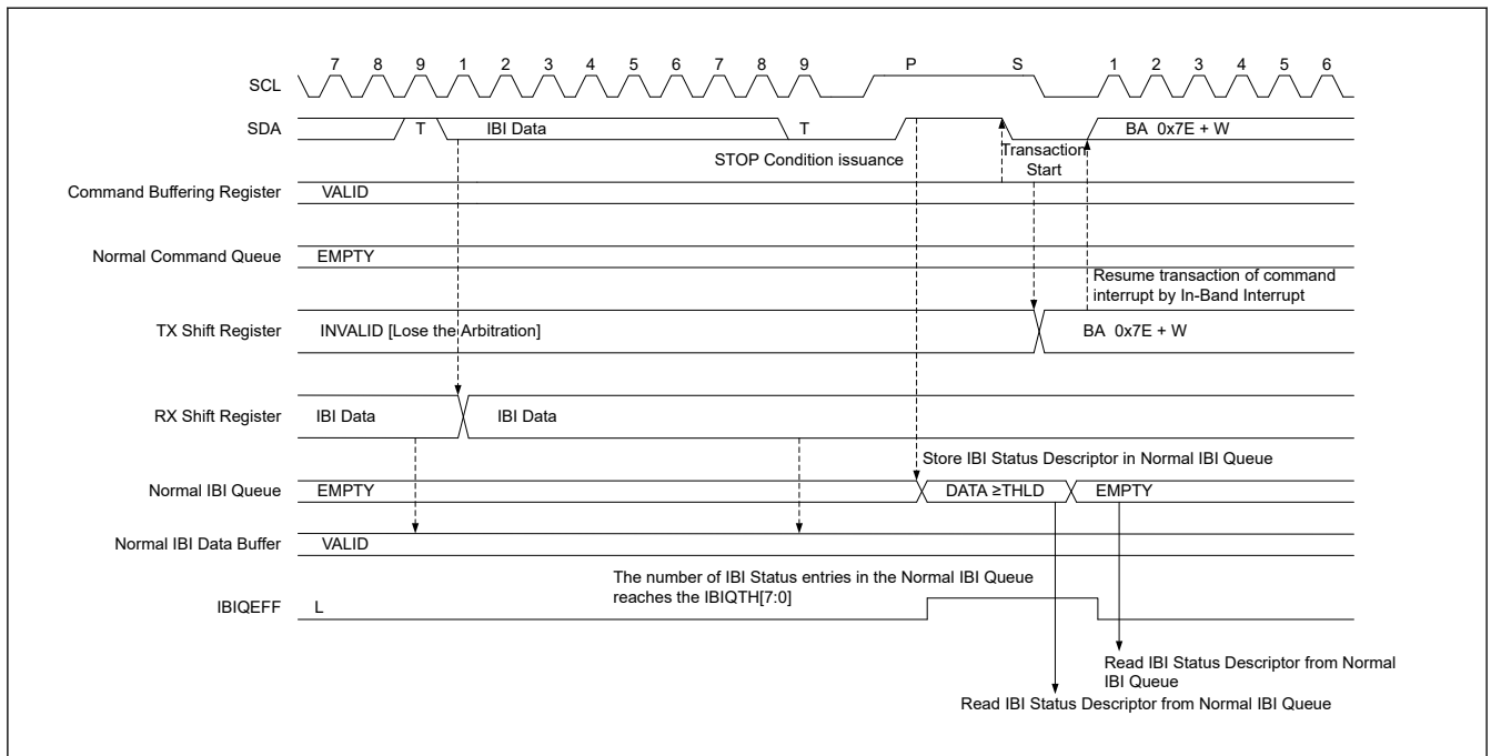
Figure 29.35 I3C master IBI transfer timing (2/2)
