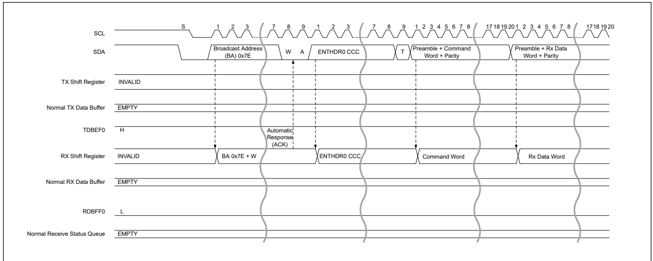
Figure 29.53 HDR data write transfer (HDR-DDR) timing (1/3)
