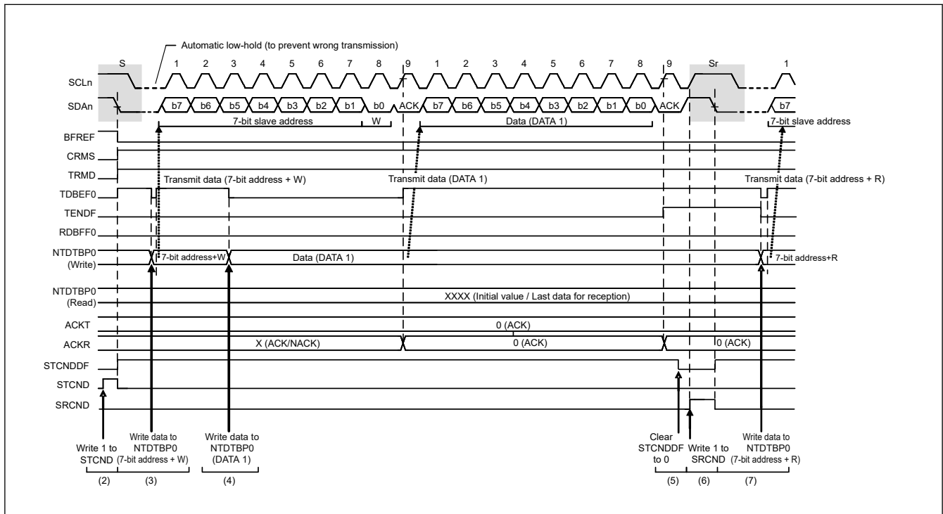
Figure 29.79 Repeated START condition issuance after the master transmission timing
