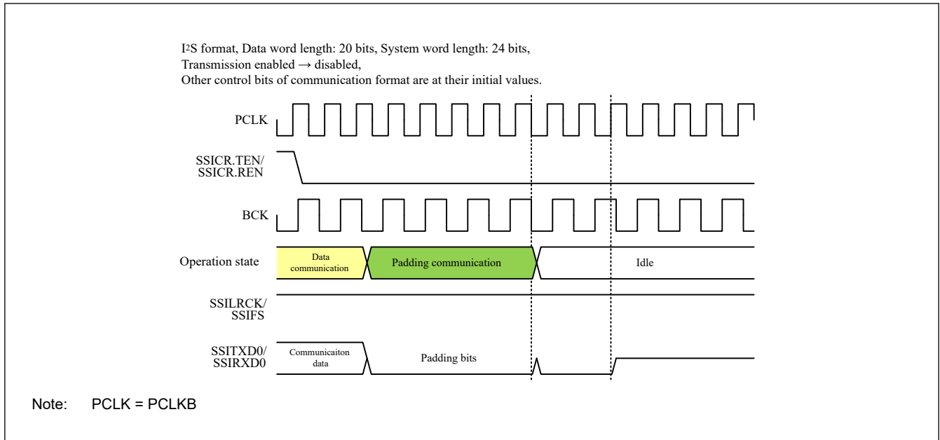
Figure 35.50 Halt from the padding communication
