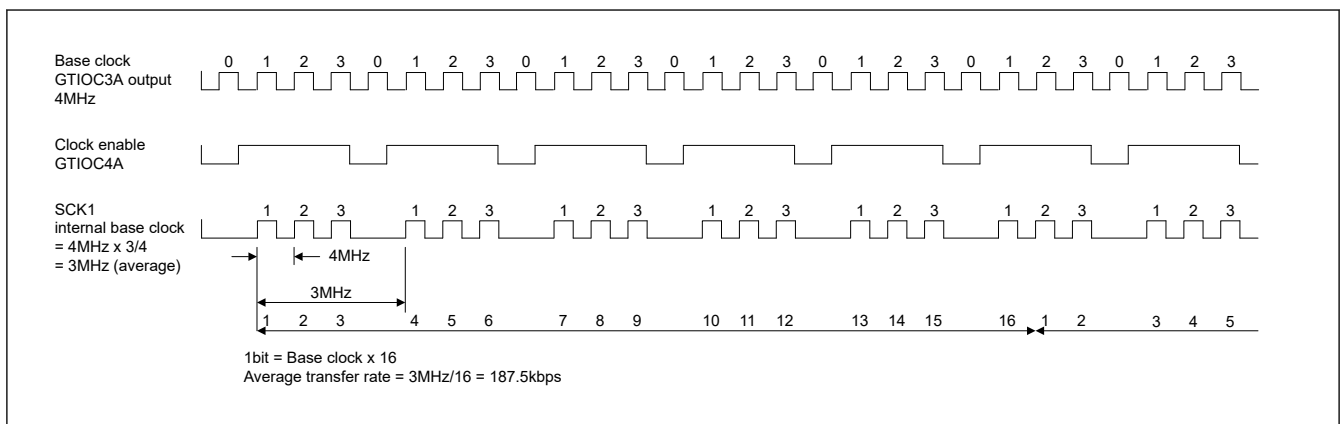
Figure 26.4 Example of average transfer rate setting when GPT clock is input
