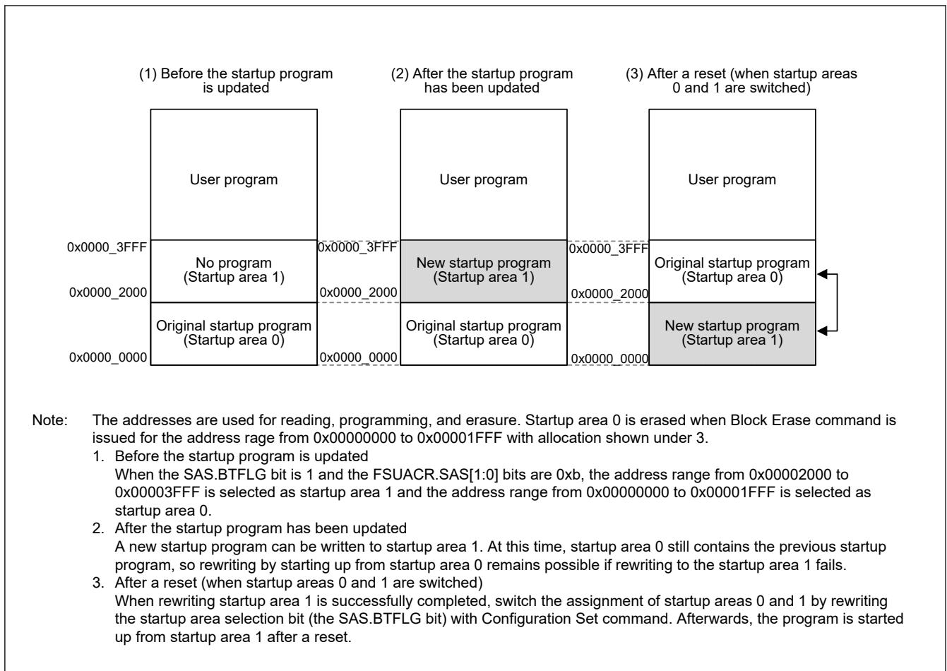
Figure 45.21 Concept of protection of the startup program
