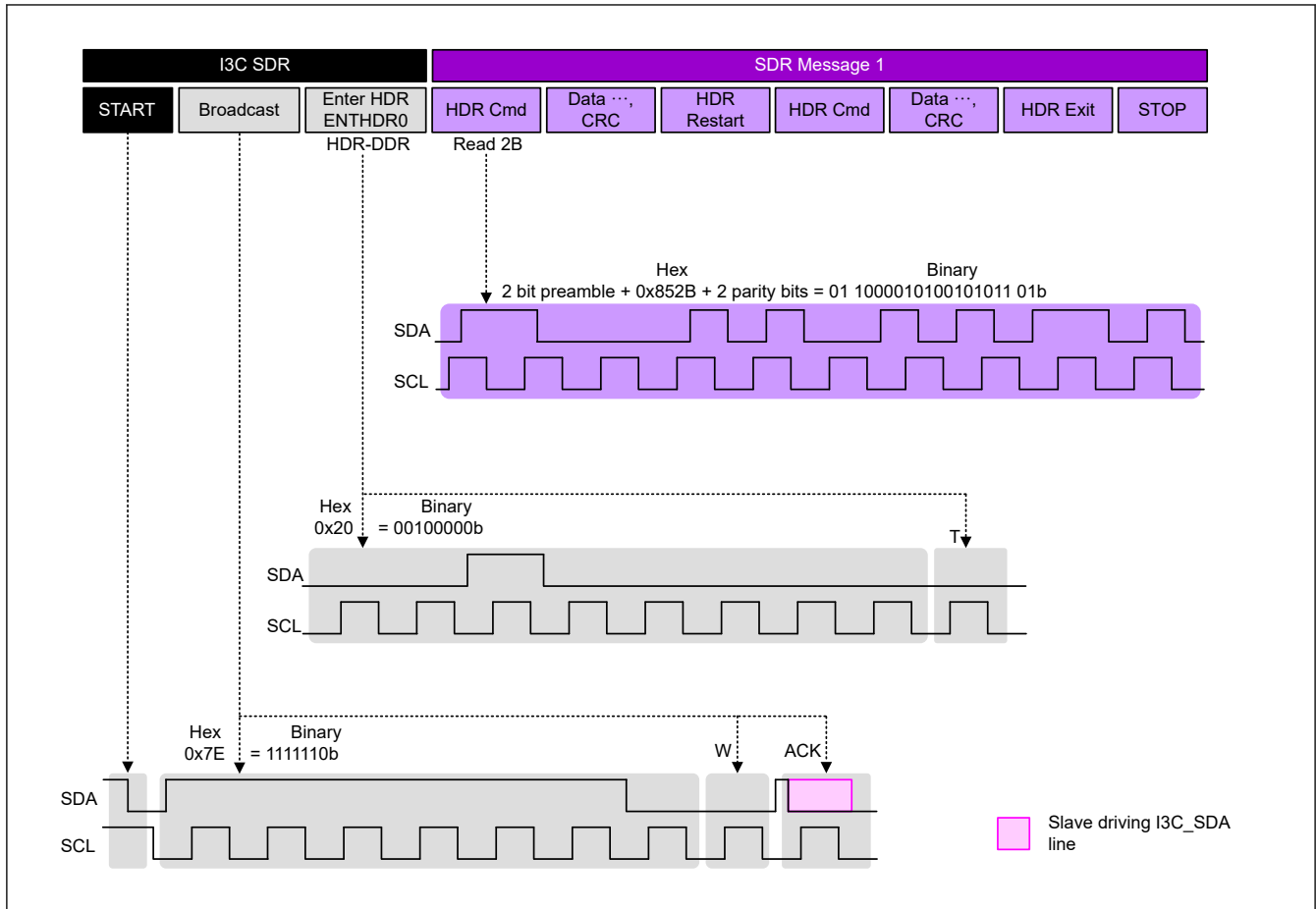
Figure 29.74 Example communication using HDR-DDR protocol
