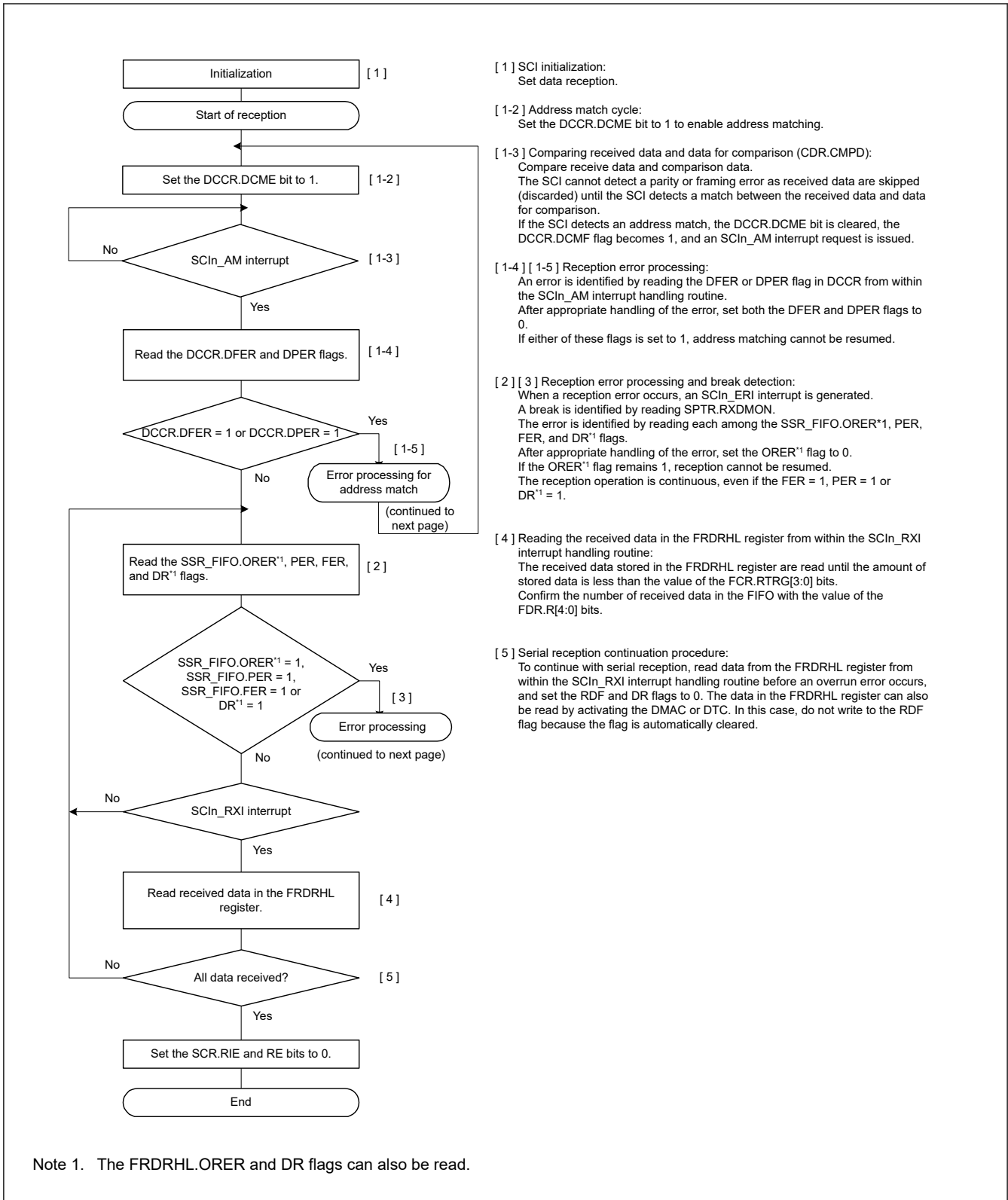
Figure 26.28 Example Flowchart of Serial Reception in Asynchronous Mode (FIFO Selected and Address Matching Enabled) (1)
