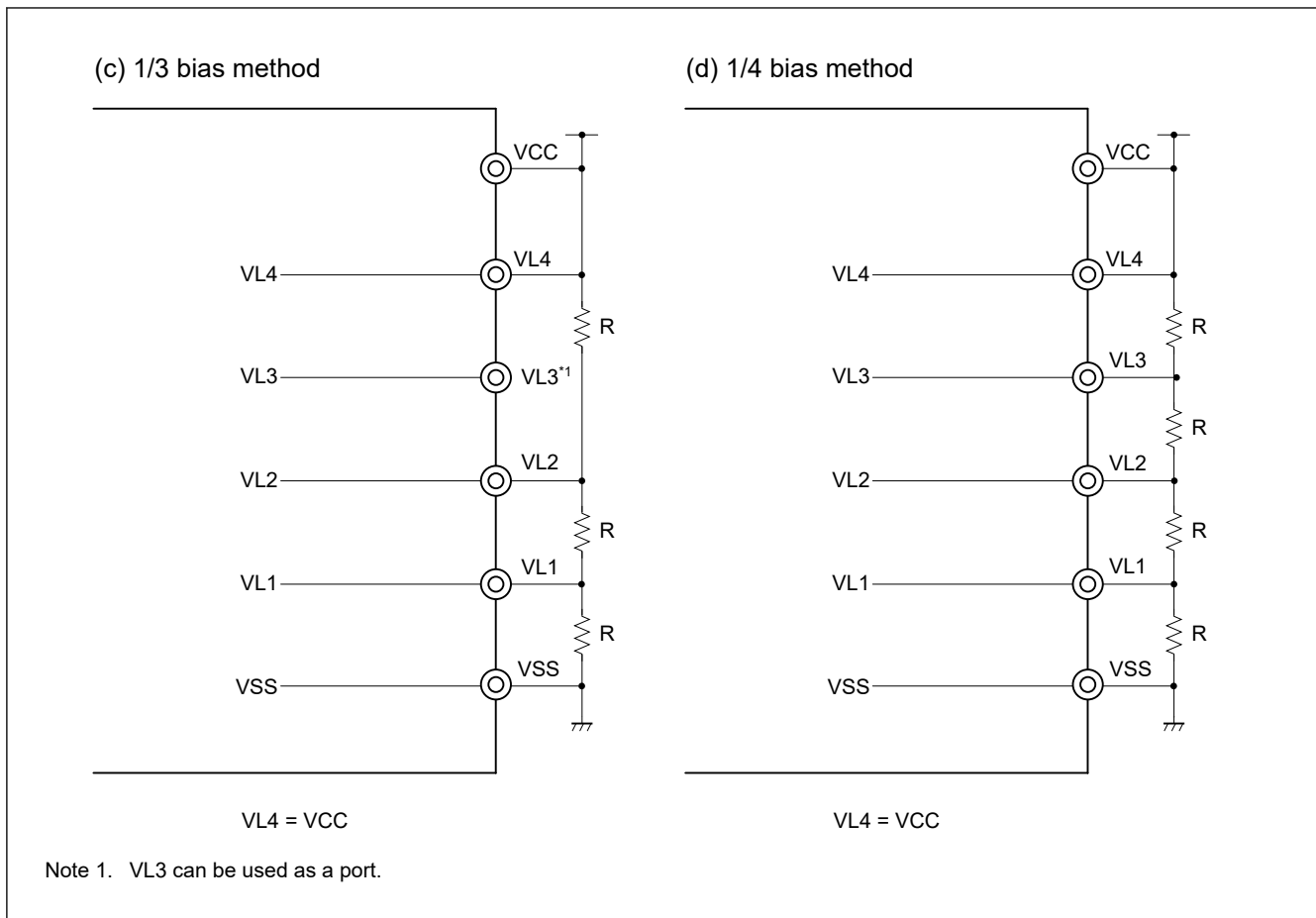
Figure 46.11 Examples of LCD drive power connections using the external resistance division method (2 of 2)
