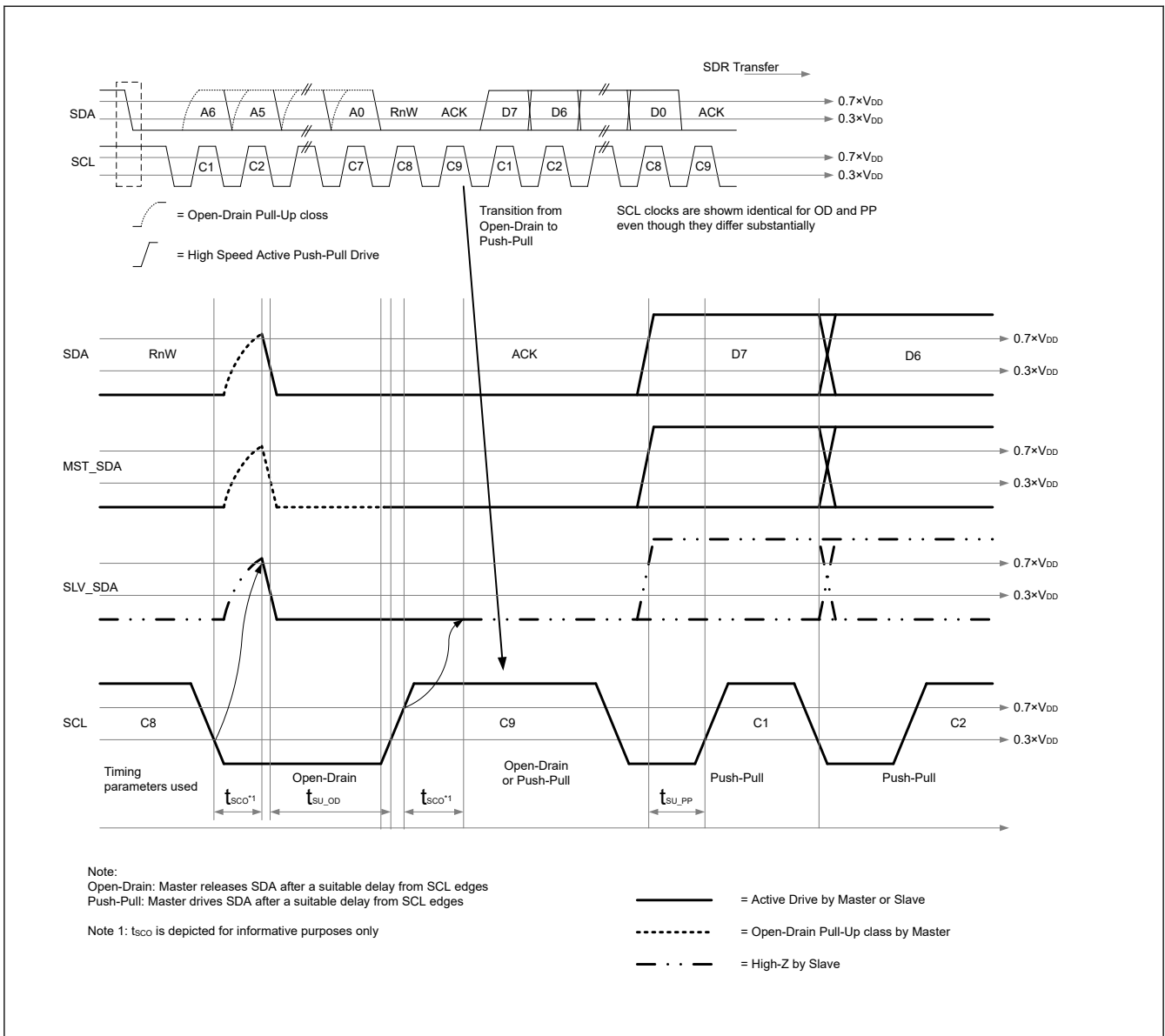
Figure 49.44 I3C data transfer – ACK by slave
