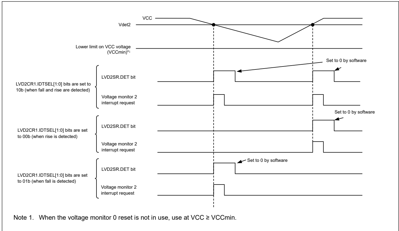
Figure 7.6 Example of voltage monitor 2 interrupt operation
