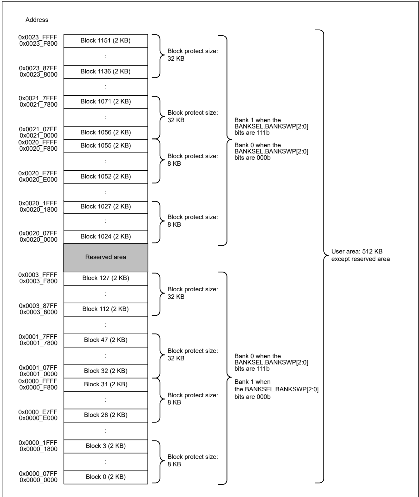
Figure 45.3 Map of the code flash memory in dual mode
