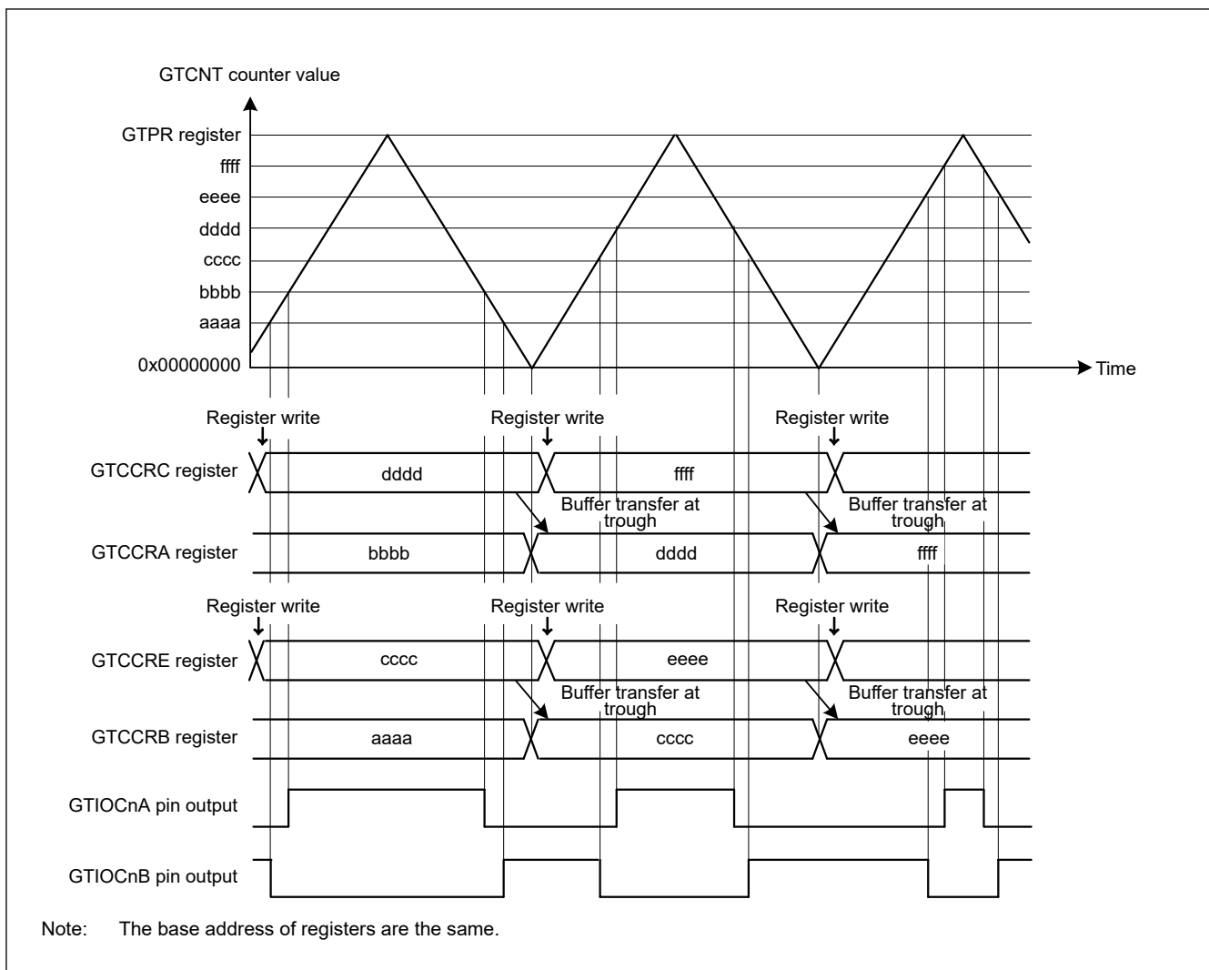
Figure 20.21 Example of triangle-wave PWM mode 1 operation with buffer operation, low output from the GTIOcNA pin and high output from the GTIOcNB pin at count start, output toggled at GTCCRA/ GTCCRB register compare match, and output retained at cycle end
