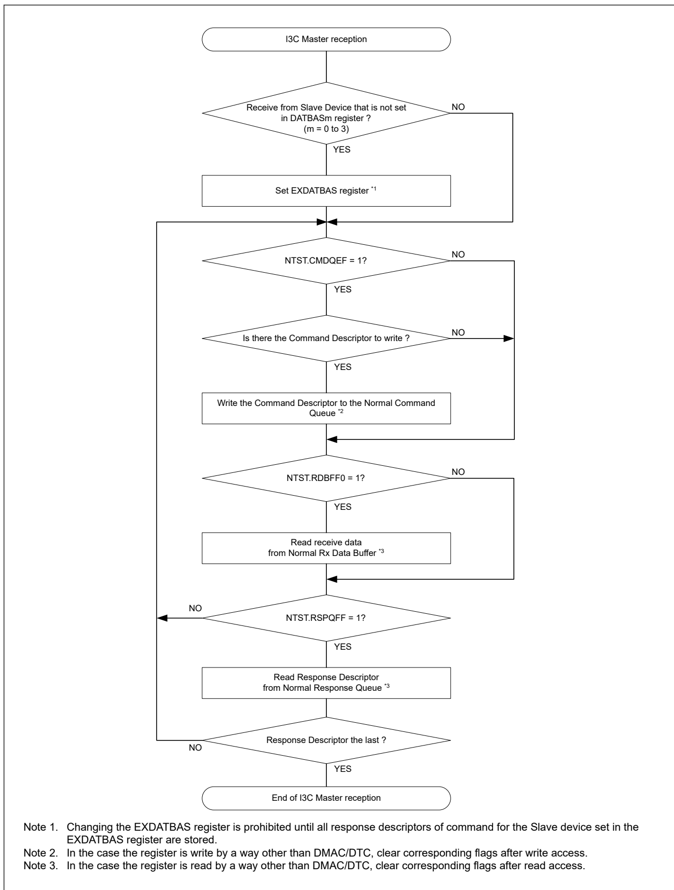
Figure 29.145 Example of I3C master reception flowchart (normal FIFO buffer transfer)
