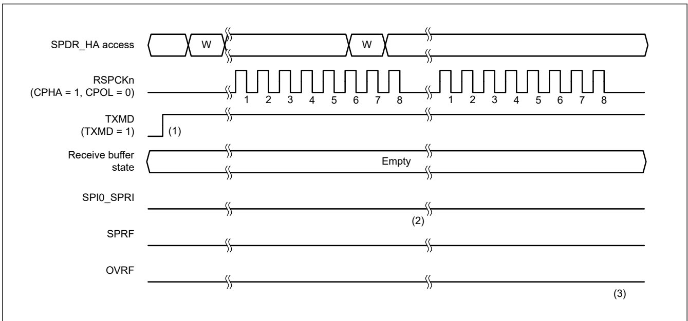
Figure 33.27 Operation example when SPCR3.ETXMD = 0 and SPCR.TXMD = 1
