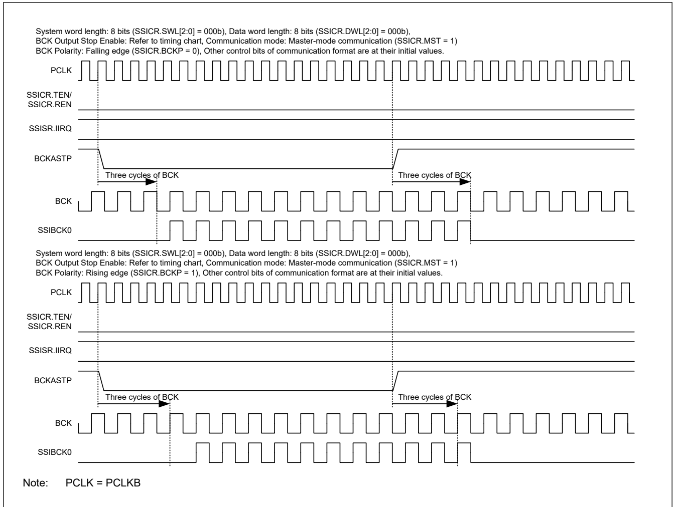
Figure 35.33 Example operation of the BCKASTP bit (idle state)
