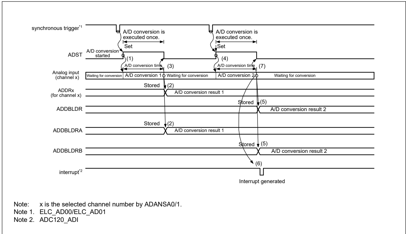
Figure 38.11 Example extended operation in double trigger mode with duplication selected for the analog input (channel x) and ELC_AD00/ELC_AD01
