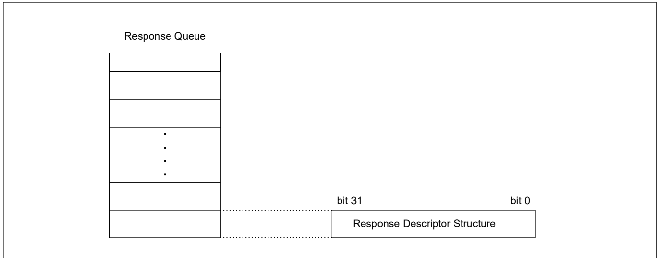
Figure 29.5 Receive status descriptor data structure
