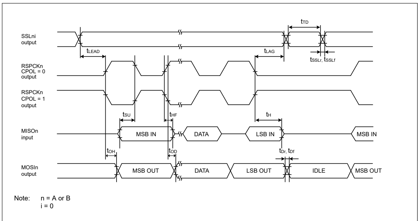
Figure 49.35 SPI timing (master, CPHA = 1) (bit rate: PCLKB division ratio is set to 1/2)
