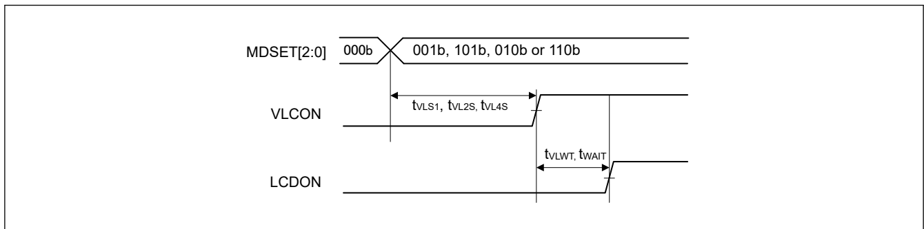
Figure 49.71 LCD reference voltage setup time, voltage boosting wait time, and capacitor split wait time
