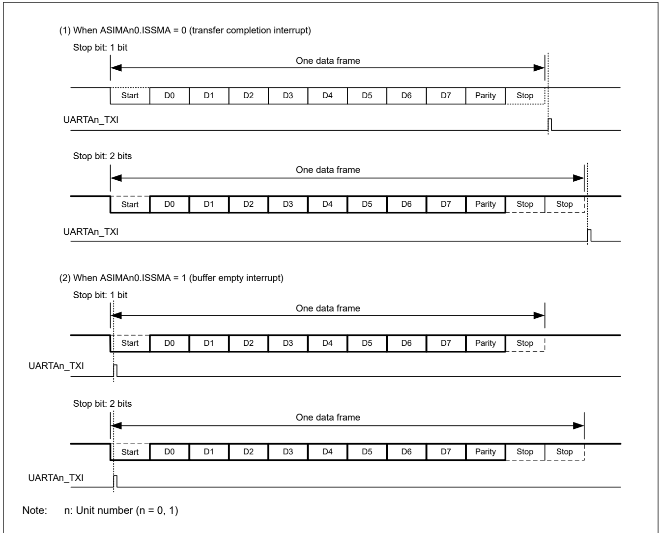
Figure 30.4 Interrupt output timing
