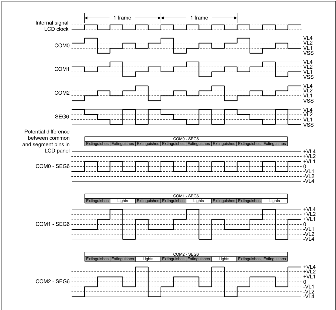
Figure 46.31 Three-time slice LCD drive waveform examples between SEG6 and each common signal using 1/3 bias method
