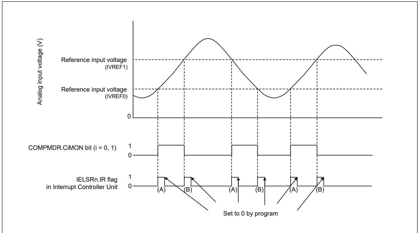
Figure 41.4 Operating example of ACMPLPi (i = 0, 1) when window function is enabled
