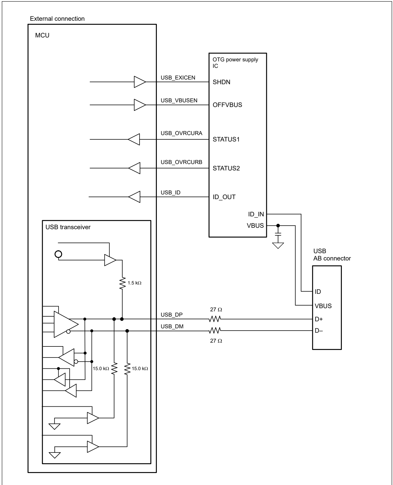
Figure 25.2 Example OTG connection in a self-powered system
