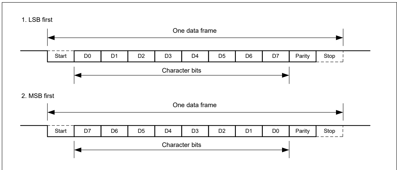
Figure 30.2 Transmit and receive data format
