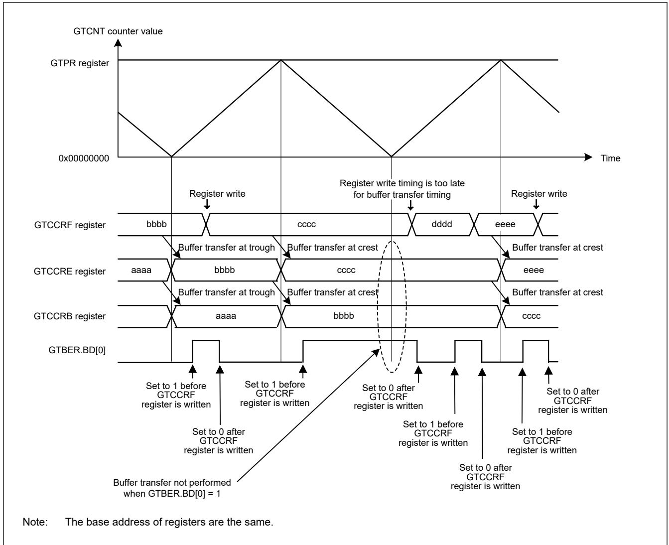
Figure 20.67 Example of operation for disabling buffer operation with triangle waves, double buffer operation, and buffer transfer at both troughs and crests
