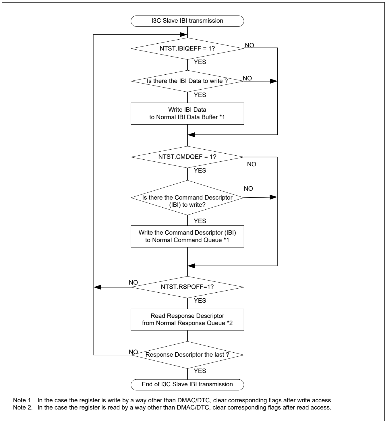
Figure 29.152 Example of I3C slave IBI transmission flowchart
