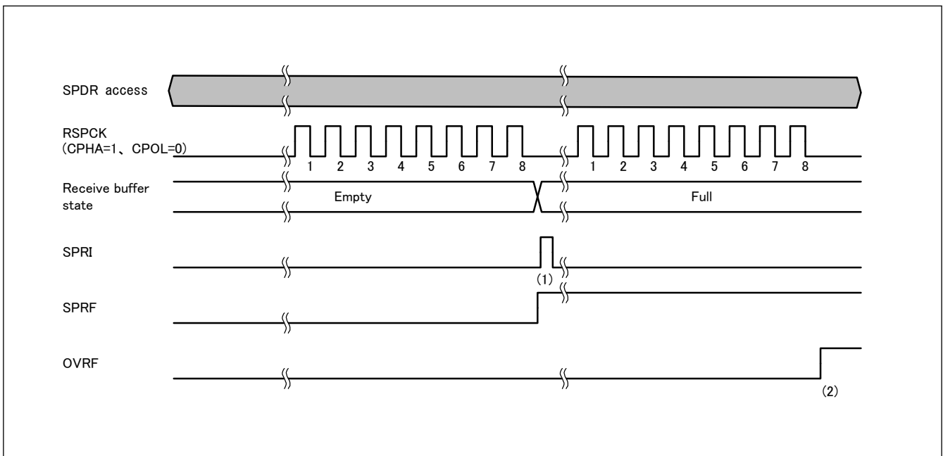
Figure 33.28 Example of Operation when MSTR = 0 and ETXMD = 1
