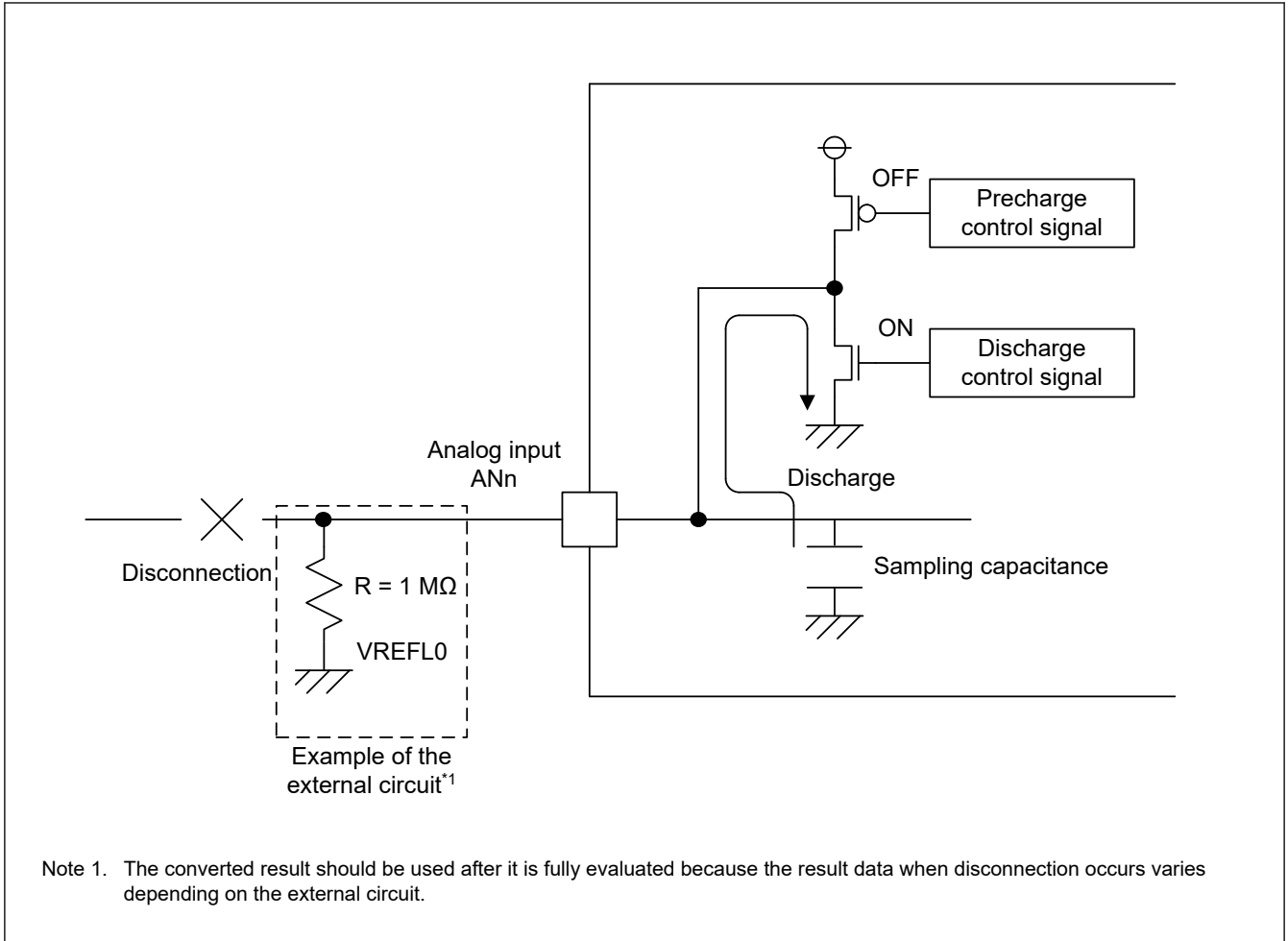
Figure 38.29 Example of disconnection detection when discharge is selected
