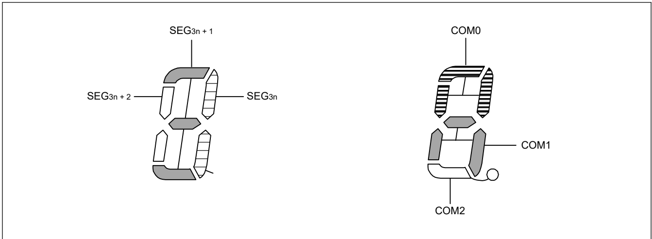
Figure 46.28 Three-time slice LCD display pattern and electrode connections
