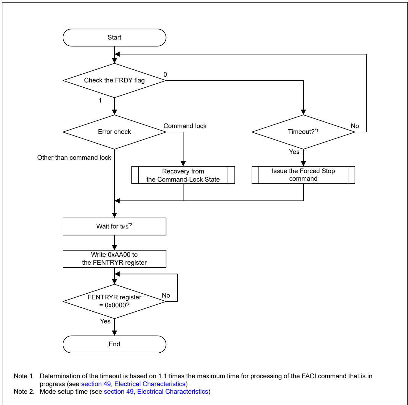
Figure 45.12 Procedure to transition to read mode
