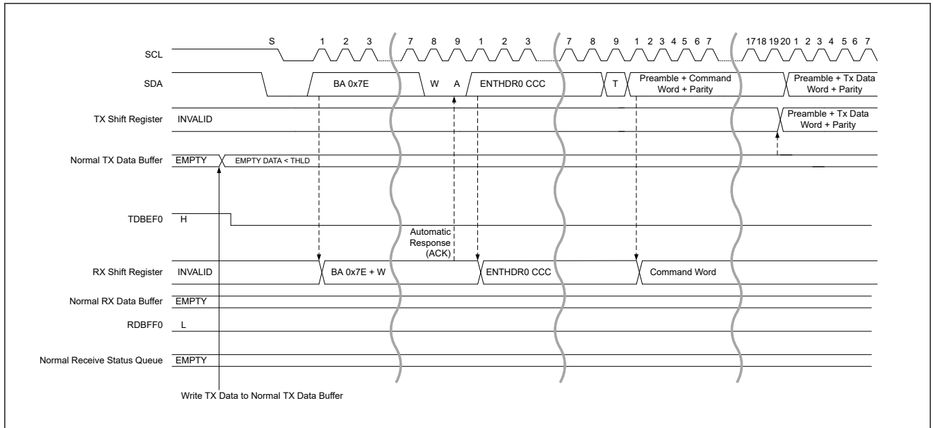
Figure 29.58 HDR data read transfer (HDR-DDR) timing (1/3)
