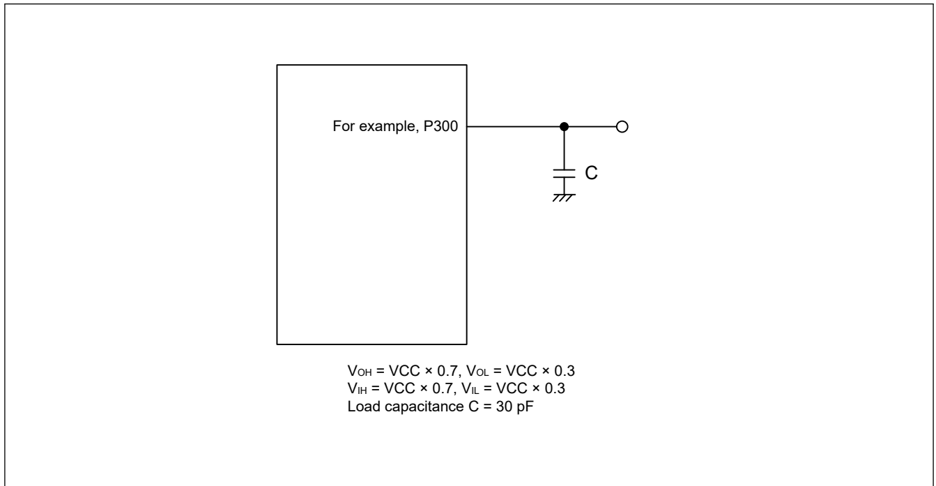
Figure 49.1 Input or output timing measurement conditions
