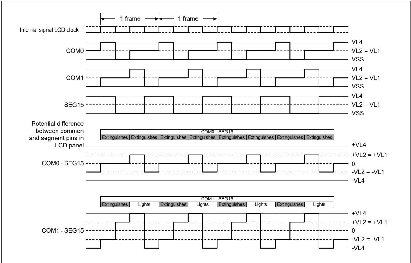
Figure 46.27 Two-time slice LCD drive waveform examples between SEG15 and each common signal using 1/2 bias method
