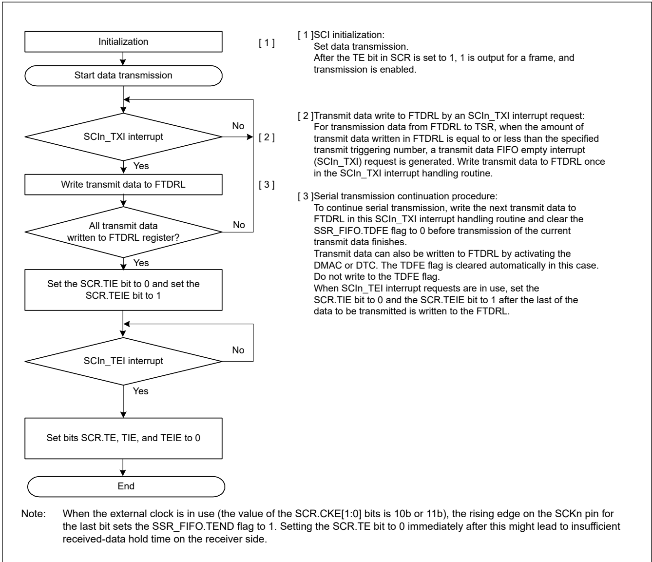
Figure 26.70 Example flow of serial transmission in clock synchronous mode with FIFO selected
