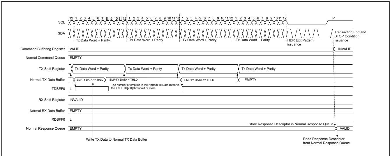
Figure 29.29 HDR data write transfer (HDR-TSP, TSL) timing (2/2)
