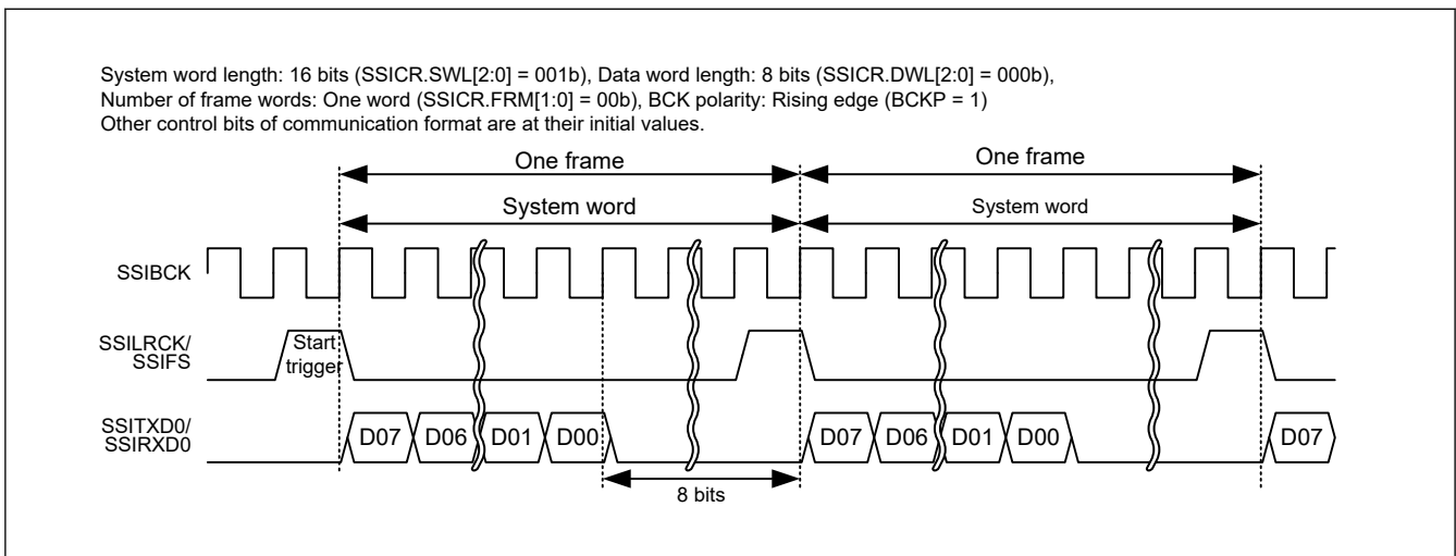
Figure 35.38 Short frame in monaural format (with padding: system word length > data word length)
