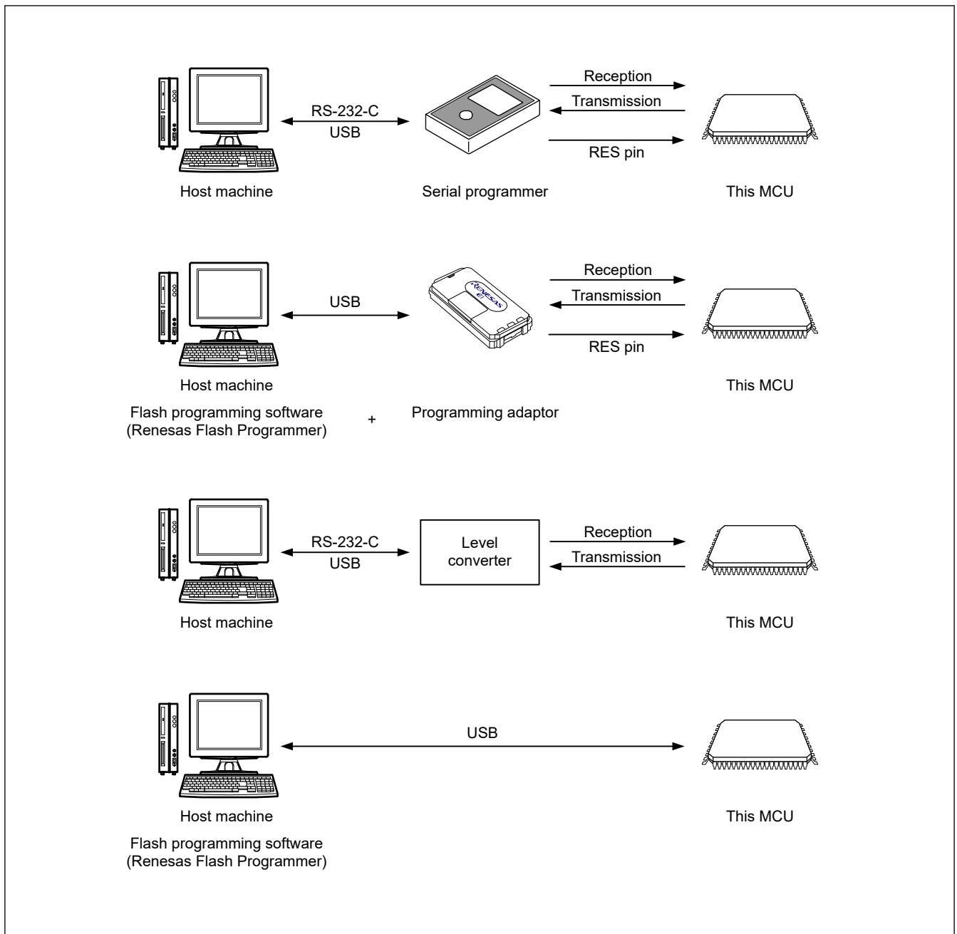
Figure 45.40 Environments for Rewriting the Flash Memory
