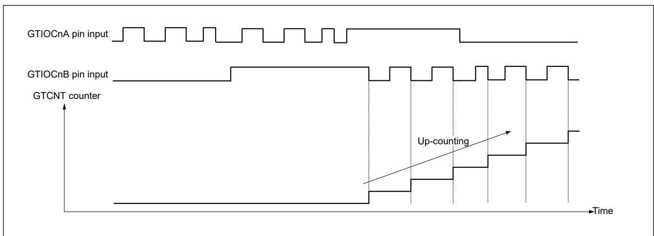
Figure 20.59 Example of phase counting mode 5 (B)
