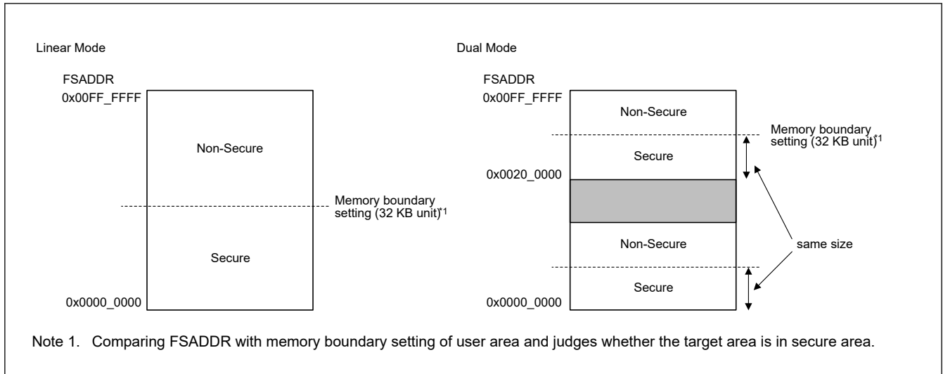
Figure 45.31 Secure/non-secure region in user area
