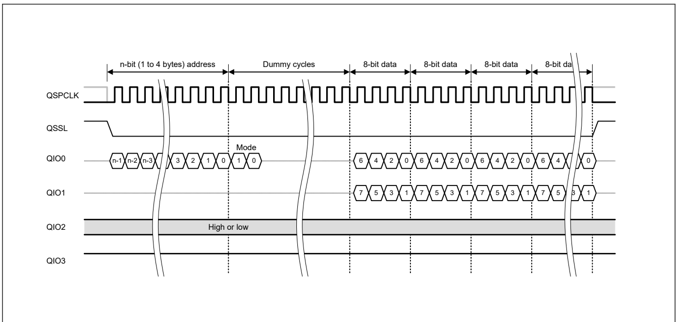
Figure 34.22 Fast Read Dual Output bus cycle in XIP mode (with extended SPI protocol)
