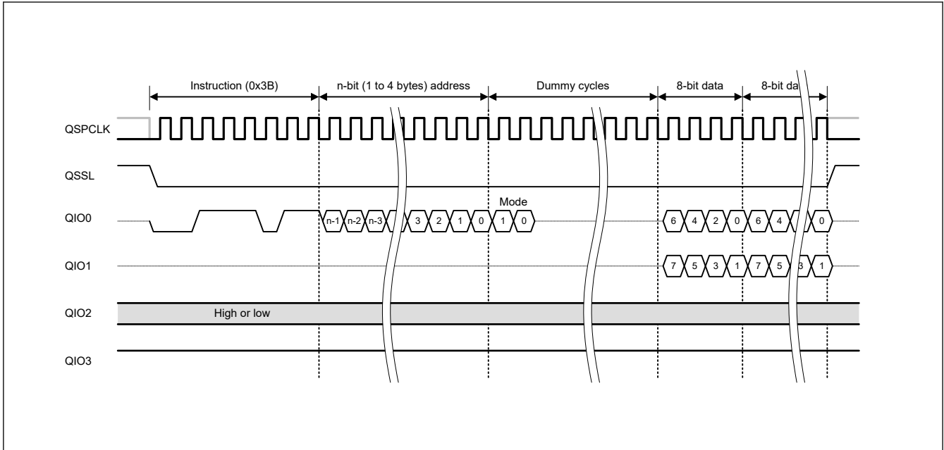
Figure 34.21 Fast Read Dual Output bus cycle (with extended SPI protocol)
