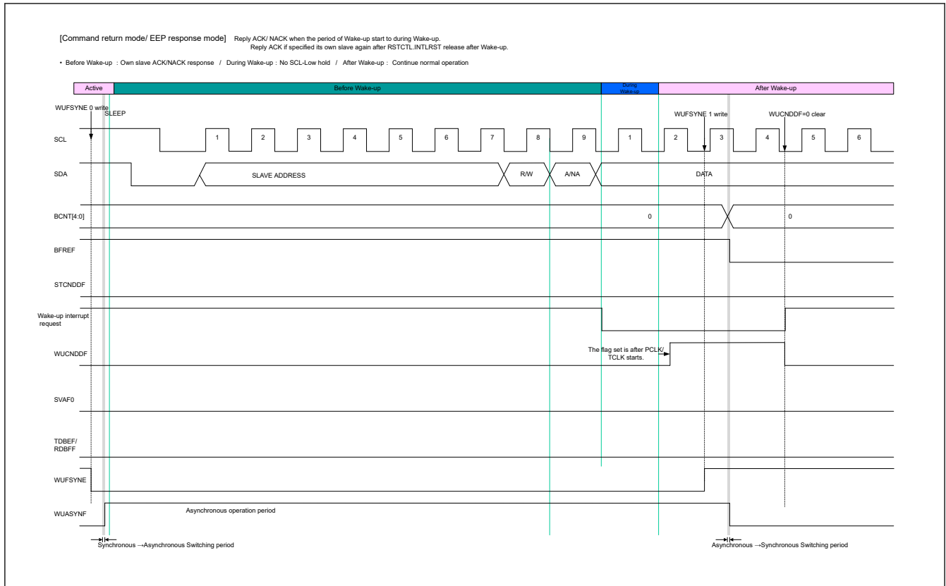
Figure 29.131 Timing of command recovery mode/EEP response mode
