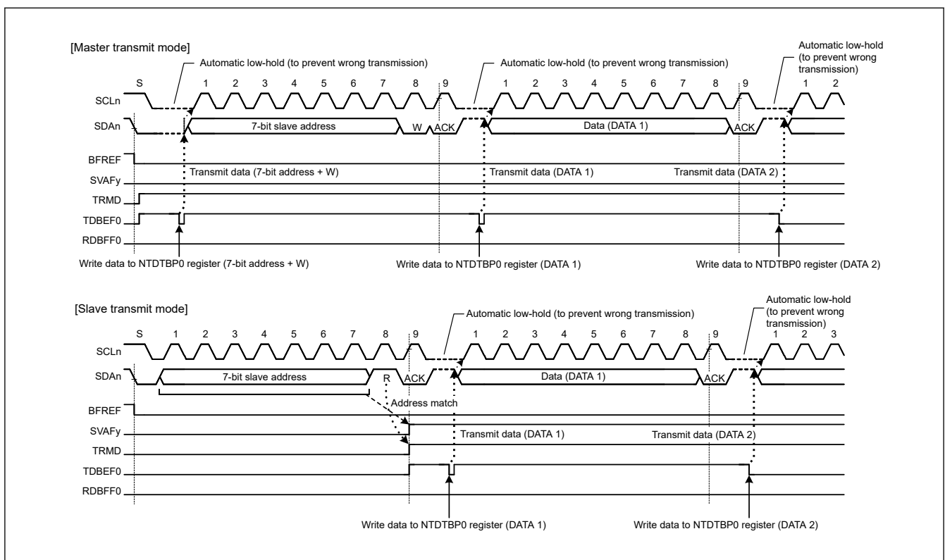
Figure 29.91 Automatic low-hold operation in transmit mode
