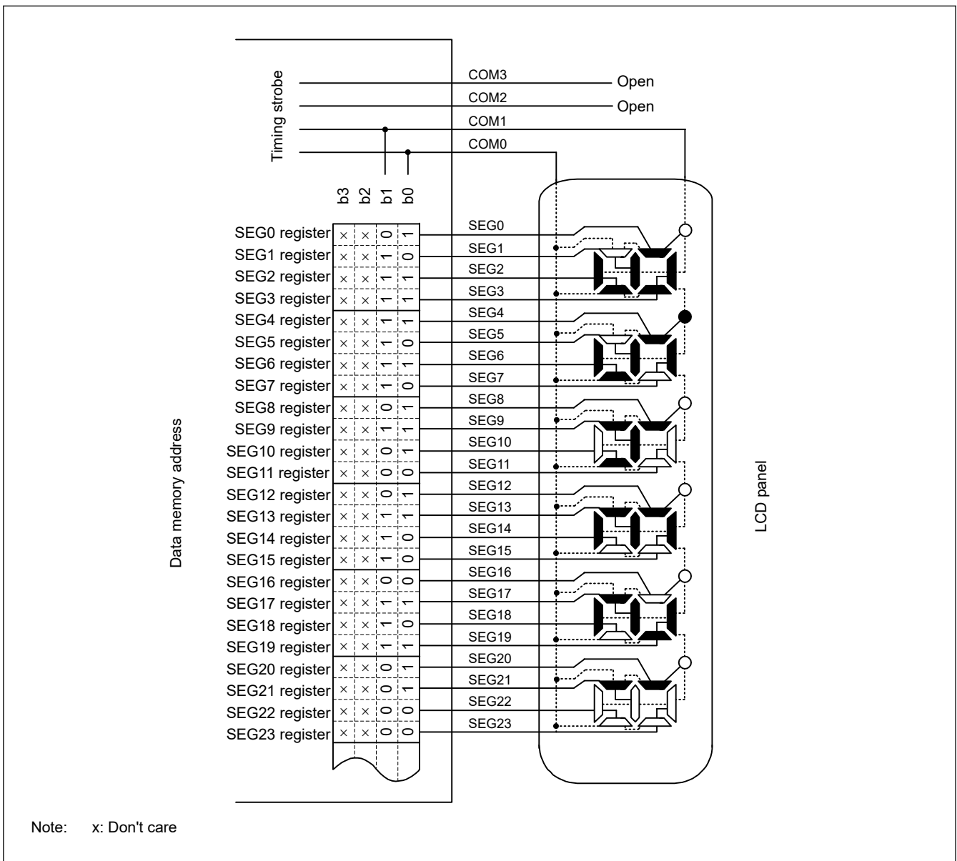
Figure 46.26 Example of connecting two-time slice LCD panel
