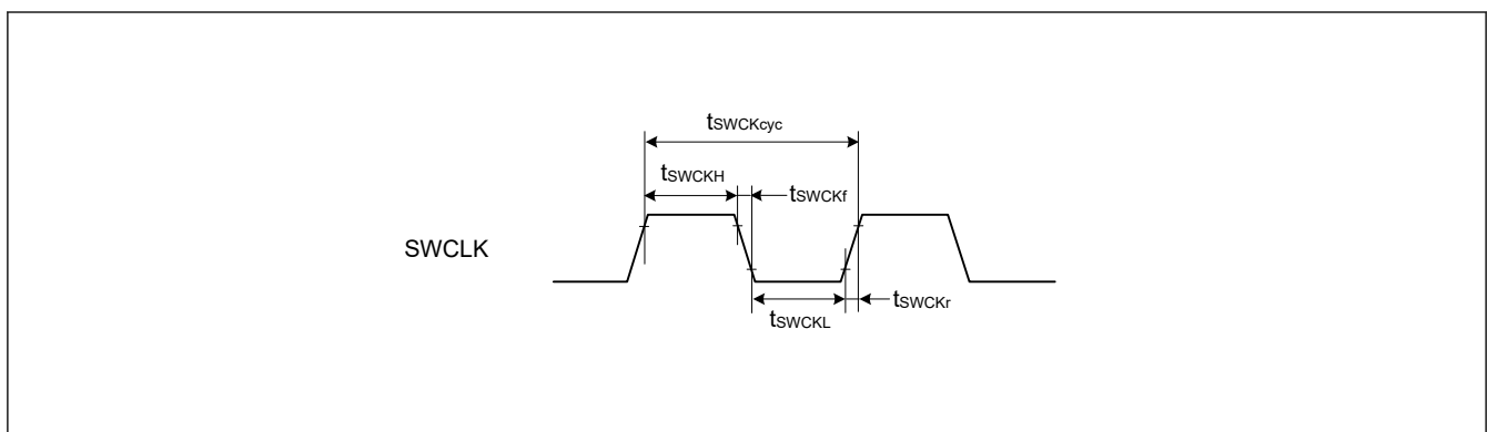
Figure 49.72 SWD SWCLK timing
