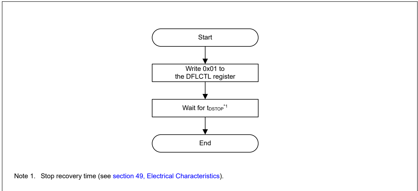
Figure 45.9 Procedure for transition to read mode from data flash disabled mode
