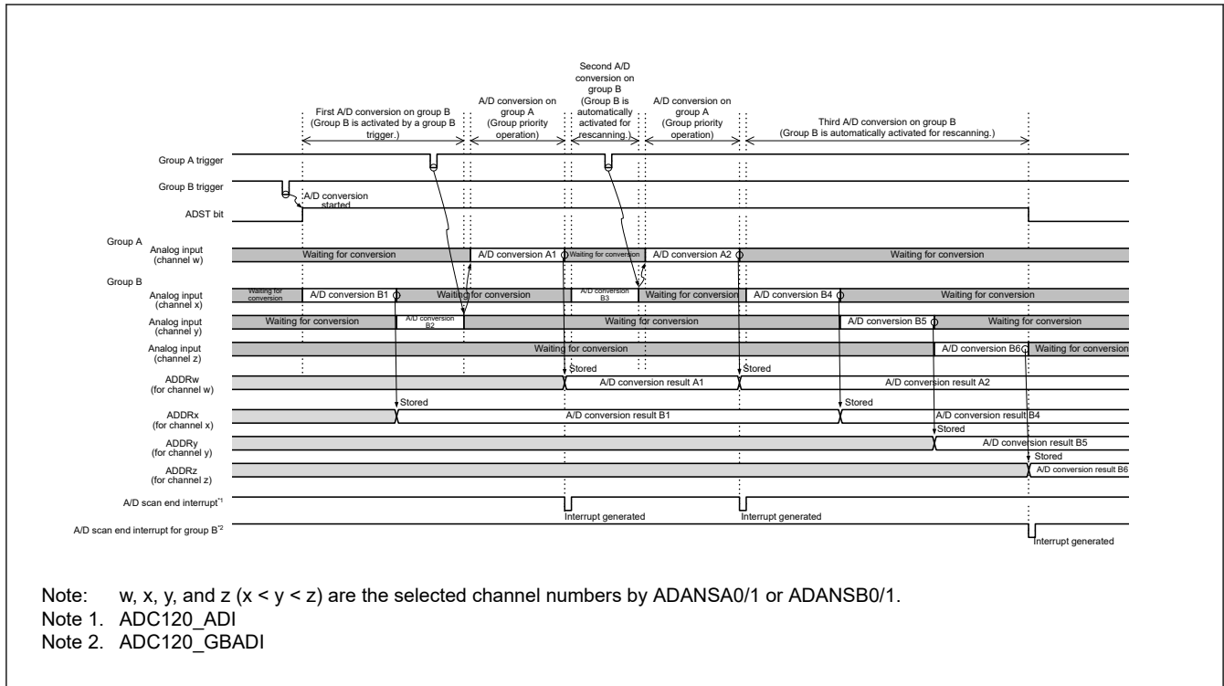
Figure 38.18 Example of group priority operation 1-2: Group A trigger input during rescanning of group B when rescanning is enabled (when ADGSPCR.GBRSCN = 1, ADGSPCR.GBRP = 0)
