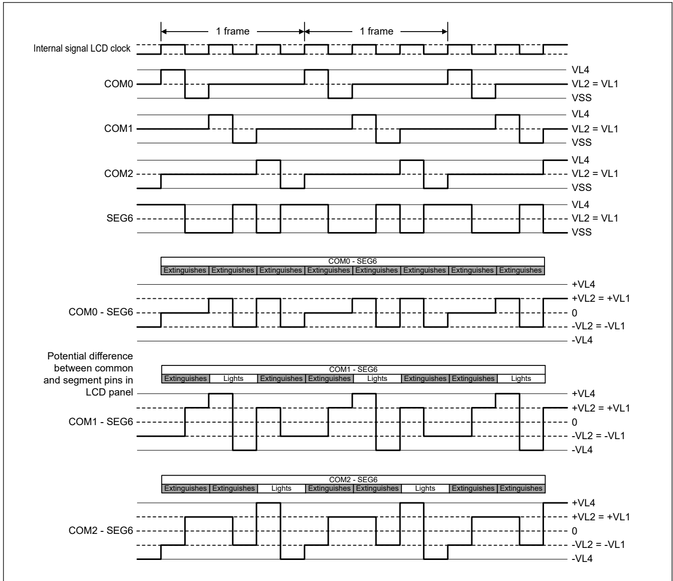
Figure 46.30 Three-time slice LCD drive waveform examples between SEG6 and each common signal using 1/2 bias method
