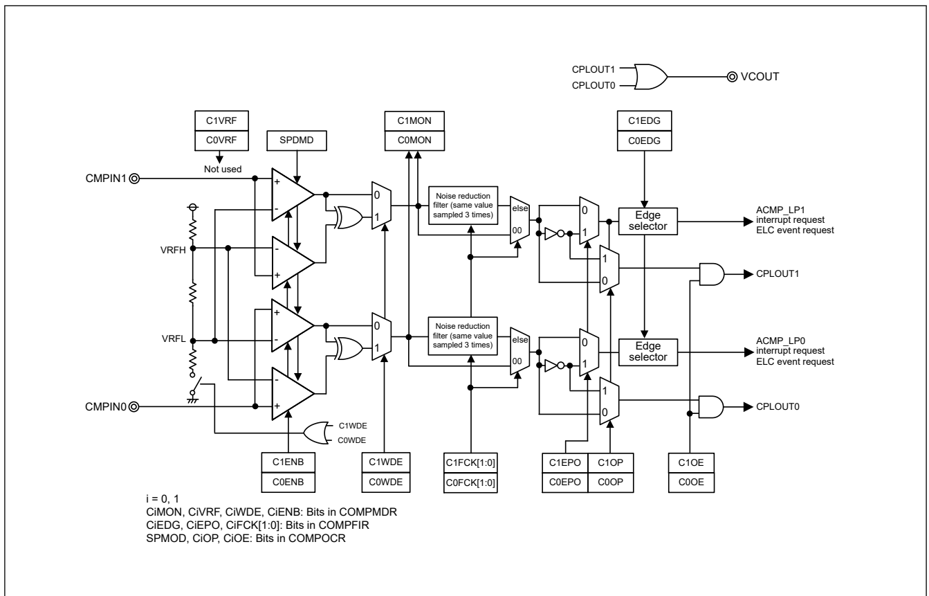
Figure 41.2 ACMPLP block diagram when window function is enabled
