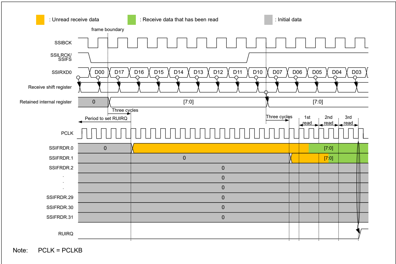
Figure 35.16 RUIRQ setting timing
