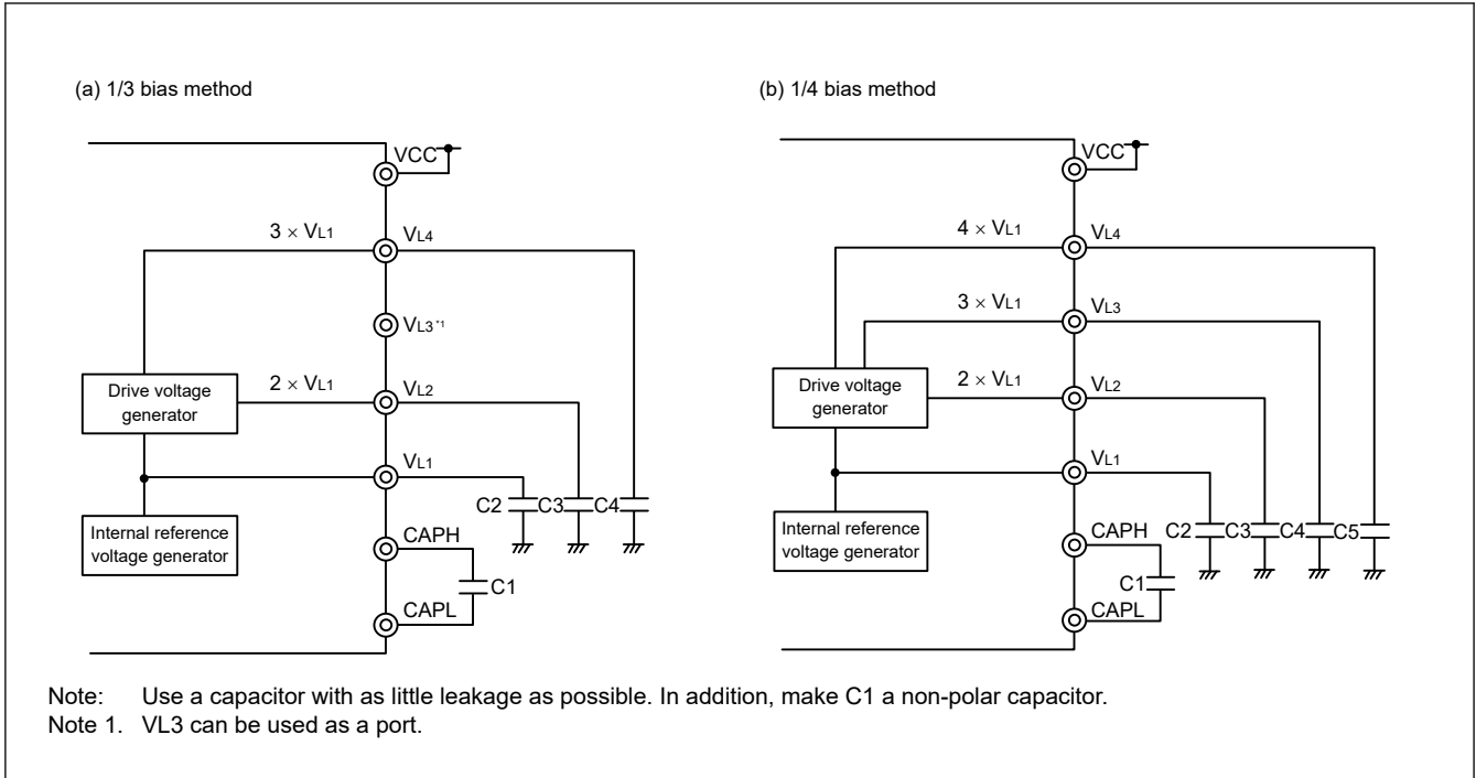
Figure 46.12 Examples of LCD drive power connections using VL1 reference mode of internal voltage boosting method
