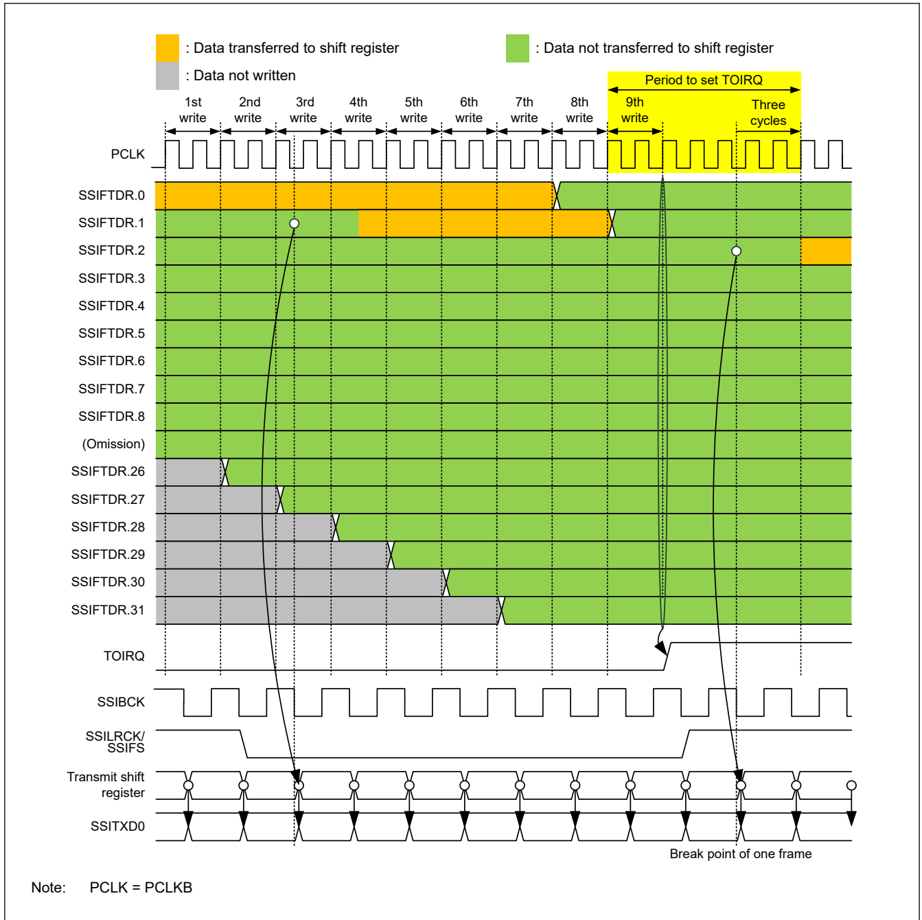
Figure 35.17 TOIRQ setting timing
