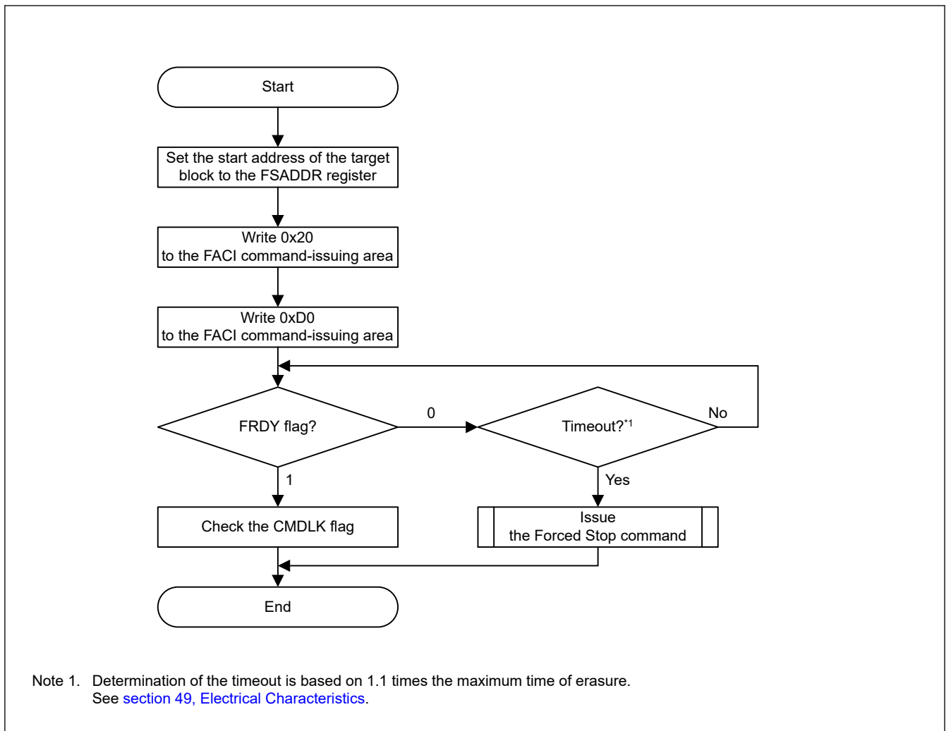
Figure 45.15 Usage flow of the Block Erase command
