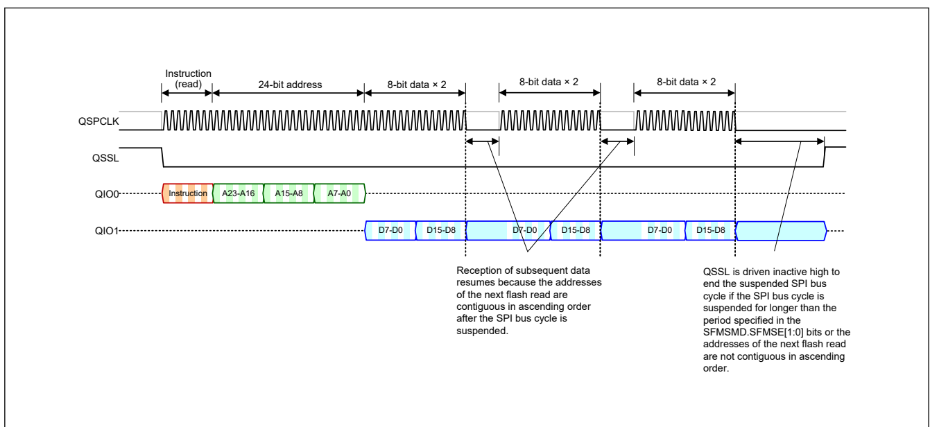
Figure 34.34 Successive data read operations using the SPI bus cycle extension
