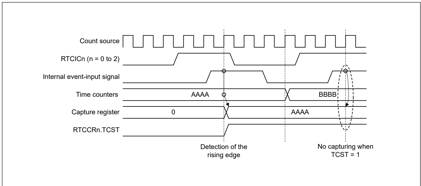
Figure 22.8 Timing of a time capture operation with the noise filter off
