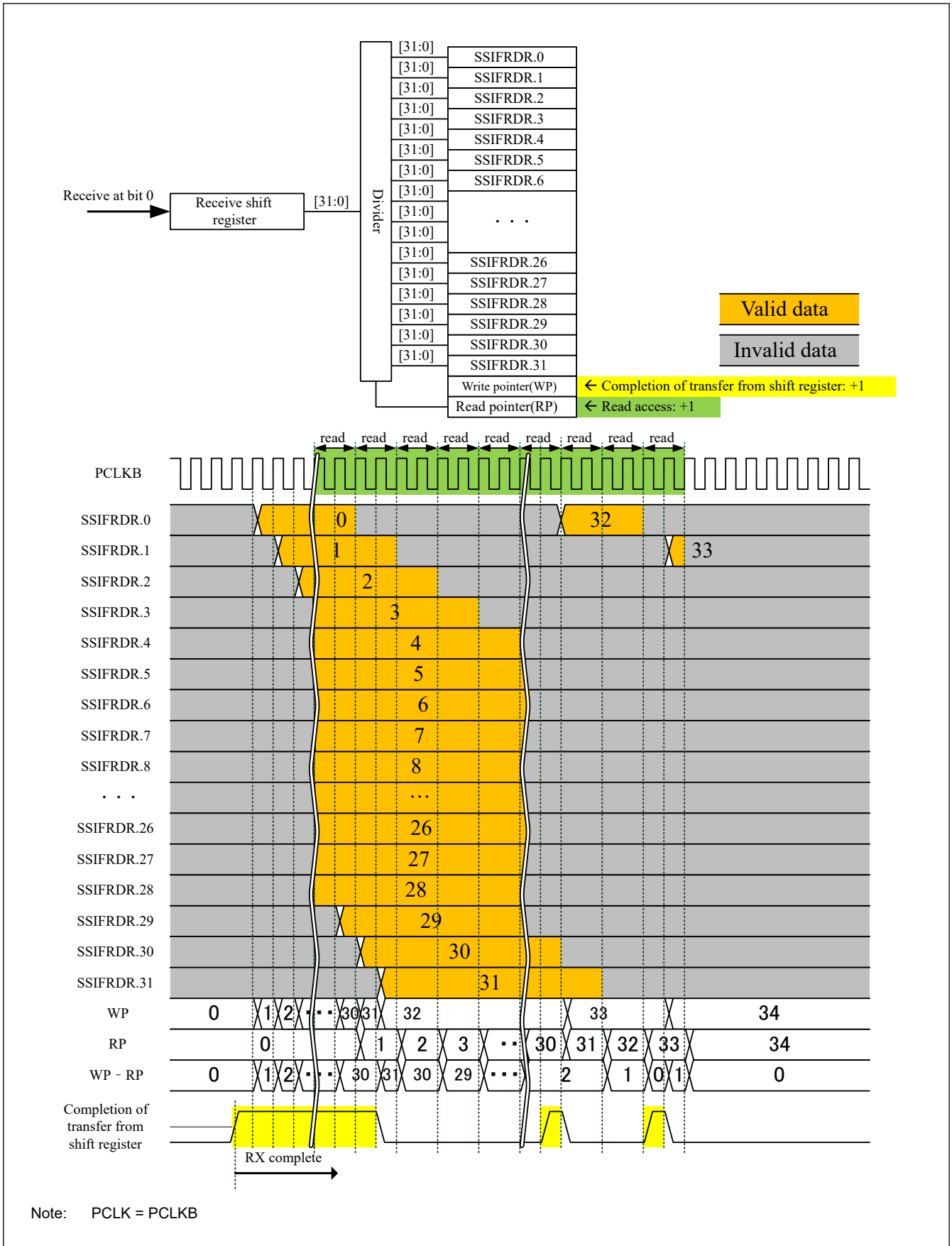
Figure 35.31 Configuration of the receive FIFO data register and receive shift register, and FIFO operation example
