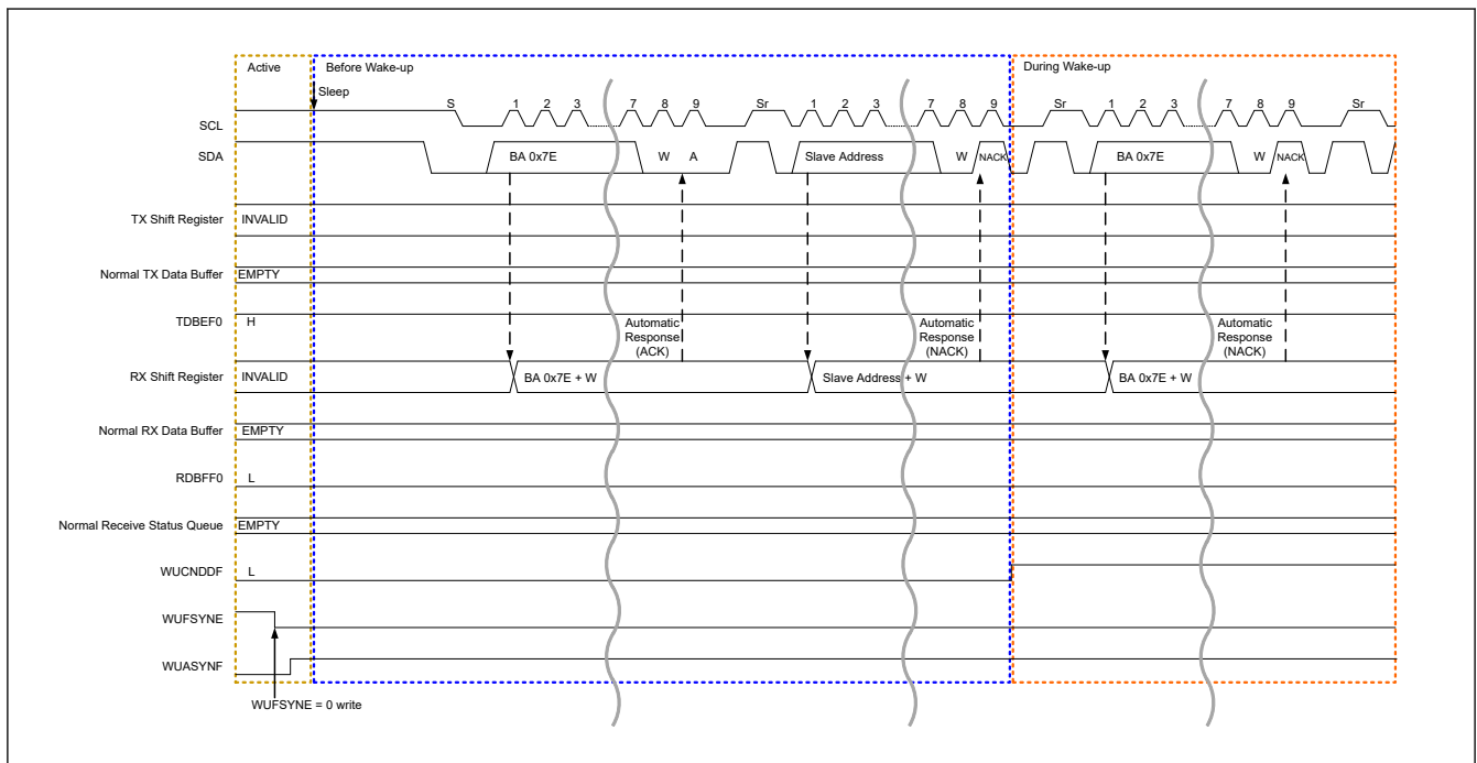
Figure 29.133 I3C slave Wake-up operation (1/2)
