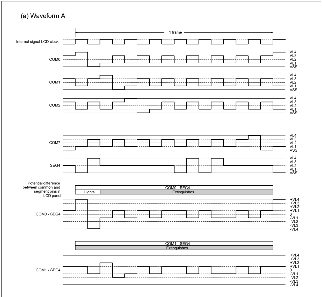
Figure 46.42 Eight-time slice LCD drive waveform examples between SEG4 and each common signal using 1/4 bias method (1 of 2)
