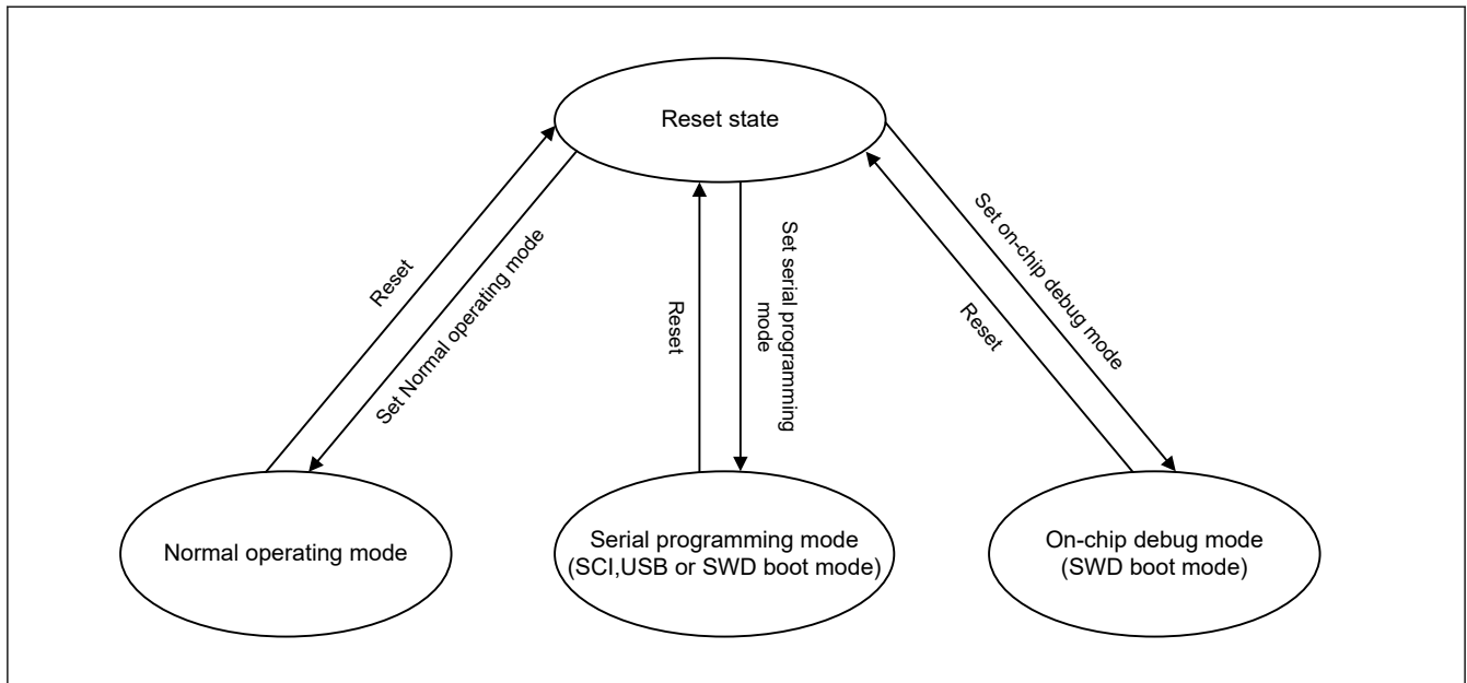
Figure 45.5 Mode transitions associated with flash memory
