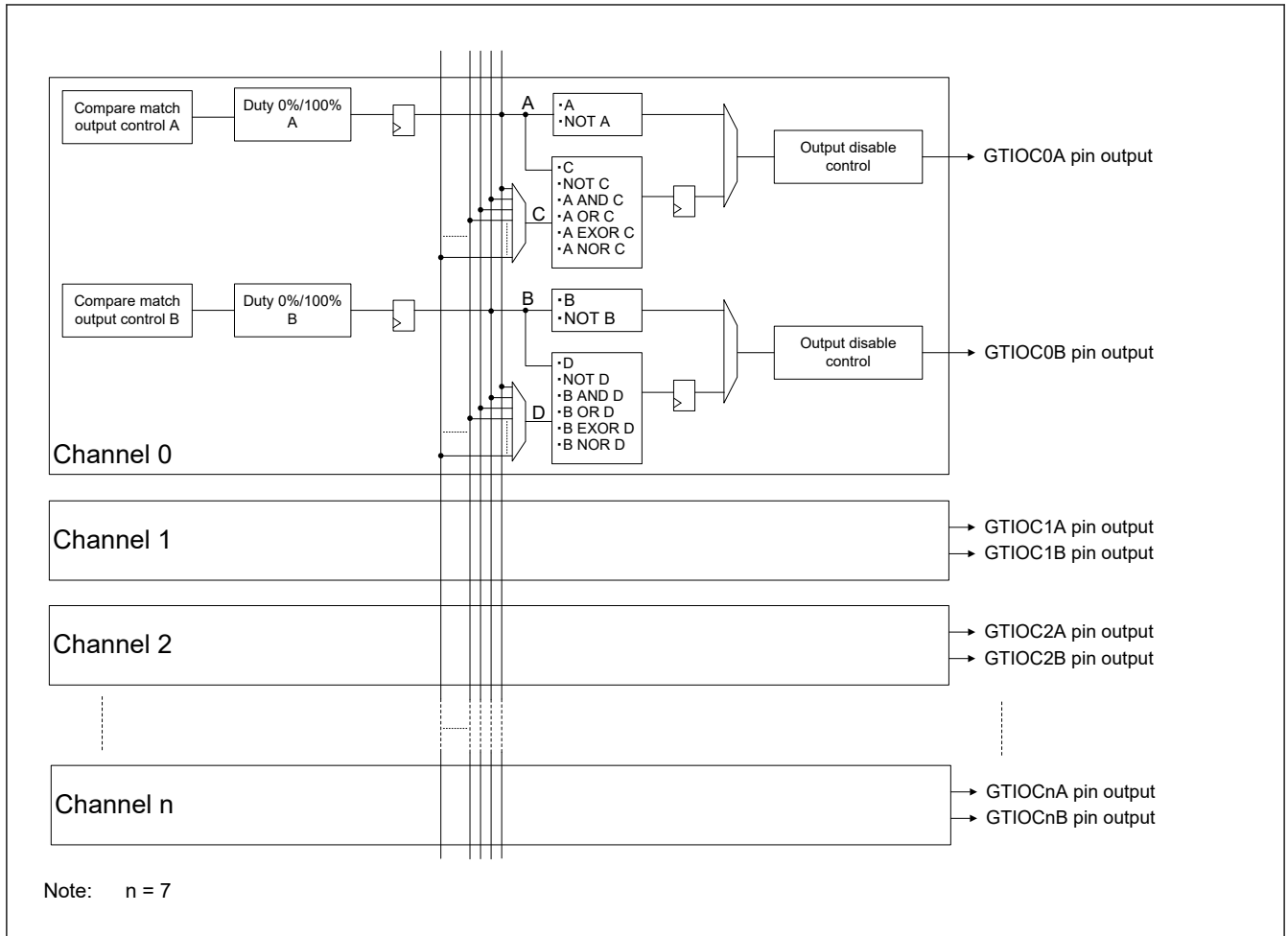
Figure 20.64 Block diagram of inter channel logical operation
