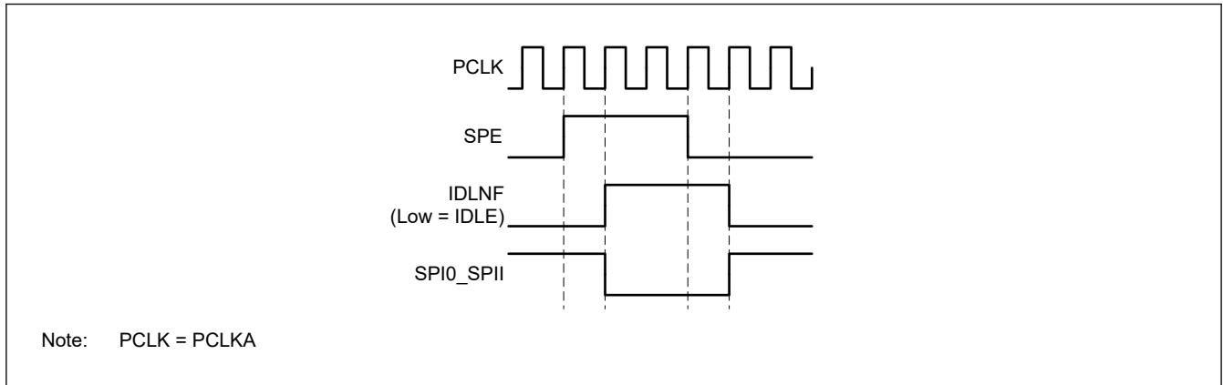
Figure 33.32 Example of idle interrupt operation (slave mode)
