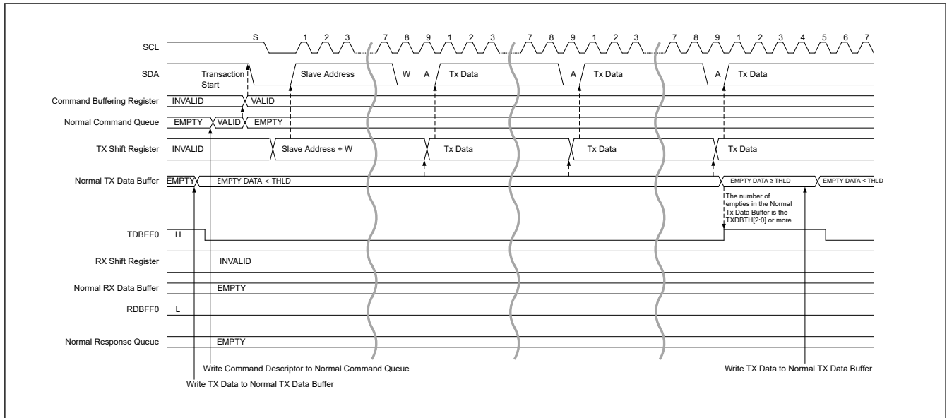
Figure 33.18 Legacy I2C message data write timing (1/2)
