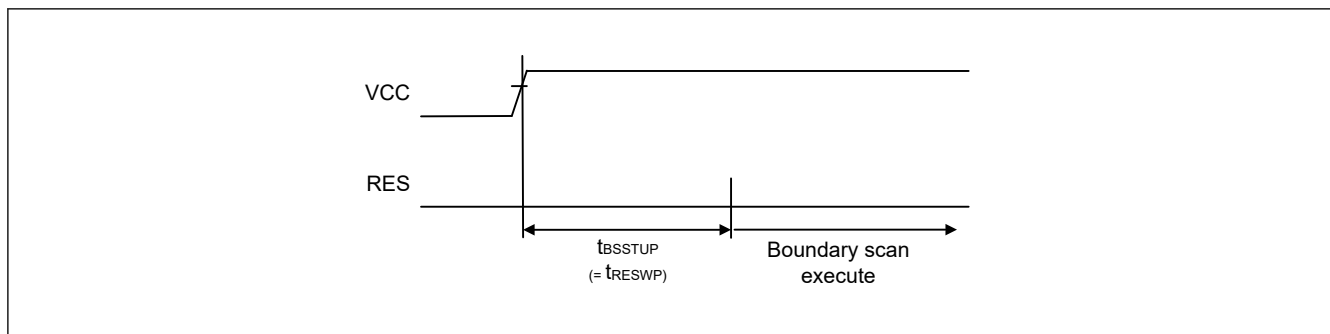
Figure 55.127 Boundary scan circuit startup timing
