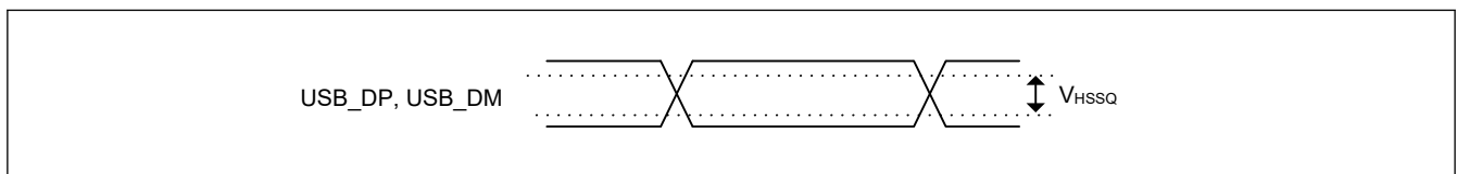
Figure 55.112 USB_DP and USB_DM squelch detect sensitivity (high-speed)
