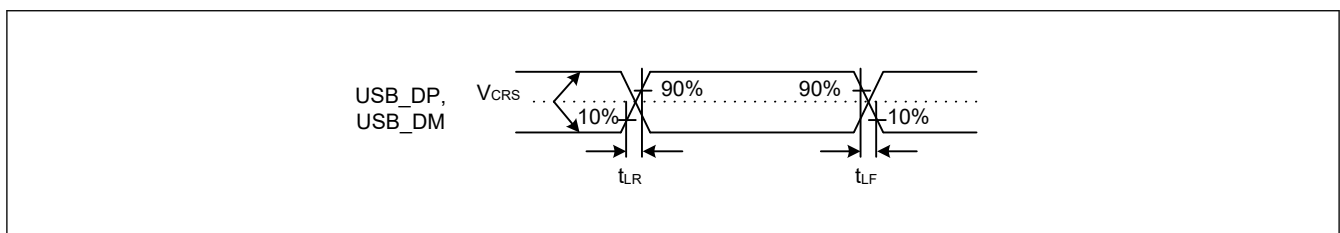
Figure 55.108 USB_DP and USB_DM output timing in low-speed mode
