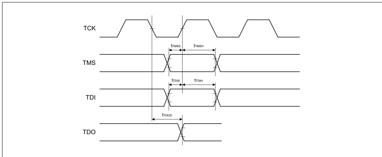
Figure 55.125 Boundary scan input/output timing (1)
