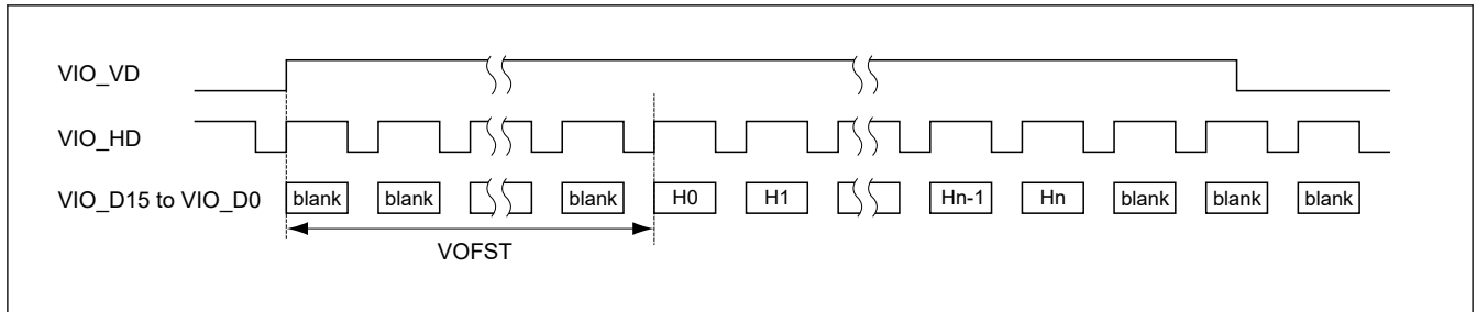
Figure 53.17 Vertical offset
