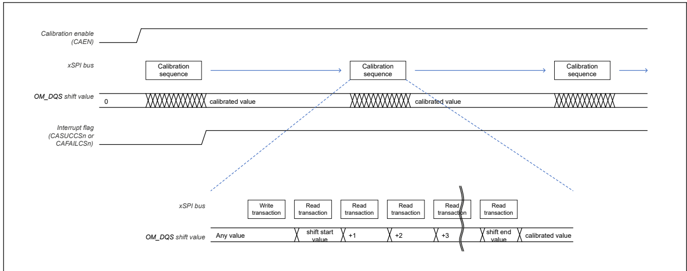
Figure 37.11 Automatic calibration
