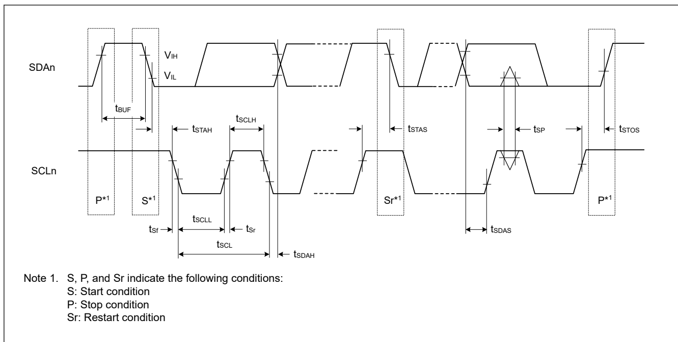
Figure 55.71 I 2 C bus interface input/output timing
