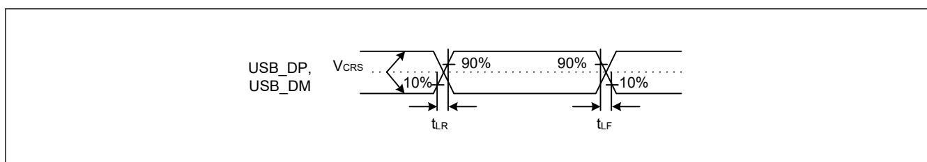
Figure 55.104 USB_DP and USB_DM output timing in low-speed mode
