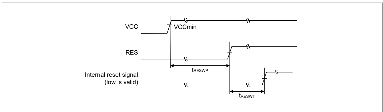
Figure 55.22 RES pin input timing under the condition that VCC exceeds V POR voltage threshold
