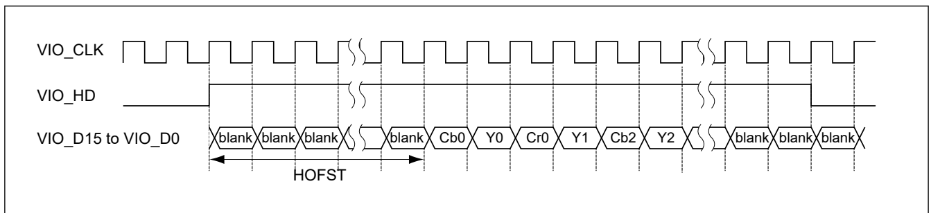
Figure 53.19 Horizontal offset
