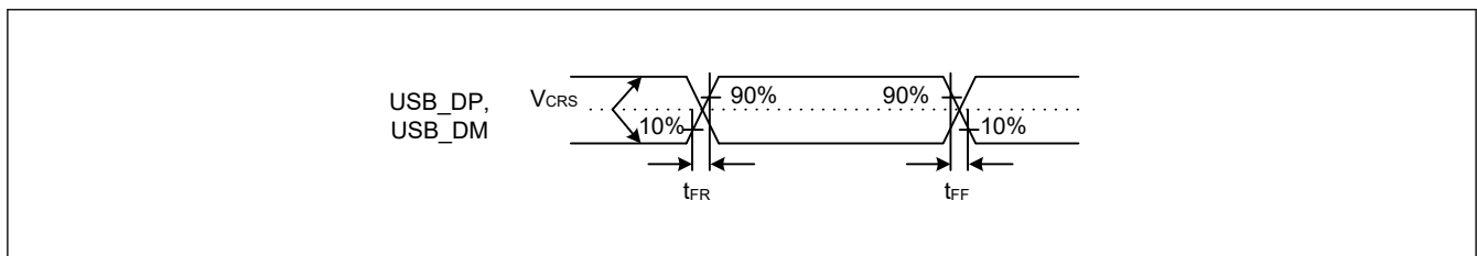
Figure 55.110 USB_DP and USB_DM output timing in full-speed mode
