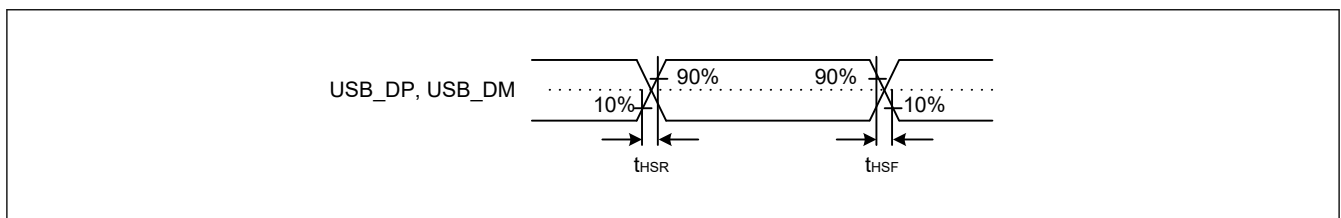
Figure 55.114 USB_DP and USB_DM output timing (high-speed)
