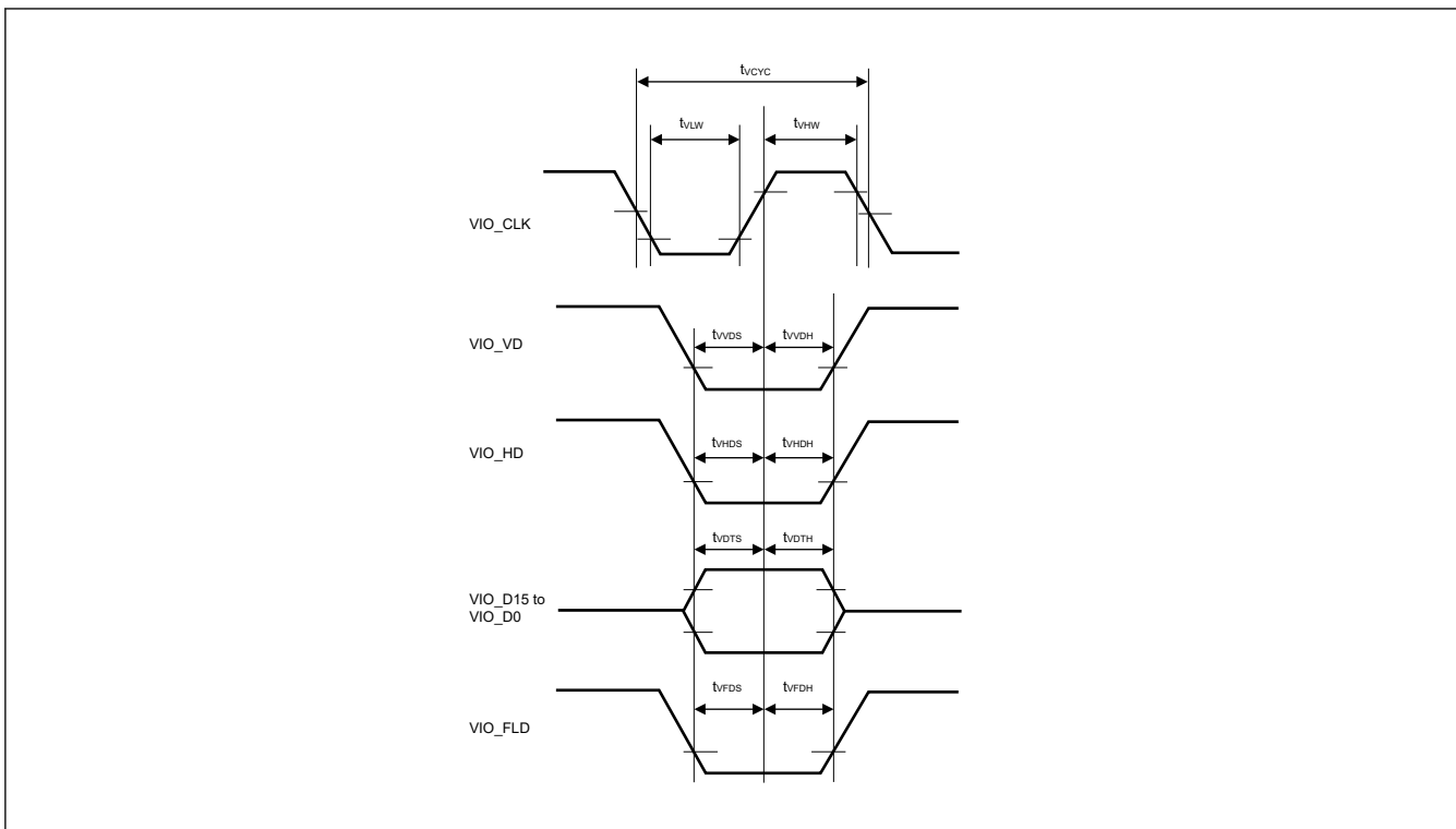
Figure 55.101 Capture Engine Unit Module Signal Timing of data capturing on the rising edge of VIO_CLK
