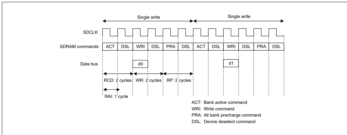
Figure 14.59 Example timing for single write (3)
