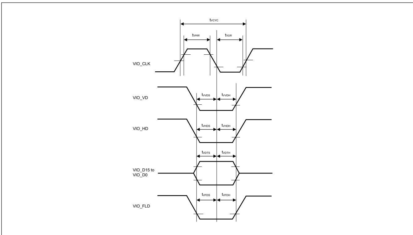
Figure 55.102 Capture Engine Unit Module Signal Timing of data capturing on the falling edge of VIO_CLK
