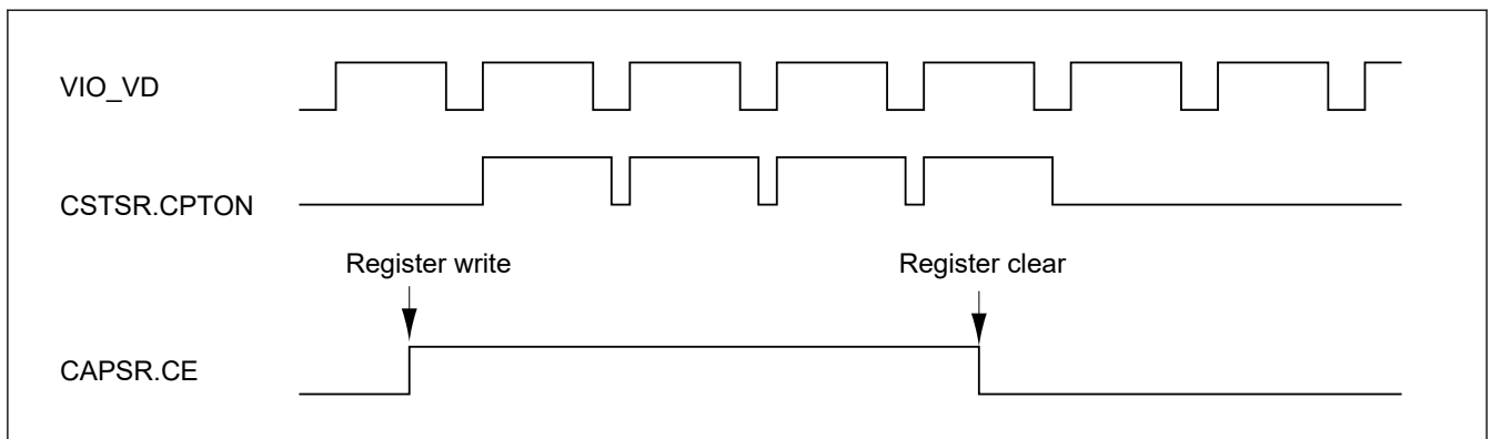
Figure 53.8 Continuous-frame capture
