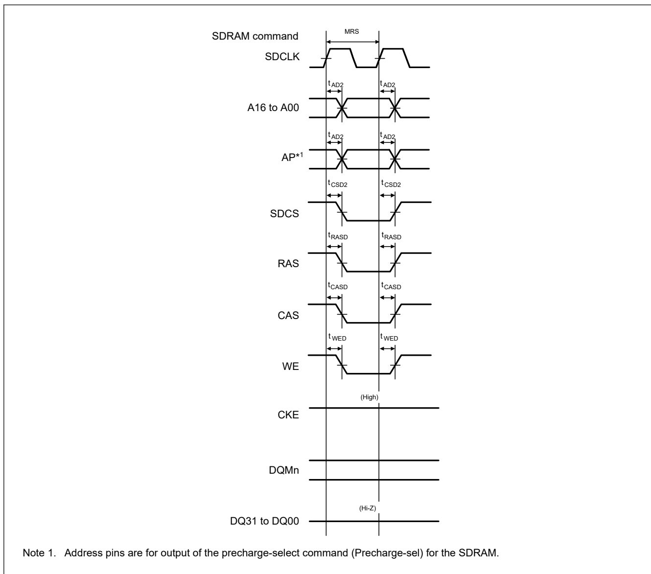
Figure 55.40 SDRAM mode register set timing
