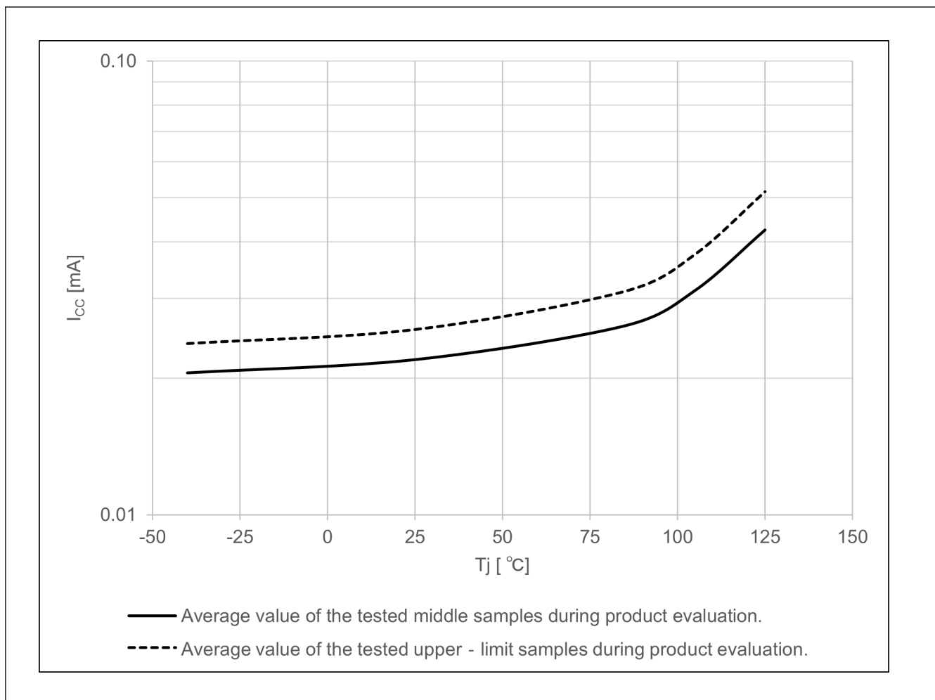
Figure 55.3 Temperature dependency in Software Standby mode ( I_{CC} ) (reference data)
