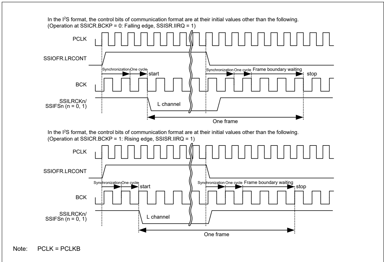
Figure 39.44 Example of disabling LR clock/frame synchronization continuation by SSIIOFR.LRCONT
