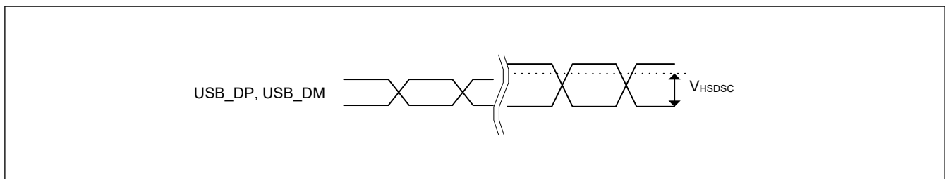
Figure 55.113 USB_DP and USB_DM disconnect detect sensitivity (high-speed)
