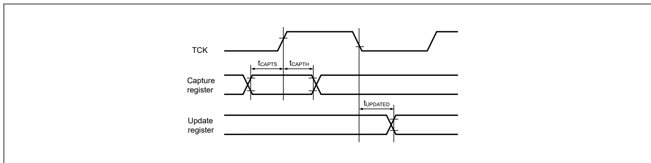
Figure 55.126 Boundary scan input/output timing (2)
