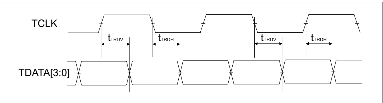
Figure 55.133 ETM output timing
