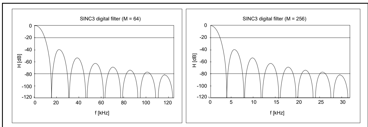
Figure 33.18 Frequency response of the SINC3 filter
