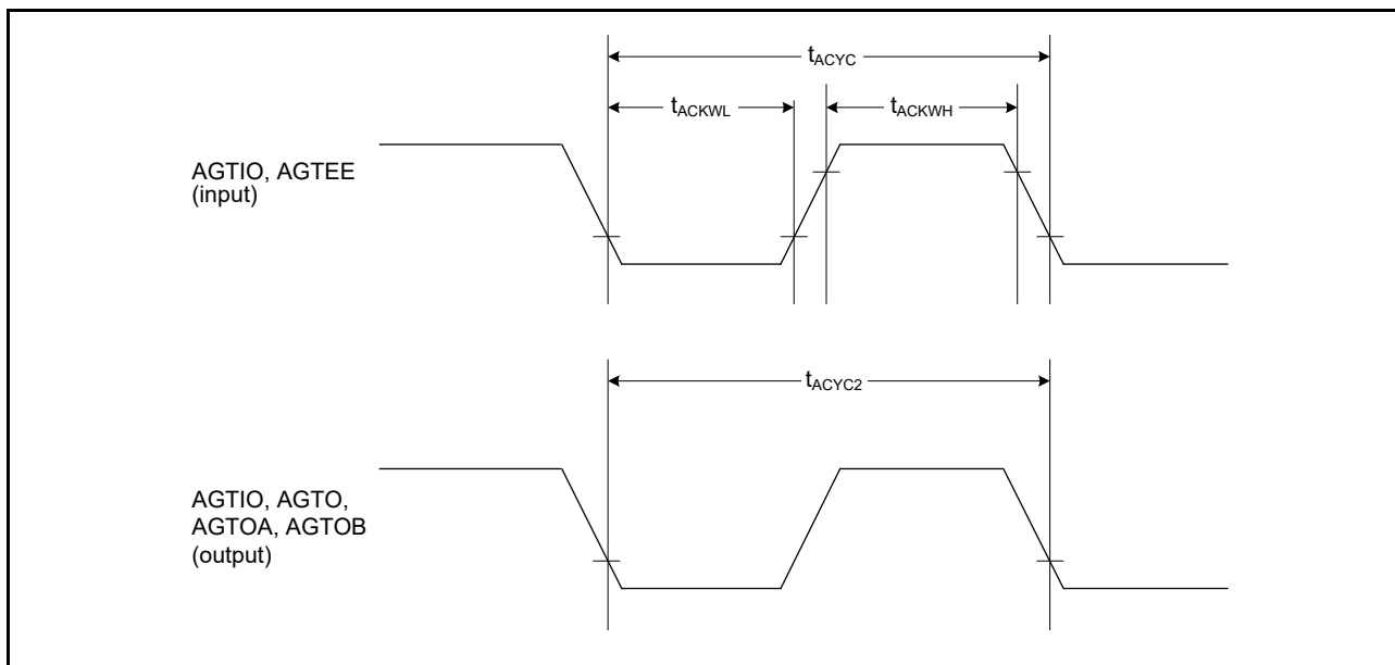
Figure 47.39 AGT I/O timing
