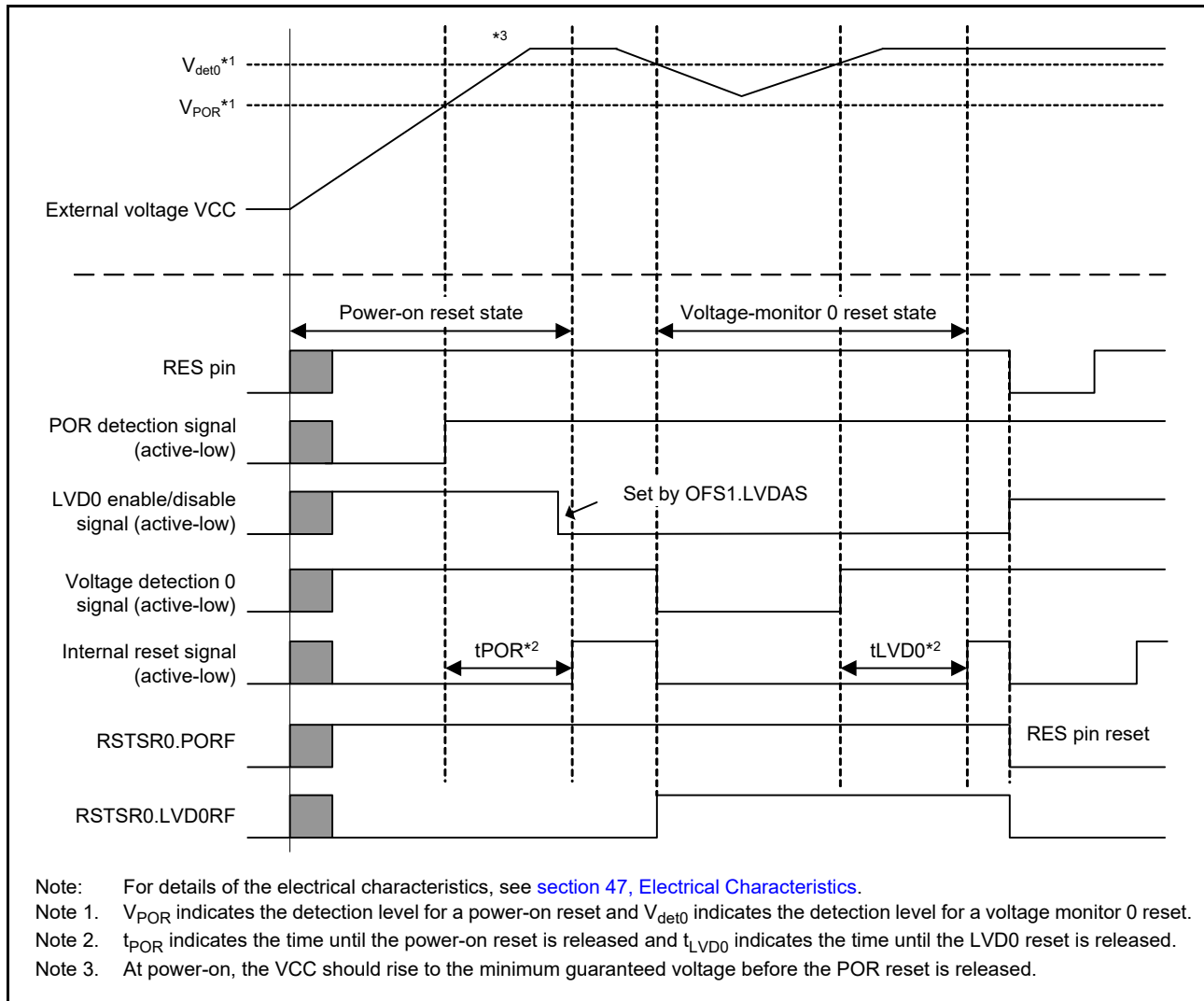
Figure 8.4 Example of voltage monitor 0 reset operation
