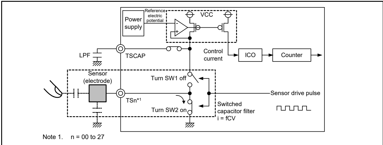
Figure 40.6 Discharging operation
