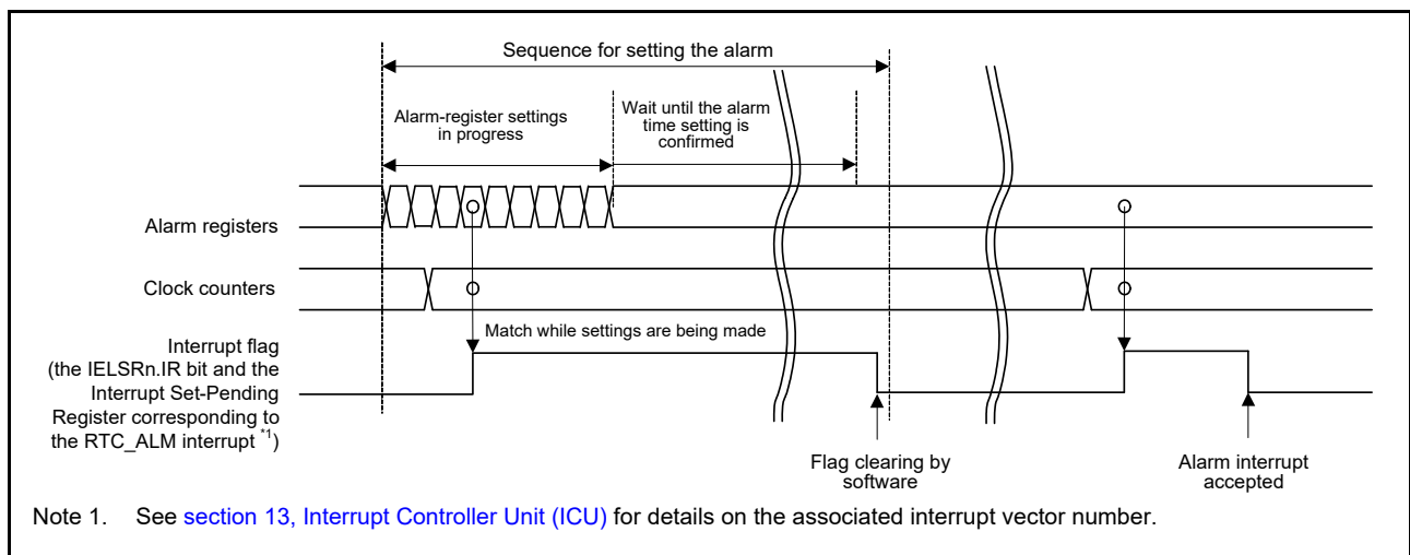
Figure 23.9 Timing for the alarm interrupt (RTC_ALM)
