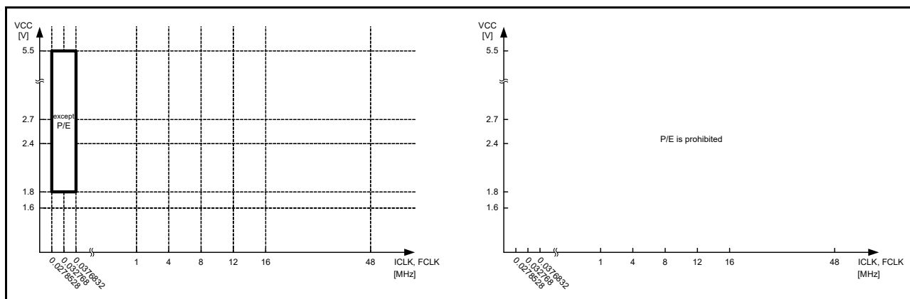
Figure 11.6 Operating voltages and frequencies in Subosc-speed mode
