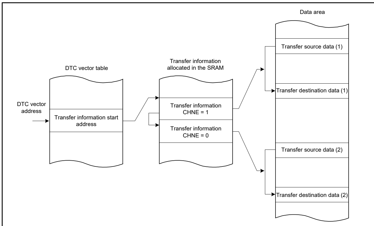
Figure 16.8 Chain transfer operation
