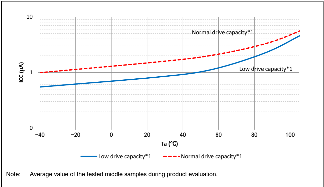
Figure 47.23 Temperature dependency of RTC operation (reference data)
