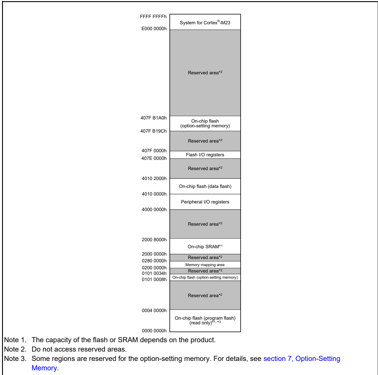
Figure 4.1 Memory map
