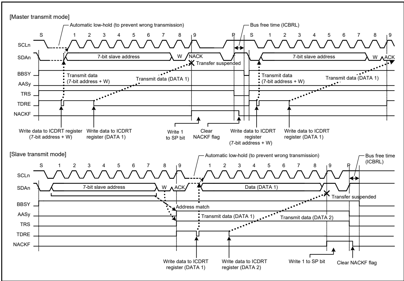
Figure 28.39 Suspension of data transfer when NACK is received (NACKF = 1)
