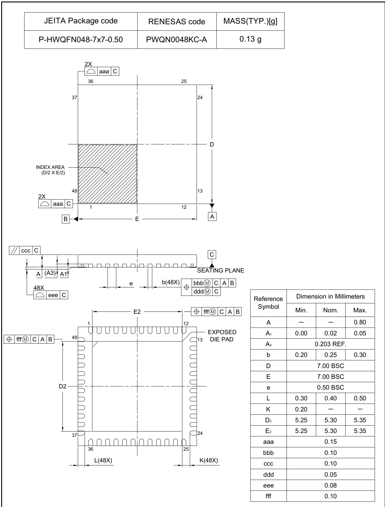
Figure 2.5 QFN 48-pin (2)
