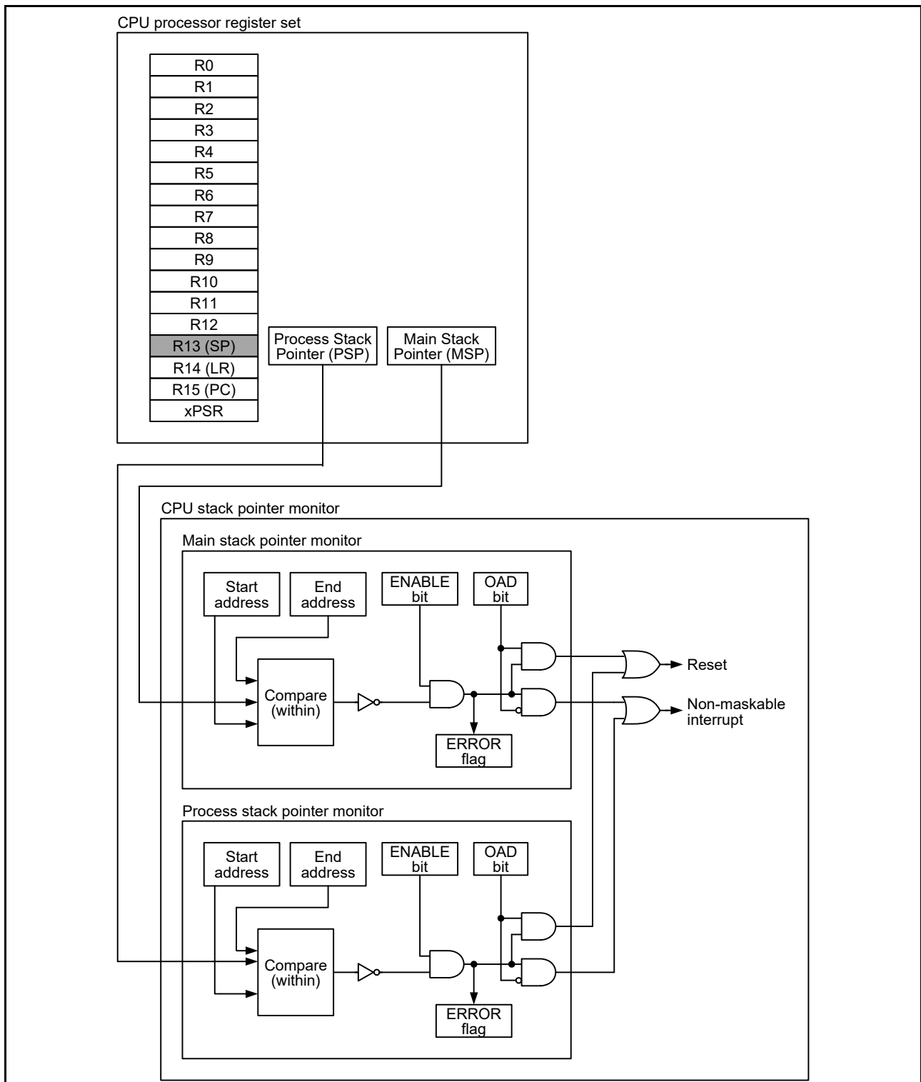
Figure 15.1 CPU stack pointer monitor block diagram
