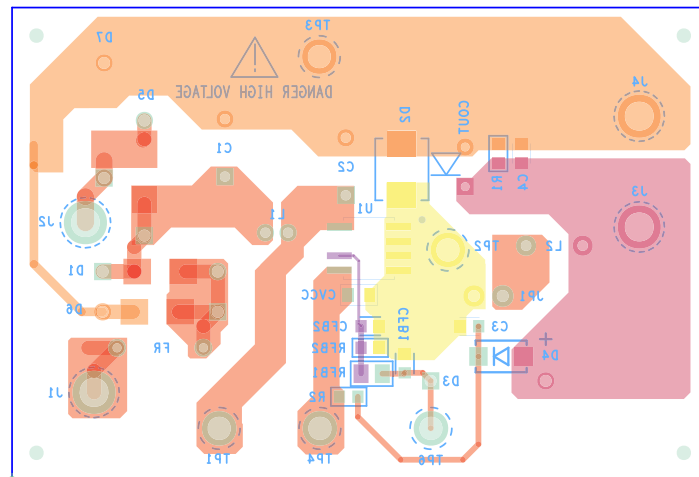
Figure 6. Bottom Layer
