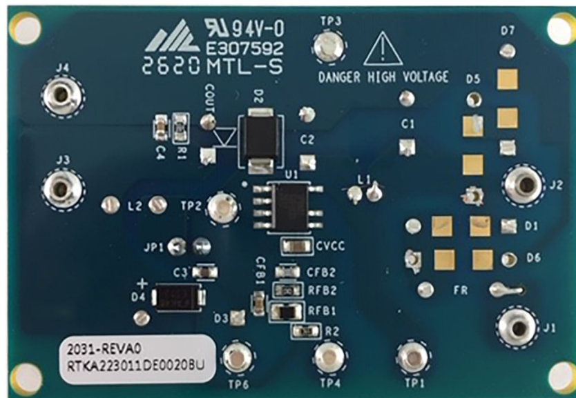
Figure 3. RTKA223011DE0020BU Evaluation Board (Bottom)
