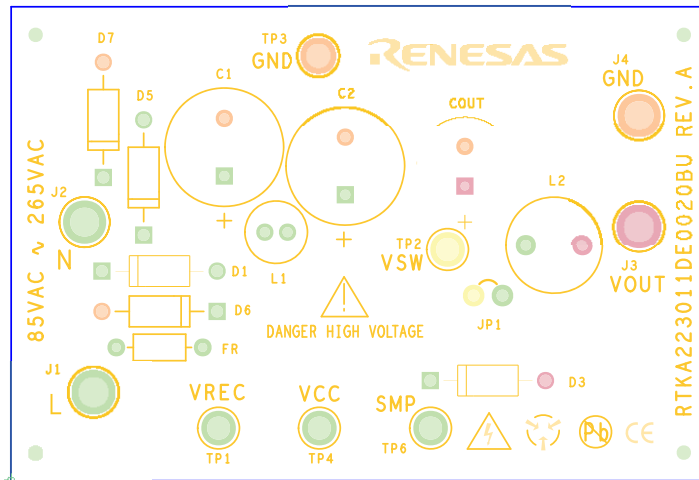
Figure 5. Top Layer
