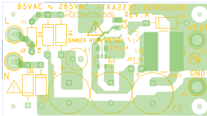
Figure 5. Top Layer
