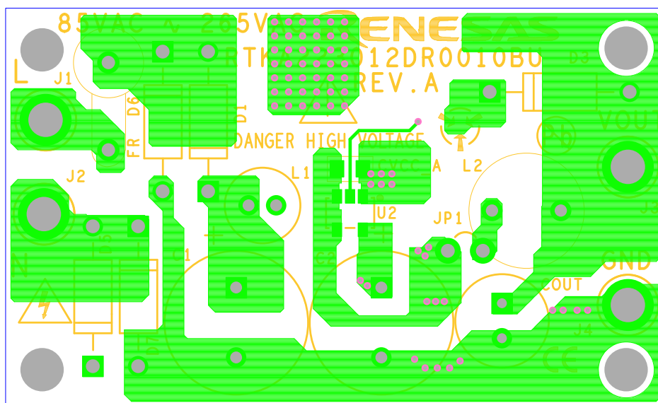
Figure 8. Top Layer
