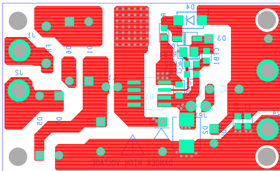
Figure 9. Bottom Layer
