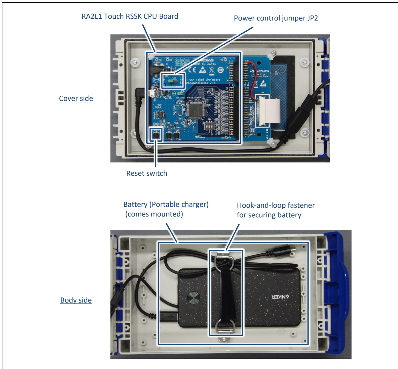
Figure 2-3. Internal Configuration
