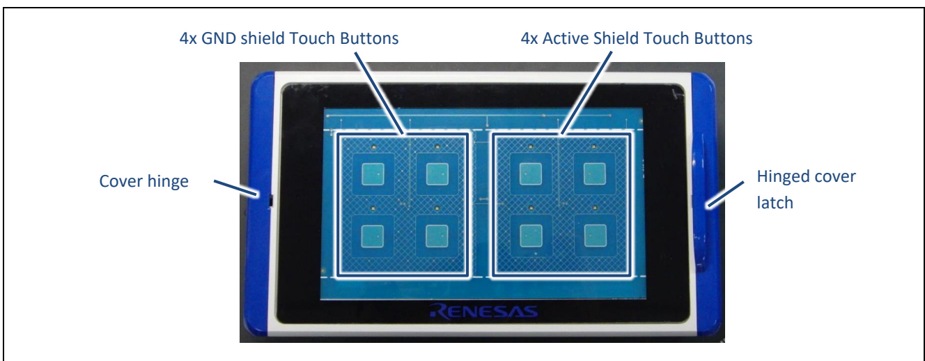
Figure 2-2 Control Panel
