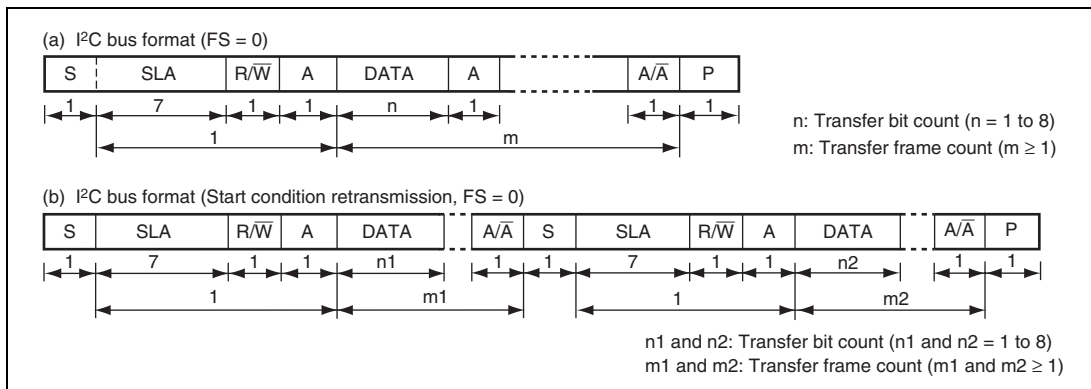
Figure 17.3 I 2 C Bus Formats
