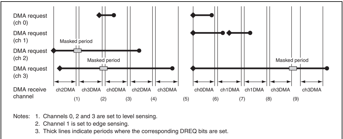
Figure 11.10 Overall Operation during Multiple DMA Requests
