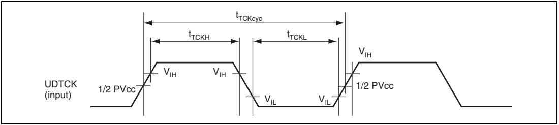
Figure 29.43 UDTCK Input Timing
