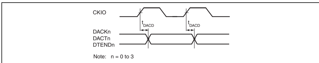
Figure 29.23 DACK, DACT, DTEND Output Timing
