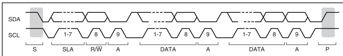
Figure 17.4 I 2 C Bus Timing
