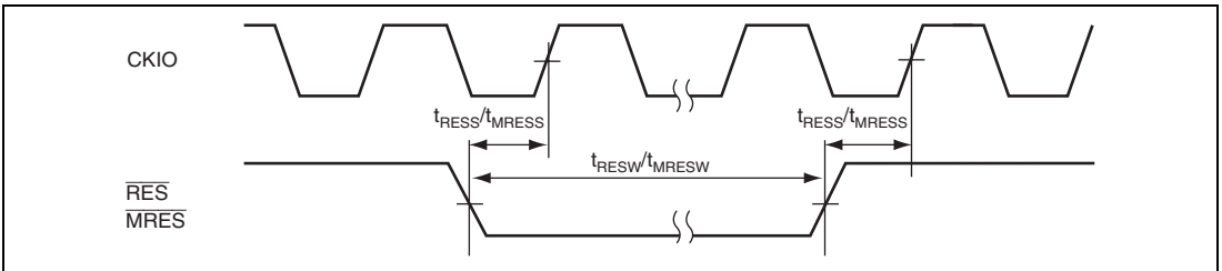
Figure 29.8 Reset Input Timing
