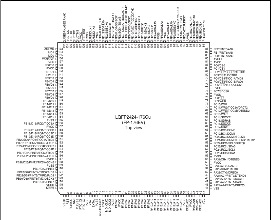
Figure 1.2 Pin Assignments
