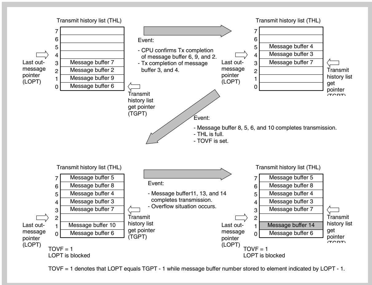
Figure 14-31 Transmit history list
