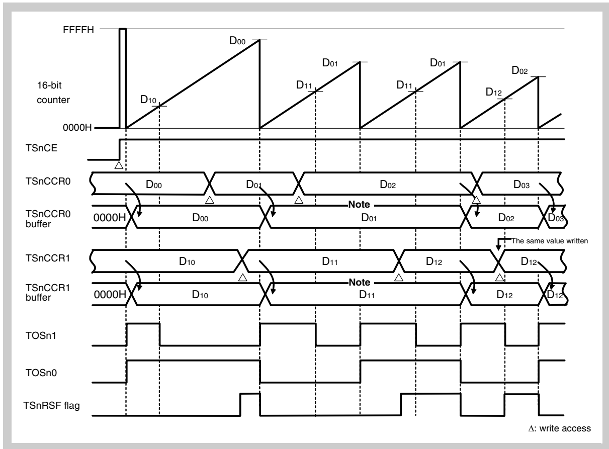
Figure 17-66 Basic operation timing in PWM mode (2/2)
