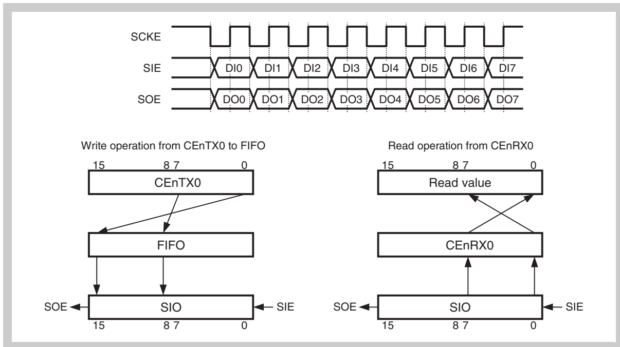
Figure 13-5 Serial data direction select function - LSB first (CEnDIR = 0)
