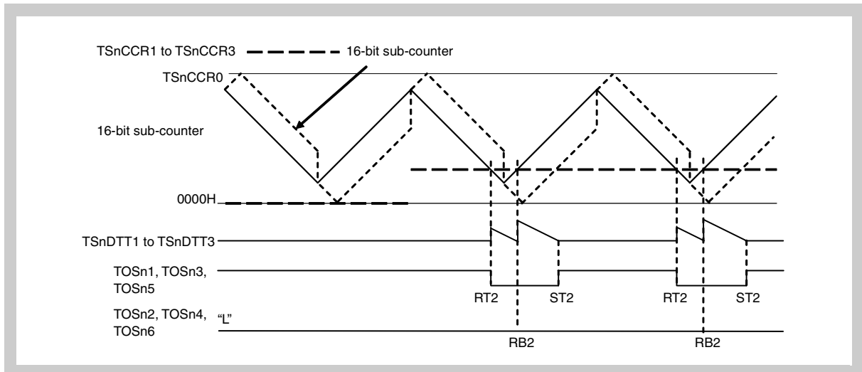
Figure 17-112 TSnCCR1 to TSnCCR3 = 0000H \rightarrow TSnDTC0 + 1 < TSnCCR1 to TSnCCR3 < TSnDTC0 + TSnDTC1
