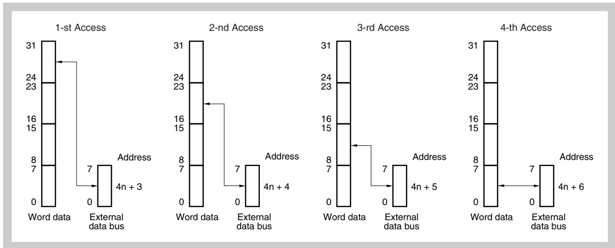
Figure 9-26 Access to address 4n + 3
