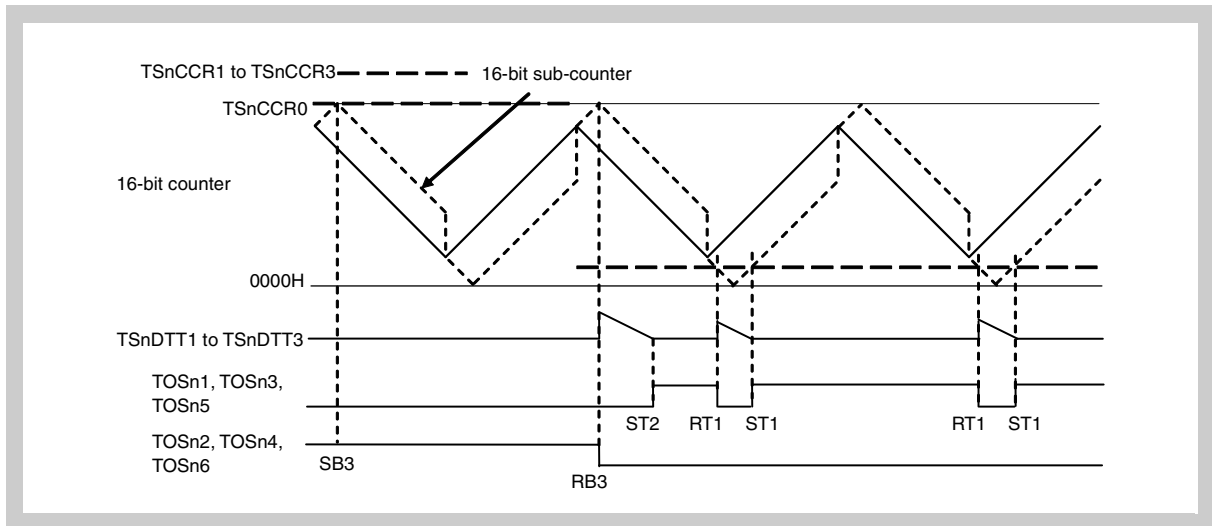
Figure 17-105 TSnCCR1 to TSnCCR3 = TSnCCR0 \rightarrow 0000H < TSnCCR1 to TSnCCR3 \leq TSnDTC0 + 1
