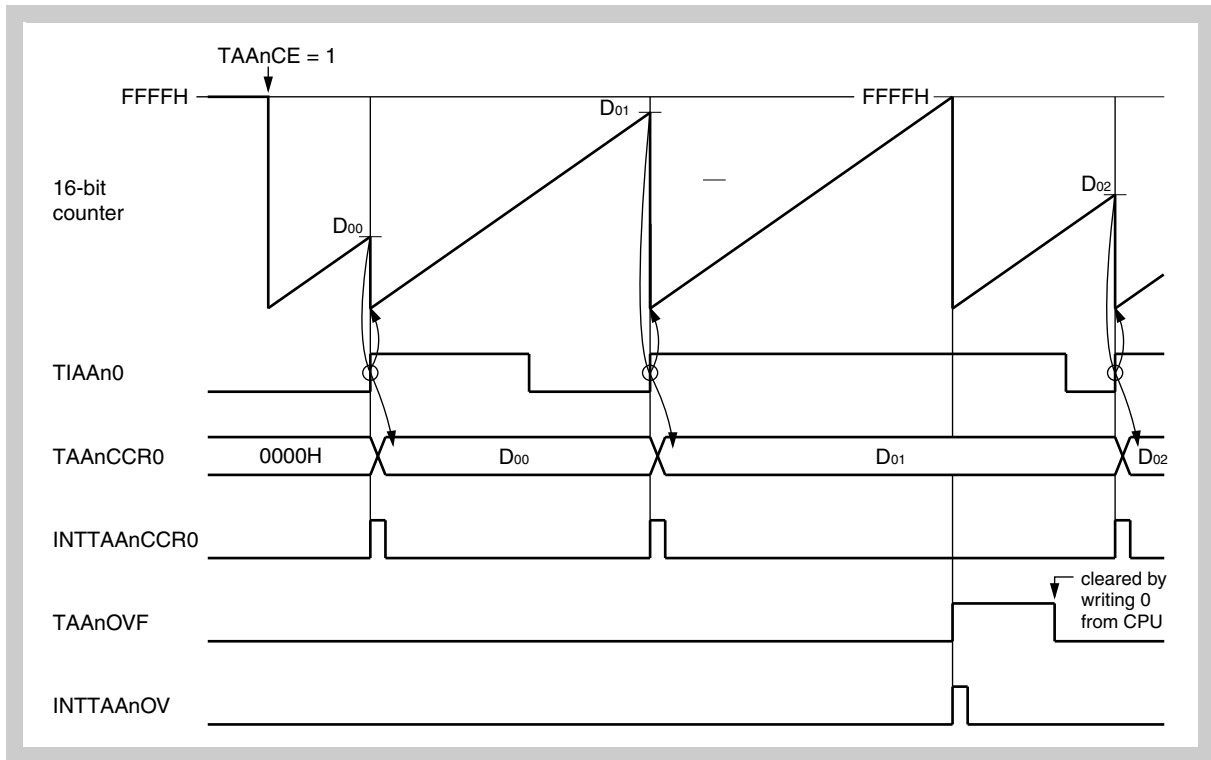
Figure 16-31 Basic operation timing of pulse period measurement
