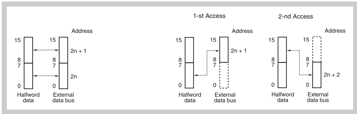
Figure 9-29 Left: Access to even address ( 2n ) Right: Access to odd address ( 2n + 1 )
