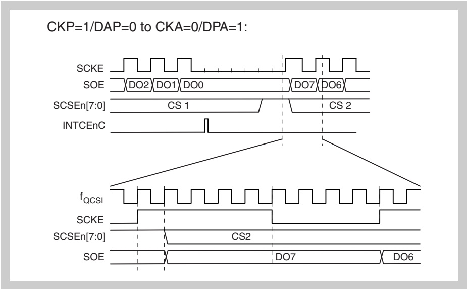
Figure 13-26 CKP=1, DAP=0 to CKA=0, DPA=0 with enhanced timing
