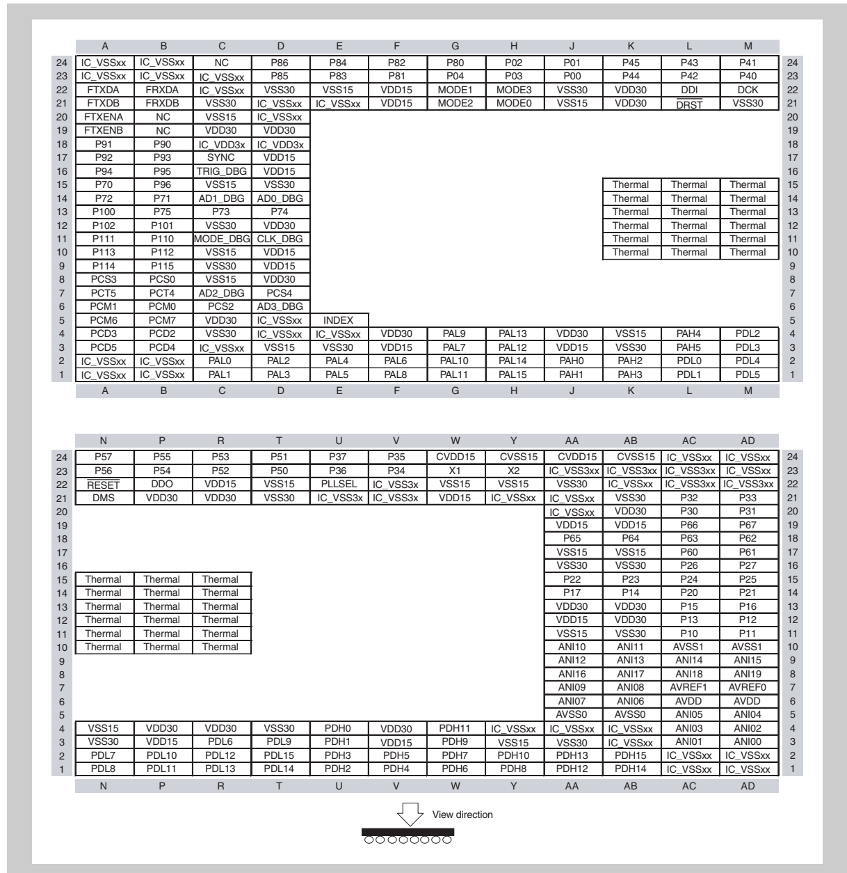
Figure 2-4 Pin overview
