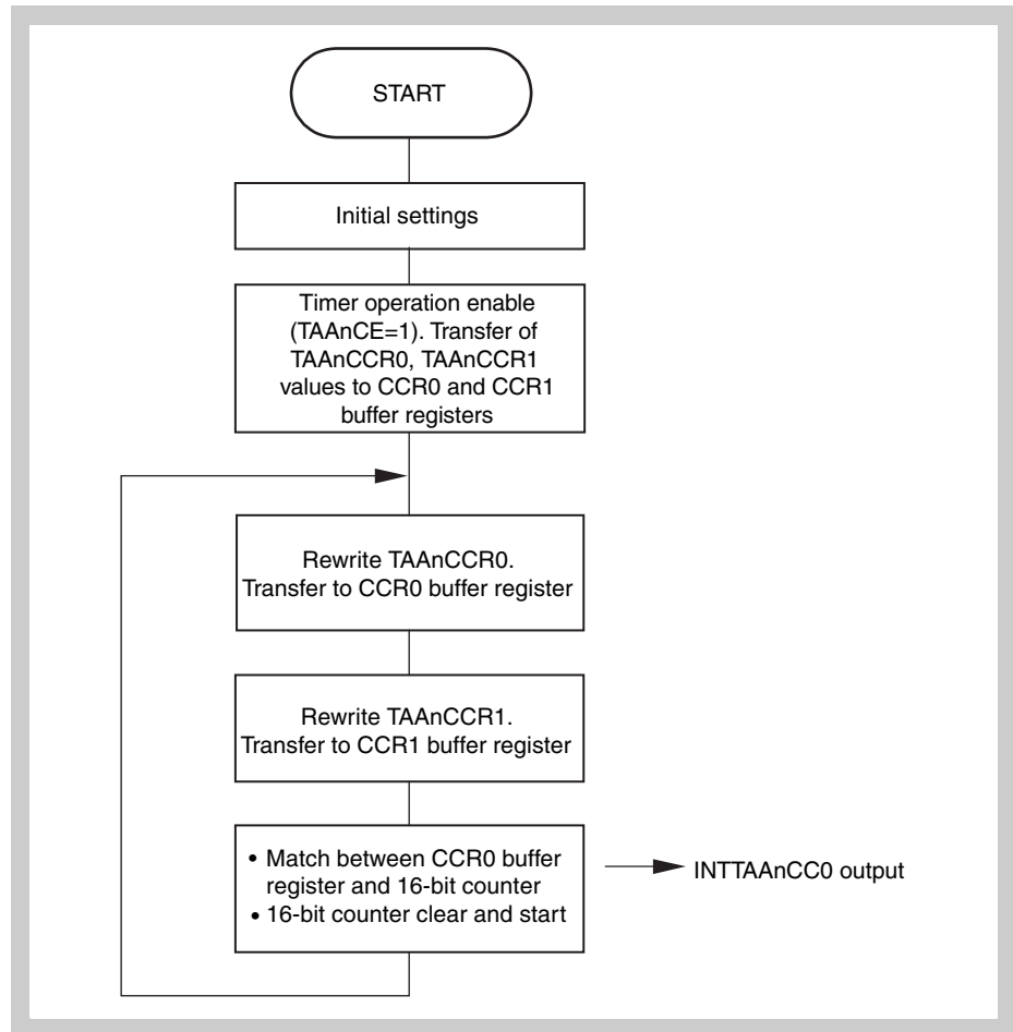
Figure 16-7 Flowchart of basic operation for anytime write
