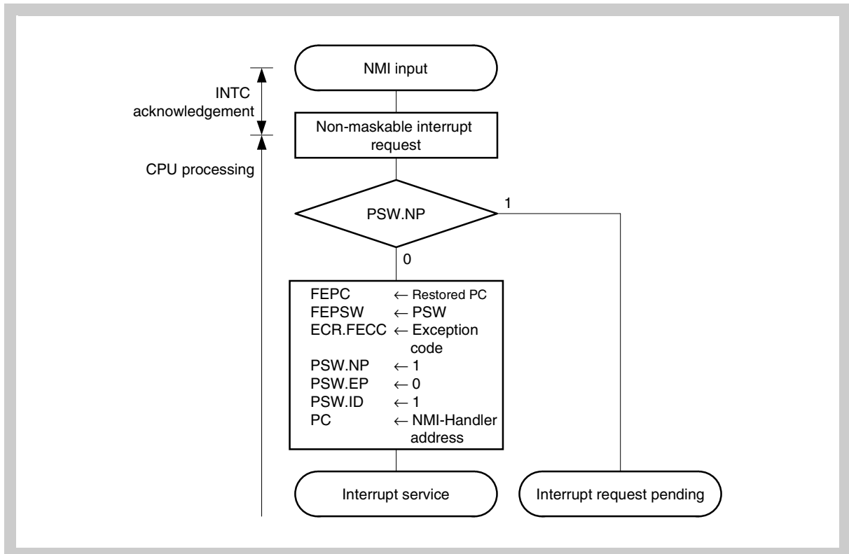
Figure 4-3 Processing configuration of non-maskable interrupt
