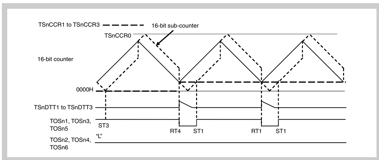
Figure 17-87 TSnCCR1 to TSnCCR3 = 0000H \rightarrow TSnCCR1 to TSnCCR3 = TSnDTC0, TSnDTC0 + 1
