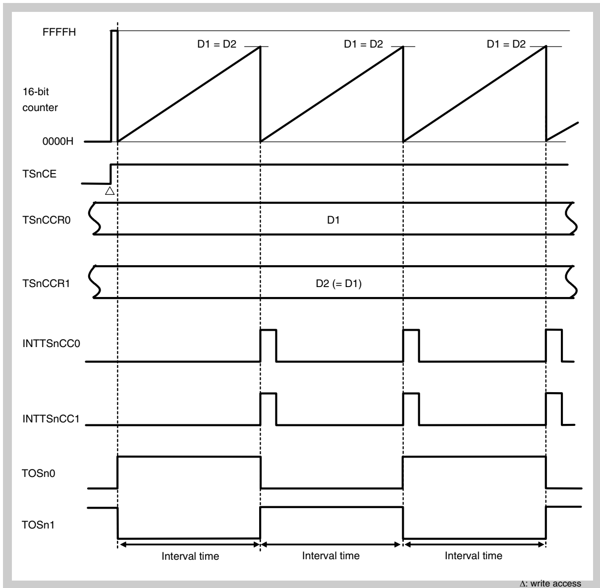
Figure 17-53 Basic timing in interval timer mode (2/2)
