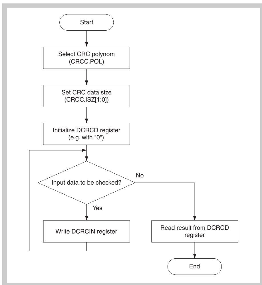
Figure 5-3 DATA-CRC flow diagram
