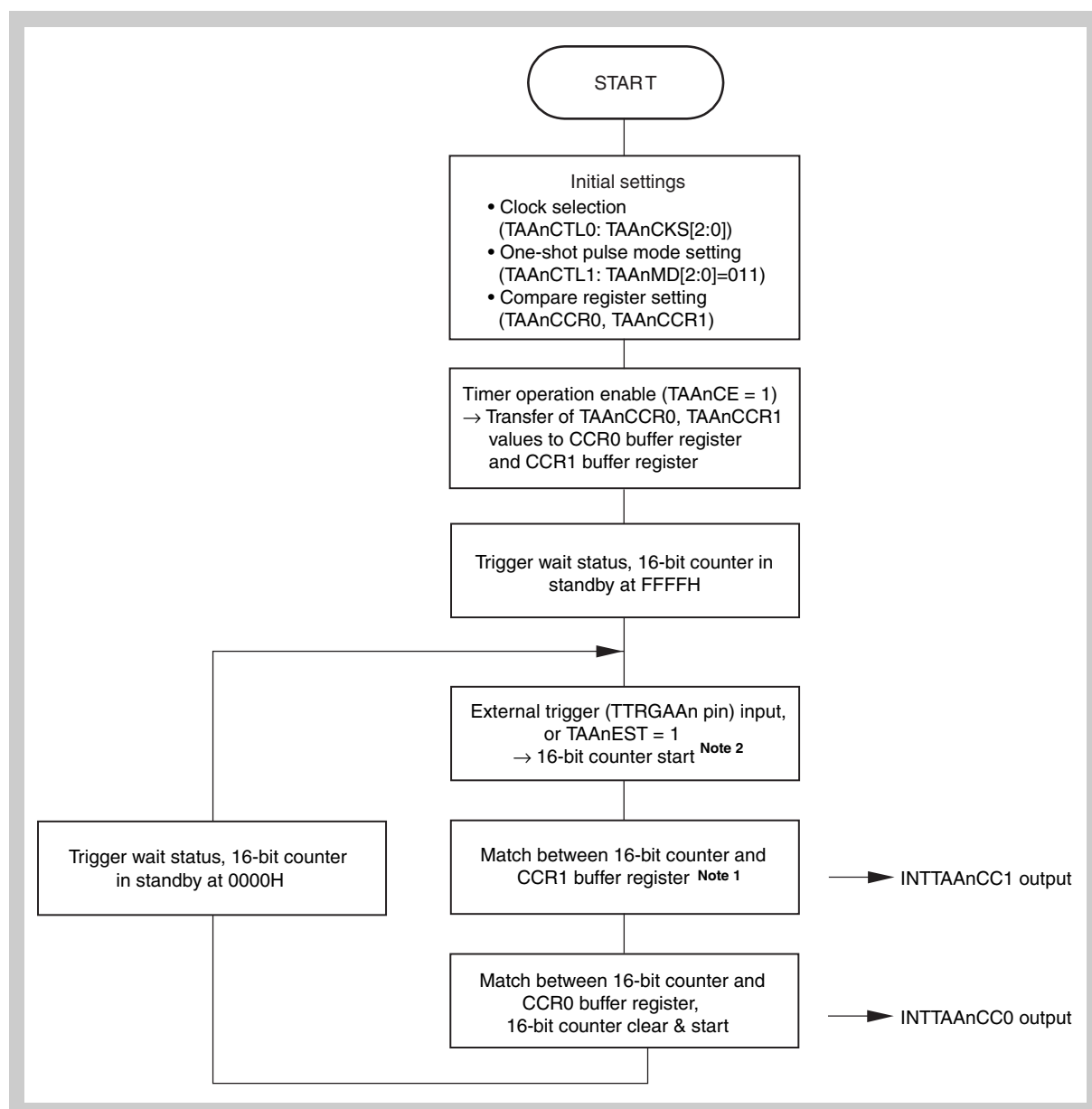
Figure 16-19 Flowchart of basic operation in one-shot pulse mode
