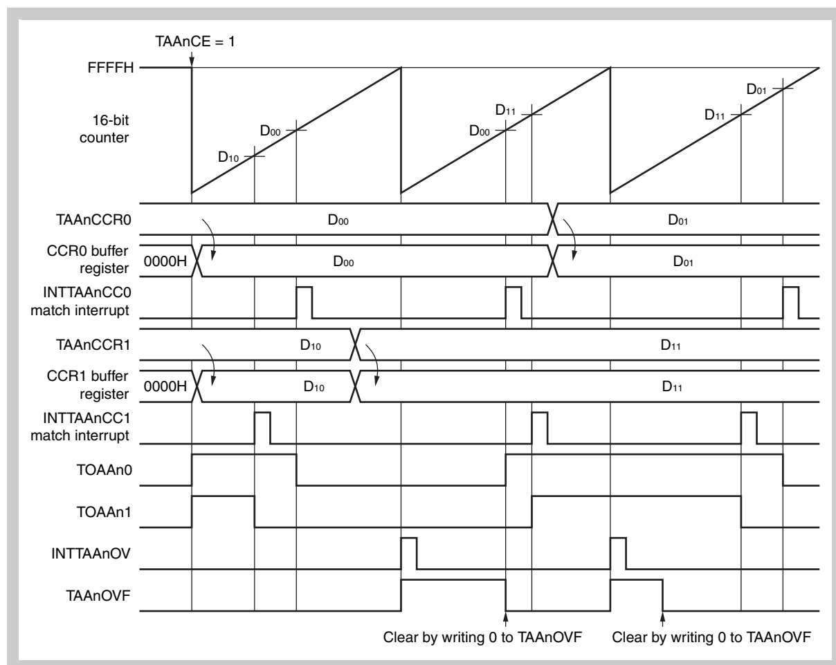
Figure 16-26 Basic Operation Timing In Free-running Mode (TAAAnCCS1 = 0, TAAAnCCS0 = 0) (TAAAnOE0 = 1, TAAAnOE1 = 1, TAAAnOL0 = 0, TAAAnOL1 = 0)
