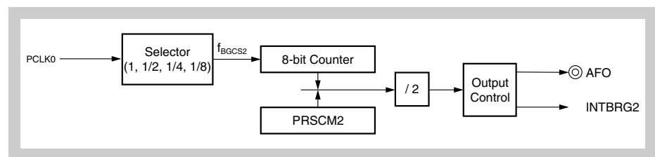
Figure 22-1 Block diagram of Auxiliary Frequency Output Function
