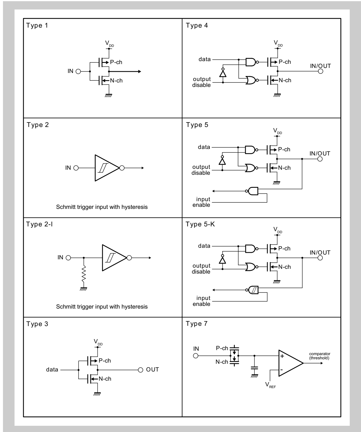
Figure 2-2 Port type diagrams
