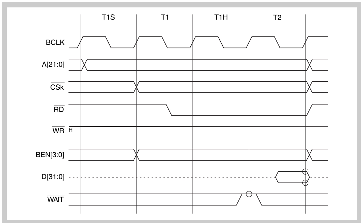
Figure 9-10 Read timing (address setup wait and address hold wait state inserted)
