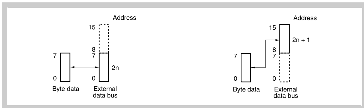
Figure 9-27 Left: Access to even address ( 2n ) Right: Access odd address ( 2n + 1 )
