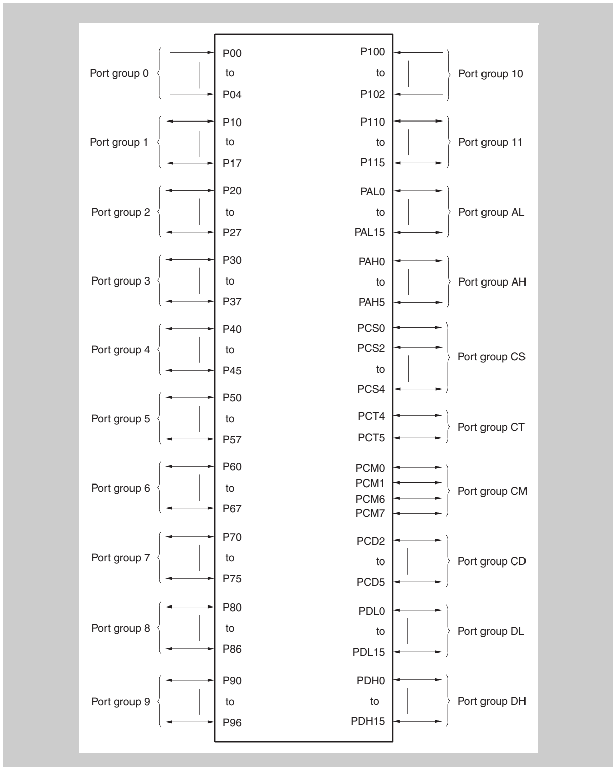
Figure 2-1 Port groups
