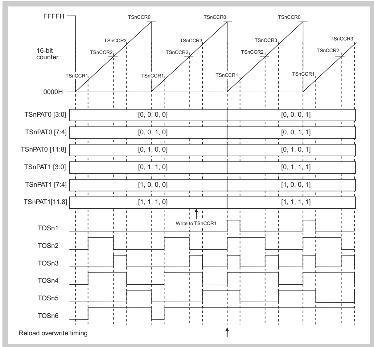
Figure 17-192 Pattern register rewriting operation in special pattern output mode
