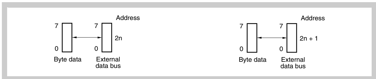
Figure 9-16 Left: Access to even address ( 2n ) Right: Access to odd address ( 2n + 1 )
