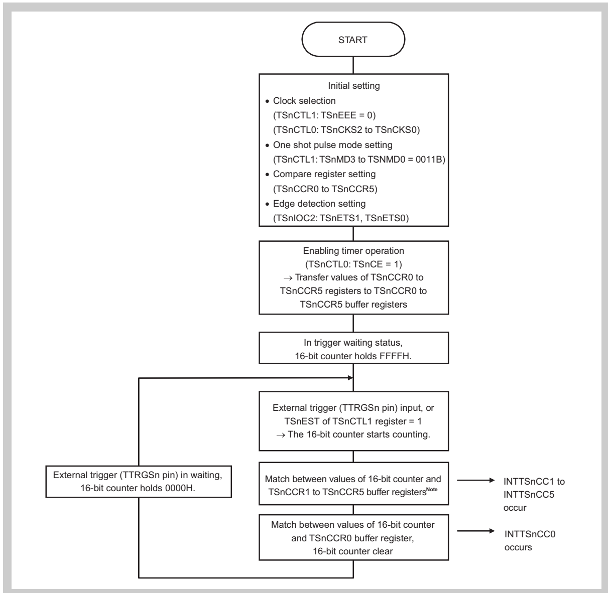
Figure 17-61 Basic operation flow in one-shot pulse mode
