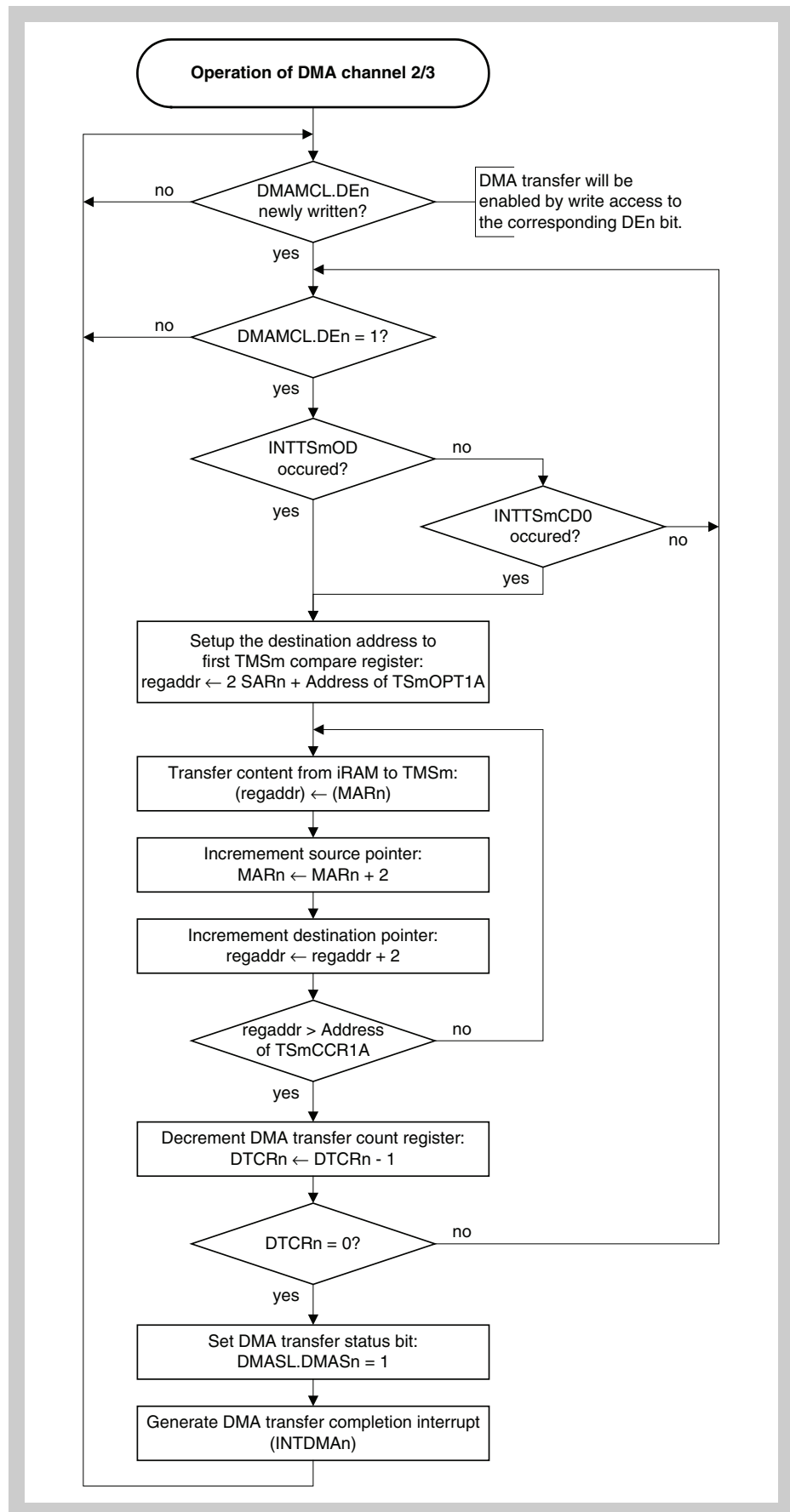
Figure 10-5 Operation of DMA Channel 2/3
