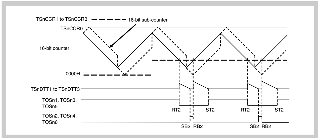
Figure 17-111 TSnCCR1 to TSnCCR3 = 0000H \rightarrow TSnDTC0 + TSnDTC1 < TSnCCR1 to TSnCCR3 \leq TSnCCR0 - TSnDTC0 - TSnDTC1
