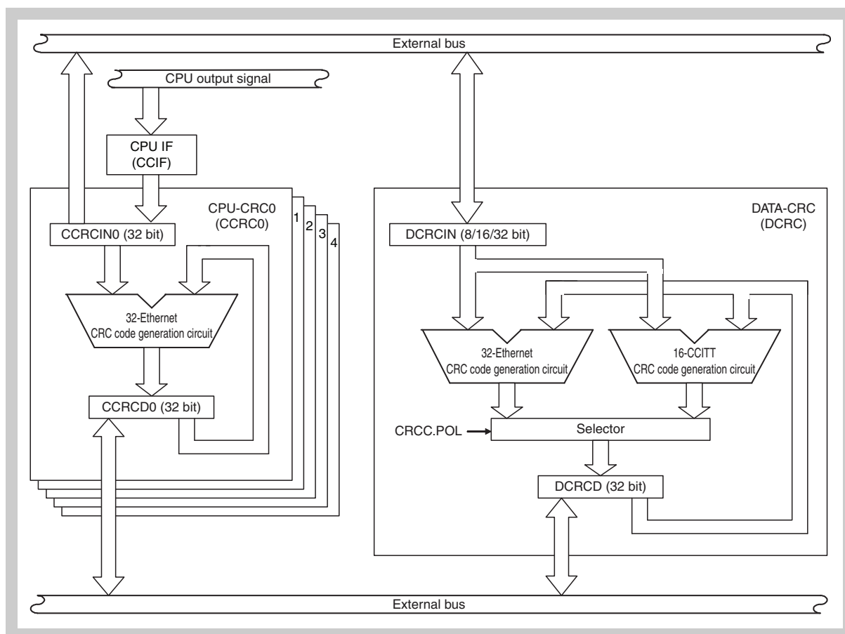
Figure 5-1 Block diagram of CPU-CRC and DATA-CRC
