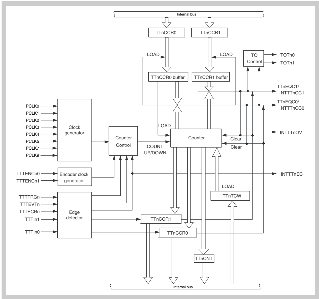
Figure 18-1 Block diagram of Timer T
