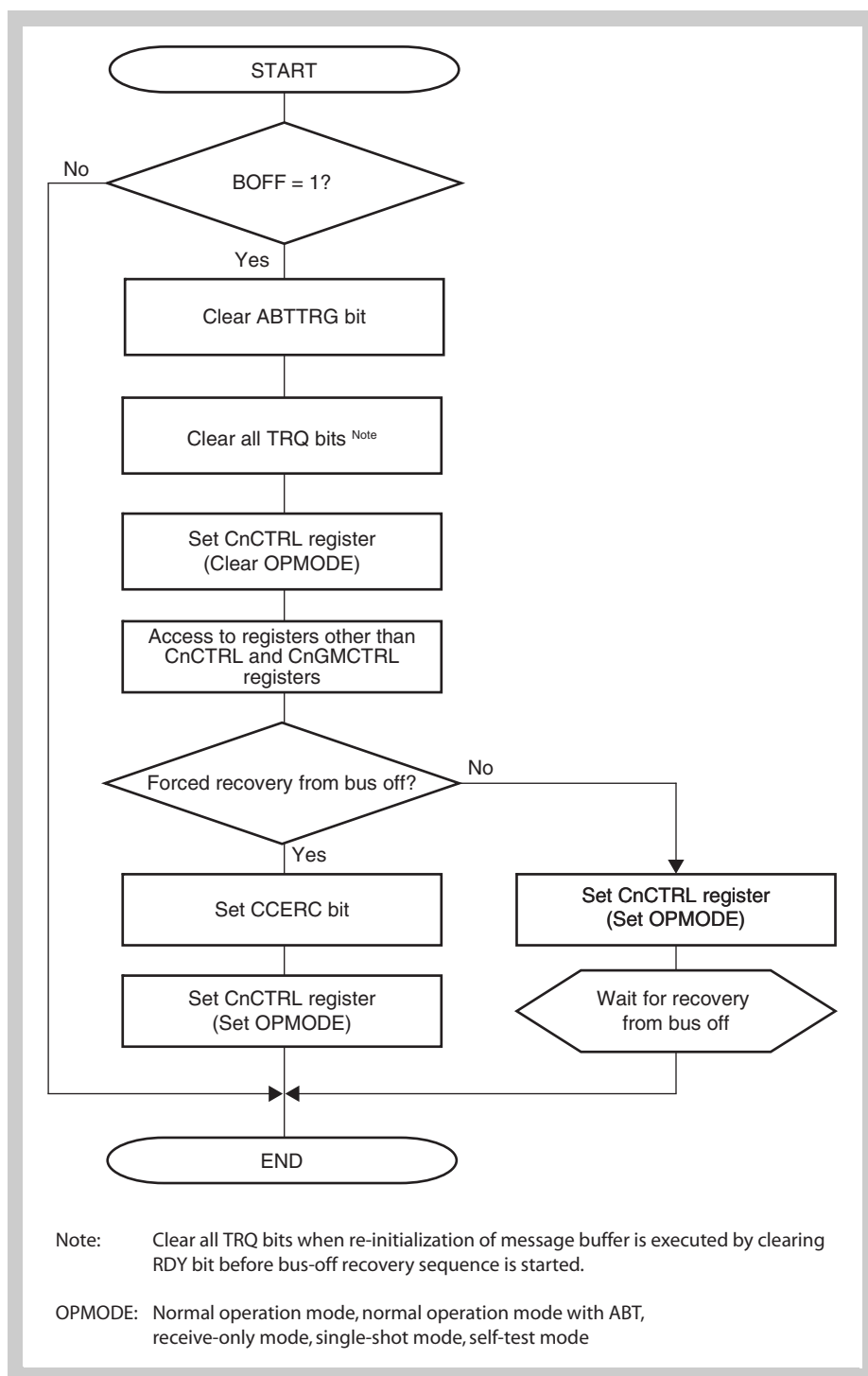
Figure 14-56 Bus-off recovery (Normal Operation Mode with ABT)
