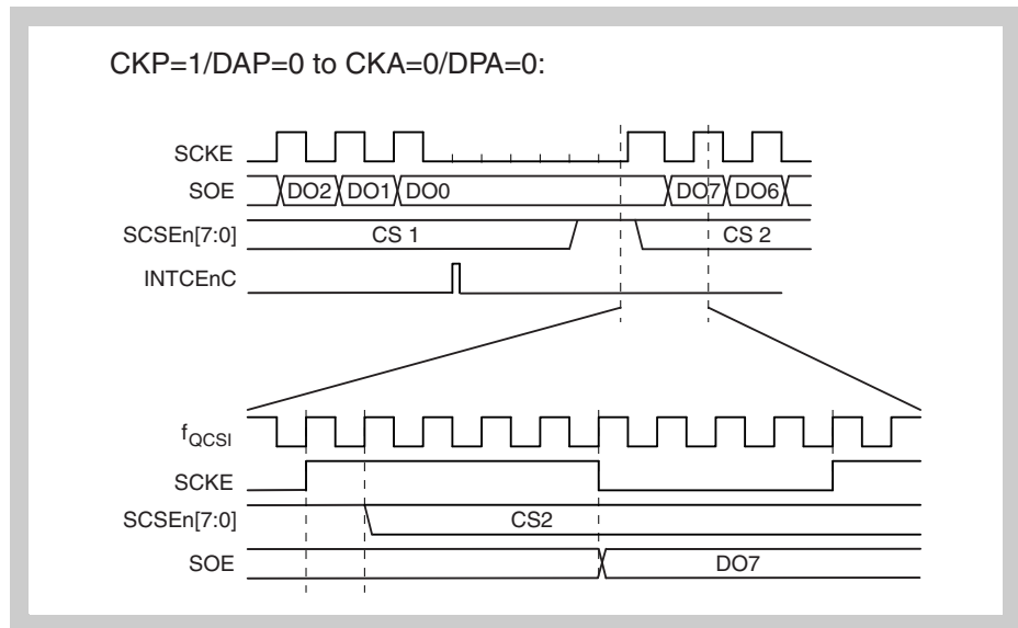
Figure 13-25 CKP=1, DAP=0 to CKA=0, DPA=1 with enhanced timing
