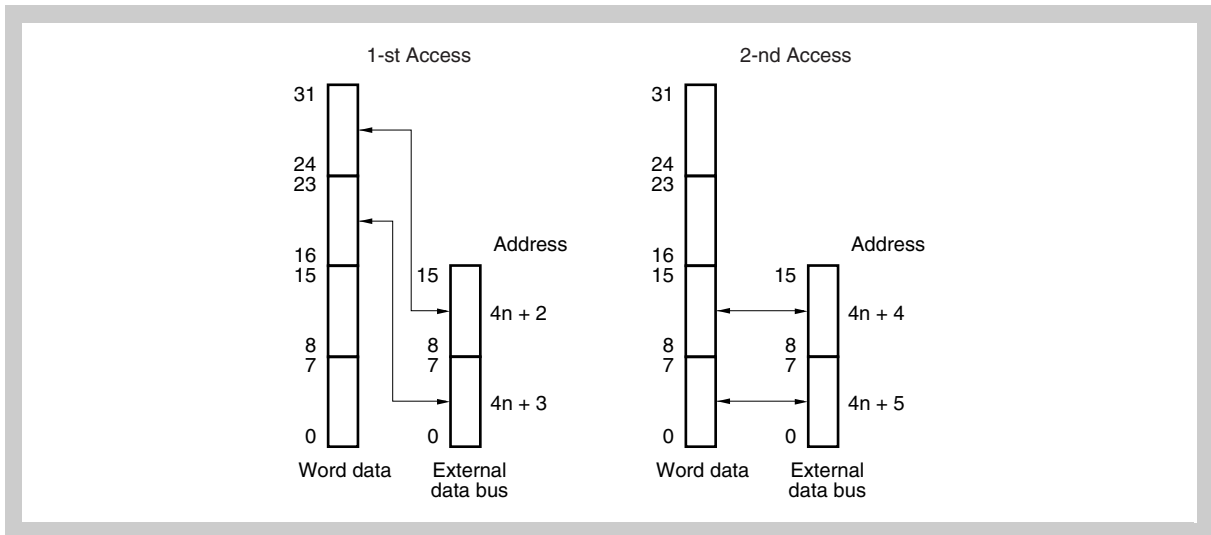
Figure 9-37 Access to address 4n + 2
