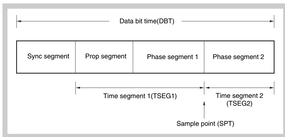
Figure 14-18 Segment setting
