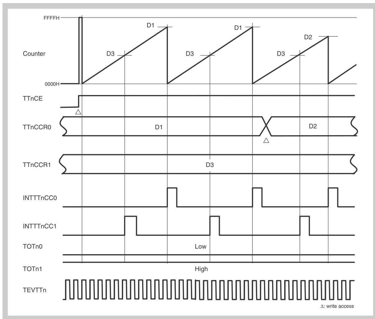
Figure 18-9 Basic operation timing in external event count mode (1/4) When D1 > D2 > D3 , only value of TnCCR0 register (0000H to FFFFH) and TOTn0 and TOTn1 are not output. The signal input from TEVTn and internally synchronized is counted as the count clock (TTnOE0, 1 = 0, TTnOL0 = 0, TTnOL1 = 1)
