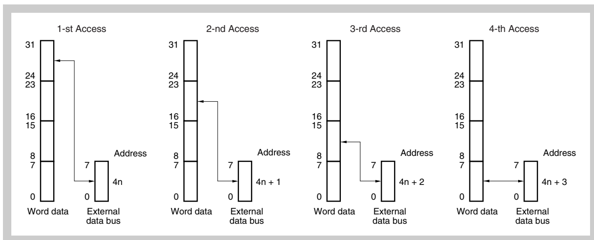
Figure 9-23 Access to address 4n
