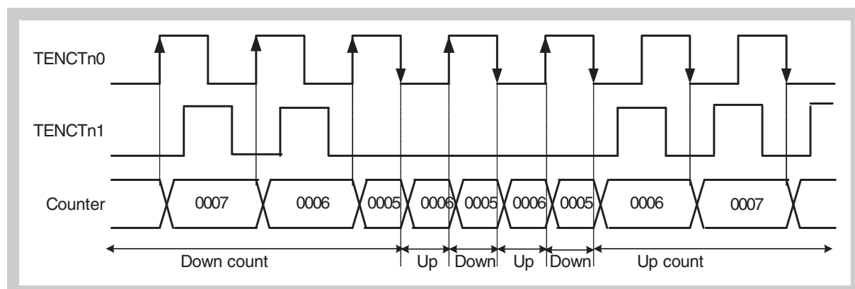
Figure 18-29 Encoder count function up/down count selection specification timings (3/6) - timing 3
