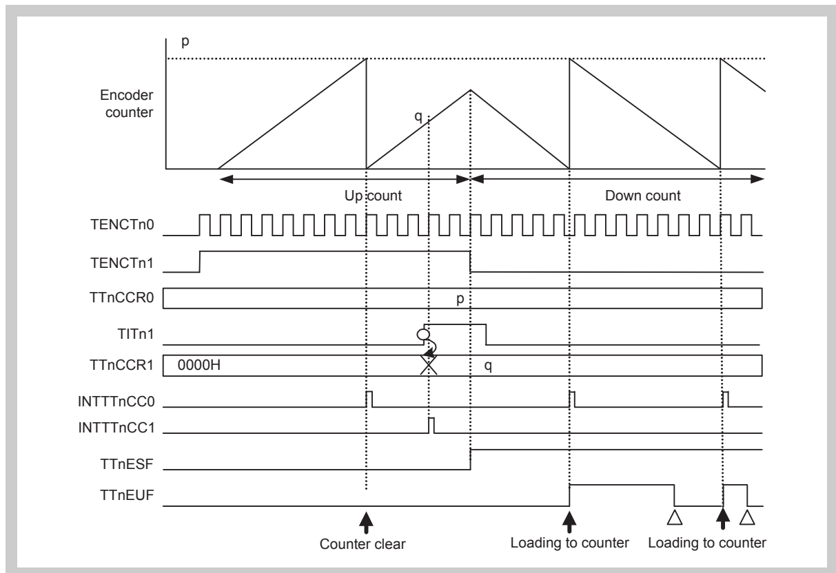
Figure 18-47 Counter hold through bit TTnECC timings (8/8) Basic timing in encoder capture compare mode (1)
