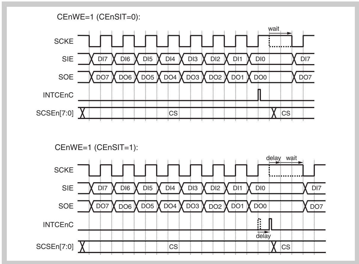
Figure 13-15 Selection of transmit wait enable/disable
