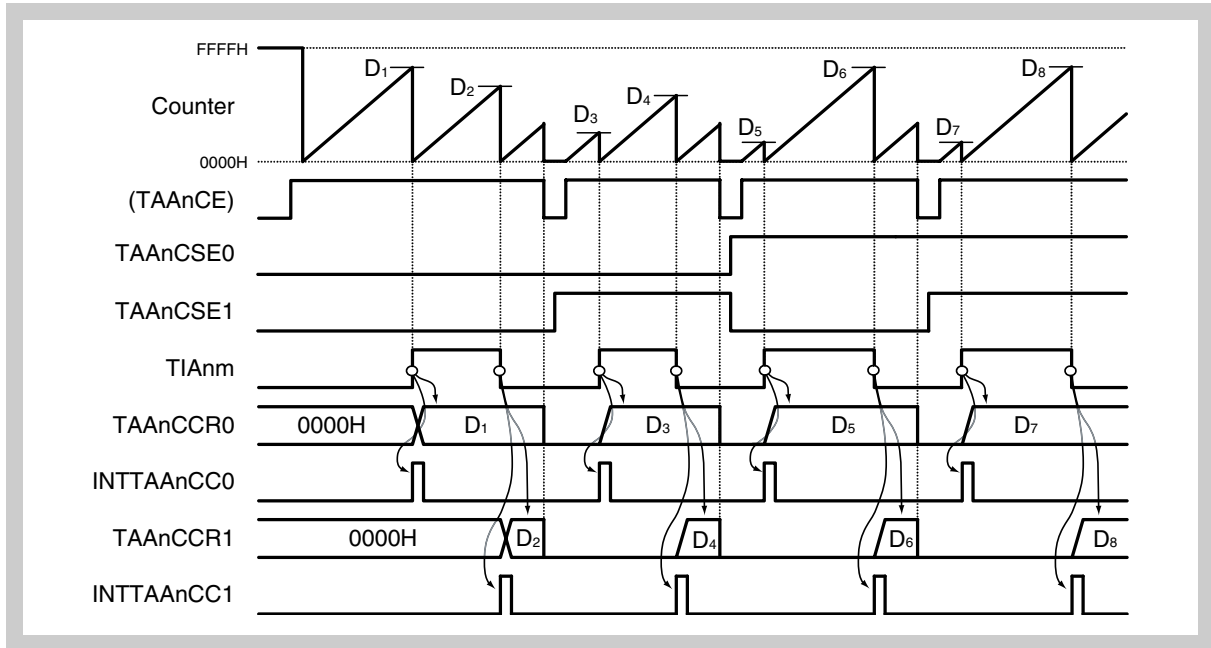
Figure 16-44 Specific overflow value write:
