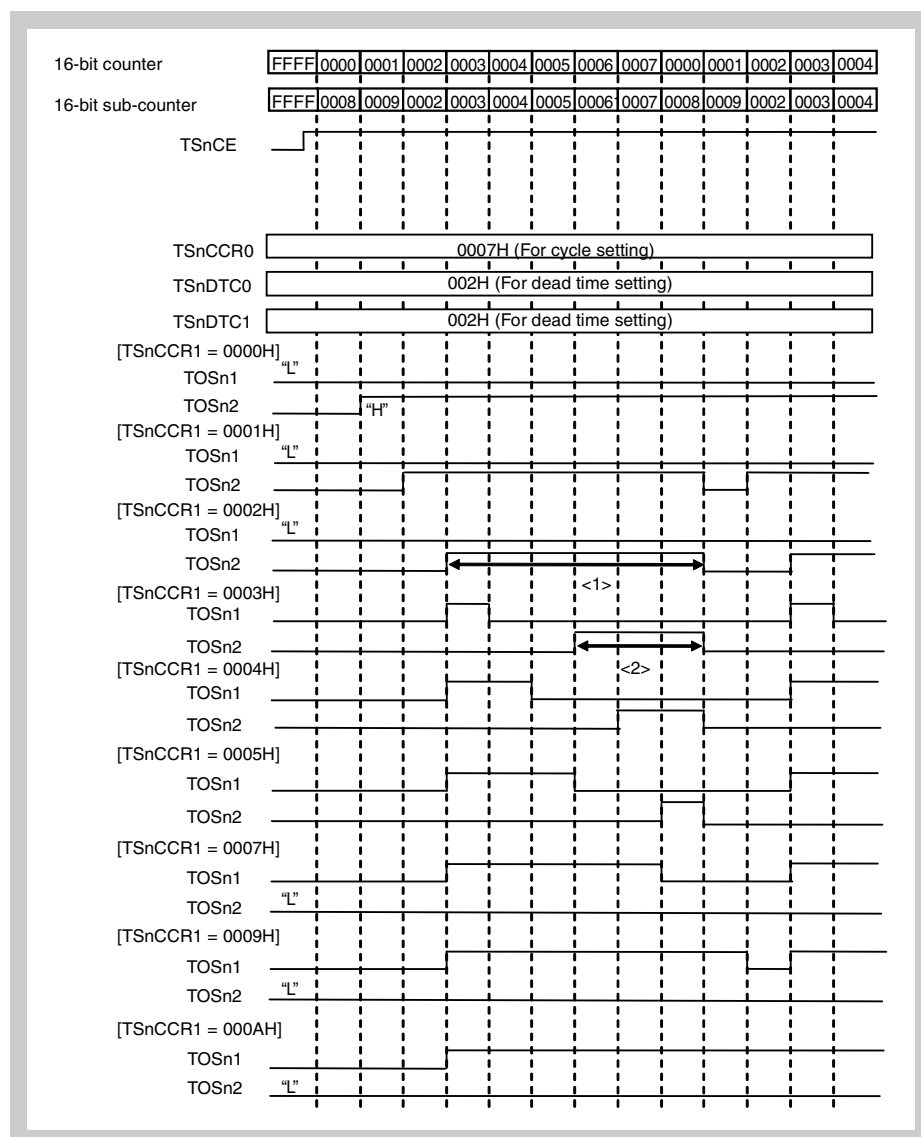
Figure 17-128 Timer output example in case of setting TSnCE = 1 (initial setting in PWM mode with dead time)
