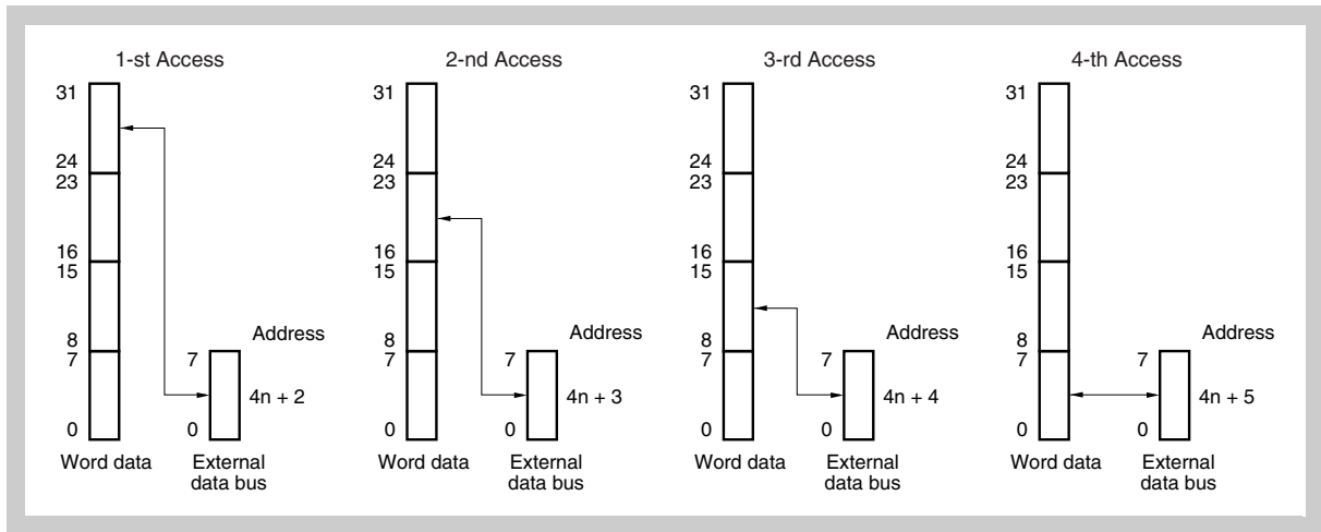
Figure 9-25 Access to address 4n + 2
