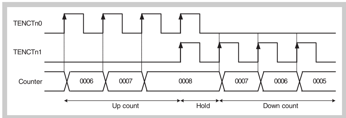
Figure 18-28 Encoder count function up/down count selection specification (2/6) - timing 2
