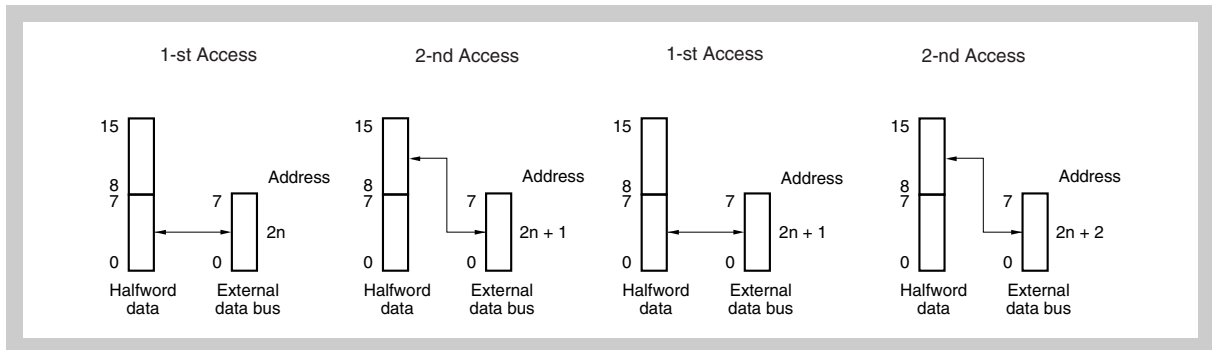
Figure 9-17 Left: Access to even address ( 2n ) Right: Access to odd address ( 2n + 1 )
