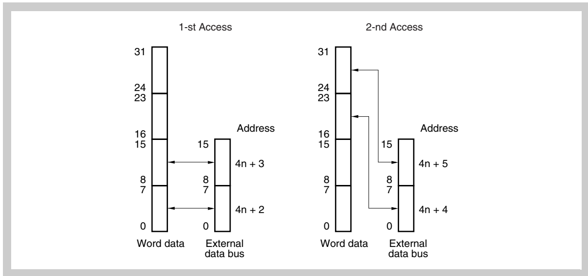
Figure 9-33 Access to address 4n + 2
