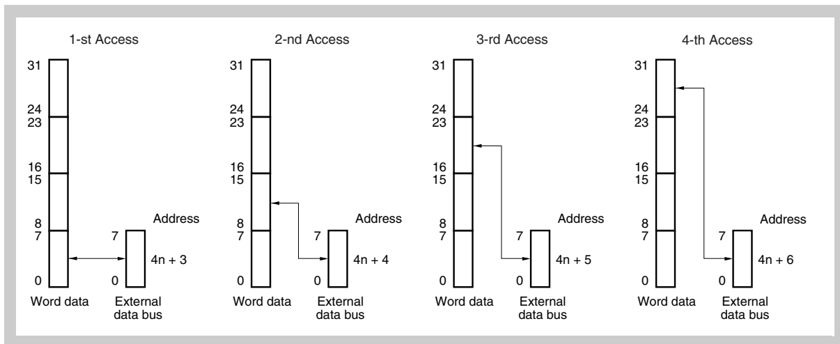
Figure 9-22 Access to address 4n + 3
