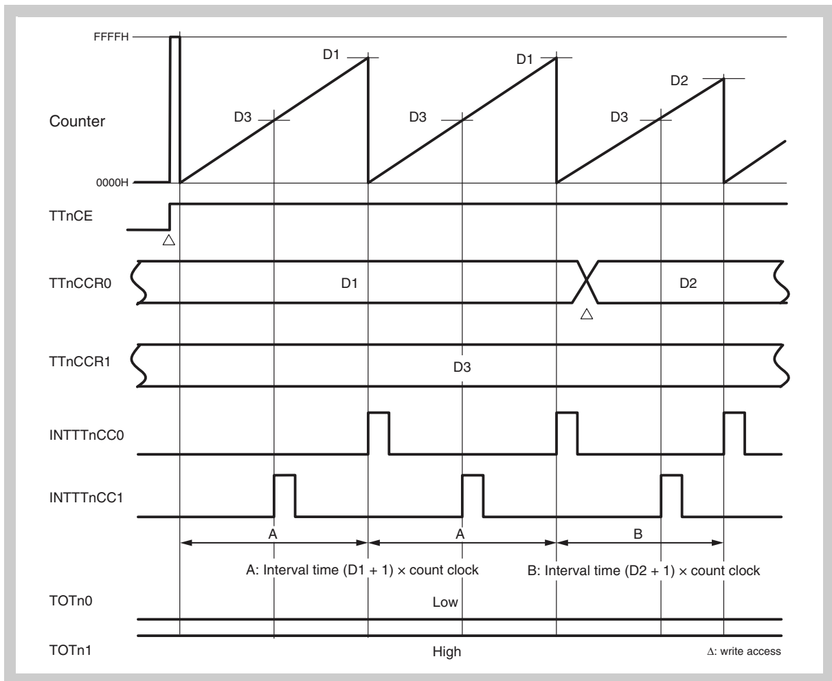
Figure 18-7 Basic timing in interval timer mode (1/2) When D1 > D2 > D3 , only value of TnCCR0 register is rewritten, TOTn0 and TOTn1 are not output (TTnOE0, 1 = 0, TTnOL0 = 0, TTnOL1 = 1)
