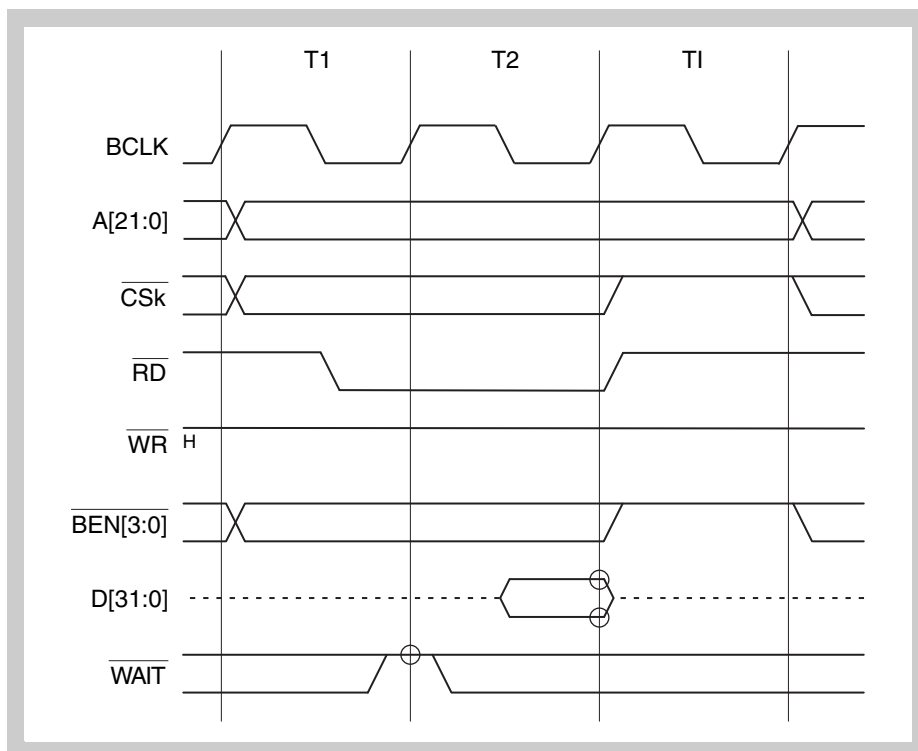
Figure 9-8 Read timing (idle state inserted)
