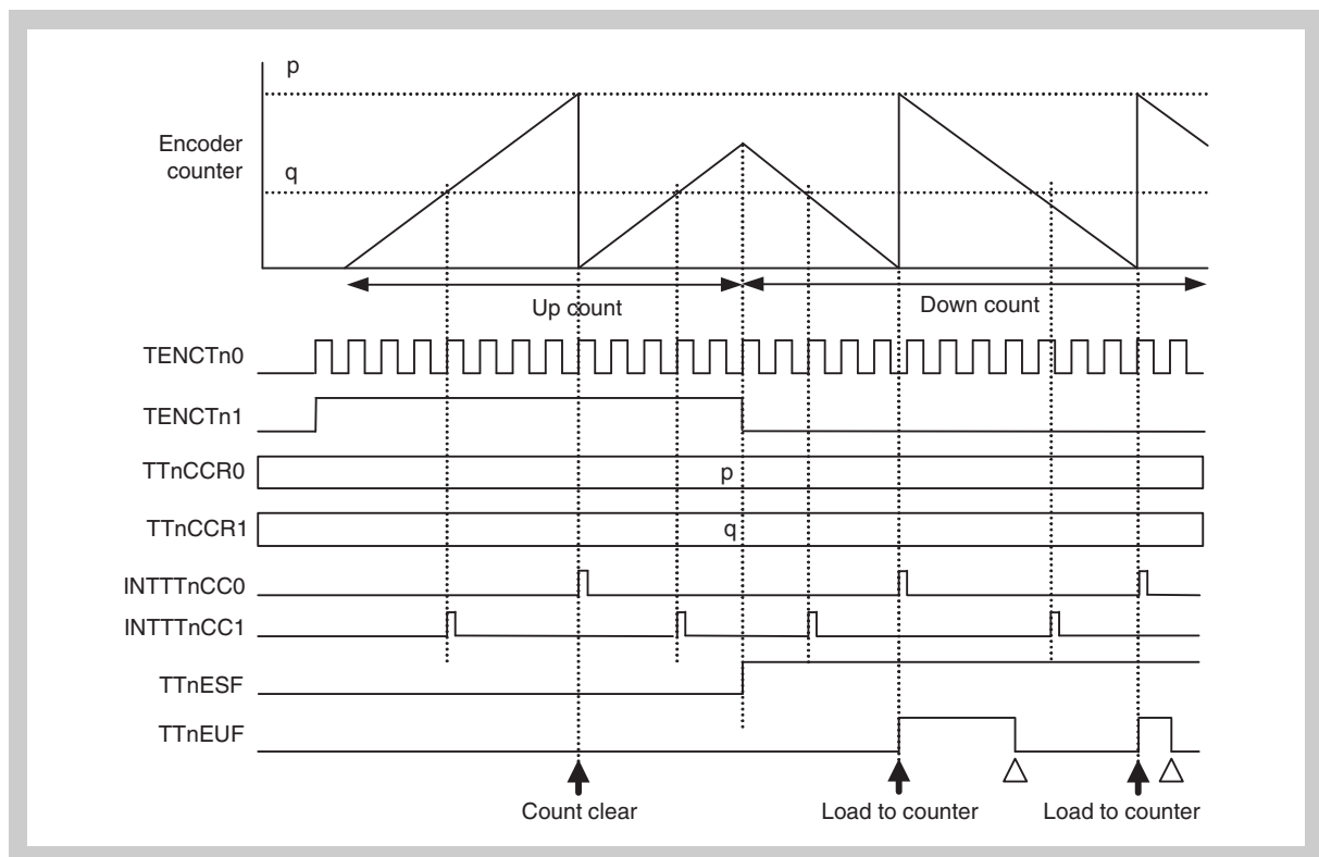
Figure 18-43 Counter hold through bit TTnECC timings (4/8) Basic timing in encoder compare mode (1)
