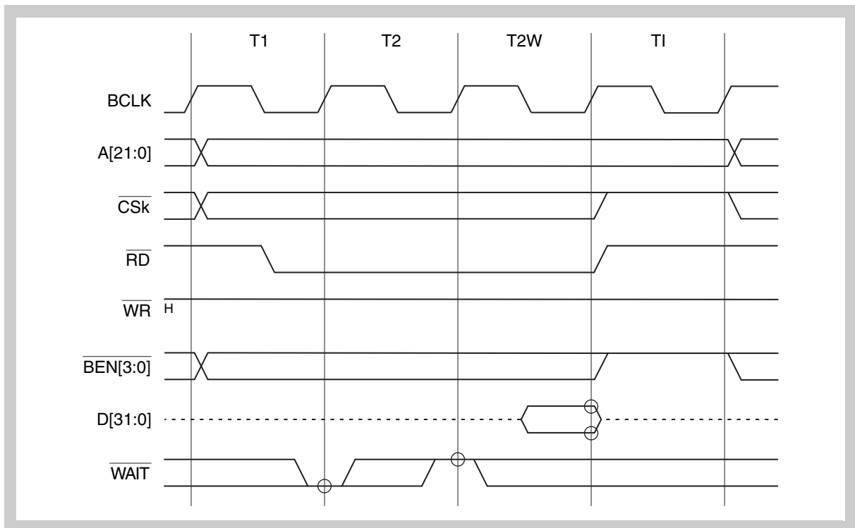
Figure 9-9 Read timing (data wait, idle state inserted)
