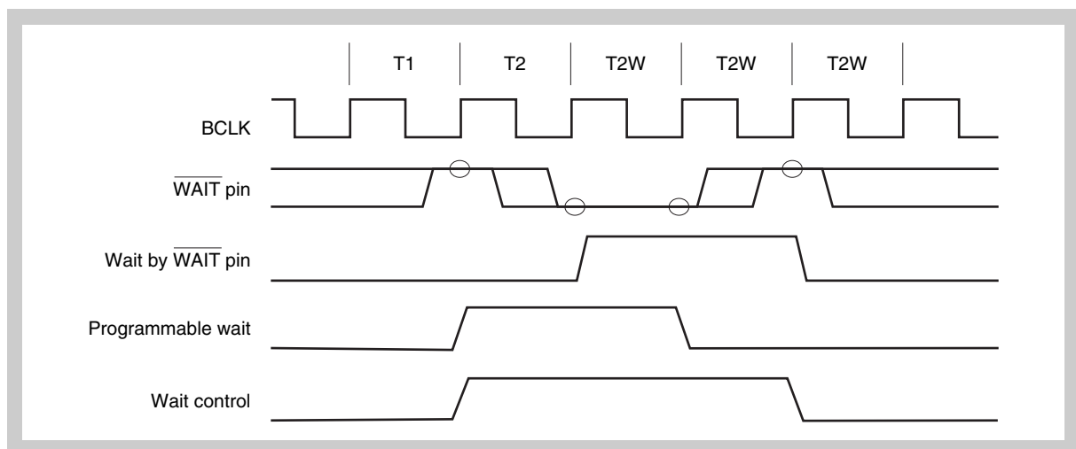
Figure 9-6 Example of wait insertion
