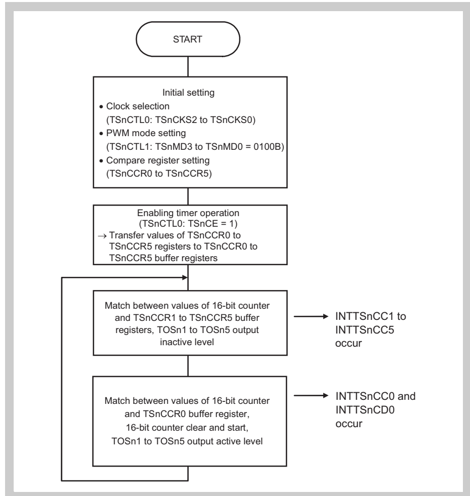
Figure 17-63 Basic operation flow in PWM mode (1/2)
