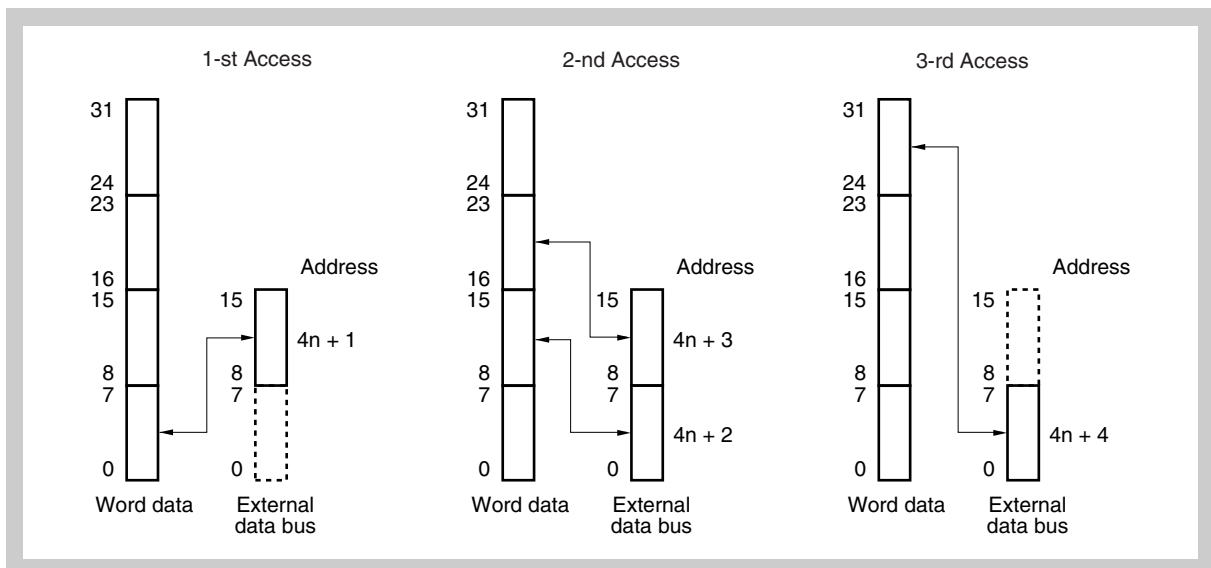
Figure 9-32 Access to address 4n + 1
