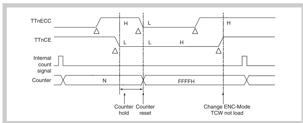
Figure 18-42 Counter hold through bit TTnECC timings (3/8) When setting value of bit TTnECC is rewritten 1 → 0 → 1 while TTnCE = 0
