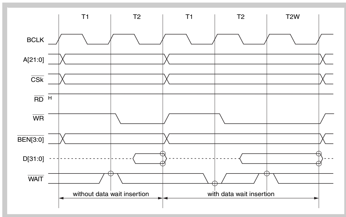
Figure 9-11 Write timing (data wait inserted)
