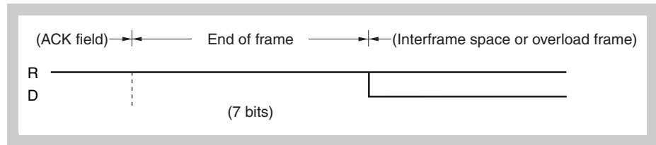
Figure 14-12 End of frame (EOF)
