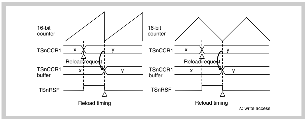
Figure 17-14 Reload request flag operation example
