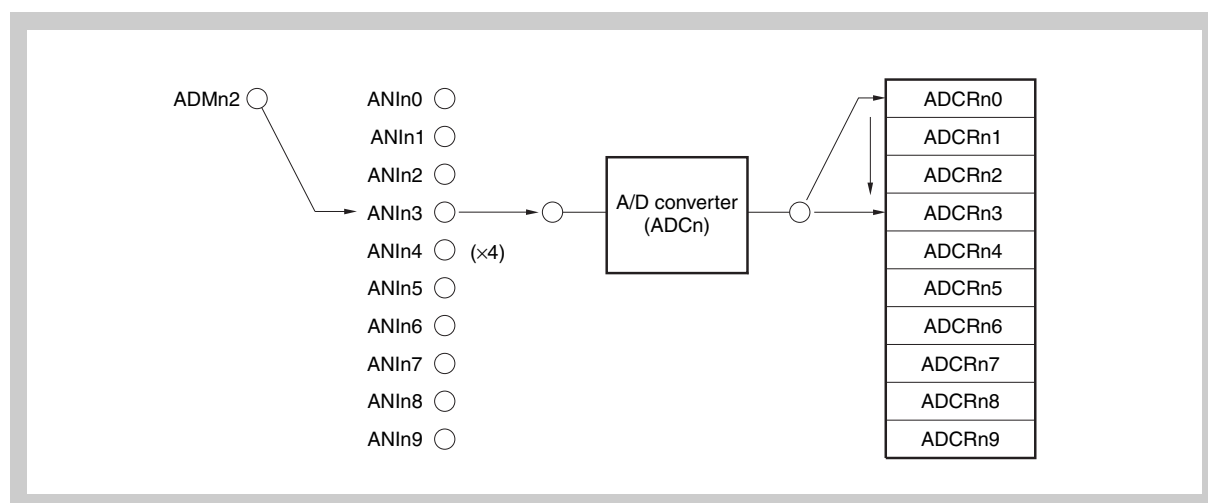
Figure 15-7 Example of 4-buffer mode operation (A/D trigger select: 4 buffers)
