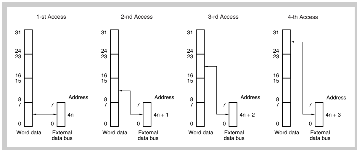
Figure 9-19 Access to address 4n
