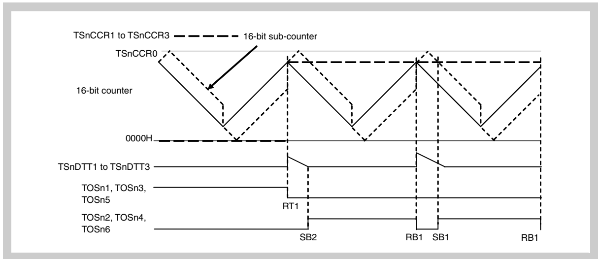
Figure 17-109 TSnCCR1 to TSnCCR3 = 0000H \rightarrow TSnCCR1 to TSnCCR3 = TSnCCR0 - TSnDTC1
