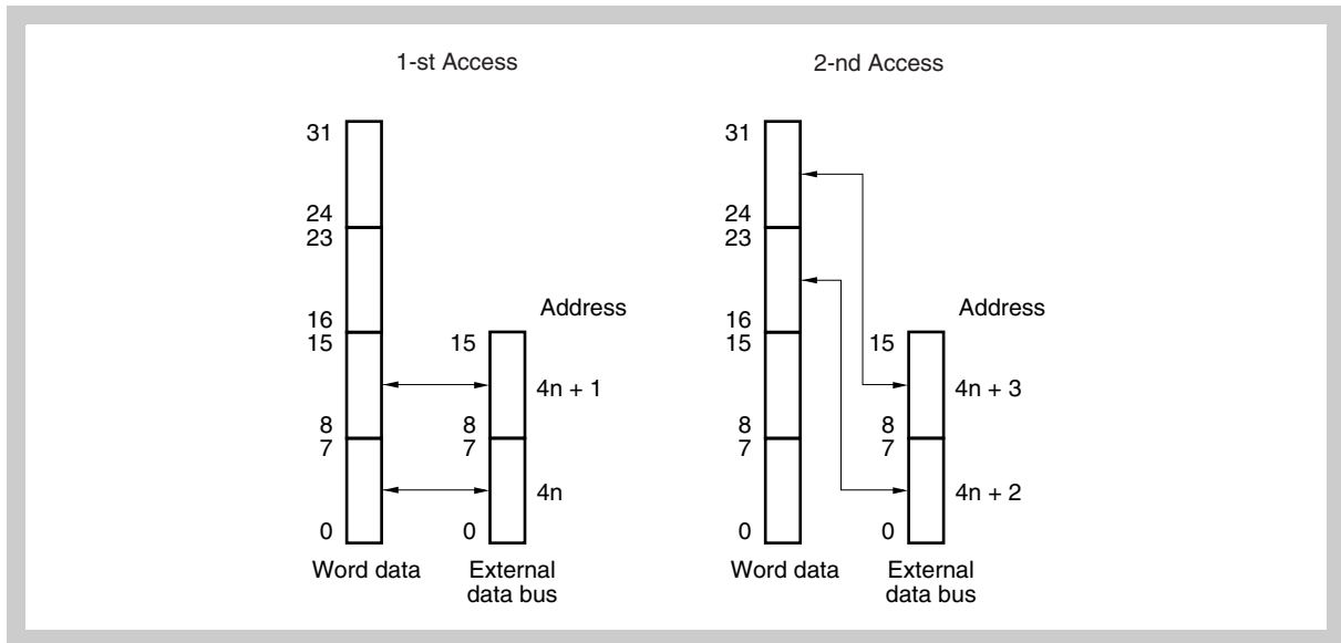
Figure 9-31 Access to address 4n
