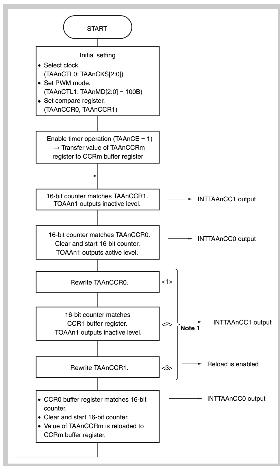
Figure 16-22 Flowchart of basic operation in PWM mode When values of TAA nCCR0, TAA nCCR1 registers are rewritten during timer operation
