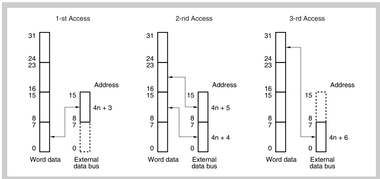
Figure 9-34 Access to address 4n + 3
