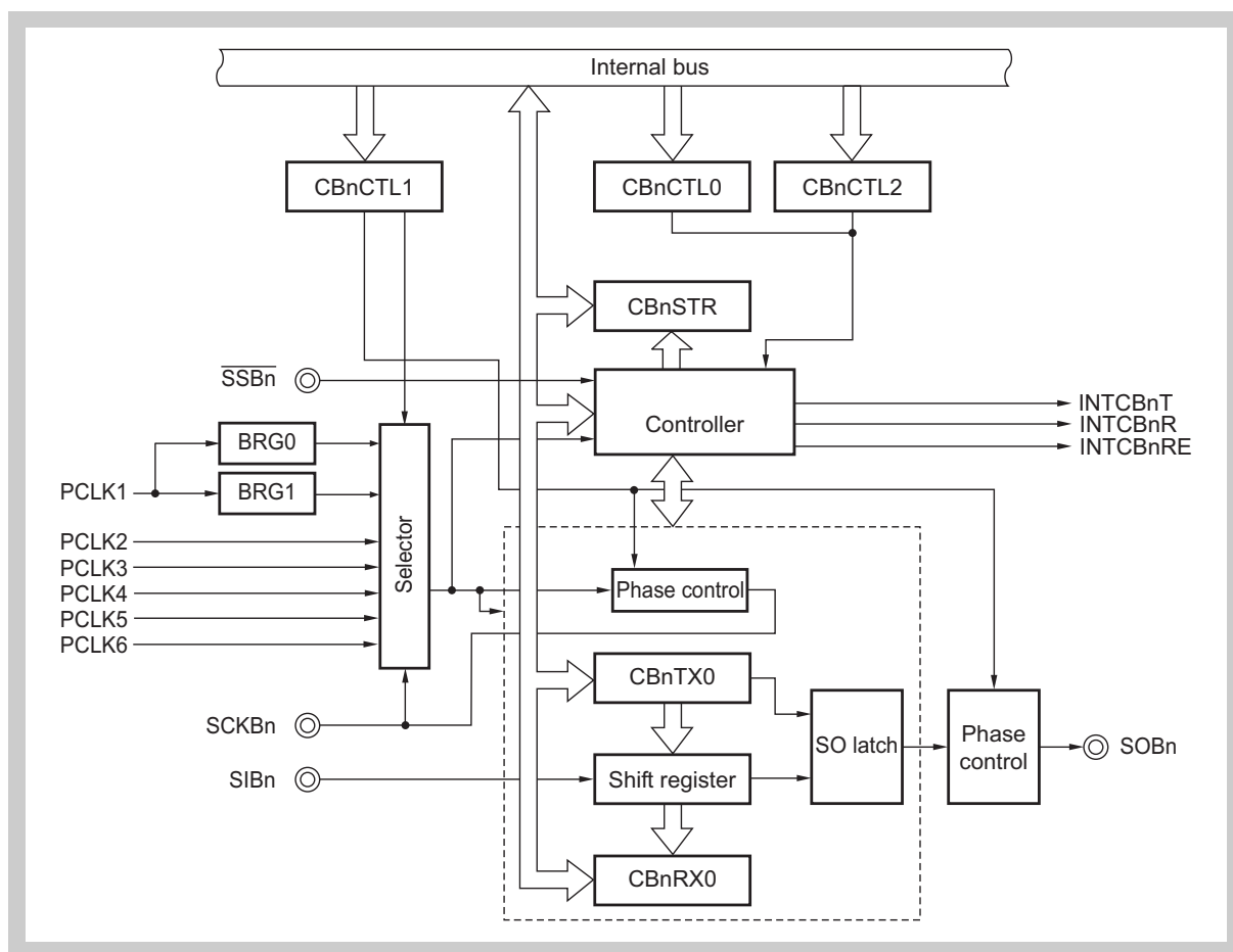
Figure 12-1 Block diagram of CSIBn
