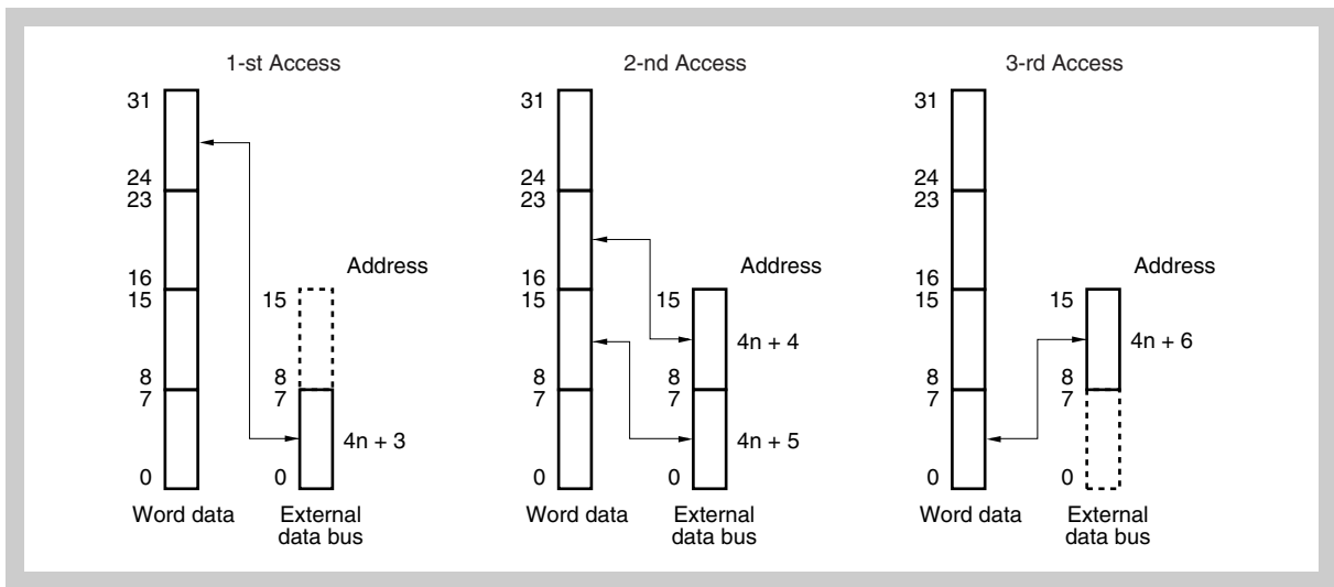
Figure 9-38 Access to address 4n + 3
