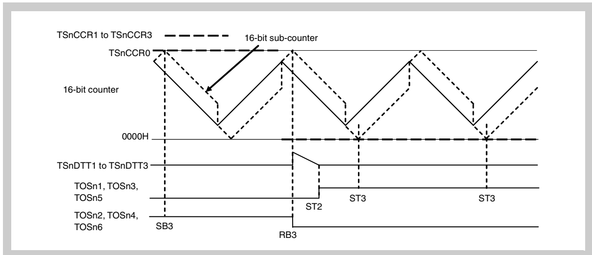
Figure 17-106 TSnCCR1 to TSnCCR3 = TSnCCR0 \rightarrow TSnCCR1 to TSnCCR3 = 0000H
