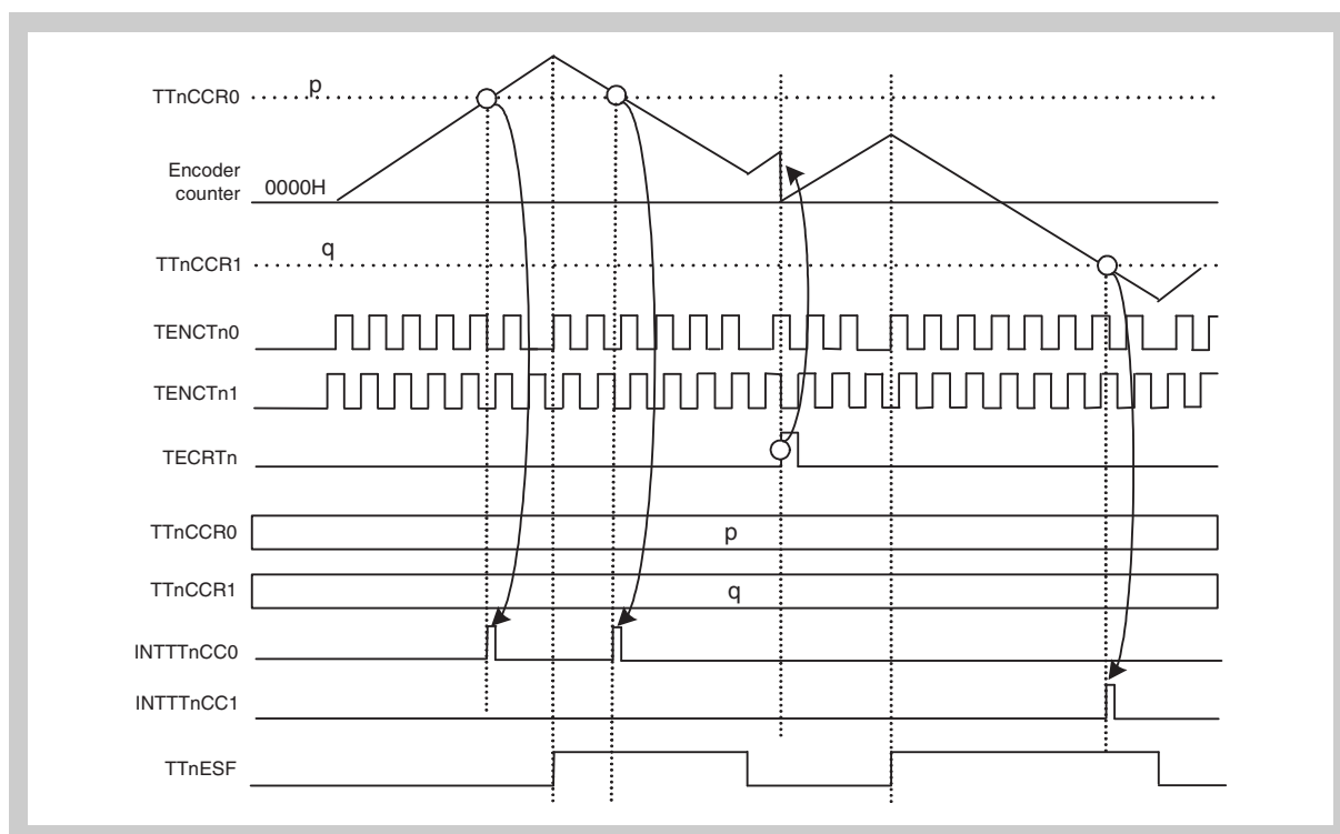
Figure 18-44 Counter hold through bitTTnECC timings (5/8) Basic timing in encoder compare mode (2)
