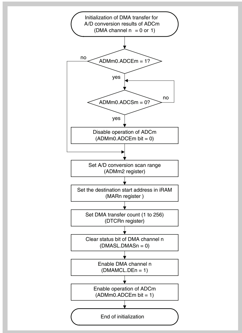
Figure 10-1 Initialization of DMA Channel 0/1 for Transfer of A/D Conversion Results
