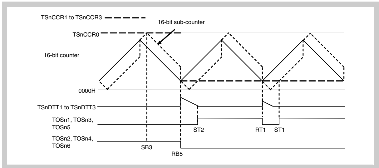
Figure 17-95 TSnCCR1 to TSnCCR3 = TSnCCR0 \rightarrow TSnCCR1 to TSnCCR3 = TSnDTC0, TSnDTC0 + 1
