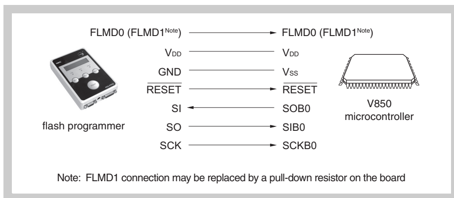
Figure 7-4 Communication with flash programmer via CSI without handshake
