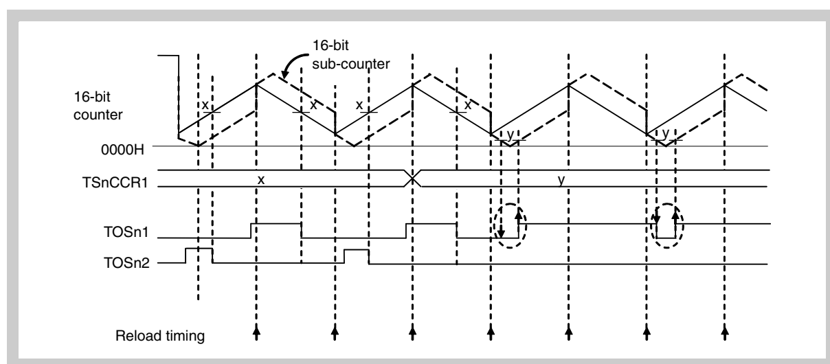
Figure 17-84 Output when rewriting from TSnDTC0 + TSnDTC1 < TSnCCR1 < TSnCCR0 - TSnDTC0 - TSnDTC1 to TSnCCR1 < TSnDTC0 + TSnDTC1
