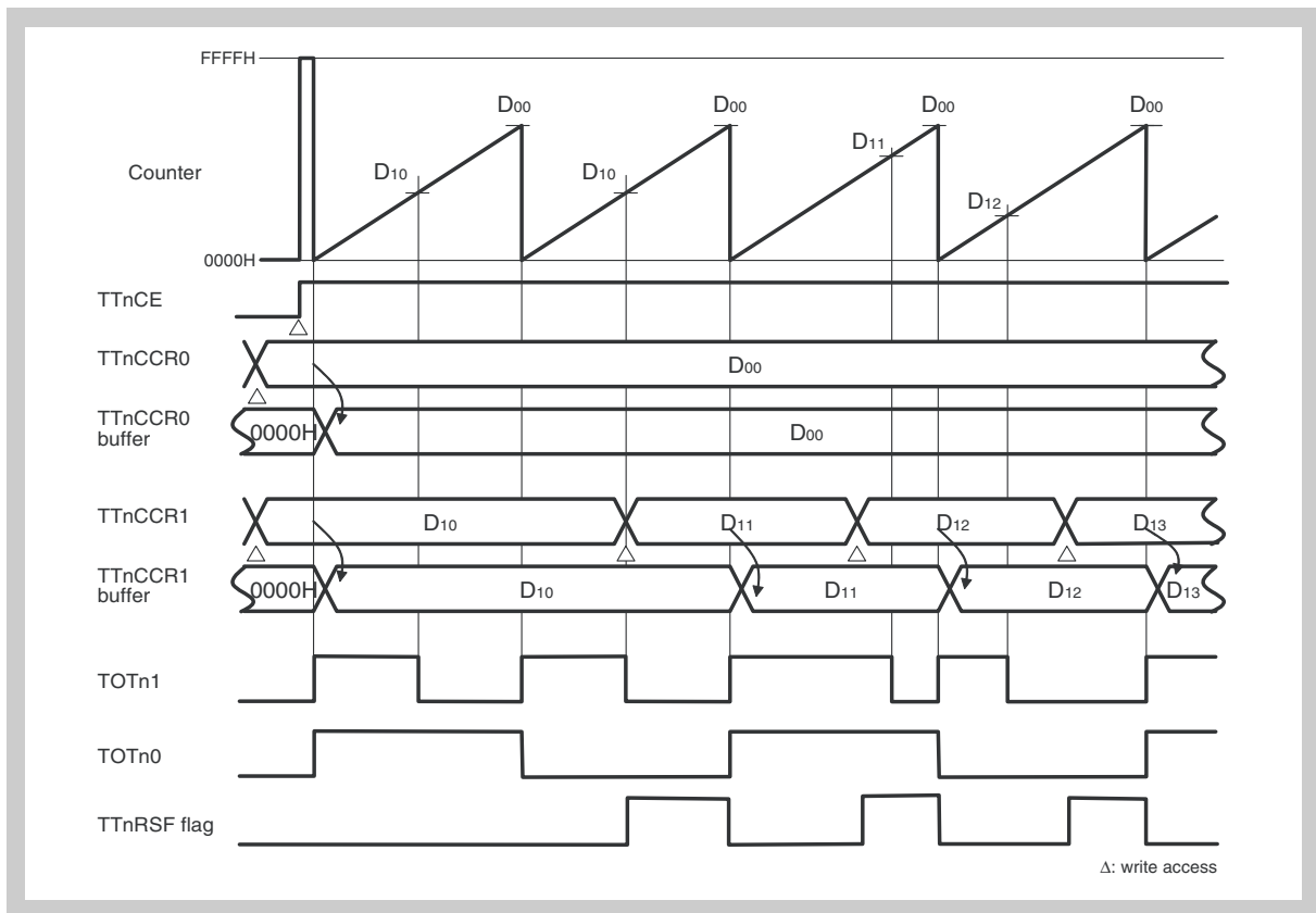
Figure 18-19 Basic operation timing in PWM mode (1/2) When only value of TnCCR1 is rewritten, and TOTn0 and TOTn1 are output (TnOE0, 1 = 1, TnOL0, 1 = 0)
