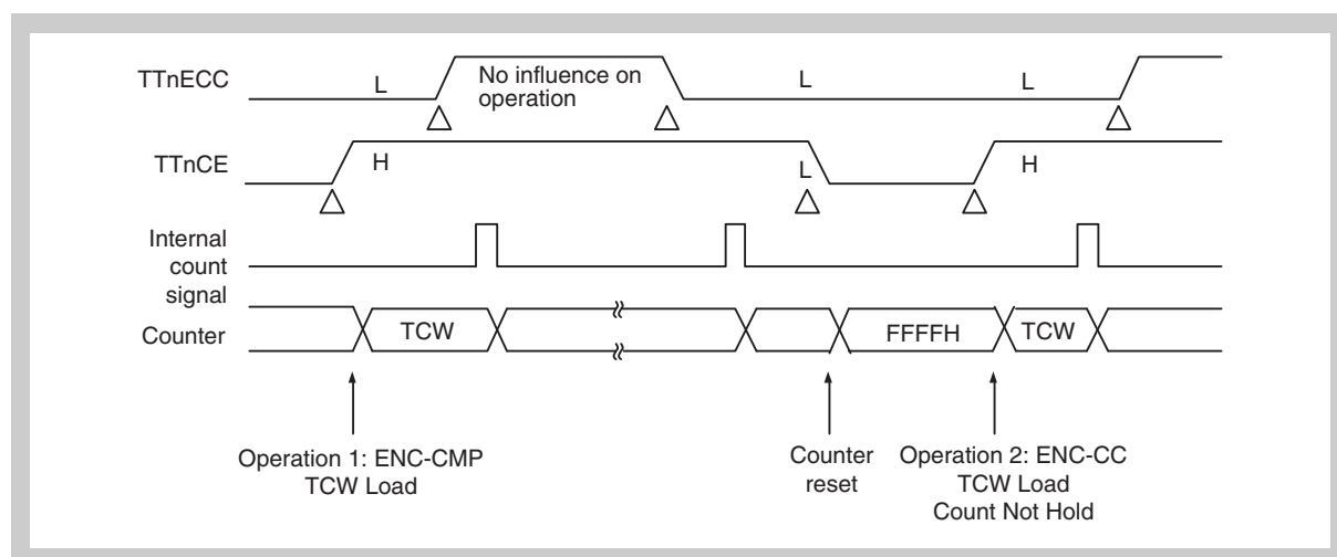
Figure 18-41 Counter hold through bit TTnECC timings (3/8) When setting value of bit TTnECC is rewritten 0 → 1 → 0 when TTnCE = 1
