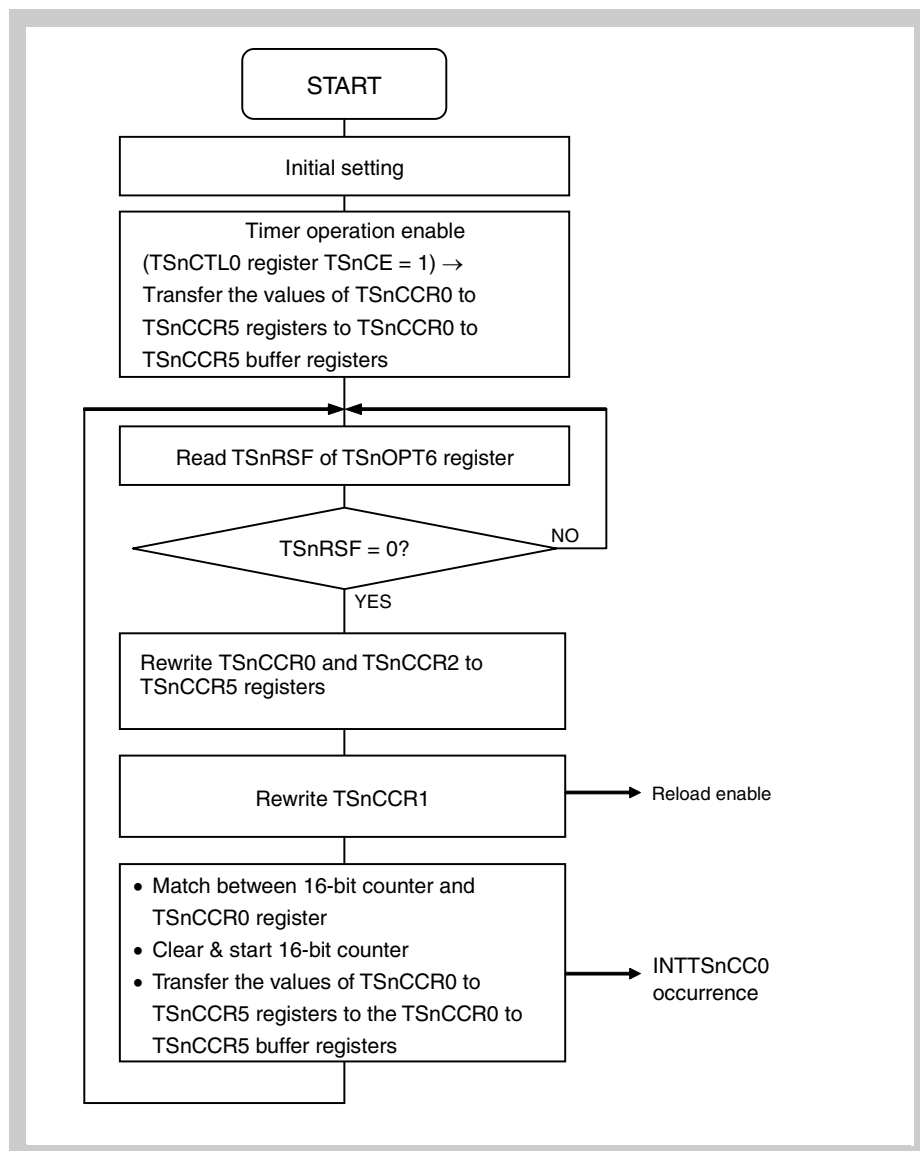
Figure 17-5 Basic operation in reload mode (batch rewrite function) <example in PWM mode>
