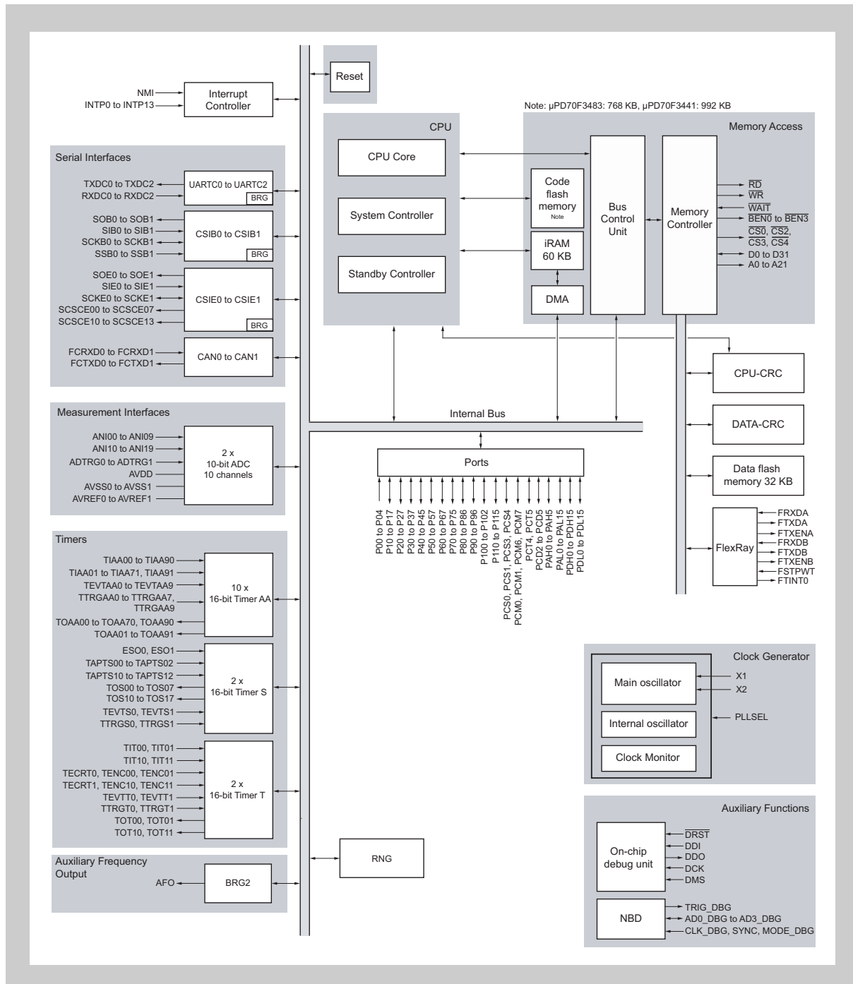
Figure 1-1 V850E/PHO3 block diagram
