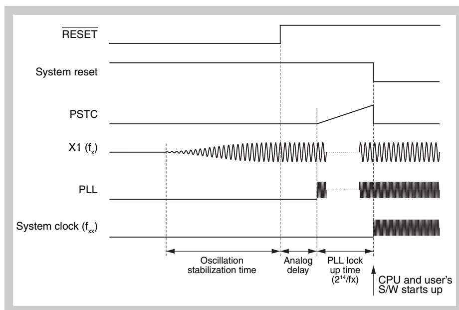
Figure 26-1 Reset timing
