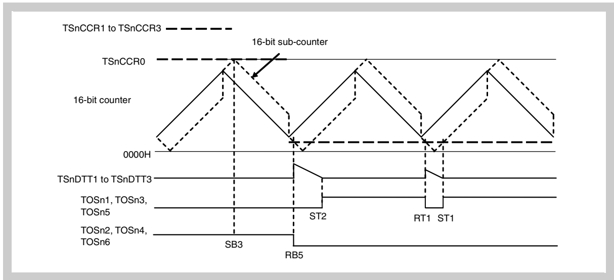
Figure 17-94 TSnCCR1 to TSnCCR3 = TSnCCR0 \rightarrow 0000H < TSnCCR1 to TSnCCR3 < TSnDTC0
