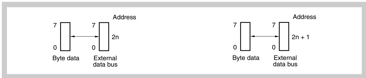
Figure 9-15 Left: Access to even address ( 2n ) Right: Access to odd address ( 2n + 1 )
