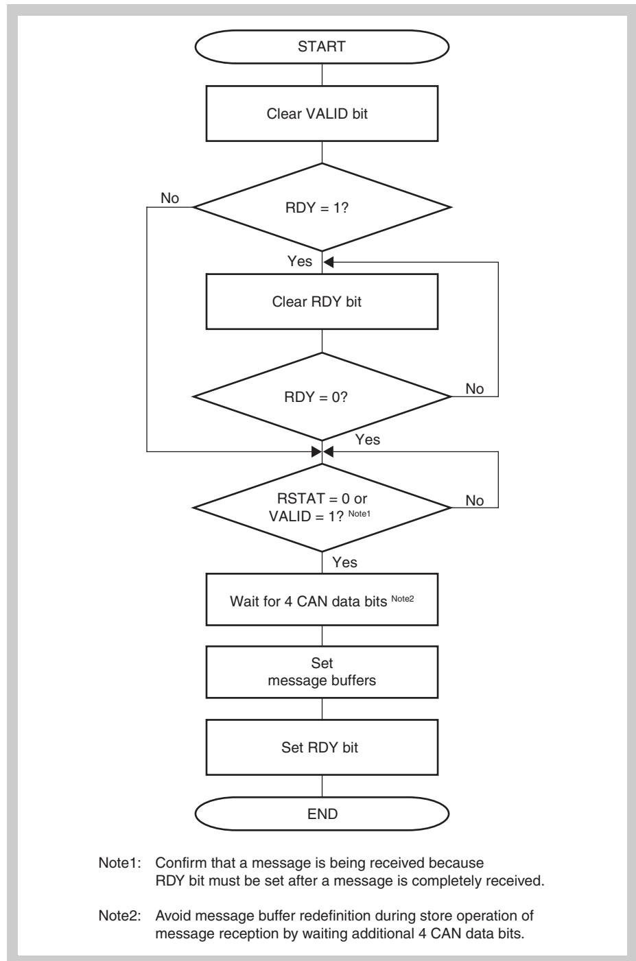
Figure 14-38 Message buffer redefinition
