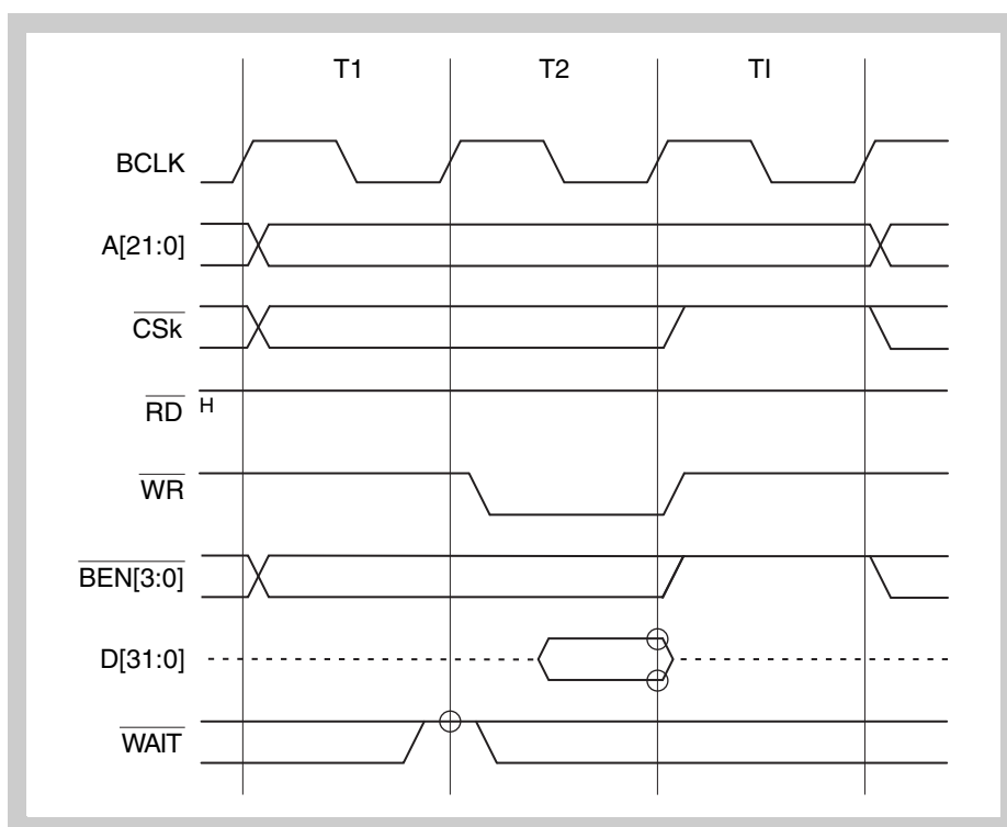
Figure 9-12 Write timing (idle state inserted)
