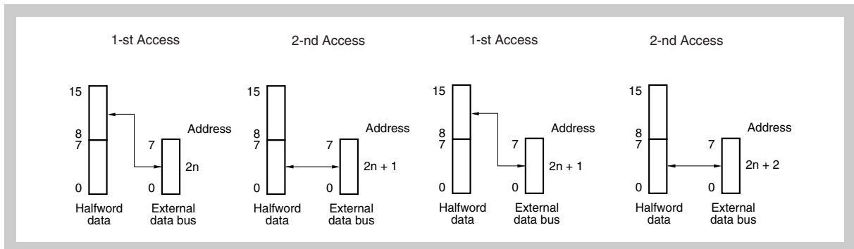
Figure 9-18 Left: Access to even address ( 2n ) Right: Access to odd address ( 2n + 1 )
