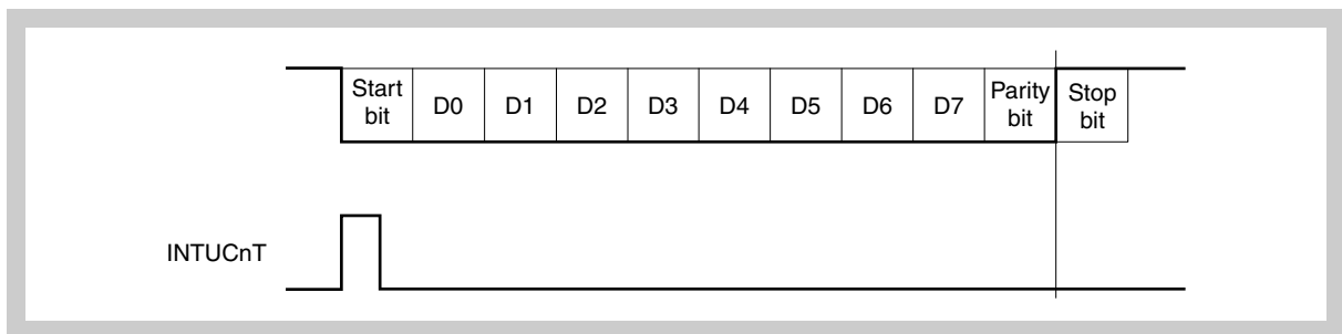
Figure 11-5 UART transmission
