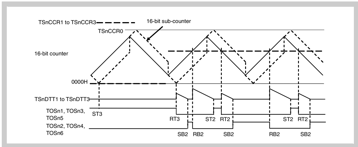
Figure 17-89 TSnCCR1 to TSnCCR3 = 0000H \rightarrow TSnDTC0 \times 2 < TSnCCR1 to TSnCCR3 < TSnCCR0 - TSnDTC1 - TSnDTC0
