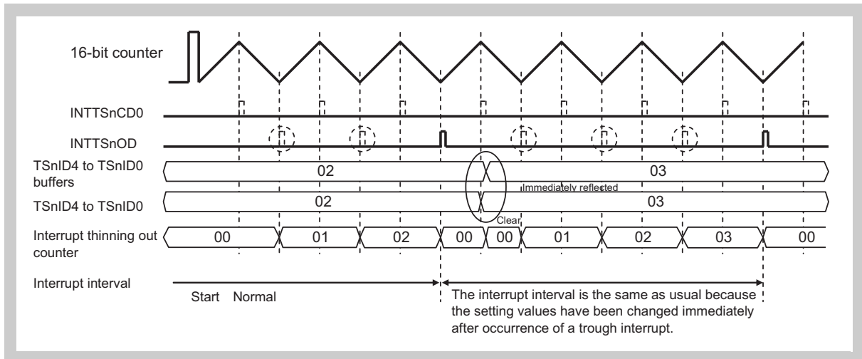
Figure 17-36 When TSnCMS of TSnOPT0 register = 1 and TSnRDE of TSnOPT1 register = x (in anytime rewrite mode)
