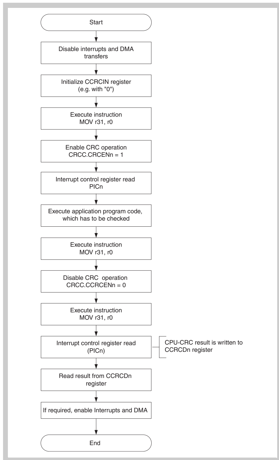
Figure 5-2 CPU-CRC flow diagram
