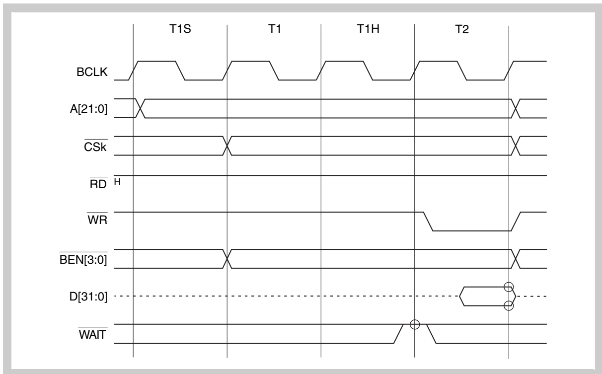
Figure 9-14 Write timing (address setup wait and address hold wait state inserted)
