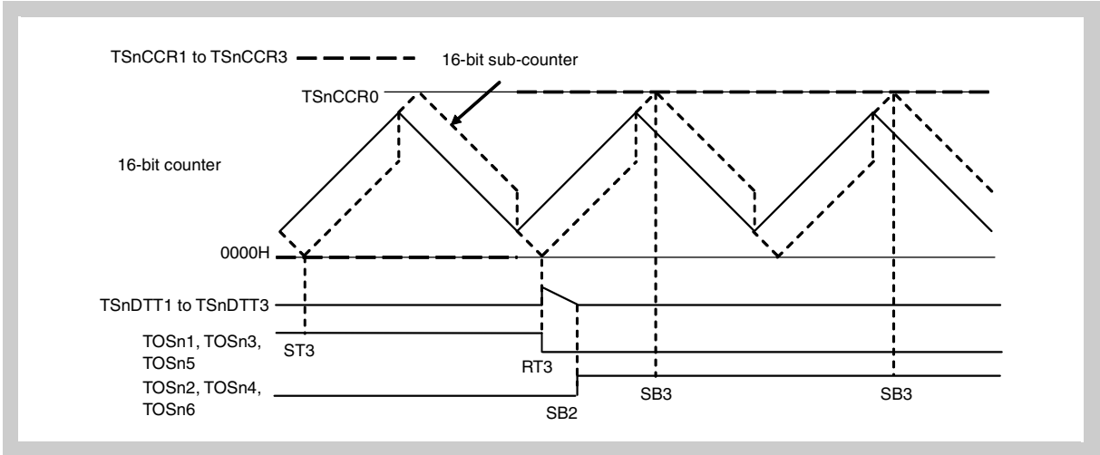
Figure 17-92 TSnCCR1 to TSnCCR3 = 0000H → TSnCCR1 to TSnCCR3 < TSnCCR0
