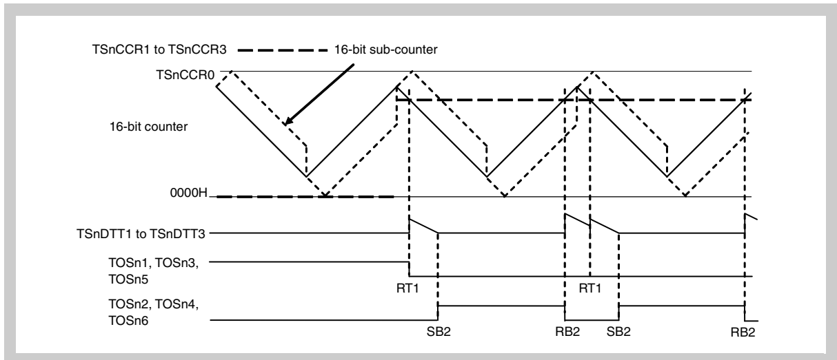
Figure 17-110 TSnCCR1 to TSnCCR3 = 0000H \rightarrow TSnCCR0 - TSnDTC0 - TSnDTC1 < TSnCCR1 to TSnCCR3 < TSnCCR0 - TSnDTC1
