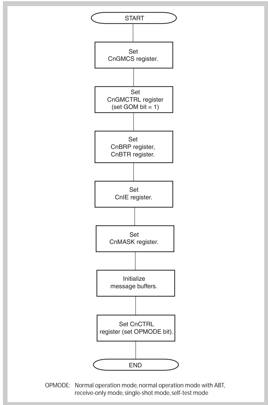
Figure 14-35 Initialization
