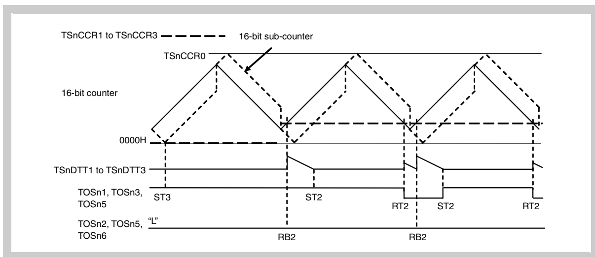
Figure 17-88 TSnCCR1 to TSnCCR3 = 0000H \rightarrow TSnDTC0 < TSnCCR1 to TSnCCR3 < TSnDTC0 \times 2
