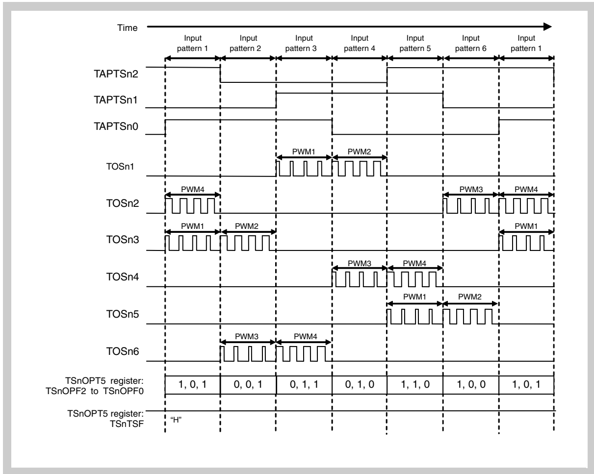
Figure 17-137 120° excitation mode operation example in use of pattern switch method (reverse rotation)
