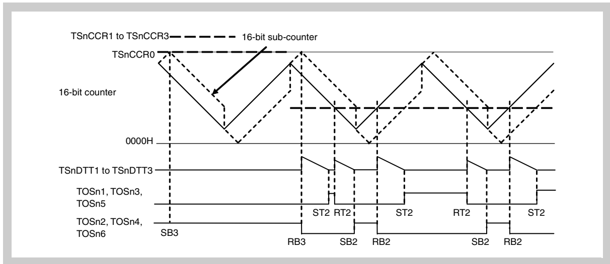
Figure 17-103 TSnCCR1 \text{ to } TSnCCR3 = TSnCCR0 \rightarrow TSnDTC0 + TSnDTC1 < TSnCCR1 to TSnCCR3 < TSnCCR0 - TSnDTC1 \times 2
