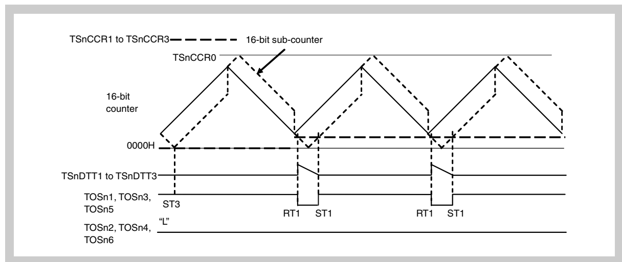
Figure 17-86 TSnCCR1 to TSnCCR3 = 0000H \rightarrow 0000H < TSnCCR1 to TSnCCR3 < TSnDTC0
