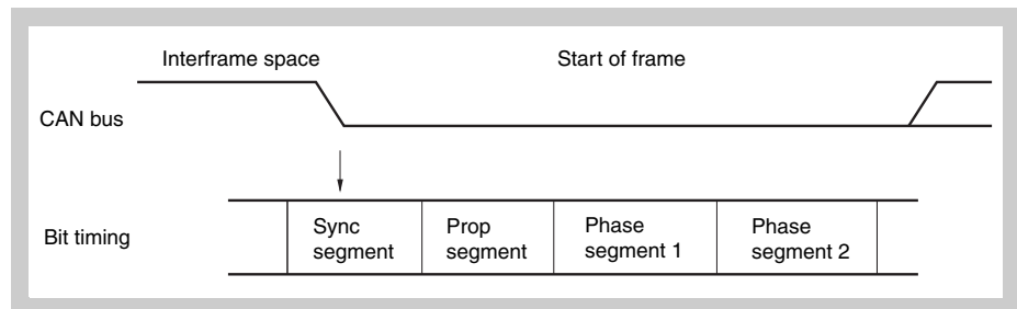
Figure 14-20 Adjusting synchronization of data bit
