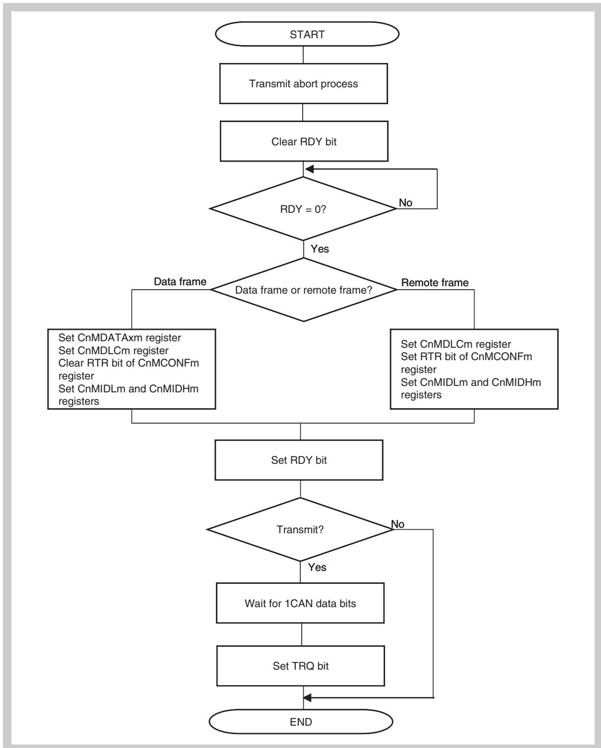
Figure 14-39 Message buffer redefinition during transmission
