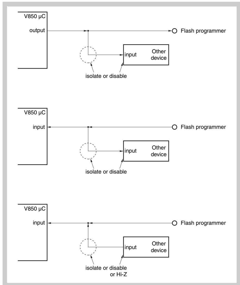
Figure 7-8 Potential conflicts with serial interfaces signals
