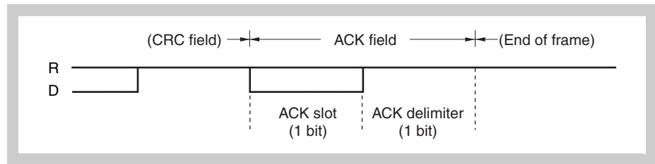
Figure 14-11 ACK field
