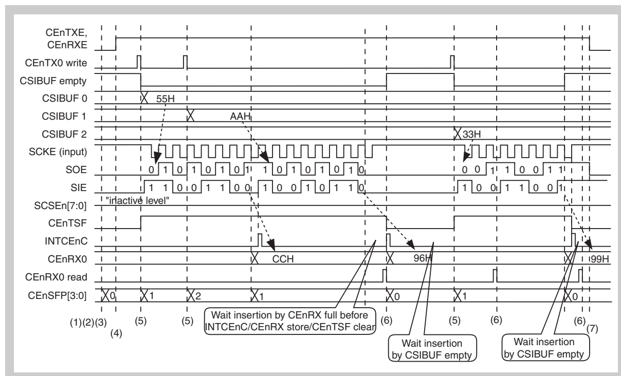
Figure 13-32 Single transfer mode (slave, transmit/receive) timing
