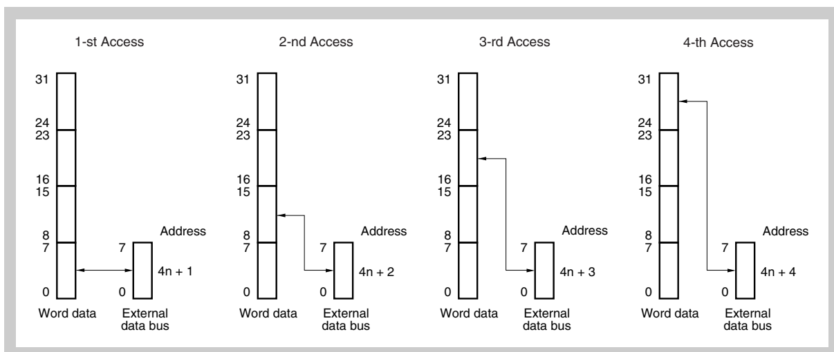
Figure 9-20 Access to address 4n + 1
