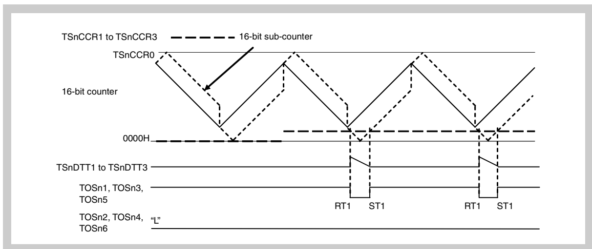
Figure 17-113 TSnCCR1 to TSnCCR3 = 0000H \rightarrow 0000H < TSnCCR1 to TSnCCR3 \leq TSnDTC0 + 1
