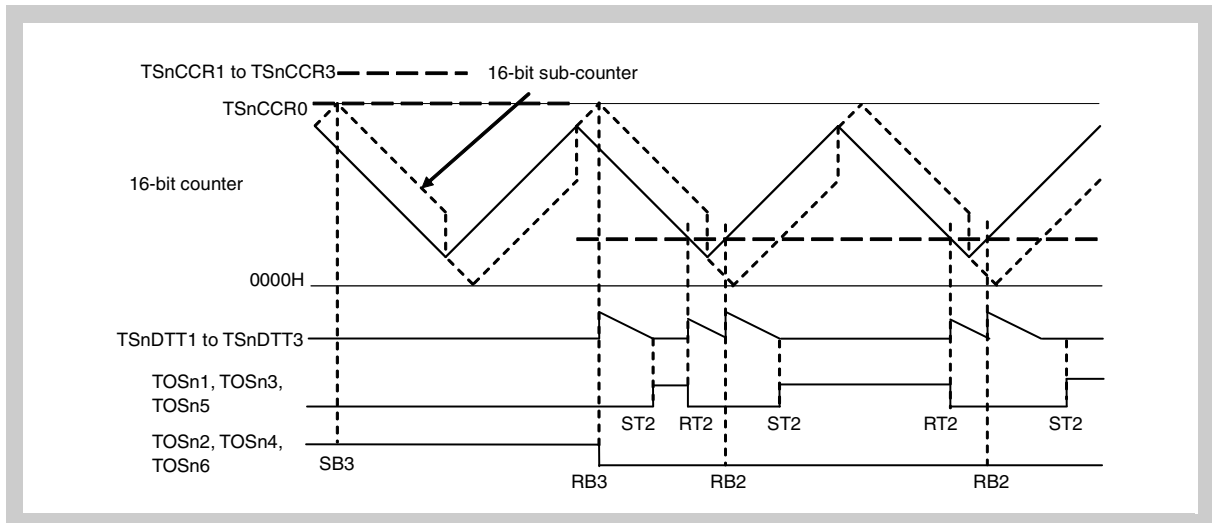
Figure 17-104 TSnCCR1 \text{ to } TSnCCR3 = TSnCCR0 \rightarrow TSnDTC0 + 1 < TSnCCR1 to TSnCCR3 \leq TSnDTC0 + TSnDTC1
