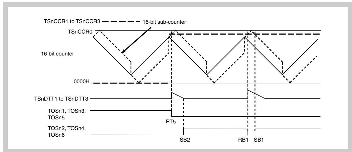
Figure 17-108 TSnCCR1 to TSnCCR3 = 0000H \rightarrow TSnCCR0 - TSnDTC1 < TSnCCR1 to TSnCCR3 < TSnCCR0
