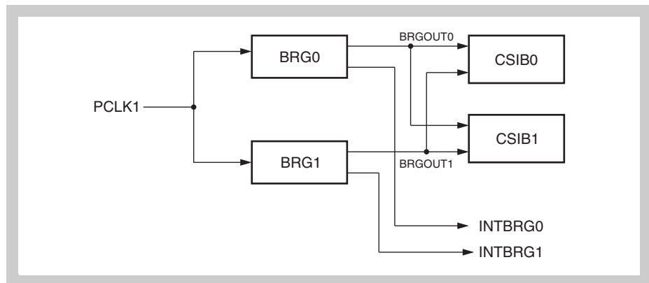
Figure 12-10 Connection between CSIBn and baud rate generators
