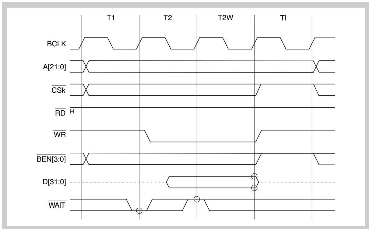
Figure 9-13 Write Timing (data wait, idle state inserted)
