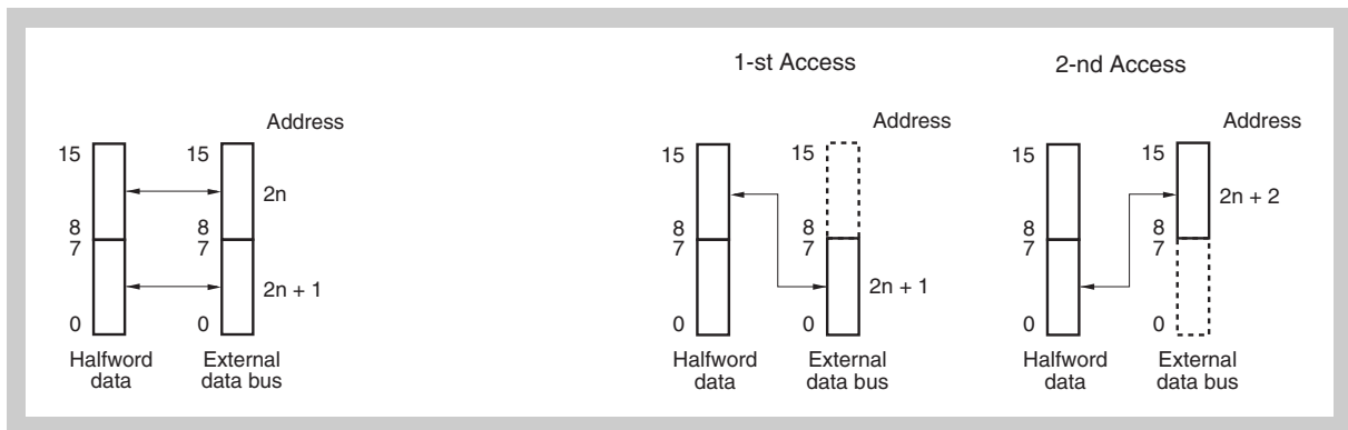
Figure 9-30 Left: Access to even address ( 2n ) Right: Access to odd address ( 2n + 1 )
