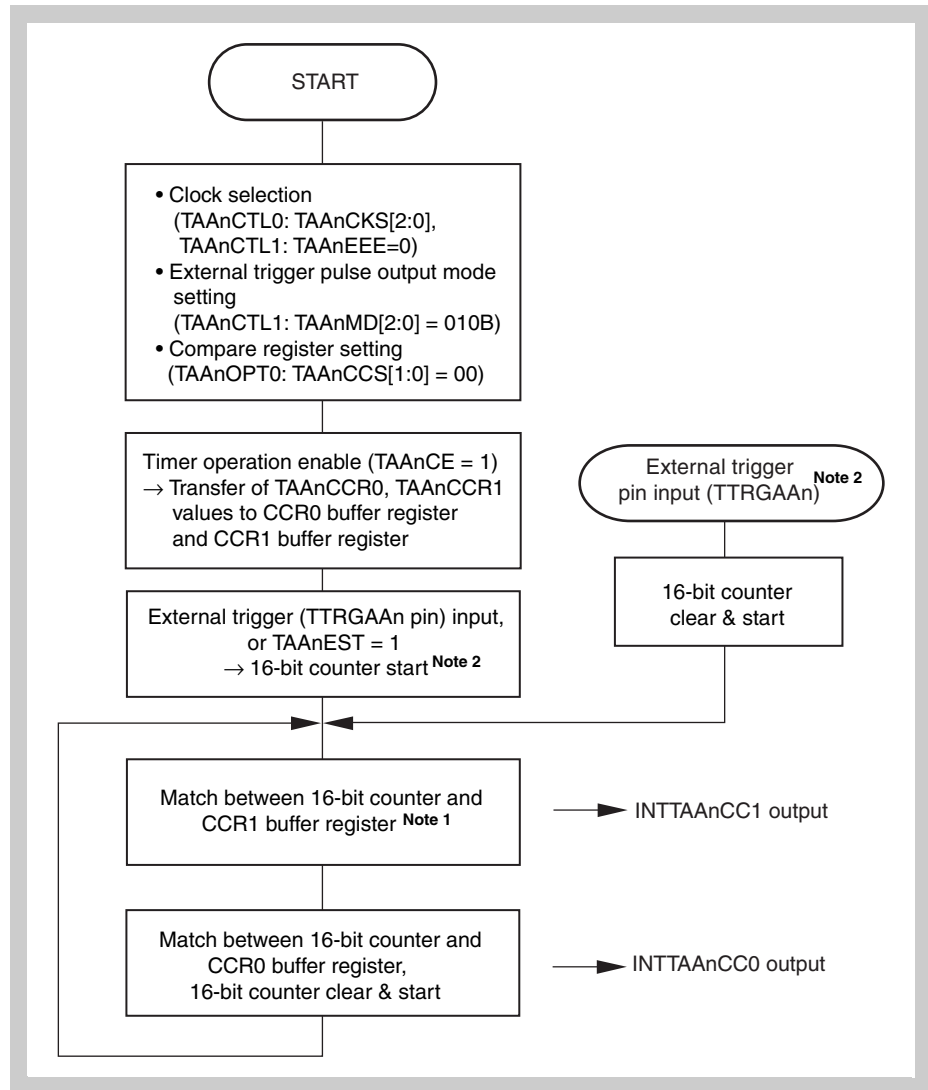
Figure 16-17 Flowchart of basic operation in external trigger pulse output mode
