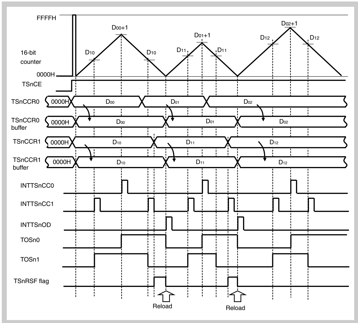
Figure 17-73 Basic operation timing in triangular-wave PWM mode
