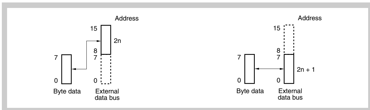
Figure 9-28 Left: Access to even address ( 2n ) Right: Access to odd address ( 2n + 1 )
