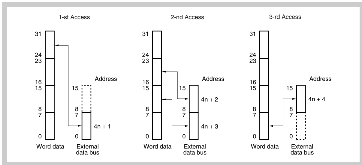
Figure 9-36 Access to address 4n + 1
