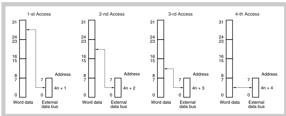
Figure 9-24 Access to address 4n + 1
