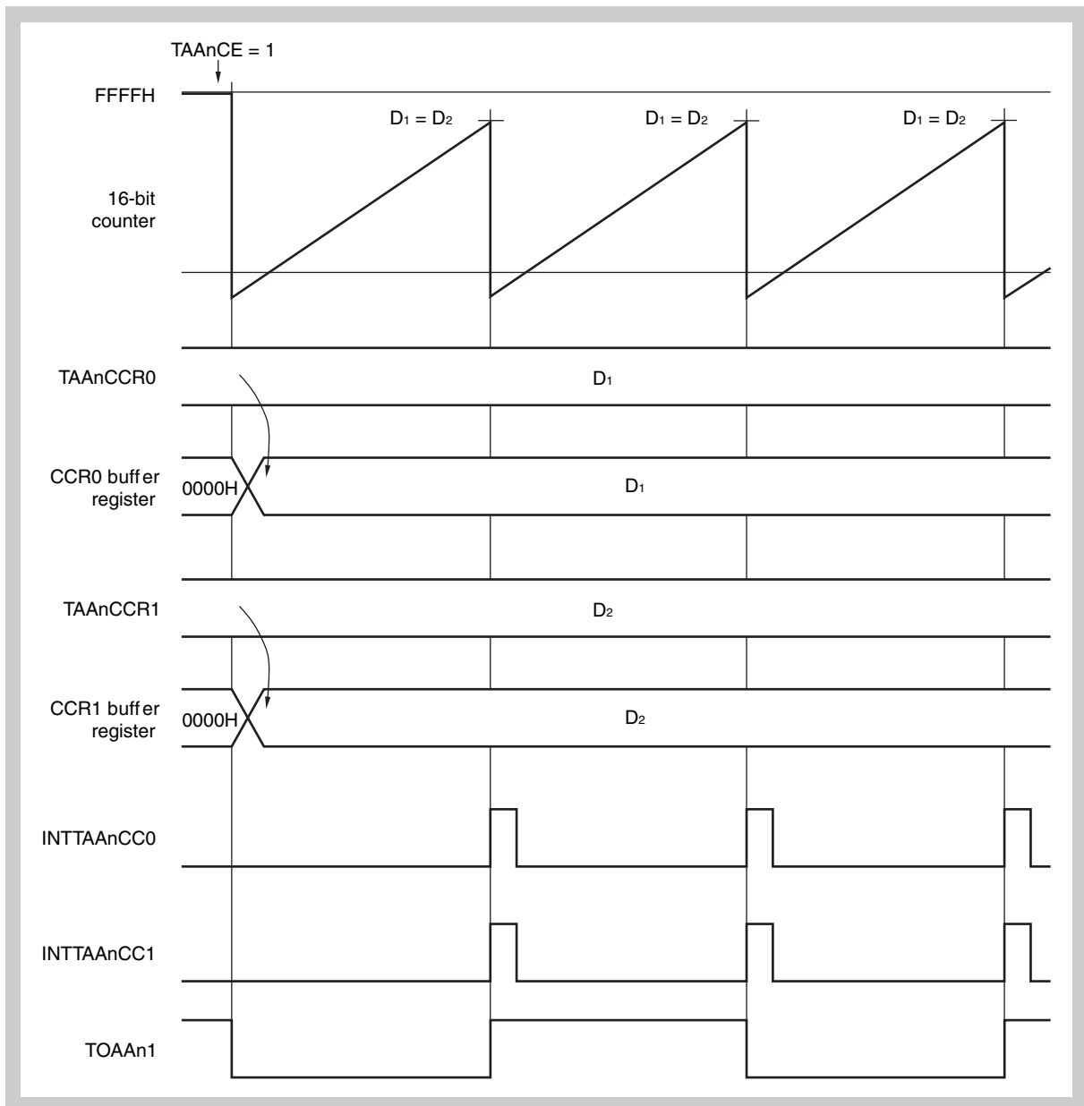
Figure 16-16 Basic operation timing in external event counter mode When D_1 = D_2 ; TAAAnCCR0 and TAAAnCCR1 are not rewritten, TOAAAn1 is output (TAAAnOE0 = 1, TAAAnOE1 = 1, TAAAnOL0 = 0, TAAAnOL1 = 1)
