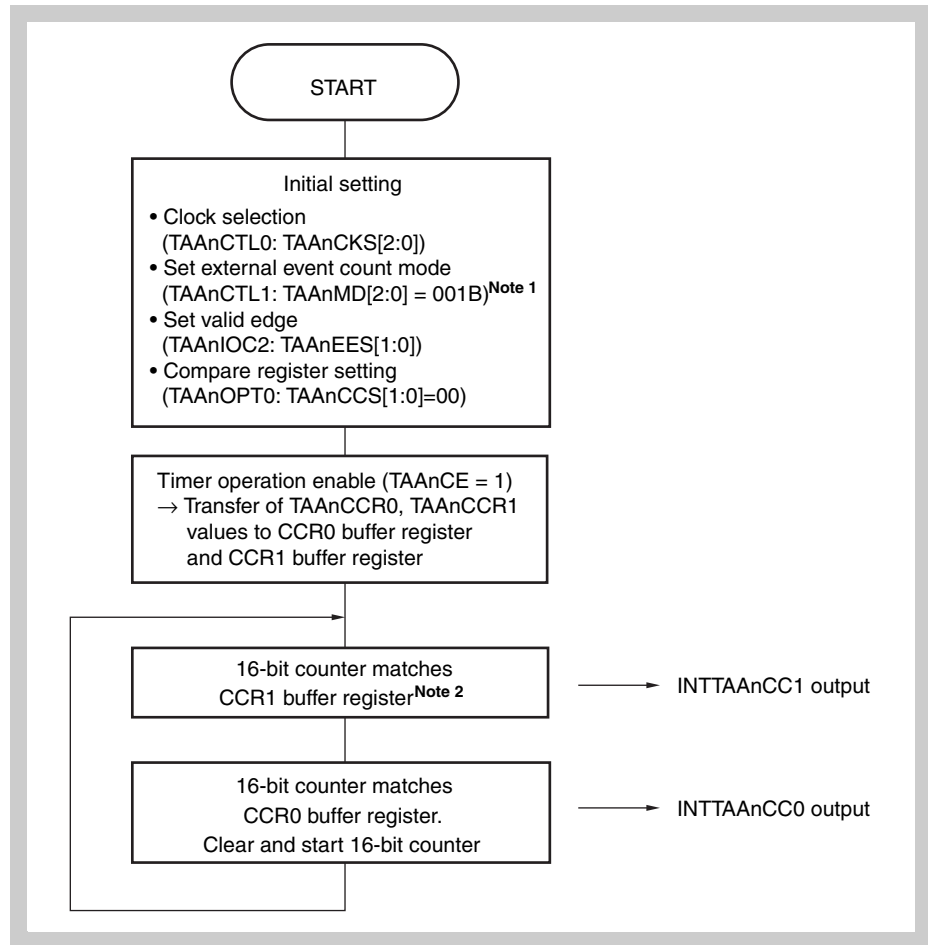
Figure 16-14 Flowchart of basic operation in external event counter mode
