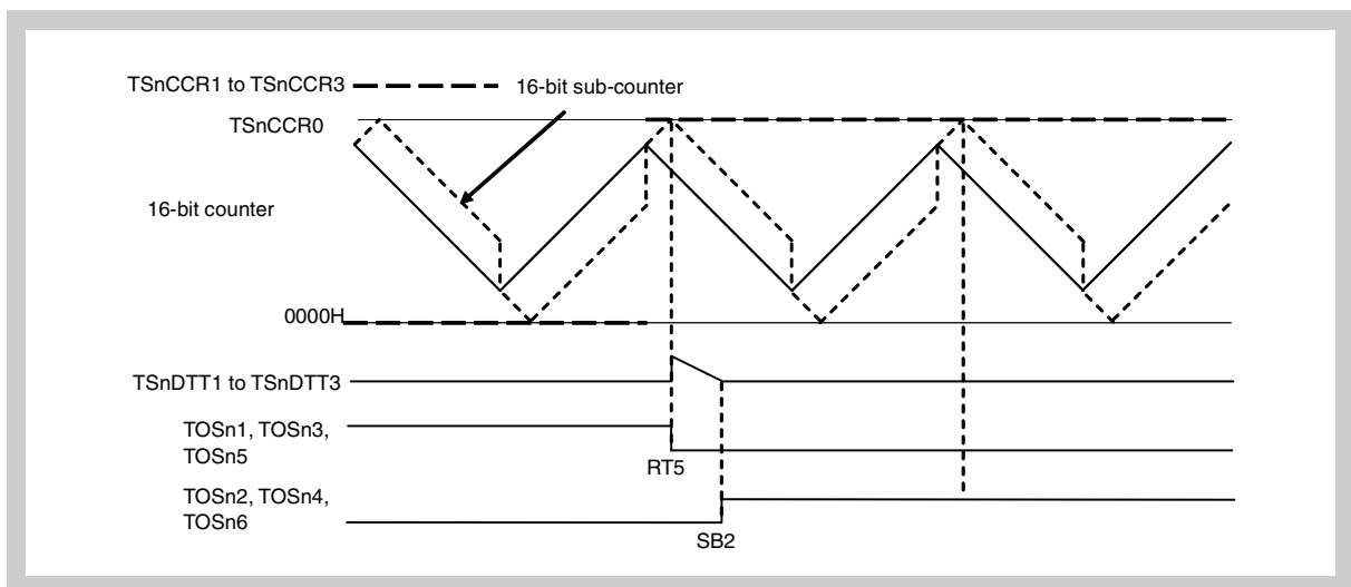
Figure 17-107 TSnCCR1 to TSnCCR3 = 0000H \rightarrow TSnCCR1 to TSnCCR3 = TSnCCR0
