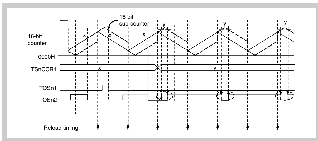
Figure 17-85 Output when rewriting from “ TSnDTC0 + TSnDTC1 < TSnCCR1 < TSnCCR0 - TSnDTC0 - TSnDTC1 ” to “ TSnCCR0 - TSnDTC1 + 1 < TSnCCR1 < TSnCCR0 ”
