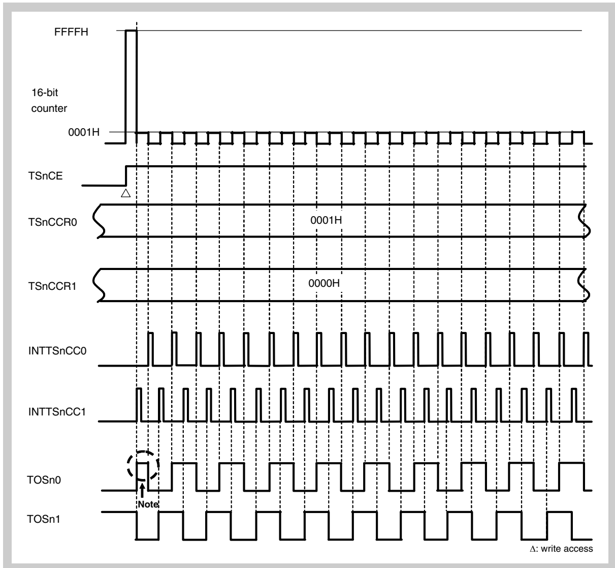
Figure 17-58 Basic operation timing in external event count mode (4/4)
