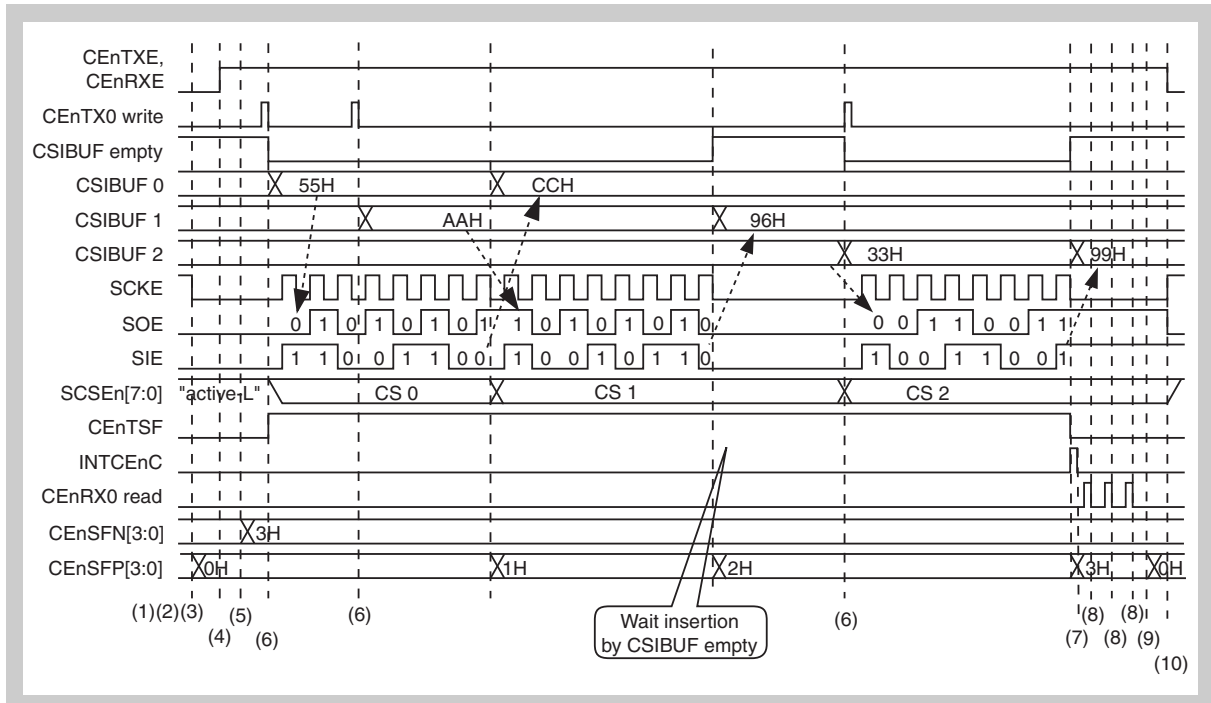
Figure 13-35 Block transfer mode (master, transmit/receive) timing
