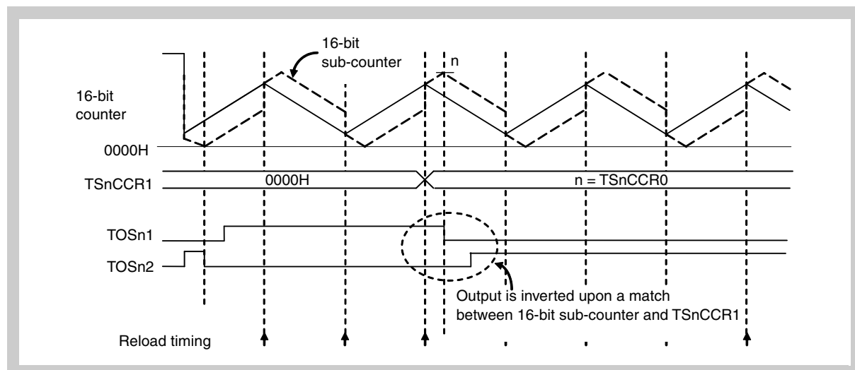
Figure 17-83 Output when rewriting from TSnCCR1 = 0000H to TSnCCR1 = TSnCCR0
