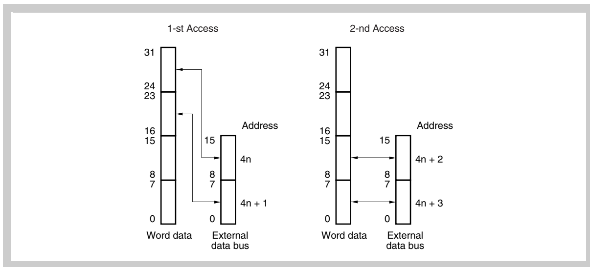
Figure 9-35 Access to address 4n
