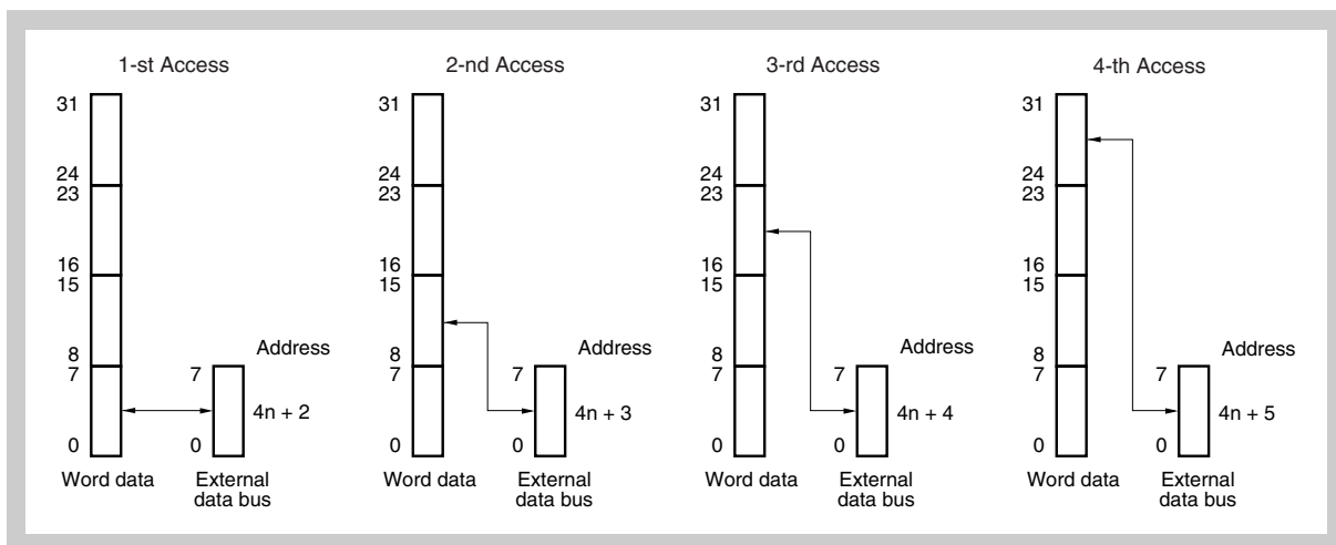
Figure 9-21 Access to address 4n + 2
