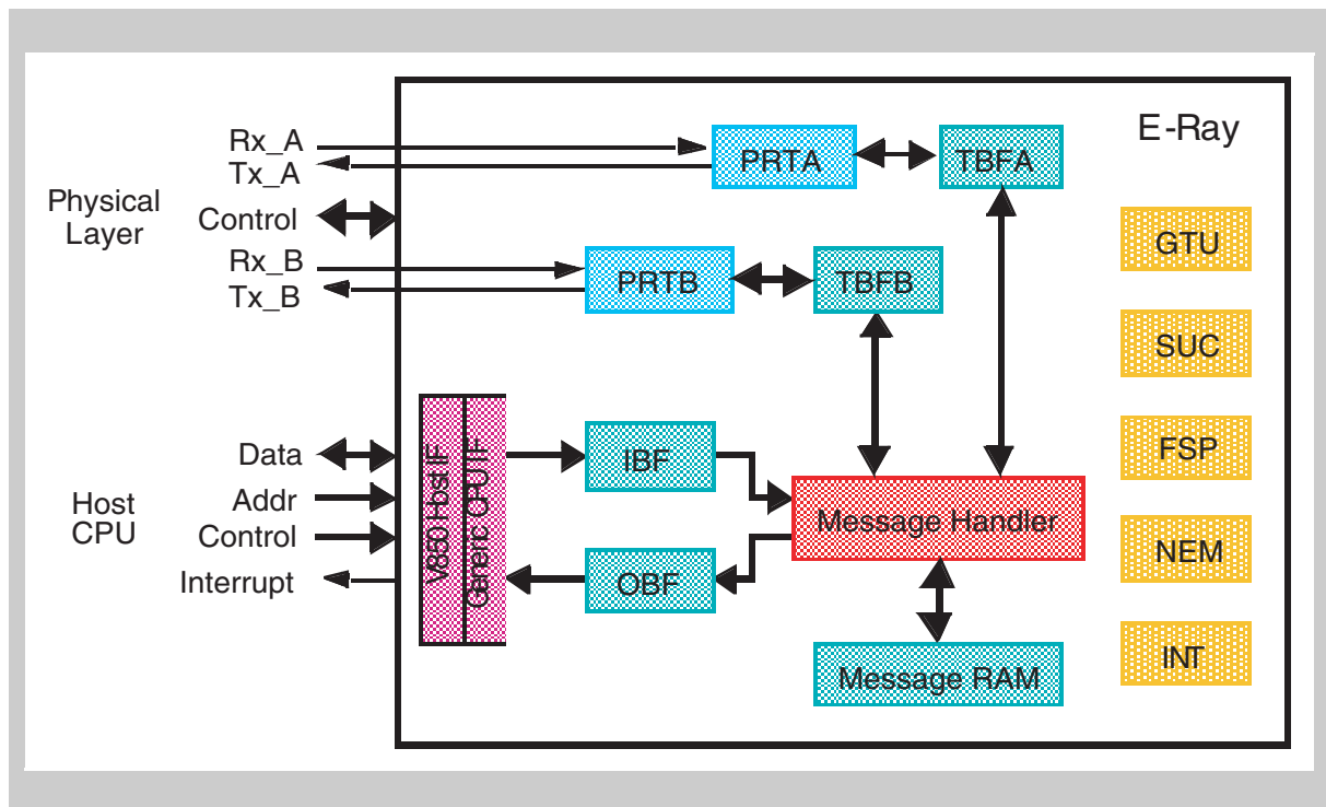
Figure 24-1 E-Ray block diagram
