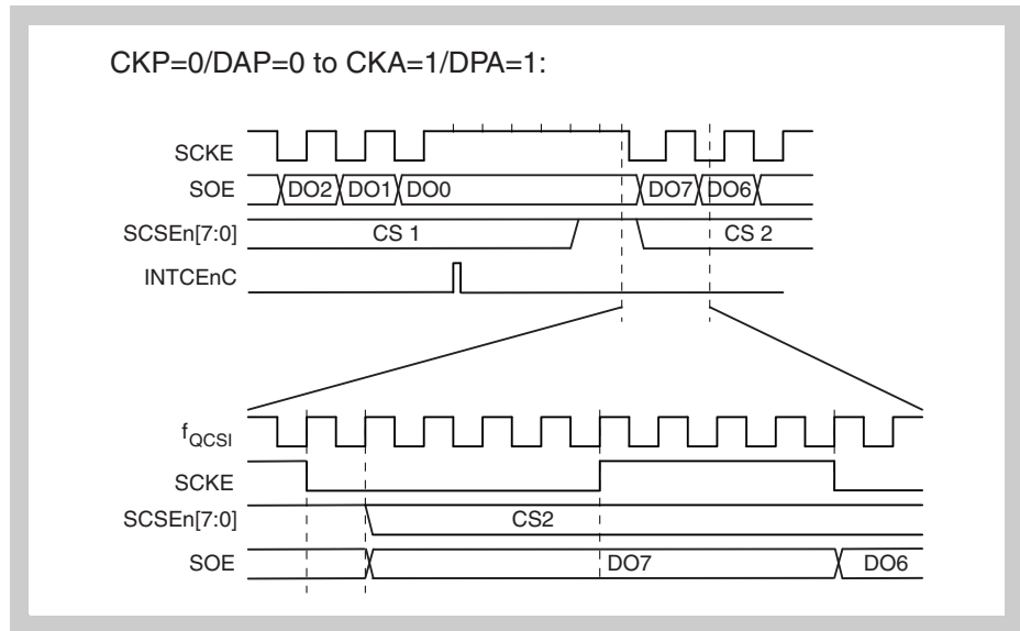
Figure 13-24 CKP=0, DAP=0 to CKA=1, DPA=1 with enhanced timing
