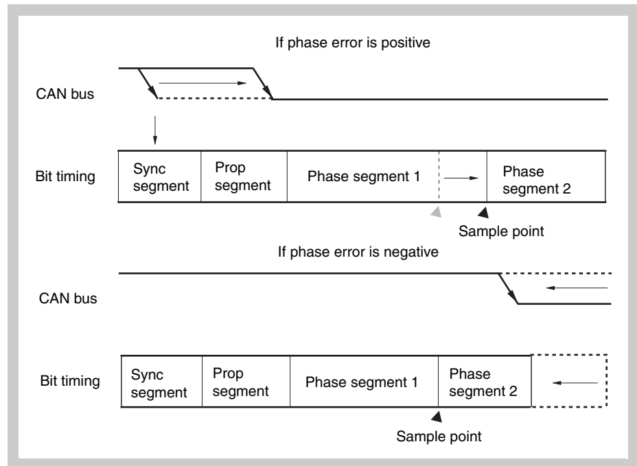
Figure 14-21 Resynchronization
