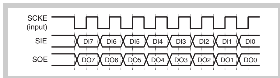
Figure 13-7 Slave mode
