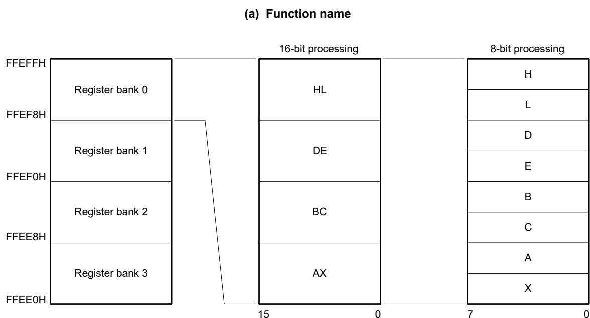
Figure 3-16. Configuration of General-Purpose Registers
