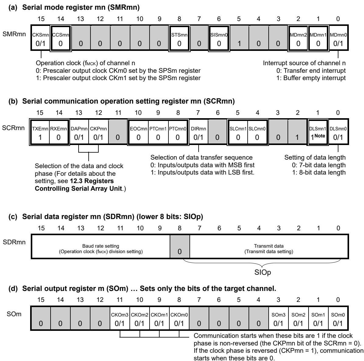
Figure 12-25. Example of Contents of Registers for Master Transmission of Simplified SPI (CSI00, CSI01, CSI10, CSI11, CSI20, CSI21, CSI30, CSI31) (1/2)
