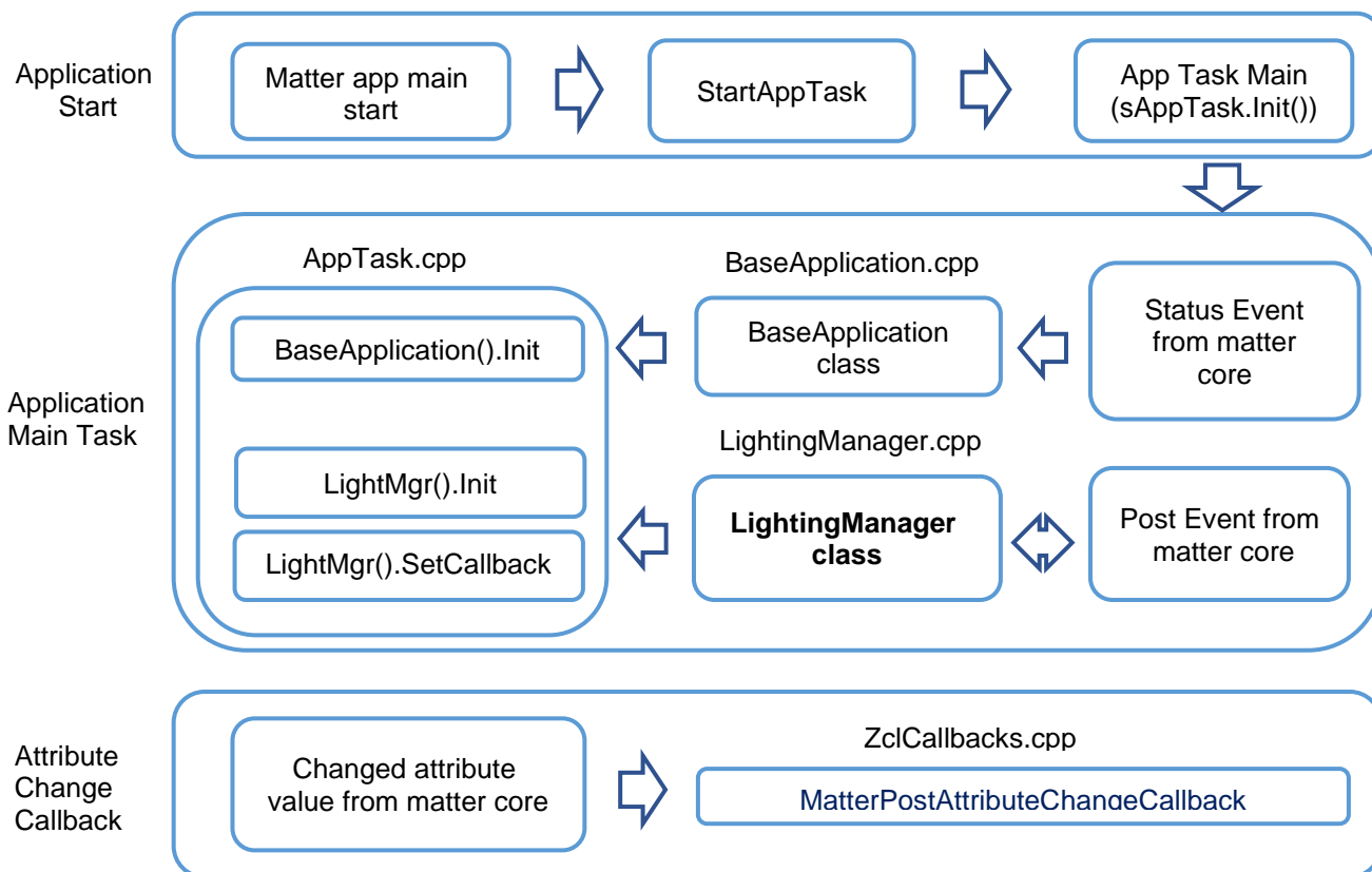
Figure 37: Lighting application structure
