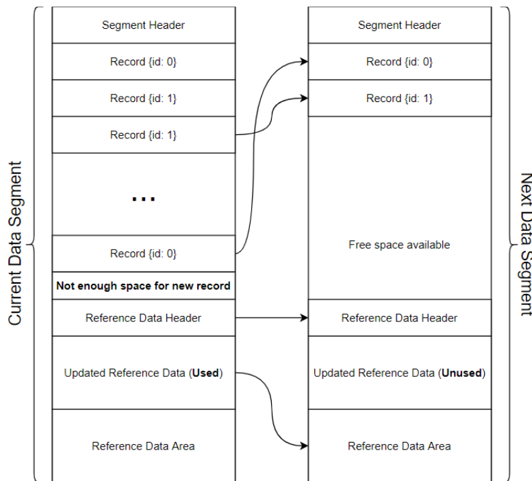
Figure 295: Refresh Operation
