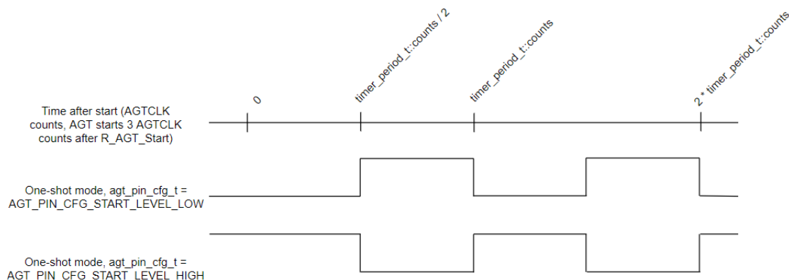
Figure 308: AGT Periodic Output
