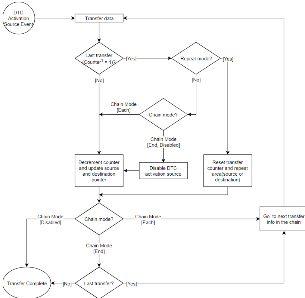
Figure 312: DTC Transfer Flowchart
