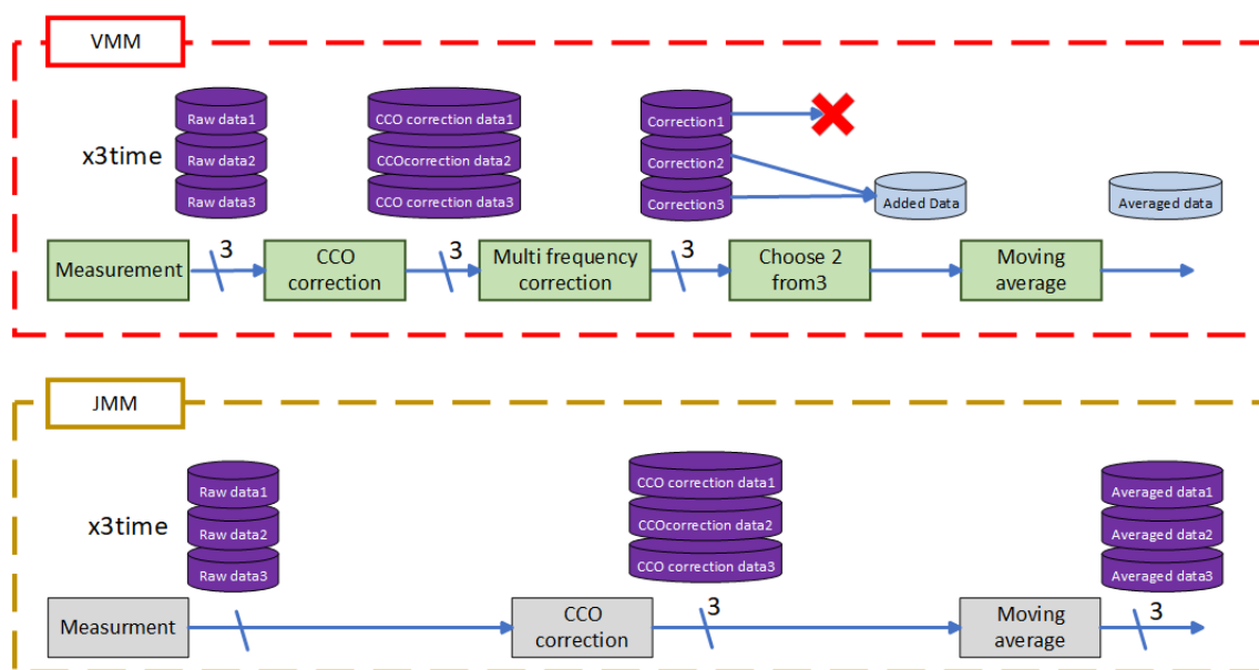
Figure 157: Data flow Comparison of JMM and VMM
