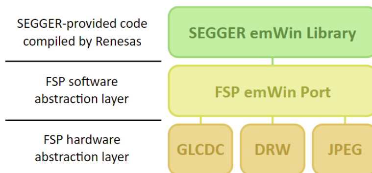
Figure 231: SEGGER emWin FSP Port Block Diagram (using RA6M3 as example)
