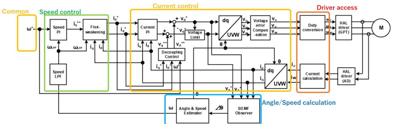
Figure 233: Image of Current Control Module(yellow block)
