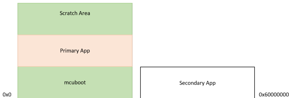
Figure 156: MCUboot Memory Map with QSPI
