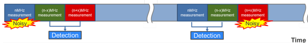
Figure 159: Multi-frequency Measurements
