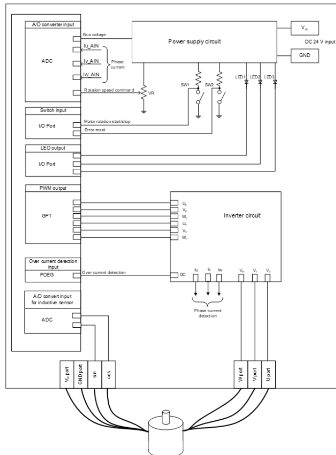
Figure 273: Example of target hardware of motor induction module
