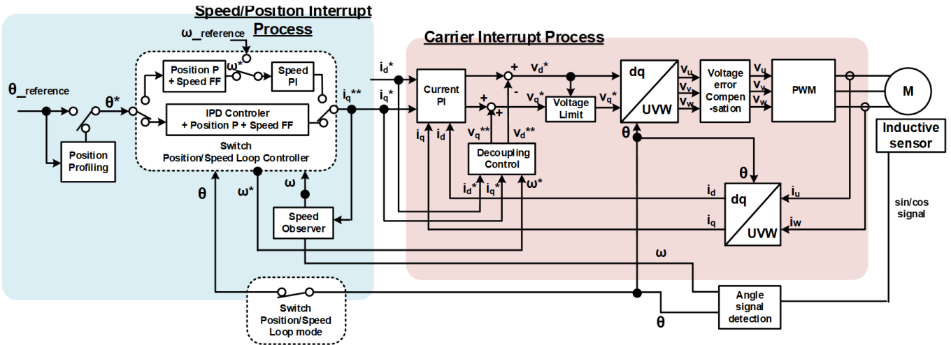
Figure 274: Block diagram of vector control with using induction sensor (PI feedback loop)
