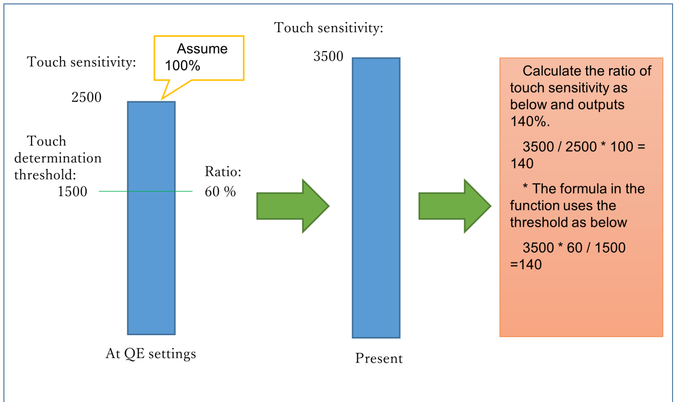
Figure 171: Example of increase touch sensitivity for thin overlay panels
