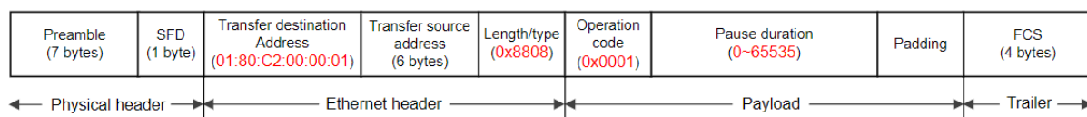
Figure 288: Pause Frame Format Image
