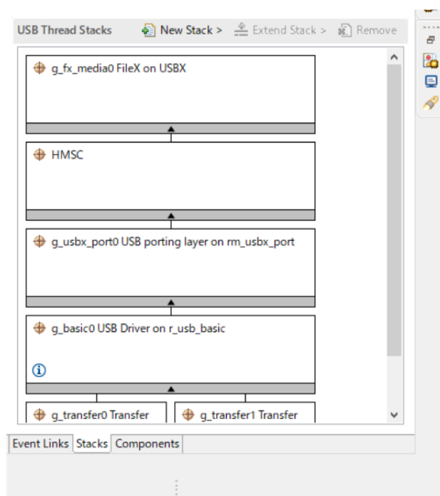
Figure 183: FileX on USBX Stack
