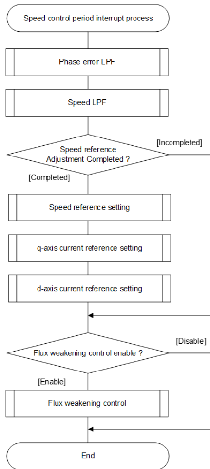
Figure 271: Speed control process
