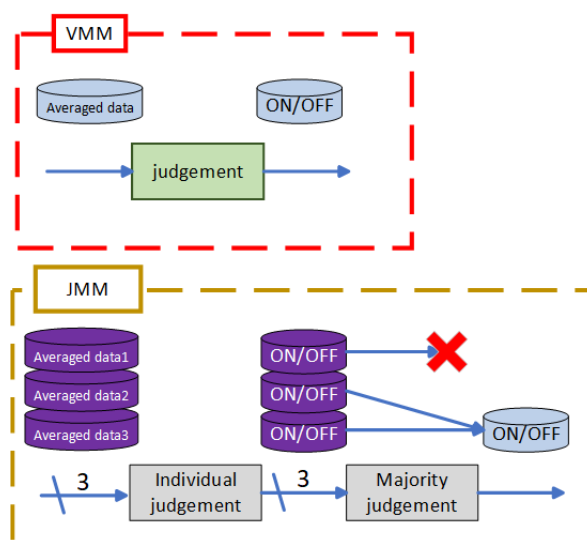
Figure 167: Data flow comparison of VMM and JMM
