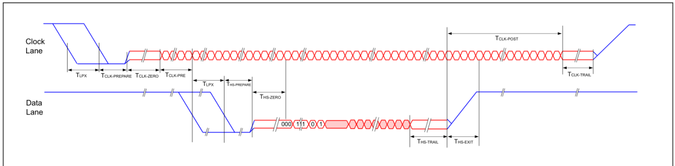
Figure 230: High-Speed data transmission in normal mode
