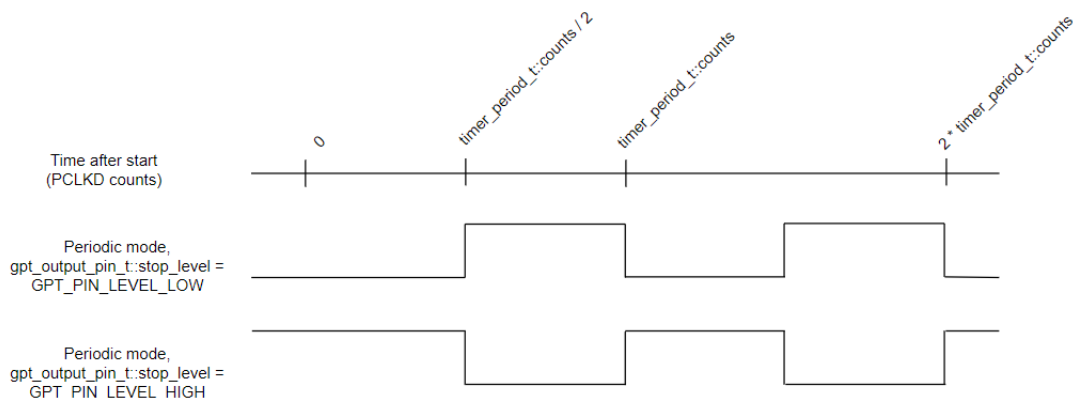
Figure 303: GPT Periodic Output
