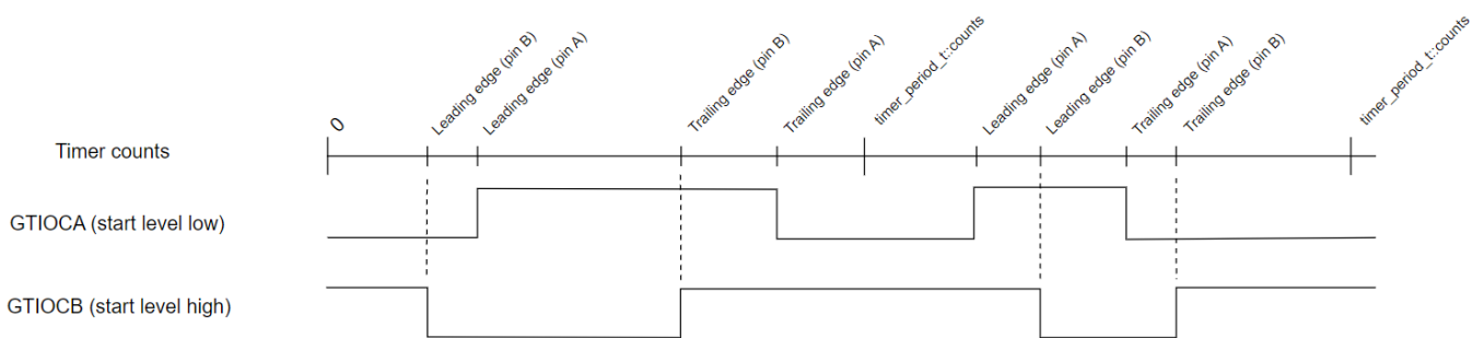
Figure 301: GPT One-Shot Pulse Output (without dead time)
