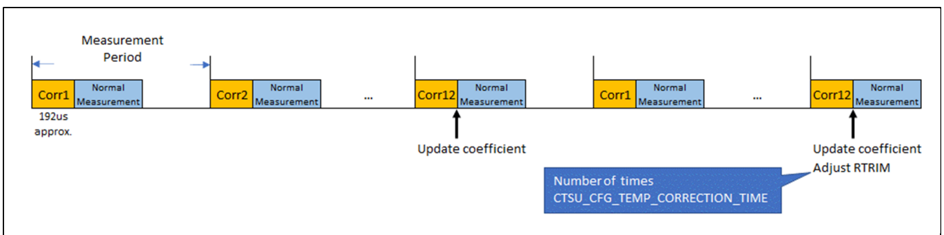
Figure 166: Temperature Correction Measurement Timing Chart
