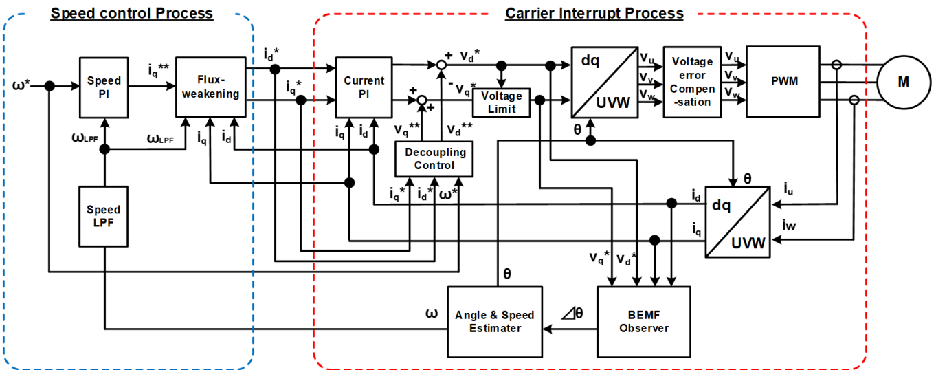
Figure 256: Block diagram of sensorless vector control (PI feedback loop)
