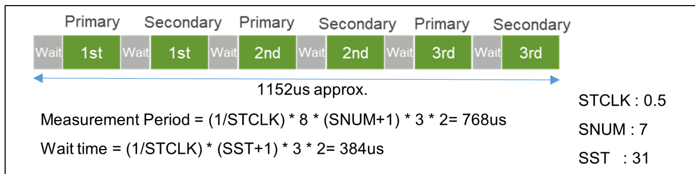
Figure 164: Mutual-capacitance Measurement Period
