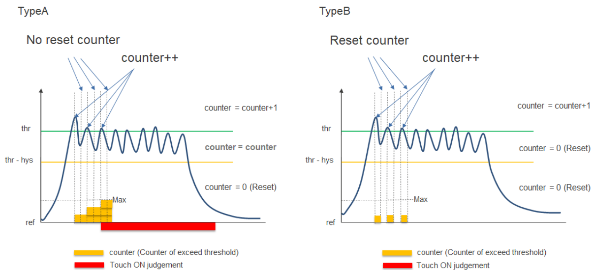
Figure 169: Chattering suppression type
