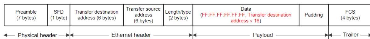
Figure 289: Magic Packet Frame Format Image
