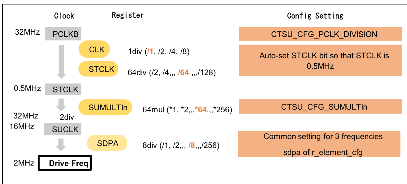
Figure 160: Drive Frequency Settings
