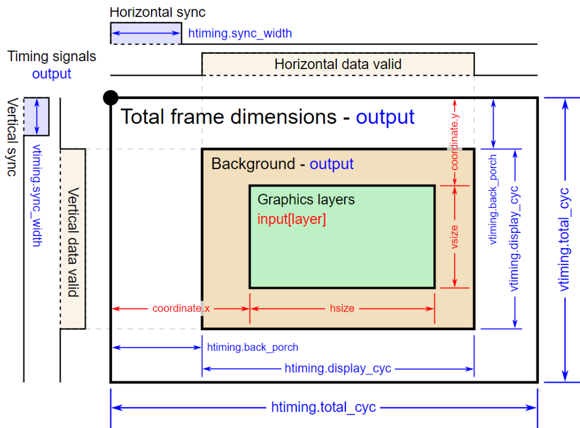
Figure 227: GLCDC layers and timing
