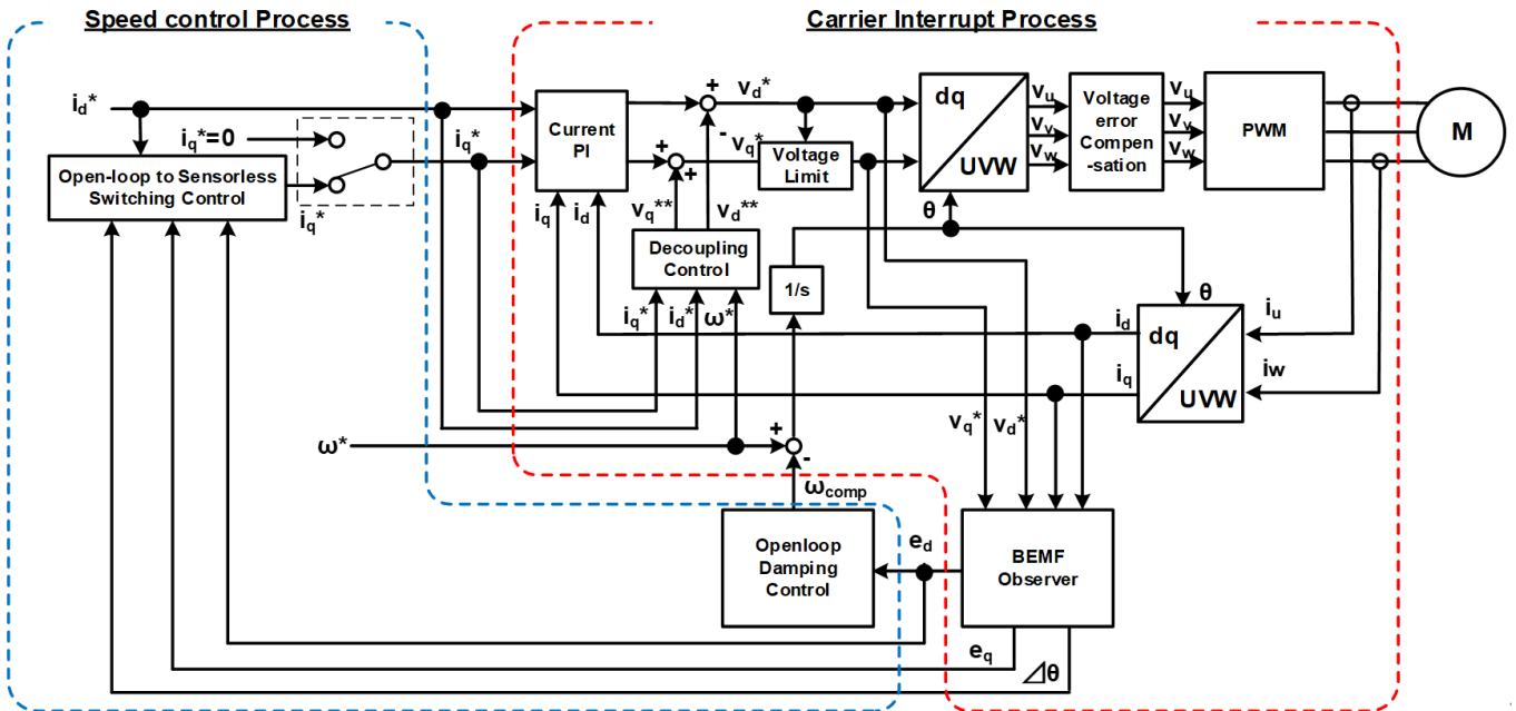
Figure 255: Block diagram of sensorless vector control (open-loop)
