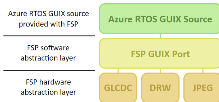
Figure 226: Azure RTOS GUIX Port Block Diagram
