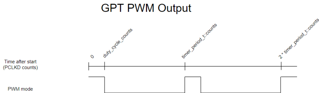
Figure 304: GPT PWM Output
