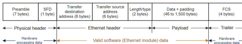
Figure 287: Frame Format Image
