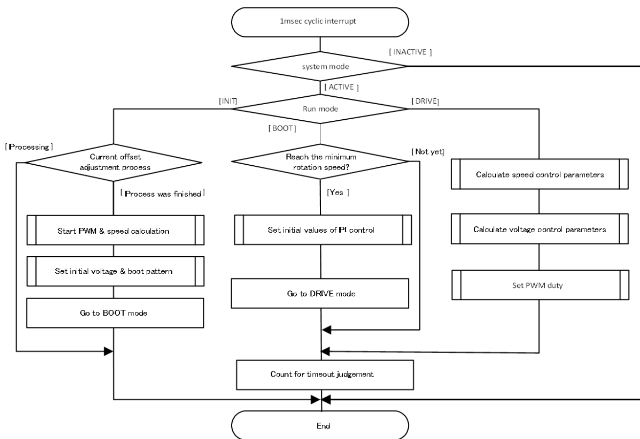
Figure 242: Speed control process of 120-degree with hall sensor
