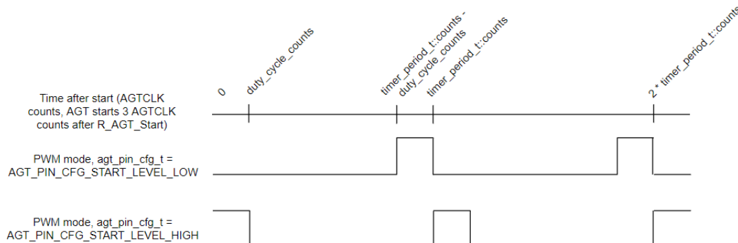
Figure 309: AGT PWM Output
