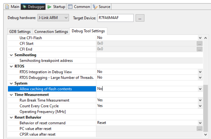
Figure 293: Debug Configuration
