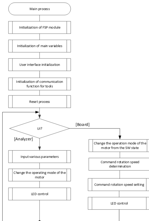
Figure 249: Main process
