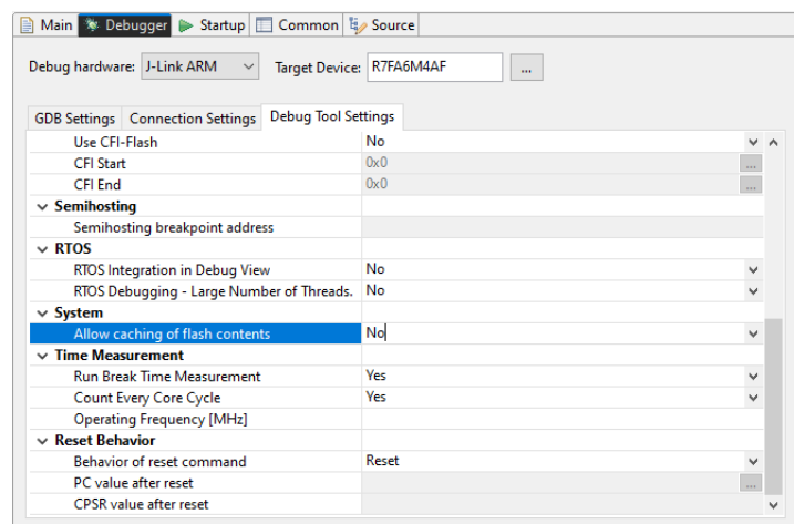
Figure 292: Debug Configuration
