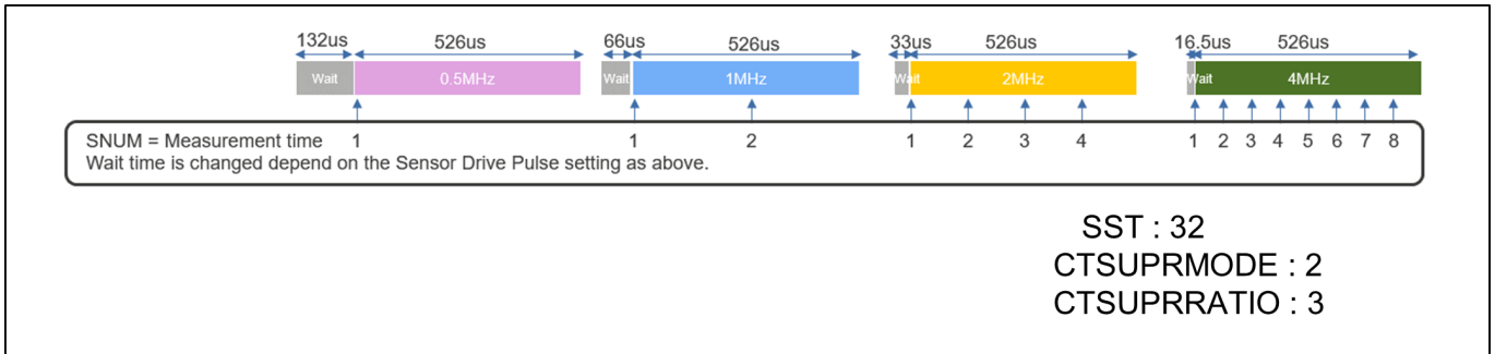
Figure 162: Self-capacitance Measurement Period (CTSU1)
