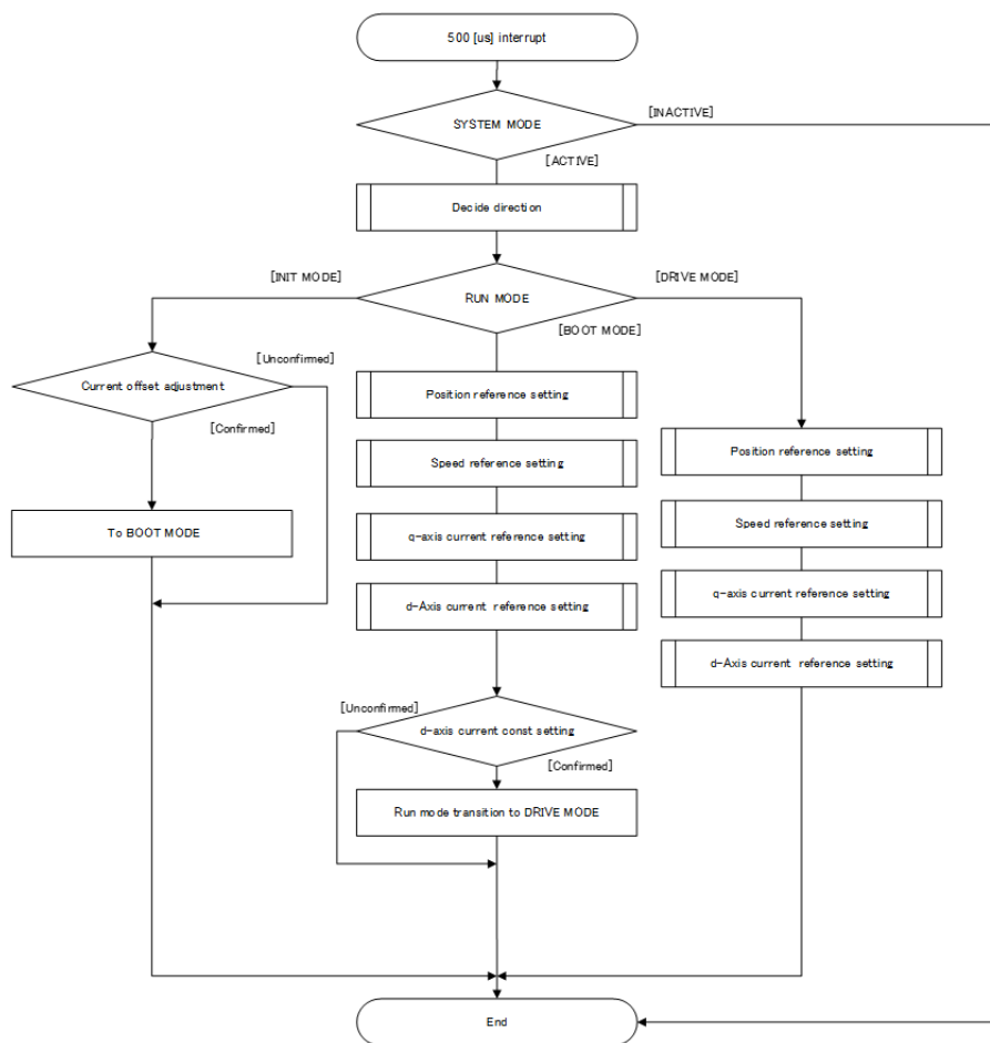
Figure 251: Speed control process
