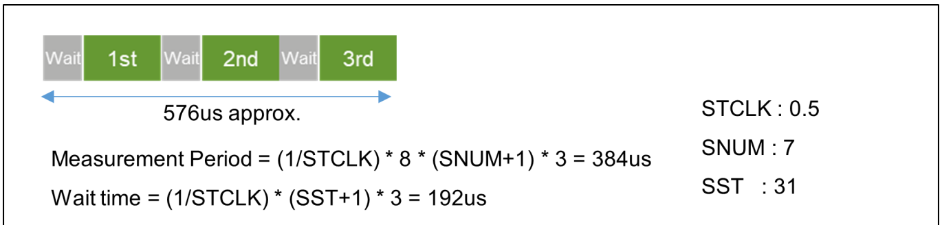
Figure 163: Self-capacitance Measurement Period (CTSU2)
