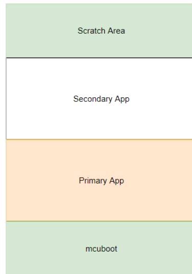
Figure 154: MCUboot Memory Map
