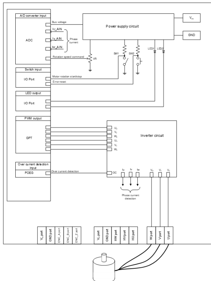
Figure 254: Example of target hardware of motor sensorless module
