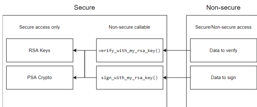
Figure 291: PSA Crypto Non-secure callable example
