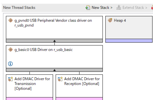
Figure 225: USB Peripheral Vendor Class Stack
