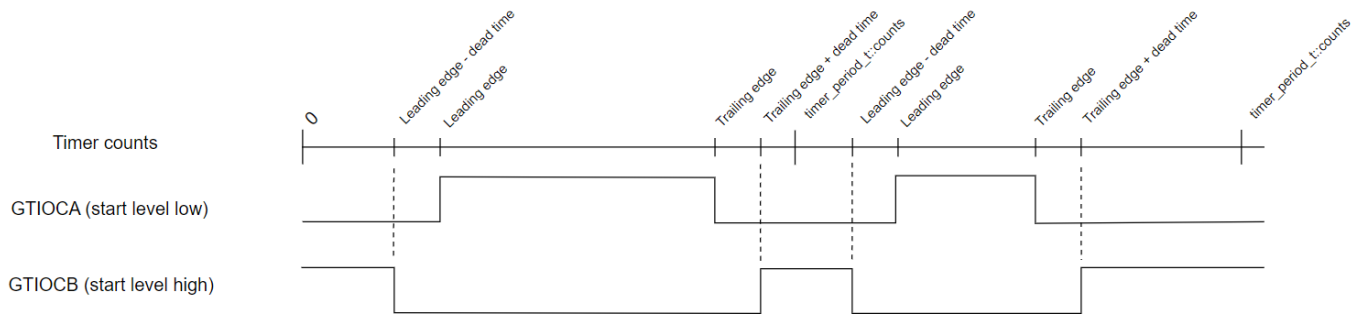
Figure 302: GPT One-Shot Pulse Output (with dead time)
