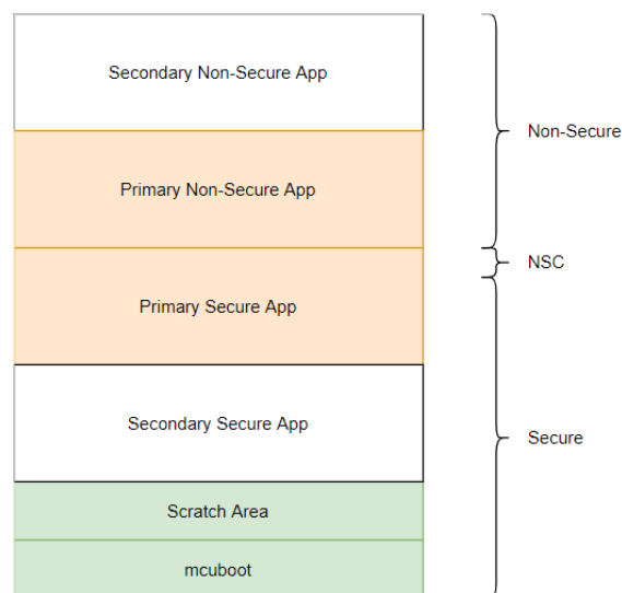
Figure 155: MCUboot Memory Map (TrustZone)
