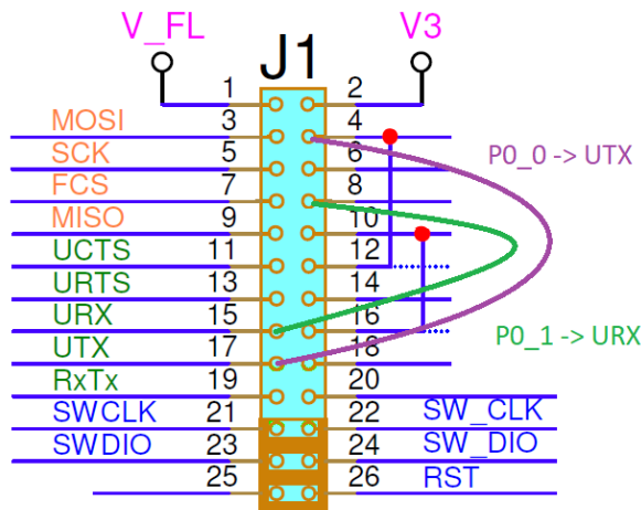
Figure 42. Enable two-wire UART with jumper wires
