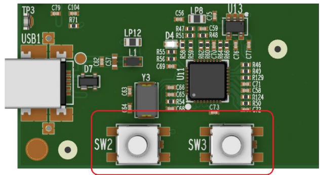
Figure 52. Push buttons position on the DA1453x Pro-motherboard
