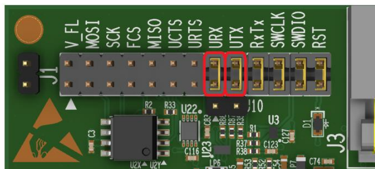
Figure 40. Two-wire UART configuration jumpers position
