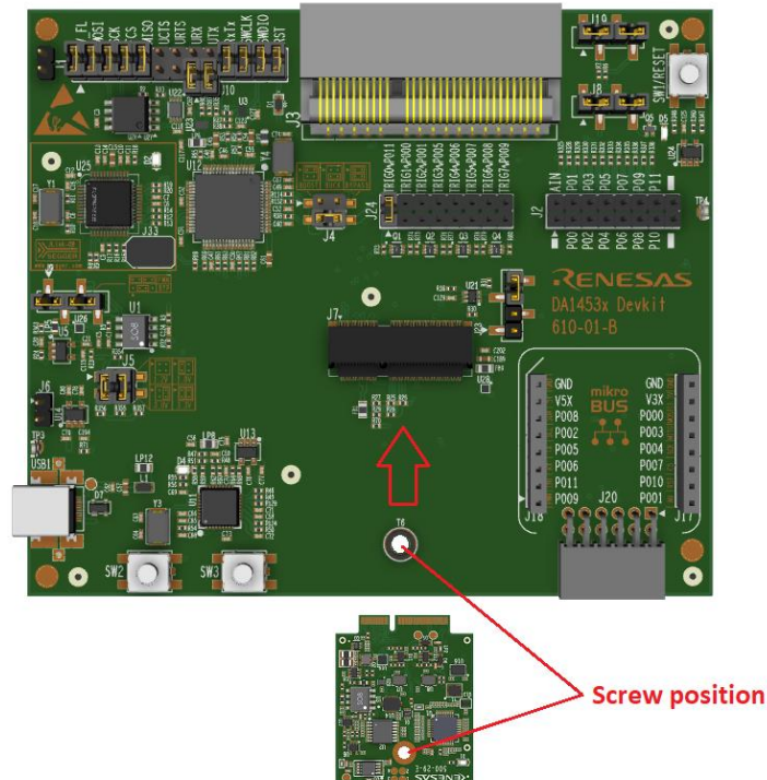
Figure 19. How to mount the PMM2 on the DA1453x Pro-motherboard
