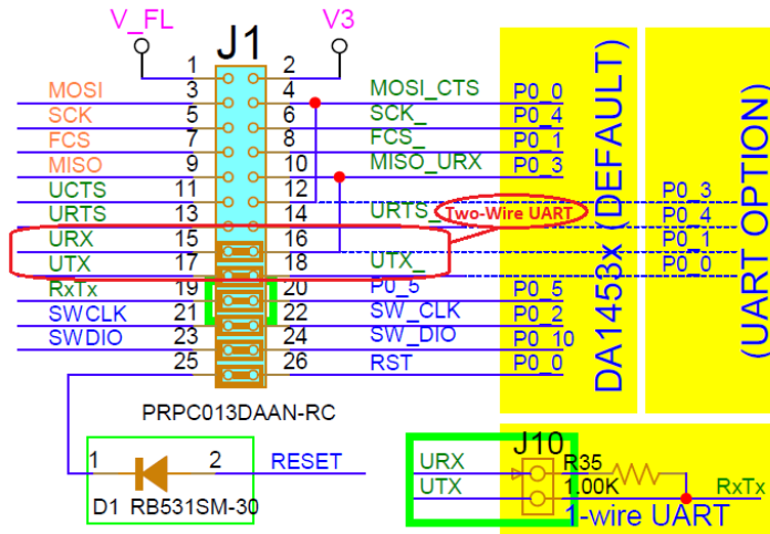
Figure 39. Two-wire UART jumper configuration at J1 header on Pro-motherboard
