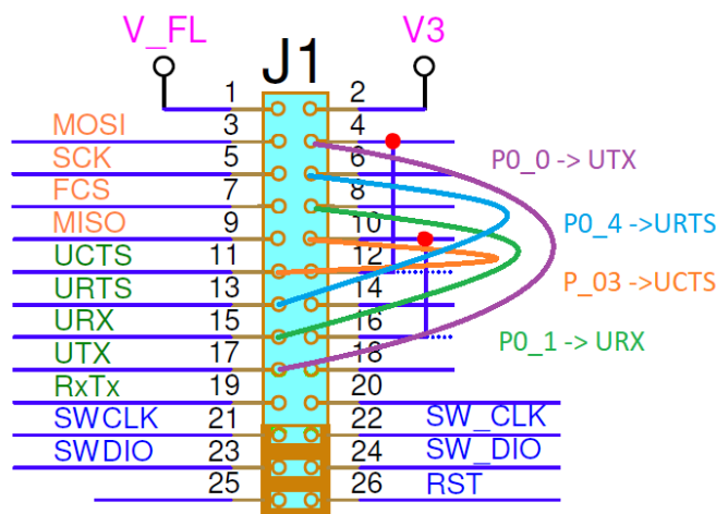
Figure 46. Enable two-wire UART with jumper wires
