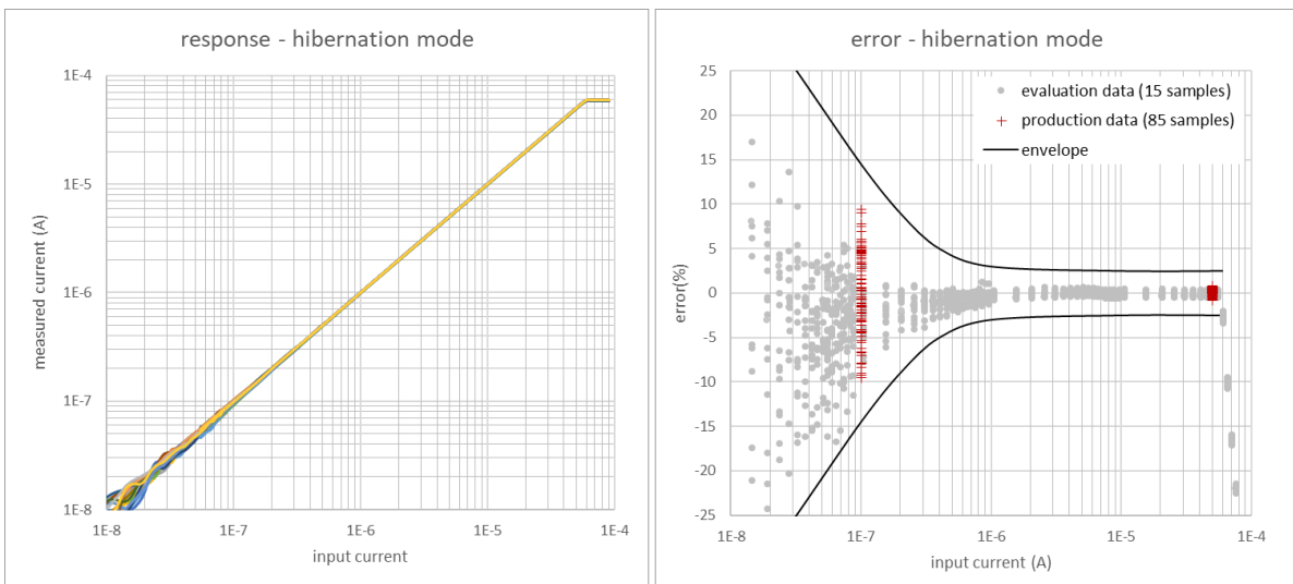
Figure 68. Hibernation mode (100 \mu A to 60 \mu A at 3.3 V) data after offset calibration
