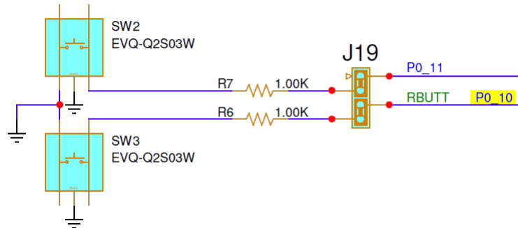
Figure 51. Push buttons SW2 and SW3
