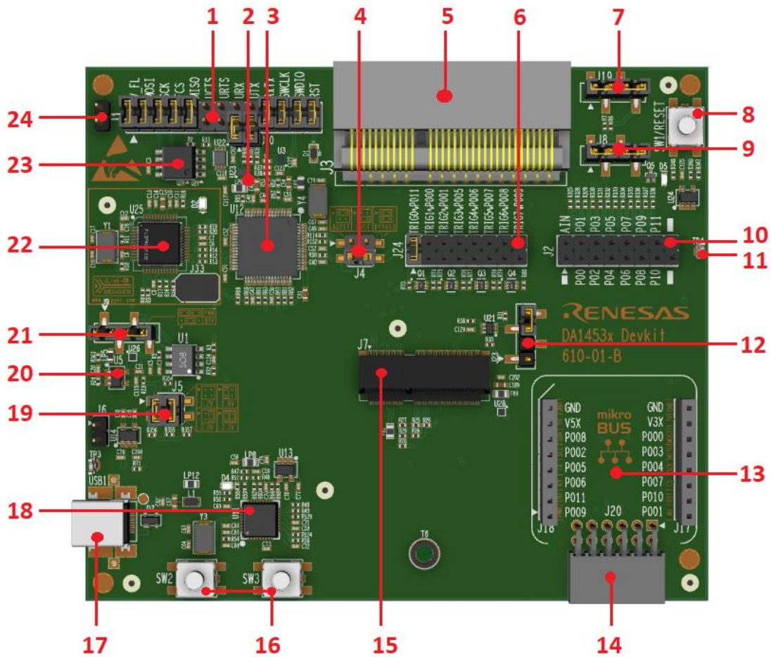
Figure 14. Pro-motherboard (610-01-A)
