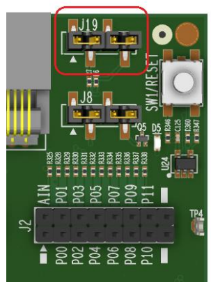
Figure 53. J19 header position on the DA1453x Pro-motherboard
