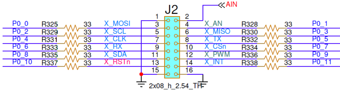
Figure 49. J2 schematic
