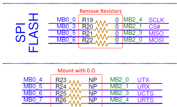
Figure 45. Enable two-wire UART on Pro-daughterboard
