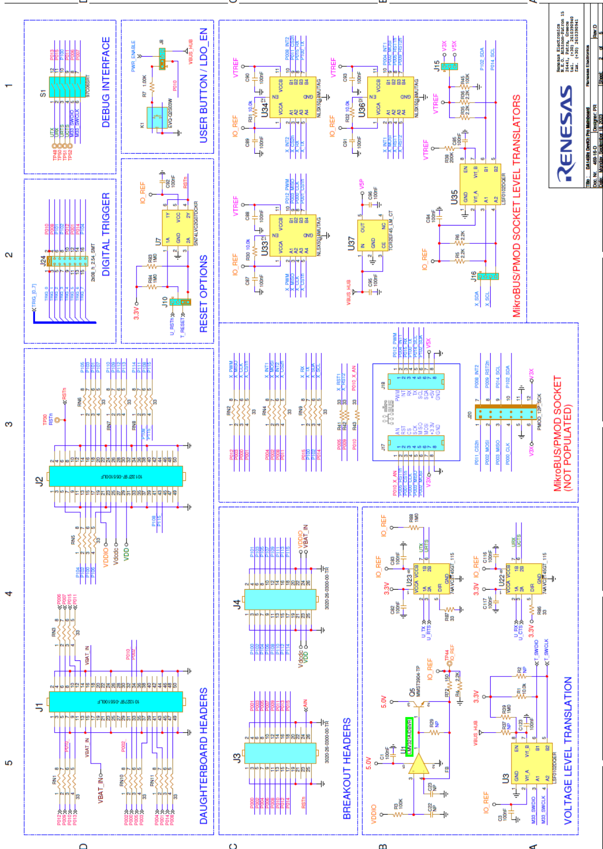
Figure 39. DA1459x Pro-Motherboard schematic, connectivity, and level translators
