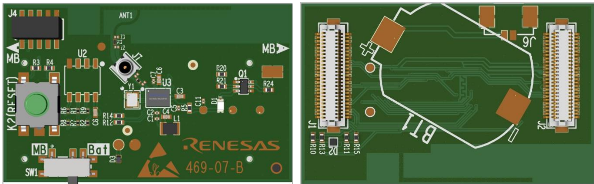
Figure 16. SW1 (left), available battery sockets on the bottom side of the daughterboards (right)
