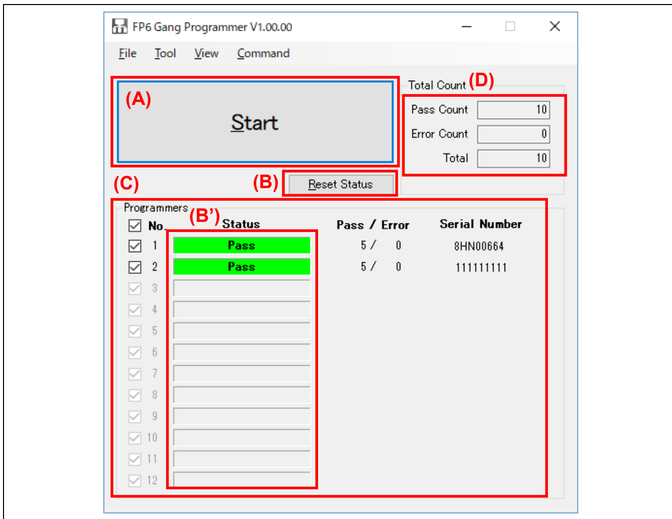
Figure 5 Main Window
