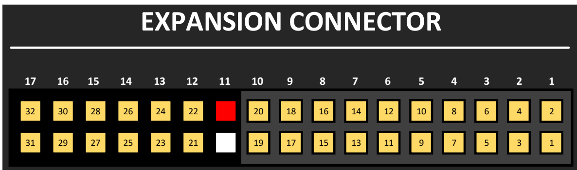
Figure 4: GreenPAK Expansion Connector Pinout
