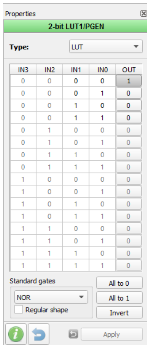
Figure 19: Look Up Table Properties Configured as a NOR Gate
