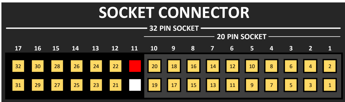
Figure 3: GreenPAK Socket Connector Pinout
