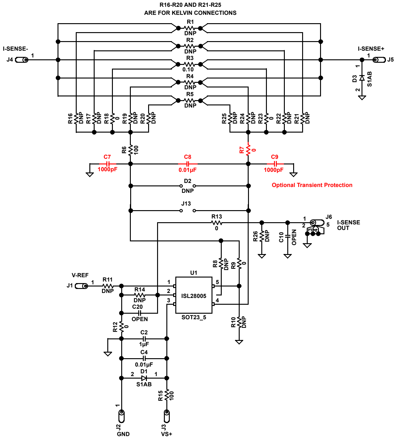
Figure 4. ISL28005xEVAL1Z Schematic Diagram
