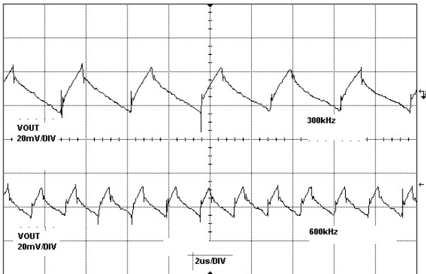
FIGURE 5. OUTPUT RIPPLE
