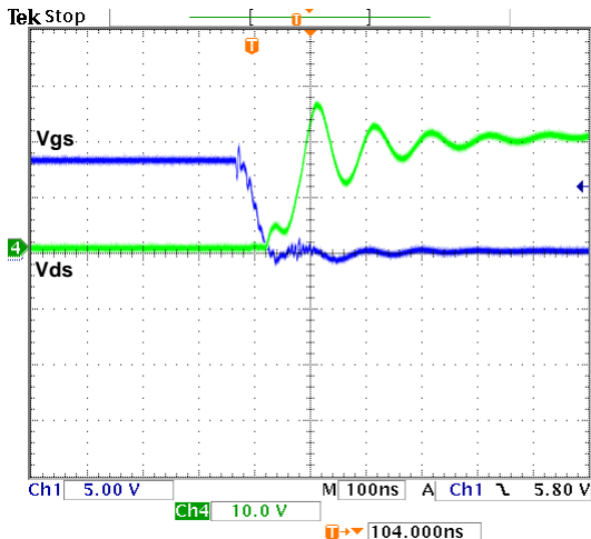
FIGURE 13. Q4 TURN OFF, NO LOAD
