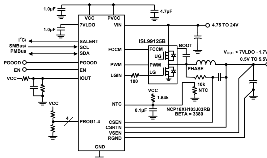
FIGURE 1. ISL68201-99125DEMO1Z SIMPLIFIED SCHEMATIC
