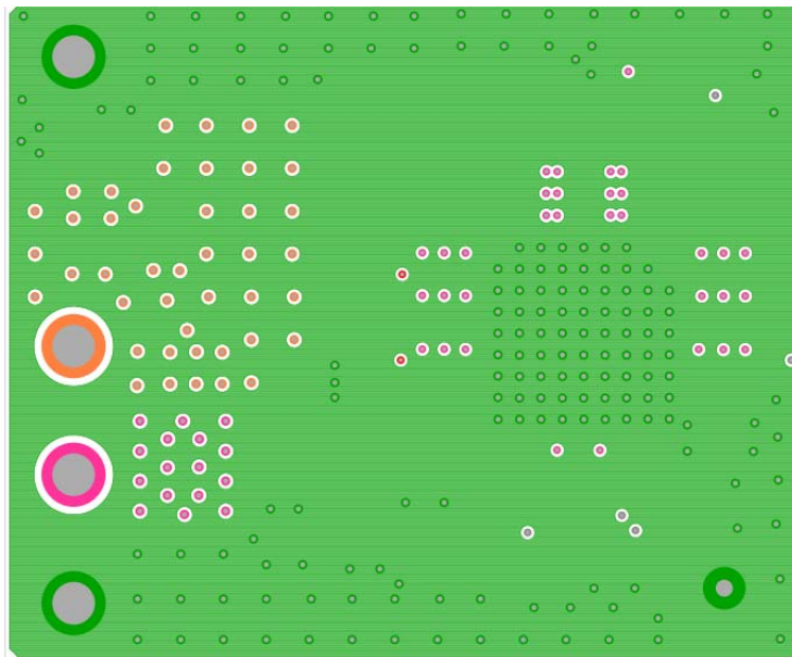
Figure 8. Layer 3
