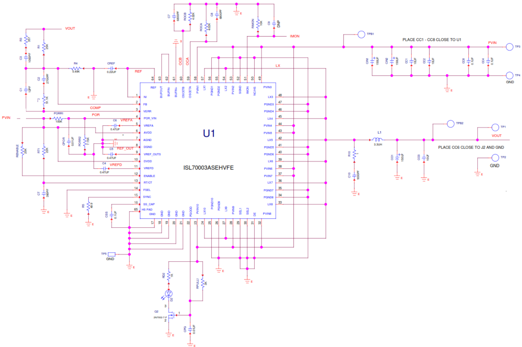
Figure 4. ISL70003ASEHEV2Z Schematic
