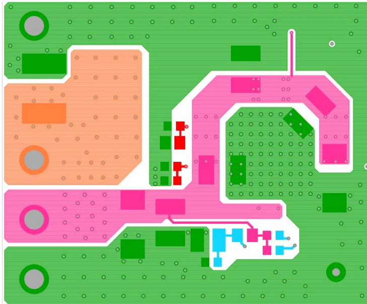
Figure 9. Bottom Component Layer
