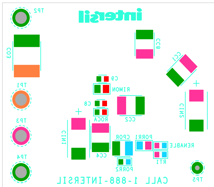
Figure 10. Bottom Silkscreen Layer
