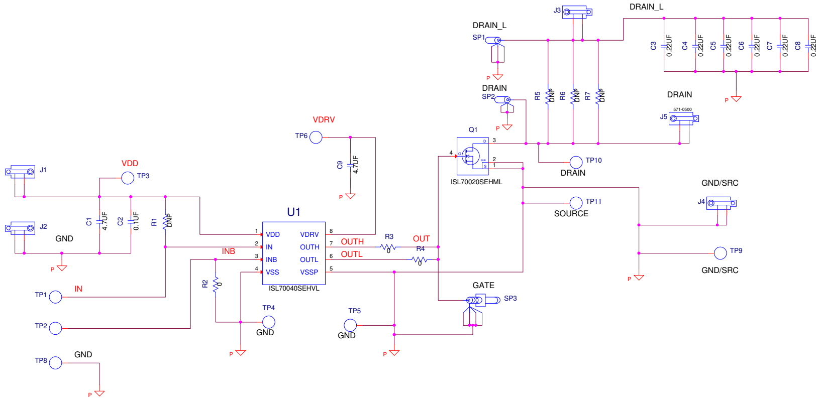
Figure 4. ISL70040SEHEV5Z Schematic
