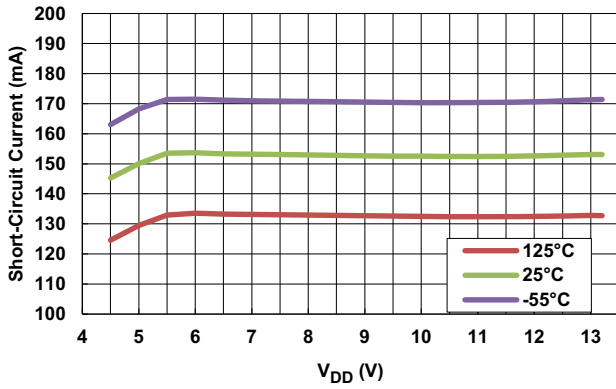
Figure 9. V DRV Short-Circuit Current vs Temperature
