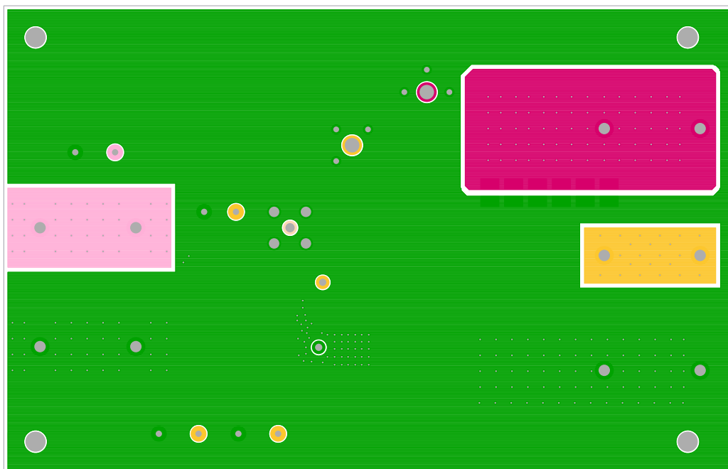
Figure 8. Bottom Layer
