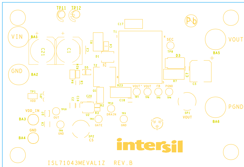
Figure 5. Top Silkscreen
