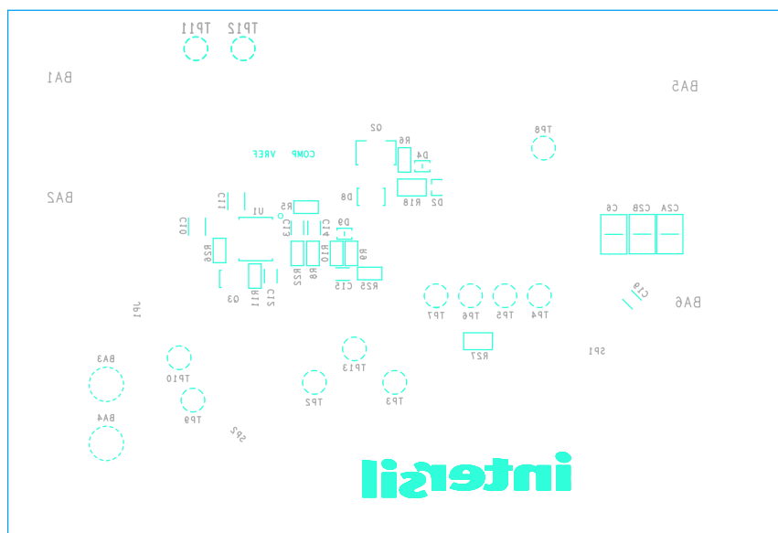
Figure 6. Bottom Silkscreen
