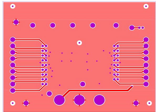
Figure 7. Bottom Layer
