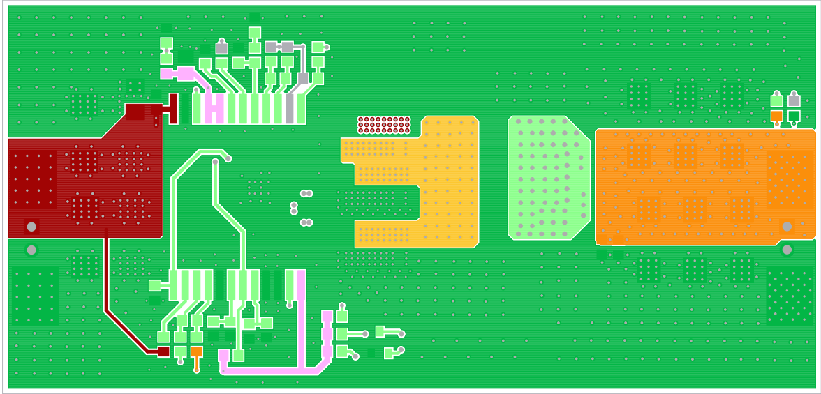
Figure 16. Bottom Layer
