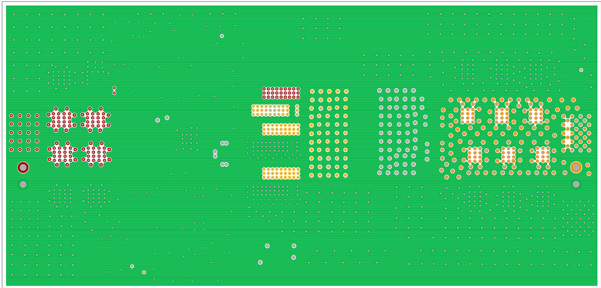
Figure 13. Layer 5
