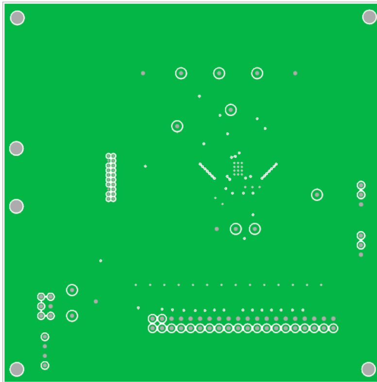
FIGURE 17. INTERNAL (LAYER 2)
