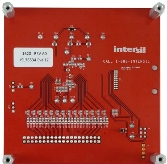
FIGURE 2. ISL76534EVAL1Z BOTTOM VIEW
