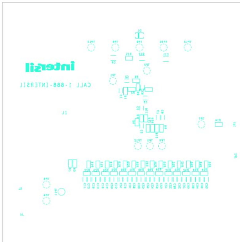
FIGURE 20. SILKSCREEN BOTTOM
