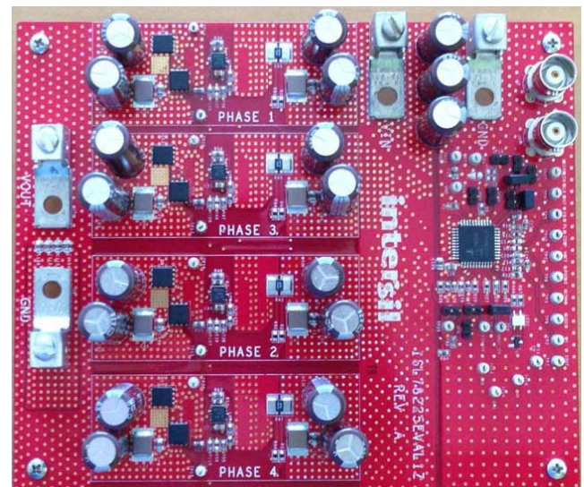
FIGURE 1. PHOTO OF ISL78225EVAL1Z EVALUATION BOARD
