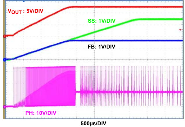
FIGURE 18. SOFT-START (NON-PREBIASED): DE MODE, V_{IN} = 36V , V_{OUT} = 12V , I_{OUT} = 0A , L = 4.7\mu H , C_{OUT} = 98\mu F , f_{SW} = 300kHz
