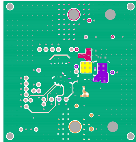
FIGURE 8. LAYER 3
