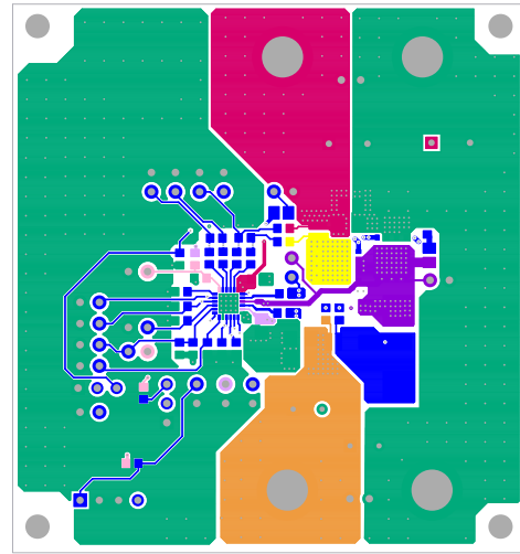
FIGURE 6. TOP LAYER
