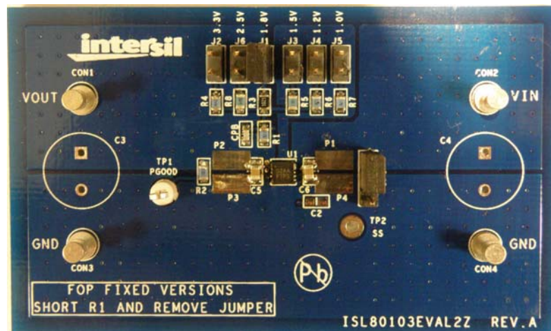
FIGURE 1. ISL80103EVAL2Z
