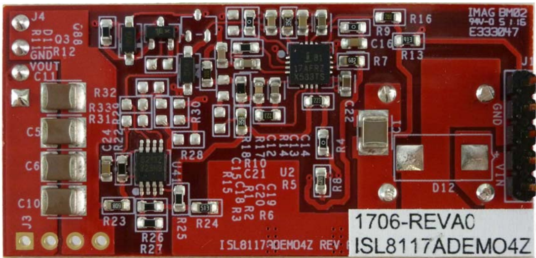
Figure 5. Bottom View
