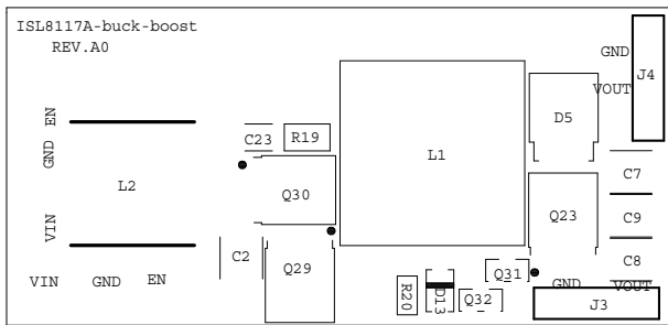
Figure 7. Assembly Top
