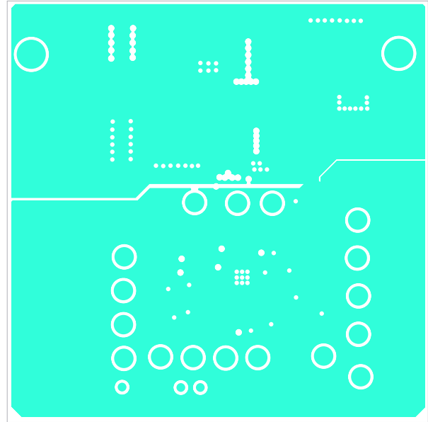
FIGURE 10. THIRD LAYER
