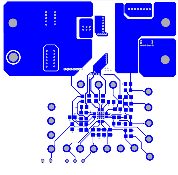
FIGURE 8. TOP LAYER
