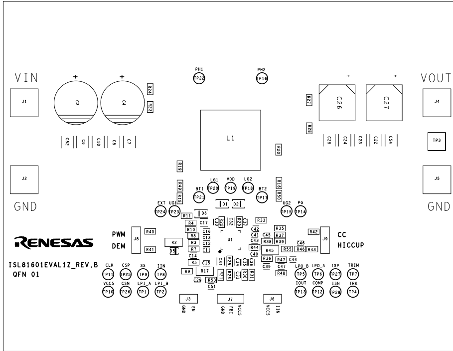
Figure 8. Silkscreen Top
