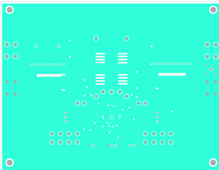
Figure 11. Third Layer
