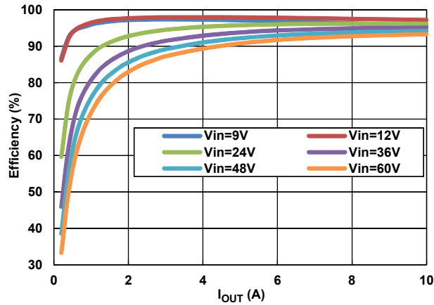
Figure 14. Efficiency, CCM
