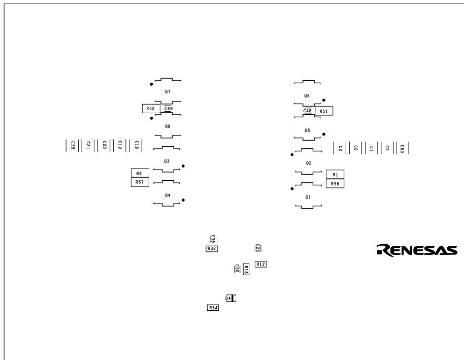
Figure 13. Silkscreen Bottom
