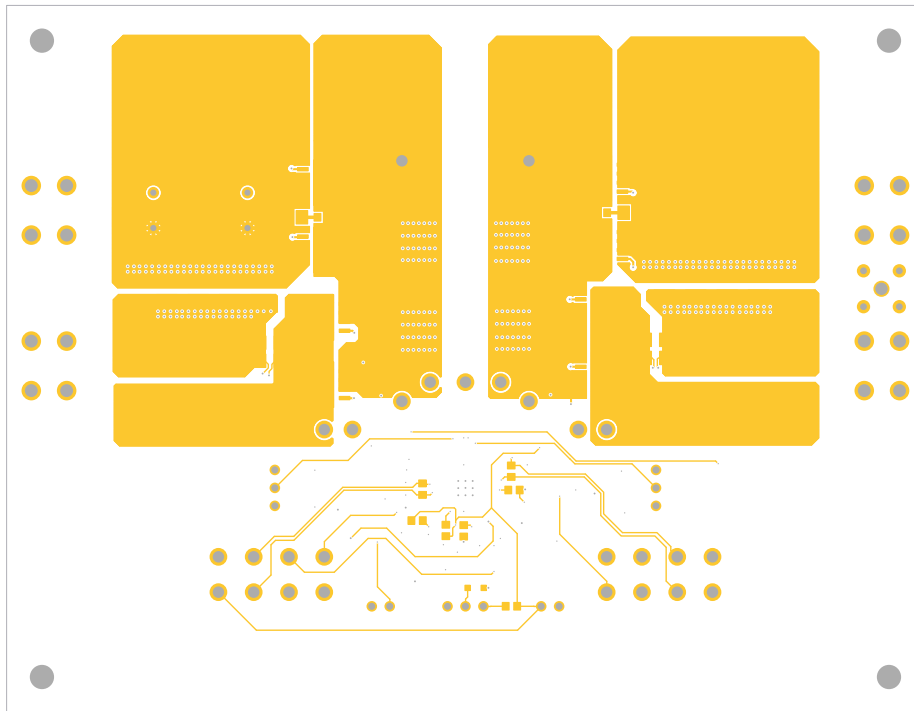
Figure 12. Bottom Layer
