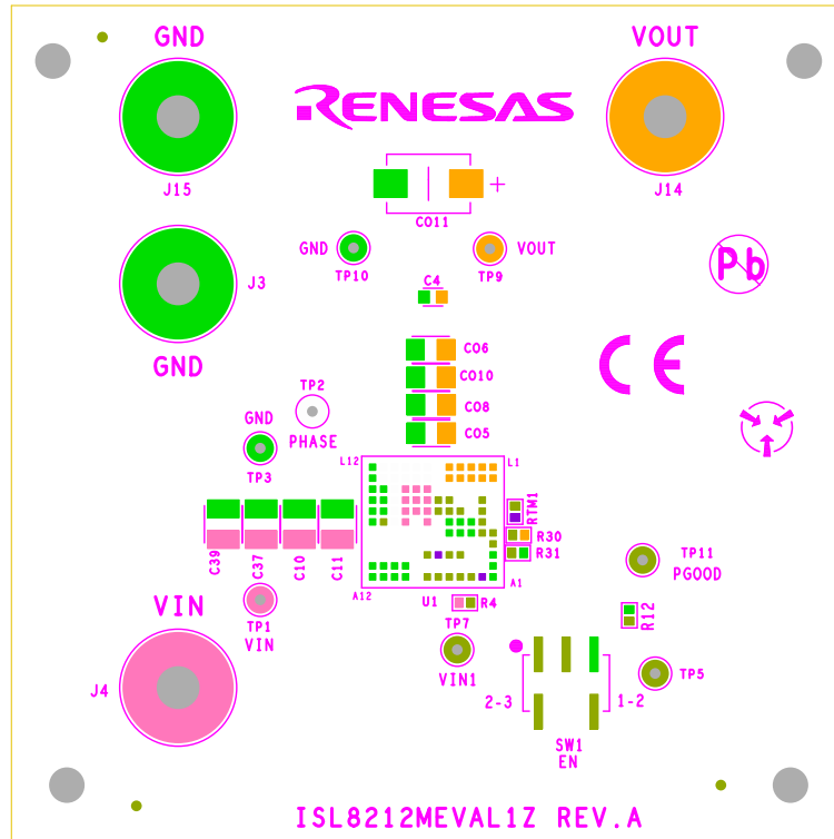
Figure 7. Silkscreen Top
