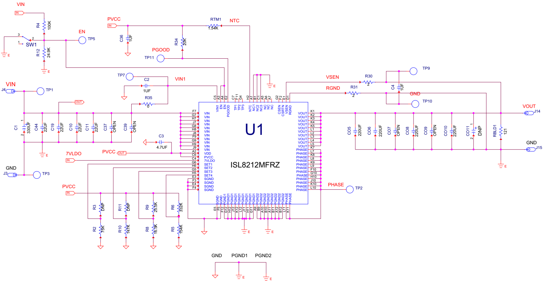
Figure 6. Schematic
