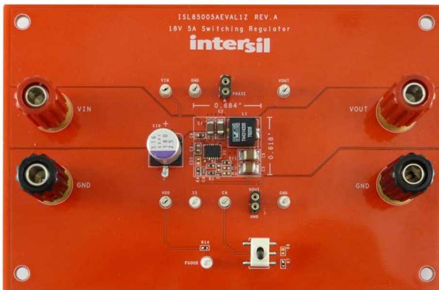
FIGURE 3. TOP VIEW
