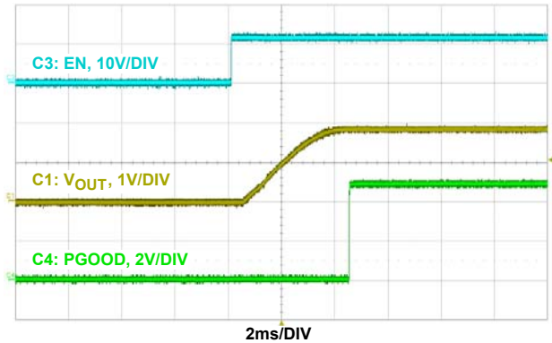
FIGURE 20. START-UP BY EN ( V_{IN} = 12V , V_{OUT} = 1.8V AT 0A, 600kHz, DCM)
