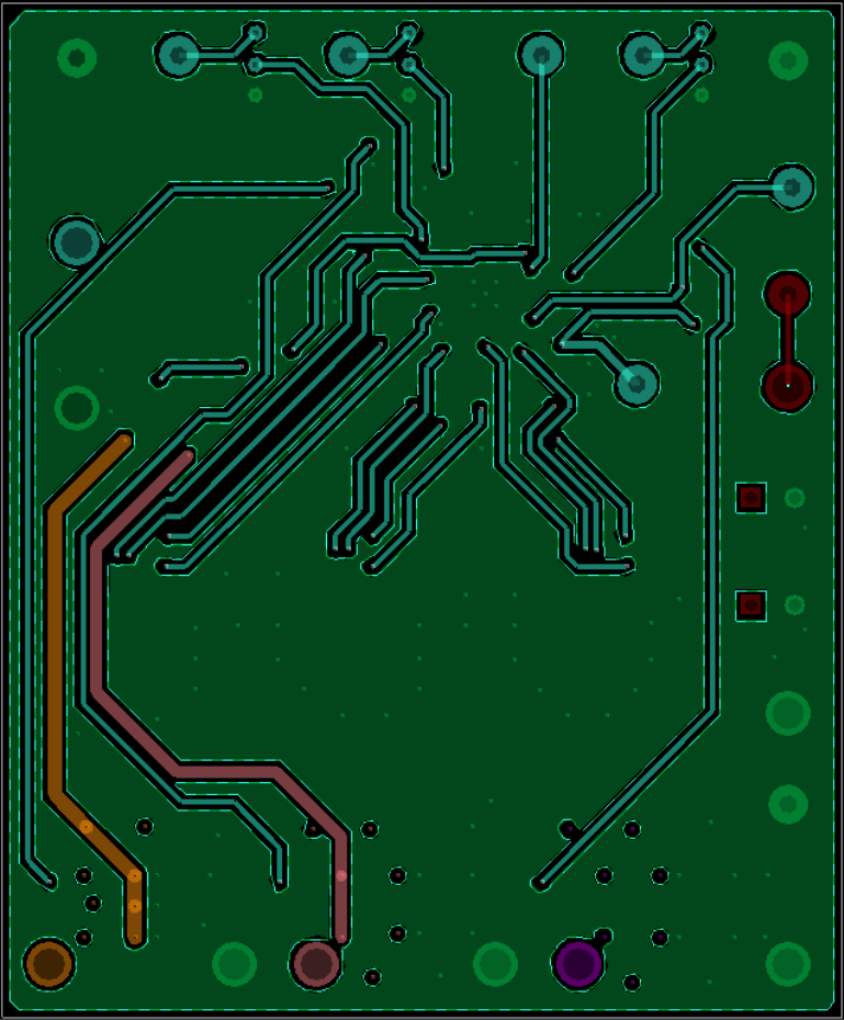
FIGURE 20. THIRD LAYER
