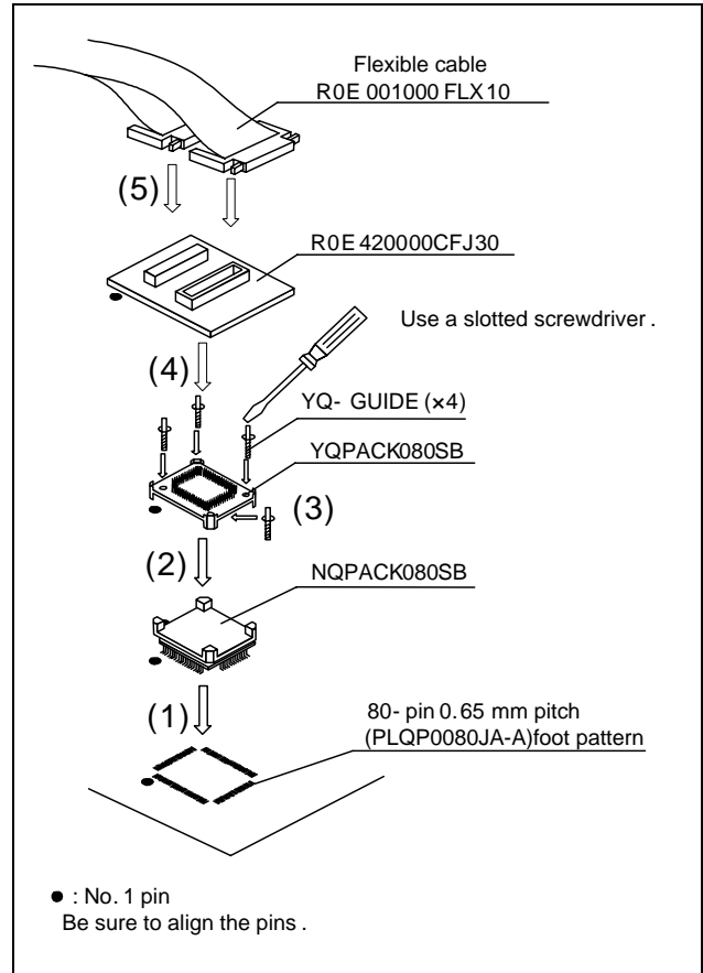
Figure 3 Connection procedure of the R0E420000CFJ30
