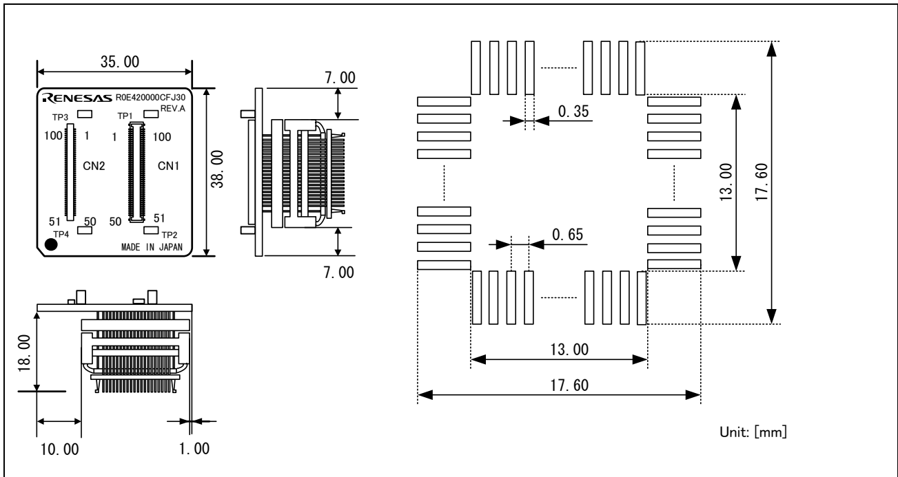
Figure 4 External dimensions and a sample foot pattern of the R0E420000CFJ30
