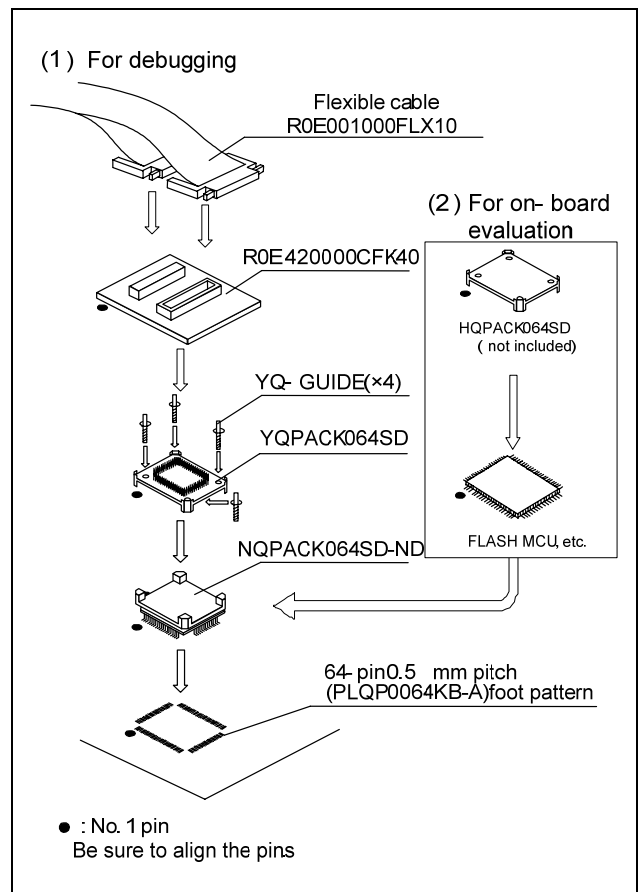
Figure 2 Usage of the R0E42000CFK40
