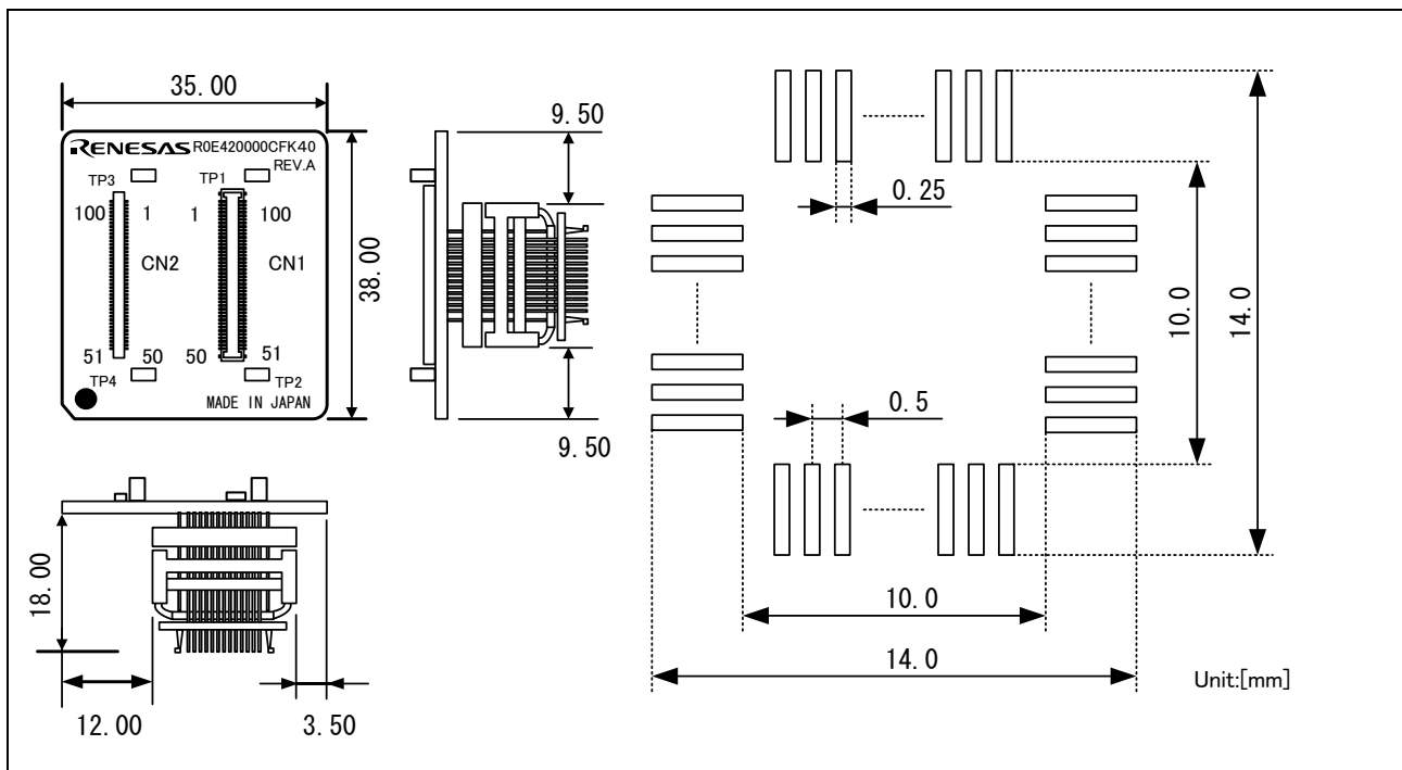
Figure 4 External dimensions and a sample foot pattern of the R0E420000CFK40
