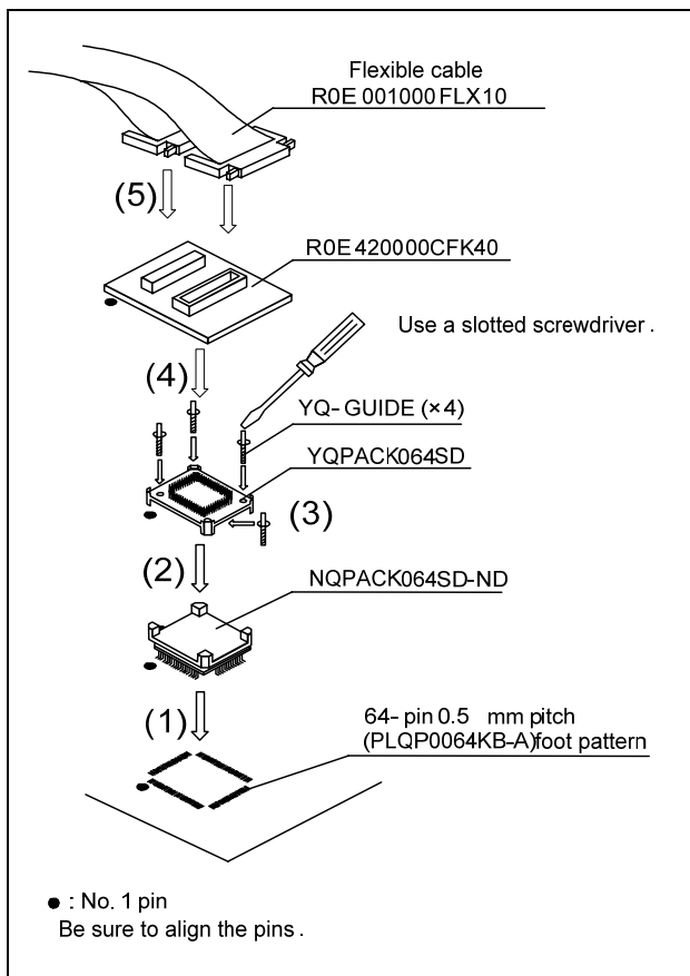
Figure 3 Connection procedure of the R0E420000CFK40
