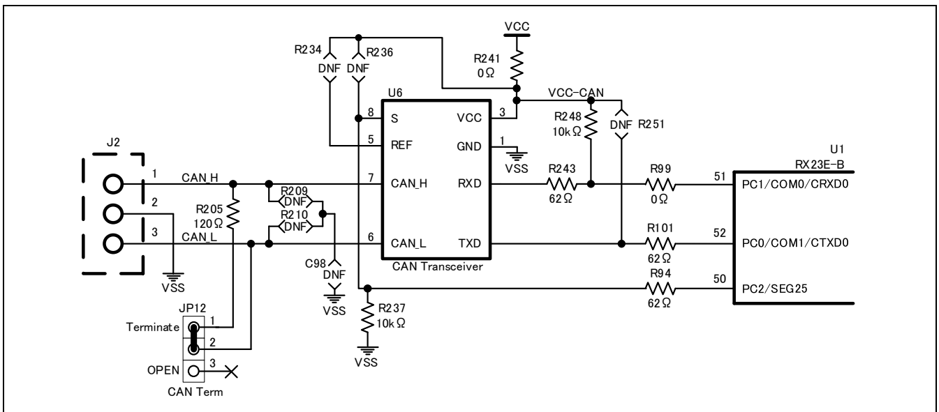
Figure 3.4 CAN Communication Circuit
