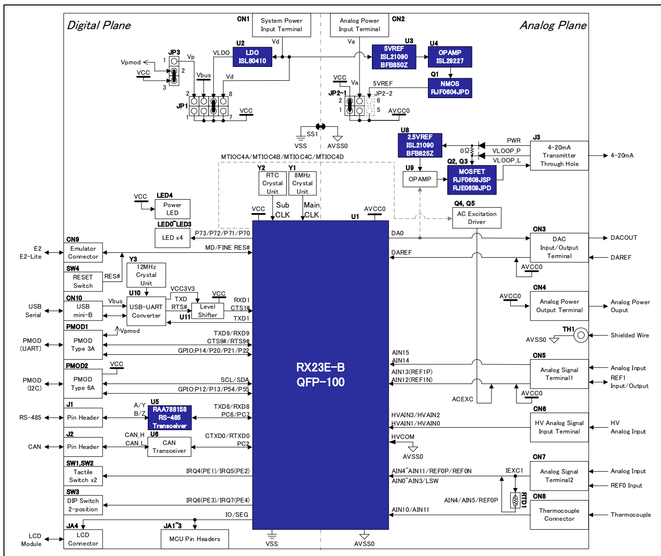
Figure 1.1 RSSKRX23E-B Board System Block Diagram
