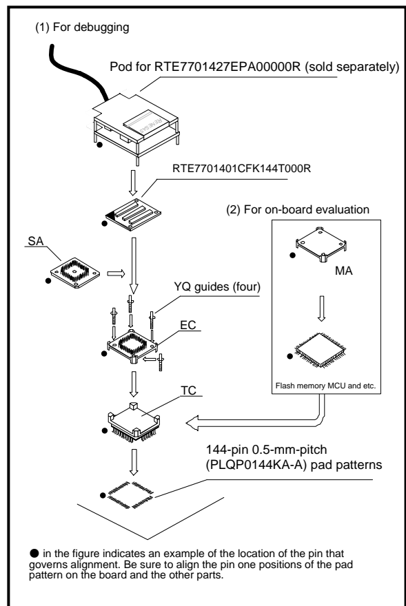
Figure 2 Usage of the RTE7701401CFK144T000R
