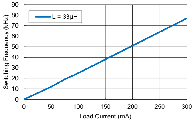
Figure 3. Switching Frequency (VIN = 24V) vs. Load Current
